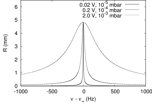
Figure 5.14 – Distance of the ion from the trap center, R , as a function of excitation frequency for three different excitation amplitudes U_d and buffer gas pressures. All plots are for an excessively long excitation time of 10 s.
