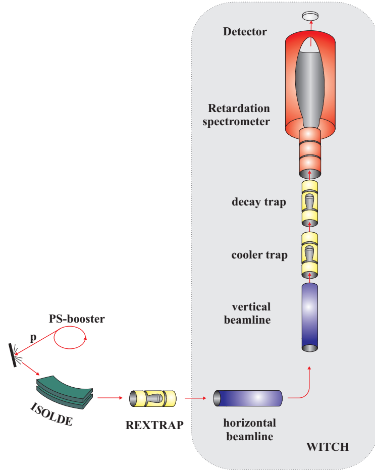
Figure 2.1 – Schematic overview of the WITCH setup and its environment. Radioactive ions received from ISOLDE are first cooled and bunched in REXTRAP before they are passed on to the WITCH experiment. Here they are decelerated and then injected into the first of two Penning traps. After cooling and mass selective purification the ions are transferred and stored in the second Penning trap which serves as scattering free source for the experiments. The energy of the recoiling ions leaving this trap is probed in the retardation spectrometer before the ions are detected in the MCP ion detector.
