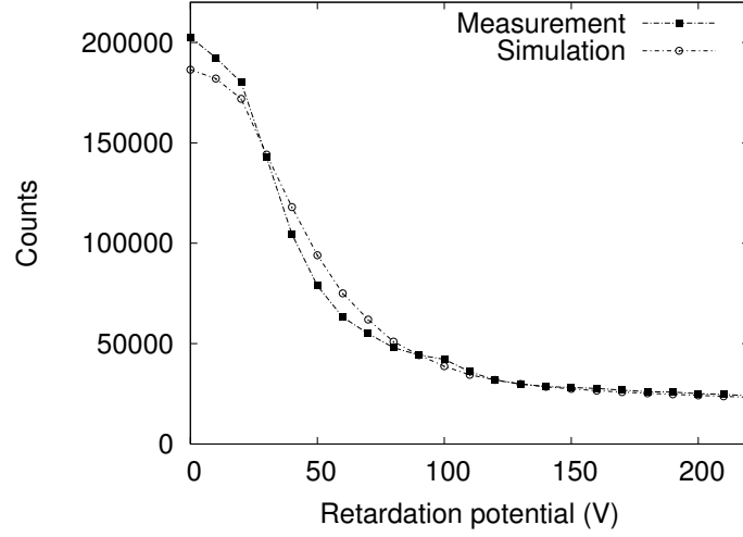
Figure 8.18 – Best fit to the measured recoil spectrum of Fig. 8.13, when omitting the higher charge states and only taking into account the \beta^- charge state distribution.
