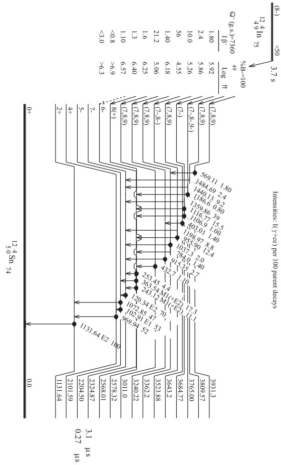
Figure C.2 – Complete decay scheme of ^{124m}\text{In} (taken from Ref. [NNDC]).
