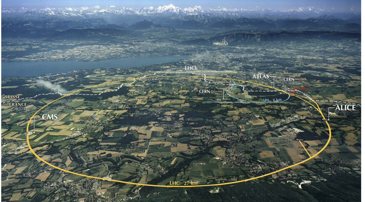
Figure 3.2: View of the Swiss/French countryside above the LHC tunnel. There are several places at which the tunnels have service access shafts. These are referred to as points. The ATLAS detector cavern is stationed at Point 1. The ALICE, CMS and LHCb detector caverns are housed at points 2,5, and 8, respectively. Image from [48].
