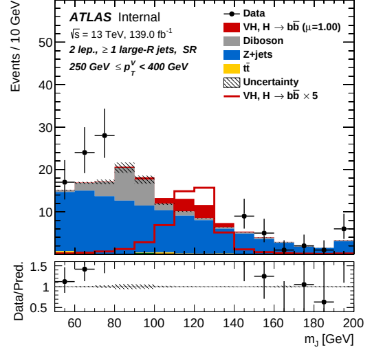
(a) m_J , 250 \text{ GeV} \leq p_T^V < 400 \text{ GeV} single- \mu trigger (b) m_J , 250 \text{ GeV} \leq p_T^V < 400 \text{ GeV} , E_T^{\text{miss}} trigger
