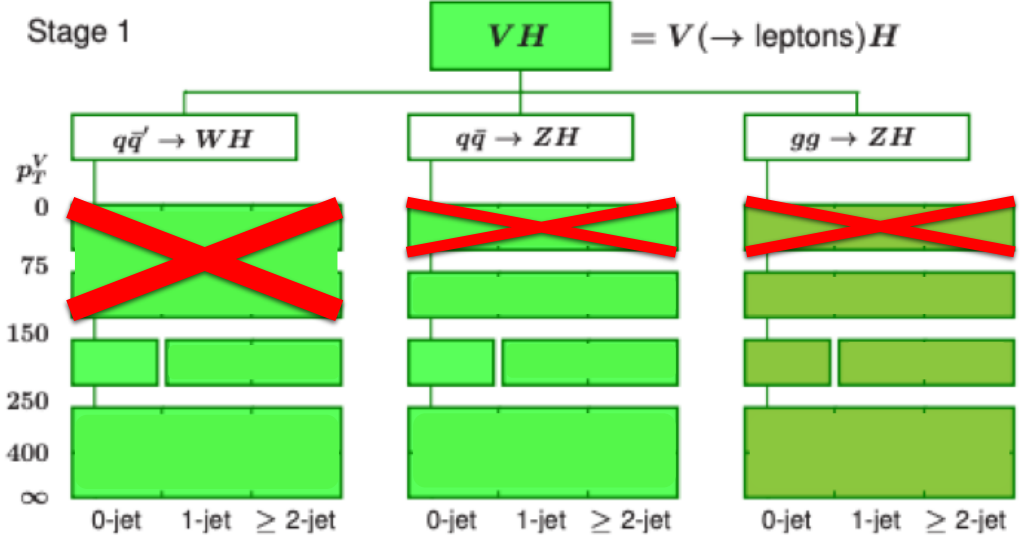
Figure 8.9: Modified Stage 1 STXS Binning Proposed Analysis regions for the 2019 STXS VH , H \rightarrow b\bar{b} analysis. Image is a modified version of the one from [143, p10].
