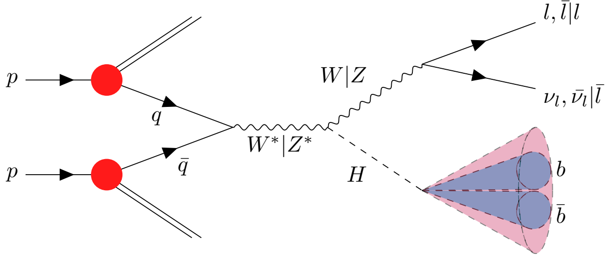
Figure 8.19: Feynman diagram showing the full Higgsstrahlung process of Higgs production at the LHC, and its decay into the final states of interest to the Boosted analysis. The purple cone is a representation of what a boosted signal event looks like. One large-radius fat jet with two objects tagged as b -jets inside it.
