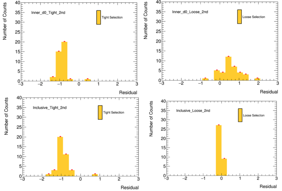
Figure 6.10: Histograms for the residuals of the ratio between data and MC for the average number of tracks against \mu after two rounds of outlier removal. Here the TightPrimary selection is referred to simply as ‘Tight’ Top left and top right, for the inner- d_0 TightPrimary and Loose selections respectively. The track selections for their respective inclusive tracks are below them.
