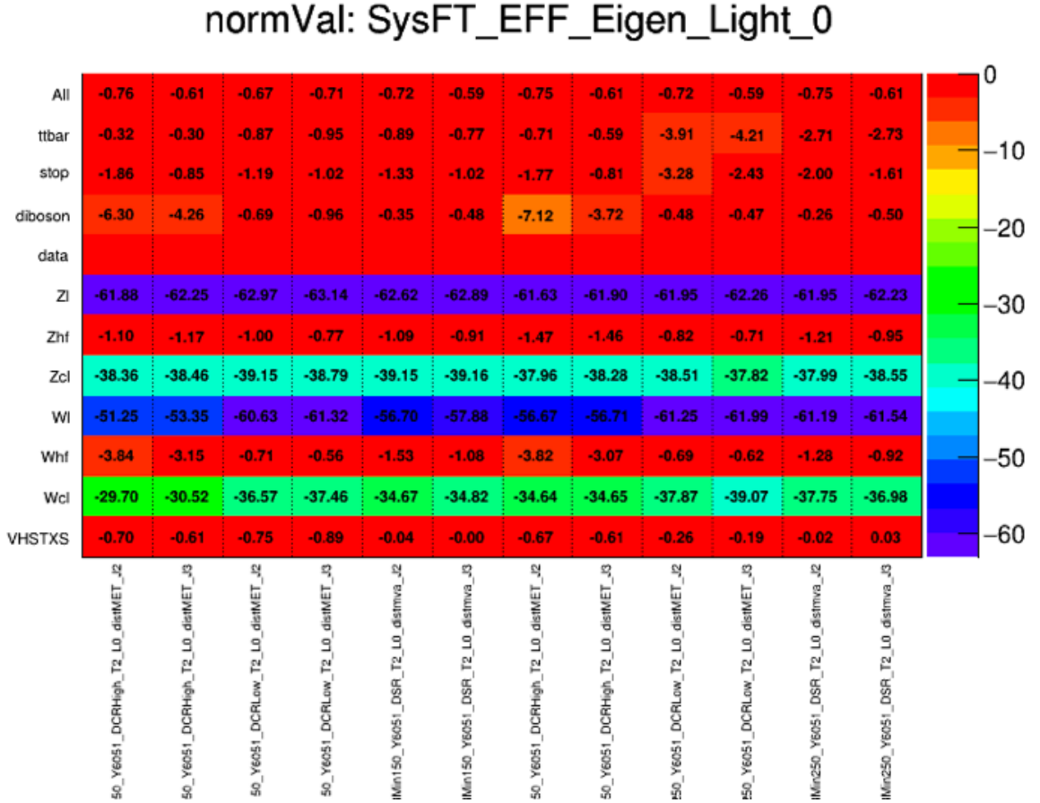
Figure 9.33: Normalisation factors from all the samples separately for each region in the 0L fit. Similarly for Figure 9.27, all the samples with prominent light jet contributions have a rough normalisation of 30% per light jet.
