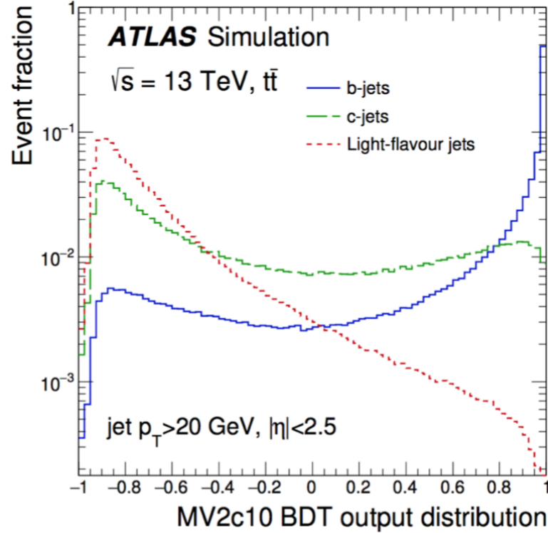
Figure 7.4: The MV2c10 output for b -jets (solid blue line), c -jets (dashed green line), and light-flavour jets (dotted red line) in simulated t\bar{t} events. Image from [135, p6].
