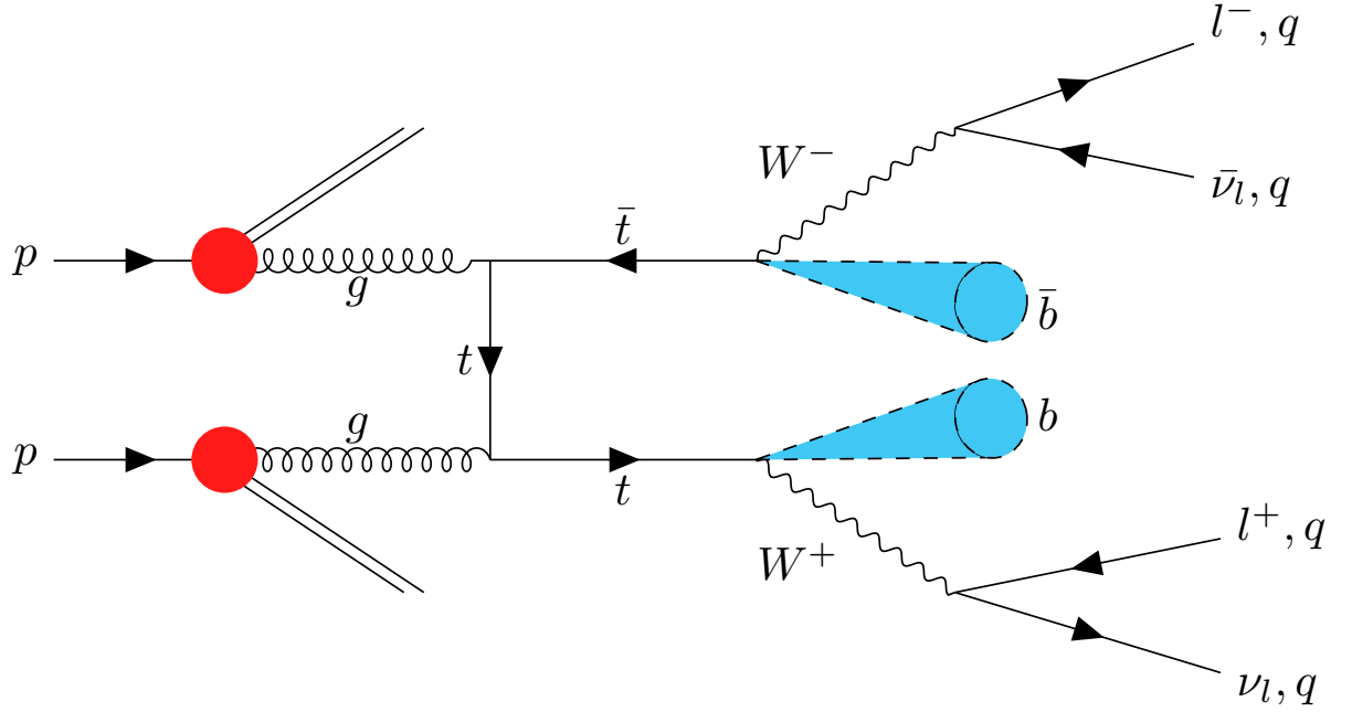
Figure 8.13: Feynman diagram showing how the t\bar{t} process enters the signal region.
