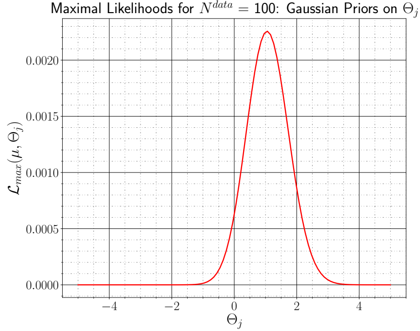
Figure 9.5: Plot of the likelihood value at different values for the number of sigma the systematic \theta_j is shifted. When N^{data}=100 and N^{exp}=80 , the systematic is pulled up by roughly 1\sigma .
