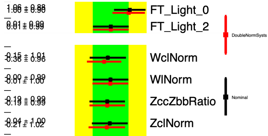
Figure 9.30: Relevant pulls that have changed in the fit where the normalisation factors have doubled (red) compared to the nominal fit (black).
