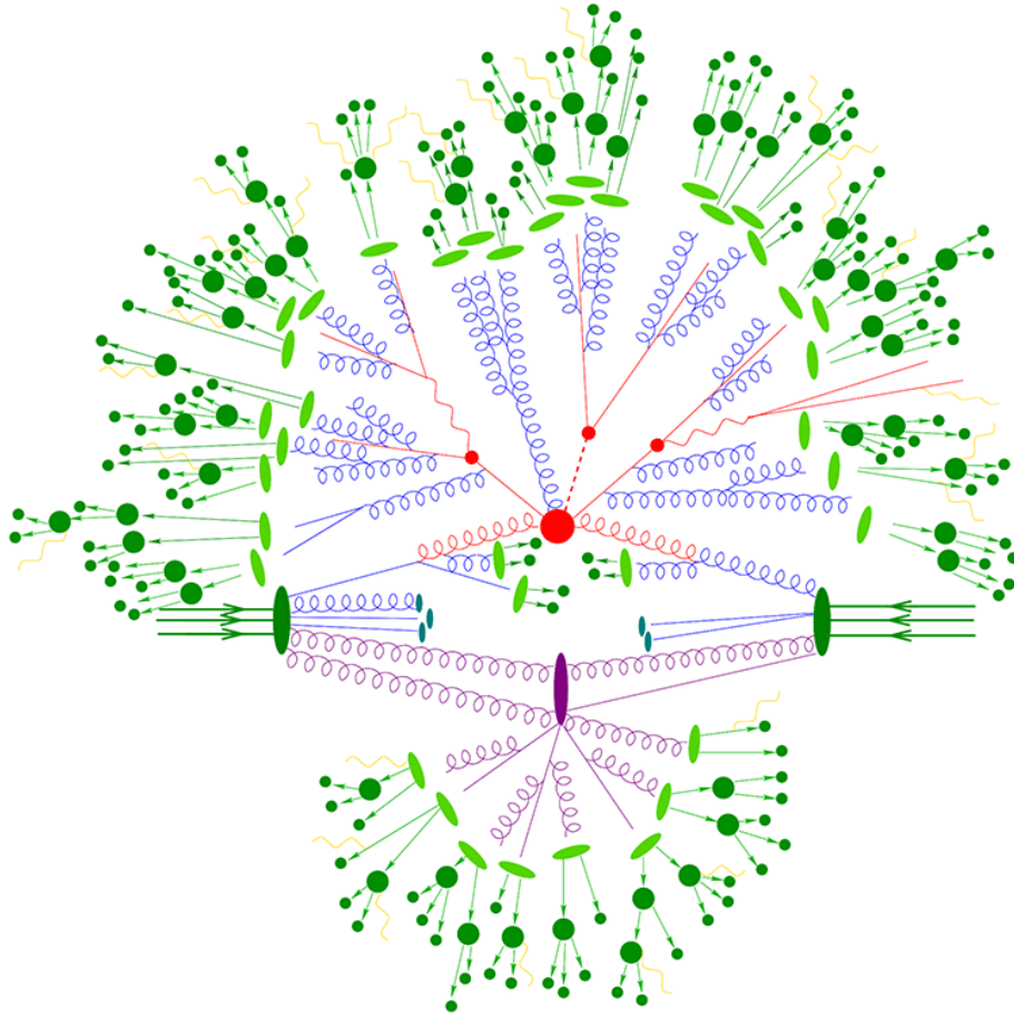
Figure 5.2: Image (from [102]) showing the different factorised stages in MC simulations. The first stage are the incoming hadrons, and these are represented by dark green lines with arrows pointing towards the IP. The next stage is the hard scattering process depicted in red and interactions with the rest of the proton (underlying event (UE) or secondary hard scattering events (Multiple Particle Interactions or MPI)) are shown in purple. The parton shower that follows the main hard scatter process is shown in blue. The subsequent hadronisation is represented by light green, with hadron decays and final state particles shown in dark green. The wavy yellow lines represent accompanying electromagnetic radiation from the final state particles.
