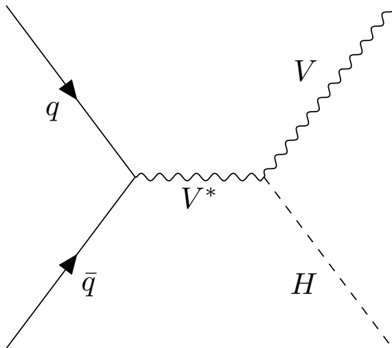
Figure 8.3: Feynman diagram of associated production of a Higgs particle with a vector boson. V here can either represent a W -boson or a Z -boson. The cross-section represented by this diagram is lower than the other diagrams because this interaction requires that a 'sea' anti-quark from one proton interacts with a valence quark of the other.
