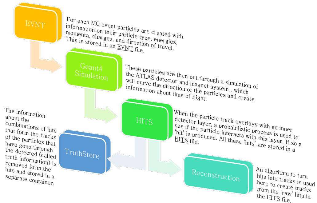
Figure 6.12: Graphic showing how MC truth track and reconstructed track objects are made.
