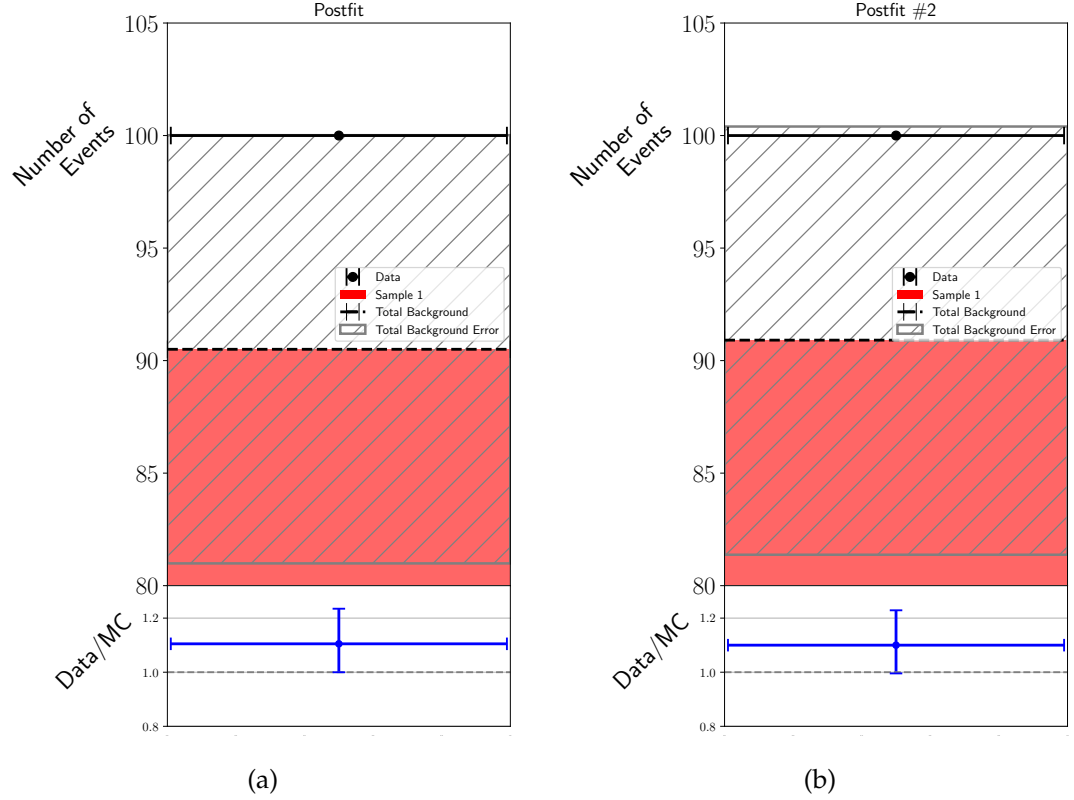
Figure 9.16: Comparison of the post-fit plots between the single and double systematic fits. The pre-fit (Figure 9.10a) for both of these fits is the same. These plots have been zoomed in around the data to show the differences between these fits more easily (the sample level still goes to zero). In the second post-fit plot (9.16b), the data point is closer to the Monte Carlo prediction.
