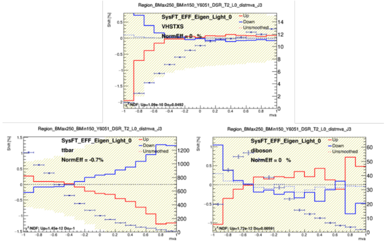
Figure 9.26: Image showing the shape and normalisation effects of the systematic SysFT_EFF_Eigen_Light_0 or (FT_Light_0 for short) in the signal (VHSTXS), t\bar{t} ( t\bar{t}bar ) and diboson samples binned by their MVA scores. This systematic has the largest impact in t\bar{t} events that look signal-like.
