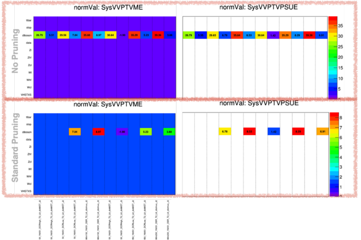
Figure 9.37: NormVal plots for the two systematics VVPTVME (left) and VVPTVPSUE (right) without pruning (top) and with pruning (bottom) for the 12 regions in the 0L standalone fit.
