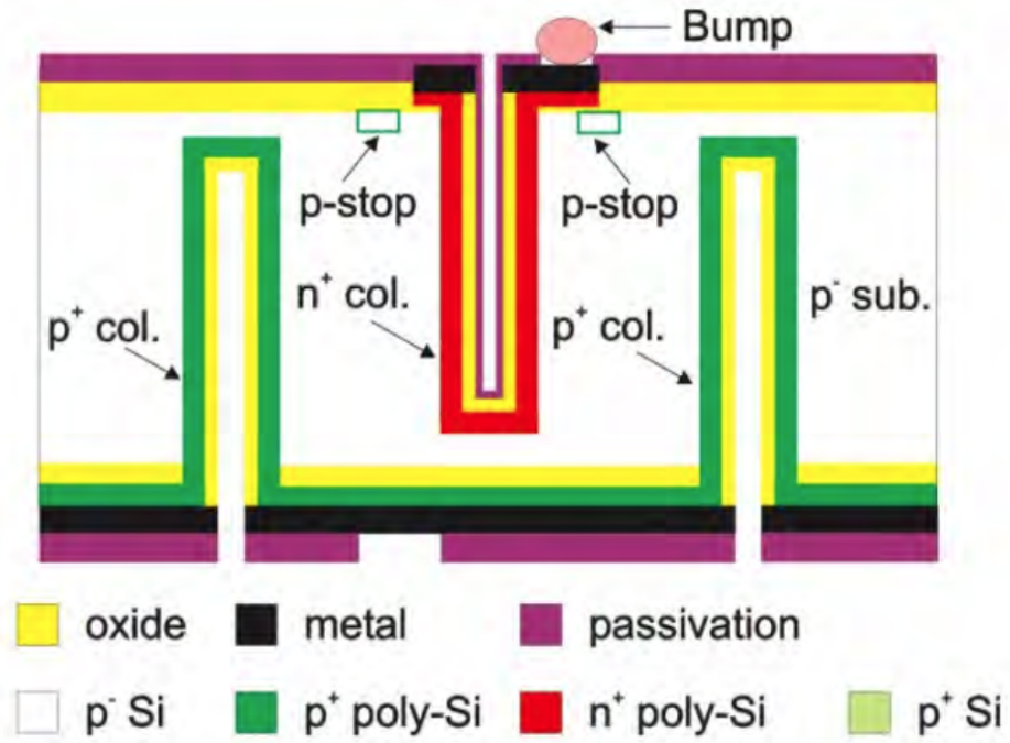
Figure 4.16: Cross-section of a 3D Pixel fabricated at CNM. Image from [87, p18].
