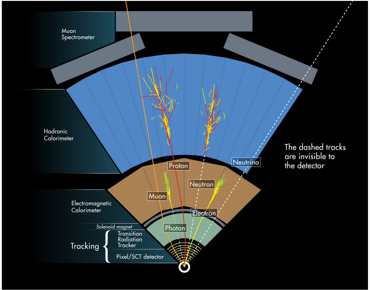
Figure 4.17: Image showing the typical energy deposits of various particles traversing through a simplified cross-section of the ATLAS detector. Image from [88].
