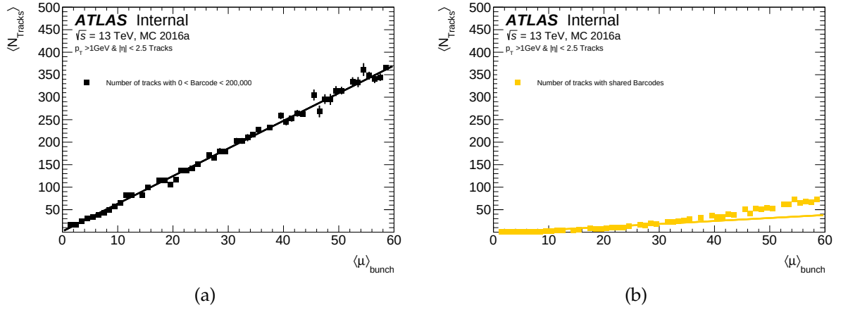
Figure 6.18: Number of stable reconstructed tracks vs \mu for all track objects that have low barcodes ( 0 < \text{barcode} < 2 \times 10^5 ) (a); and for all track objects that share the same barcode (b).
