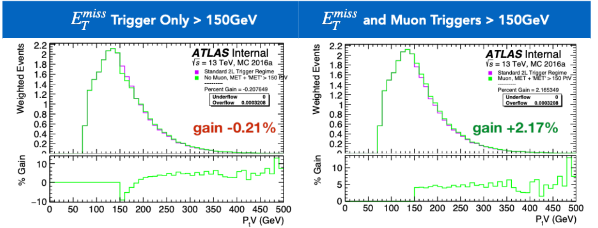
Figure 10.6: Preliminary results for the impact on the decided E_T^{miss} trigger regime on the Resolved analysis. MET + 'MET' refers to the final E_T^{miss} proxy used by this study which is a vector addition of MET_{dimuon} and MET.
