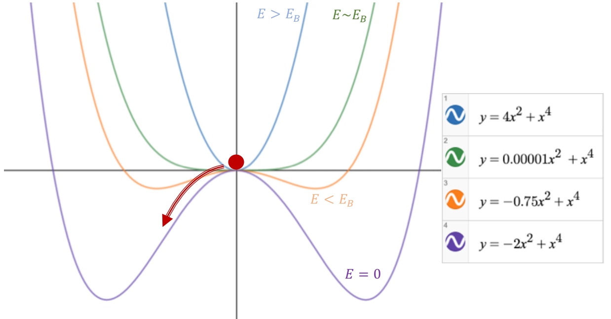
Figure 2.6: Image showing a rough sketch of the Higgs potential complete with a Higgs Boson for a fixed \lambda (the coefficient of the x^4 term) and a running m^2 (the coefficient of the x^2 term) for four different values of m^2 . The y-axis represents energy, and the x-axis represents the magnitude of the complex field, \phi , assuming that the potential is symmetric in the phase. E_B signifies the point where the potential becomes non-trivial and this is taken to be O(100 \text{ GeV}) . The potential is spherically symmetric such that there is a continuous ring of minimum point values. Image generated using [28].
