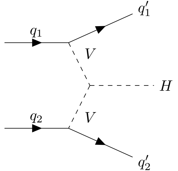
Figure 8.2: Feynman diagram of the production of a Higgs particle via vector boson fusion. V here can either represent a W -boson or a Z -boson.
