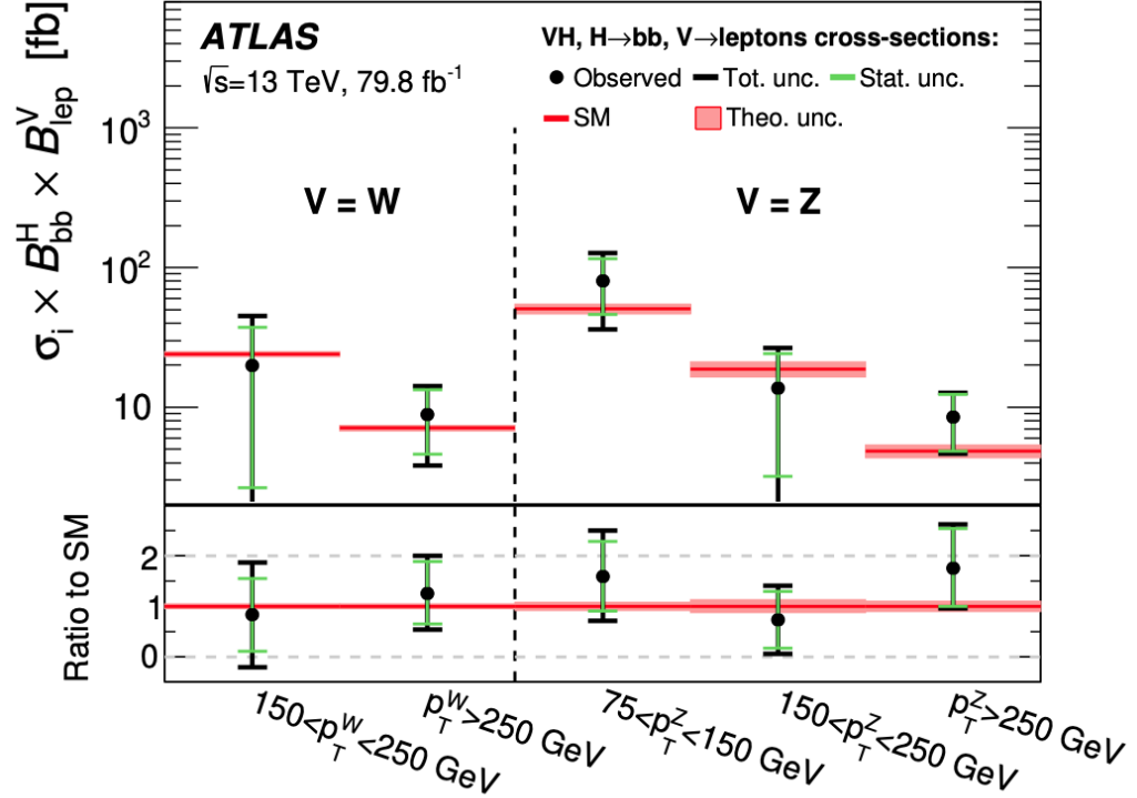
Figure 8.11: Measurements of cross-section \times branching fractions of H \rightarrow b\bar{b} and V \rightarrow ll for each of the 5 POI's. The pad below shows the ratio of these partial signal strengths to the SM values. Image from [143, p11].
