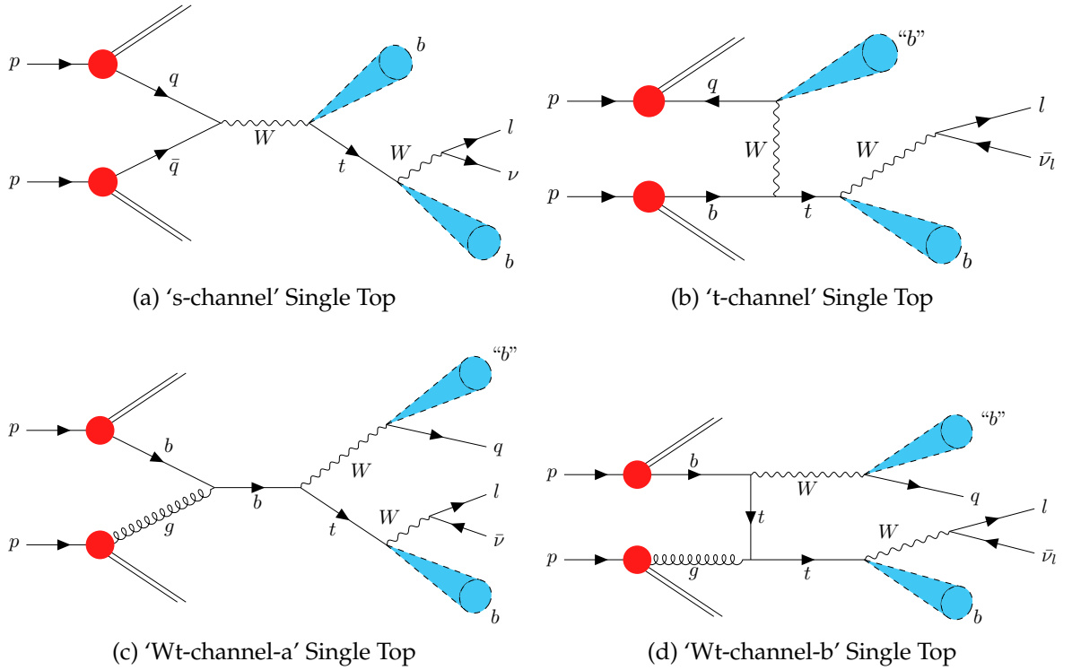
Figure 8.14: Image showing the four tree-level single top Feynman diagrams. The top diagrams are weak processes referred to as s -channel (top left) and t -channel (top right). The bottom two are irreducible (can't be distinguished from each other) 'Wt-channel' diagrams. Particles misidentified as b -jets are labelled as " b ".
