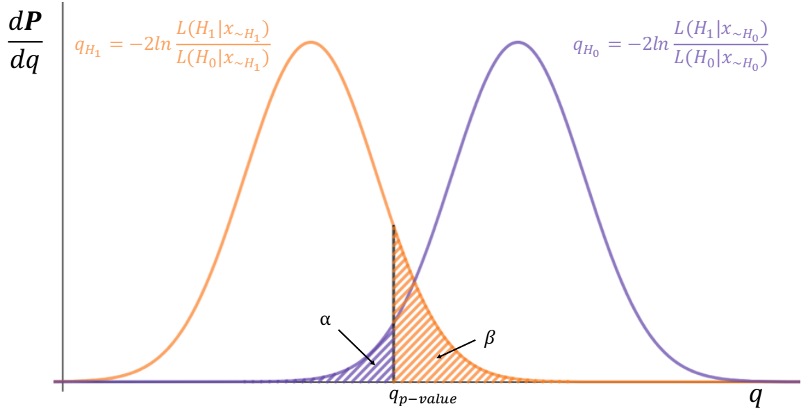
Figure 9.1: Example formulation of the test statistic for the null ( q_{H_0} ) and alternative hypothesis ( q_{H_1} ). \alpha , given by the purple hatched area, corresponds to the probability that the null hypothesis is rejected given that the null hypothesis is true, and \beta , given by the orange hashed area, is the probability that the alternative hypothesis is rejected given that the null hypothesis is not true. Smaller q values are in general more signal like. The value of q that corresponds to \alpha equalling the p -value is denoted by q_{p\text{-value}} . Before any measurement is taken, the strength or power of the statistical test can be measured from the relative areas of \alpha and \beta given a observed q(q_{obs}) equalling this q_{p\text{-value}} . Image generated using [28].
