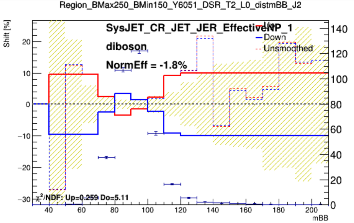
Figure 9.17: Illustration of the possible effect a systematic can have when it is present in multiple bins. The shape effect of the systematic is split into each sample and this plot is the effect of the first eigenvalue for the Jet energy resolution systematic on the diboson sample in the Boosted analysis. The dashed horizontal black line is the nominal MC simulated events prediction. The dashed red and blue lines are the unsmoothed +1\sigma and -1\sigma variations of the systematic in each bin respectively. The solid red and blue line correspond to the smoothed (see Section 9.3.3) +1\sigma and -1\sigma fluctuations of the uncertainty with respect to the nominal prediction. The left y-axis is the percentage shift in the events the systematic lines represent. The blue data points in this bin with the right y-axis being the number of events in the bin. The beige hashed lines are the errors on the number of MC simulated events events in each bin. The plot also contains information about the normalisation effect for this uncertainty in all these bins.
