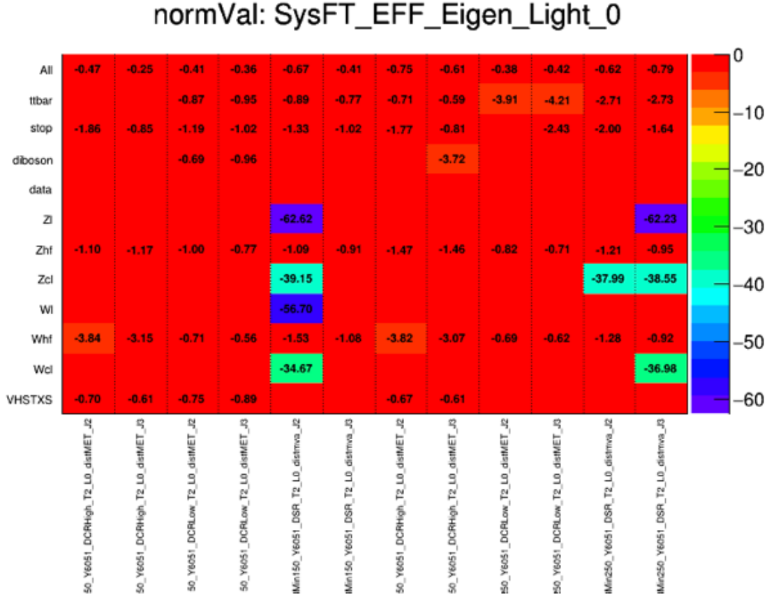
Figure 9.27: Image showing the normalisation effect of the systematic SysFT_EFF_Eigen_Light_0 (FT_Light_0 for short). This systematic appears to have the largest effect in the 2-Jet 150 \text{ GeV} \leq p_T^V < 250 \text{ GeV} Signal Region and the 3-Jet p_T^V \geq 250 \text{ GeV} Signal Region. Since the analysis was blinded at this point, there are no normalisations recorded for data in any region.
