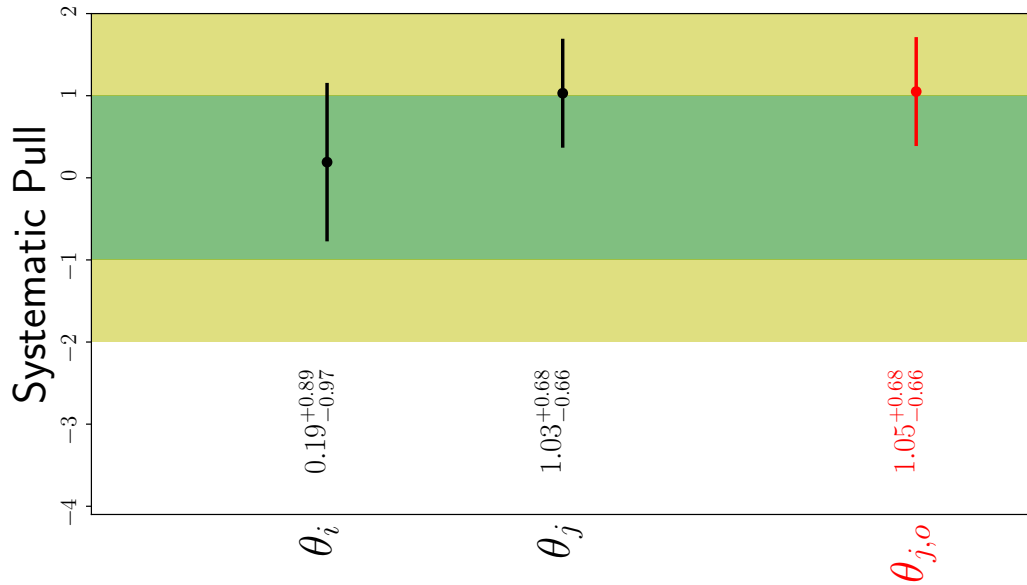
Figure 9.12: Pull plot showing the pull and variance for \theta_i and \theta_j . The inclusion of the red point \theta_{j,o} provides a comparison to the previous fit with its only systematic \theta_j . The presence of the second systematic in the same bins means the fit can be optimised by not pulling the systematic \theta_j to the full extent it was pulled in the previous version of the fit.
