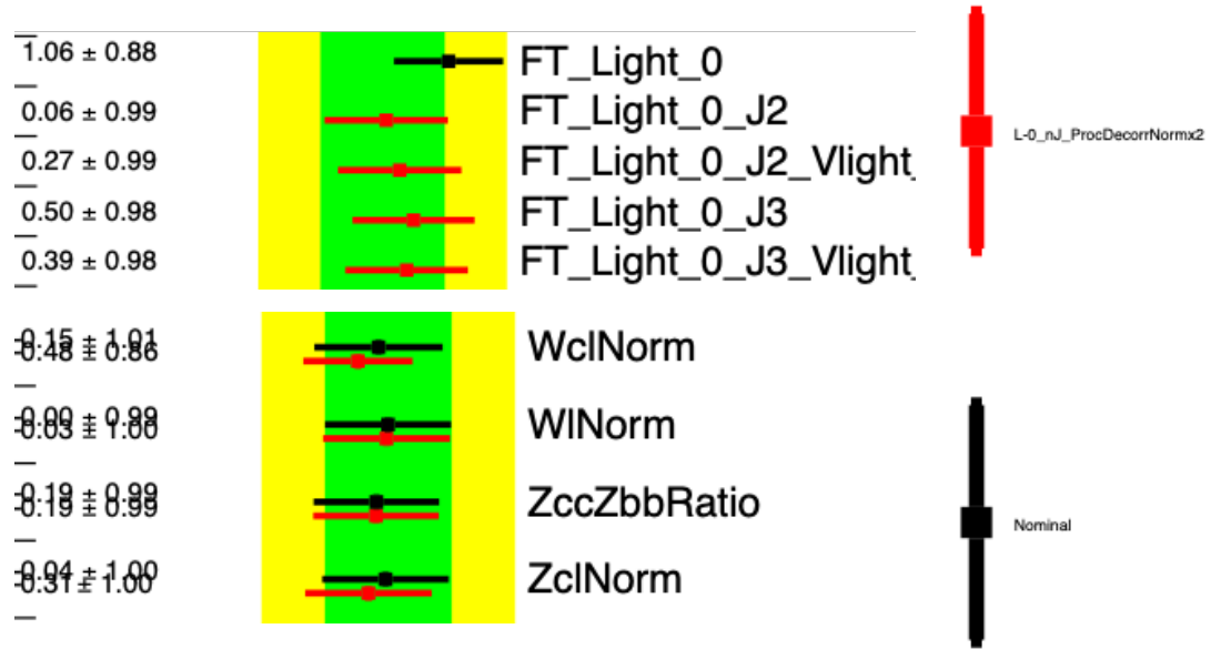
Figure 9.31: Pull plot where the nominal fit (black) is compared to the fit decorrelated in both n -jet and V +light categories and the normalisation systematics are doubled (red).
