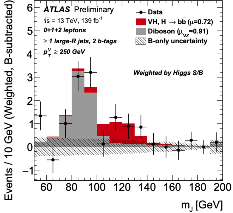
Figure 11.2: m_J distributions in all of the lepton channels and p_T^V regions combined for data and MC simulations simulations after the removal of all non-diboson backgrounds in the Boosted analysis. The combined regions are weighted by their ratios of the Higgs-signal-to-background ratio. The hatched band shows the total uncertainty minus uncertainties on VH or VZ . Image from [4, p17].
