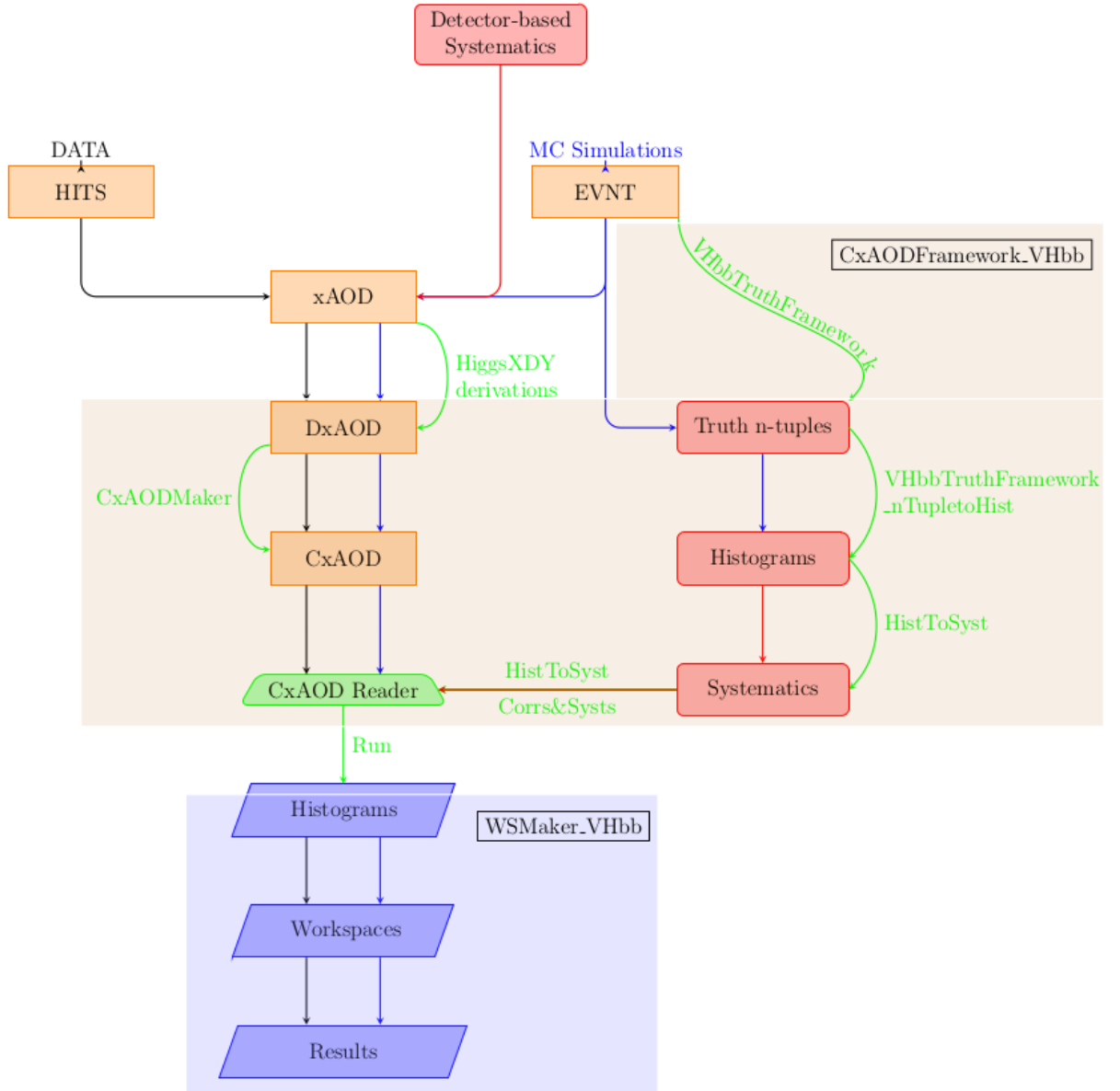
Figure 8.17: Picture showing the rough workflow of the analysis. Black lines represent data, blue lines represent MC simulations, red lines represent systematics. Green curved lines are packages in the analysis. Detector-based systematics are propagated to Monte Carlo Simulations into the xAOD format and end up being stored in CxAOD's as 'shallow copies'.
