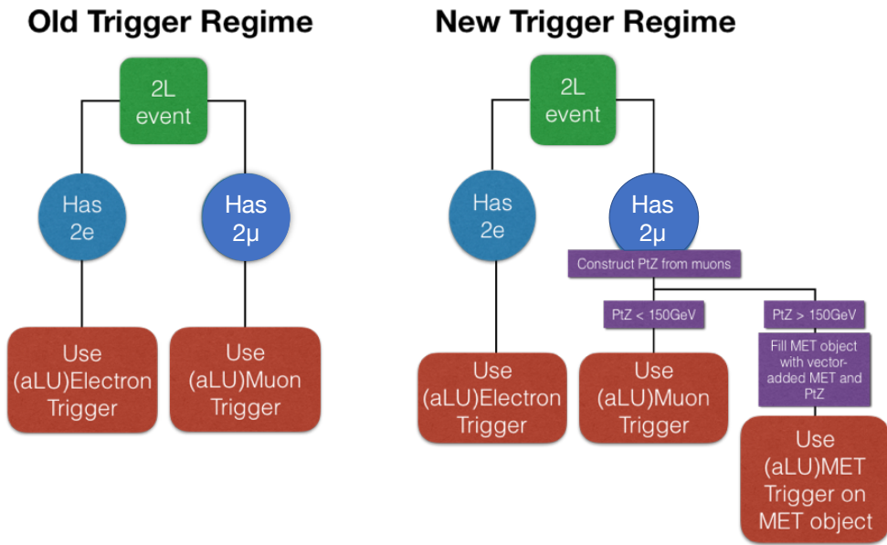
Figure 10.7: A simple graphic showing differences between the new and the older trigger regime. ALU stands for ‘add lowest un-prescaled’ triggers, which means the triggers with the lowest energy threshold not adjusted for any other effects.
