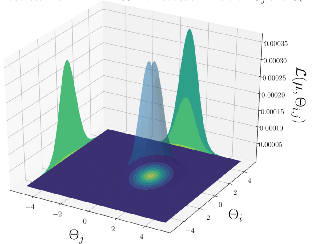
Figure 9.11: 3D plot showing the change of the likelihood with variation of two systematics: \theta_i and \theta_j . The maximal point in this (\theta_i - \theta_j) phase space roughly corresponds to a \theta_i pull of 0 and a \theta_j pull of 1.
