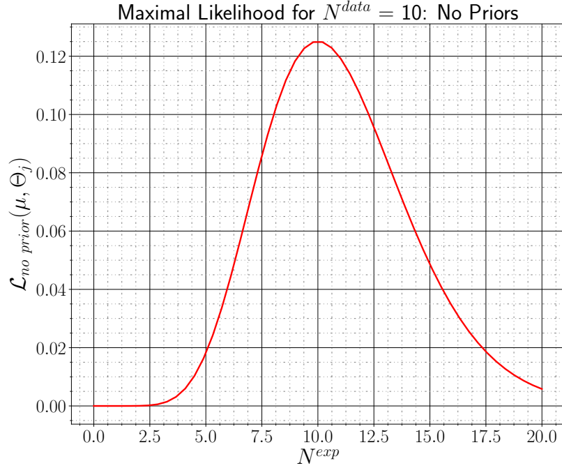
Figure 9.3: Variation of the likelihood for different values of the number of expected events ( \mathcal{N}^{exp} ). The maximum possible likelihood is reached when \mathcal{N}^{exp} = \mathcal{N}^{data} .
