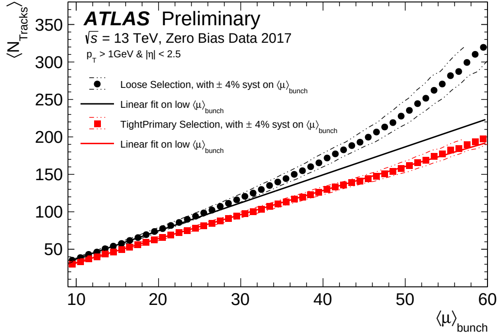
Figure 6.3: Plot of the average number of tracks as a function of pile-up for the Loose and TightPrimary tracks in Run 2 data. Here the p_T cut-off at 1 GeV rather than 400 MeV reflects the fact that the majority of analyses that use tracks do not find tracks of that low energy to be useful. The black and red lines are linear fits made between 9 \leq \langle\mu\rangle_{\text{bunch}} \leq 16 and extended out to higher \langle\mu\rangle_{\text{bunch}} .
