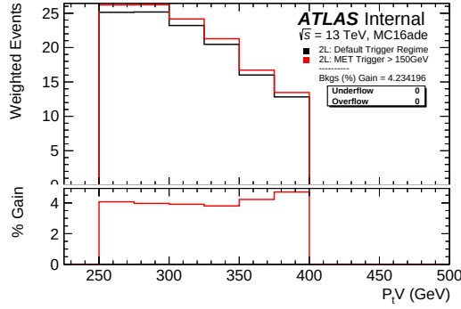
(c) Background yield increase: 4.23%, 250 \text{ GeV} \leq p_T^V < 400 \text{ GeV}
