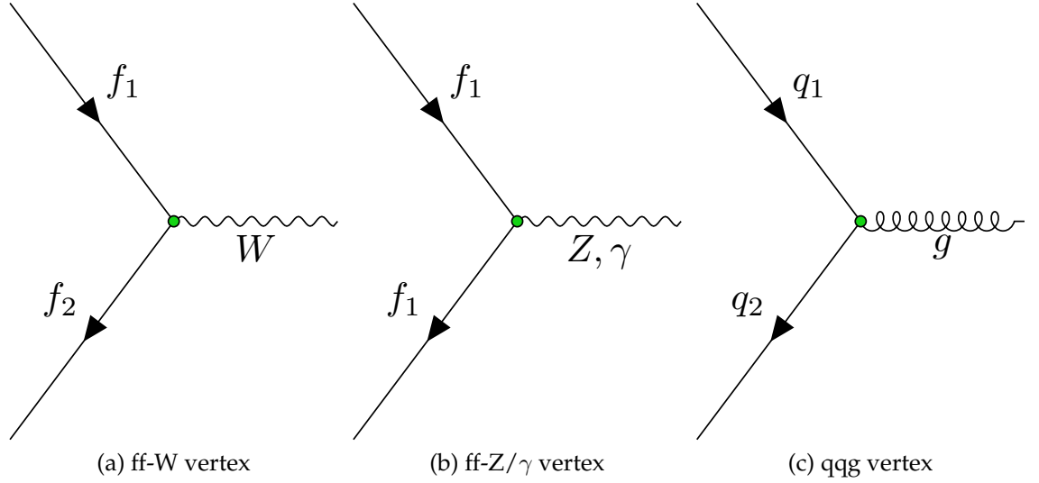
Figure 2.4: Image showing the three Standard Model Feynman vertices allowed by the \mathcal{L}_{Fermions} term in the Standard Model Lagrangian. The f represents quarks, and both charged and neutral leptons. For fermion species interacting with a W-boson the two incoming and outgoing fermions must be different but for fermions interacting with a Z-boson or a photon, the species must be the same. For the strong qqg vertex, while the flavour of q_1 and q_2 are the same they will have different colour charges as the gluon also carries colour charge.
