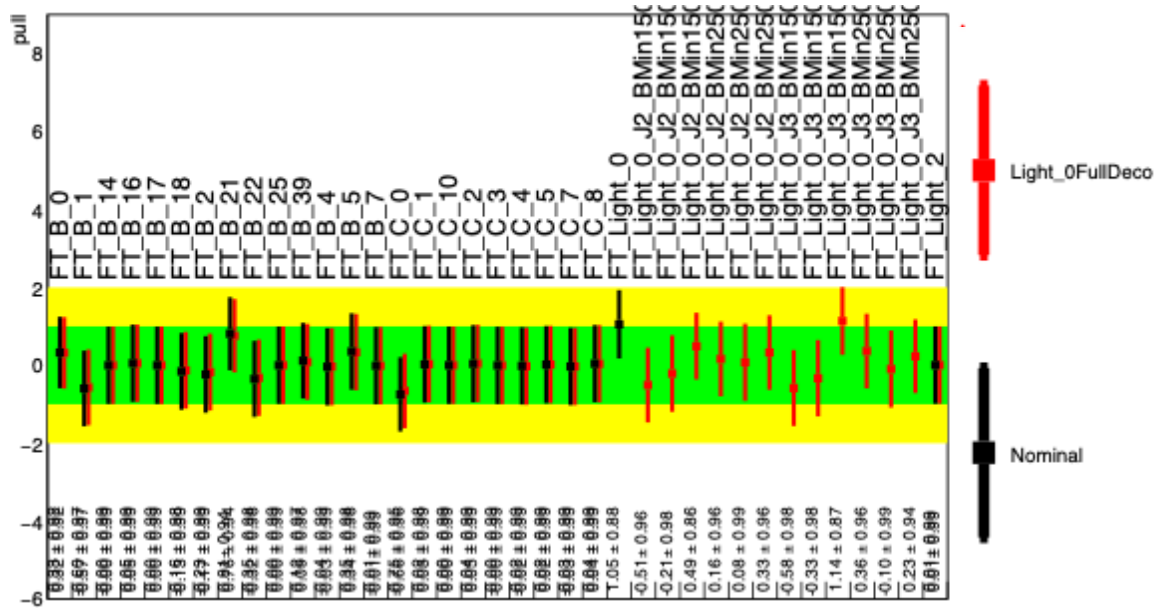
Figure 9.22: B -tagging pulls comparing the fits of the nominal fit (in black) with the fit where the \text{Light}_0 pull is fully decorrelated (in red). The name of decorrelated systematics are too long to fit on the plot, so the region part has been cut off. The naming convention is such that the systematics are organised into 4 sets of three regions. In each three the first region is \text{CR}_{\text{Low}} , the second is \text{CR}_{\text{High}} , and the final one is the SR. J(X) refers to the number of jets in the category ( J3 = \text{a 3-Jet event} ). \text{BMin150} corresponds to the 150 \text{ GeV} \leq p_T^V < 250 \text{ GeV} region and \text{BMin250} corresponds to the p_T^V \geq 250 \text{ GeV} region. Here the overall pull is coming from one region: The 3-Jet 150 \text{ GeV} \leq p_T^V < 250 \text{ GeV} SR.
