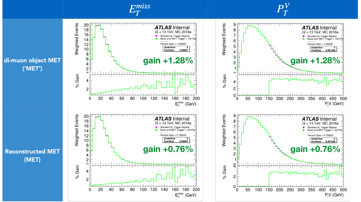
Figure 10.3: Preliminary plots showing the effect of the E_T^{\text{miss}} study in the Resolved 2-lepton analysis. Here an event will be selected if it passes one of the muon or E_T^{\text{miss}} trigger sets. A di-muon object with missing E_T labelled as ('MET') is a stand-in for MET_{\text{dimuon}} . Note that the ratio of new to old trigger regime doesn't change for p_T^V values below 150 GeV as events at these values of p_T^V are not affected by these changes.
