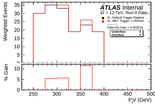
(e) Data yield increase: 4.40%, 250 \text{ GeV} \leq p_T^V < 400 \text{ GeV}
