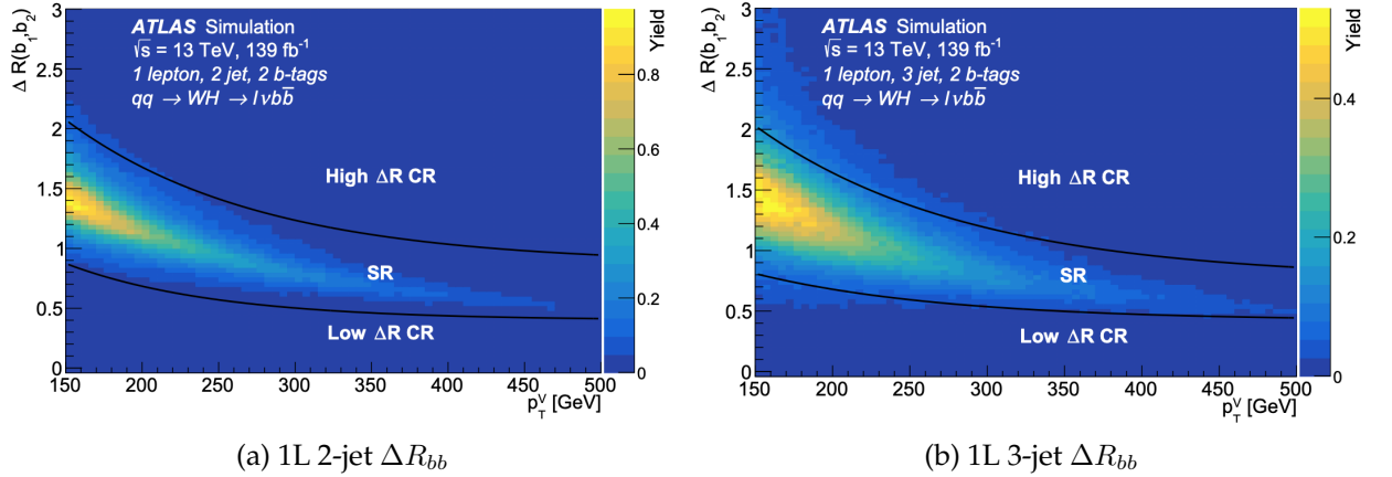
Figure 8.18: Distribution of the signal yield under the radial difference between the two leading jets for (a) 2-jet and (b) 3-jet 1-lepton channel. The dark lines show the distinction between the High \Delta R CR, SR and the Low \Delta R CR. Image from [3, p11].
