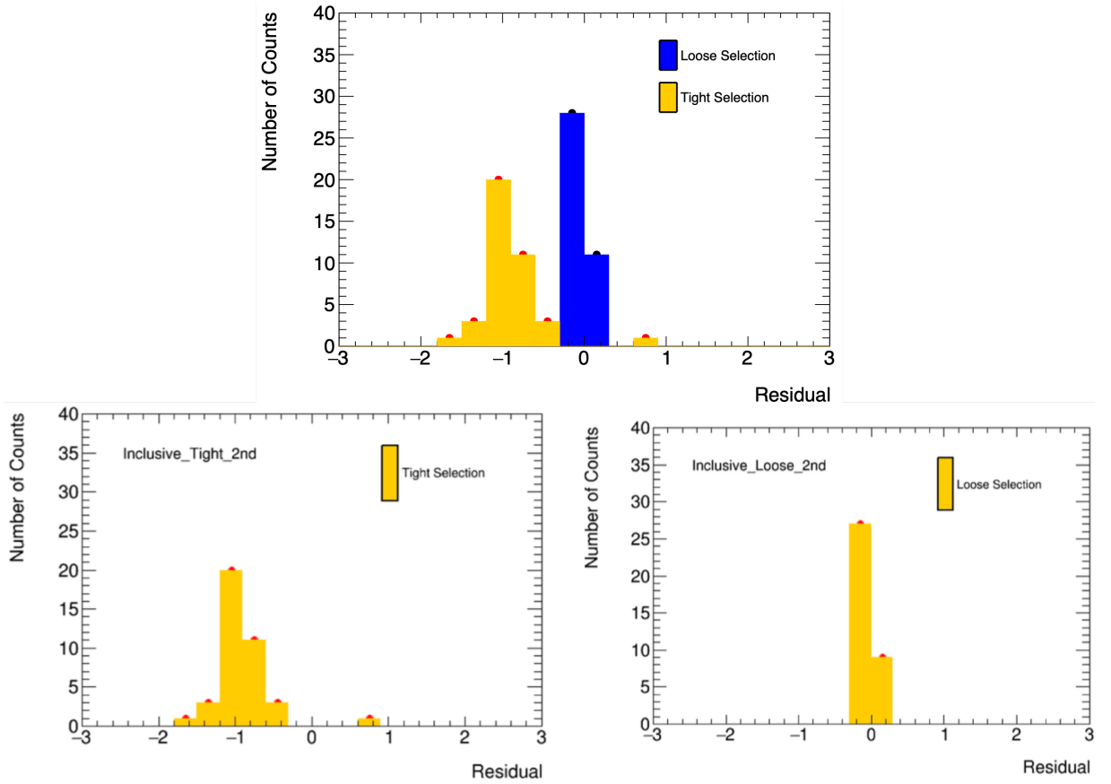
Figure 6.6: Histograms for the residuals of the ratio between data and MC simulations for the average number of tracks against \mu . On the top these are shown for the Loose and the TightPrimary (referred to in these figures as simply 'Tight') selections and on the bottom after two rounds of outlier removal, for the TightPrimary (left) and Loose selections (right) respectively.
