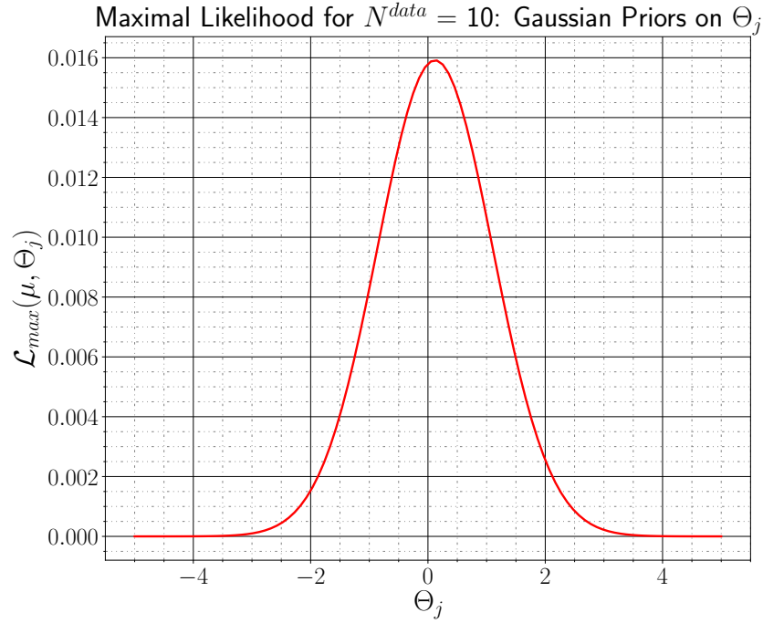
Figure 9.4: Plot of the likelihood value at different values for the number of sigma the systematic \theta_j is shifted. For the simple fit, the systematic is only slightly pulled from no shift at all.
