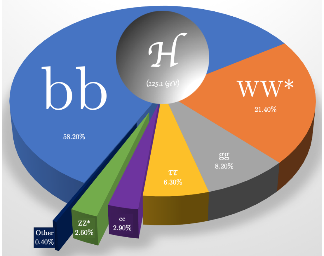
Figure 2.9: Pie chart showing the decay ratios of the Higgs boson to other particles. Even though pairs of W - and Z -bosons are heavier than the Higgs rest mass, the masses of the virtual particles can differ from the nominal masses such that the decay is still kinematically possible. This is known as being produced ‘off-shell’ and the asterisk shows that at least one of the particles is produced in this manner. The Higgs boson also can decay into gluons via an intermediate (top) quark loop. These branching fractions are dependent on the energy of the Higgs particles. These ratios are taken from a Higgs with its nominal mass.
