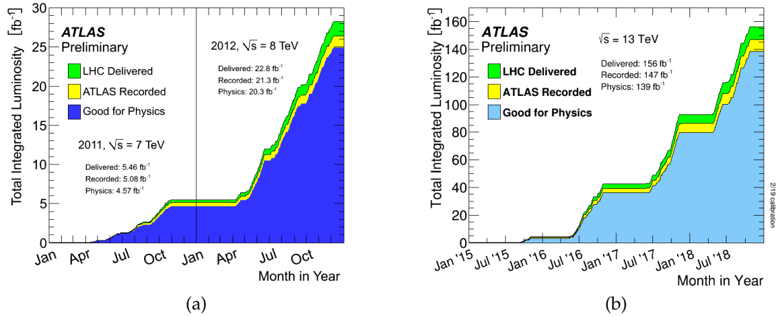
Figure 4.1: Cumulative luminosity delivered by the LHC and recorded by ATLAS detector for the entire lengths of Run-I (a) [65] and Run-II (b) [66]. The total physics-quality data recorded over Run-1 and Run-2 is 163.87 \text{ fb}^{-1} .
