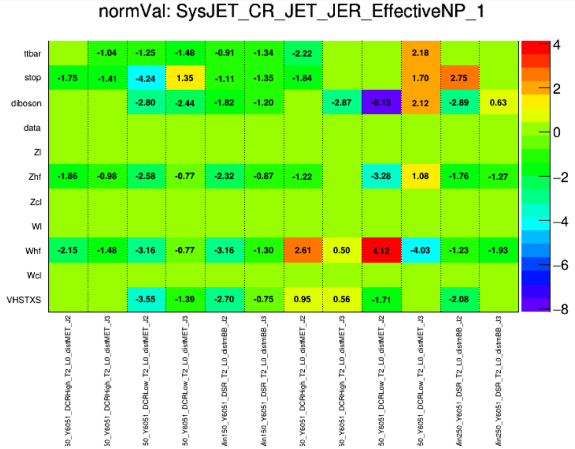
Figure 9.18: Image showing the normalisation effect of a systematic SysJET_CR_JET_JER_EffectiveNP_1. Each sample present in a region is separated on the y-axis, and the (0L) Standalone fit regions are shown on the x-axis. Each number in the boxes is a percentage. Spaces that are empty within rows that have values in them are empty because those effects were pruned (see Section 9.3.4). If the entire row is empty this means that the systematic has no effect on that region whatsoever, or in the case of data; the effect is purposefully hidden. This systematic appears to have the largest effect in the 2-Jet 150 \text{ GeV} \leq p_T^V < 250 \text{ GeV} Low \Delta R_{bb} control region. The size of these effects are more easily judged by looking at the number of events that this systematic can effect, which is accessed in a shape plot.
