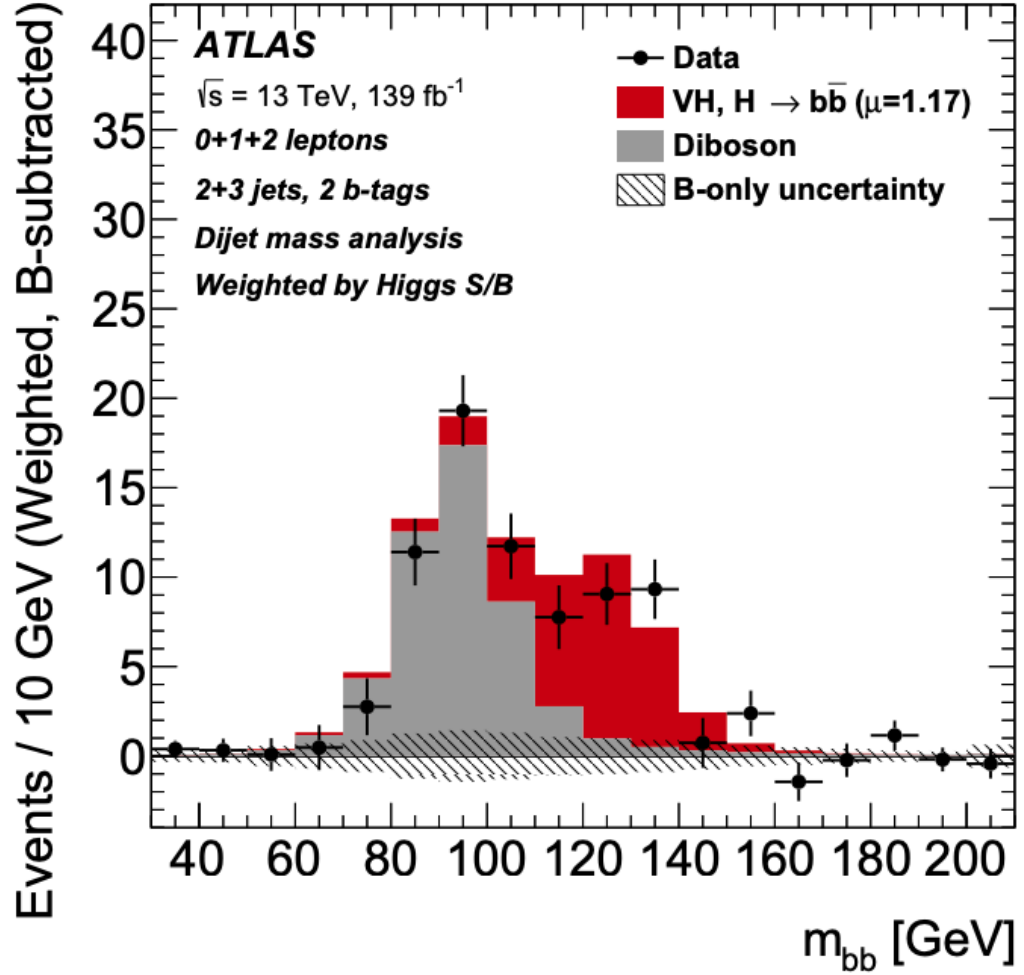
Figure 11.5: Final m_{bb} distributions in all of the lepton channels and p_T^V regions combined for data and MC simulations after the removal of all non-diboson backgrounds in the Resolved analysis. The combined regions are weighted by their ratios of the Higgs-signal-to-background ratio. The hatched band shows the total uncertainty minus uncertainties on VH or VZ . Image from [3, p29].
