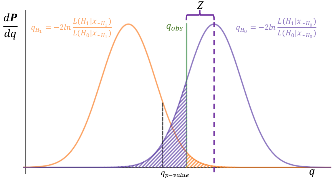
Figure 9.2: Upon measurement of q_{obs} , the alternative hypothesis is rejected as the q_{obs} is smaller than the p-value set. The significance of the result is given by Z , the number of standard deviations by which the central values of q_{H_0} and q_{obs} are separated. Image generated using [28].
