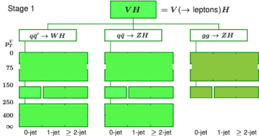
(a) Stage 1 STXS Binning
