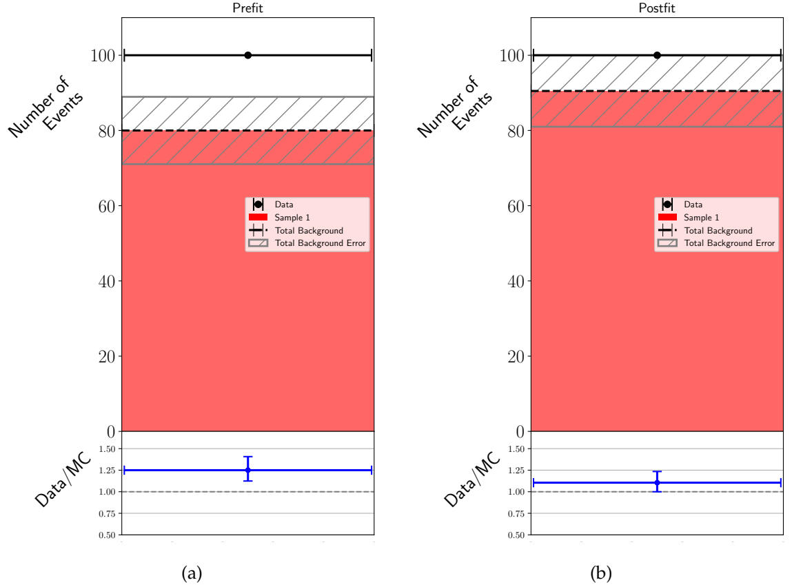
Figure 9.10: Pre-fit (9.10a) and post-fit (9.10b) plots for the example fit. Each sample that contributes to the number of events in that particular bin would get its own colour. In this case, the assumption was made that the bin was a background-only bin with only one sample contributing to events. The ideal result for the post-fit plot would be the black data point meeting the black dotted line. This would result in the blue point in the ratio plot lying on the data/MC = 1 line. Normally in a plot of this type, the y-axis would show weighted events, but there are no weights put on any events in this example for simplicity. The grey hashed line, therefore, represents the \sqrt{N} error on the number of counts.
