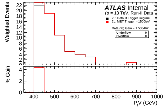
(f) Data yield increase: 1.53%, p_T^V \geq 400 \text{ GeV}
