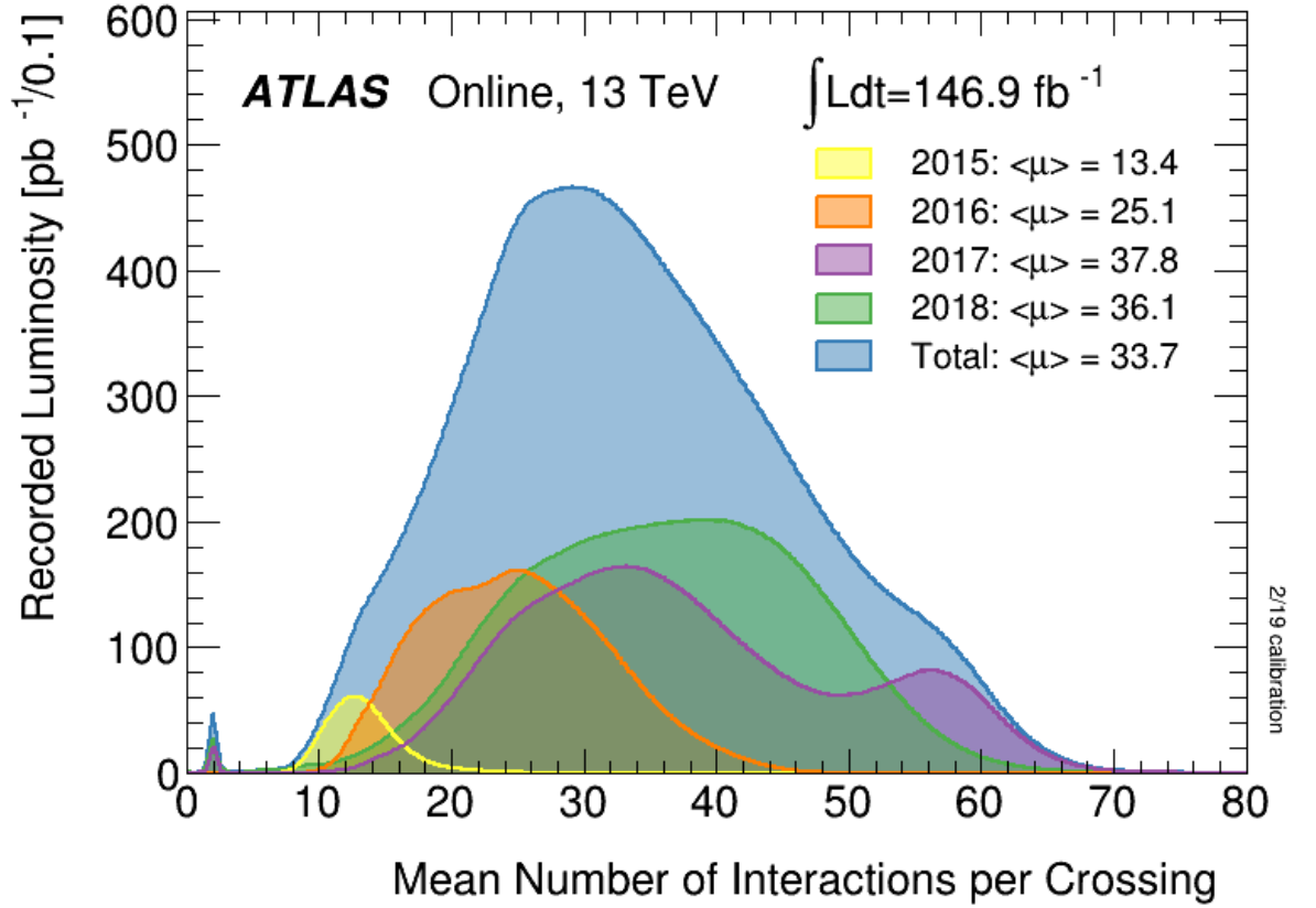
Figure 4.18: Average number of pile-up interactions per bunch crossing for each year in Run-2. Image from [66].
