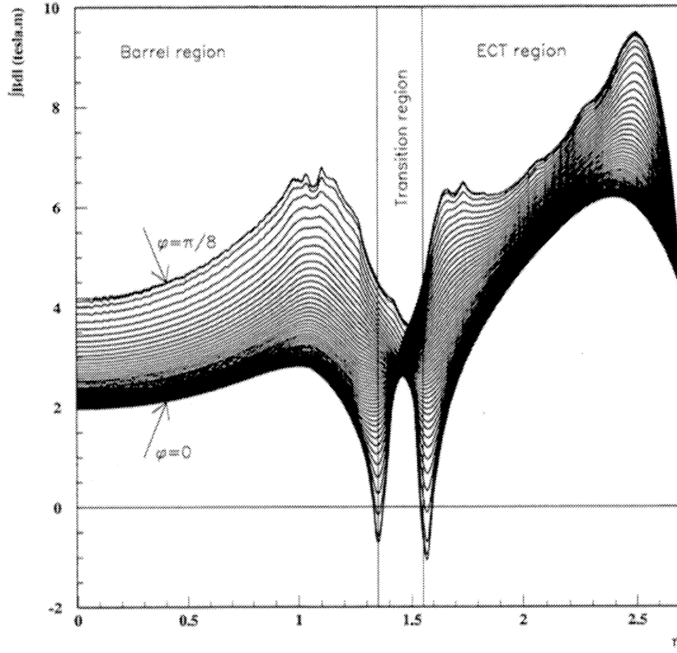
Figure 4.9: Plot showing the bending power as a function of |\eta| . Image from [75, p15].
