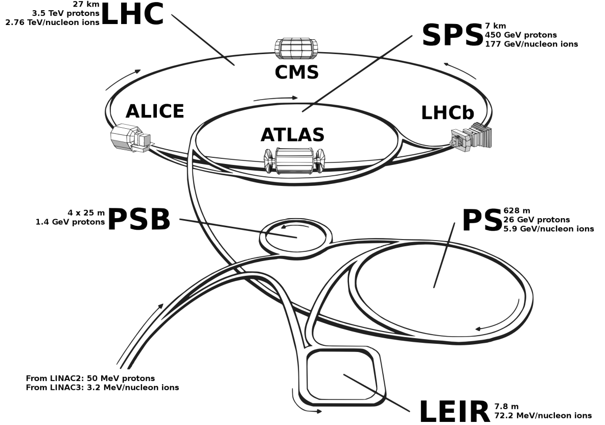
Figure 3.3: Labelled diagram of all the parts of the CERN accelerator complex that are important for the running of the LHC. Image from [54].
