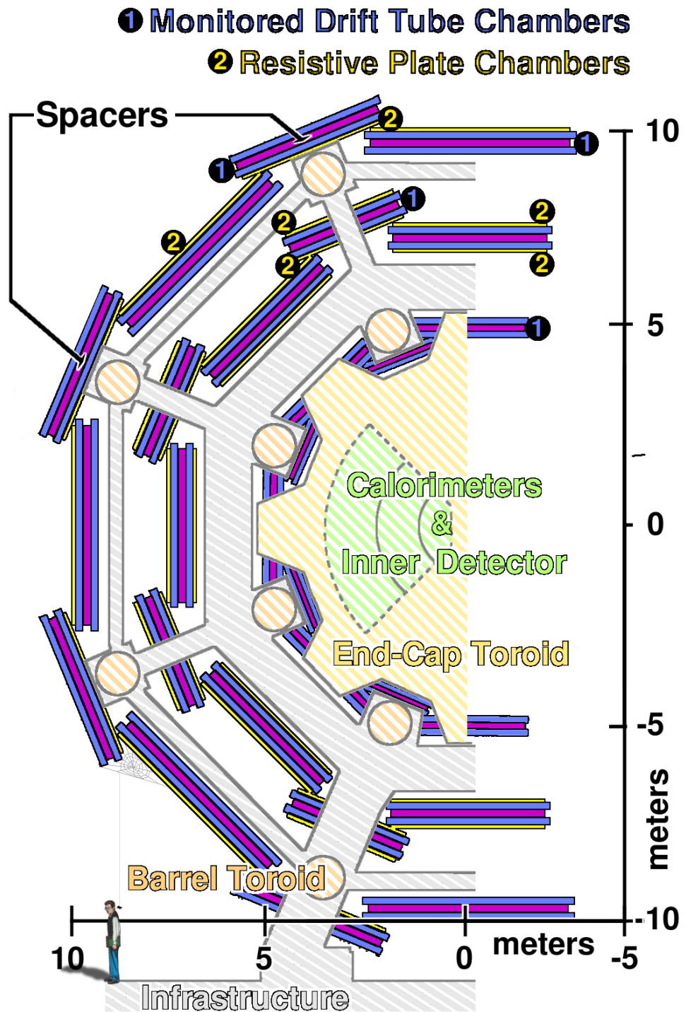
Figure 4.4: Schematic of the Muon Spectrometer shown here in indigo and violet. The dashed yellow lines indicate the presence of the magnetic toroids and the grey hashed lines represent non-tracking infrastructure. This image shows how the layers in the barrel interlace in a cylindrical fashion and how they surround the barrel toroid coil. Peter Parker and accompanying spider for scale. Image from [54].
