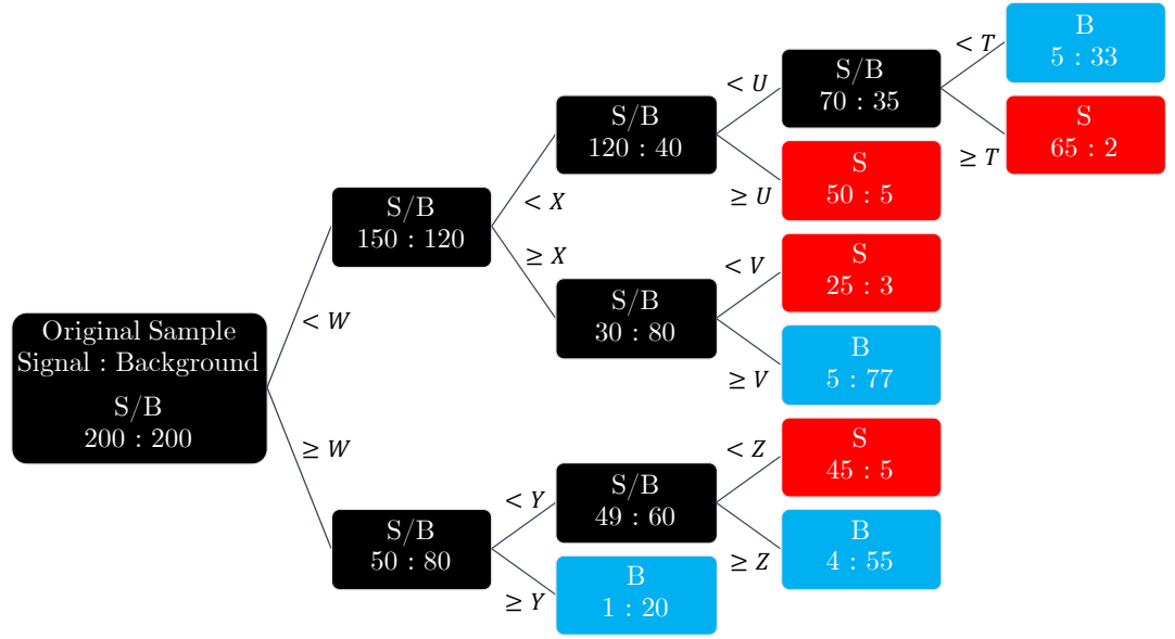
Figure 7.1: A schematic showing an example decision tree separation of a training set into signal (red) and background (blue) leaves. The black represents branches without any such designation and the letters T-Z are values in different variables that perform the best optimisation of signal and background at each splitting stage. Since Y and Z are variable splittings in a different branch path to T,U,V and X, Y and Z can be (but don't have to be) any one of the variables that correspond to the splittings T,U,V,X but they both cannot be the same.
