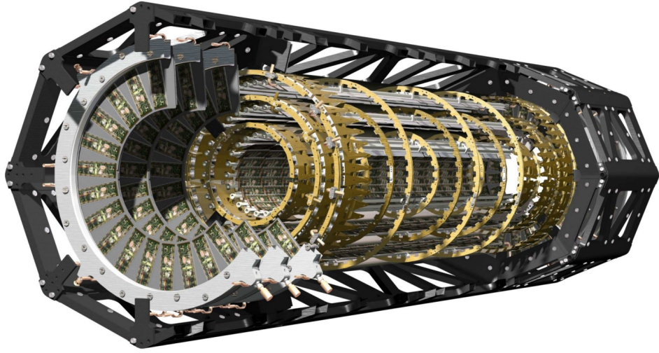
Figure 4.15: Cross-section of the entire pixel detector without the Inner Barrel Layer. Image from [69, p86].
