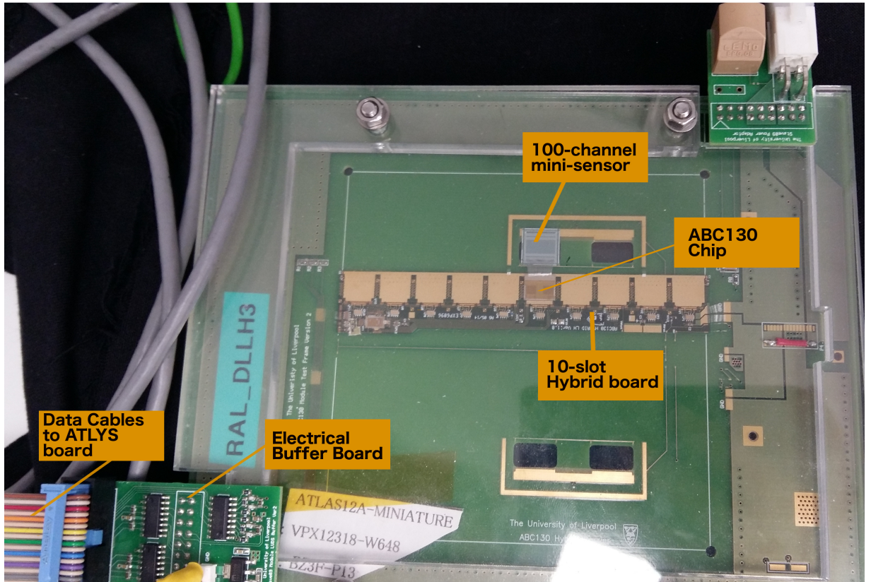
Figure 4.20: The RAL_DLLH3 set-up at the University of Glasgow. The test hybrid set-up has slots for 10 ABC130 chips. Only one of them is used, and that chip has a mini-sensor put across some of the pins to add a capacitance load across the chip. The buffer board ensures that the correct voltages are being applied to the chip from the power supply.
