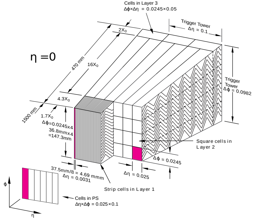
Figure 4.7: Sketch of the EM Barrel LAr Calorimeter. Image from [74].
