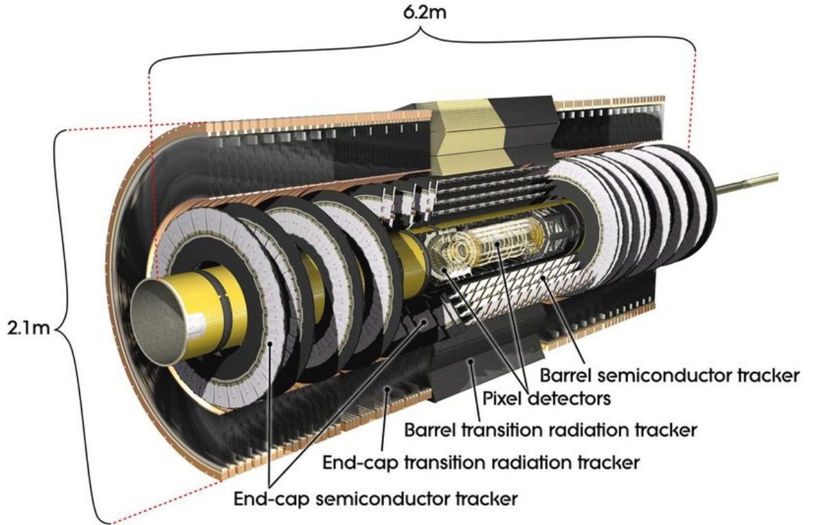
Figure 4.10: Schematic showing a close-up cross-section of the Barrel and Endcap Inner Tracker System at ATLAS. Image from [78].
