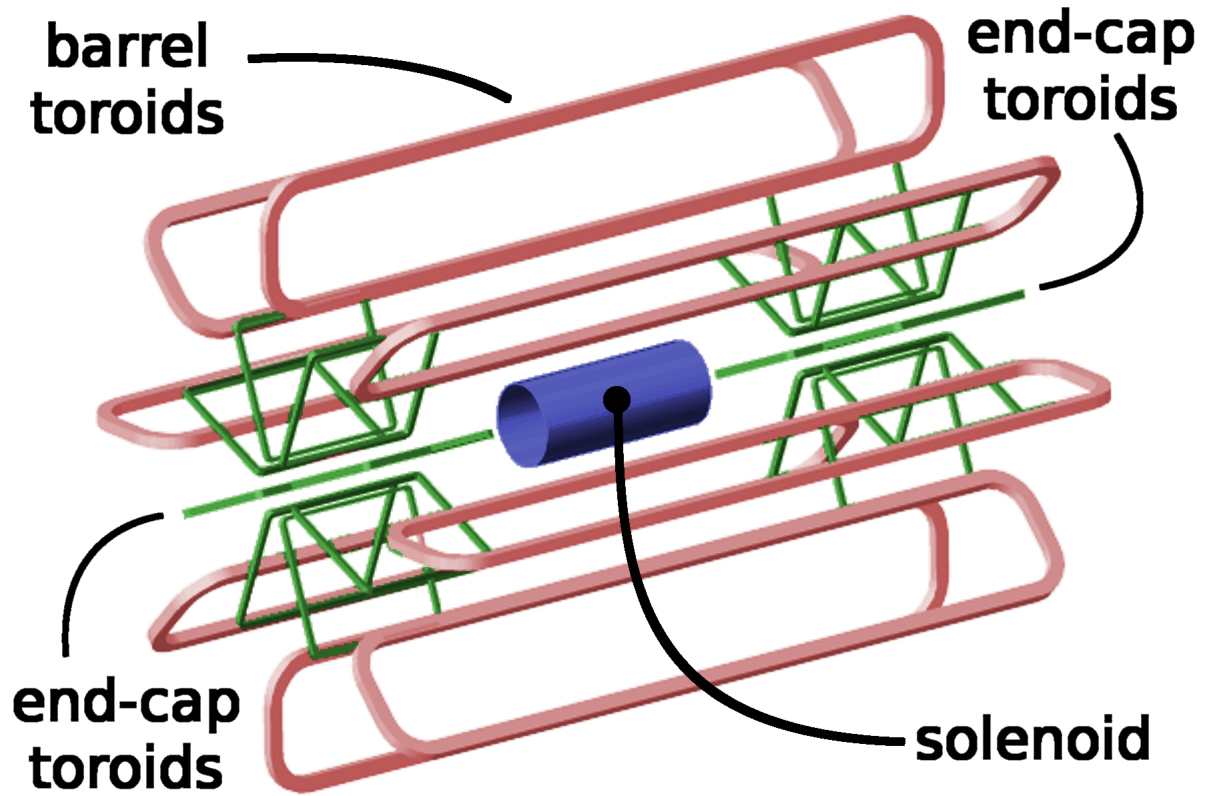
Figure 4.8: Schematic showing the Magnet System at ATLAS. Image from [54].
