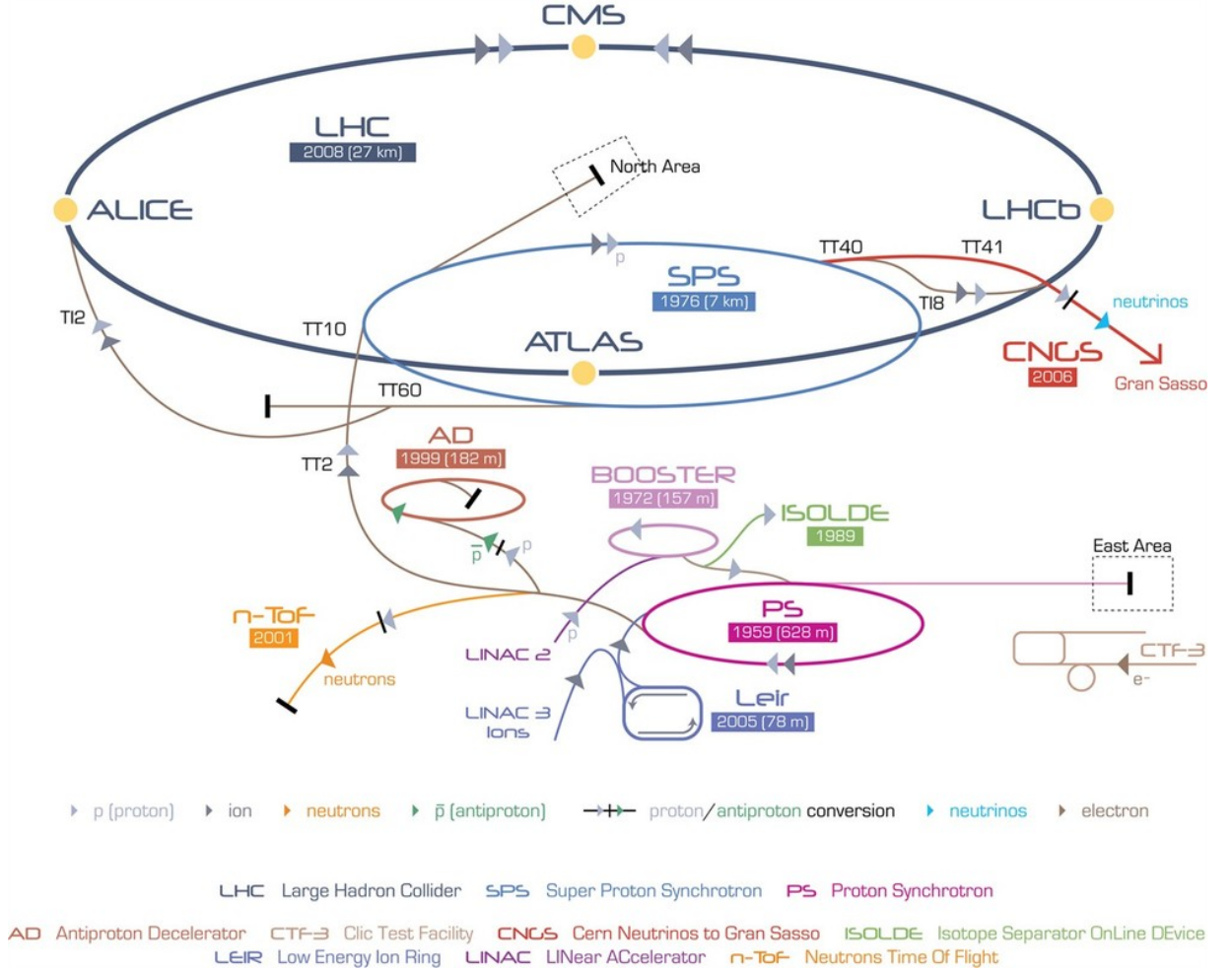
Figure 3.1: Image showing the CERN accelerator machine complex complete with the particles that traverse each of the sections [37].
