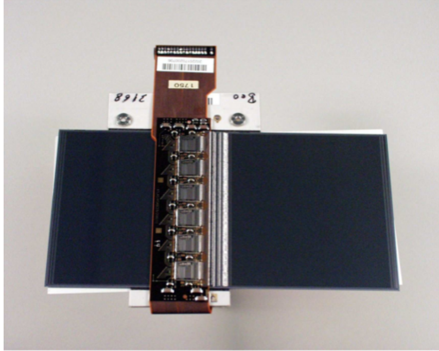
Figure 4.14: Picture of a SCT barrel module. The middle electronics board is placed over the junction of two sensors. Image from [69, p65].
