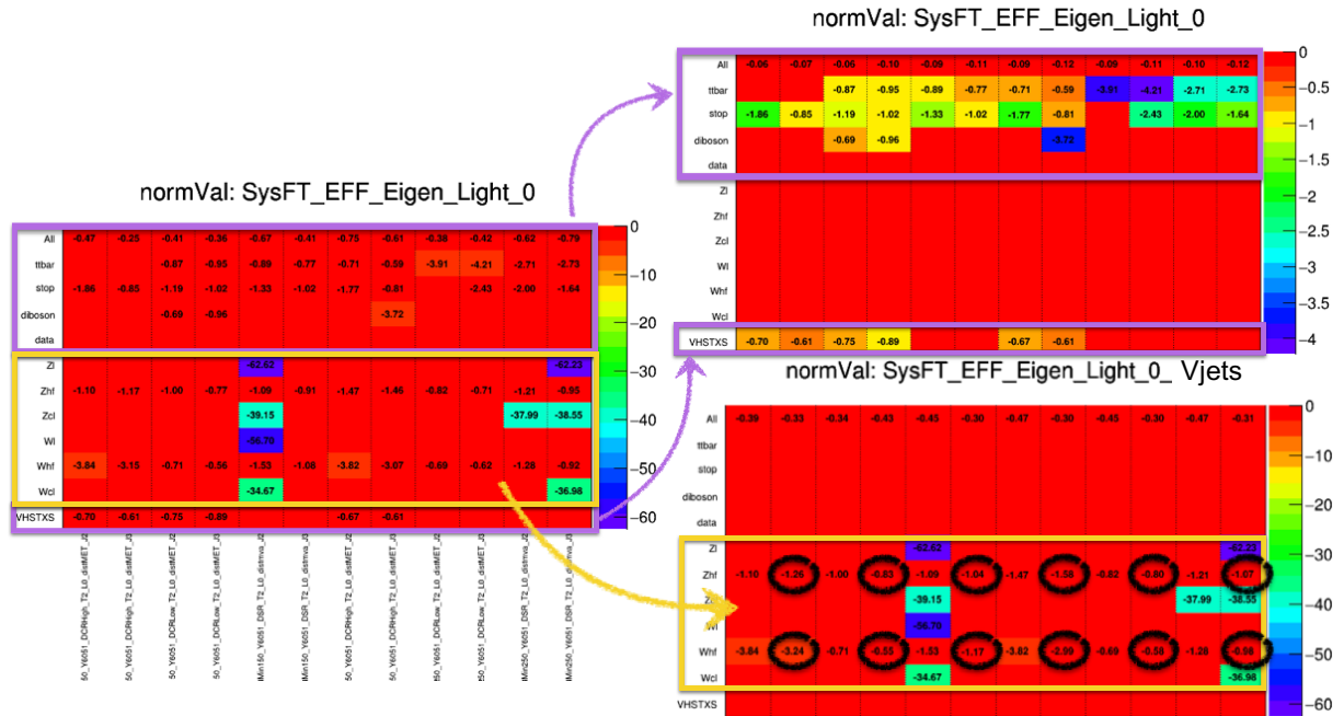
Figure 9.29: Comparison between the NormVal plots of the single bin fit (left - Figure 9.27) and the V+jets decorrelated single bin fit (top right and bottom right). The two sets of NormVal plots on the right are independent. The bottom right plot has the normalisations from all the V+jets samples in Light_0 and the right plot has the rest of the normalisations in Light_0. When compared to the single bin fit, it can be seen that the large majority of the normalisations do not change. The exception to this are the values circled black. These are the 3-jet V+hf normalisations which have all varied by less than one percent.
