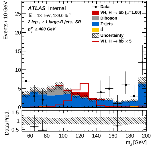
(c) m_J , p_T^V \geq 400 \text{ GeV} , single- \mu trigger
