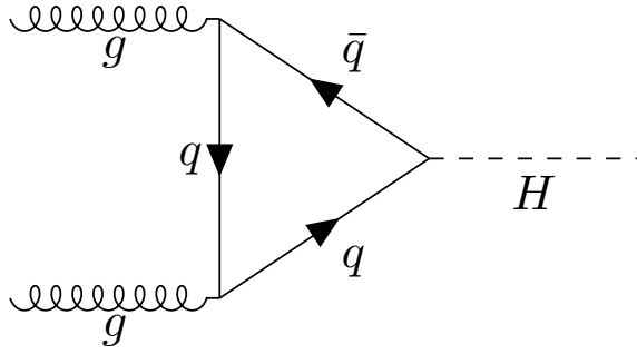
Figure 8.1: Feynman diagram of the Higgs production process with the highest cross-section: gluon-gluon fusion. Theoretically, the loop in the diagram is possible for all quarks, but due to the substantially larger mass of the top quark than the other quarks and the Higgs couples preferentially to heavier particles, the loop mainly consists of top quarks. This process has the highest cross section because at high energies the parton distribution function of the proton is roughly 50% gluons [137, p117] making gluon-gluon interactions the most likely occurrence from colliding protons.
