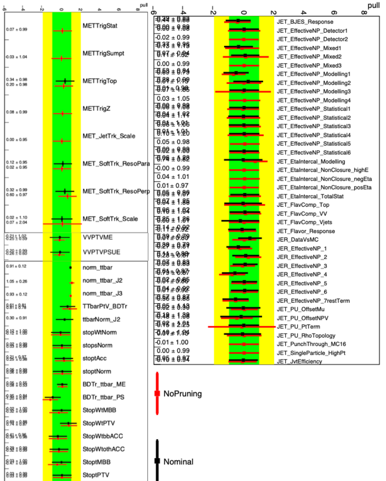
Figure 9.35: Selection of non-flavour tagging pulls from the Nominal OL fit (black) compared to a fit where no systematic are pruned (red). The lack of pruning results in some systematics with small effects now visible. The interesting pulls are those that change or become more or less constrained when pruning is removed.
