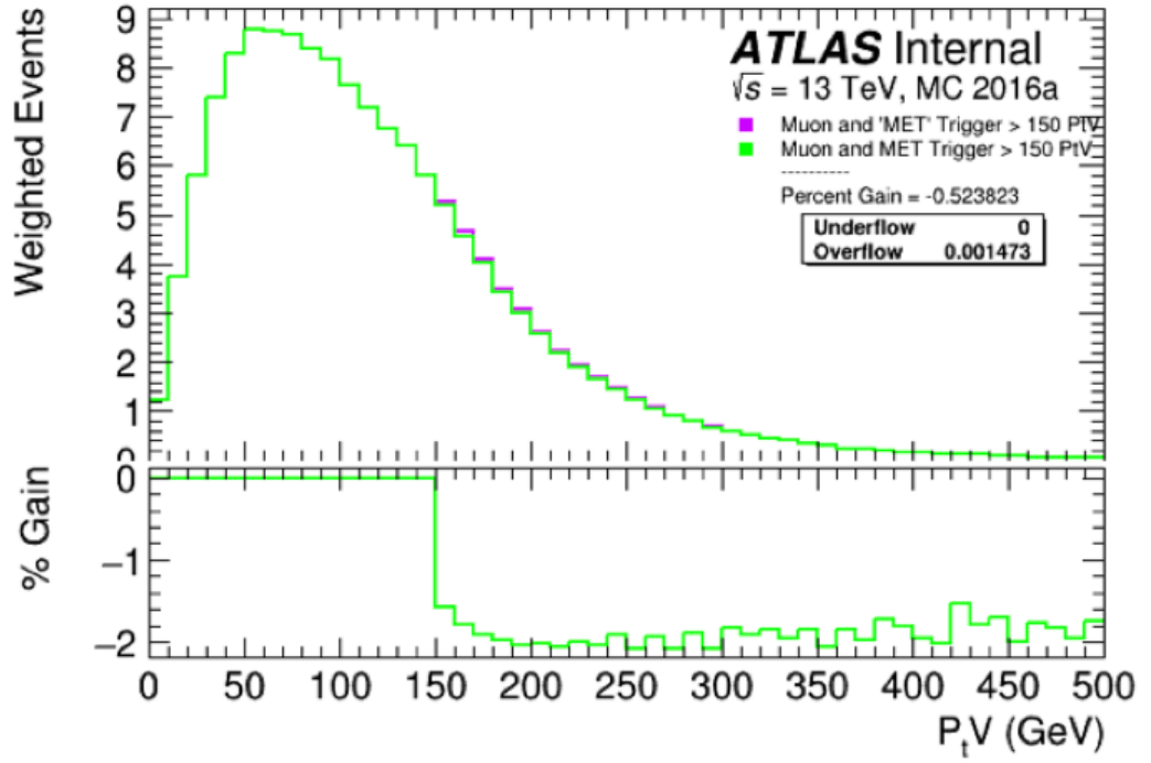
Figure 10.5: Plot showing the difference between the event selection yields when using MET_{dimuon} ('MET') as the trigger proxy, and MET. Here the event selection uses both muon and E_T^{miss} information to filter events.
