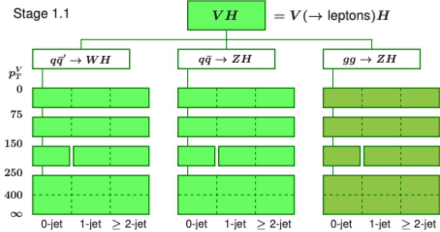
(b) Stage 1.1 STXS Binning
