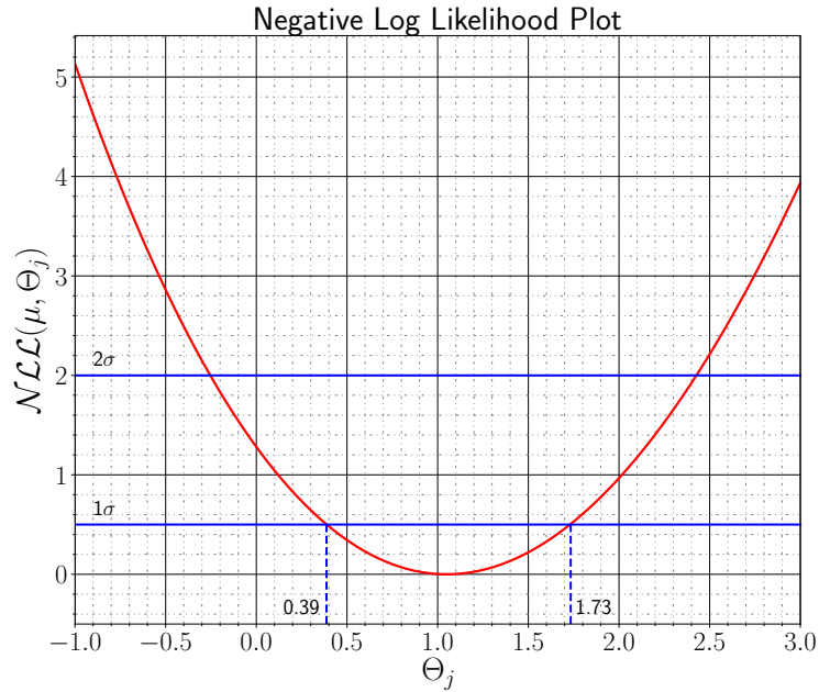
Figure 9.7: Plot showing the variations of the NLL when the systematic \theta_j is varied around nominal pull value. When the NLL changes by +0.5 from the minimum, the pull has varied by \pm 1\sigma . A change of +2 corresponds to a \pm 2\sigma shift.
