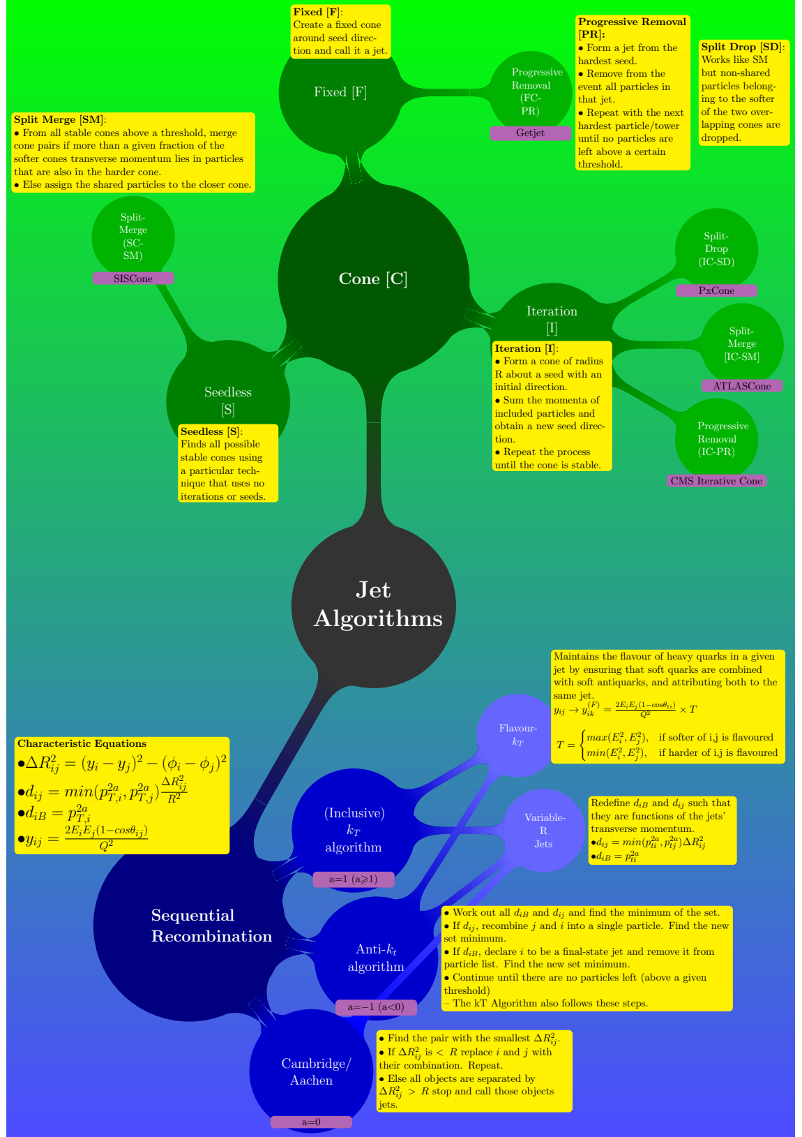
Figure 7.2: A graphic giving a brief overview of the types of jet algorithm that exist. y_i , \phi_i and p_{T,i} are the rapidity, azimuthal angle, and the transverse momentum of the candidate object to be added to the jet; B is the beampipe; R is the radius of the jet cone, and \Delta R_{ij} is the radial distance between the candidate and 'seed' jet object.
