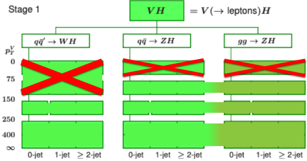
(a) Stage 1 STXS Binning.
