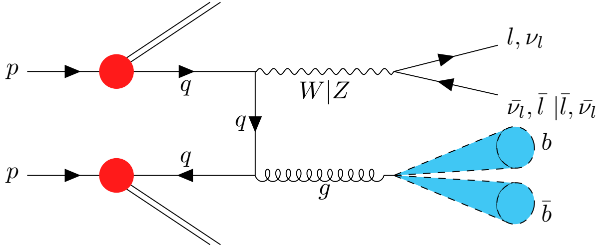
Figure 8.12: Feynman diagram showing how the V+jets process enters the signal region.
