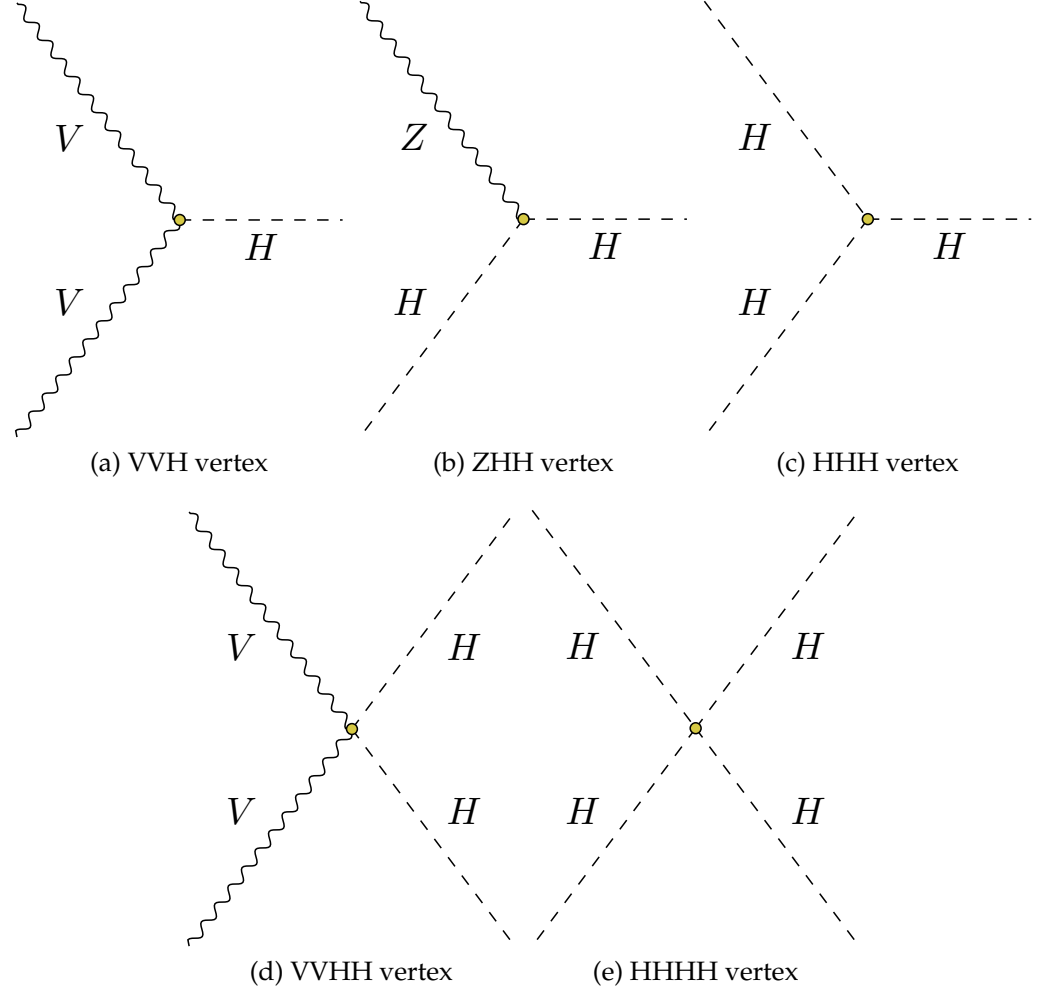
Figure 2.7: Image showing the Feynman vertices introduced to the Standard Model by the addition of a Higgs potential. Here, V generalises both the W -boson and the Z -boson as Vector bosons. In each diagram with a pair of V 's, both species must be the same. The self interaction diagrams are the reasons that the Higgs Boson has mass.
