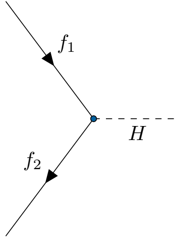
Figure 2.8: Image showing the one Feynman interaction between the Higgs Boson and fermions: the ffH vertex. It is this interaction that gives the fermions their mass and the interaction probability is proportional to the mass of the fermion.
