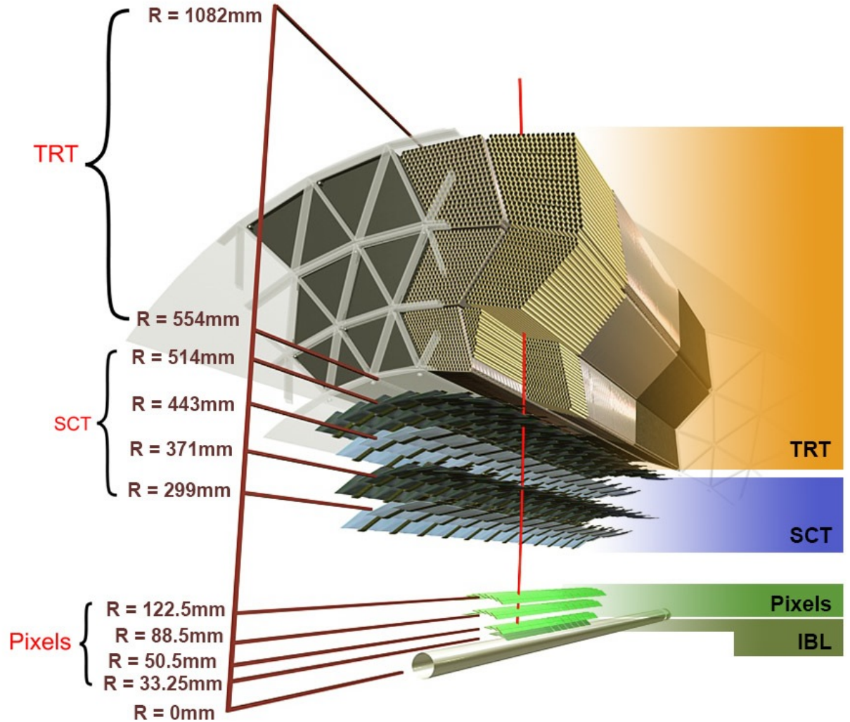
Figure 4.11: Schematic showing a blown up cross-section of the Barrel Inner Tracker System at ATLAS, and the distance each layer of the sub-system is from the beamline. Image from [78].
