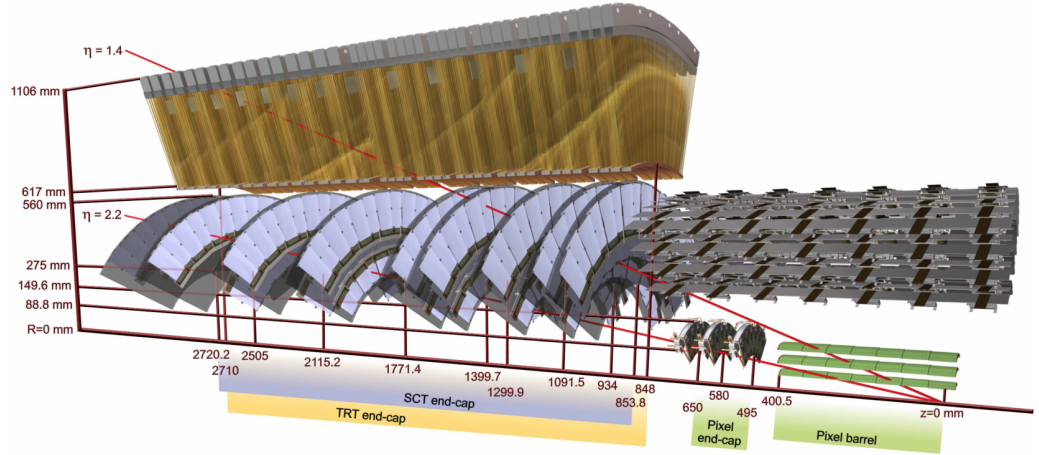
Figure 4.12: Schematic showing a blown up cross-section of the Endcap Inner Tracker System at ATLAS, and the distance each layer of the sub-system is from the beamline. The IBL Image from [69, p56].
