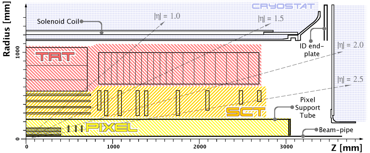
Figure 4.19: Schematic showing the Inner Tracker System at ATLAS. Here the TRT is in Red, the SCT is in orange and the Pixel is in yellow. Image from [54].
