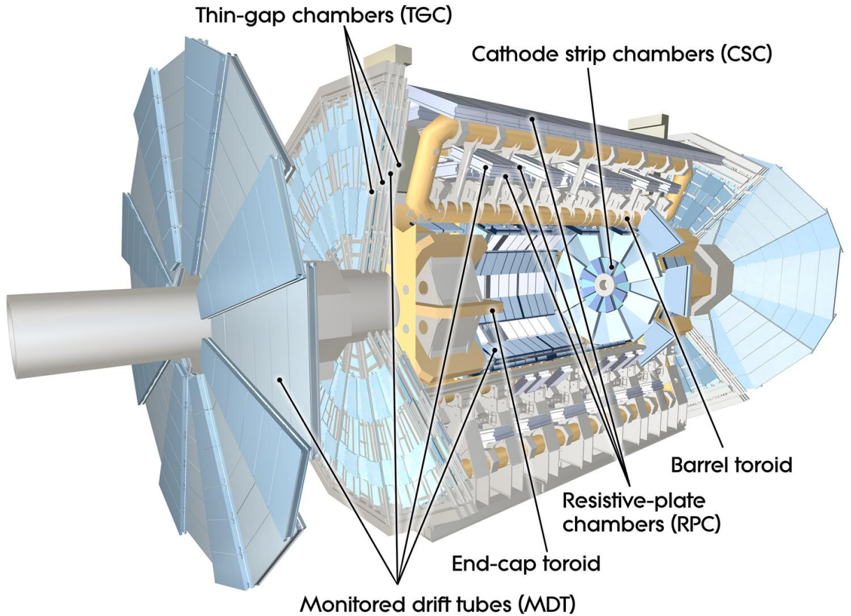
Figure 4.3: Schematic of the ATLAS detector with particular emphasis on the components that make up the Muon Spectrometer. Image from [67].
