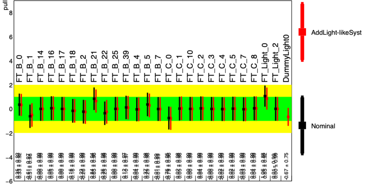
Figure 9.32: Pulls from the Nominal 0L fit (black) compared to a fit where an additional systematic is added (red). This additional systematic is called DummyLight0 and is designed to look to the fit like a more amenable version of the Light_0 pull.
