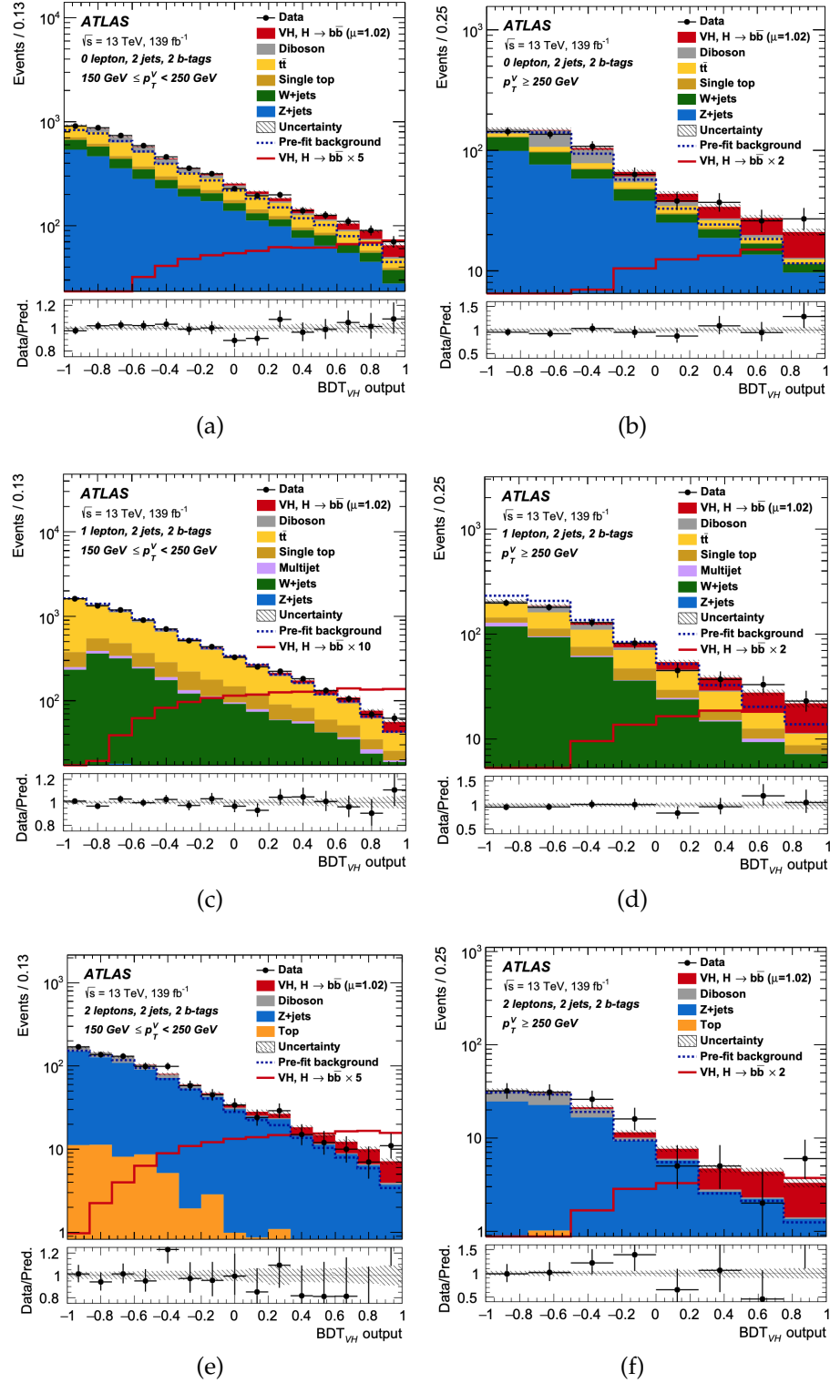
Figure 11.4: Output of the multivariate BDT_{VH} distributions in the (a,b) 0-lepton, (c,d) 1-lepton, and the (e,f) 2-lepton 2-jet, 2-b-tagged jet signal region of the Resolved analysis. The left hand side plots are from the 150 \text{ GeV} \leq p_T^V < 250 \text{ GeV} region and those on the right are from the p_T^V \geq 250 \text{ GeV} region. The predicted background before the fit is marked as a black dashed line. Image from [3, p26].
