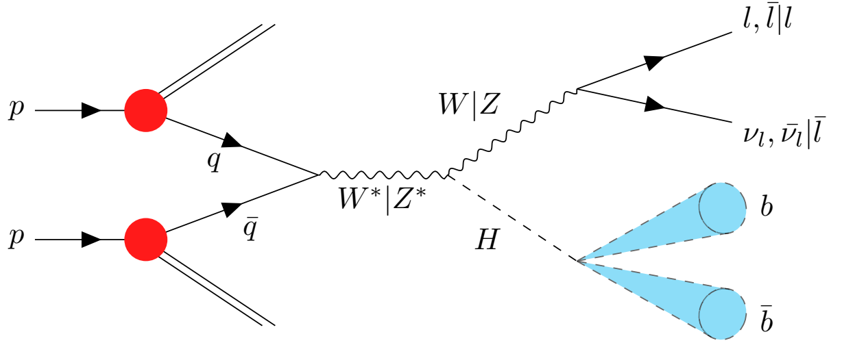
Figure 8.5: Feynman diagram showing the full Higgsstrahlung process of Higgs production at the LHC, and its decay into the final states of interest to the analysis. Gluon initiated (rather than quark) diagrams do exist but they require two additional vertices and are thus rarer.
