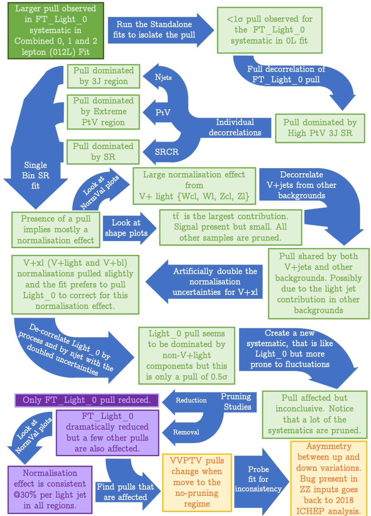
Figure 9.21: Fit study flow chart. Fit tests are represented by blue arrows. The initial observation is in darker green, with later observations pertaining to the editing of the Light_0 systematic in a lighter green. Observations marked in orange and purple represent the study's evolution into pruning tests, and fixing new pulls caused by the new changes, respectively
