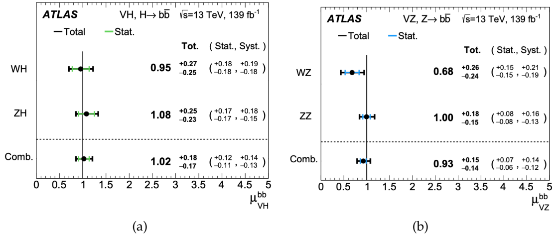
Figure 11.6: (a) Values of \mu_{ZH}^{bb} and \mu_{WH}^{bb} for the Resolved analysis 2-POI fit, and their combined 1-POI value. (b) Values of \mu_{ZZ}^{bb} and \mu_{WZ}^{bb} for the Resolved analysis diboson cross-check fit, and their combined 1-POI value. Images from [3, p27, p30].
