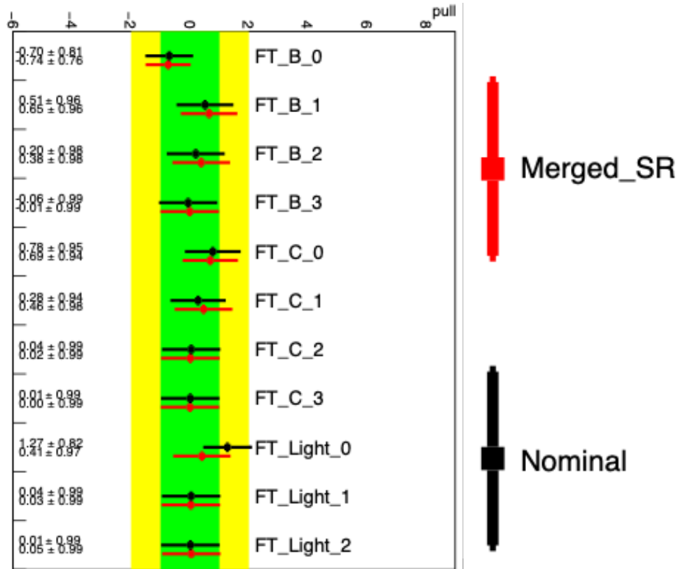
Figure 9.24: Selection of flavour tagging pulls from fits where the control and signal regions are separated (black), and where the signal and control regions are merged (red). In the latter fit the outlying Light_0 pull is reduced to a far more reasonable level.
