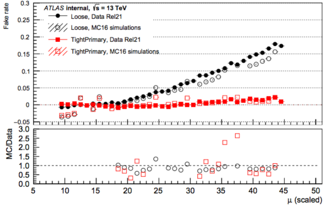
Figure 6.5: Plot of the average number of fake tracks as a function of pile-up for the Loose (in black circles) and TightPrimary (in magenta squares) tracks in Run-2 (2016) data (filled) compared to the equivalent MC simulations events (empty). The ‘fake rate’ is the difference between the points and the line of the respective colour in Figure 6.4 divided by the total number of tracks for that selection.
