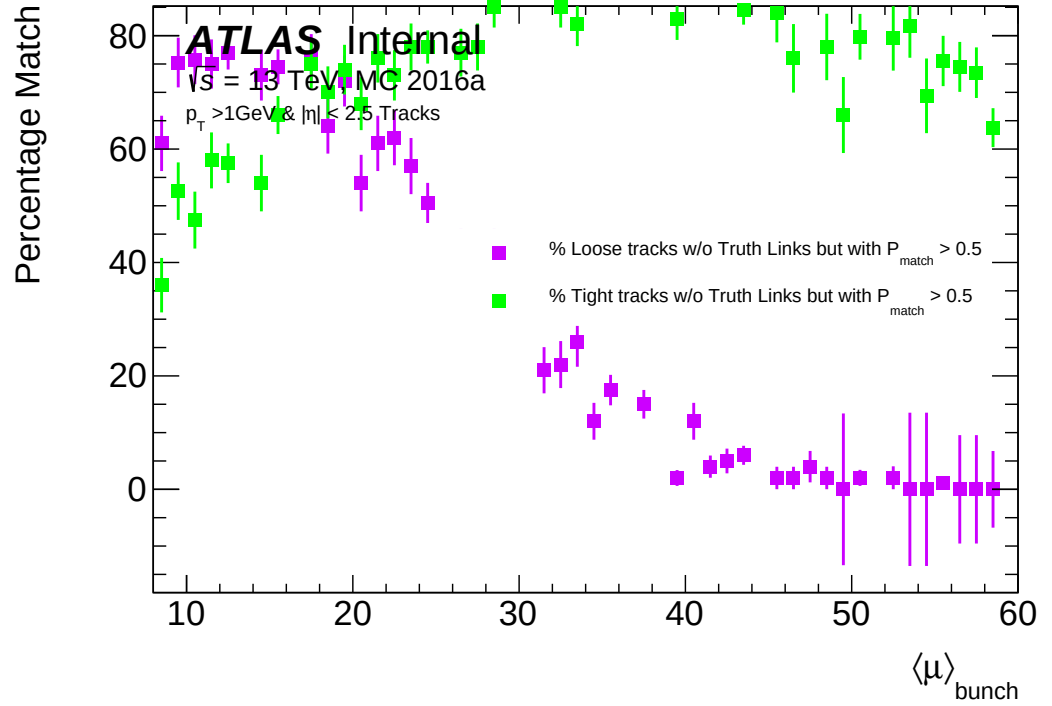
Figure 6.15: Image showing the percentage of tracks of a given selection without truth links but have matching probabilities of greater than 0.5.
