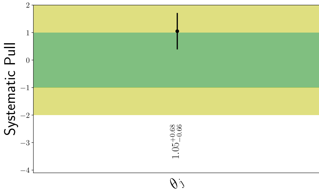
Figure 9.8: Example ‘pull plot’ for \theta_j . Multiple pulls can be shown on such a plot, and the fit produces several of these with pulls common to various processes displayed on the same pull plot.
