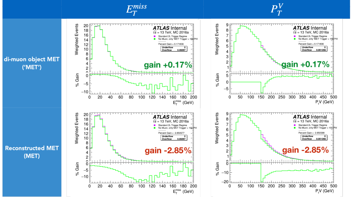
Figure 10.4: Preliminary plots showing the effect of the E_T^{\text{miss}} trigger study in the Resolved 2-lepton analysis. Here only the E_T^{\text{miss}} trigger set is being used to select events. A di-muon object with missing E_T labelled as ('MET') is a stand-in for MET_{\text{dimuon}} . Note that the ratio of new to old trigger regime doesn't change for p_T^V values below 150 GeV as events at these values of p_T^V are not affected by these changes.
