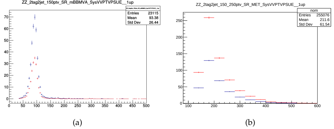
Figure 9.41: Plots of the number of events that correspond to the 1\sigma upward fluctuation of the systematic ZZPTVPSUE in the previous (a) and current analysis (b). In (a), the nominal distribution is in red, and the upward fluctuation is in blue. In (b), the nominal distribution is in blue, and the upward fluctuation is in red. In both analyses, there seems to be double the number of events expected in the upwards fluctuation.
