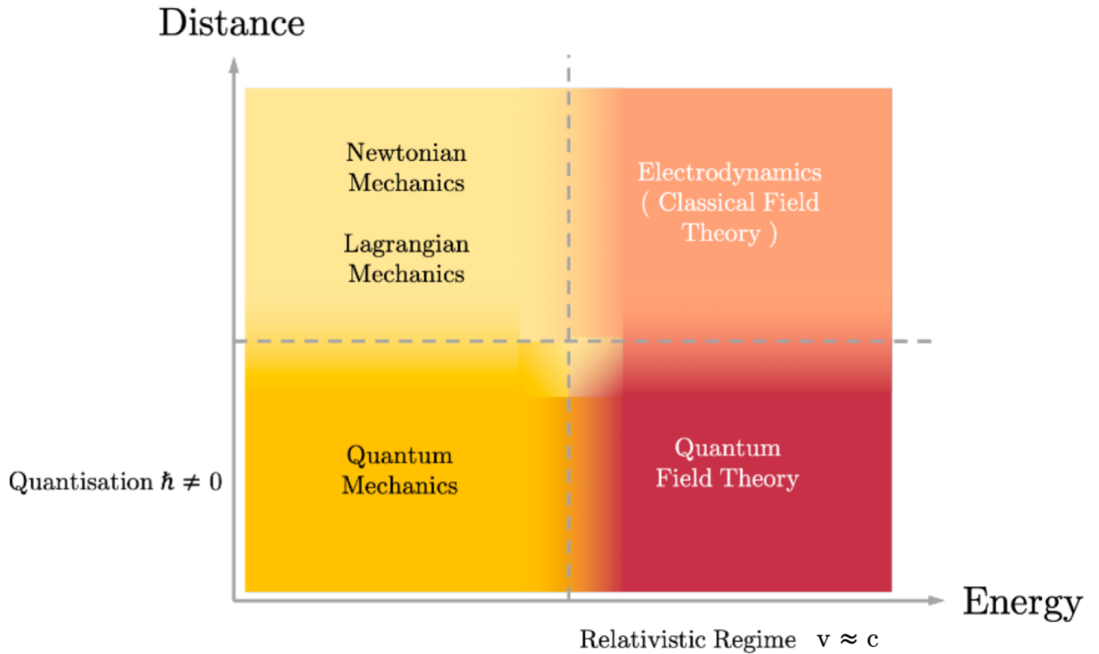
Figure 2.1: Picture showing the rough scales at which certain theories are valid. At small distances the description moves from particle having any energy to energy coming in small packets called quanta. This 'quantisation' comes with a constant. At large energies, particles travel closer to the cosmic speed limit - the speed of light and theories need to be compatible with Einstein's Special Relativity.
