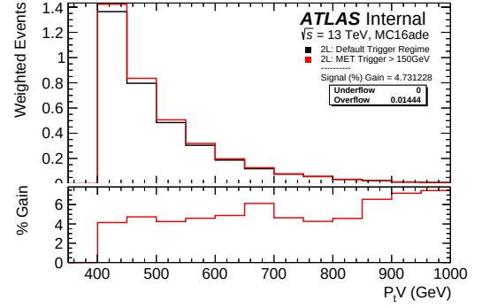
(b) Signal yield increase: 4.73%, 250 \text{ GeV} \leq p_T^V < 400 \text{ GeV}
