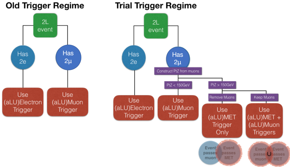
Figure 10.2: Graphic showing differences between the new and the older trigger regime. ALU stands for Add Lowest Unprescaled triggers. Two options are presented here for the analysis for after the point where the E_T^{\text{miss}} triggers start to become 100% efficient. One with both the muon and the E_T^{\text{miss}} triggers active on the same events and one where the E_T^{\text{miss}} triggers alone are implemented.
