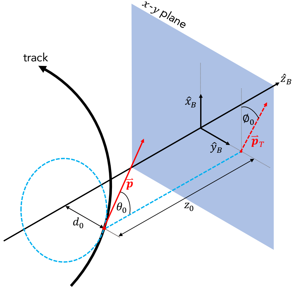
Figure 6.2: Pictorial definition of the parameters that make up a track at the ATLAS detector. All of the parameters are defined with respect to a perigee surface, shown here in blue. The transverse momentum ( \vec{p}_T ) is the 2-D projection of the total momentum of the track ( \vec{p} ) at the distance of closest approach onto the perigee surface. The B subscript on the axis directions refers to the beam, which travels in the z -direction.
