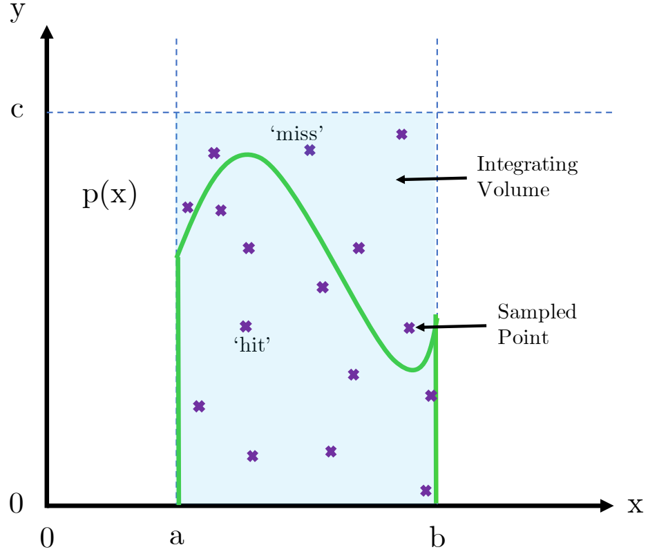
Figure 5.1: Diagram showing how the Monte Carlo Integration method is used to evaluate the integral of p(x) between the points 'a' and 'b'. The integrating volume is given by the area between the points a and b on the x-axis extended up to the line y = c . Points are randomly sampled in [x, y] and those that are less than p(x) are called 'hits' while those that are larger than p(x) are called 'misses'.
