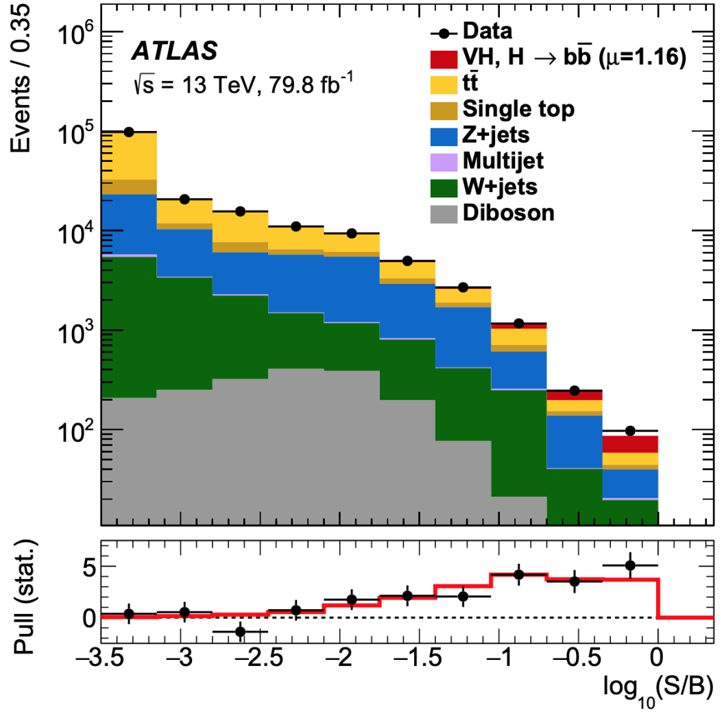
Figure 8.7: Event yield as a function of \log_{10}(S/B) for data, background, and a 125 GeV Higgs boson signal. The final BDT_{VH} discriminants from all the analysis regions are combined into bins of \log_{10}(S/B) where S and B are the fitted signal and background yields respectively. The 125 GeV Higgs boson signal is shown as a red filled histogram on top of the fitted backgrounds but is normalised to the \mu extracted from the data (1.16). The lower panel shows the statistical significance (pull) of the difference between the data and the fitted background-only model. The points show the observed pulls and the red line is the expected pulls. The vertical error bars on the points are statistical uncertainties only.
