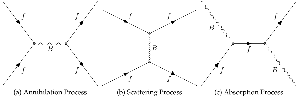
Figure 2.2: Images showing the three different kinds of 2-2 processes as depicted by basic Feynman diagrams. Fermions are depicted as straight continuous lines, and all other types of lines (wavy, curly or dashed) depict a boson of some description. If the y-axis represents spatial separation and the x-axis represents time, vertices occur when particles interact via collisions ( 2 \rightarrow 1 lines) or decays ( 1 \rightarrow 2 lines). The left annihilation diagram shows two fermion particles merging into a boson which then decays into two fermions. The central scattering diagram shows two particles approaching one another, exchanging a boson and then drifting apart. The right absorption diagram depicts a fermion absorbing a boson and then emitting another boson later. The combinations of fermions and bosons ( fff , ffb , fBB , BBB ) that can meet at vertices are limited by the theory the diagram is trying to describe.
