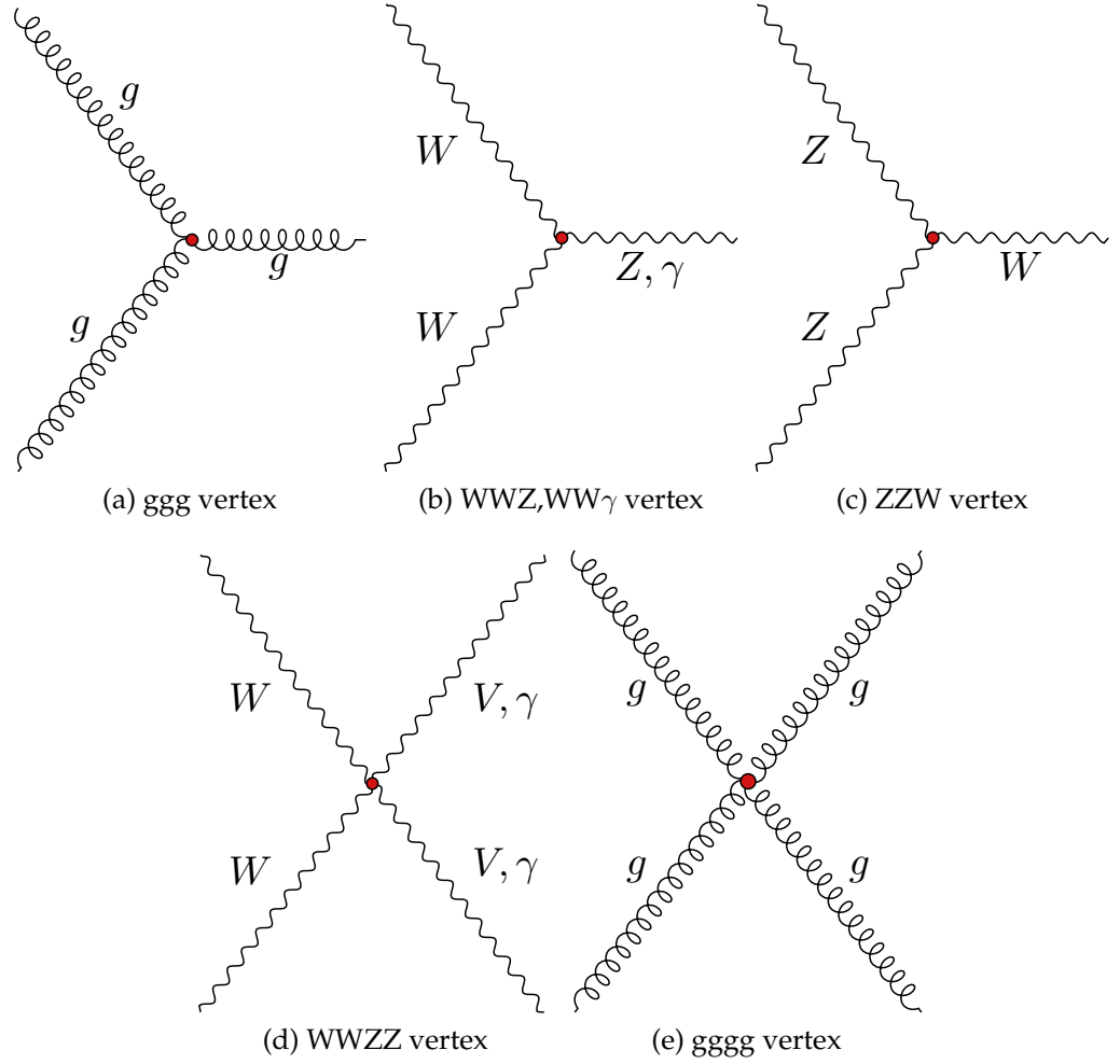
Figure 2.5: Image showing the self interaction vertices for the gauge bosons post symmetry-breaking. Since F_{\mu\nu} = \partial_\mu A_\nu - \partial_\nu A_\mu + gf^* A_\mu A_\nu [23, p509], for a group to be non-Abelian, f^* must be non-zero. Since the term in the Standard Model Lagrangian is essentially the square of this, and each A_\mu represents a bosonic field, in addition to the three point vertices, there are also the four point vertices: gggg and WWZZ.
