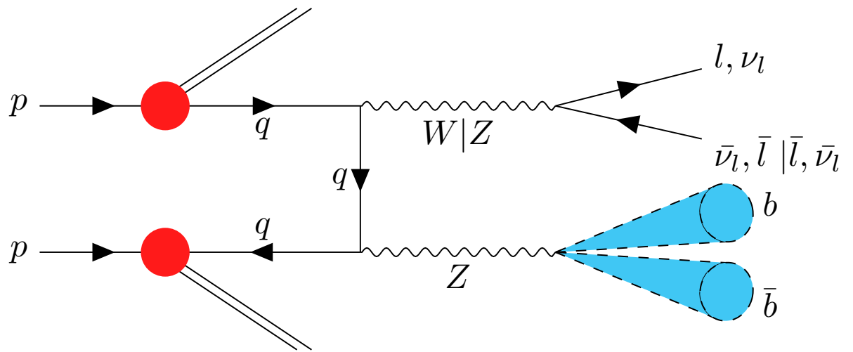
Figure 8.16: Feynman diagram of the two leading diboson contributions to the background.
