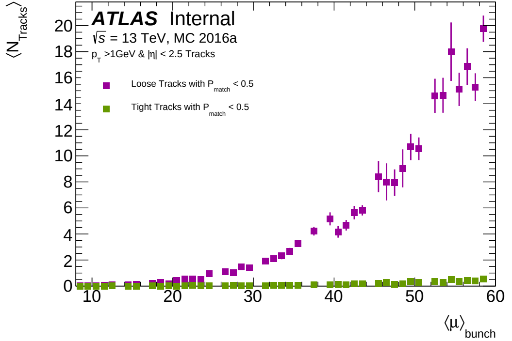
Figure 6.14: Loose and TightPrimary that have P_{\text{match}} < 0.5 . It is important to note that the failure rate for the Loose selection increases non-linearly. At high \mu there are roughly 20 tracks failing this requirement. This is about 8% of the 250 tracks seen in Figure 6.13a.
