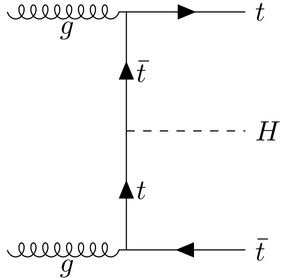
Figure 8.4: Feynman diagram of production of a Higgs boson produced alongside a pair of top quarks. Theoretically, this diagram is possible for all quarks, but due to the substantially larger mass of the top quark relative to the other quarks, this specific process has the only relevant cross-section.
