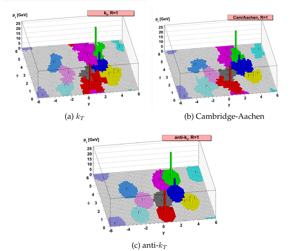
Figure 7.3: Three sequential combination algorithms run on a sample event with many soft particles added. This is designed to illustrate one of the properties of the jet: the catchment areas of the hard jets. The shapes in the k_T and Cambridge-Aachen algorithms are partially determined by the specific set of soft particles added, making anti- k_T the ideal algorithm. Images taken from [127, p4].
