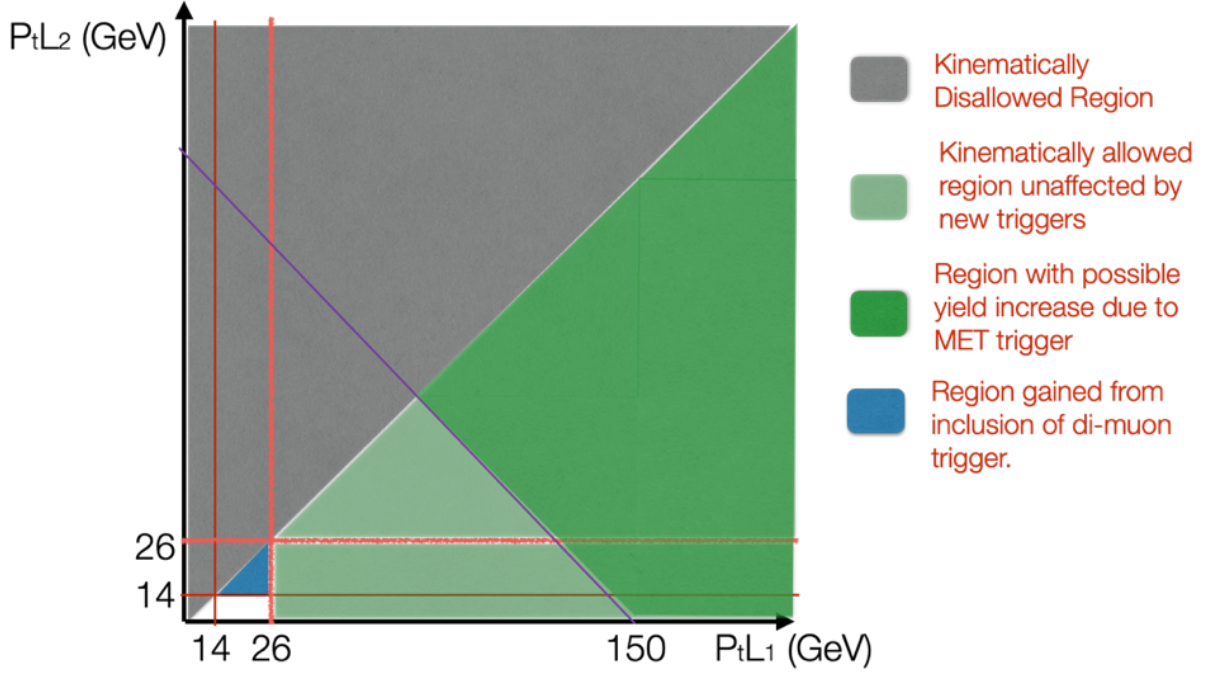
Figure 10.1: Graphic showing possible event yields differences with the introduction of certain triggers into the event selection. The x -axis denotes the energy of the leading lepton, and the y -axis shows the energy of the sub-leading lepton. The orange lines correspond to the lowest energy threshold of the current single lepton trigger. The addition of a dimuon trigger lowers the energy threshold of the leading lepton (to the red lines) and allows access to the blue region not yet considered by the analysis. The inclusion of a E_T^{\text{miss}} trigger would increase the likelihood an event passes a trigger at whatever point the E_T^{\text{miss}} trigger is active. Since the E_T^{\text{miss}} trigger is close to fully efficient at p_T^V \leq 150 GeV, the E_T^{\text{miss}} trigger will only be active in the analysis from this point. Here p_T^V \sim P_{tL1} + P_{tL2} and hence the kinematically-allowed region above the purple line P_{tL1} + P_{tL2} = 150 GeV could see an increase in events (shown in dark green).
