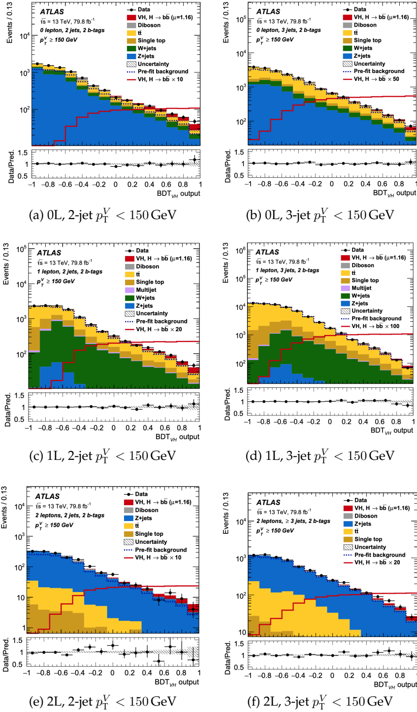
Figure 8.6: BDT_{VH} post-fitting output distributions for the 0-lepton (top), 1-lepton (middle) and 2-lepton (bottom) channels, in the 2-jet (left) and 3-jet (or \geq 3 jets for the 2-lepton case) (right) categories in the p_T^V < 150 GeV region. The background contributions are shown as coloured filled histograms which each contribution having its own colour. The 125 GeV Higgs boson signal is shown as both a red filled histogram on top of the fitted backgrounds but is normalised to the \mu extracted from the data (1.16), and unstacked as a red line, scaled by a factor, which is indicated in the legend. The dashed line shows the total level of the pre-fit background. The hashed region in each bin indicates the total size of the statistical and systematic uncertainties for the fitted signal and background. The ratio of the data to the sum of the fitted signal and background is shown in the lower panel.
