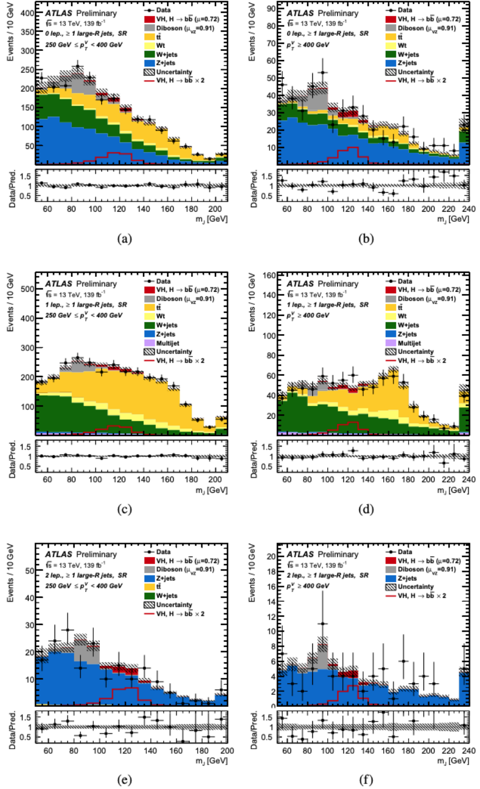
Figure 11.1: Mass distributions of the large- R jet in the (a,b) 0-lepton, (c,d) 1-lepton, and the (e,f) 2-lepton 2- b -tagged jet signal regions. The left hand side plots are from the 250 \text{ GeV} \leq p_T^V < 400 \text{ GeV} region and those on the right are from the p_T^V \geq 400 \text{ GeV} region. In this plot the Low and High purity sub-regions in the 0- and 1-lepton regions have been merged. Image from [4, p14].
