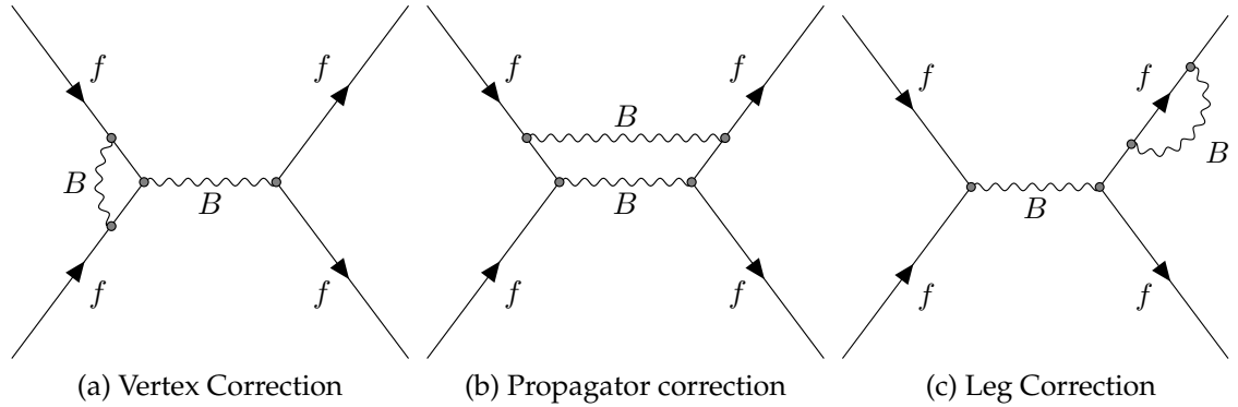
Figure 2.3: Feynman diagrams showing the three different kinds of corrections to a 2-2 annihilation processes that can occur. All of these processes have four vertices as opposed to 3. All the correction diagrams that have three vertices would change the number of input or output particles and describe a different process.
