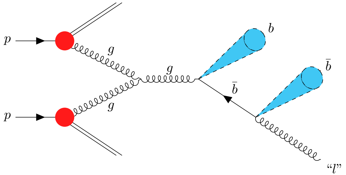
Figure 8.15: Multi-jet background example Feynman diagram. Here a gluon emission from a jet has been misidentified by the detector as a lepton.
