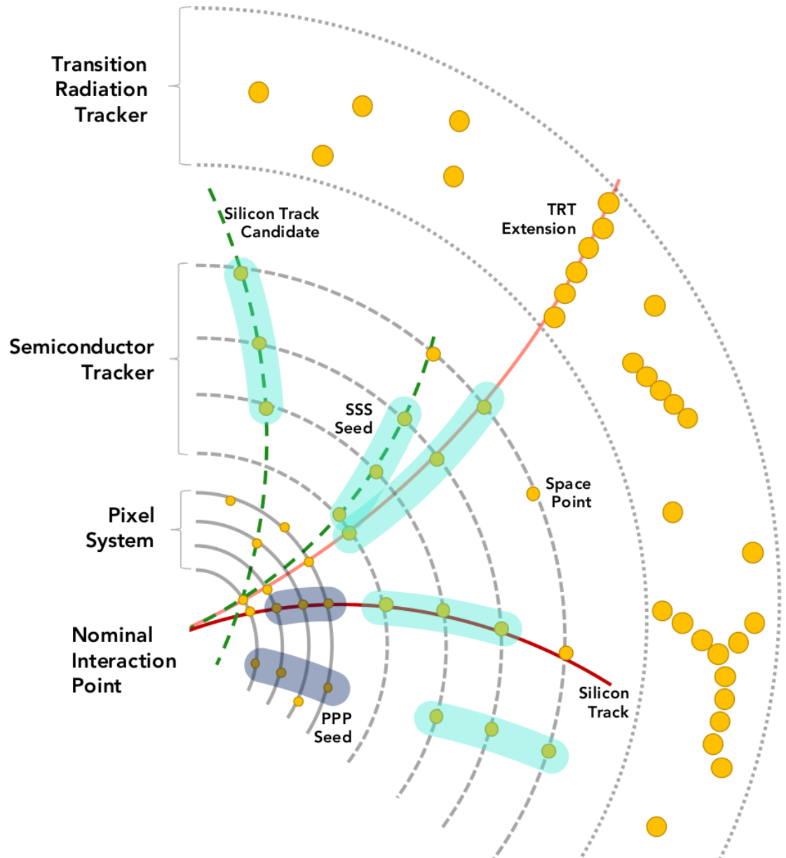
Figure 6.1: Image showing the different objects that are formed while creating tracks at the ATLAS experiment. Charged particle interactions with detector components induce electrical signals which in turn inform the position of this interaction. This information is contained within space points, shown as yellow points. These points are combined to form track ‘seeds’ which are cyan if they are formed in the Semiconductor Tracker (SSS seeds); and navy blue if they are formed in the Pixel system (PPP seeds). The momentum information from the seeds is then extended to find other points that lie on this to form silicon track candidates (shown in dashed green). The third track going clockwise shows the tracks are then extended into the TRT to see if they align with TRT deposits. Track candidates that fulfil further quality requirements become tracks, shown in red. The lighter red track has one pixel ‘hole’ and one SCT ‘hole’ so passes loose track requirements, and the darker red track has hits in every layer, so passes the tight track requirement. The two track candidates left in the diagram do not become actual tracks because they either miss the nominal interaction point when extended, or do not have any unique space points attributed to the track in the pixel system.
