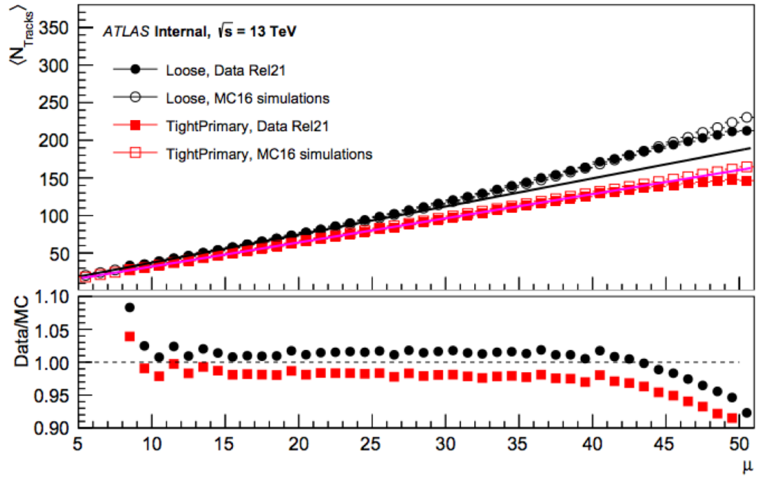
Figure 6.4: Plot of the average number of tracks as a function of pile-up for the Loose (in black circles) and TightPrimary (in magenta squares) tracks in Run 2 2016 data (filled) compared to the equivalent MC simulations events (empty). The solid lines represent extrapolations of a linear fit to MC simulations seeded between 9 \leq \mu \leq 16 .
