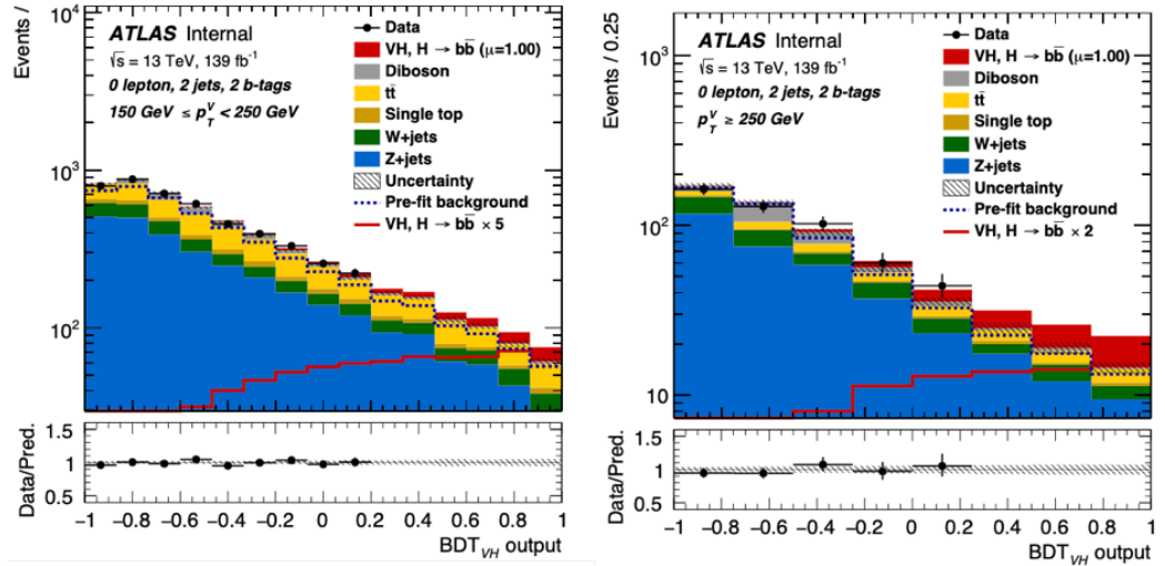
Figure 9.19: Example post-fit plots from the 0L standalone fit. The 150 \text{ GeV} \leq p_T^V < 250 \text{ GeV} region is on the left and the p_T^V \geq 250 \text{ GeV} region is on the right. These plots were taken when the fit was blinded, so the most sensitive bins in the fit have no data points in them.
