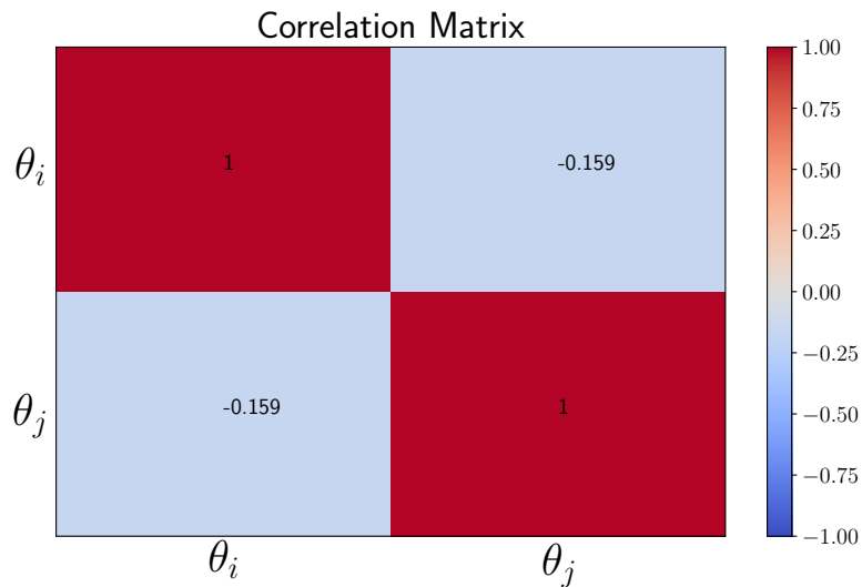
Figure 9.15: Correlation matrix for \theta_i and \theta_j . Since a variable is always perfectly correlated with itself, the leading diagonal will always be unity. \theta_i and \theta_j have a slight anti-correlation.
