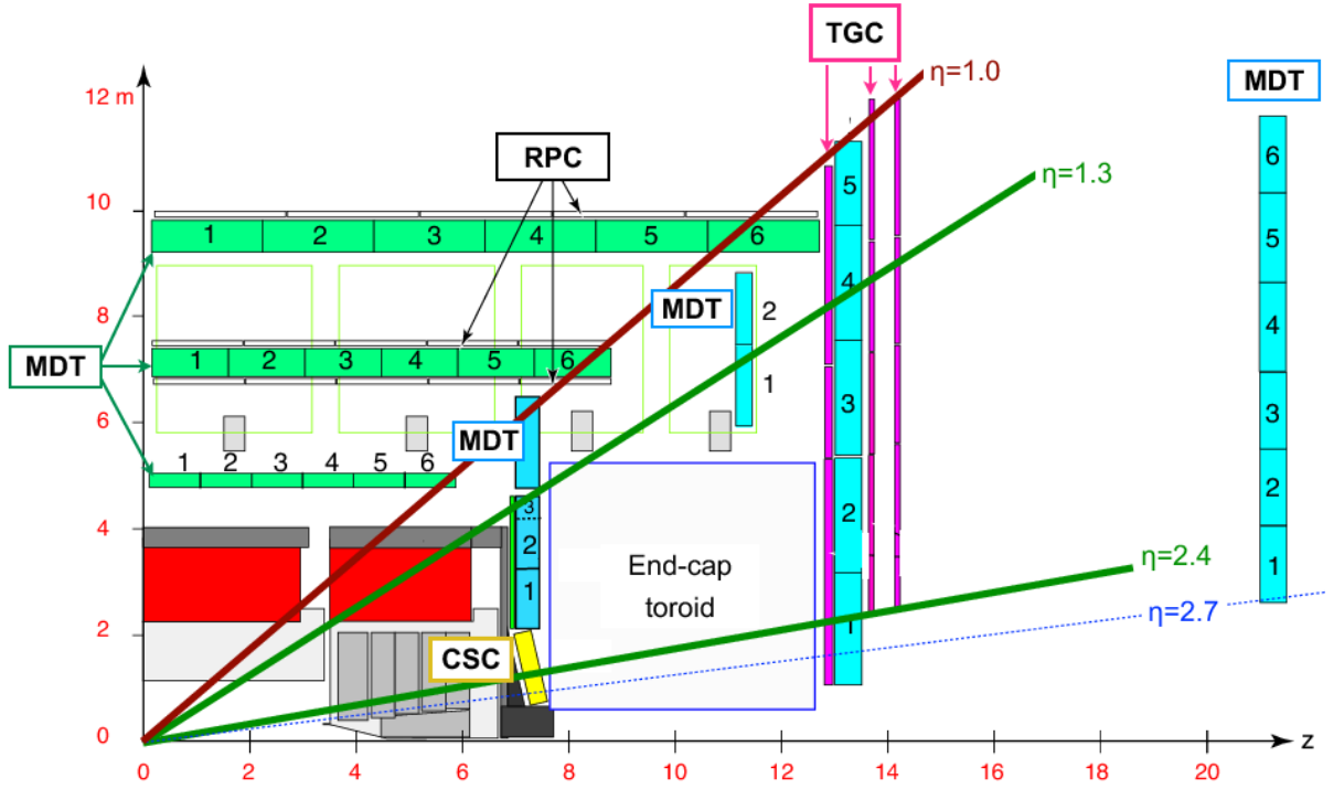
Figure 4.5: Schematic of the Muon Spectrometer showing how the MS was designed such that particles passing through it will interact with at least three chambers. Image from [70].
