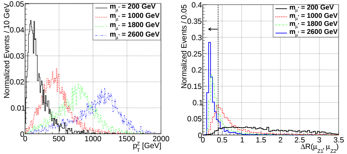
(c) p_T -distribution of the Z-boson (d) \Delta R between the two muons from the Z decay
