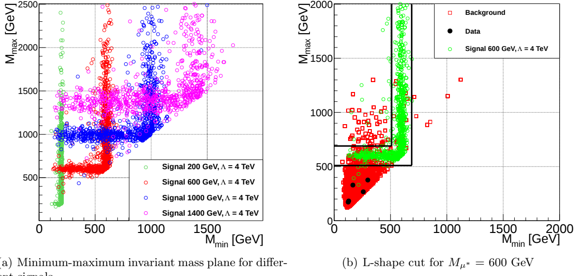
Figure 8.1.: Two-dimensional minimum-maximum invariant mass plane (a) for different signal masses (Gen-Level in Fig. 7.1) and (b) for the "L-shape" cut of M_{\mu^*} = 600 GeV after applying the full selection. The histogram includes 5 data points, the two on the bottom-left are close to each other.
