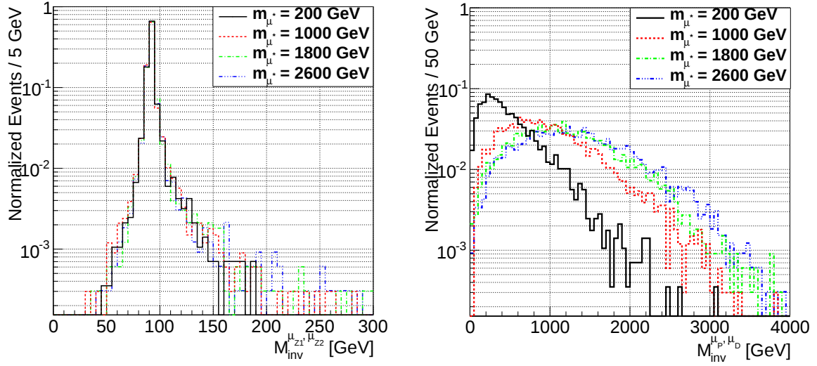
(a) Reconstructed Z-boson mass from the two muons \mu_{Z1} and \mu_{Z2} (b) Reconstructed mass from the two muons \mu_{\text{partner}} and \mu_{\text{decay}}
