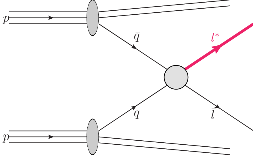
Figure 3.1.: Single excited lepton production together with a Standard Model lepton via contact interaction.
