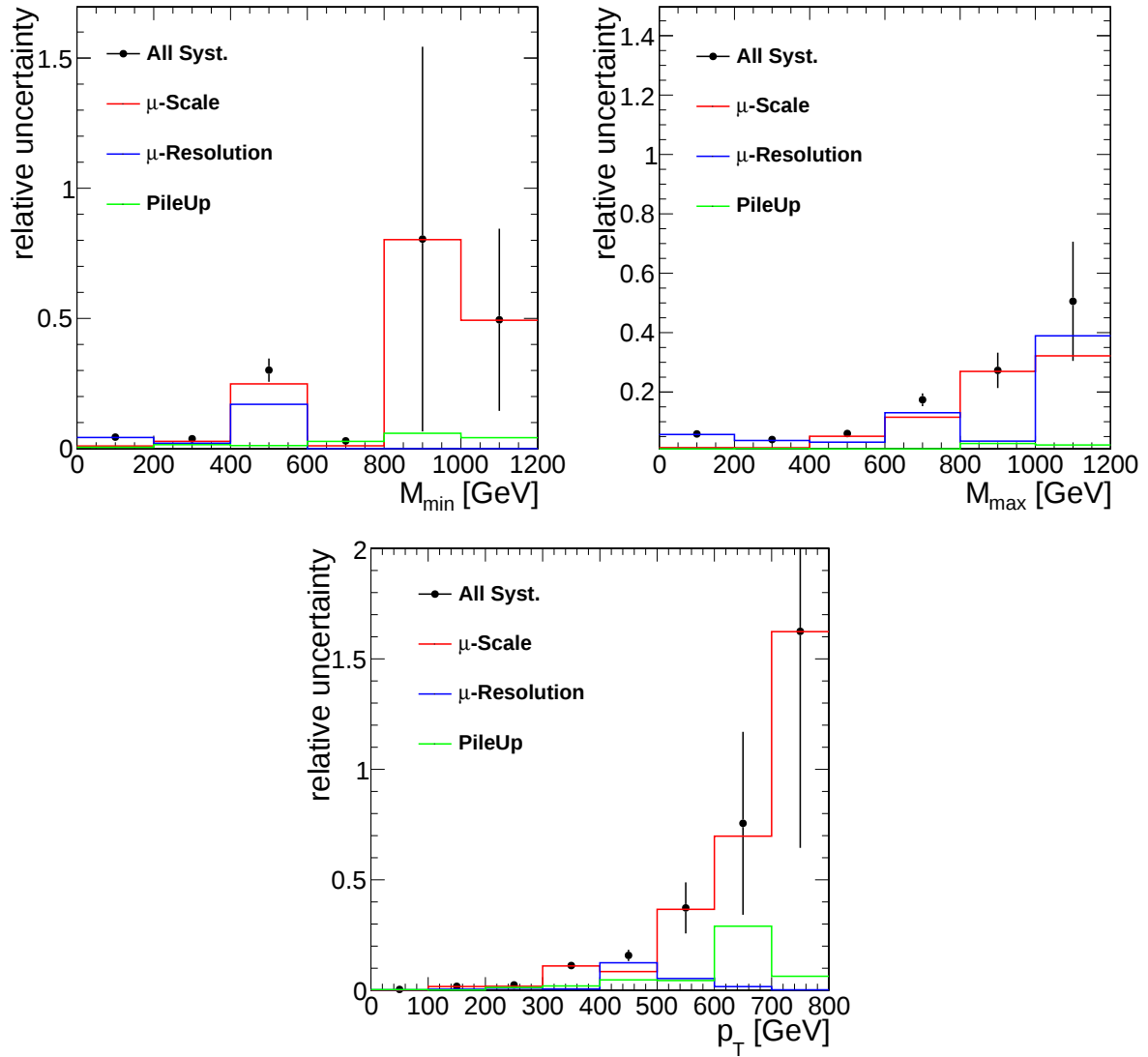
Figure 7.15.: Relative systematic uncertainties on the background expectation for pileup reweighting, muon momentum scale and muon momentum resolution. Top left: M_{\min} -distribution; Top right: M_{\max} -distribution; Bottom: p_T -distribution.
