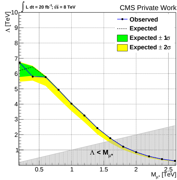
(b) Limit on the compositeness scale \Lambda
