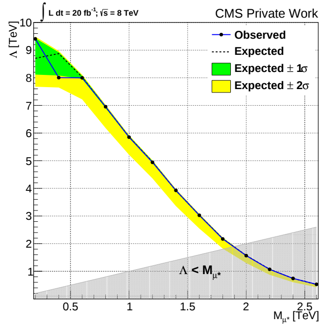
(b) Limit on the compositeness scale \Lambda
