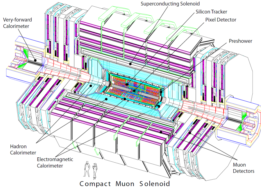
Figure 4.2.: Schematic view of the CMS detector, taken from [33].
