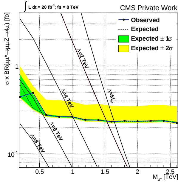
(a) Cross section limit
