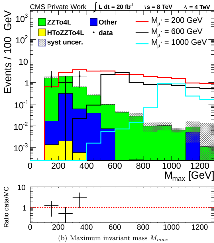
Figure 7.12.: Minimum and maximum invariant mass distribution after applying all the cuts. The uncertainty bands include muon scale, muon resolution and pileup uncertainties, but no uncertainties on the cross section and luminosity.
