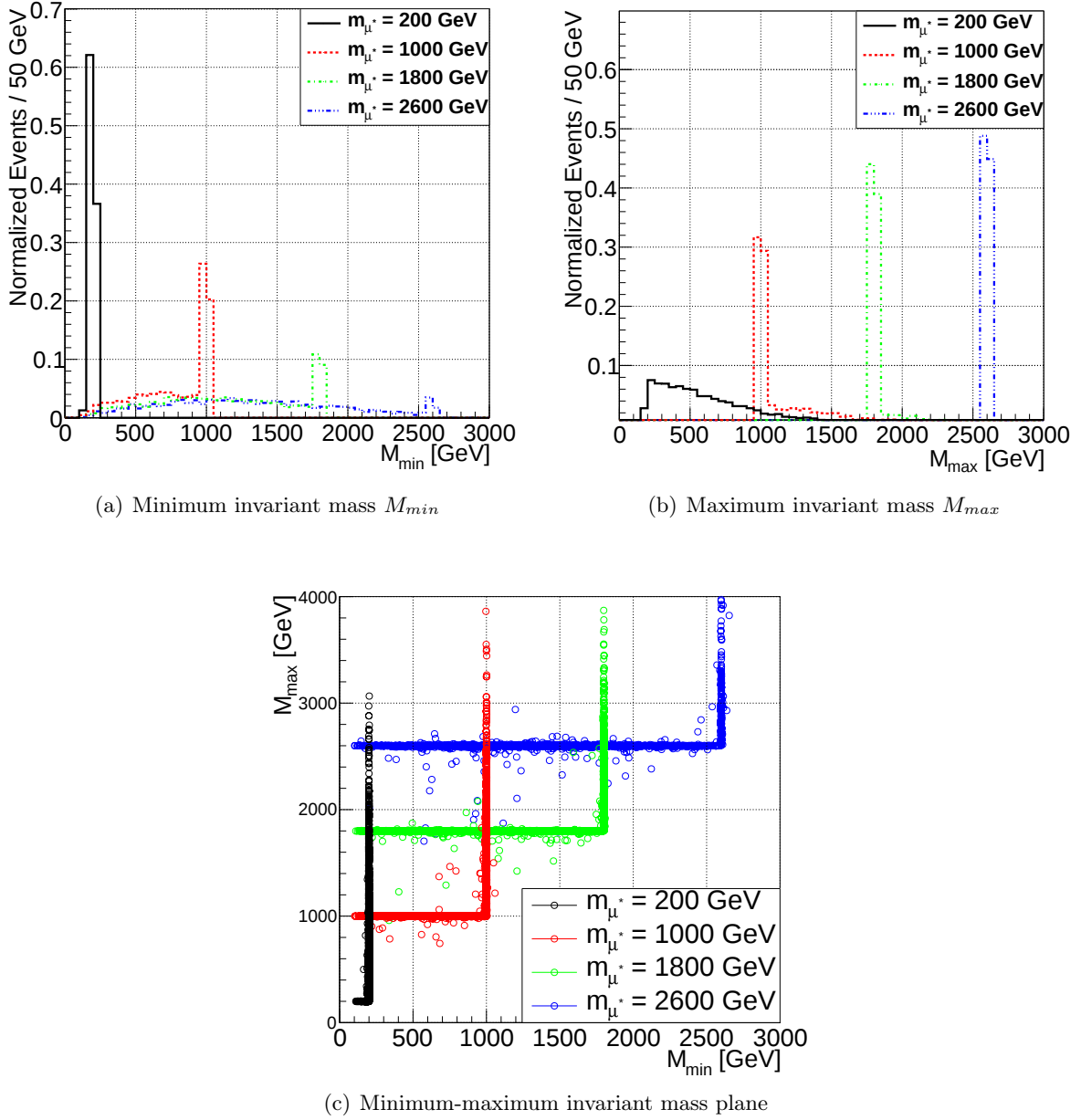
Figure 7.1.: Invariant mass plots on generator level for different \mu^* -masses: (a) Minimum invariant mass M_{min} ; (b) Maximum invariant mass M_{max} ; (c) 2-dimensional minimum-maximum invariant mass plane, also called "L-shape" diagram.
