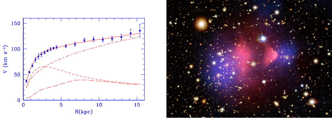
Figure 2.2: Evidences of the DM. (left) The rotation velocity of the galaxy M33 as a function of the distance from the center of the galaxy [38]. The points show the observed M33 rotation curve with the best fit model (solid line). The contribution of the halo (dashed-dotted line), stellar disk (short dashed line) and gas (long dashed line) are shown together. (right) Image of Bullet Cluster 1E0657-558 [39]. Image of the bullet cluster observed by X-ray is shown in red and the cluster observed by gravitational lensing effect is shown in blue.
