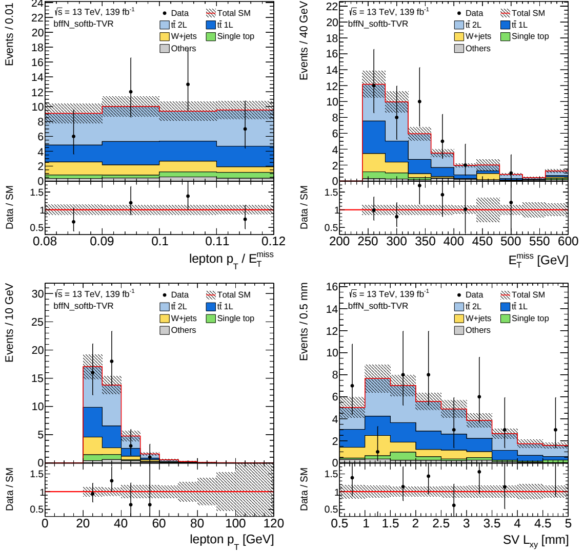
Figure 9.9: Comparison of data and simulation for the t\bar{t} VR after applying the normalization factors: (top left) the p_T^\ell / E_T^{\text{miss}} , (top right) E_T^{\text{miss}} , (bottom left) lepton p_T , and (bottom right) soft b -tag SV L_{xy} . Statistical and experimental uncertainties are displayed. The last bin includes the overflow.
