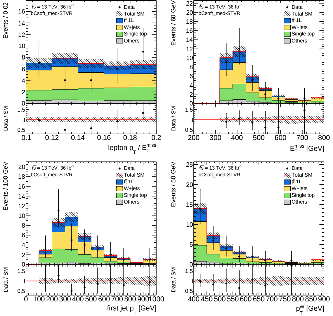
Figure 7.12: Comparison of data and simulation distributions for the single top VR after applying the normalization factors: the p_T^\ell/E_T^{\text{miss}} (top left), E_T^{\text{miss}} (top right), leading jet p_T (bottom left), and p_T^W (bottom right). The statistical and experimental uncertainties are displayed. The last bin includes the overflow.
