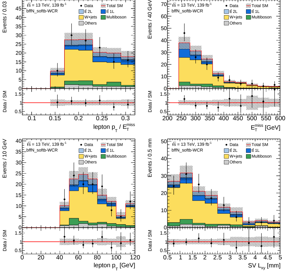
Figure 9.8: Comparison of data and simulation for the W +jets CR after applying the normalization factors: (top left) the p_T^\ell/E_T^{\text{miss}} , (top right) E_T^{\text{miss}} , (bottom left) lepton p_T , and (bottom right) soft b -tag SV L_{xy} . Statistical and experimental uncertainties are displayed. The last bin includes the overflow.
