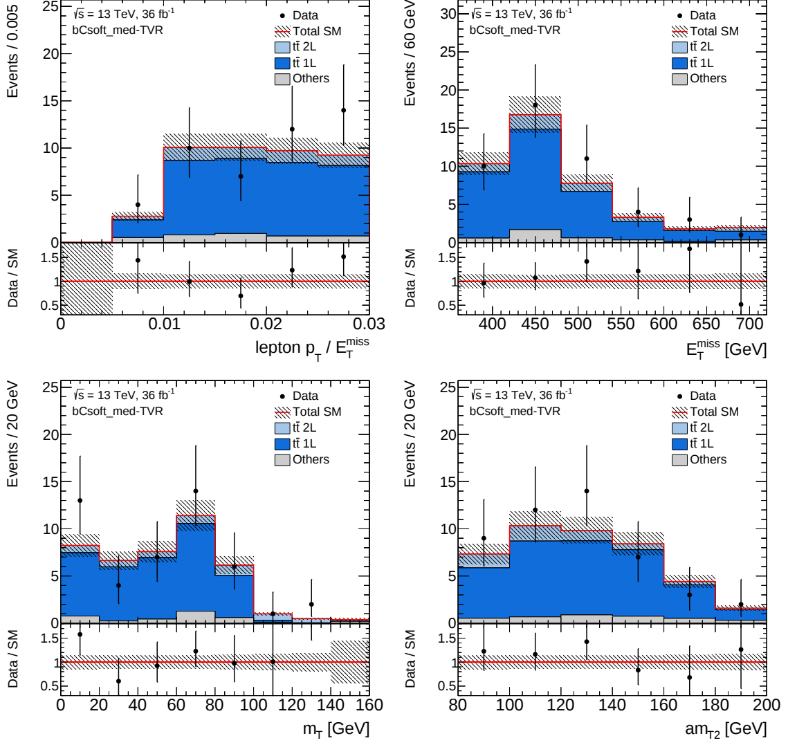
Figure 7.10: Comparison of data and simulation distributions for the t\bar{t} VR after applying the normalization factors: the p_T^\ell / E_T^{\text{miss}} (top left), E_T^{\text{miss}} (top right), m_T (bottom left), and am_{T2} (bottom right). The statistical and experimental uncertainties are displayed. The last bin includes the overflow.
