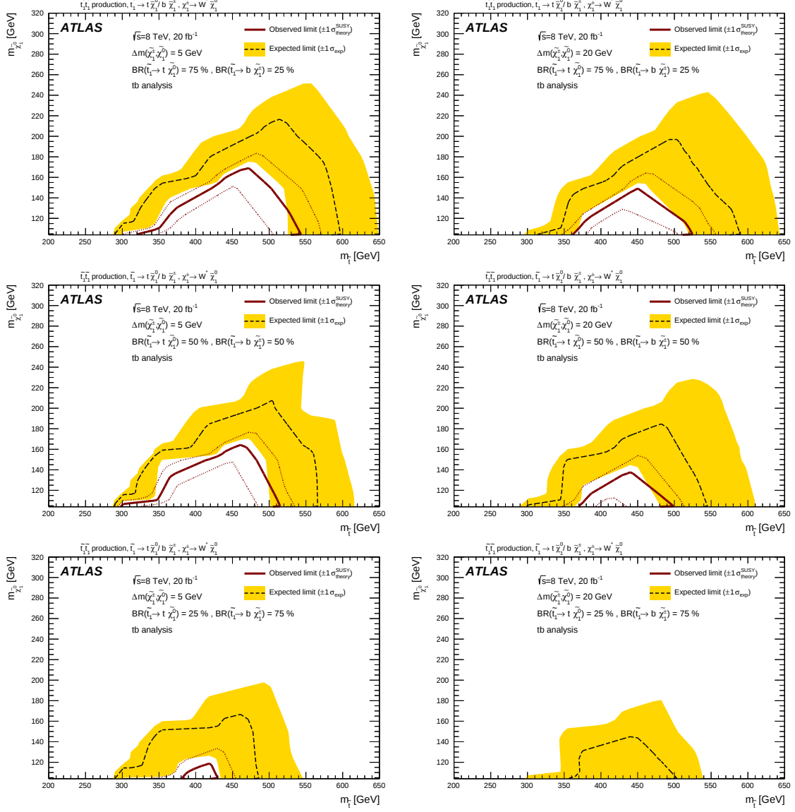
Figure 6.10: Exclusion limits for the t\tilde{\chi}_1^0 \rightarrow t\tilde{\chi}_1^\pm/b\tilde{\chi}_1^\pm decays with \text{BR}(b\tilde{\chi}_1^\pm) = 25, 50 , and 75% (in descending rows) and \Delta m(\tilde{\chi}_1^\pm, \tilde{\chi}_1^0) = 5 (left) and 20 (right) GeV from the Run 1 analysis [142]. Following the \tilde{t}_1 \rightarrow b\tilde{\chi}_1^\pm decay, \tilde{\chi}_1^\pm decays into W^* \tilde{\chi}_1^0 . The analysis was performed with one lepton final states requiring two b -jets and high E_T^{\text{miss}} .
