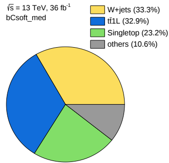
Figure 7.4: Breakdown of the individual SM contributions to the signal region. The prefit background yields are used. The minor backgrounds are merged into “Others.”
