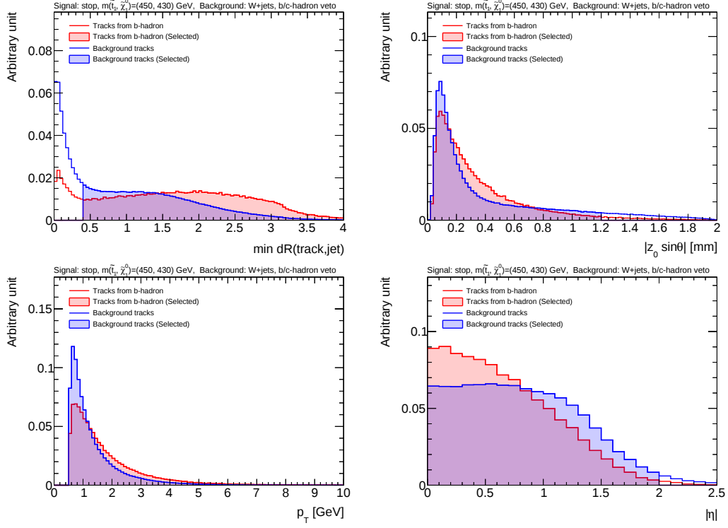
Figure 8.5: Track variables used to define the track selection: (top left) the minimum \Delta R between the track and EM topo jets with p_T > 30 GeV, (top right) |z_0^{\text{PV}} \sin \theta| , (bottom left) p_T , and (bottom right) |\eta| . The red histograms show the tracks from b -hadrons in the stop signal events, and the blue histograms show the tracks in the W +jets. W +jets events that have b - or c -hadrons are not used. All cuts described in Table 8.1 are applied, except for the cut on the variable that is shown in each plot. The shaded part of the histograms shows the distribution adding the cut on the displayed variable.
