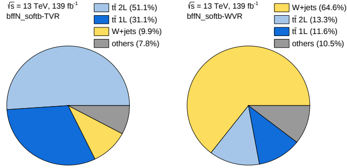
Figure 9.6: Breakdown of the individual SM contributions to the TVR (left) and WVR (right). The pre-fit yields are shown. The minor background processes are merged into “Others.”
