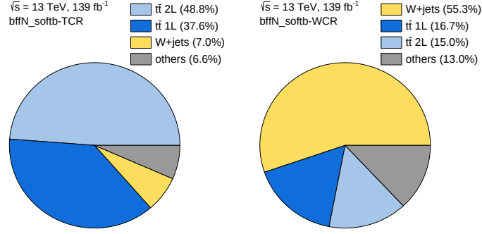
Figure 9.5: Breakdown of the individual SM contributions to the TCR (left) and WCR (right). The pre-fit yields are shown. The minor background processes are merged into “Others.”
