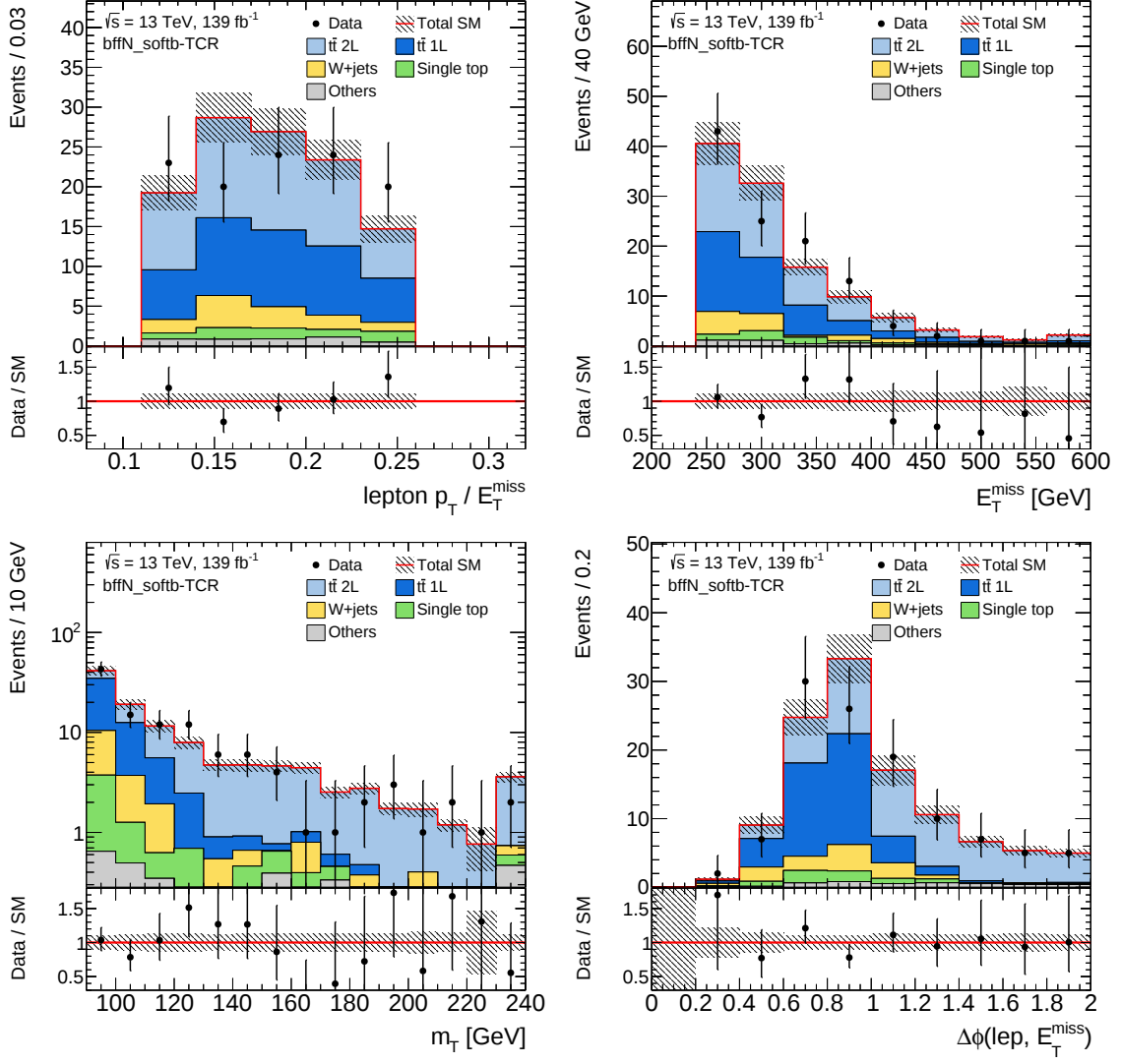
Figure 9.7: Comparison of data and simulation for the t\bar{t} CR after applying the normalization factors: (top left) the p_T^\ell/E_T^{\text{miss}} , (top right) E_T^{\text{miss}} , (bottom left) m_T , and (bottom right) \Delta\phi(\vec{E}_T^{\text{miss}}, \ell) . Statistical and experimental uncertainties are displayed. The last bin includes the overflow.
