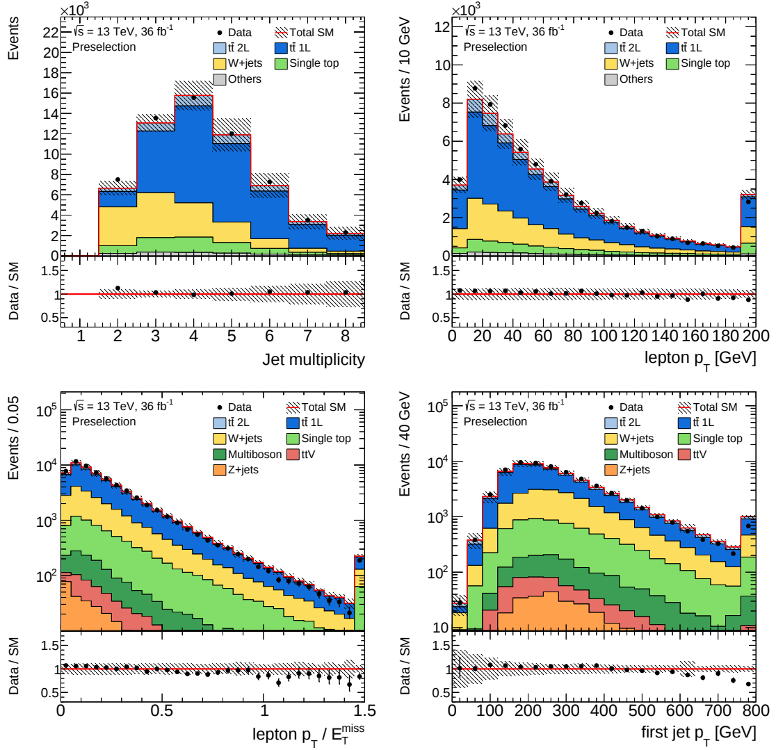
Figure 7.2: Comparison of data and simulation distributions with the preselection: the jet multiplicity (top left), lepton p_T (top right), p_T^\ell/E_T^{\text{miss}} (bottom left), and leading jet p_T (bottom right). The statistical and experimental uncertainties are displayed. The overflow is included in the last bin.
