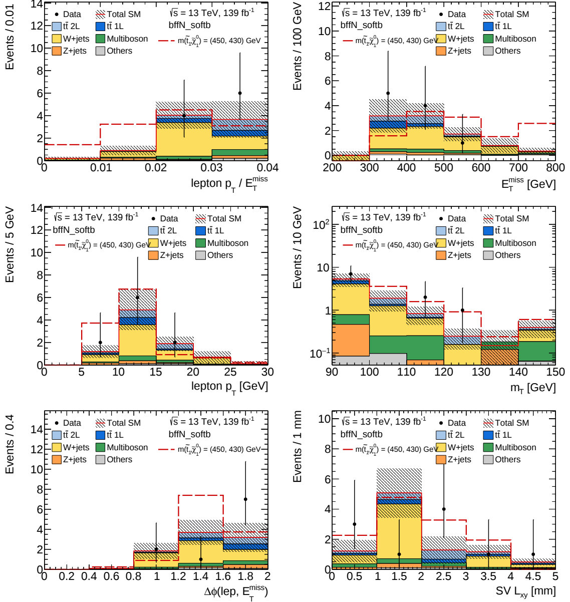
Figure 9.11: Distribution of the variables used to define the bffN_softb discovery SR with the SR selection: (top left) the p_T^\ell / E_T^{\text{miss}} , (top right) E_T^{\text{miss}} , (middle left) lepton p_T , (middle right) m_T , (bottom left) \Delta\phi(\vec{E}_T^{\text{miss}}, \ell) , and (bottom right) soft b -tag SV L_{xy} . The NFs are applied to the t\bar{t} and W +jets backgrounds. Statistical, theoretical, and experimental uncertainties are included. The last bin includes the overflow.
