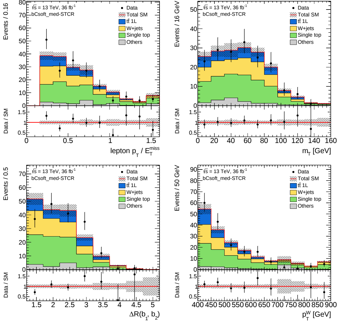
Figure 7.9: Comparison of data and simulation distributions for the single top CR after applying the normalization factors: the p_T^\ell/E_T^{\text{miss}} (top left), m_T (top right), \Delta R(b_1, b_2) (bottom left), and p_T^W (bottom right). The statistical and experimental uncertainties are displayed. The last bin includes the overflow.
