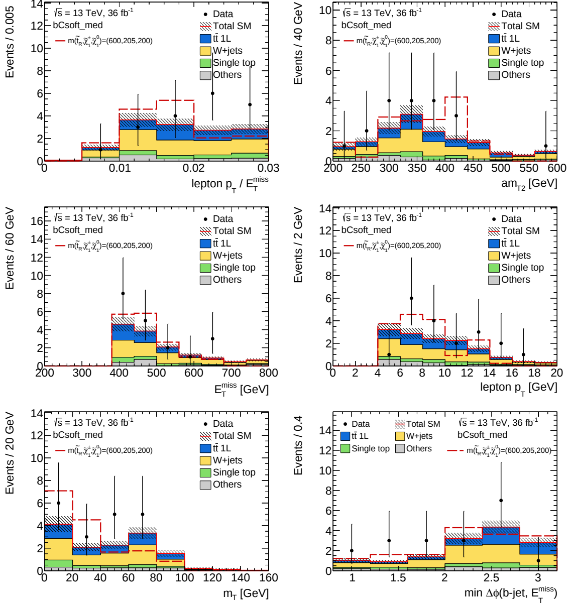
Figure 7.13: Distribution of the variables used to define the bCsoft_med discovery SR: (left column) p_T^\ell / E_T^{\text{miss}} , E_T^{\text{miss}} , m_T , (right column) am_{T2} , lepton p_T , and \min(\Delta\phi(\vec{p}_T^{\text{miss}}, b\text{-jet})) , in descending rows. The benchmark signal is overlaid.
