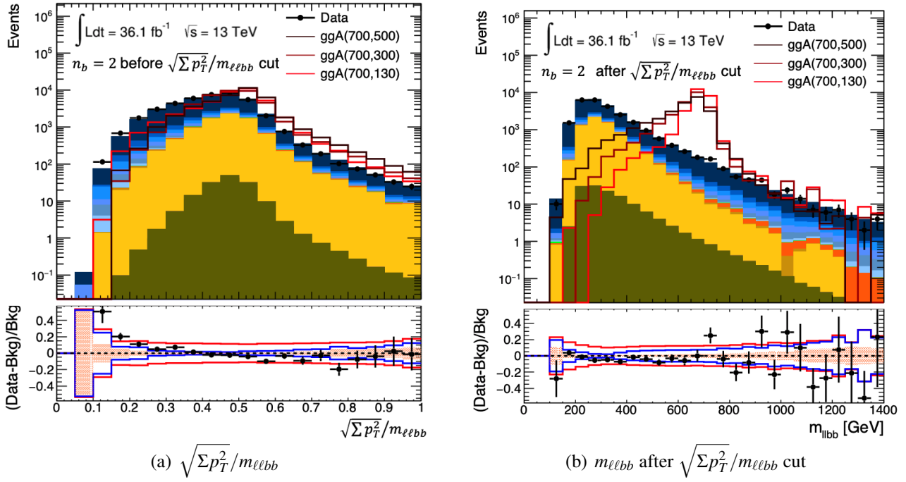
Figure 5.2: The (a) \sqrt{\Sigma p_T^2 / m_{\ell\ell bb}} distribution and the (b) m_{\ell\ell bb} distribution after the \sqrt{\Sigma p_T^2 / m_{\ell\ell bb}} cut. Only events in n_b = 2 category are shown. For the background simulated samples, color code shown in Figure 3.5 has been used. At the bottom panel, the filled area represent the statistical uncertainties, while the blue line shows the combined uncertainty from statistical and shape uncertainties. The total uncertainty which combines statistical and systematic uncertainties are also shown as a red line. Figures for these distributions in the n_b \geq 3 category can be found in Appendix B.
