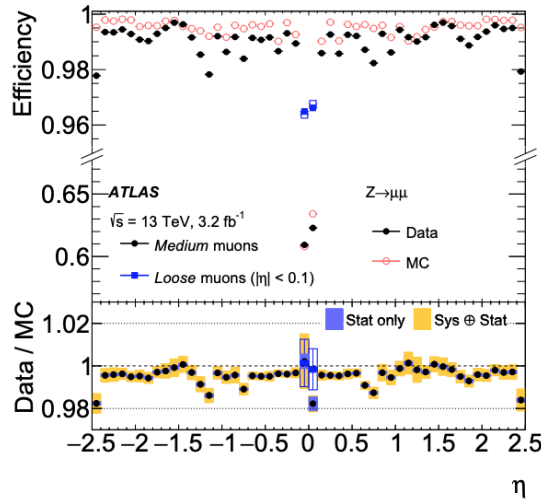
Figure 3.9: Muon reconstruction efficiency as a function of \eta measured in Z \rightarrow \mu\mu events for muons with p_T > 10 \text{ GeV} shown for Medium (black dots) and Loose (blue squares) muon operating points. The error bars on the efficiencies indicate the statistical uncertainty. The bottom panel shows the ratio of the measured to predicted efficiencies, with statistical and systematic uncertainties [106].
