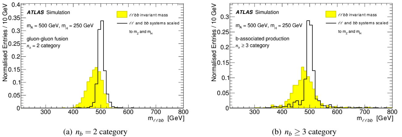
Figure 5.5: The signal m_{\ell\ell b\bar{b}} distribution shapes calculated by taking the mass of the \ell\ell b\bar{b} system (filled histograms) and after scaling the b\bar{b} and \ell\ell systems with respected to the hypothetic H boson mass and the Z boson mass (lines) for (a) the gluon-gluon fusion in the n_b = 2 category and (b) b-associated production in the n_b \geq 3 category of a A boson assuming m_A = 500 \text{ GeV} and m_H = 250 \text{ GeV} .
