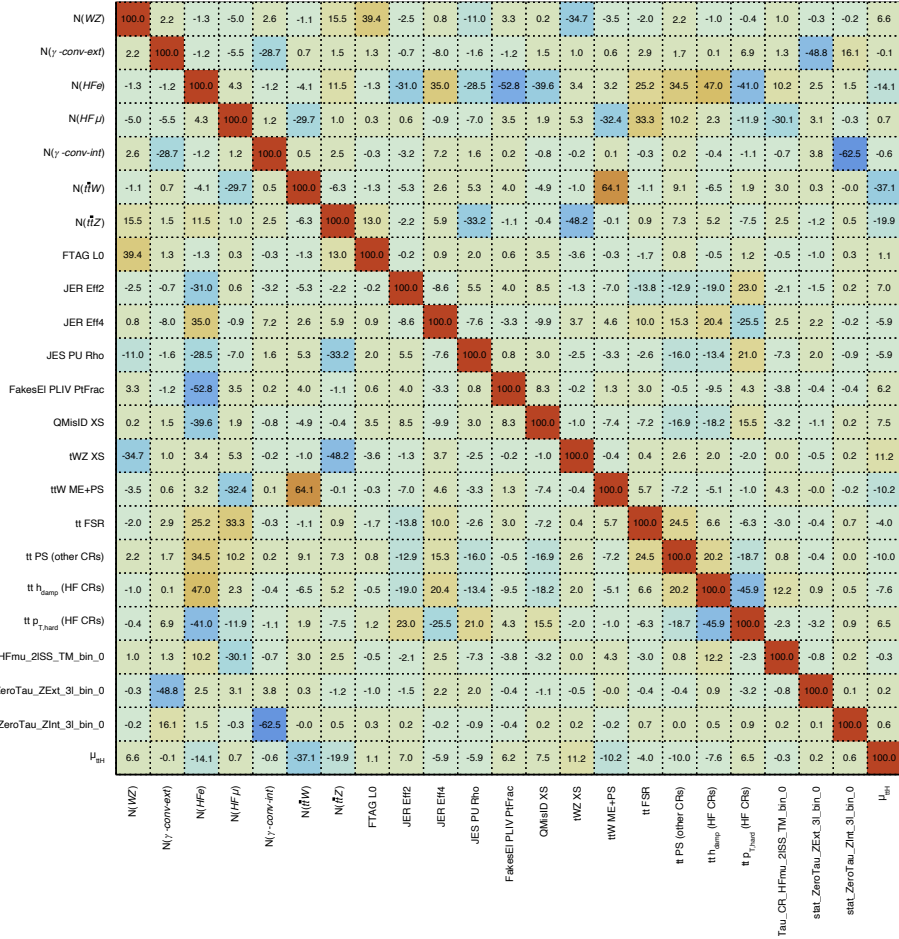
Figure 6.19: Correlation matrix of the fit parameters (POI, NFs and NPs) after the inclusive fit to real data in all analysis regions. Only parameters having at least one correlation larger than 30% with another parameter are shown.
