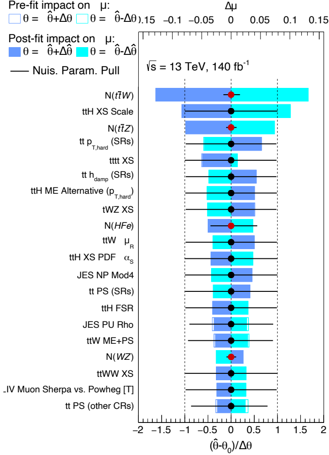
Figure A.4: The 20 most relevant fit parameters of the inclusive Asimov fit, ranked according to their impact on the \mu_{t\bar{t}H} POI. The impact ( \Delta\mu_{t\bar{t}H} ) associated with each fit parameter (NFs or NPs) is computed at both pre-fit and post-fit levels. Specifically, this impact is evaluated by comparing the nominal best-fit value of \mu_{t\bar{t}H} , \hat{\mu}_{t\bar{t}H} , to the value obtained from a fit where the parameter under consideration is fixed to its nominal best-fit value \hat{\theta} shifted by its pre-fit (post-fit) uncertainties \pm\Delta\theta ( \pm\Delta\hat{\theta} ). In total, four additional fits are performed for each parameter, corresponding to shifts of +\Delta\theta (dark blue, non-filled area), -\Delta\theta (light blue, non-filled area), +\Delta\hat{\theta} (dark blue, filled-colored area), and -\Delta\hat{\theta} (light blue, filled-colored area). The nominal best-fit values and uncertainties of the fit parameters are shown as black points with their corresponding error bars and are identical to those presented in Figure 6.13.
