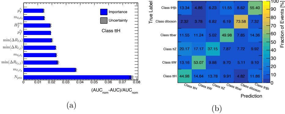
Figure 6.8: (a) Permutation importance of the ten most important BDT input variables for the t\bar{t}H class. This metric is defined for a given input variable as the relative difference between the area under the ROC curve (AUC) of the nominal training and the AUC of a training obtained after randomly permuting the values of the variable. The idea of the random permutation is to break the correlation between the variable and the target. The larger the difference between the two AUCs, the more important the variable is. The uncertainty on the permutation importance is computed by running several trainings shuffling the variable values and taking the standard deviation of the AUC values distribution. (b) Confusion matrix of the BDT. The sum of the elements in each row is normalised to 100%.
