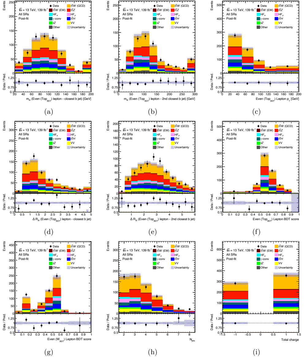
Figure B.10: Comparison between data and post-fit predictions, combining the SRs, for the BDT input variables of the selected signal-like even lepton: (a) m_{\ell b_0} , (b) m_{\ell b_1} , (c) lepton p_T , (d) \Delta R_{\ell b_0} , and (e) \Delta R_{\ell b_1} . Then, the BDT discriminator values for the two even leptons: (f) for the selected signal-like lepton, and (g) for the background-like lepton. Additionally, distributions of (h) N_{jets} and (i) the total charge of the leptons. The uncertainty bands represent the total uncertainty of the post-fit predictions. The lower panel shows the ratio of data to the total post-fit prediction. Events exceeding the upper limit of the x-axis range are included in the last bin (overflow).
