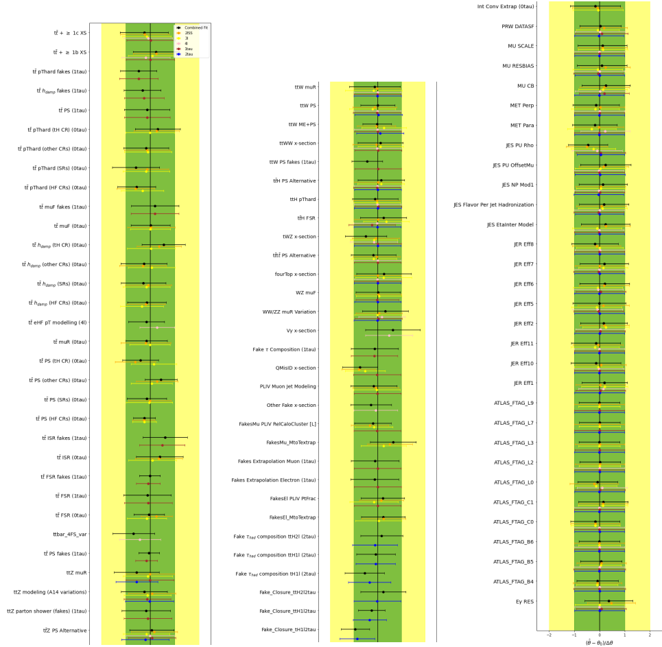
Figure A.21: Best-fit value \hat{\theta} and uncertainty \Delta\hat{\theta} of the NPs after the inclusive combined fit of the six t\bar{t}H -ML channels. They are represented by the black points and black error bars, respectively. Moreover, the fitted NPs for the individual-channel fits are shown in orange ( 2\ell SS + 0\tau_{\text{had}} ), yellow ( 3\ell + 0\tau_{\text{had}} ), pink ( 4\ell ), red ( 2\ell SS + 1\tau_{\text{had}} ) and blue ( 1\ell/2\ell OS + 2\tau_{\text{had}} ). The green (yellow) areas represent the \pm 1\sigma ( 2\sigma ) pre-fit uncertainties. Each NP is shown relative to its nominal value, \theta_0 , and in units of its pre-fit uncertainty \Delta\theta .
