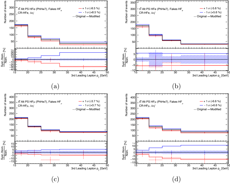
Figure 7.8: Alternative t\bar{t} PS modelling for (a) CR-HF _e \Delta\eta^- , (b) CR-HF _e \Delta\eta^+ , (c) CR-HF _{\mu} \Delta\eta^- , and (d) CR-HF _{\mu} \Delta\eta^+ . Uncertainty bands include the MC statistical uncertainties of the nominal sample. The Original (discontinuous) and Modified (continuous) lines correspond to the alternative-modelling template before and after smoothing, respectively.
