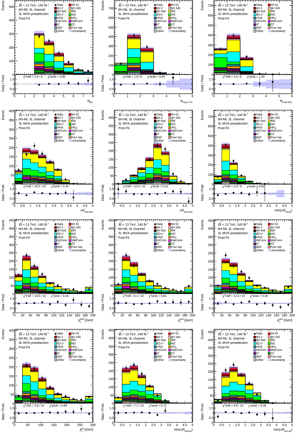
Figure A.18: Post-fit Data/MC comparison for twelve of the BDT input variables at the 3l MVA preselection level. The blue hashed bands represent the post-fit systematic uncertainty in each bin.
