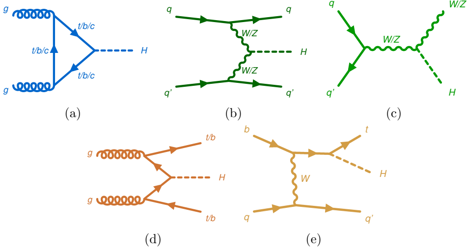
Figure 2.9: Example LO Feynman diagrams of the dominant Higgs-boson production modes at the LHC: (a) gluon-gluon fusion, (b) vector-boson fusion, and associated production with (c) vector bosons, (d) top- or bottom-quark pairs, or (e) a single top quark. Source: Ref. [17].
