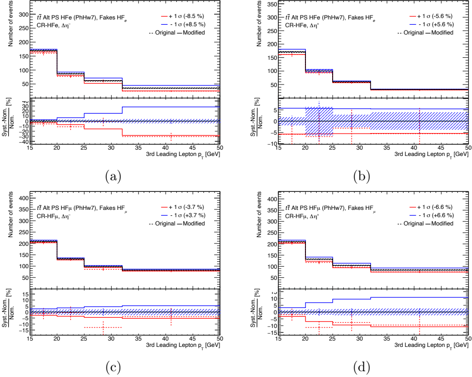
Figure B.3: Alternative t\bar{t} PS modelling for (a) CR-HF _e \Delta\eta^- , (b) CR-HF _e \Delta\eta^+ , (c) CR-HF _{\mu} \Delta\eta^- , and (d) CR-HF _{\mu} \Delta\eta^+ . Uncertainty bands include the MC statistical uncertainties of the nominal sample. The Original (discontinuous) and Modified (continuous) lines correspond to the alternative-modelling template before and after smoothing, respectively.
