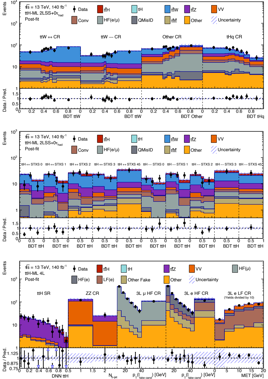
Figure 6.26: Comparison of observed and predicted yields in all bins for the 2\ell SS + 0\tau_{\text{had}} and 4\ell channels. The POI, background NFs, and NPs are set to their best-fit values obtained from the combined fit. The uncertainty band includes all uncertainties and their correlations.
