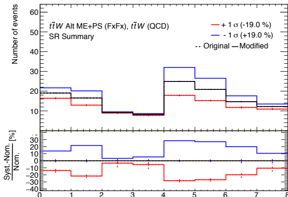
Figure B.1: Two-point systematic variations for the AMC@NLO + PYTHIA FxFx generator setup for t\bar{t}W production in the SRs. From left to right, each pair of bins represents SR-1 b -low N_{\text{jets}} , SR-1 b -high N_{\text{jets}} , SR-2 b -low N_{\text{jets}} , and SR-2 b -high N_{\text{jets}} . Within each pair, the left bin corresponds to \Delta|\eta_{\ell}^{\text{BDT}}| \leq 0 and the right bin to \Delta|\eta_{\ell}^{\text{BDT}}| > 0 . Uncertainty bands include the MC statistical uncertainties of the nominal SHERPA sample.
