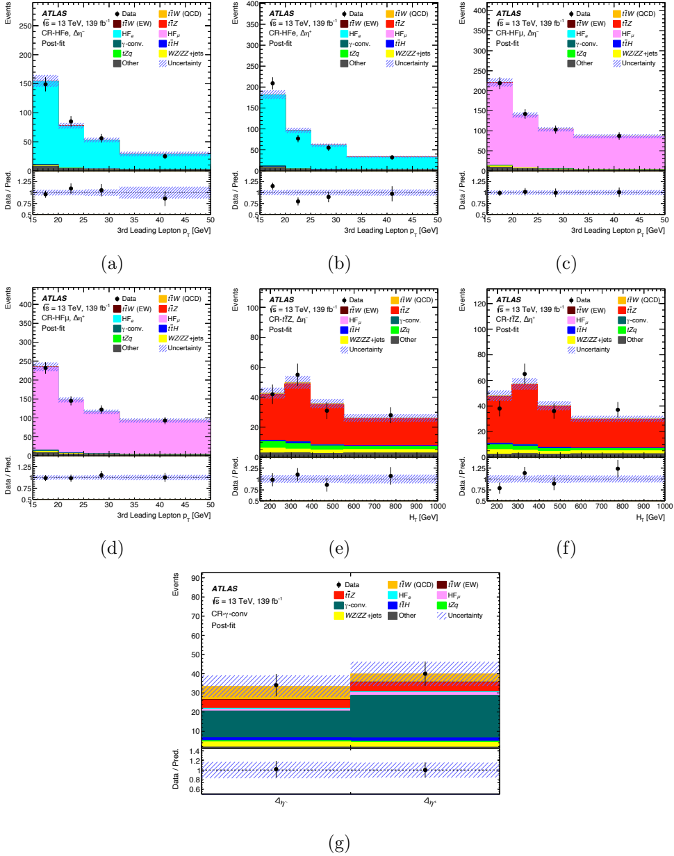
Figure 7.16: Comparison between data and post-fit predictions in (a,b) CR-HF e , (c,d) CR-HF μ , (e,f) CR- t\bar{t}Z , and (g) CR- \gamma -conv. The distributions shown correspond to the bins used in the likelihood fit. The regions are separated into \Delta|\eta_\ell^{\text{BDT}}| \leq 0 ( \Delta\eta^- ) and \Delta|\eta_\ell^{\text{BDT}}| > 0 ( \Delta\eta^+ ). The uncertainty bands represent the total uncertainties in the post-fit predictions. The ratios of data to the total post-fit predictions are shown in the lower panels. Events exceeding the upper limit of the x-axis range are included in the last bin (overflow).
