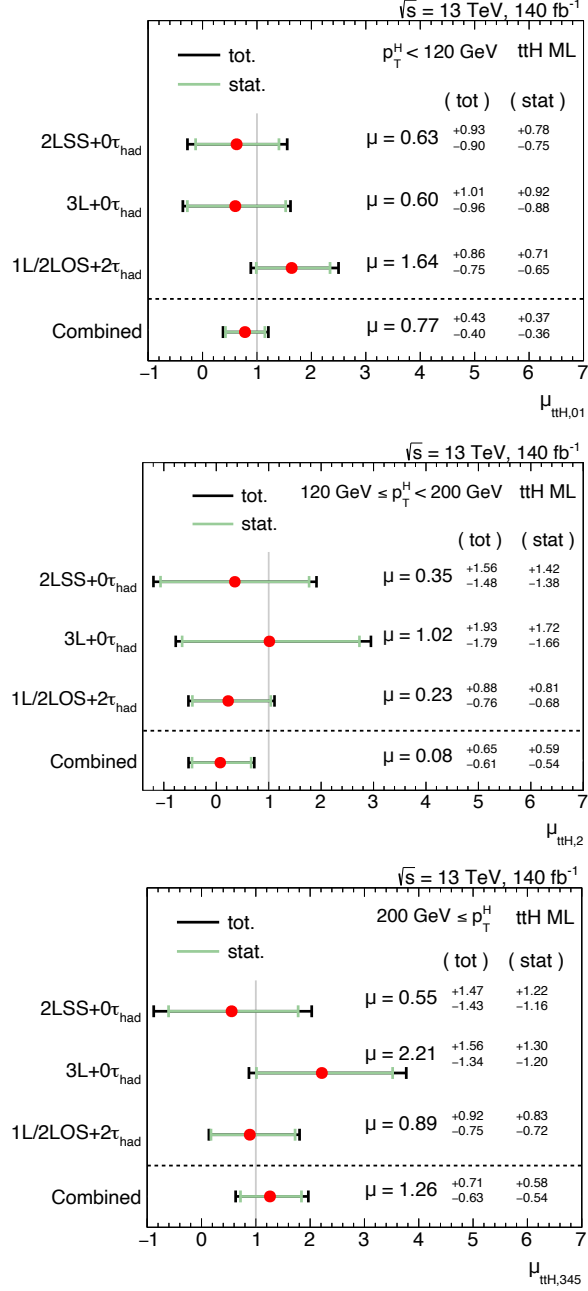
Figure 6.31: Observed best-fit values of the three POIs and their uncertainties for the individual channels (3 \ell +0 \tau_{\text{had}} , 2LSS+0 \tau_{\text{had}} , 1 \ell +2 \tau_{\text{had}} and 2 \ell OS+2 \tau_{\text{had}} ) and their combination. From top to bottom: \mu_{t\bar{t}H,01} , \mu_{t\bar{t}H,2} , and \mu_{t\bar{t}H,345} , corresponding to p_T^H [GeV] \in [0, 120), [120, 200), and [200, \infty ), respectively. The SM prediction corresponds to \mu_{t\bar{t}H} = 1 .
