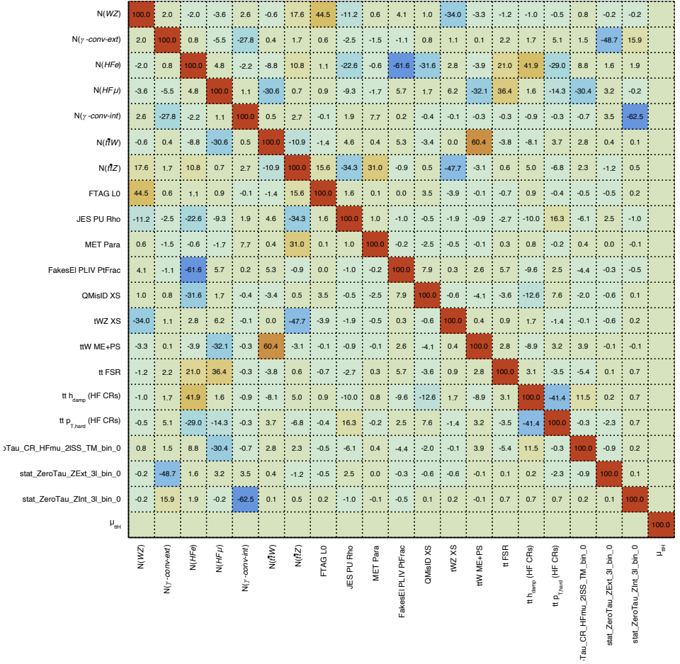
Figure A.15: Correlation matrix of the fit parameters (POI, NFs and NPs) after the fit to real data in the CRs. Only parameters having at least one correlation larger than 30% with another parameter are shown.
