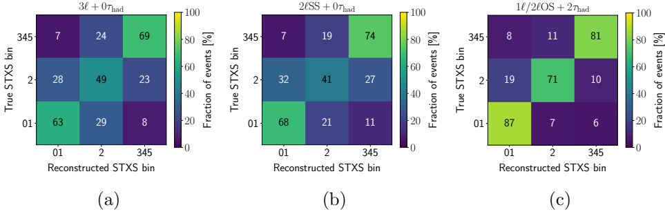
Figure 6.30: STXS migration matrices evaluated for the t\bar{t}H events in the (a) 3\ell + 0\tau_{\text{had}} , (b) 2\ell\text{SS} + 0\tau_{\text{had}} , and (c) 1\ell + 2\tau_{\text{had}} and 2\ell\text{OS} + 2\tau_{\text{had}} channels. The sum of the elements in each row is normalised to 100%.
