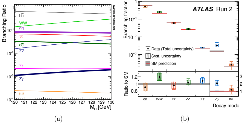
Figure 2.12: (a) Theoretical Higgs boson branching ratios and their uncertainties for the mass range around 125 GeV. Source: Ref. [73]. (b) Observed and expected branching fractions assuming SM values for the cross-sections. Both ATLAS measurements and theory predictions correspond to a centre-of-mass energy of 13 TeV (LHC Run 2). Source: Ref. [17].
