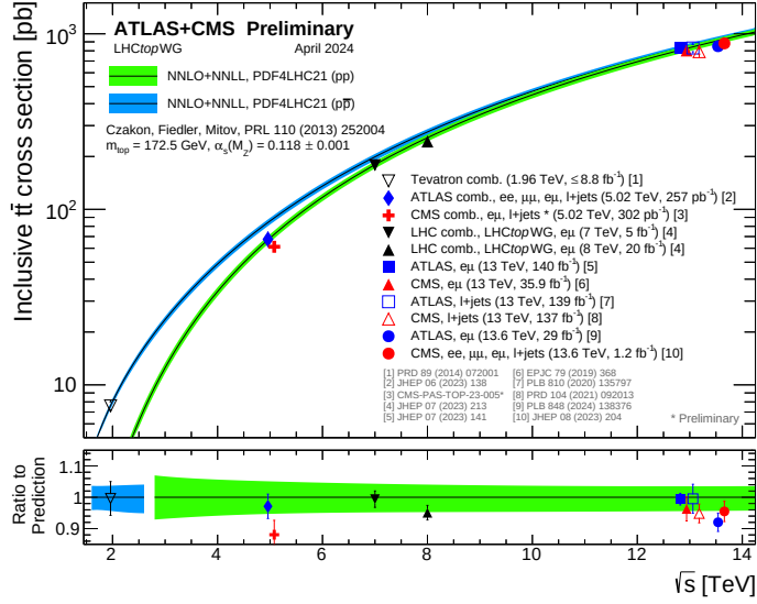
Figure 2.2: Overview of t\bar{t} production cross-section measurements from the LHC and Tevatron at various centre-of-mass energies, compared to NNLO+NNLL theoretical calculations. The theoretical band reflects uncertainties from renormalisation/factorisation scales, PDF sets, and \alpha_s . Calculations and data use m_t = 172.5 \text{ GeV} . Source: Ref. [29].
