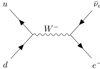
Figure 1.4: Tree-level Feynman diagram for a \bar{u}d \rightarrow e^-\bar{\nu}_e process mediated by a W^- boson.
