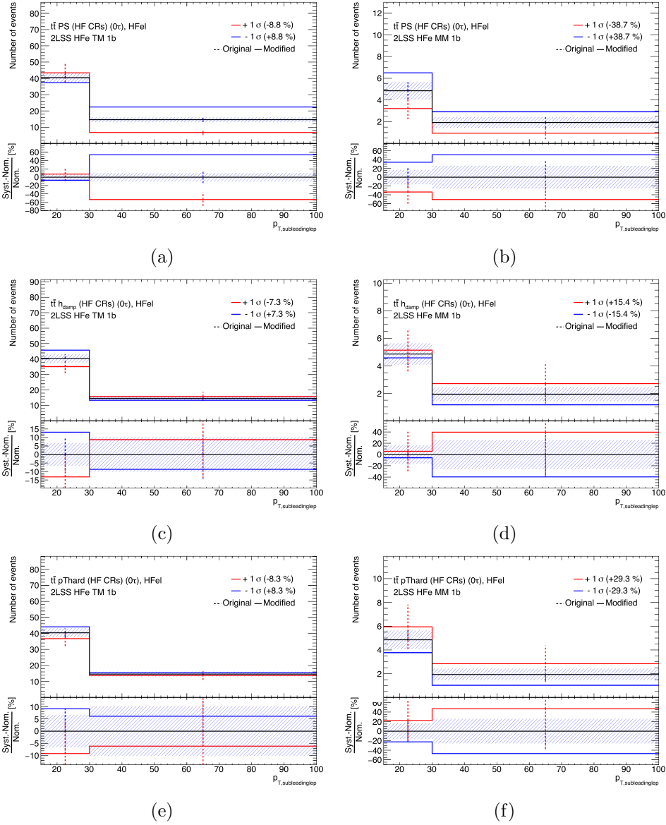
Figure 6.14: Alternative modelling of the t\bar{t} (a,b) PS, (c,d) h_{\text{damp}} and (e,f) p_{\text{T}}^{\text{hard}} for the HF _{\ell} background in the HF _{\ell} TM_{\text{ex}} (left column) and M_{\text{ex}}M_{\text{ex}} (right column) CRs. Uncertainty bands include the MC statistical uncertainties of the nominal sample.
