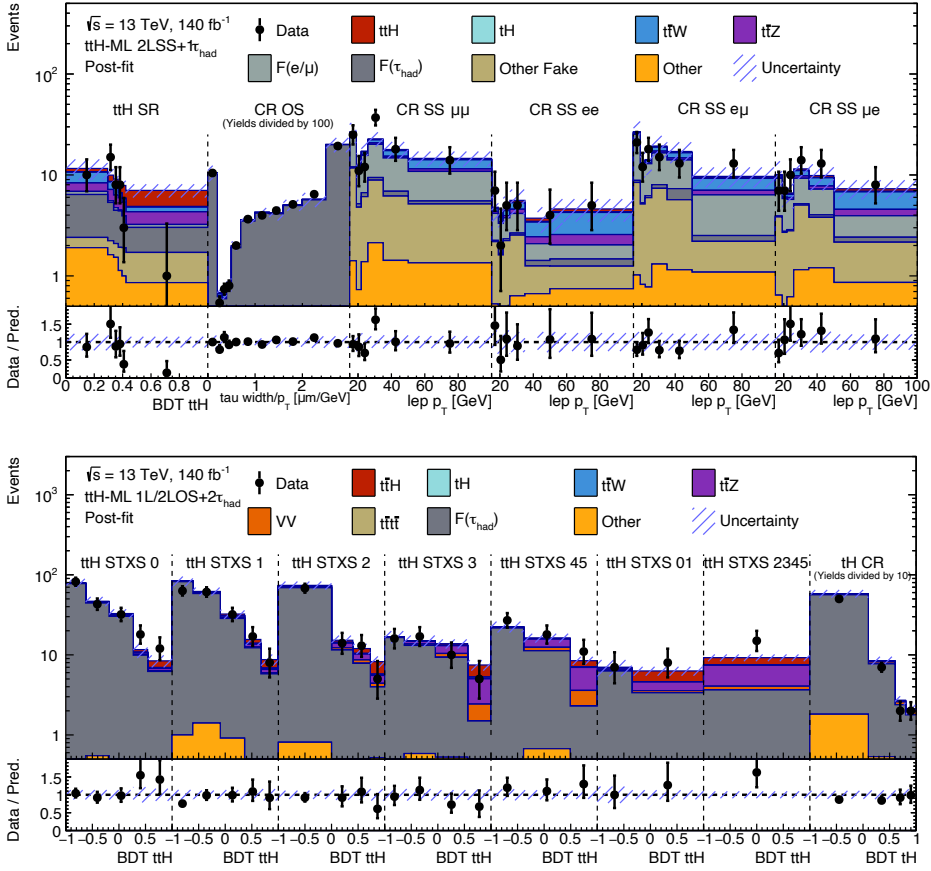
Figure 6.27: Comparison of observed and predicted event yields across all bins used in the statistical analysis for the 2\ell SS + 1\tau_{\text{had}} , 1\ell + 2\tau_{\text{had}} , and 2\ell OS + 2\tau_{\text{had}} channels. The POI, background NFs, and NPs are set to their best-fit values obtained from the combined fit. The uncertainty band incorporates all uncertainties and correlations.
