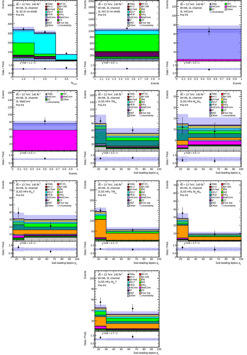
Figure 6.12: Fit input bins associated to the non-MVA regions, namely the t\bar{t}Z and WZ \ell\ell -on-shell CRs, the IntConv and MatConv CRs, and the HF_e and HF_\mu CRs. The blue hashed bands represent the systematic uncertainty of each bin.
