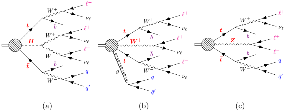
Figure 6.2: Example Feynman diagrams for the (a) t\bar{t}H , (b) t\bar{t}W and (c) t\bar{t}Z processes in the 3\ell + 0\tau_{\text{had}} final state. The t\bar{t}H diagram is shown for the H \rightarrow WW^* decay mode, as it is the dominant one in this channel (see Figure 6.1a).
