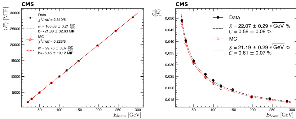
Figure 2.23: Left: The mean measured energy is plotted against the beam energy for both experimental data and simulation outcomes. Right: The relative energy resolution of the measured energy is illustrated for both experimental data and simulation results [52].
