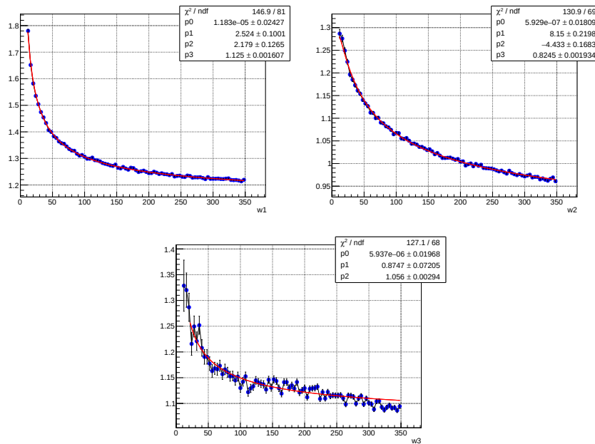
Figure A.1: The energy dependent weights \alpha, \beta, \gamma shown on X axis and referred as w_1 , w_2 , and w_3 respectively, extracted as a function of energy using \chi^2 minimization for pions start showering in CE-E (CE-E pions) are shown above. A parametric function has been fitted to extract these weights for any energy values.
