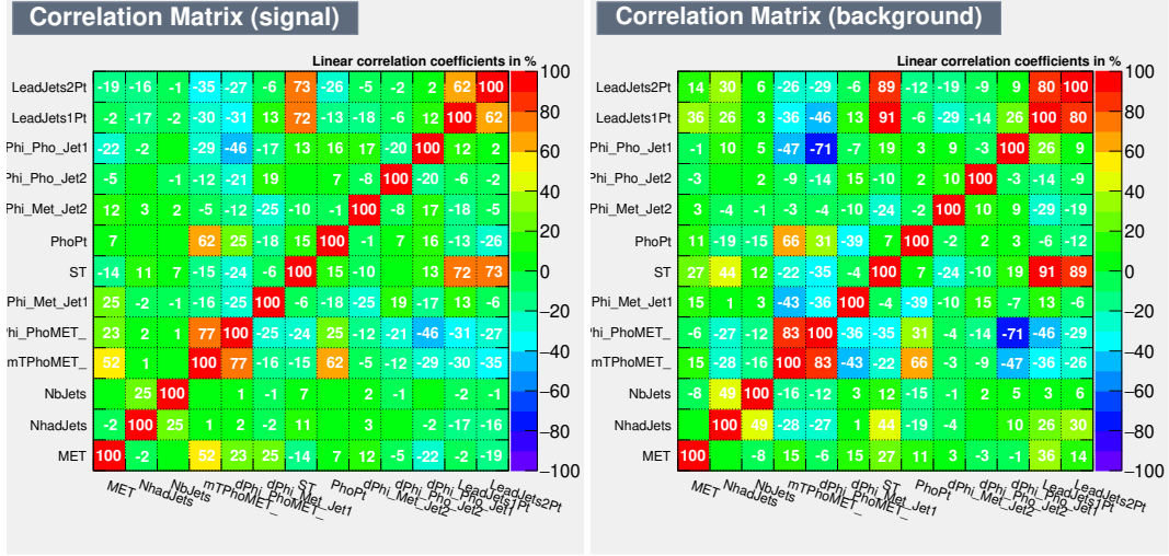
Figure 7.49: Correlation among input variables for signal (left) and background (right).
