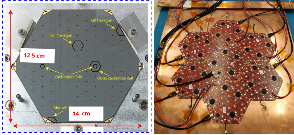
Figure 5.47: A layer of CE-E (right) and CE-H (left) from the beam test setup, highlighting the sizes of the absorber and active plates.
