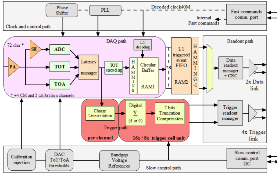
Figure 6.3: The different components of the HGCROC chip are shown in the above schematic diagram [143].
