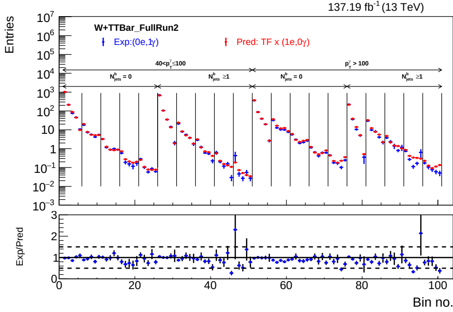
Figure 7.31: Expected SR (blue markers) are compared to those predicted by equation 7.6 (red markers) in MC with Run-2 luminosity. The lower panel shows the expected-to-predicted ratio.
