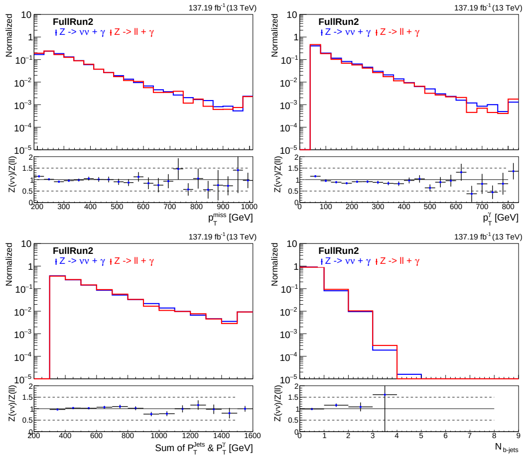
Figure 7.40: The p_T^{\text{miss}} in the top left, p_T^\gamma in the top right, S_T in the bottom left, and N_{\text{b-jets}} in the bottom right distributions in Z(\nu\bar{\nu})\gamma + \text{jets} SR and Z(\ell\bar{\ell})\gamma + \text{jets} CR.
