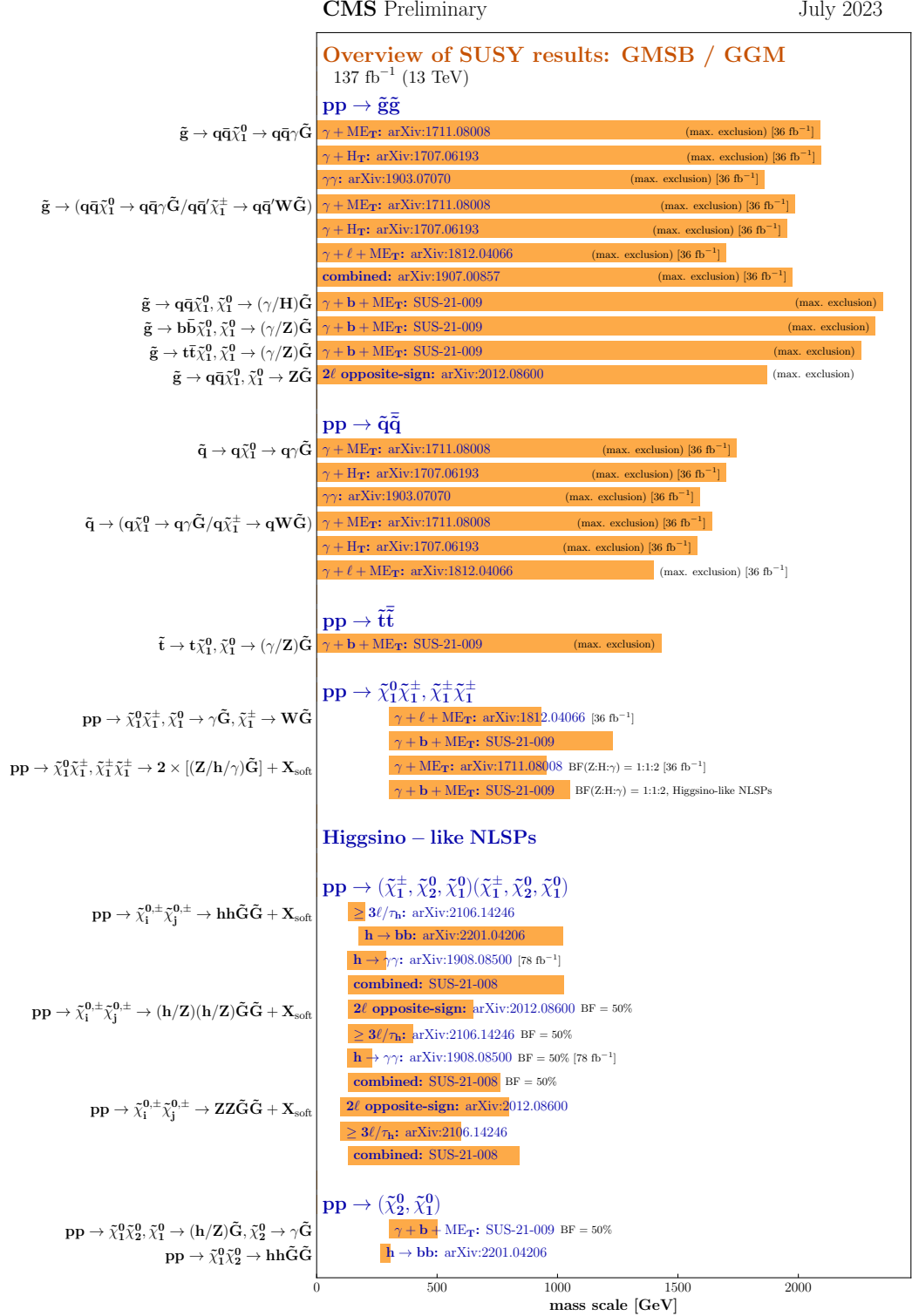
Figure 1.2: Excluded mass range of different particles for simplified models within GMSB scenarios. [15]
