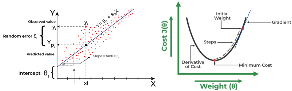
Figure 4.1: Left; correlation between X and Y s. Right; Cost or loss values as a functions of \theta . The A 's are represented as \theta 's. [108]
