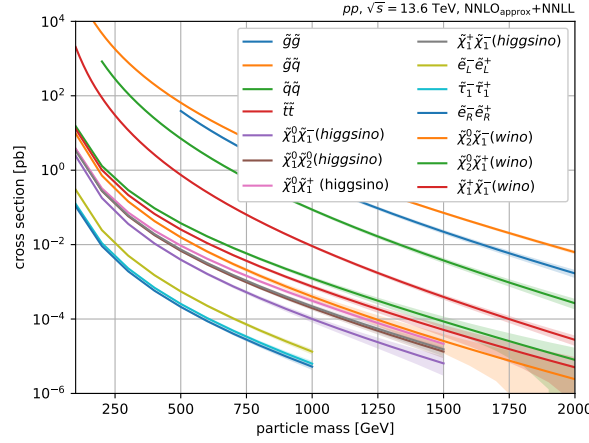
Figure 2.7: Cross sections for various subprocesses at 13.6 TeV with analyzed simplified topologies. [43]
