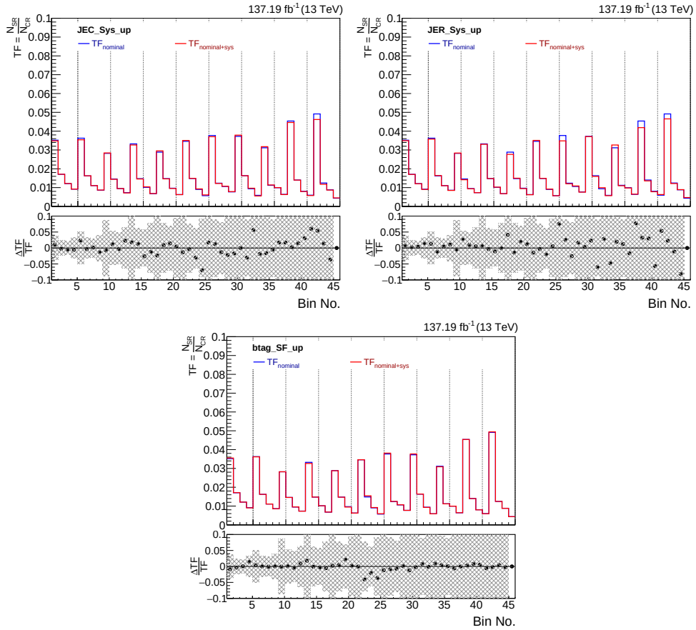
Figure 7.38: Comparison of nominal TF (in blue) with TF after varying the JEC factors (top left) and JER (top right) by +1\sigma_{sys} , and varying the scale factor of b-tagging (bottom) are shown in the top panel. Shaded region represents the statistical uncertainty in the bottom panel and black points are showing relativistic differences in the TF defined as the ratio of (TF_{nominal} - TF_{nominal+sys}) to TF_{nominal} .
