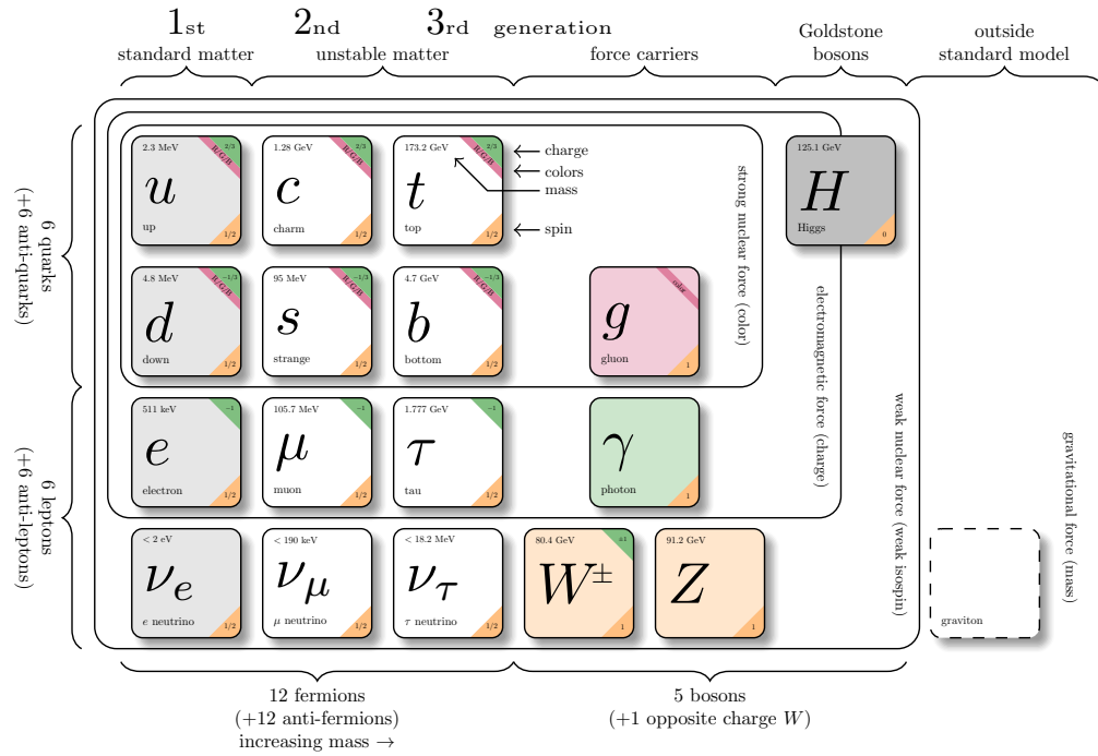
Figure 2.1: Table of elementary particles in the Standard Model, comprising quarks, leptons, and gauge bosons.[20]
