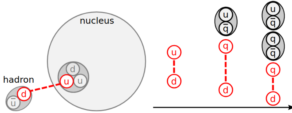
Figure 2.25: Left: The development of strings between the constituent quarks of an incoming hadron and those within a target nucleus. Right: The fragmentation of gluon strings through the generation of quark-antiquark pairs, succeeding which, hadronisation occurs [64].
