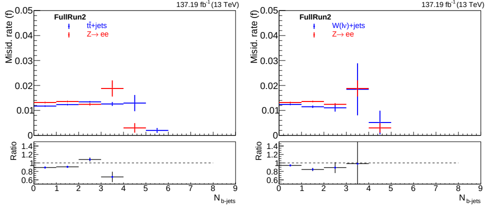
Figure 7.36: A comparison of fake rate for DY process ( Z \rightarrow e^+e^- ) and t\bar{t} is presented on the left as a function of the variable N_{b\text{-jets}} , using W/t\bar{t} like selections. On the right, a similar comparison is shown for DY ( Z \rightarrow e^+e^- ) and W +jets.
