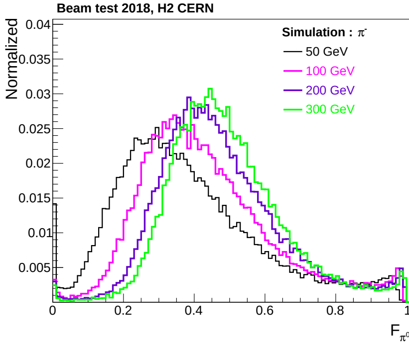
Figure 5.55: Distribution of fraction of EM component defined as F_{\pi^0} in hadron showers of different energy pions. This has been calculated using beam test simulation with FTFP_BERT_EMN physics list.
