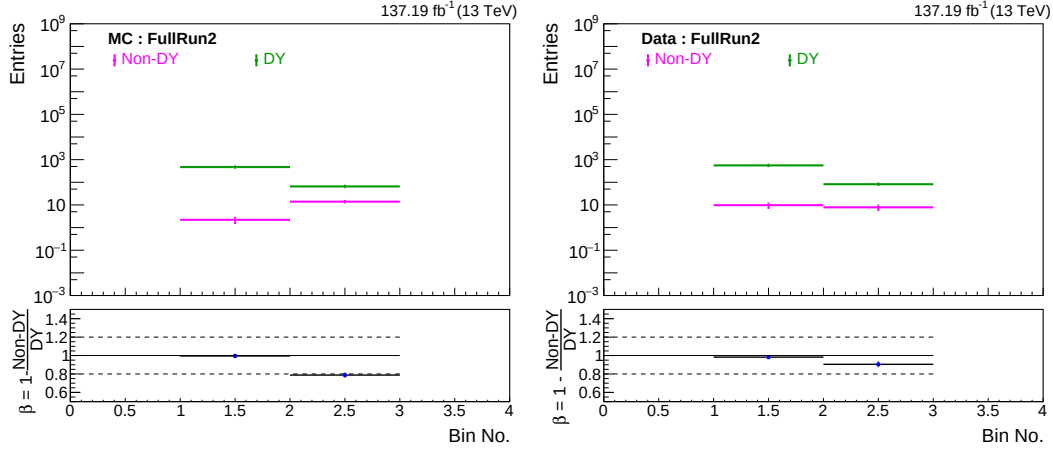
Figure 7.42: Purity factor obtained in N_{\text{bjets}} bins and shown in bottom panel using MC (left) and data (right) with full Run 2 luminosity.
