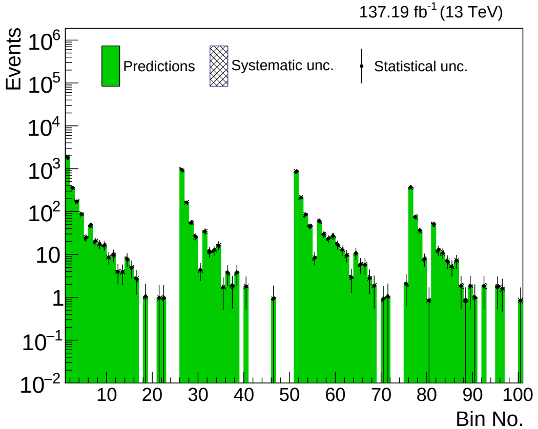
Figure 7.27: The predicted background events in the SRs for Lost lepton background. The black points indicate statistical uncertainty and gray shaded region represents systematic uncertainty.
