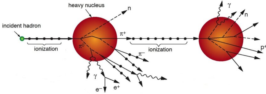
Figure 2.12: Illustration of hadronic interactions with material [46].
