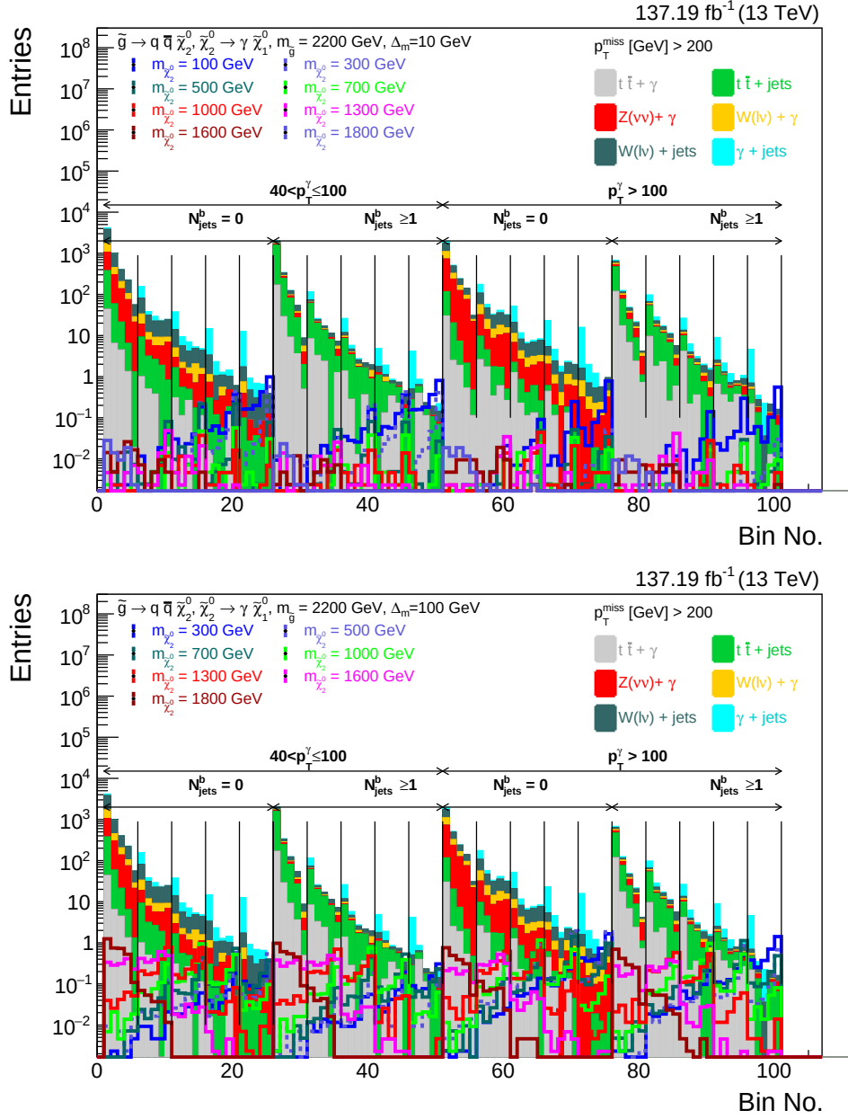
Figure 7.15: The distributions of background and a selection of T5gg motivated m_{\tilde{\chi}_2^0} signal points, with \Delta m set to 10 (top) & 100 GeV (bottom), respectively is shown in new SRs based on (p_T^{\text{miss}}, S_T, N_{\text{bjets}} \text{ \& } p_T^\gamma) with p_T^\gamma > 40 GeV.
