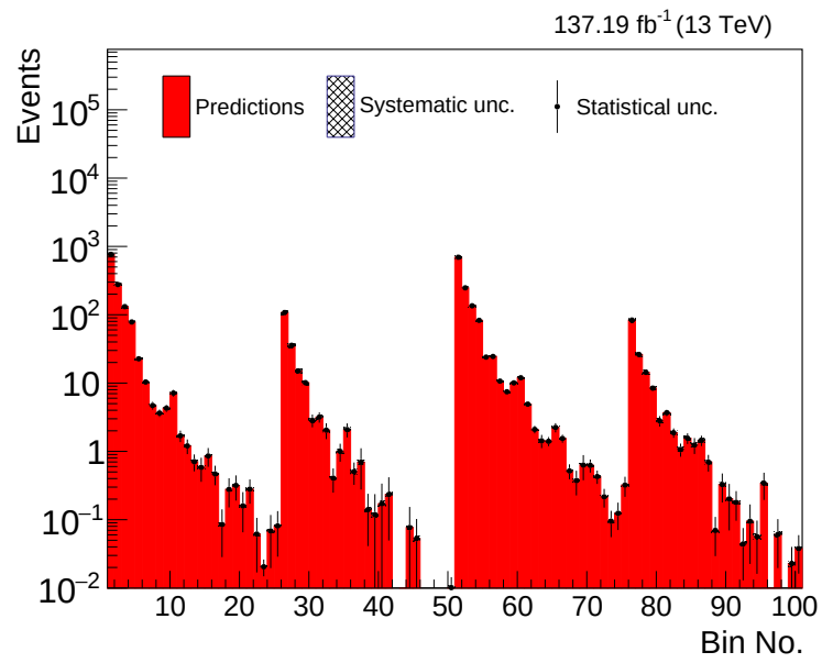
Figure 7.45: The predicted background events in the SRs for Z(\nu\bar{\nu}) + \gamma . The black points indicate statistical uncertainty.
