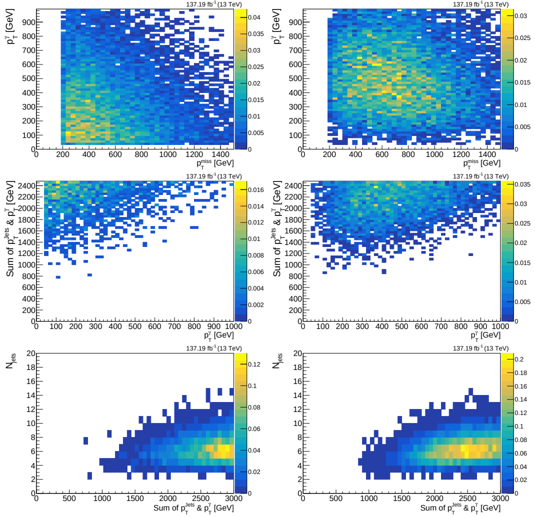
Figure 7.7: The distributions of p_T^{\text{miss}} versus p_T^{\gamma} (top row) and S_T versus p_T^{\gamma} (middle row), and S_T versus N_{\text{jets}} (bottom row) with m_{\tilde{\chi}_1^0} = 10 GeV in the first column (indicating high mass splitting) and m_{\tilde{\chi}_1^0} = 1000 GeV in the second column (indicating low mass splitting) are shown.
