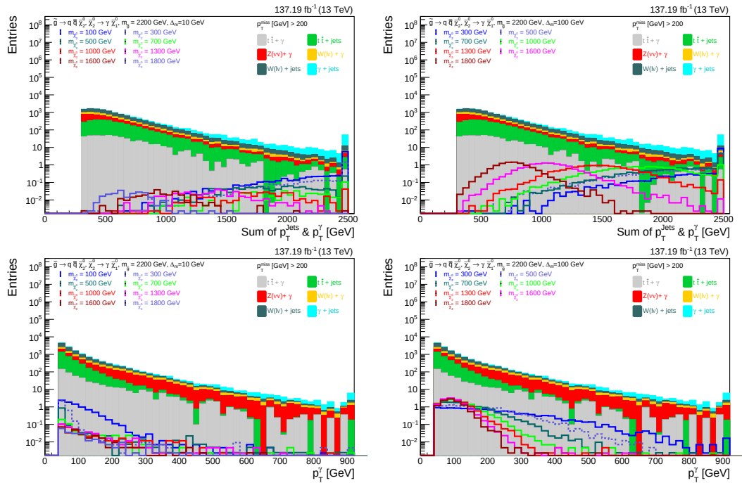
Figure 7.14: The top and bottom rows illustrate the distribution of S_T and p_T^\gamma , respectively, for SM backgrounds and a selection of T5gg motivated m_{\tilde{\chi}_2^0} signal points, with \Delta m set to 10 & 100 GeV, respectively.
