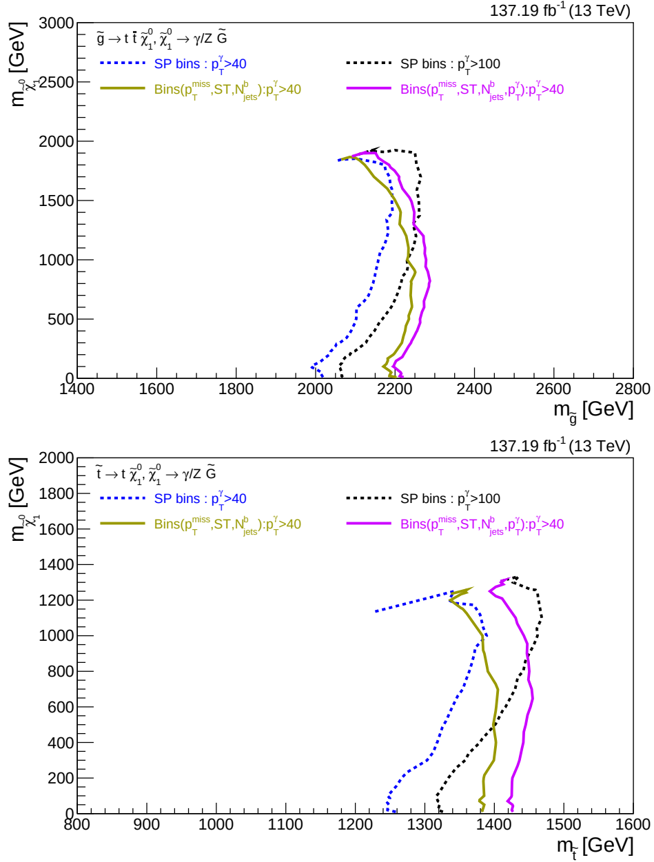
Figure 7.12: The expected exclusion limits at 95% confidence interval (CL) for T5tttZG (top) and T6ttZG (bottom) models with different SRs. The new SR bins in Magenta line shows improvement in mass exclusion in small \tilde{\chi}_1^0 masses.
