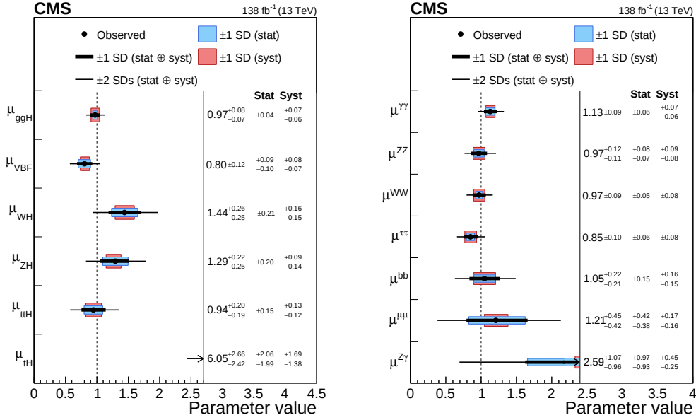
Figure 1.1: Comparison of observed and SM predictions for both production modes (left) and decay channels (right). Signal strength parameters are derived for (left) distinct production modes \mu_i , under the assumption BF=(BF)_{SM} , and (right) decay channels \mu_f , assuming \sigma^i = (\sigma^i)_{SM} . The dashed vertical line at one denotes the SM values for \mu_i and \mu_f [11].
