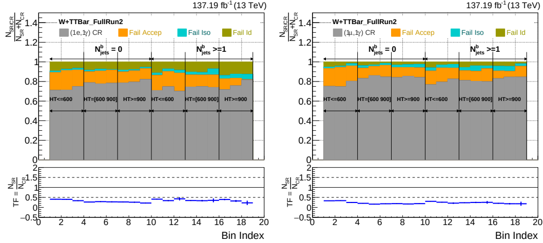
Figure 7.20: Distribution of individual normalized fraction of the contributions of these three categories in the lost electron SR (left) and the lost muon SR (right) as a function of different TF bins.
