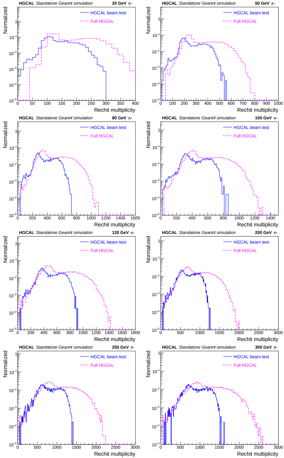
Figure A.22: Comparison of total number of rechits recorded in the full HGICAL geometry vs the beam test geometry for different pion energies. For the full HGICAL, all the rechits within dR cone of 0.5 and passing noise threshold criteria are considered here.
