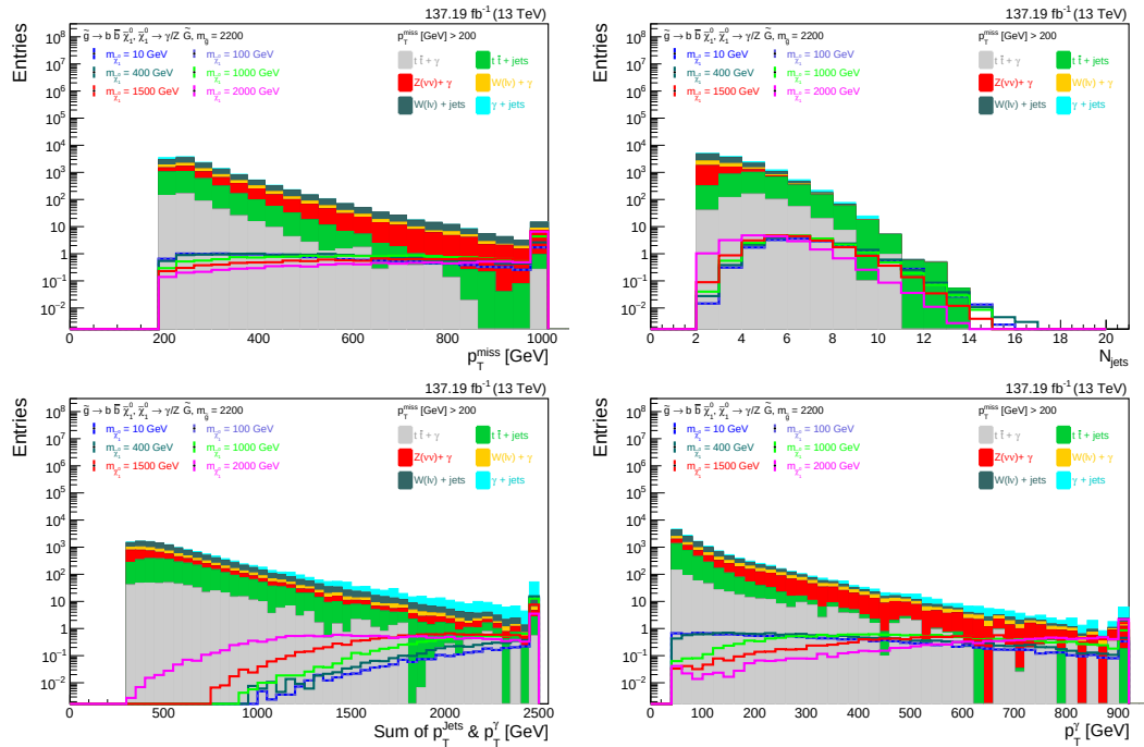
Figure 7.6: Distribution of p_T^{\text{miss}} (top left), N_{\text{jets}} (top right), S_T (bottom left) and p_T^\gamma (bottom right) for SM backgrounds and different SUSY signal topologies after applying baseline selections.
