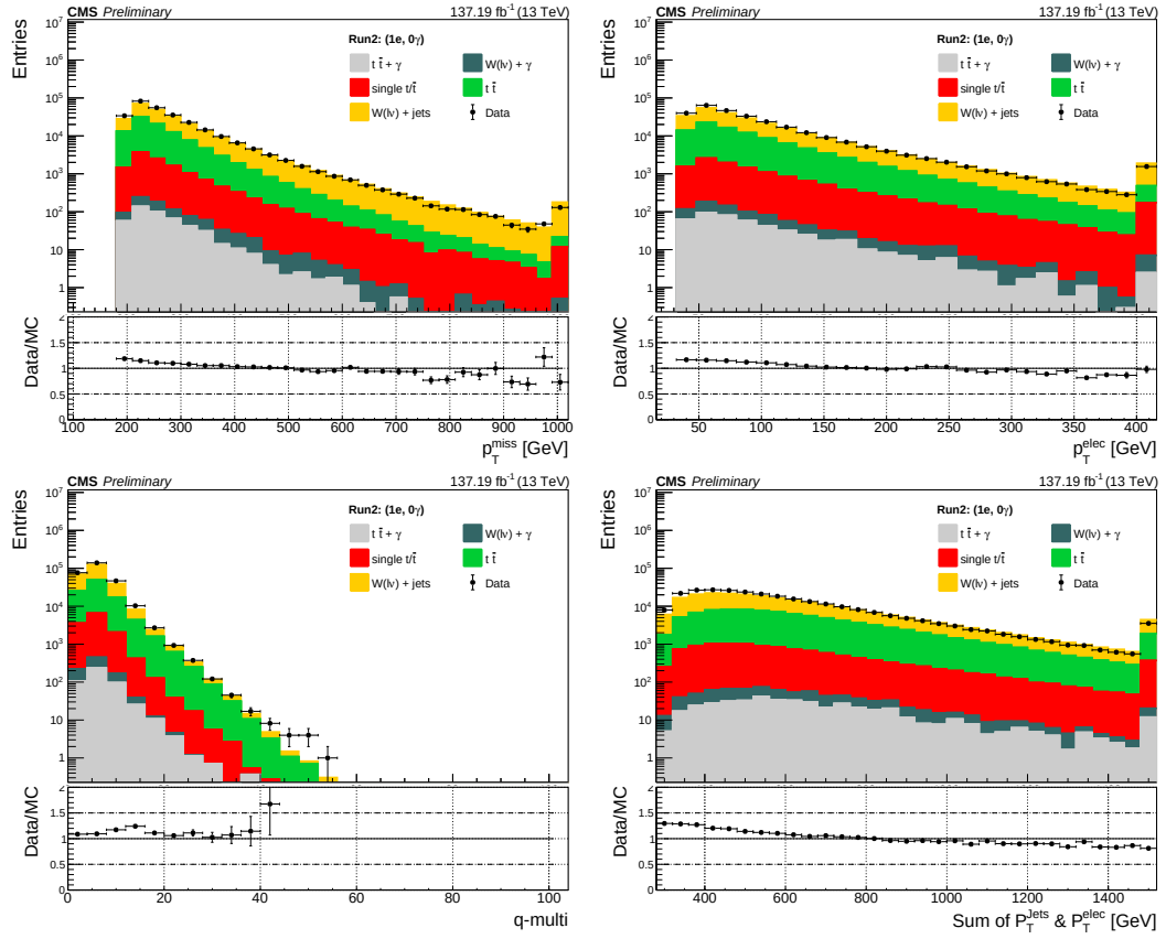
Figure 7.28: p_T^{\text{miss}} (top left), p_T^{\text{elec}} (top right), q -multiplicity (bottom left), and S_T (bottom right) for single electron CR are compared in MC (filled histograms) and Data (black point) with complete Run 2 luminosity.
