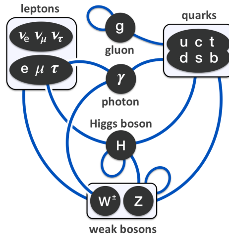
Figure 2.2: Elementary particles in the Standard Model are categorized within dark ovals, with blue arcs indicating interactions. Image courtesy - Wikipedia
