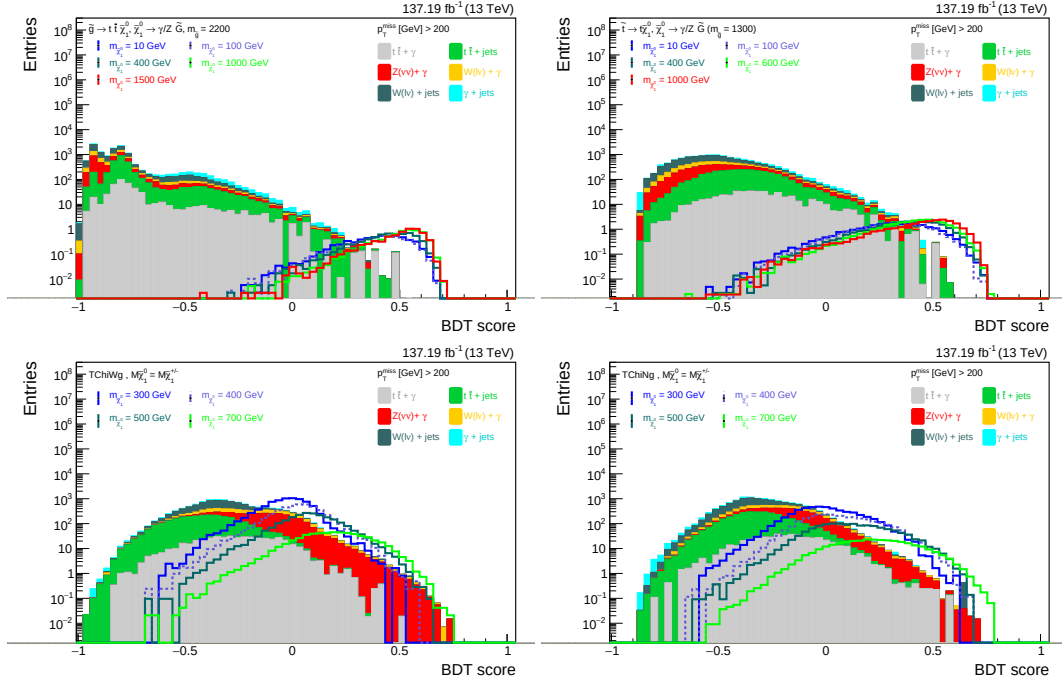
Figure 7.50: BDT score distribution in different BDTs trained on SM backgrounds and different simplified signal models: T5ttttZG (top left), T6tttZG (top right), TChiWG (bottom left) and TChiNG (bottom right). Signal and background events are cross section weighted and scaled to full Run 2 luminosity.
