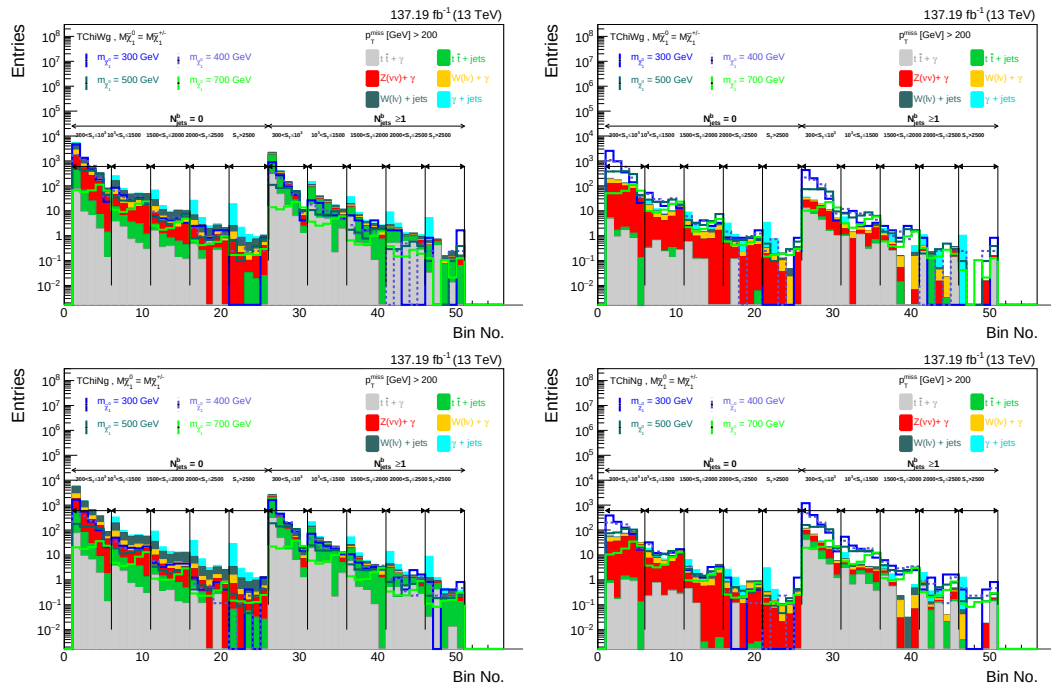
Figure 7.53: Distributions of signal and background events in SRs defined in (p_T^{\text{miss}}, S_T and N_{\text{bjets}}) without BDT (left) and with BDT preselection (right) shown for TChiWG (top) and TChiNG (bottom).
