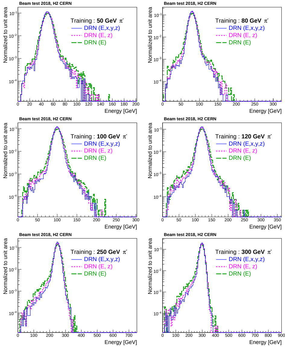
Figure A.12: Distributions of energies predicted using different DRN models for 50, 80, 100, 120, 250 and 300 GeV pions on training datasets.
