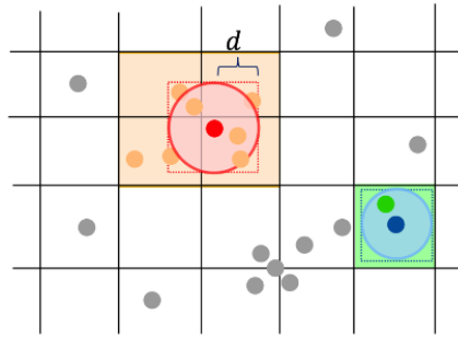
Figure 5.58: A fixed grid based on parameter d is defined for each 2D points such that finding the highest neighbour is fast as compared to other algorithms. For local density calculation and querying for neighbourhood, all the points in the bins touched by square window [x \pm d_i], [y \pm d_i] are considered as shown green and blue points in the above image [131].
