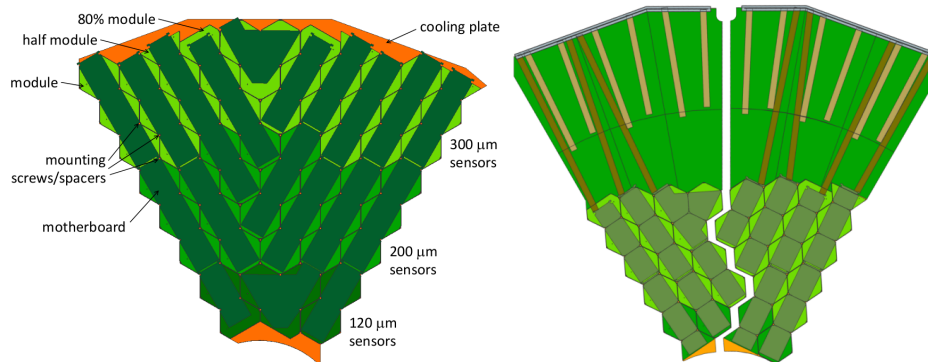
Figure 3.15: An example 60° cassette and two 30° mixed silicon and scintillator cassettes of CE-E and CE-H are shown from left to right respectively. [94].
