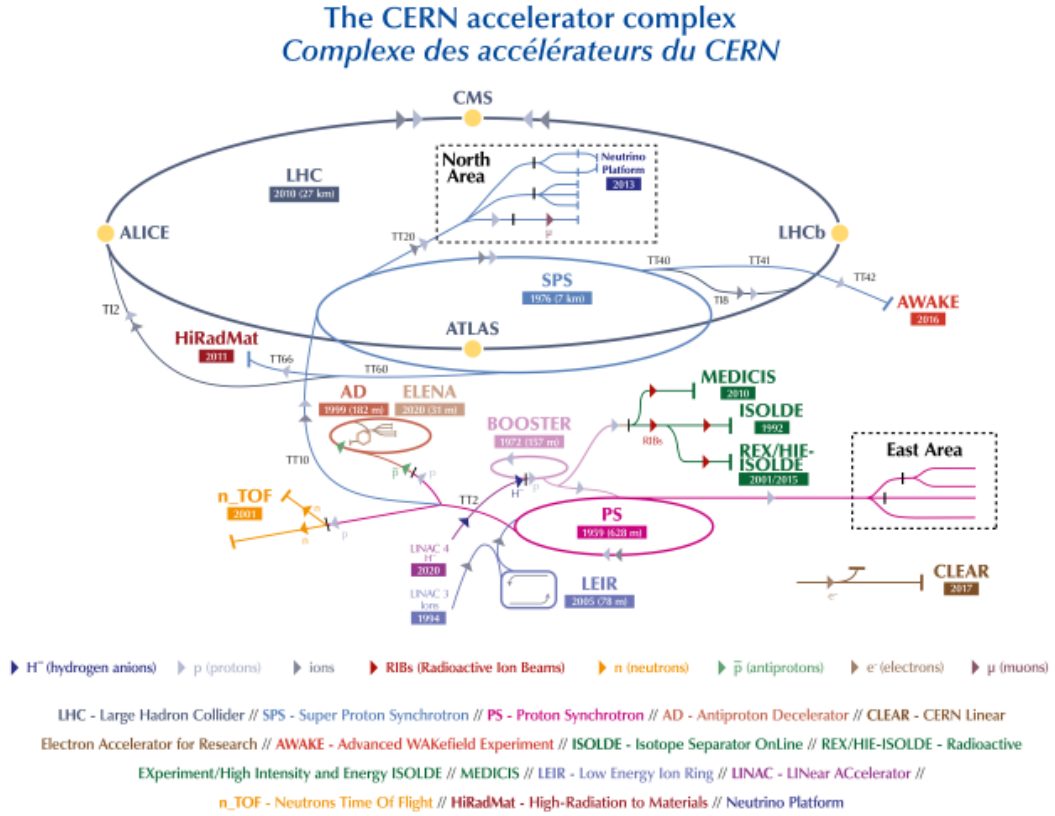
Figure 3.1: CERN accelerator complex. (Image Credit CERN)
