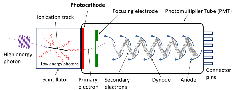
Figure 2.20: Illustration of the scintillator detector : An incoming high-energy photon produces scintillation photons, which are then transformed into photoelectrons and subsequently amplified. Image Credit - Wikipedia
