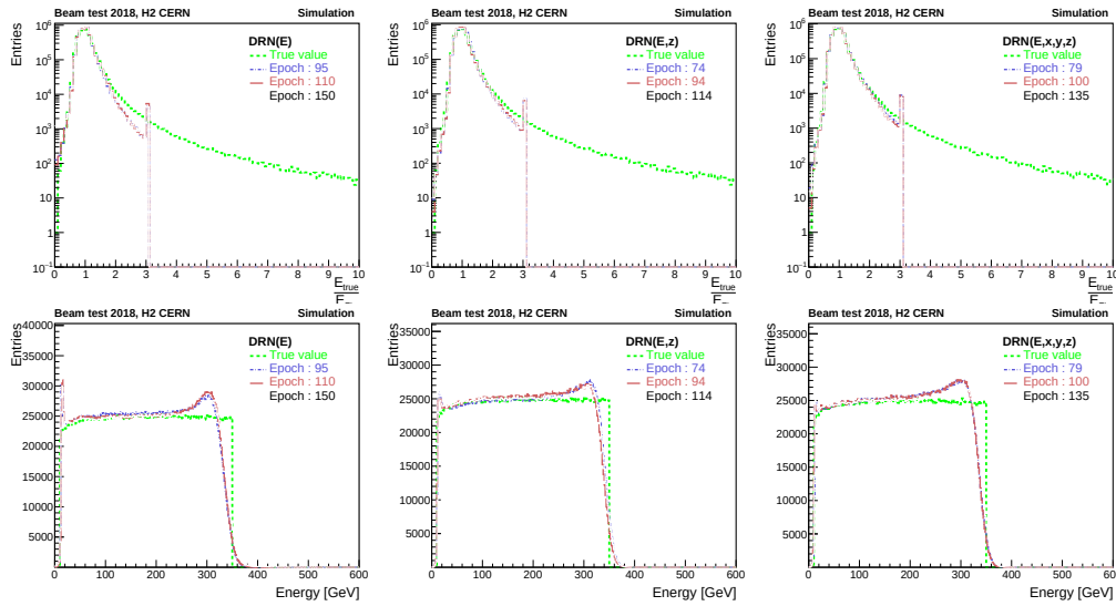
Figure 5.21: The shape of predictions obtained from DRNs (top row), and the shape of predicted energy for flat sample (bottom row), for DRN(E), DRN(E,z) and DRN(E,x,y,z) models from left to right, respectively.
