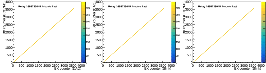
Figure 6.57: The plots compare BX counter values for ECON-D and miniDAQ (left), miniDAQ and Slink (middle), and ECON-D and Slink (right) for the east train. The Slink's BX counter is always 4 ahead of that from ECON-D (HGCROC) and miniDAQ.
