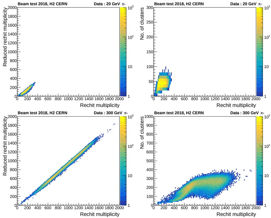
Figure 5.60: The left and right column shows the total number of rechits (X-axis) vs the rechits selected to create the clusters (Y-axis) and total number of rechits(X-axis) vs the total number of clusters created (Y-axis) respectively. Reduction in granularity up to 40-30% and up to \sim 50\% if we reject rechits that are not considered for clustering or consider only clusters respectively.
