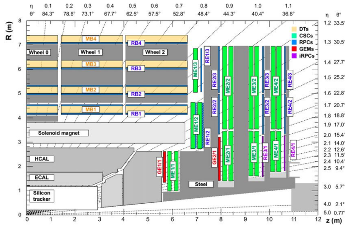
Figure 3.6: The CMS muon spectrometer upgrade project features, highlighted in red (purple), the proposed installations of GEMs and RPCs stations [81].
