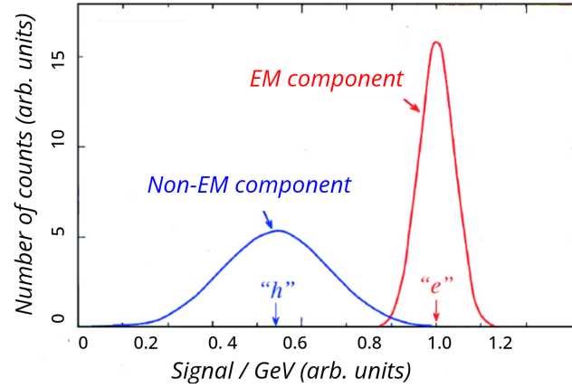
Figure 2.22: The calorimeter's response to both electromagnetic and non-electromagnetic components of hadronic showers is depicted. The width of the non-electromagnetic component reflects the energy deposition fluctuations caused by hadrons [51].
