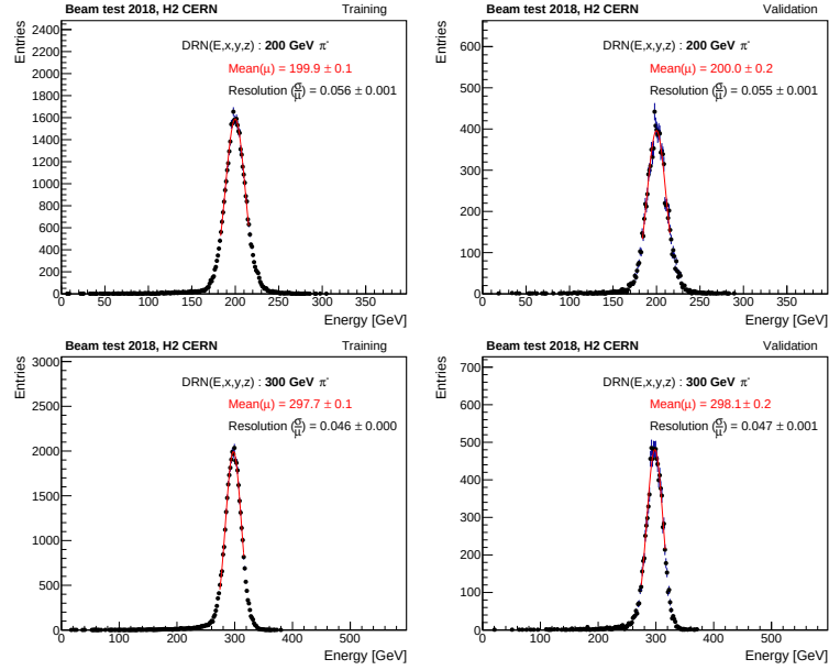
Figure A.10: Energy distributions reconstructed by \text{DRN}(E,x,y,z) along with the Gaussian fitted to extract \sigma and \mu , shown in legend.
