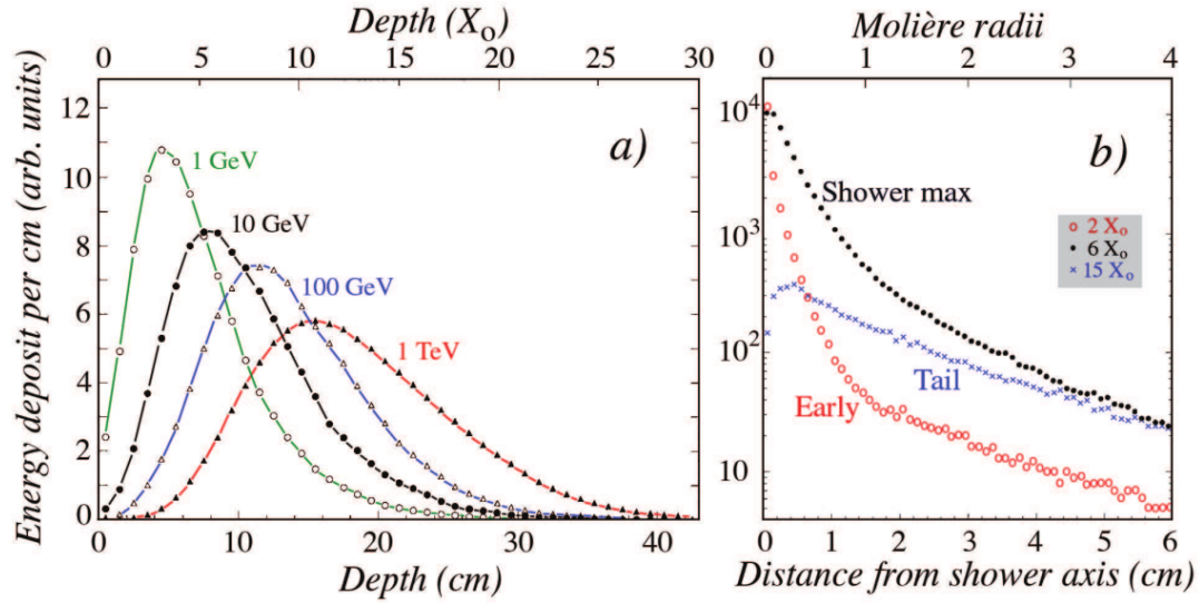
Figure 2.14: Longitudinal energy profiles of electromagnetic showers with different energies (left). The energy distribution profiles from 10 GeV electron showers in copper at different penetration depths (right) [45].
