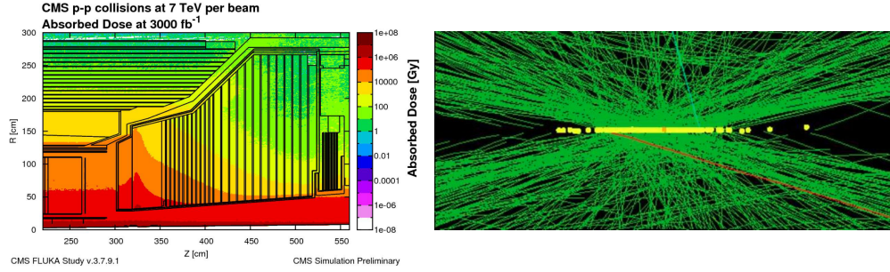
Figure 3.7: Left: The two-dimensional maps in the radial ( r ) and longitudinal ( z ) coordinates are shown for radiation dose accumulated in the CMS detector after an integrated luminosity of 3000 \text{ fb}^{-1} , simulated using the FLUKA program. Right: A model showing multiple p-p interaction vertices (yellow points) during HL-LHC operation, with green lines representing soft particle trajectories from bunch-crossing events [18].
