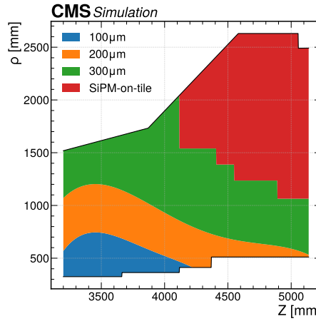
Figure 5.64: Schematic of standalone geometry of expected HGCal configuration showing the boundaries between sections and Si thickness implemented in simulation.
