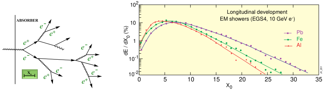
Figure 2.13: (Left) Schematic of electromagnetic shower development. (Right) Longitudinal energy deposition profiles of EM showers for different materials (see text for more details) [47].
