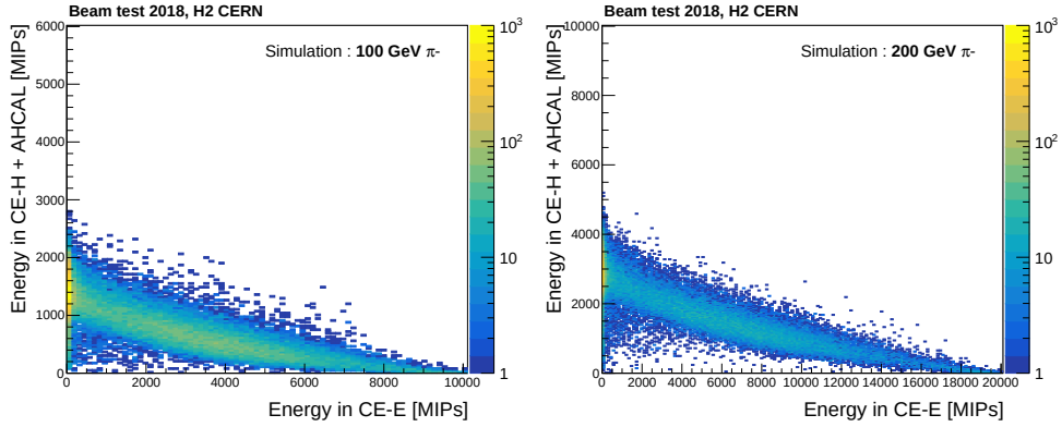
Figure 5.33: Energy measured in electromagnetic and hadronic sections in units of MIPs for 100, and 200 GeV incident pions energies in Simulation.
