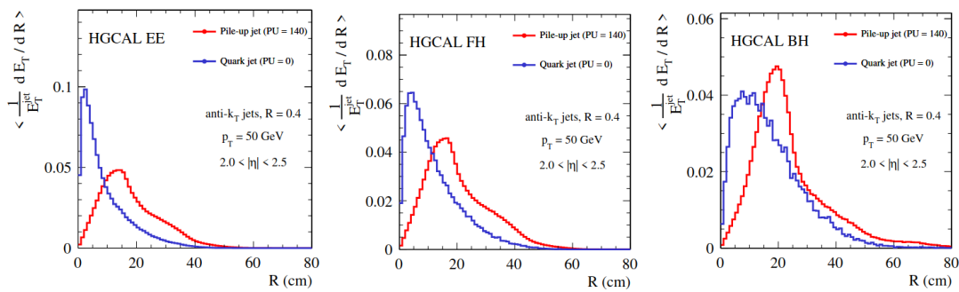
Figure 3.17: Comparison of radial profiles of pileup originated jets (red) and quark originated jets (blue) across the longitudinal depth of HGCAL [94].
