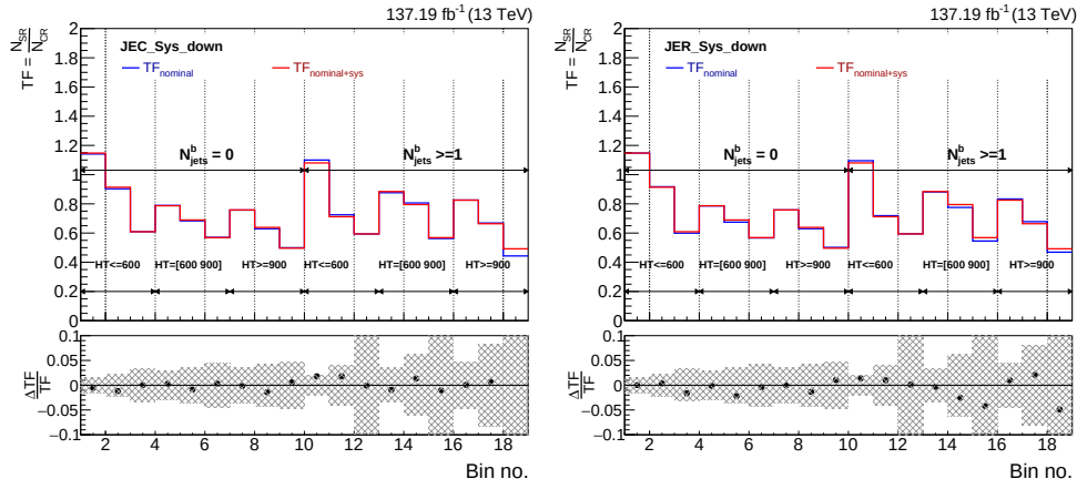
Figure B.1: Top panel: the nominal TF distribution (blue) with the TF (red) obtained with adjusting JEC factors (left) and JER (right) by -1 \sigma uncertainty. Bottom panel: shaded region represents statistical uncertainty, with black points showing TFs' relative discrepancies defined as the ratio of (TF_{\text{nominal}} - TF_{\text{nominal}+\text{sys}}) to TF_{\text{nominal}} .
