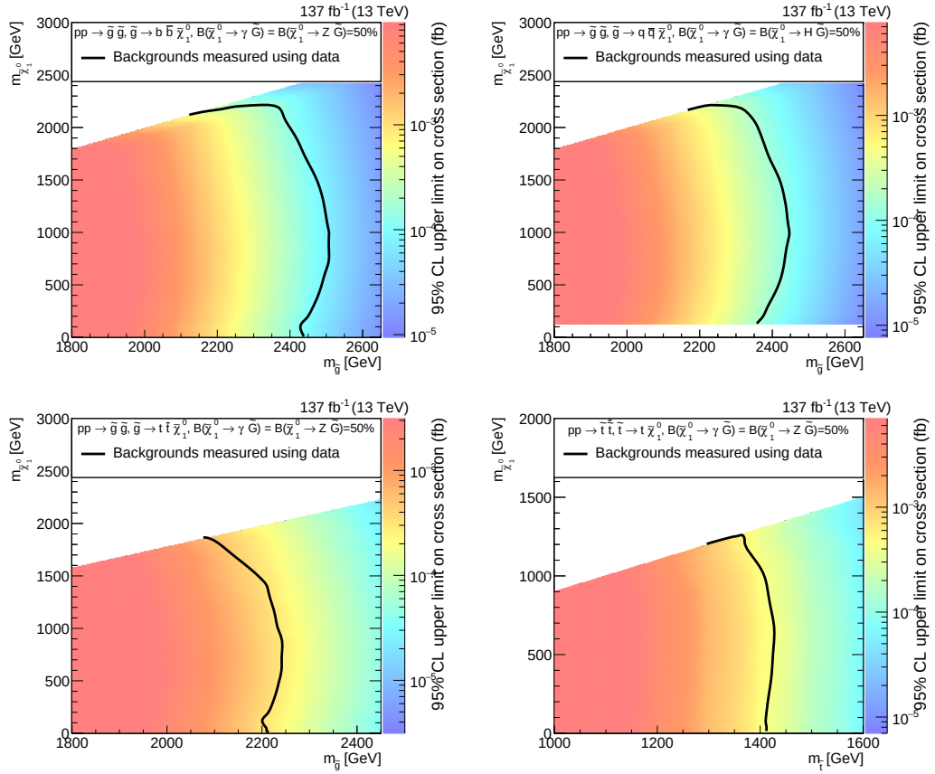
Figure 7.47: Comparison of expected exclusion in data with 95% CL, for T5bbbbZG (top left), T5qqqqHG (top right), T5ttttZG (bottom left) & T6ttZG (bottom right) model.
