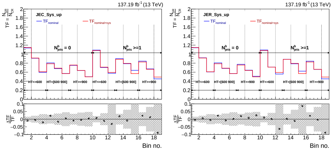
Figure 7.25: Top panel: the nominal TF distribution (blue) with the TF (red) obtained with adjusting JEC factors (left) and JER (right) by +1 \sigma uncertainty. Bottom panel: shaded region represents statistical uncertainty, with black points showing TFs' relative discrepancies defined as the ratio of (TF_{\text{nominal}} - TF_{\text{nominal+sys}}) to TF_{\text{nominal}} .
