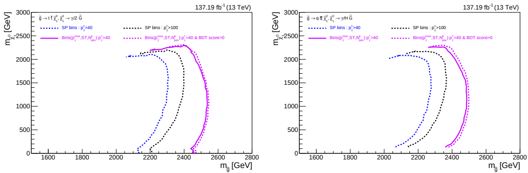
Figure 7.51: The expected exclusion curve, represented by the dotted magenta line for including events with BDT score ( > 0 ) and the solid magenta line for those without such preselection, is shown for T5bbbbZG (left) and T5qqqqHG (right) for comparison.
