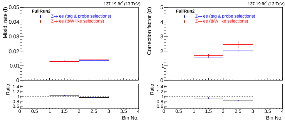
Figure 7.37: A comparison of fake rate obtained using Tag and probe method (blue line) and using W/t\bar{t} like selections (red line) for DY process is shown on left. On the right, comparison of scale factor obtained with different methods is shown.
