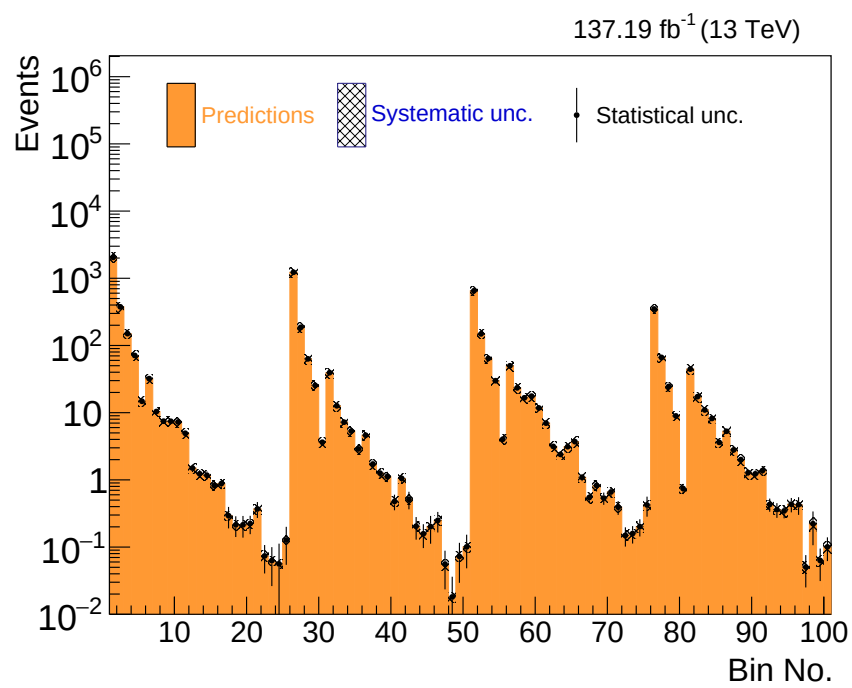
Figure 7.39: The predicted background events in the SRs for electron faking photon background. The black points indicate statistical uncertainty and shaded region represents systematic uncertainty.
