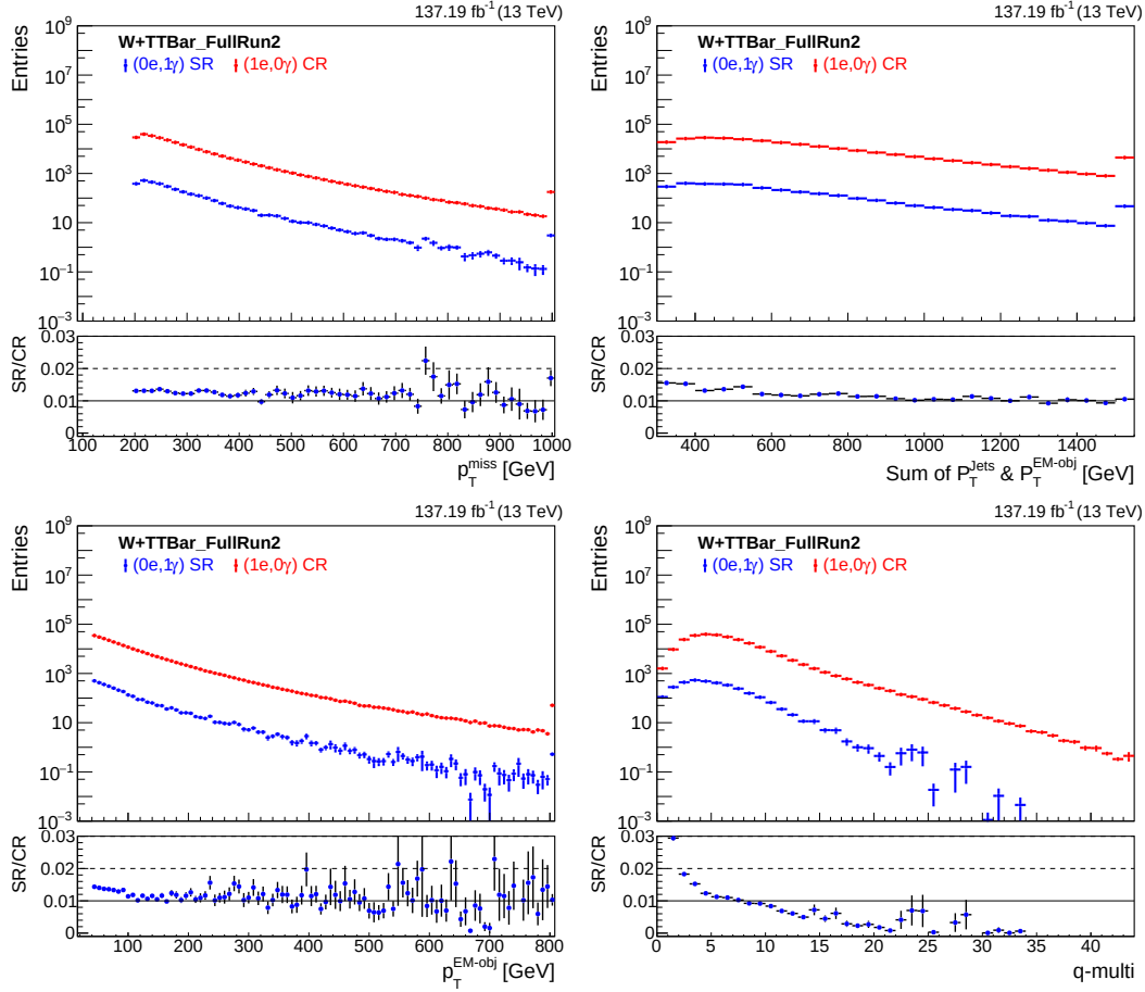
Figure 7.29: p_T^{\text{miss}} (top left), S_T (top right), p_T^{\text{EM-obj}} (bottom left) and the q-multiplicity (bottom right) in single electron CR and photon SR in MC with bottom panel representing the ratio of SR to CR.
