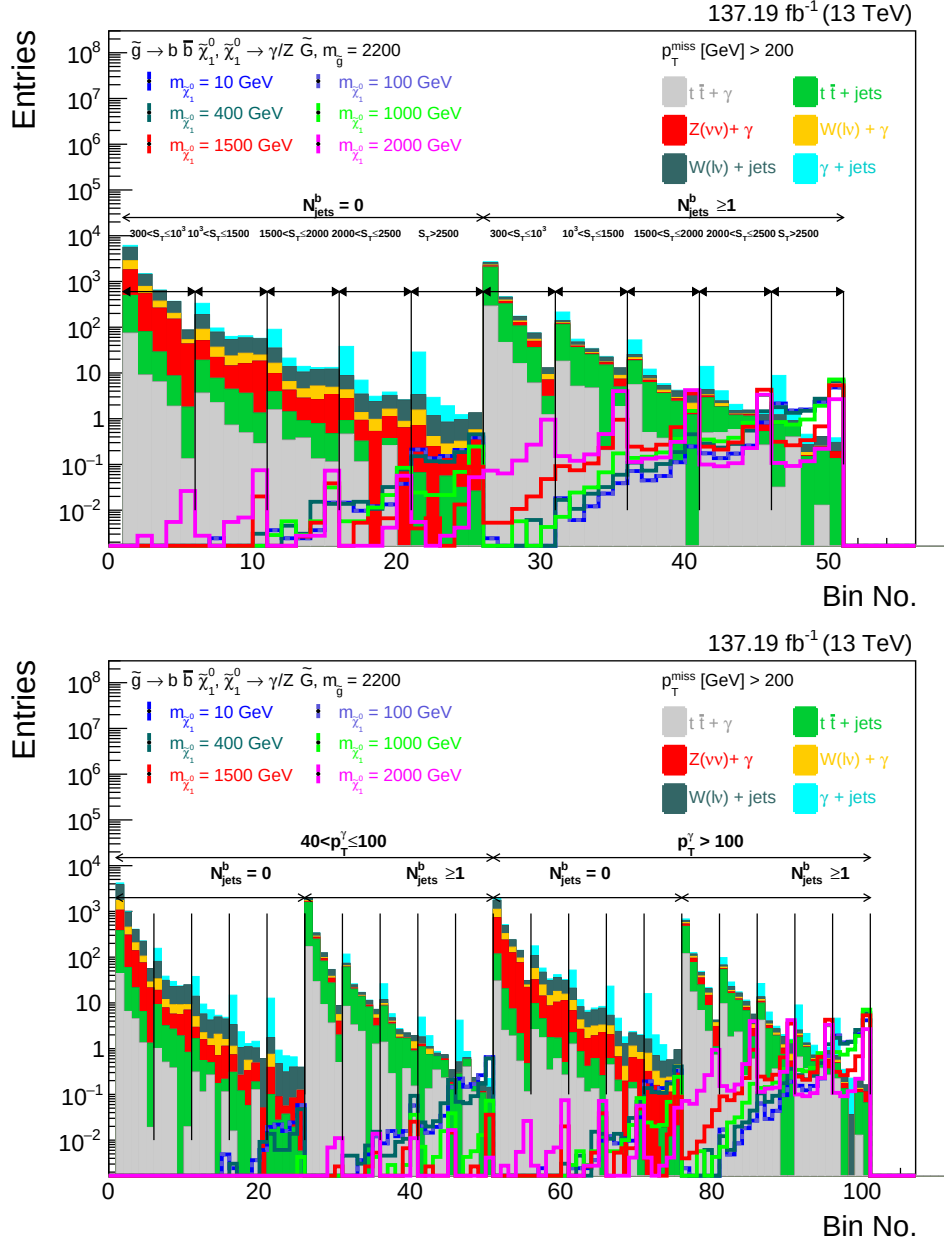
Figure 7.10: The distributions of background and signal events in new SRs based on (p_T^{\text{miss}}, S_T, N_{\text{bjets}}) (top) & (p_T^{\text{miss}}, S_T, N_{\text{bjets}}, \& p_T^\gamma) (bottom) with p_T^\gamma > 40 GeV.
