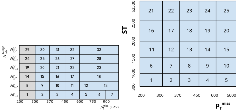
Figure 7.8: Definition of the different bin indexing based on Strong Production (SP) motivated search bins, as derived from (p_T^{\text{miss}}, N_{\text{jets}} \& N_{\text{bjets}}) (left), and the newly established search bins within (p_T^{\text{miss}}, S_T) (right).
