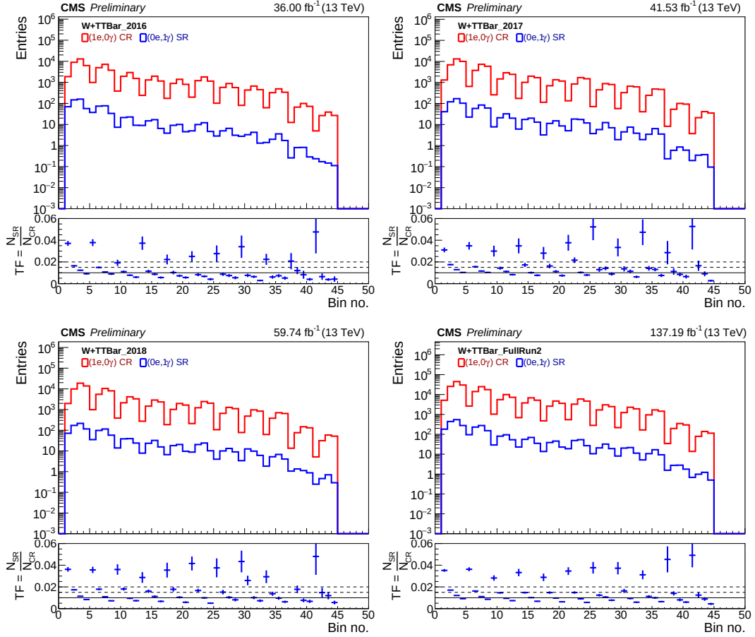
Figure 7.30: CR (red curve) and SR (blue curve) (upper panel) and parametrization of TF (bottom panel) as a function of different bins in p_T^{EM-obj} and q-multiplicity for 2016 (top left), 2017 (top right), 2018 (bottom left) and full Run 2 (bottom right).
