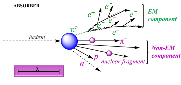
Figure 2.16: Schematic representation of a hadronic interaction in a shower.
