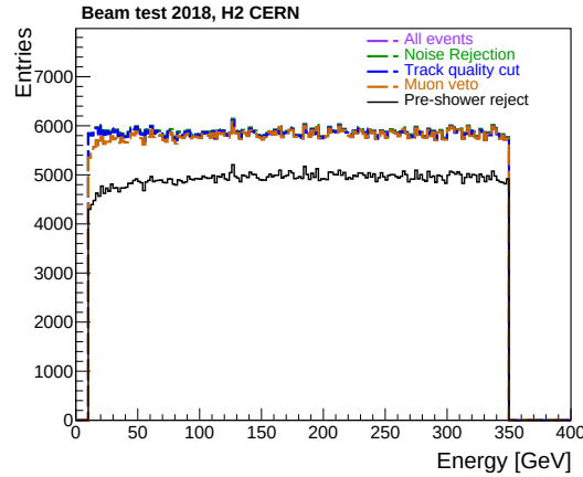
Figure 5.1: Energy distribution of simulated pion sample after sequentially applying event rejection criteria described in the text.
