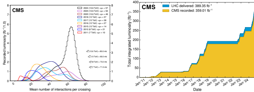
Figure 3.2: Left: Number interactions per event crossing (pileup). Right: The cumulative luminosity delivered and recorded [68].
