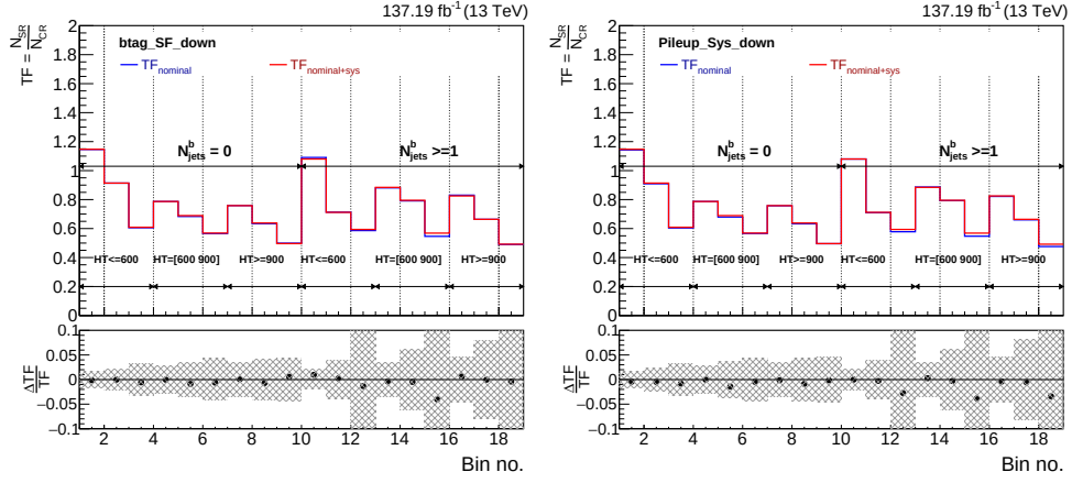
Figure B.2: Top panel: the nominal TF distribution (blue) with the TF (red) obtained with adjusting btag SF (left) and pileup weights (right) by -1\sigma uncertainty. Bottom panel: shaded region represents statistical uncertainty, with black points showing TFs' relative discrepancies defined as the ratio of (TF_{\text{nominal}} - TF_{\text{nominal+sys}}) to TF_{\text{nominal}} .
