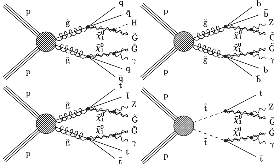
Figure 7.2: The strong production simplified SUSY models, T5qqqqHG (top left), T5bbbbZG (top right), T5ttttZG (bottom left), and T6ttZG (bottom right).
