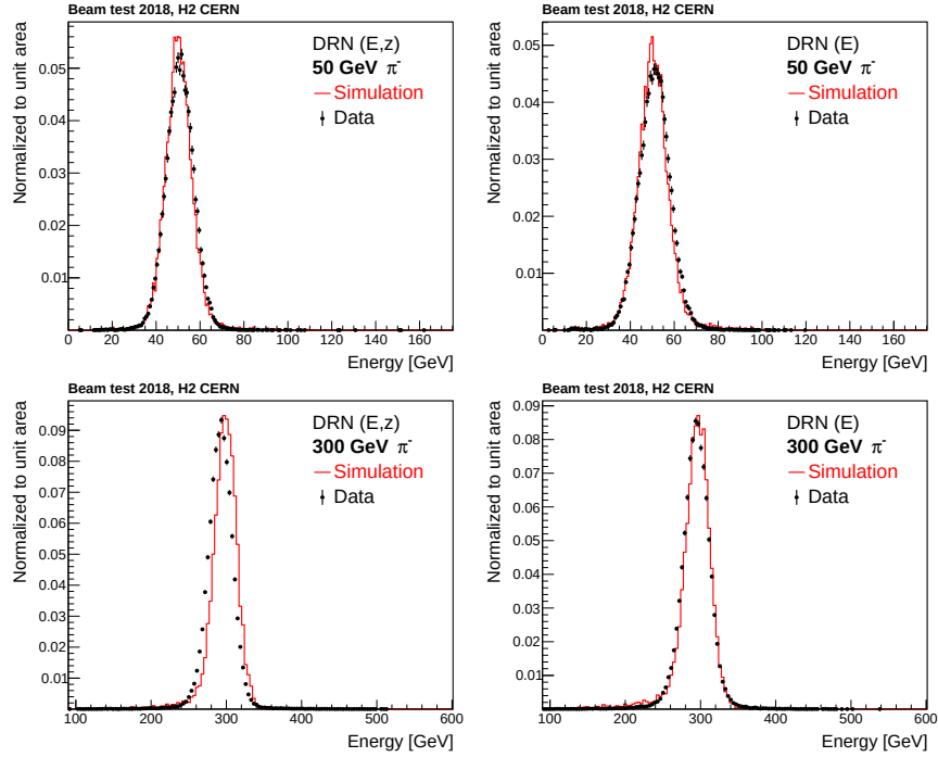
Figure 5.39: Distribution of energy predicted by the DRN(E,z) (left) and DRN(E) (right) model on hadron showers generated by pions of true energy 50 and 300 GeV in beam test HGCAL prototype detector and its simulation.
