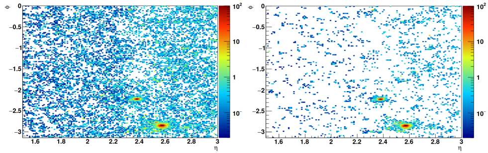
Figure 3.18: Depicted is a singular event illustrating the VBF process with the decay H \rightarrow 2\gamma , where one photon and a pair of VBF jets are confined to one quadrant of HGICAL, projected onto its outer surface [94].
