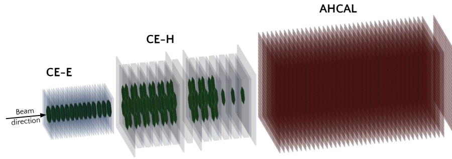
Figure 3.21: Simulated geometry of the CE-E, CE-H and AHCAL detector prototypes depicting the position of active layers and absorbing material.
