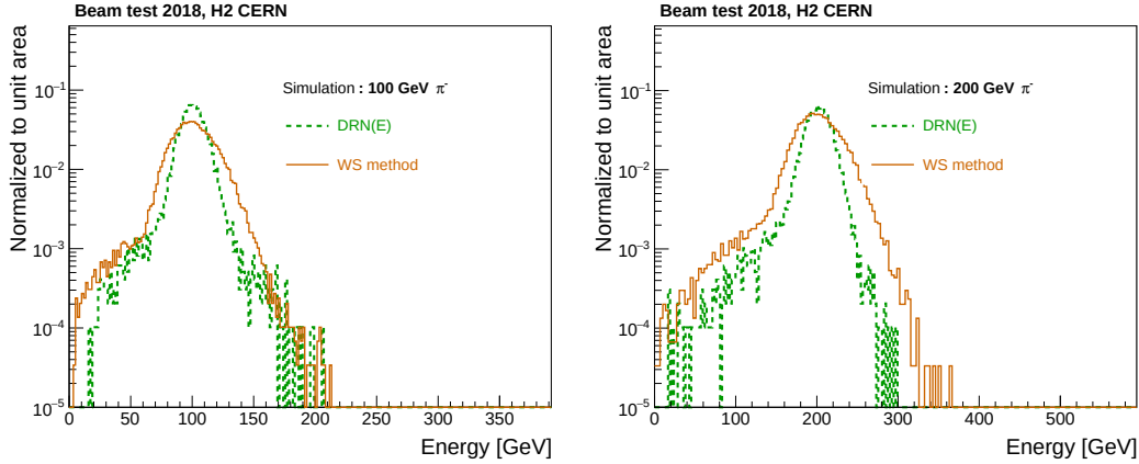
Figure 5.28: Comparisons of energy distributions predicted using different DRN(E) and WS method 100, and 200 GeV pions for validation datasets.
