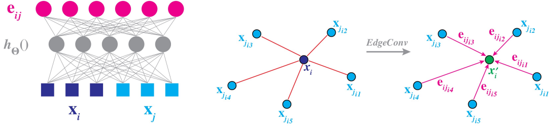
Figure 4.7: Left: The derivation of an edge feature ( e_{ij} ) (top), based on a pair of points, x_i and x_j (bottom), utilizing the function h_{\theta}() defined in text. Right: The EdgeConv mechanism computes the result by aggregating the edge features of all edges emanating from each connected vertex. [115]
