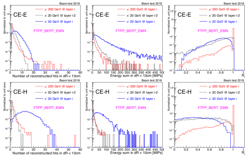
Figure 5.44: The left column shows reconstructed hits, the middle displays energy comparisons, and the right illustrates lateral energy ratios. The top row refers to CE-E, and the bottom to CE-H, contrasting muons with 20 GeV pions at the start layer of the shower and the one before [102].
