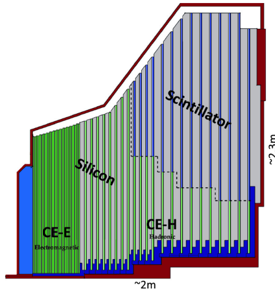
Figure 3.11: The cross sectional view of HGCAL detector highlighting its Silicon and Scintillator based CE-E and CE-H sections [94].
