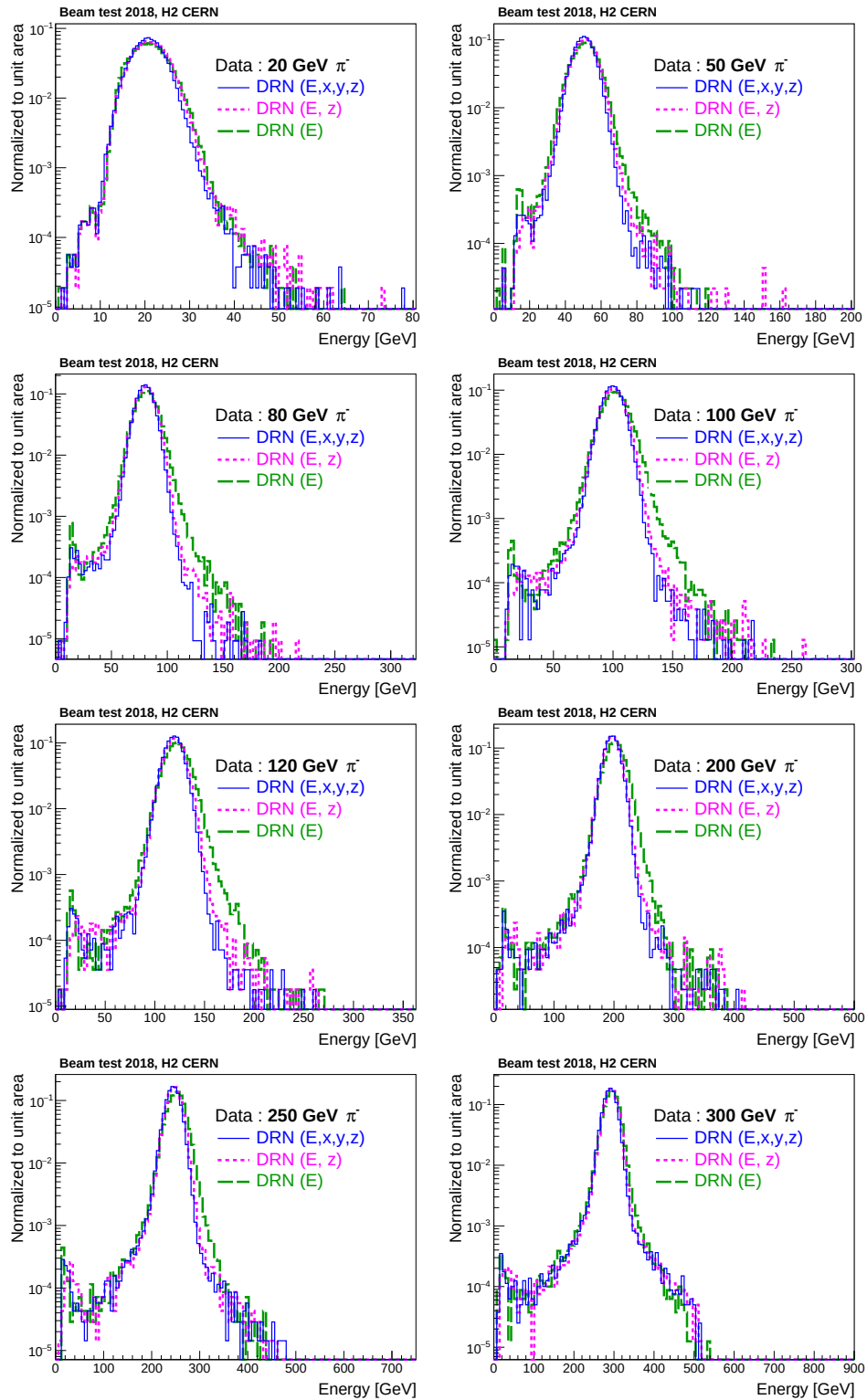
Figure A.15: Distributions of energies predicted using different DRN models for 20, 50, 80, 100, 120, 200, 250 and 300 GeV pions on data recorded in the beam test setup.
