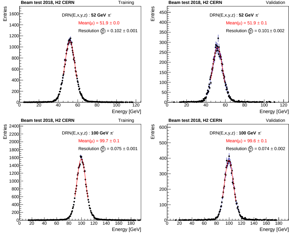
Figure 5.23: Energy distributions reconstructed by \text{DRN}(E,x,y,z) along with the Gaussian fitted to extract \sigma and \mu , shown in legend.
