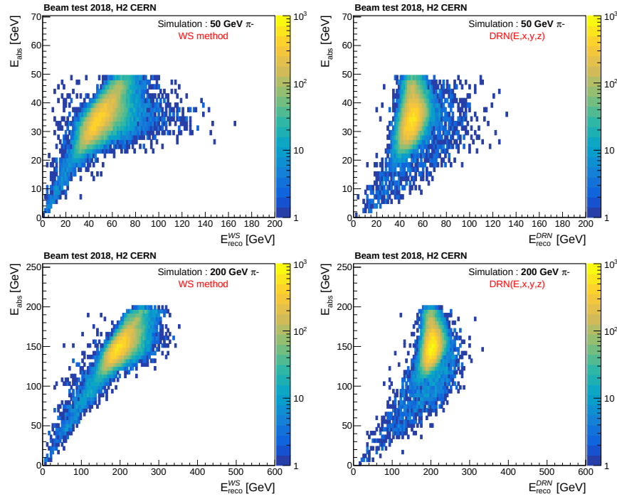
Figure 5.50: Reconstructed energies using WS method (left) and DRN( E,x,y,z ) (right), as a function of E_{abs} for 50 (top) and 200 (bottom) GeV pions. The E_{reco} using WS method is showing a linear dependence on the E_{abs} and DRN is able to compensate and reconstruct correctly even for the smaller values of E_{abs} .
