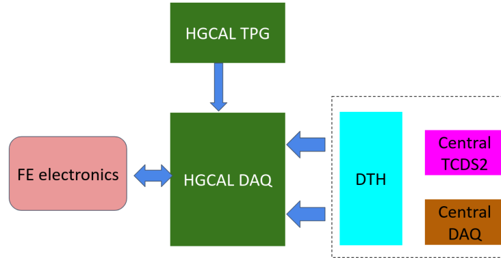
Figure 6.9: Schematic showing the interfaces of different systems with BE DAQ system [94].
