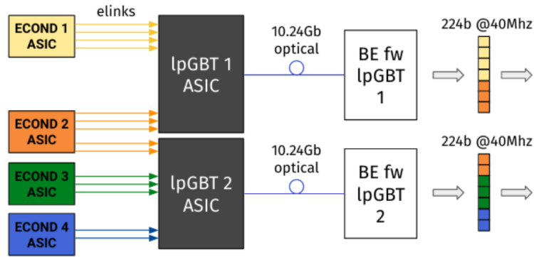
Figure 6.11: An illustration of ECON-D to lpGBT mapping. [149].
