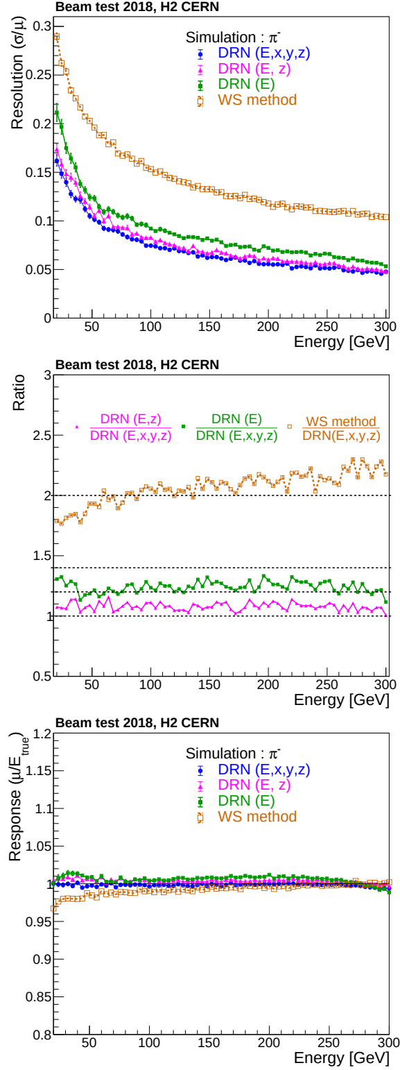
Figure 5.30: Resolution (top), ratio of resolution to DRN(E,x,y,z) (middle), and response (bottom) as function of pion energy obtained from the three models trained with different features in simulation.
