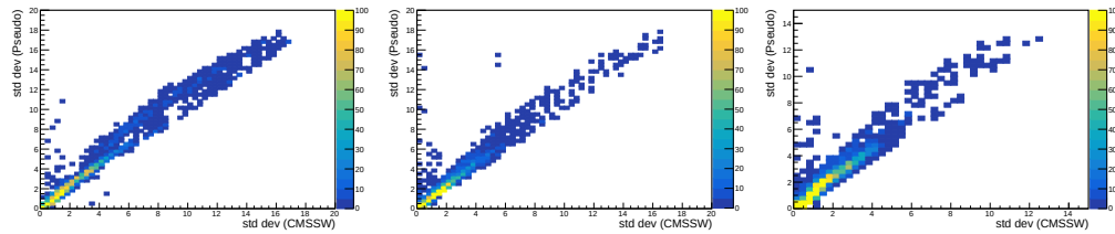
Figure 6.24: The comparison standard deviation of occupancy distributions obtained from pseudo events (Y axis) and CMSSW (X axis) for n10 , n20 , n30 formats shown from left to right, respectively.
