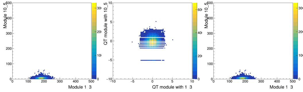
Figure 6.20: The plots show the correlations of the module at (1,3) with module at (10,5) in terms of occupancies: from CMSSW (left), after quantile transformation to Gaussian (middle), and after inverse QT back to the original space (right).
