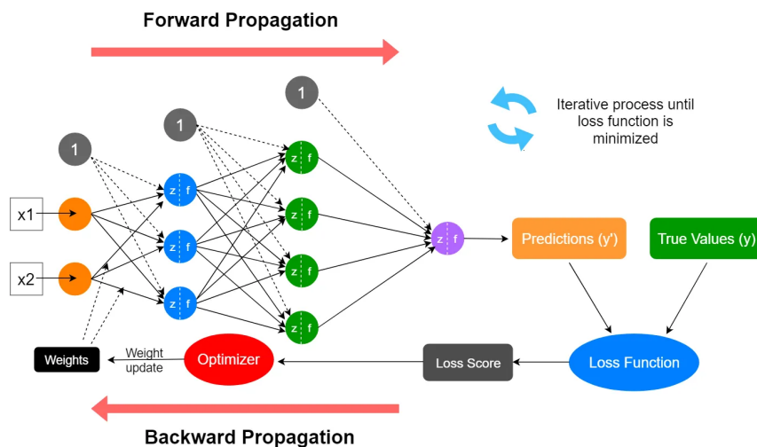
Figure 4.4: The learning mechanism of a neural network, emphasizing the forward and backward propagation processes [113].
