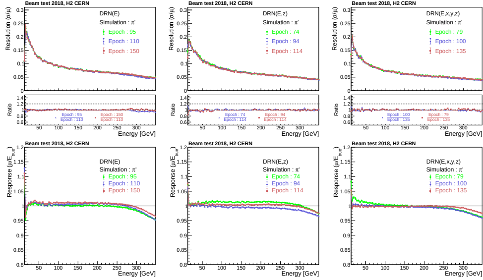
Figure 5.25: Energy resolution (top) and response (bottom) versus incident pion energies for various DRNs are compared at different epochs on the validation dataset. Epochs 110 th , 114 th , and 135 th are chosen for DRN(E), DRN(E,z), and DRN(E,x,y,z), respectively, as the best for further studies.
