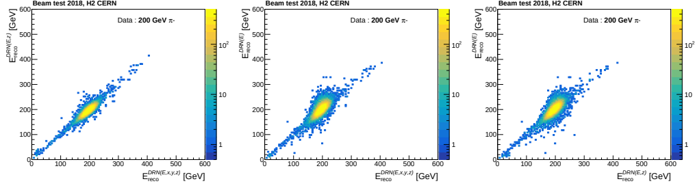
Figure 5.41: Event by event comparisons of the energy reconstructed for 200 GeV pions in data using DRN( E,x,y,z ) with DRN( E,z ), DRN( E,x,y,z ) with DRN( E ), and DRN( E,z ) with DRN( E ) in the first, second and third rows.
