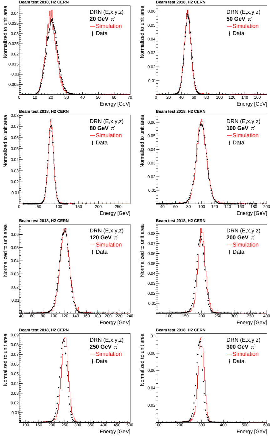
Figure 5.38: Distribution of energy predicted by the DRN( E,x,y,z ) on hadron showers generated by pions of true energy 20, 50, 80, 100, 120, 200, 250 and 300 GeV in beam test HGCAL prototype detector and its simulation. The bulk is matching well in simulation and data within few-%.
