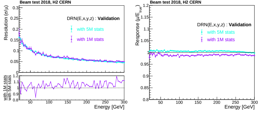
Figure 5.13: Energy resolution (left) and response (right) comparisons from DRN trained on 5M and 1M events for validation datasets. Bottom panel shows the resolution ratio of 1M to 5M event statistics.
