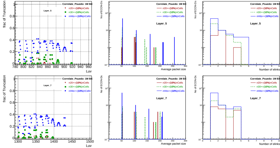
Figure 6.36: The ECON-Ds featuring non-zero truncation, represented by their respective luvs (left), mean packet size (center), and associated count of active elinks (right), are illustrated when 10% of nCells is added to layer 5 (top row) and 7 (bottom row).
