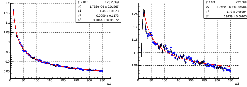
Figure A.2: The energy dependent weights \alpha, \beta, \gamma extracted as a function of energy using \chi^2 minimization for pions start showering in CE-H (CE-H pions) are shown above. A parametric function has been fitted to extract these weights for any energy values.
