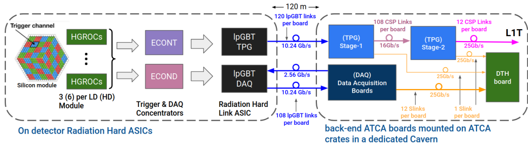
Figure 6.1: Schematic diagram showing the key components of the readout system of HGCAL [139].
