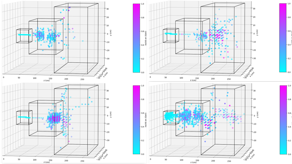
Figure 5.9: Displays of showers within the beam test geometry for 100 GeV (top) and 300 GeV (bottom) pions.
