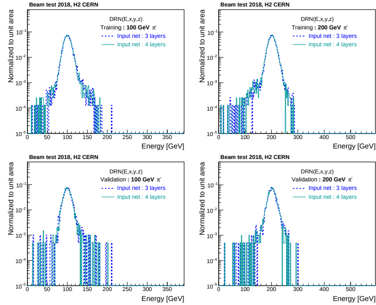
Figure A.3: Comparisons of reconstructed energy distributions for 100 (left) and 200 (right) GeV pions using DRN trained with 4 layers or 3 layers in its input net for training (upper row) and validation (bottom row) datasets.
