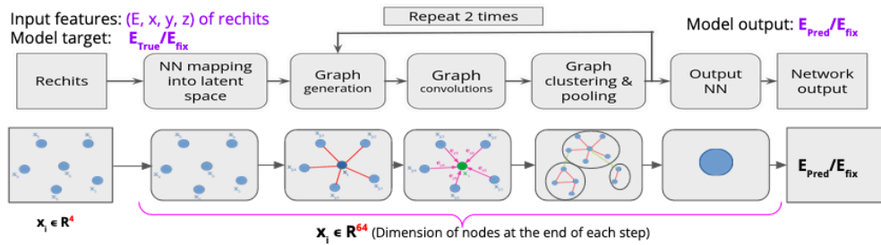
Figure 4.10: This diagram shows a GNN-based dynamic reduction network. Rechits are labeled as x_i , with red lines indicating their latent space connections, refined by graph convolution in magenta. In the graph clustering stage, clusters are small circles with blue dot nodes inside. Final predictions are made through the output neural network.
