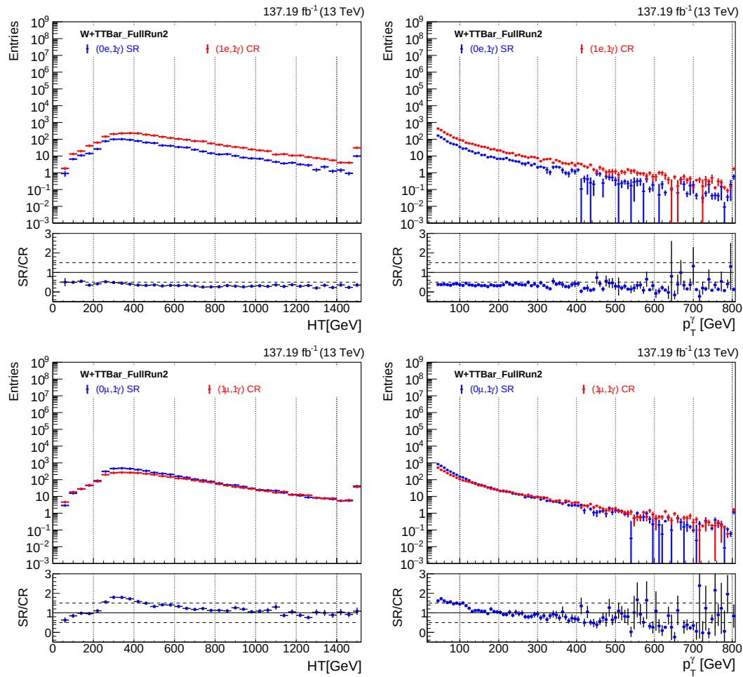
Figure 7.17: Distributions of H_T (left column), p_T^\gamma (right column) are shown in CR (red curve) and SR (blue curve) for lost electron case (top row) and lost muon + \tau - hadronic using MC with complete Run 2 luminosity. The bottom panel of the plots represents the ratio of SR events yields to CR in different bins.
