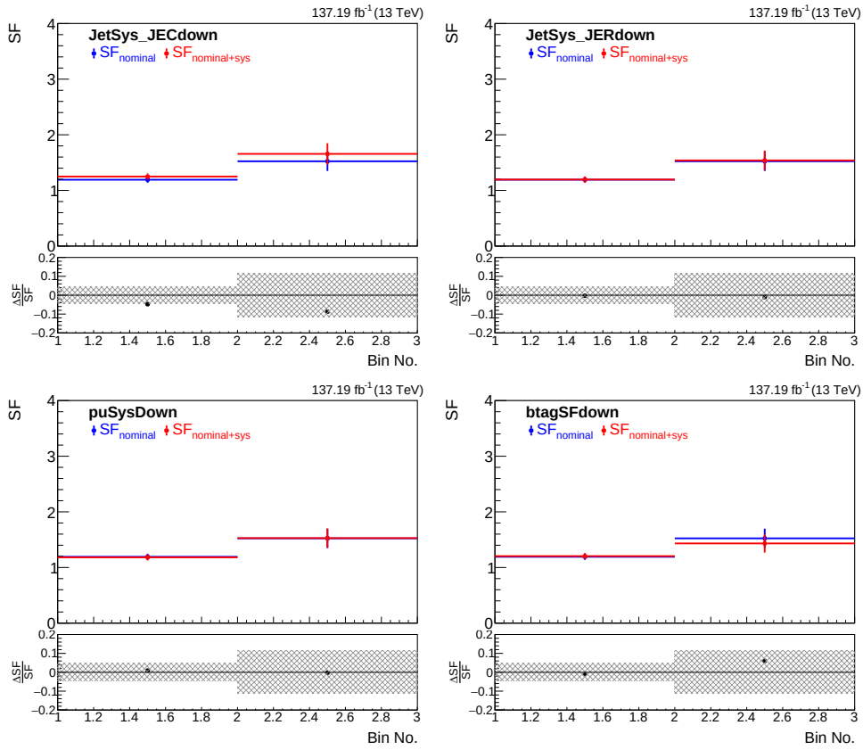
Figure B.4: Comparison of nominal \alpha or SF (in blue) with \alpha after varying the JEC factors (top left) and JER (top right) by -1\sigma_{sys} , and varying the pile up weights (bottom left) and scale factor of b-tagging (bottom right) are shown in the top panel. Shaded region represents the statistical uncertainty in the bottom panel and black points are showing relativistic differences in the \alpha or SF defined as the ratio of (\alpha_{nominal} - \alpha_{nominal+sys}) to \alpha_{nominal} .
