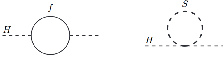
Figure 2.4: One-loop quantum corrections to the Higgs squared mass parameter m_H^2 from a Dirac fermion f (left) and for a scalar S (right). [12]
