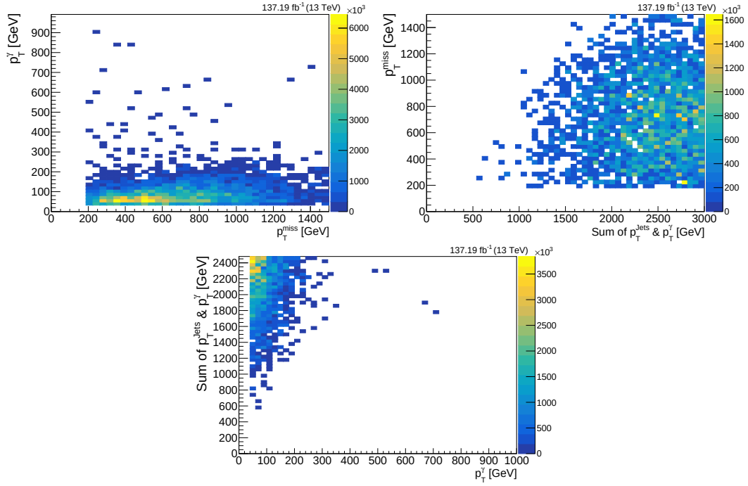
Figure 7.13: The distributions of p_T^{\text{miss}} versus p_T^\gamma (top), S_T versus p_T^{\text{miss}} (middle), and S_T versus p_T^\gamma (bottom), with m_{\tilde{\chi}_2^0} = 100 GeV and \Delta m = 10 GeV in T5gg model.
