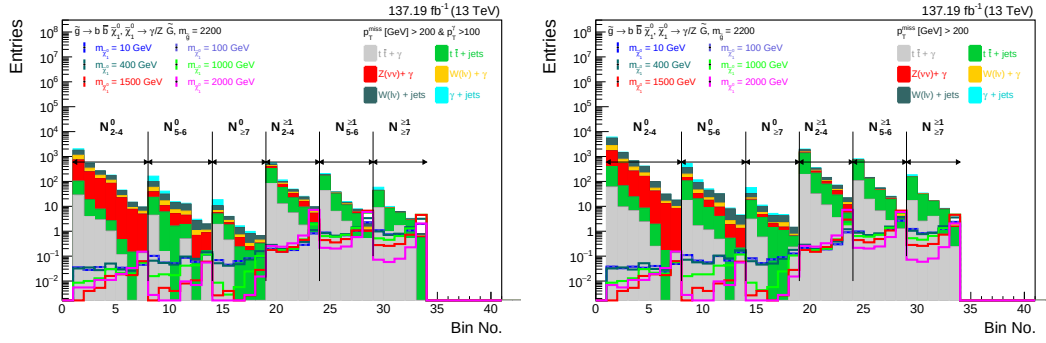
Figure 7.9: The distributions of background and signal events in SP bins with p_T^{\gamma} > 100 GeV (left) and p_T^{\gamma} > 40 GeV (right).
