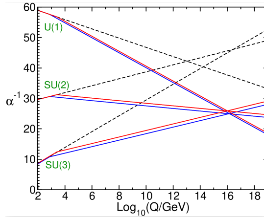
Figure 2.5: Examination of two-loop renormalization group behavior for inverse gauge couplings \alpha_a^{-1}(Q) within the SM (dashed) versus the MSSM (solid). In MSSM analysis, sparticle mass thresholds range from 750 GeV to 2.5 TeV, with \alpha_3(m_Z) ranging between 0.117 and 0.120. [12]
