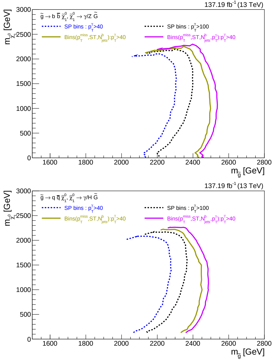
Figure 7.11: The expected exclusion limits at 95% confidence interval (CL) for T5bbbbZG (top) and T5qqqqHG (bottom) models with different SRs. The new SR bins in Magenta line shows improvement in mass exclusion by 200 GeV in both the models.
