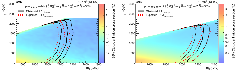
Figure 7.1: The observed and expected exclusion at 95% confidence level for T5bbbbZG (left) and T5ttttZG (right) achieved in previous round of analysis [16] with high p_T^\gamma . The exclusion limits are worse for smaller NLSP masses given Gluino mass.
