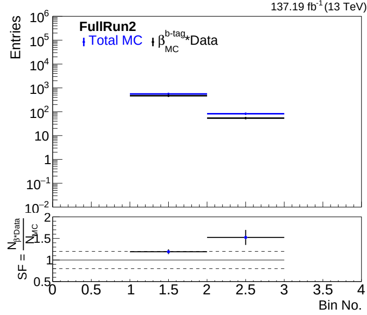
Figure 7.43: Data-MC correction factor ( \alpha ) in N_{bjets} bins is shown in the bottom panel.
