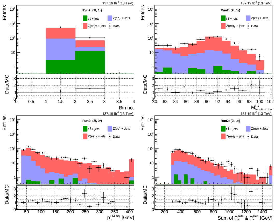
Figure 7.41: Data-MC comparisons in dilepton control region in terms of N_{\text{bjets}} (top left), m_{\ell\ell} (top right), p_T^\gamma (bottom left) and S_T (bottom right) with bottom panel as the data to MC ratio. The non-DY contributions are not mitigated from data yet.
