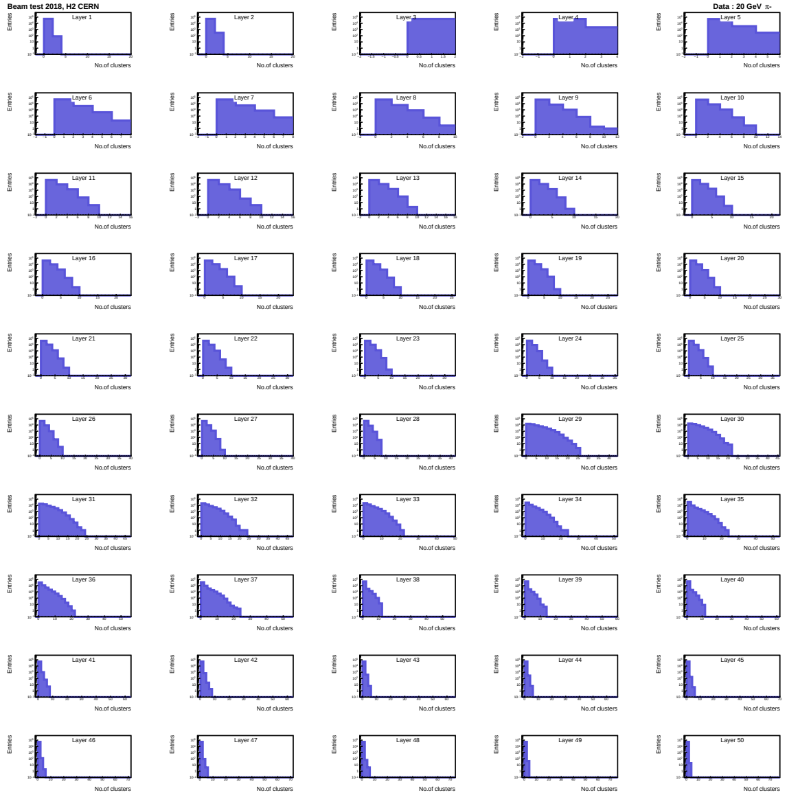
Figure A.20: Number of clusters per layer for 20 GeV pions in beam test data.
