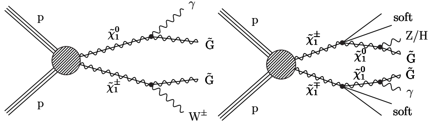
Figure 7.3: Simplified electroweak production SUSY models, TChiWG (left) and TChiNG (right).
