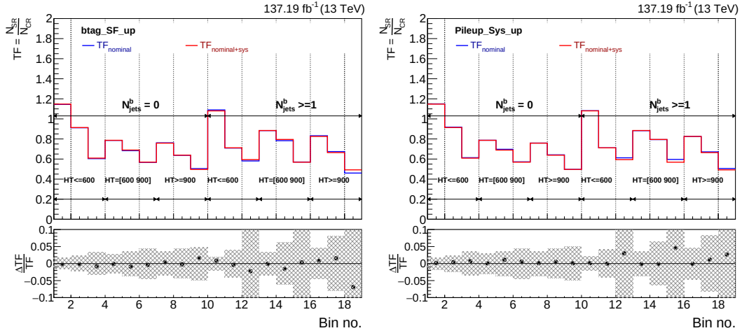
Figure 7.26: Top panel: the nominal TF distribution (blue) with the TF (red) obtained with adjusting btag SF (left) and pileup weights (right) by +1\sigma uncertainty. Bottom panel: shaded region represents statistical uncertainty, with black points showing TFs' relative discrepancies defined as the ratio of (TF_{nominal} - TF_{nominal+sys}) to TF_{nominal} .
