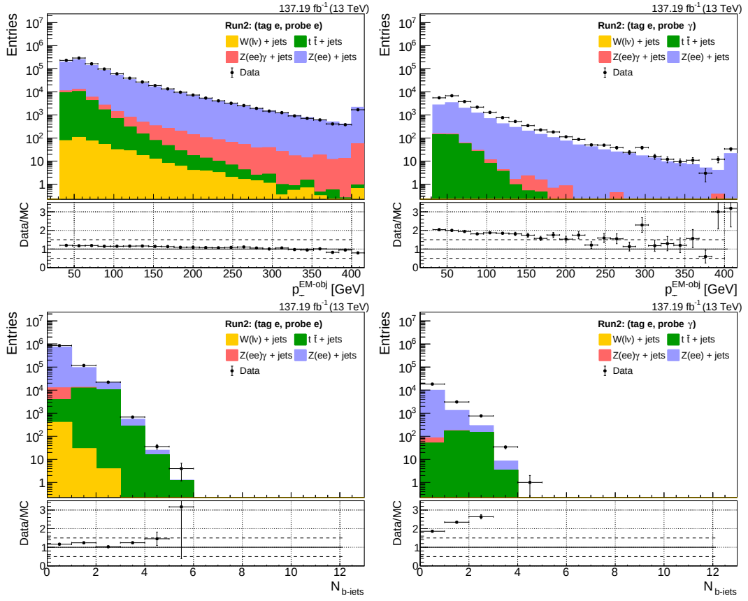
Figure 7.33: For categories where the probe is an electron (first column) and \gamma (second column), MC and data event distributions are shown as functions of p_T^{\text{probe}} (top) and N_{\text{b-jets}} (bottom), with the data-MC ratio across bins.
