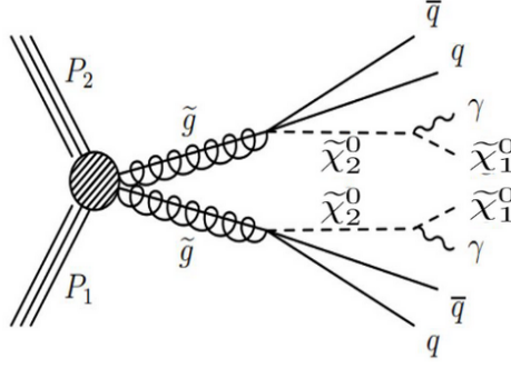
Figure 7.4: The T5gg model, inspired by scenarios within the pMSSM, illustrating the production of gluino pairs.
