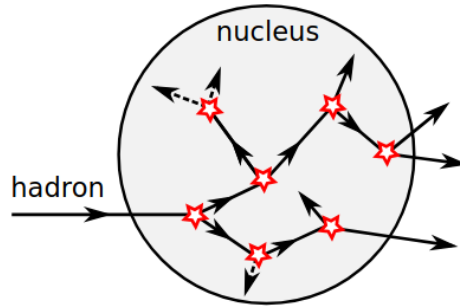
Figure 2.24: Illustrated operational concept of cascade models realized in GEANT4 [64].
