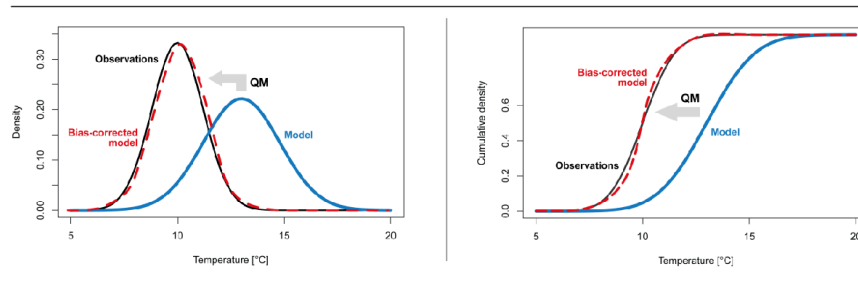
Figure 6.19: This example shows how a biased simulated distribution (blue) is adjusted to match the observed distribution (black) using PDF (left) and CDF (right). The corrected distribution (dashed red) closely resembles the observed distribution, although exact matching might be hindered by sampling uncertainty or QM implementation specifics [153].
