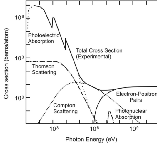
Figure 2.11: Dominant photon interaction processes as a function of incident photon energy [44].
