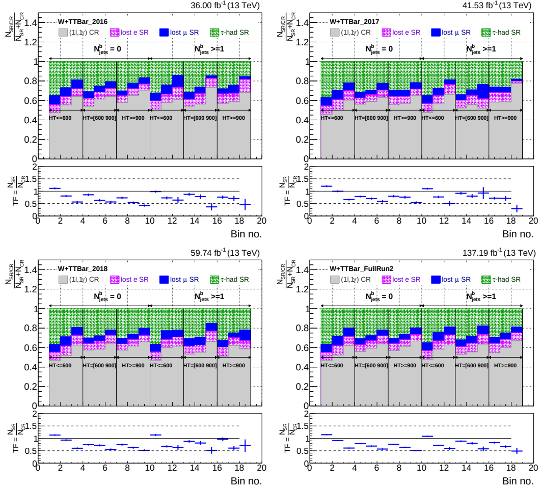
Figure 7.19: The fractional distributions of lost electrons, lost muons, and tau hadronic SRs along with the total CR, which combines single electron and muon CR, are depicted as a function of different TF bins for datasets from the years 2016 (top left), 2017 (top right), 2018 (bottom left), and Run 2 (bottom right). The bottom panel of the plots illustrates the transfer function derived for each respective bin.
