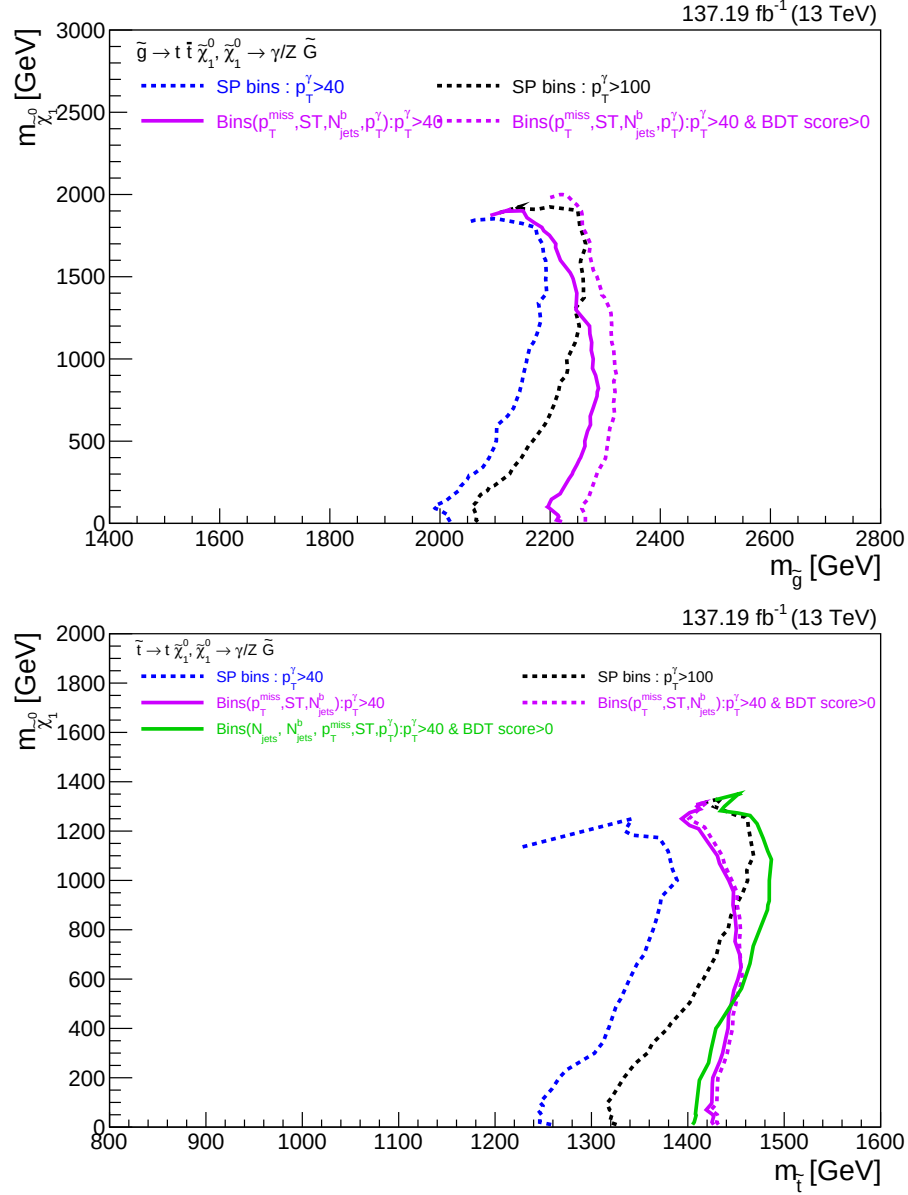
Figure 7.52: The expected exclusion curve, represented by the dotted magenta line for including events with BDT score ( > 0 ) and the solid magenta line for those without such preselection, is shown for T5ttttZG (top) and T6ttZG (bottom) for comparison. Additionally, limits obtained with using N_{\text{jets}} as one of search variables is shown in green curve for T6ttZG.
