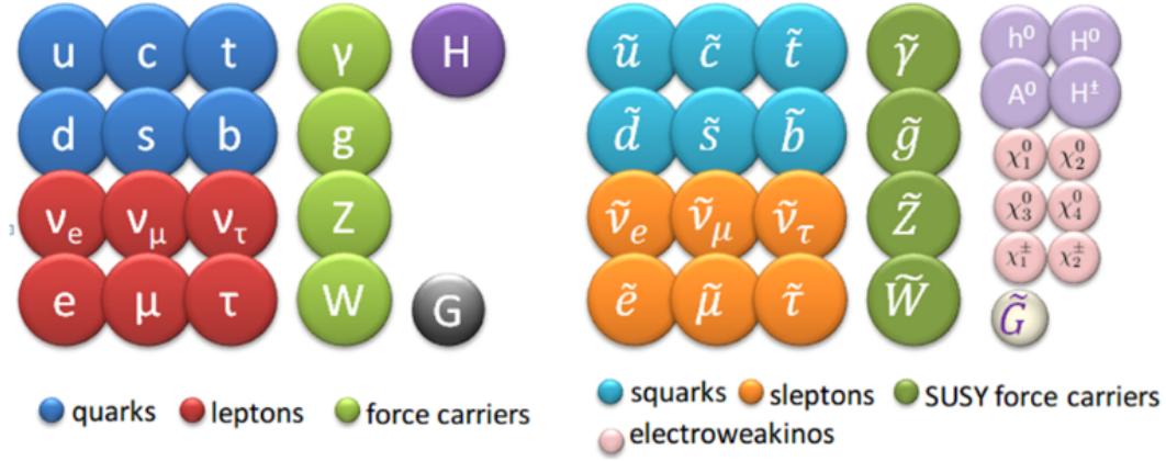
Figure 2.6: Different particles within the MSSM framework. [35]
