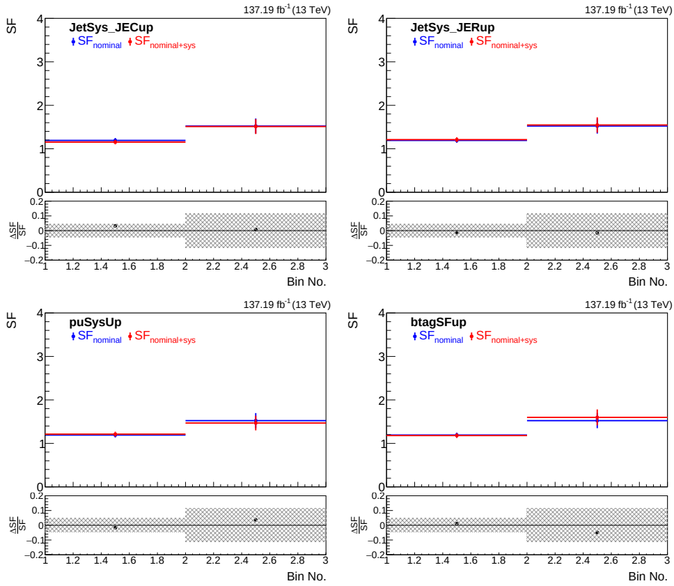
Figure 7.44: Comparison of nominal \alpha or SF (in blue) with \alpha (SF) after varying the JEC factors (top left) and JER (top right) by \pm 1\sigma_{sys} , and varying the pile up weights (bottom left) and scale factor of b-tagging (bottom right) are shown in the top panel. Shaded region represents the statistical uncertainty in the bottom panel and black points are showing relativistic differences in the \alpha defined as the ratio of (\alpha_{nominal} - \alpha_{nominal+sys}) to \alpha_{nominal} .
