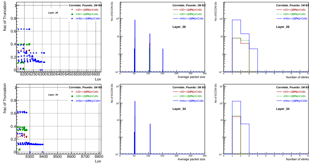
Figure 6.37: The ECON-Ds featuring non-zero truncation, represented by their respective luvs (left), mean packet size (center), and associated count of active elinks (right), are illustrated when 10% of nCells is added to layer 26 (top row) and 34 (bottom row).
