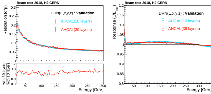
Figure 5.11: Energy resolution (left) and response (right) as functions of incident pion energy for DRNs with 39 versus 10 sampling layers in AHCAL on validation dataset. The left bottom panel compares resolutions obtained with 39 versus 10 sampling layers.
