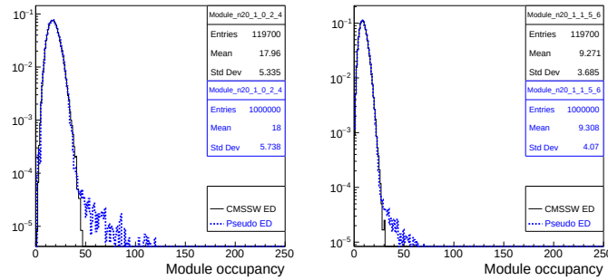
Figure 6.27: Module occupancy in CMSSW and pseudo events. These are the modules where the corresponding ECON-D buffers have higher occupancy with pseudo events compared to CMSSW events.
