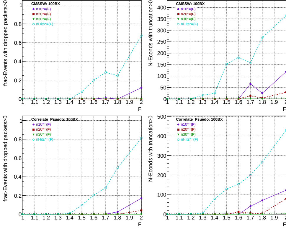
Figure 6.30: The left column shows the percentage of events with dropped packets or incomplete events, and the right column shows the average number of ECON-Ds truncated per event as a function of scale factor for n10 , n20 , and n30 individually. Data is from CMSSW (top row) and pseudo events (bottom row).
