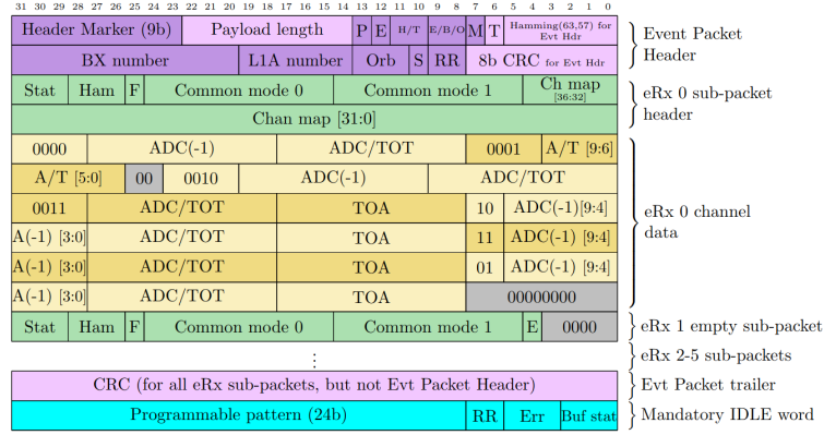
Figure 6.6: The above is the standard data format from the ECON-D [145].
