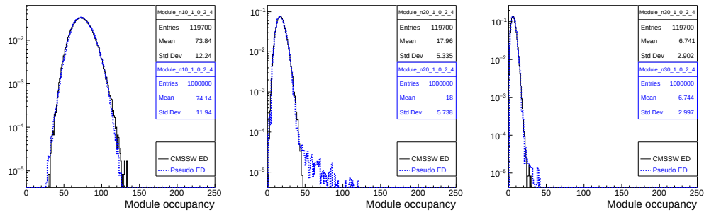
Figure 6.22: Shapes of n10 occupancy distributions from CMSSW & from Pseudo event generation.
