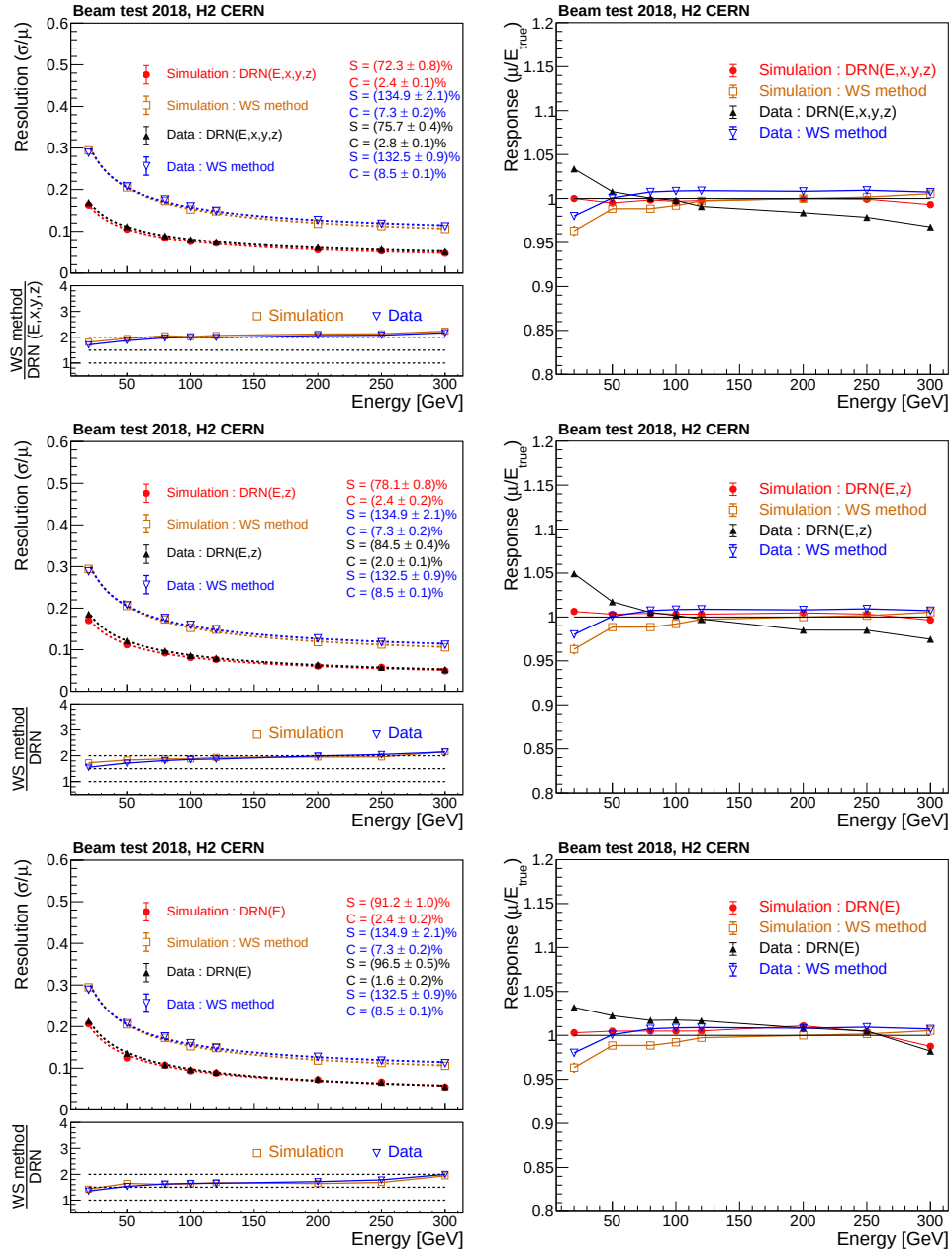
Figure 5.42: Energy resolution (left) and response (right) of pion showers reconstructed in beam test data and simulation using WS method and DRN(E,x,y,z) (top), DRN(E,z) (middle) and DRN(E) (bottom) models. The resolution curve is fitted with the functional form \sqrt{S^2/E + C^2} where S and C are the stochastic and constant term governing the resolution for any calorimeter.
