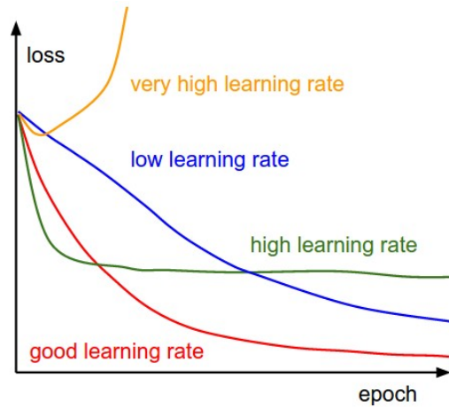
Figure 4.2: An illustration shows that low learning rates lead to gradual progress, while higher rates cause rapid improvements but can get stuck at non-optimal loss values (green line) [110].
