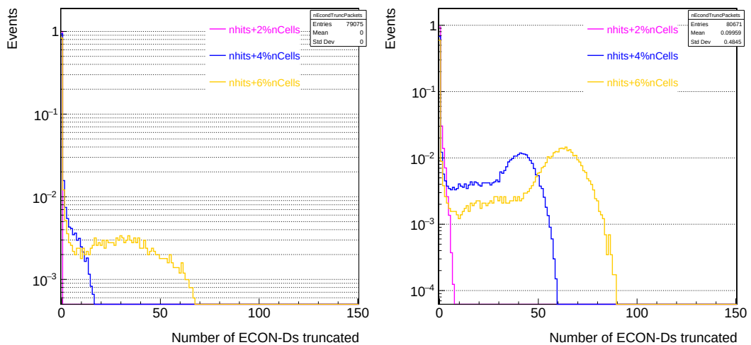
Figure 6.46: Distributions of ECON-D numbers with event truncation for different fractions of nCells added to nhits across all modules for High and low watermarks are 1850 (2550) and 1450 (2150) shown in left and right, respectively.
