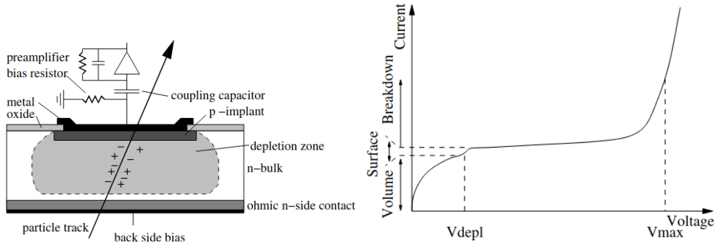
Figure 2.19: Left: Illustration of a charged particle ionizing and creating the e-h pairs in the silicon sensor. Right: The behavior of dark current (when no signal is present) versus the voltage applied between p-n junction [48].
