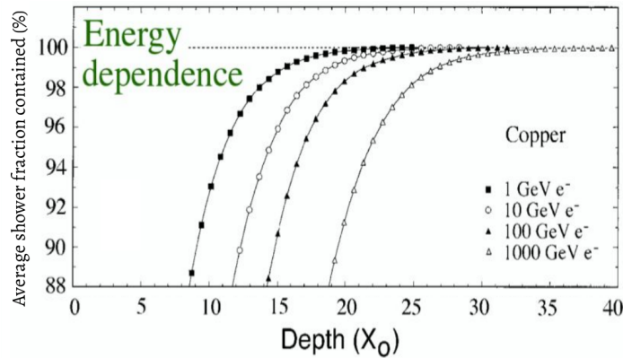
Figure 2.15: The average energy fraction retained in a material block with infinite transverse dimensions as a function of absorber thickness for different electron energy levels. [45].
