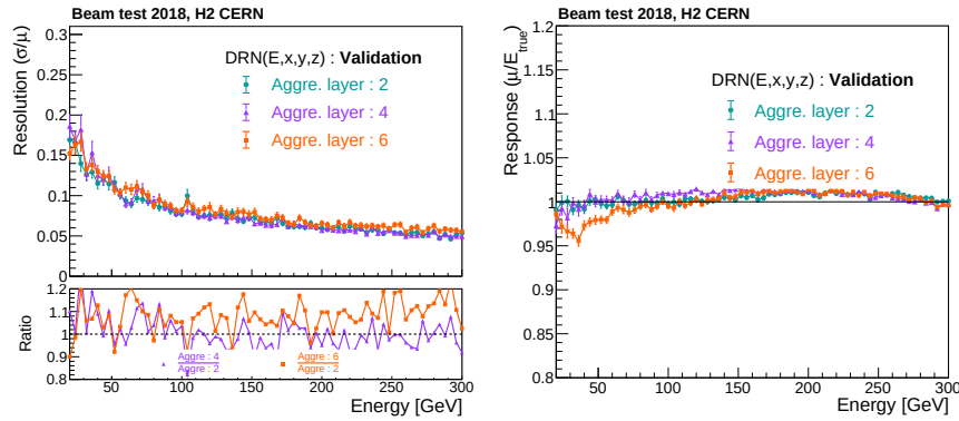
Figure 5.15: Energy resolution (left) and response (right) versus incident pion energy for DRN models with 2, 4, and 6 aggregation layers on validation datasets. The ratio panel on left shows resolution ratios using 4 and 6 layers compared to 2 layers.
