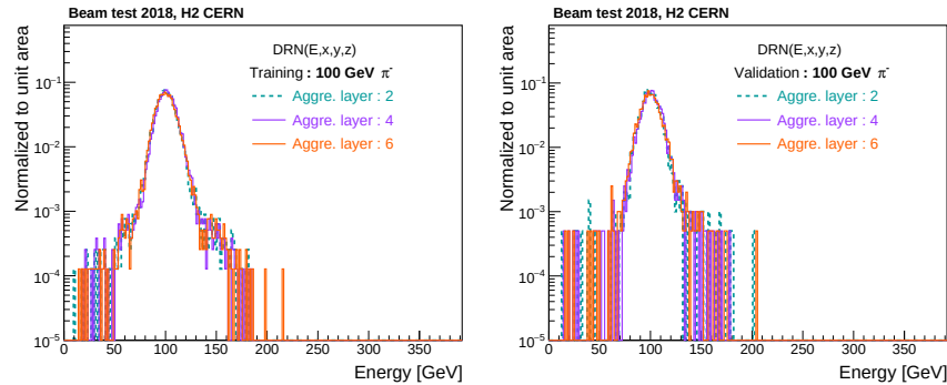
Figure 5.14: Distributions of reconstructed energy for pions of 100 GeV in training (left) and validation (right) datasets using DRNs with different aggregation layers.
