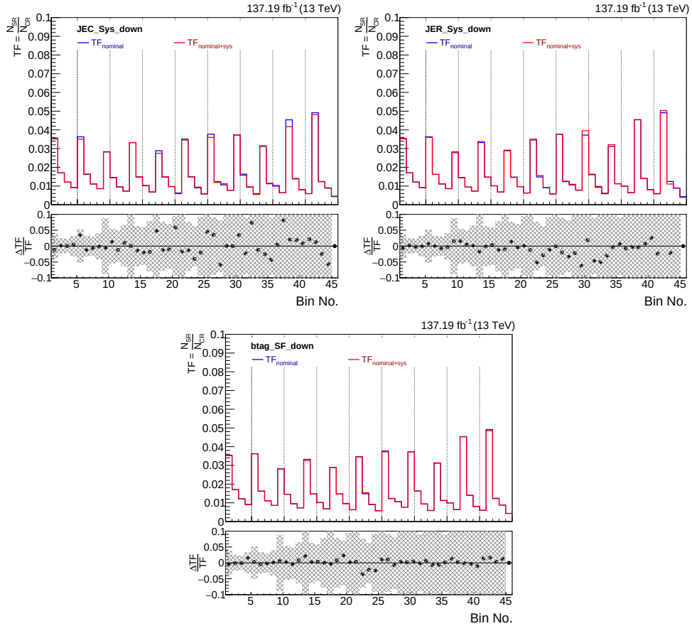
Figure B.3: Comparison of nominal TF (in blue) with TF after varying the JEC factors (top left) and JER (top right) by -1\sigma_{\text{sys}} , and varying the scale factor of b-tagging (bottom) are shown in the top panel. Shaded region represents the statistical uncertainty in the bottom panel and black points are showing relativistic differences in the TF defined as the ratio of (TF_{\text{nominal}} - TF_{\text{nominal+sys}}) to TF_{\text{nominal}} .
