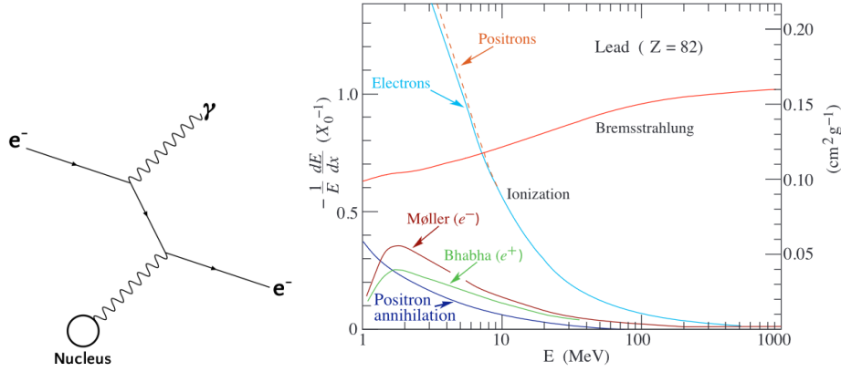
Figure 2.10: Feynman diagram on the left illustrates the Bremsstrahlung mechanism. On the right, the plot shows the fractional energy loss per radiation length in lead as a function of the electron's energy. [1]
