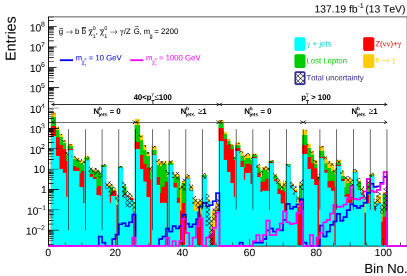
Figure 7.46: Background events in the SRs comprise stacked histograms of lost lepton, fake photon, and Z(\nu\bar{\nu}) + \gamma predictions in data, as well as simulated QCD multijet + \gamma +jets. The gray-shaded area indicates statistical uncertainty including a 20% systematic error. The open histograms illustrate the T5bbbbZG signal distribution within SRs for m_{\tilde{g}} = 2.2 TeV, comparing m_{\tilde{\chi}_1^0} = 10 GeV (blue) and = 1000 GeV (magenta).
