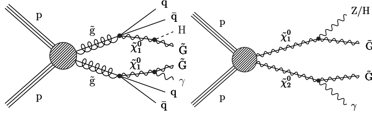
Figure 2.8: Simplified model of Gluino pair strong production (T5bbbbZG) (left) and direct production of neutralinos(right).
