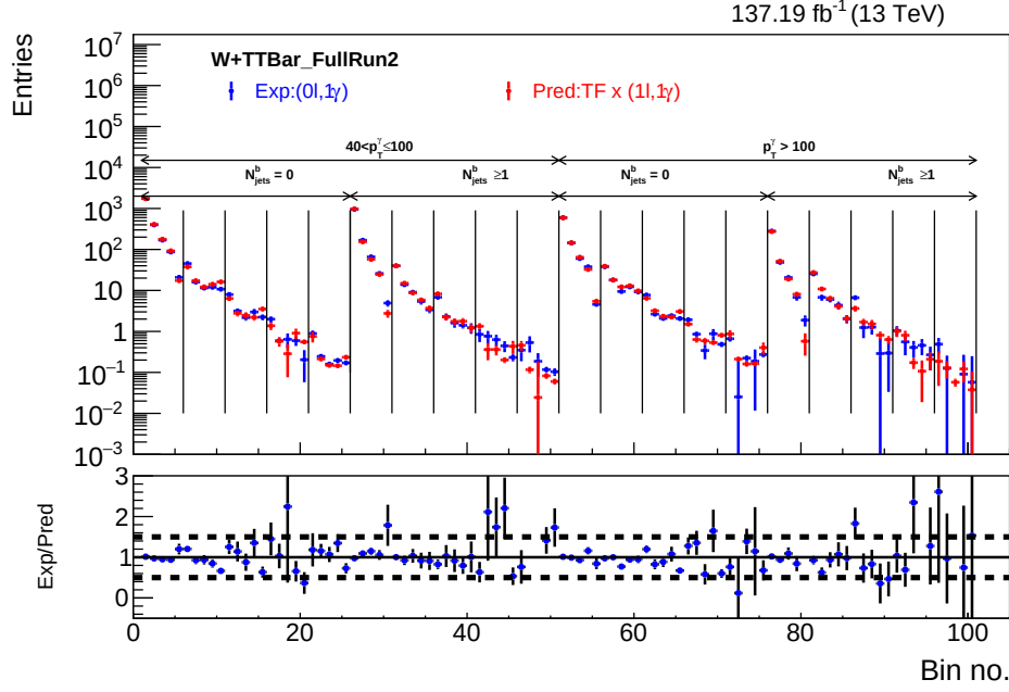
Figure 7.21: The comparison between the anticipated SR derived from MC (blue markers) and the SR predicted using equation 7.4 (red markers) is illustrated. The bottom panel of the plots delineates the ratio between the expected and predicted signal regions.
