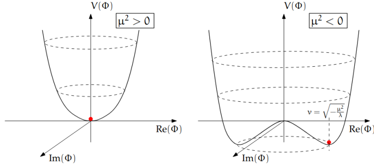
Figure 2.3: Representation of Higgs potential for different values of \mu^2 [29].
