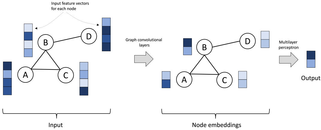
Figure 4.6: Diagrammatic representation of the fundamental architecture of Graph convolutional networks (GCNs), elucidating the operation of the graph convolutional (message-passing) layer. [117]
