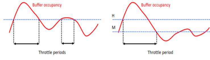
Figure 6.39: Above schematic shows the impact on throttling time if we have single throttling threshold or double throttling thresholds.
