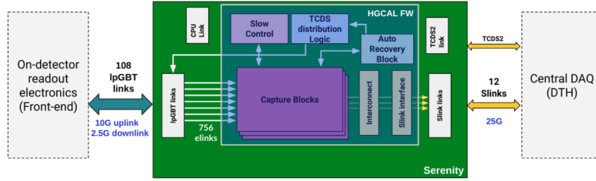
Figure 6.10: Schematic highlighting the key parts of DAQ firmware designed for HGCAL [149].
