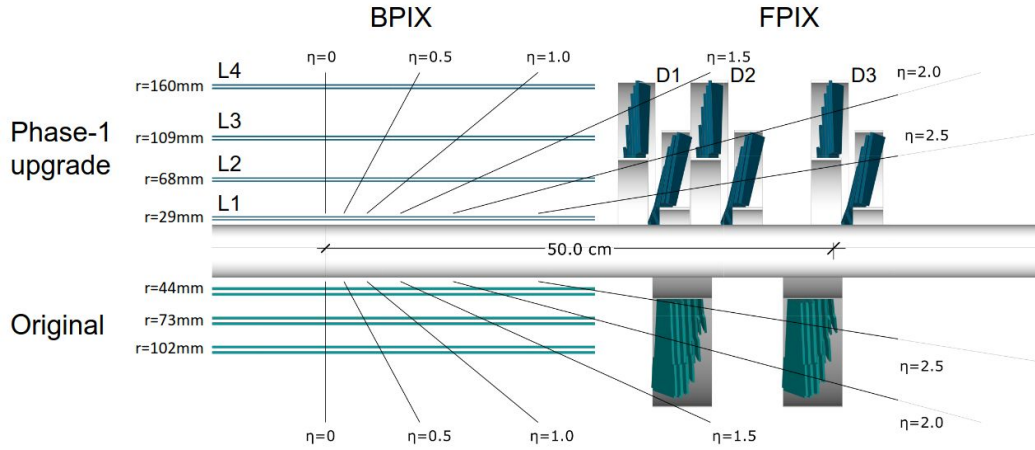
Figure 3.4: The structural configuration of the CMS Phase-1 pixel detector, shown in a longitudinal perspective, is compared with that of the initial detector's arrangement. [79]
