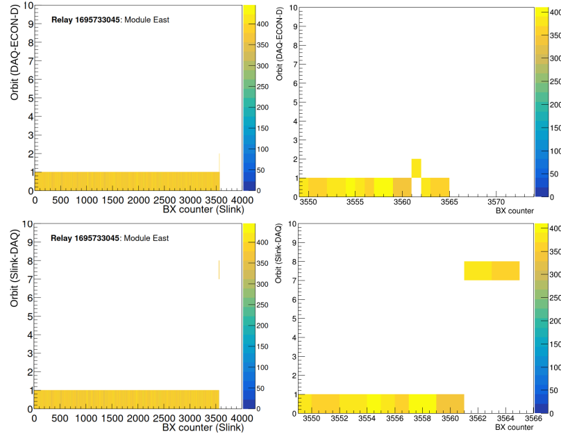
Figure 6.60: The difference between the Orbit counters versus the Slink BX where L1A is issued, for miniDAQ and ECON-D (top left), for Slink and miniDAQ (bottom left) are shown. Zoomed in version of the left plots are added on right side. (with a different Y axis label).
