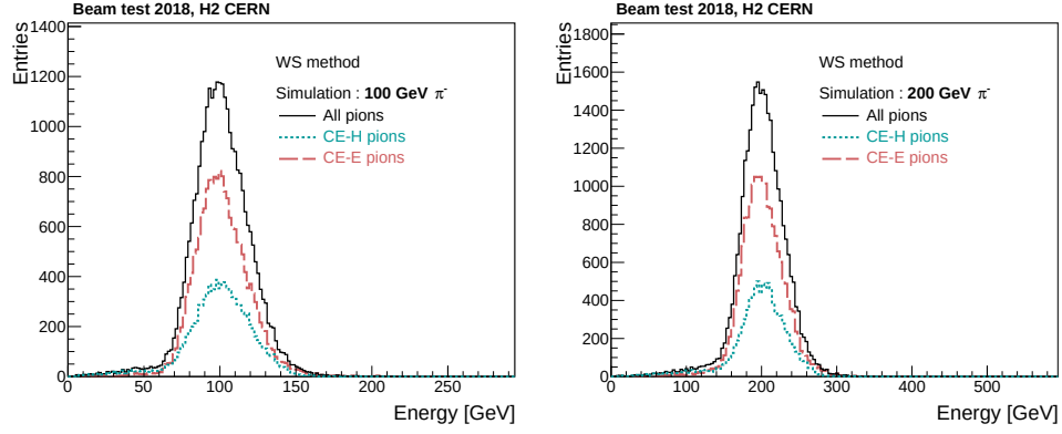
Figure 5.7: Reconstructed energy distributions for different event categories including "All events", "CE-E pions" and "CE-H pions" using WS method for simulated pions of energies 100 (left) and 200 GeV (right).
