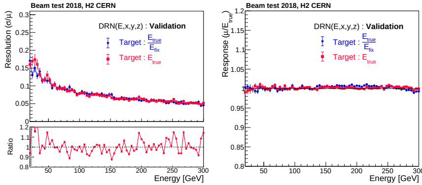
Figure 5.18: The left plot shows energy resolution, while the right plot illustrates energy response, both as functions of incident pion energy for validation datasets using DRN( E, x, y, z ) with ratio E_{true} to E_{fix} as the target, and DRN with E_{true} as the target. The bottom panel on the left displays the ratio of the latter mode to the former.
