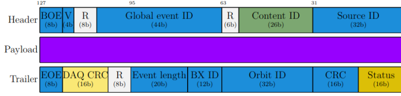
Figure 6.52: The slink packet format indicating different fields in its header and trailer [148].
