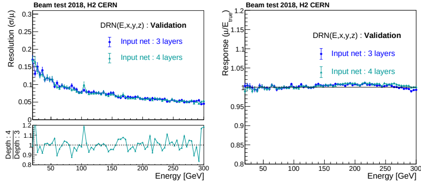
Figure 5.16: Energy resolution (left) and the energy response (right) as a function of incident pion energy obtained on validation dataset using DRNs with different number of input layers.
