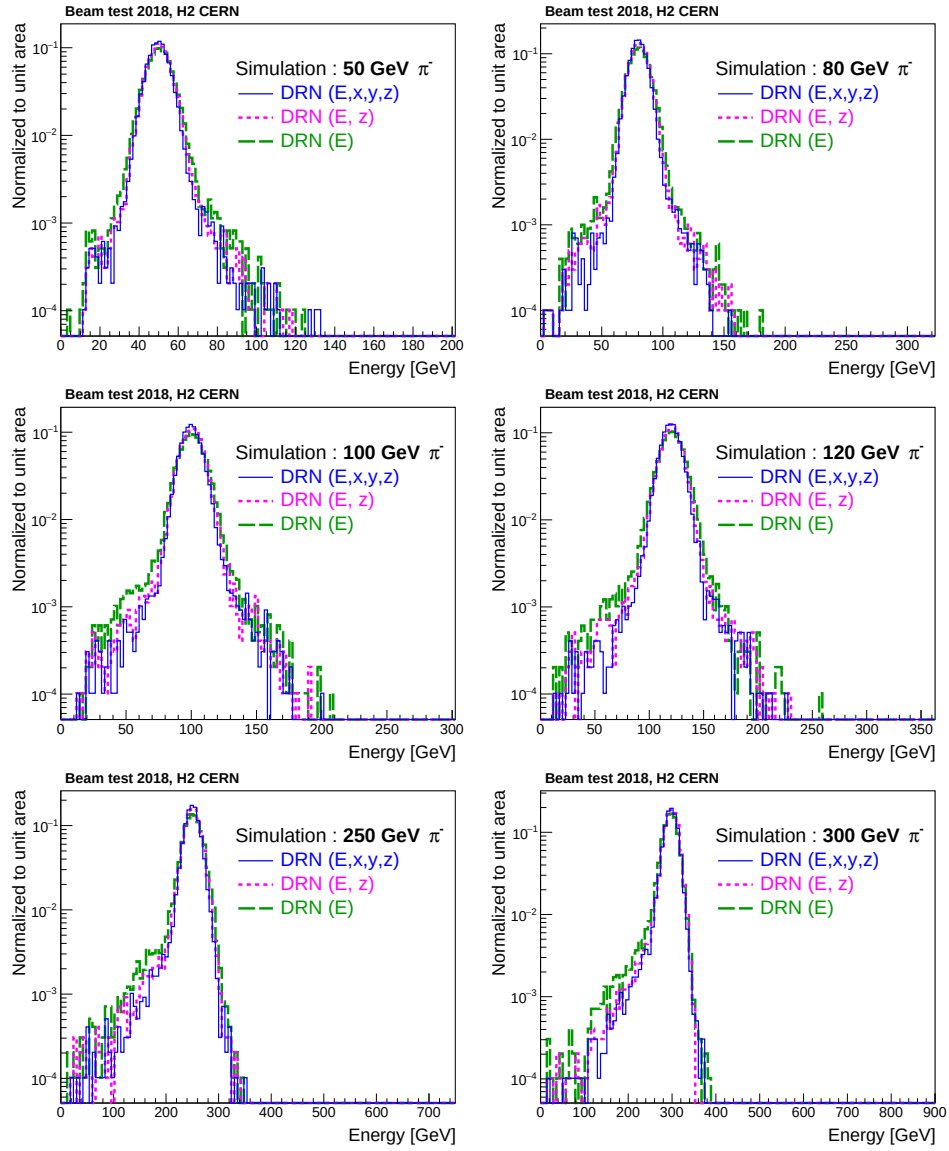
Figure A.13: Distributions of energies predicted using different DRN models for 50, 80, 100, 120, 250 and 300 GeV pions on validation datasets.
