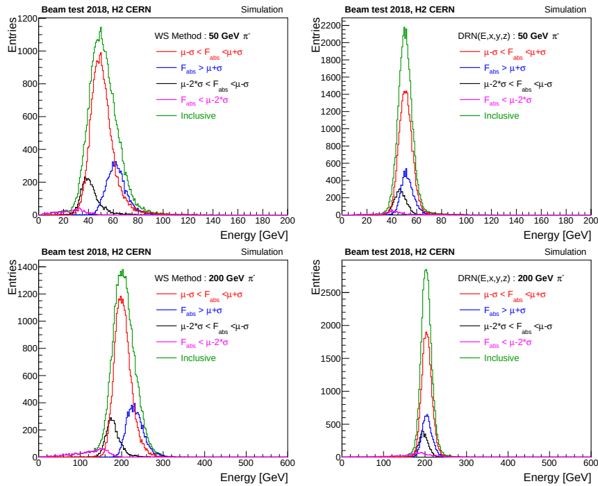
Figure 5.53: The reconstructed energy using DRN(E,x,y,z) (right) and WS method (left) is compared for different event categories defined based on F_{abs} in the above plots for 50 and 200 GeV pions. "Inclusive" line represents the energy predictions for all events.
