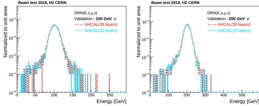
Figure 5.10: Distribution of energy reconstructed with 39 AHCAL layers and 10 AHCAL layers for incident pions of 100 GeV (left) and 200 GeV (right) in validation dataset.
