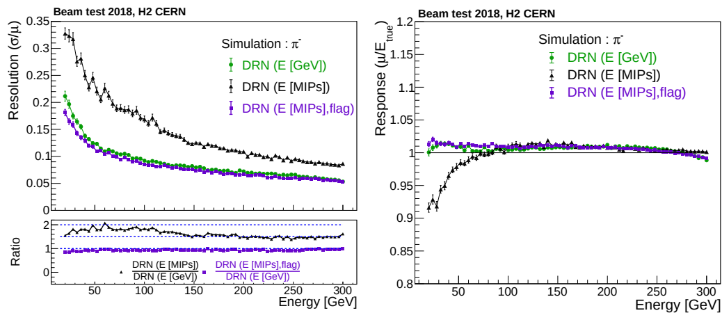
Figure 5.37: Resolution curves obtained with the models DRN(E), DRN(E[MIPs]), DRN(E[MIPs],Flag) are displayed above with validation dataset. By including a flag indicating in which subsection of the calorimeter the rehit belongs to, the resolution obtained with DRN(E) is recovered.
