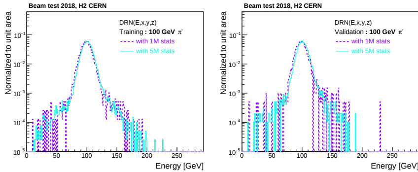
Figure 5.12: Reconstructed energy distributions for 100 GeV pions in training (left) and validation (right) dataset obtained by training the DRN with 5 M and with 1 M events.
