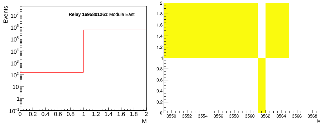
Figure 6.58: The plot shows the "M" bit from the ECON-D header, representing the agreement between HGCROC and ECON-D during the beam test. About 100 events occur at BX "3561" without agreement between ECON-D and HGCROCs.
