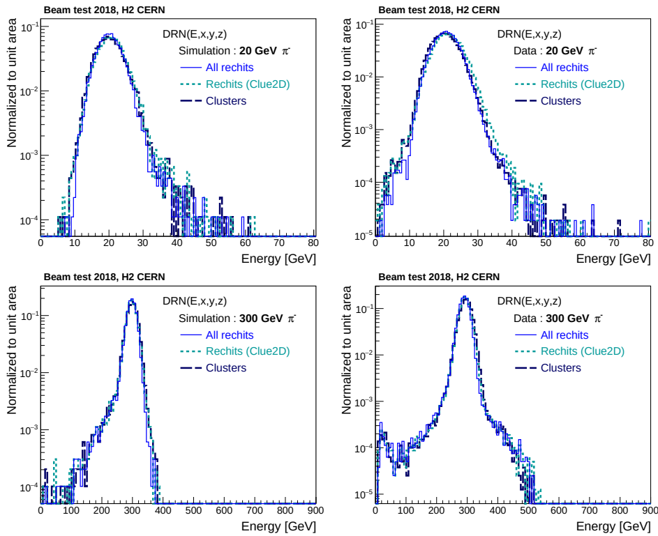
Figure 5.61: Reconstructed energy distributions using DRNs trained on clusters, rechits used to create cluster and all rechits for different energies ranging from 20 and 300 GeV are shown for simulation (left) and data (right). DRN was using four input features that is energy and x, y, z position of rechits/cluster (DRN( E,x,y,z )).
