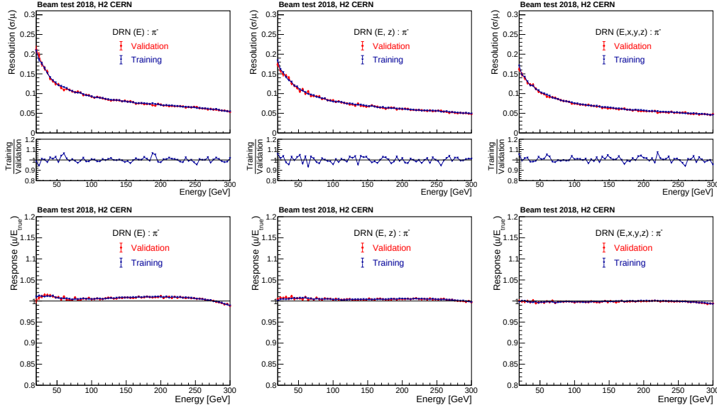
Figure 5.27: Comparison of resolution (upper row) and response (bottom row) obtained in training and validation datasets for the models DRN(E) (left), DRN(E,z) (middle), and DRN(E,x,y,z) (right) as function of incident pion energy.
