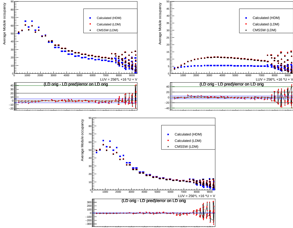
Figure 6.15: The above figure illustrates the comparison of calculated occupancies (Y-axis) for LDM with that obtained from CMSSW for total signal (top left), only noise (top right) and signal (bottom). X axis is indicating its position in luv variable as defined in equation 6.1.
