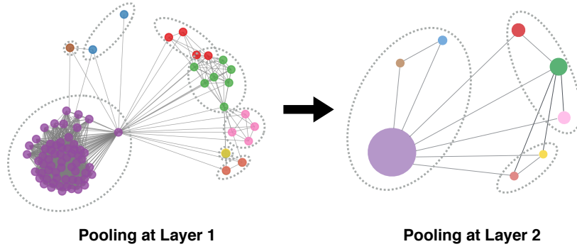
Figure 4.9: Two-layer hierarchical clustering is shown. Second-layer nodes represented by color denote first-layer clusters represented by dotted lines. [122]
