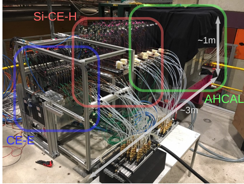
Figure 3.19: A picture of the CE-E, CE-H, and AHCAL prototypes setup mounted on a concrete platform in the H2 experimental area of the CERN SPS.
