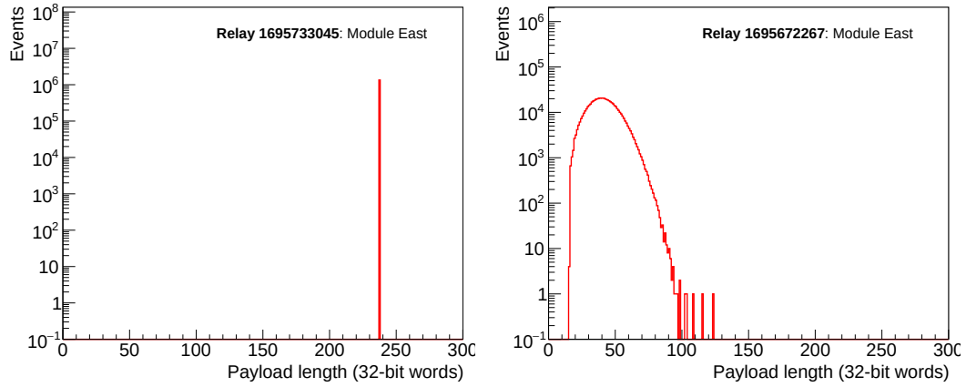
Figure 6.50: The payload length field values listed at the ECON-D header for all events recorded during a run when ECON-D is in pass through mode (left) and when in zero suppression mode (right).
