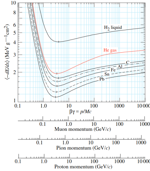
Figure 2.9: The mean energy loss ( dE/dX ) as a function of \beta\gamma in different materials. X-axis scale is represented as a function of momentum for different particles [1].
