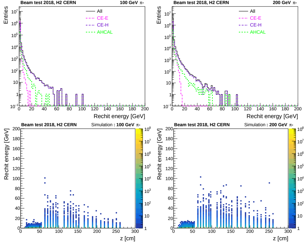
Figure 5.5: The distribution of rehit energies (top) and its distribution as a function of depth z (bottom) for 100(left) and 200(right) GeV pions. The rehit energy is represented in units of GeV which is calibrated using fixed weights.
