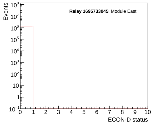
Figure 6.51: Value of ECON-D status bits field of the BE miniDAQ header for all events recorded in a run during beam test.
