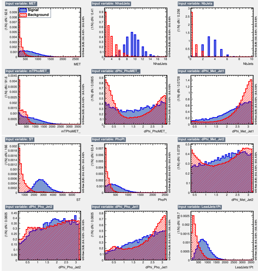
Figure 7.48: The shape comparisons of 12 out of 13 input variables for the T5ttttZG signal model (blue) against the SM background (red).
