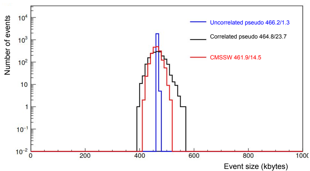
Figure 6.25: The plots display the total event size per 120^\circ after running the emulator with CMSSW events, and both uncorrelated and correlated pseudo-events. While the mean event size is consistent across datasets, the standard deviations differ.
