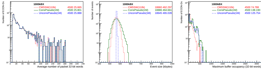
Figure 6.26: Comparison of CMSSW and pseudo events (correlated and uncorrelated); average packet size in 32-bits of words (left), total event size (middle) and maximum buffer occupancy for ECON-Ds (right).
