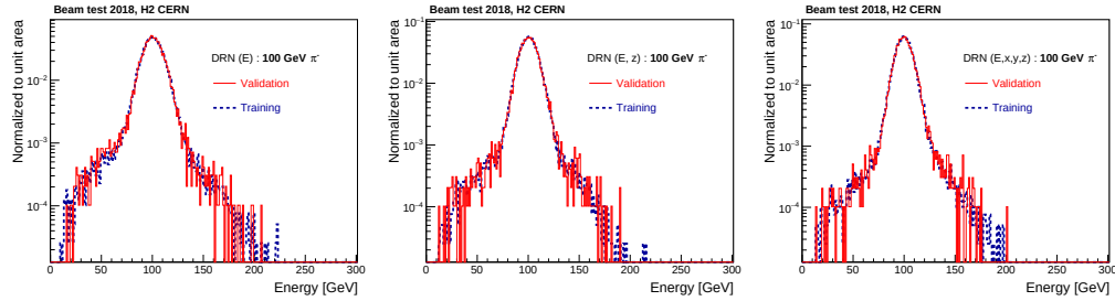
Figure 5.26: Comparison of distribution of energy obtained in training and validation datasets for the models DRN(E) (left), DRN(E,z) (middle), and DRN(E,x,y,z) (right) for pions with incident energy of 100 GeV.
