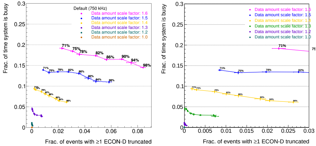
Figure 6.40: The left plot compares system deadtime from ECON-D buffer constraints with event truncation rates across different truncation threshold fractions. The right plot zooms in, emphasizing lower scaling factors. Each point represents the high water marks set at certain fraction of truncation threshold (2600 32-bit words). For each scale factor value, the high (low) water marks are varied in the range of 1850 – 2550 (1450 – 2150) 32-bit words maintaining the difference between two at 400.
