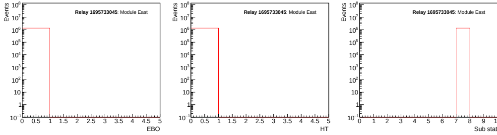
Figure 6.49: EBO field, HT field and sub stat bit field extracted from the ECON-D header for all events recorded in an electron of 100 GeV during beam test are shown.
