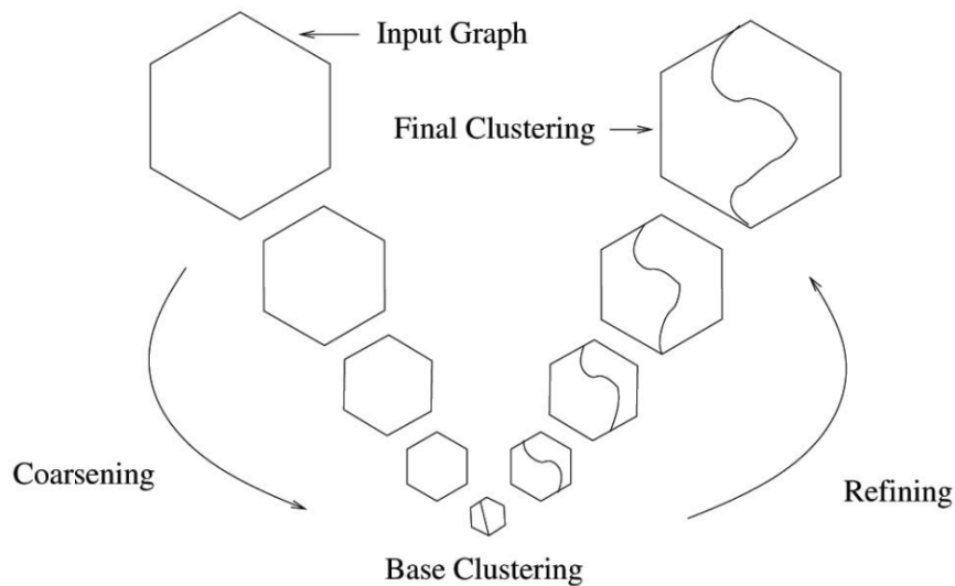
Figure 4.8: Illustration of multi-level algorithm used in graclus clustering highlighting the coarsening and refining of graph [120]. The process commences by aggregating points based on the maximum number of adjacent nodes from a top-down perspective. Conversely, during the bottom-up phase, points are segmented back, with cluster assignments determined by the "popularity" or the quantity of neighboring nodes.
