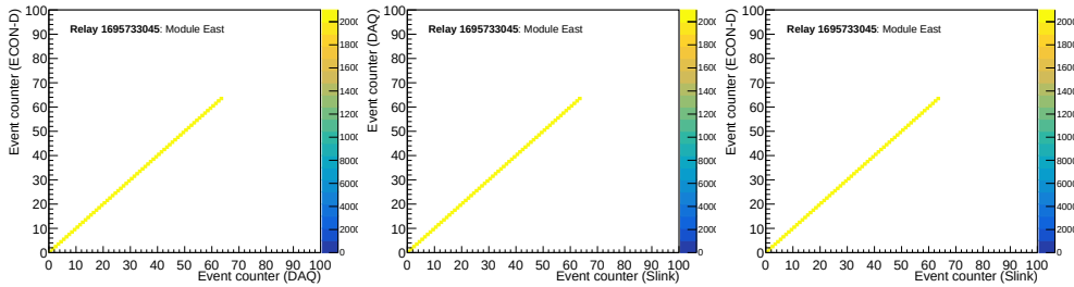
Figure 6.53: The plots compare Event counter values for ECON-D and miniDAQ (left), miniDAQ and Slink (middle), and ECON-D and Slink (right) for the east train.
