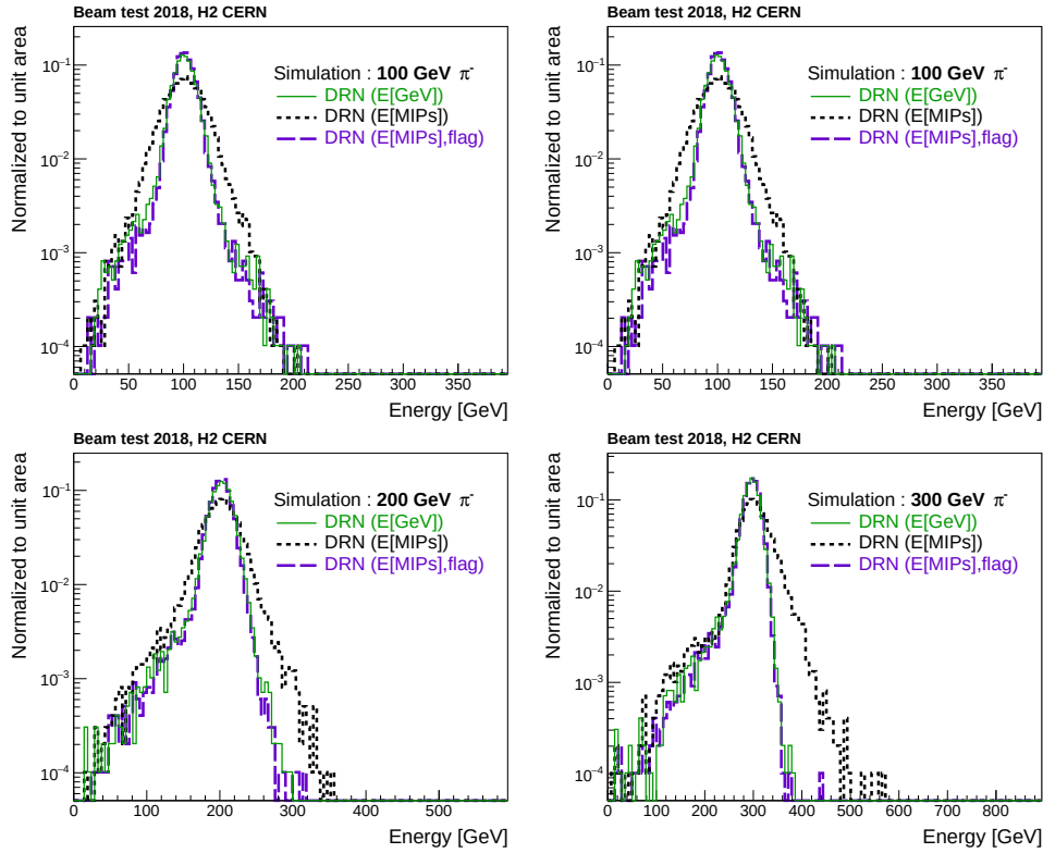
Figure 5.36: The energy reconstructed for 52, 100, 200 and 300 GeV pions using DRN(E[GeV]), DRN(E[MIPs]) and DRN(E[MIPs],flag) in simulation (validation dataset).
