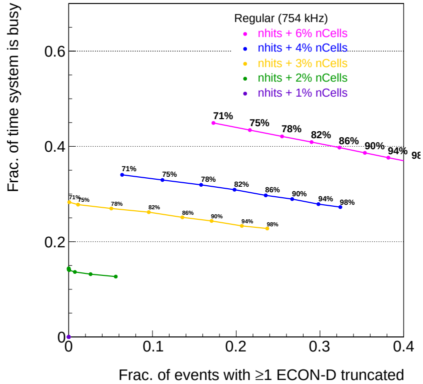
Figure 6.45: The left plot compares the system's busy time due to ECON-D buffer limits against events with at least one truncation, using different watermarks as fractions of the truncation threshold and varying nCells added across all occupancy formats.
