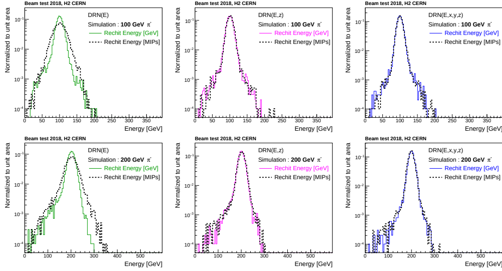
Figure 5.34: Energy distributions reconstructed with DRN(E) (left), DRN(E,z) (middle) & DRN(E,x,y,z) (right) trained on rehit energy in MIPs versus GeV at 100 and 200 GeV pions from the validation dataset.
