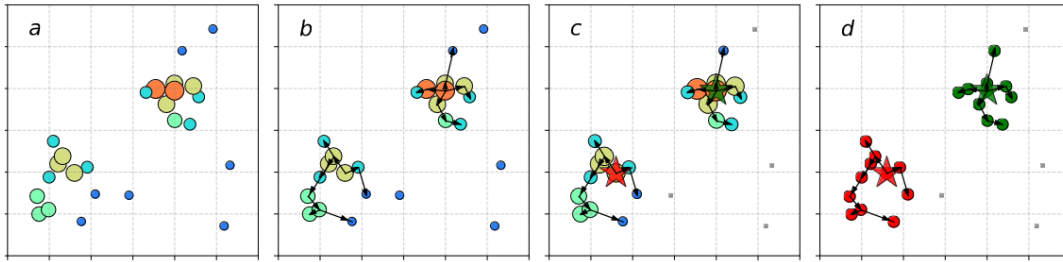
Figure 5.59: This image demonstrates the step wise process of CLUE algorithm. In step (a) local density \rho is calculated and represented by color and size of each point. In step (b), pointing arrows towards other point represents nearest higher points after calculating separation \delta . Seed and outliers are selected based on \delta and \rho in step (c) and nearest neighbor points are clustered with the seed in step (d) [131].
