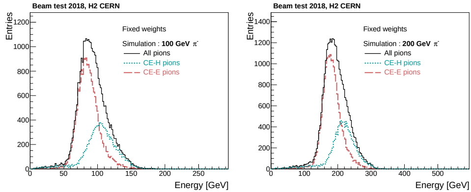
Figure 5.6: Distributions of reconstructed energies for simulated 100 GeV (left) and 200 GeV (right) pions in different event categories including "All events", "CE-E pions" and "CE-H pions" using fixed weights.
