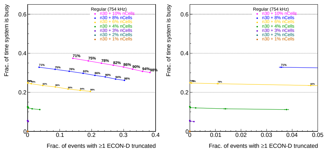
Figure 6.44: The left plot illustrates the time fraction when the system is busy due to ECON-D buffer limits and the fraction of events with ECON-D truncation across different watermarks and nCells fractions added to n30 for all modules. The right plot focuses on smaller factors with a zoomed-in view.
