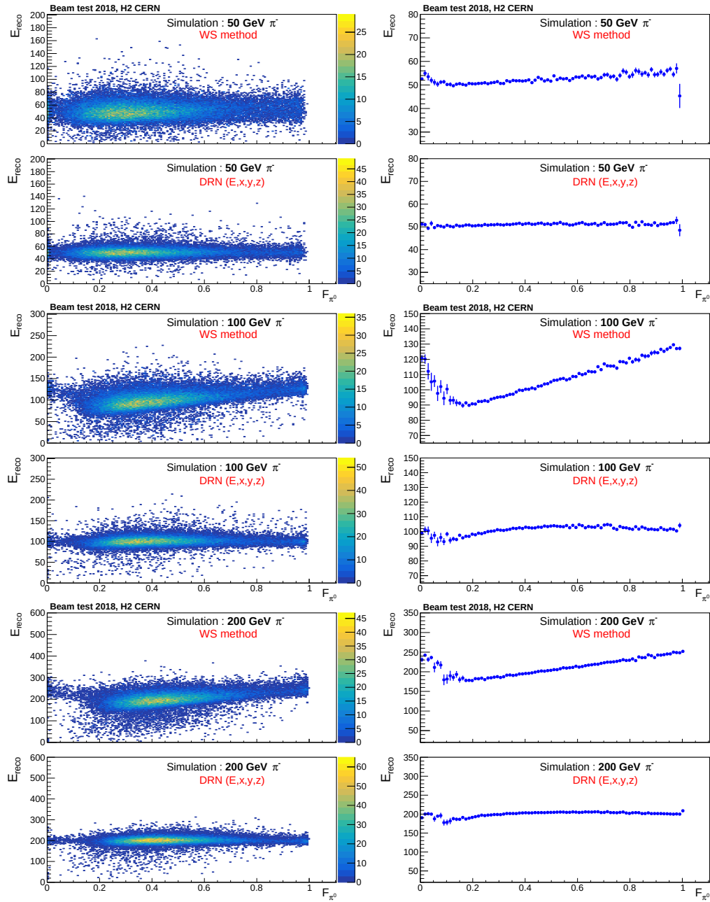
Figure 5.56: Energy reconstructed using WS method (top panel) and DRN( E,x,y,z ) model (lower panel) for pions of energy 50 GeV, 100 GeV and 200 GeV as a function of fraction of energy carried by \pi^0 s in a given shower (left). The right column shows the profile plots created after calculating the mean of reconstructed energy for different bins in F_{\pi^0} .
