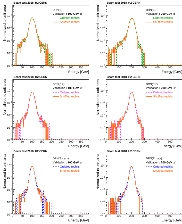
Figure A.14: The reconstructed energy distributions are compared for DRNs inferred on shuffled rechits versus inferred on ordered rechits for 100 and 200 GeV pions in validation dataset. The overall shape comes out to be identical.
