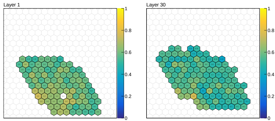
Figure 6.17: Correlations for a module ( l,u,v = 1,5,3 ) with neighboring modules in layer 1 (left) and with layer 30 (right).
