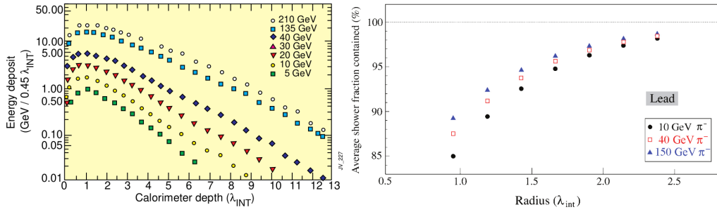
Figure 2.18: Left : Longitudinal profile of hadronic showers of different energies in Lead. Right : The average shower fraction contained in lateral as a function of \lambda_{int} , shown for different energies [45].
