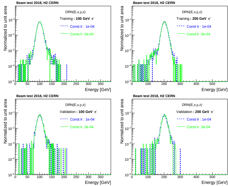
Figure A.5: Reconstructed energy distributions for 100 and 200 GeV pions using different constant learning rates when training DRNs are shown. The plots display results for training (top row) and validation (bottom row) datasets.
