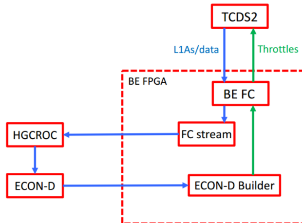
Figure 6.38: Above schematic shows how L1As and throttling signal travels through the readout system.
