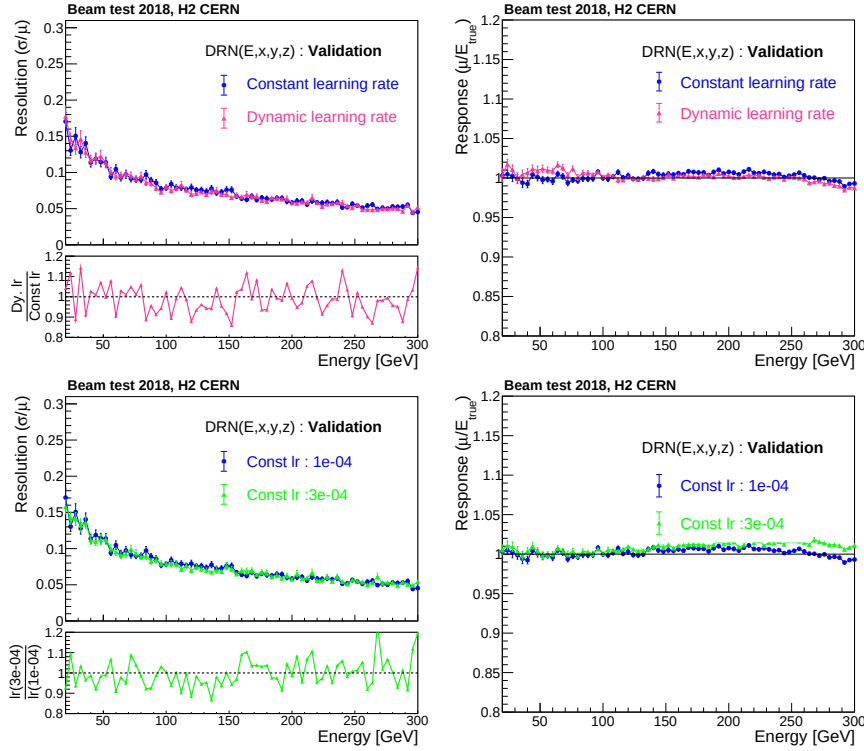
Figure 5.17: Energy resolution (left) and energy response (right) versus incident pion energy for DRNs trained with a constant versus dynamic learning rate (top row) and 3 \cdot 10^{-4} vs 10^{-4} constant learning rates (bottom row) for validation datasets. The bottom left panel compares the resolution ratio of dynamic to constant and 3 \cdot 10^{-4} vs 10^{-4} learning rate.
