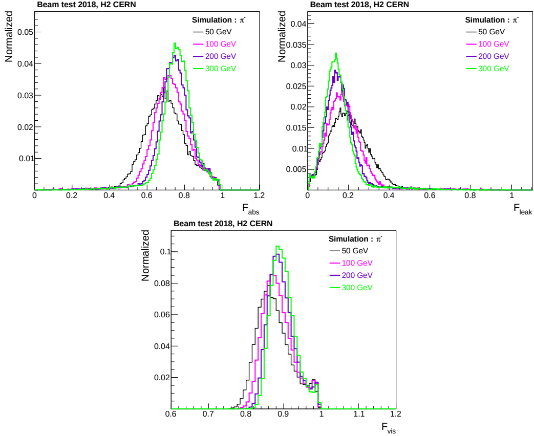
Figure 5.48: F_{abs} , F_{leak} and F_{vis} for incident pion energies of (50, 100, 200, 300) GeV. These are calculated as per the equations 5.14, 5.15 and 5.16 respectively with the help of additional truth information added in the simulation.
