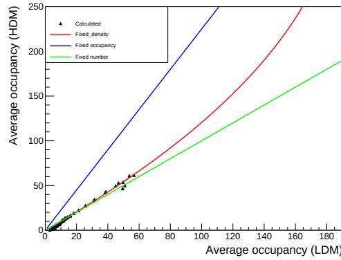
Figure 6.16: The transformation of occupancies from LDM to HDM predicted by different analytic approaches and obtained using the fits is shown.
