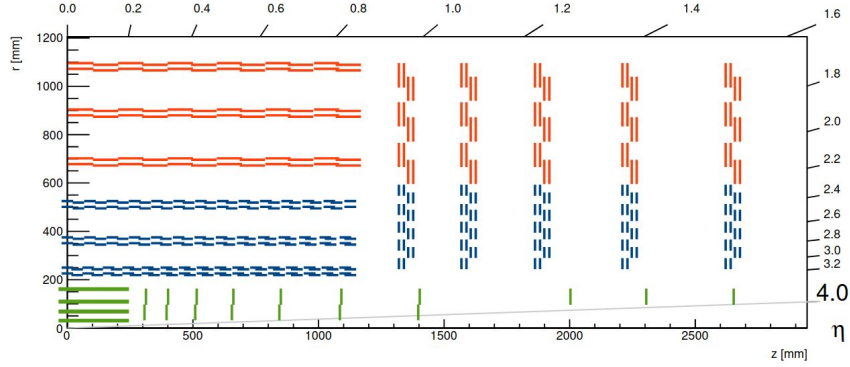
Figure 3.8: Illustration of a quarter section of the Tracker. Blue and red lines represent the Outer Tracker, with blue for PS modules and red for 2S modules (see text for details). The green highlights the Inner Pixel detector and its forward extension [82].
