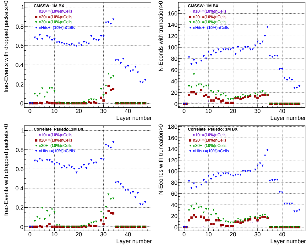
Figure 6.35: The Y-axis shows the fraction of events with dropped packets (left) and average truncated ECON-Ds per event (right). The X-axis represents layer numbers with 10% of n_{Cells} added to n_{10} , n_{20} , n_{30} , and n_{hits} for these layers, using CMSSW (top) and pseudo-events (bottom).
