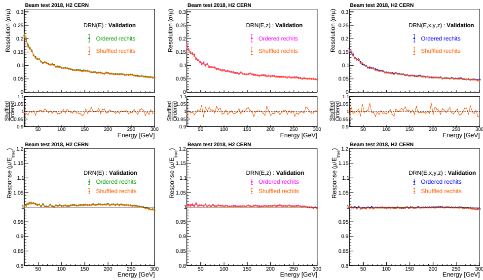
Figure 5.31: Energy resolution (top) and the energy response (bottom) obtained with inferring DRNs on shuffled order of rechits are compared with the DRNs inferred on ordered rechits. The bottom panel shows the ratio of resolutions obtained with inferring on shuffled rechits to that with ordered rechits.
