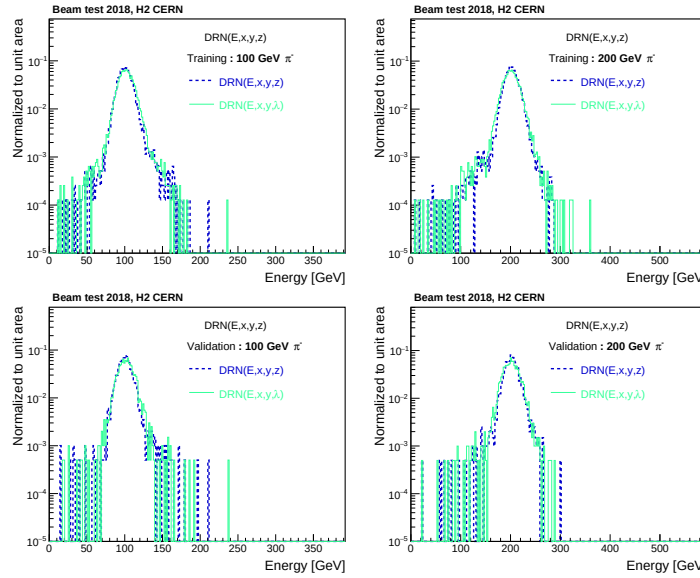
Figure A.8: Reconstructed energy distributions for 100 and 200 GeV pions obtained for training (top) and validation (bottom) datasets with DRN(E,x,y,z) and DRN(E,x,y,λ int ) are shown.
