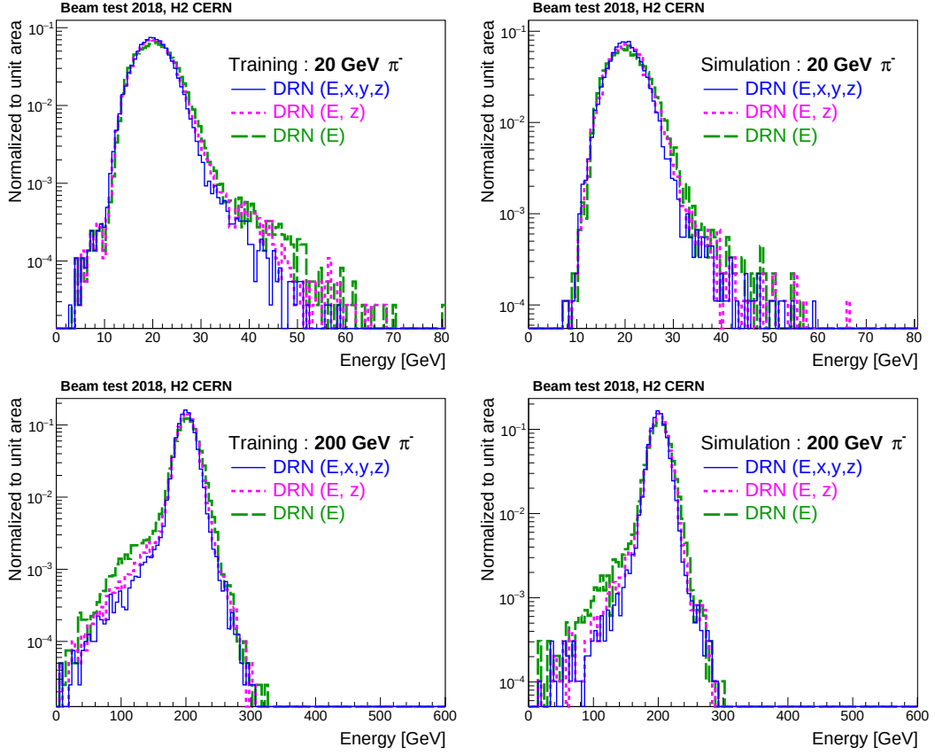
Figure 5.29: Distributions of energies predicted using different DRN models for 20 GeV (up) (middle) and 200 GeV (lower) pions on training (left) & validation referred as "Simulation" (right) datasets.
