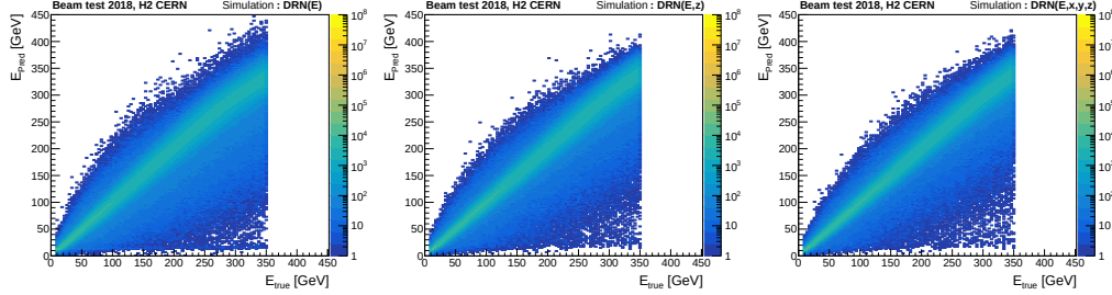
Figure 5.24: The event-by-event comparison of the true pion energy versus the reconstructed using different DRNs evaluated at the best epochs for \text{DRN}(E) , \text{DRN}(E,z) and \text{DRN}(E,x,y,z) from left to right respectively.
