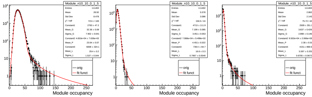
Figure 6.21: The occupancy distributions for different modules along with the different parameters obtained after fitting it as per equation 6.21 are shown.
