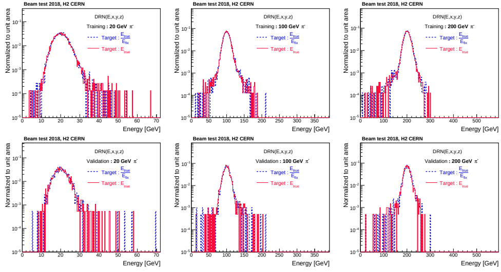
Figure A.6: The reconstructed energy distributions for 20, 100 and 200 GeV pions obtained for training (upper row) and validation (bottom row) datasets with DRN(E,x,y,z) but with different targets used are shown.
