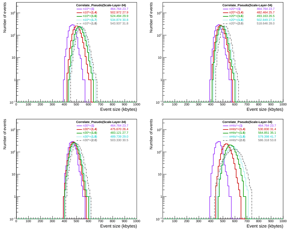
Figure 6.29: The average event size obtained after scaling only n10 (top left), n20 (top right), n30 hits (bottom left), and all three at once (bottom right). The emulator was run using pseudo events and different scaling factor.
