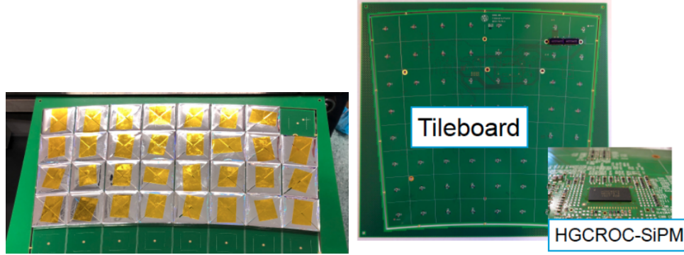
Figure 3.14: This image is showing the tileboards to be used in scintillator sections [97].
