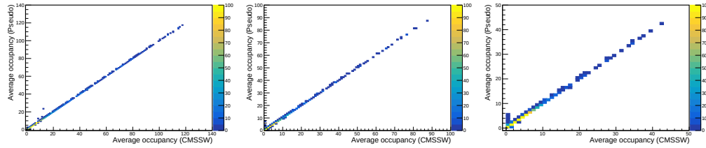
Figure 6.23: The comparison of the average occupancy obtained from pseudo events (Y axis) and CMSSW (X axis) for n10 , n20 , n30 formats shown from left to right, respectively.
