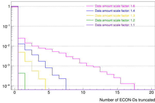
Figure 6.41: Distributions of ECON-Ds truncating per event for varying scaled data across all occupancy formats (nhits) and modules. High and low watermarks are 2550 and 2150.
