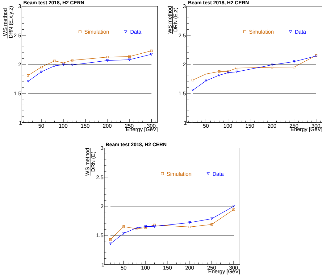
Figure 5.43: The ratio of energy resolutions obtained using different DRNs compared to the WS method in both simulation and data is shown. We observed a twofold improvement in energy resolution when using DRN(E,x,y,z) for pion energy reconstruction.
