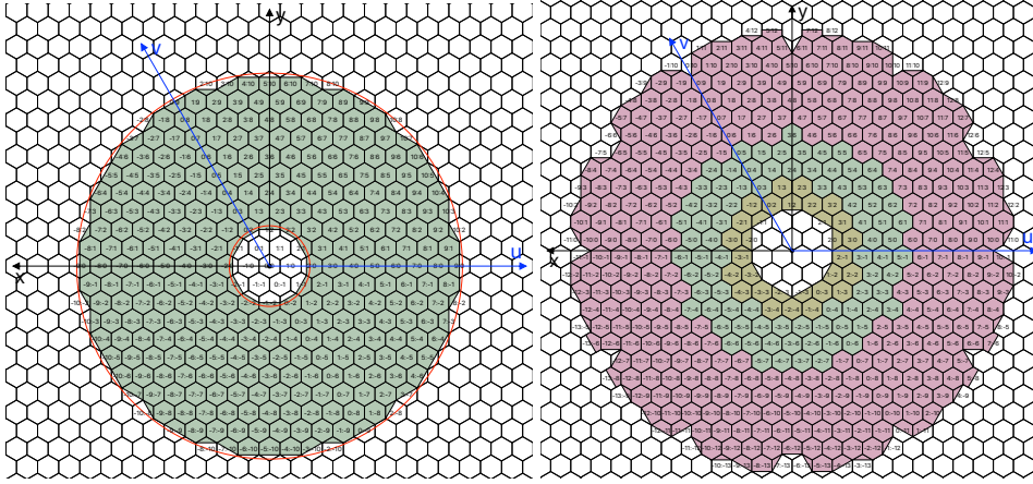
Figure 3.16: The above figure illustrates the (u,v) coordinate systems as well as highlighting the three sectors per endcap in HGCAL layer-1 and layer-35.
