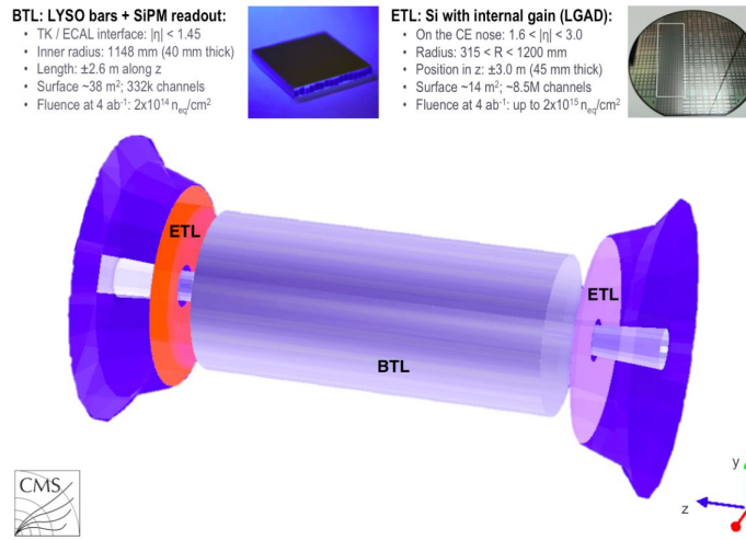
Figure 3.9: GEANT4 simulated schematic representation of Mip Timing Detector (MTD). The setup includes a barrel layer (grey cylinder) at the tracker-ECAL junction and two silicon timing layers (orange and light violet discs) before the endcap calorimeter. [84].
