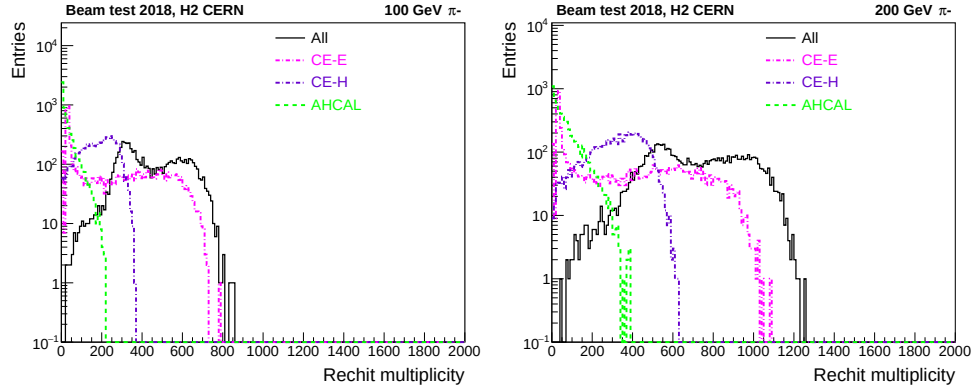
Figure 5.2: Distribution of number of rechits across different detector sections of beam test setup, as well as the total number of rechits across all three sections (denoted as "All") or 100 and 200 GeV incident pion energy.
