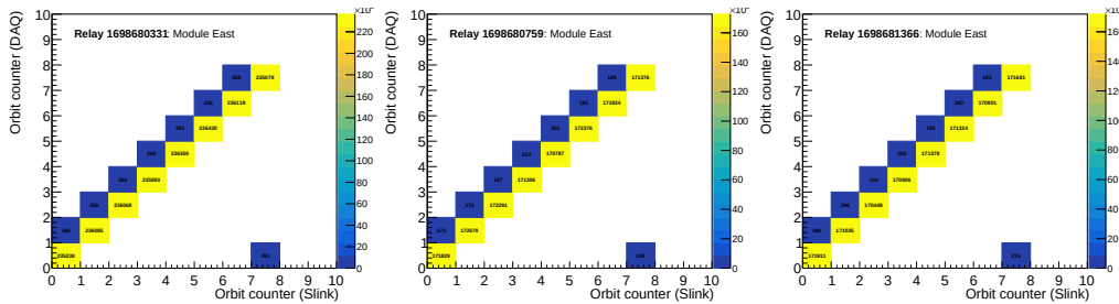
Figure 6.62: The plots compare Orbit counter values for miniDAQ and Slink for the east trains across three different relays recorded with updated firmware after taking the Orbit counters out of reset, and re-initialising the system in between.
