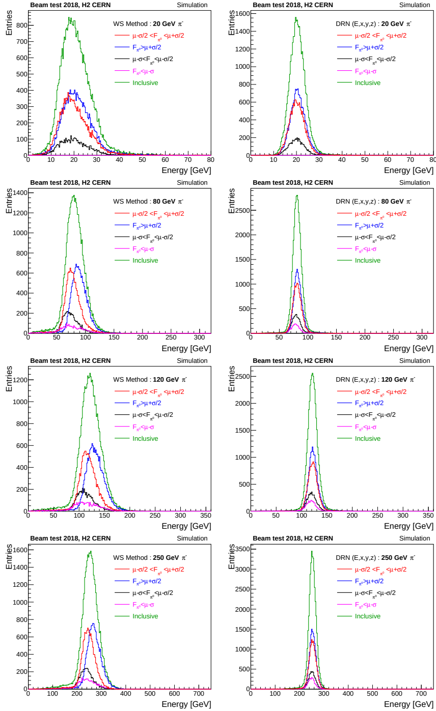
Figure A.19: This figure illustrates performance of DRN and WS method in terms of reconstructing the energy for different events falling into different categories for 20, 80, 120 and 250 GeV pions.
