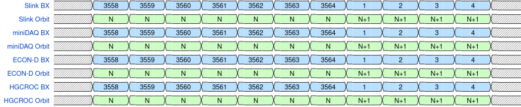
Figure 6.54: The above wave diagram shows BX and Orbit counters represented by N , in sync for Slink, miniDAQ, ECON-D and HGCROC in ideal scenarios.
