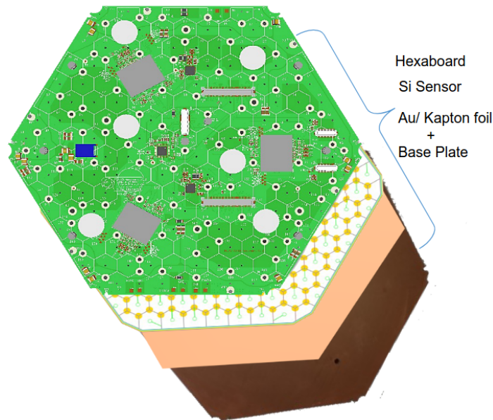
Figure 3.13: This image is showing the different components stacked to make a silicon module [96].
