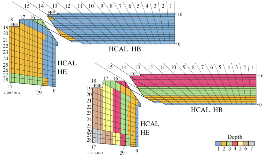
Figure 3.5: HCAL segmentation in Phase-0 (upper section) and Phase-1 (lower section) configuration [80].
