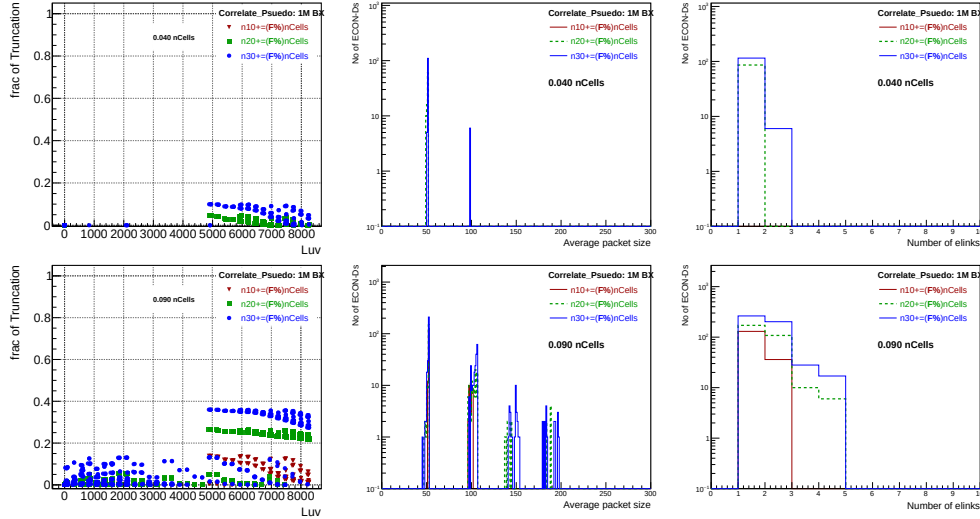
Figure 6.34: The ECON-Ds featuring non-zero truncation, represented by their respective luvs (left), mean packet size (center), and associated count of active elinks (right), are illustrated for a fraction F of 4% (top row) and 9 % (bottom row) of nCells, respectively.
