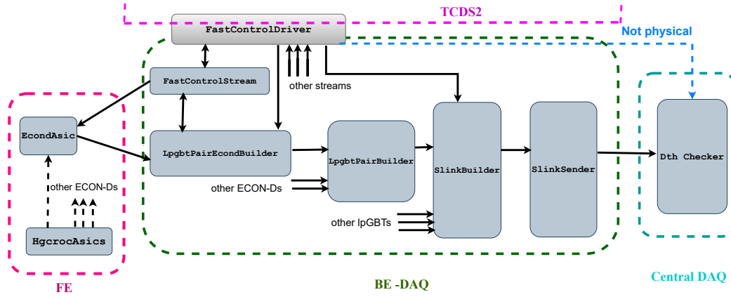
Figure 6.12: Schematic illustrating the different entities of the HGCAL buffer model emulator.
