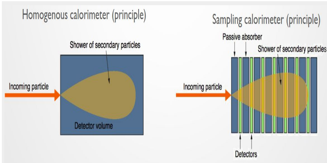
Figure 2.21: Illustration of basic principle behind the homogeneous (left) and sampling calorimeters (right) [50].
