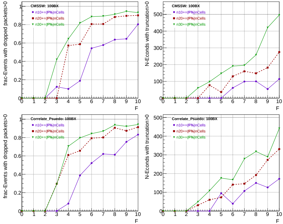
Figure 6.33: The fraction of events with at least one dropped packet or incomplete event (left column) and the average number of ECON-Ds showing truncation per event (right column) are displayed above when F\% (X-axis) of nCells have been added individually at a time, to n10 , n20 and n30 obtained from CMSSW (top row) and pseudo events (bottom row).
