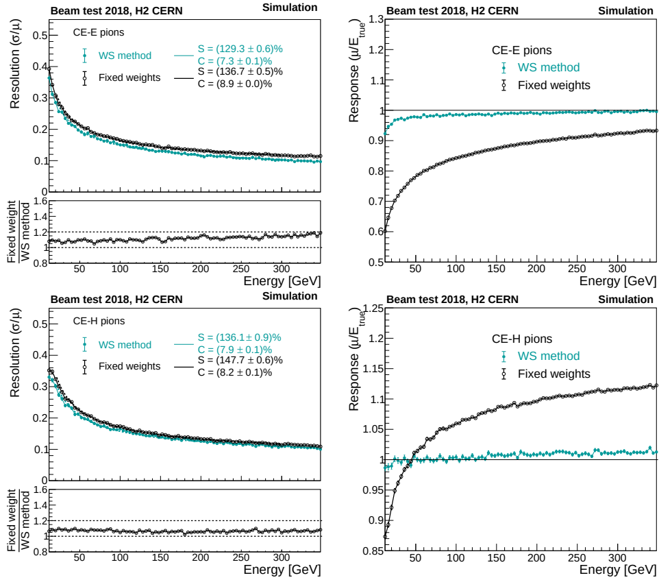
Figure 5.8: The energy resolution (left) and response (right) for CE-E pions (top) and CE-H pions (bottom) using fixed weights and WS method as functions of pion energy.
