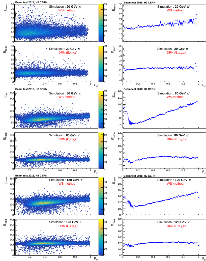
Figure A.17: Energy reconstructed using WS method (top panel) and DRN(E,x,y,z) model (lower panel) for pions of energy 20, 80 and 120 GeV (in the left column) as a function of fraction of energy carried by \pi^0 s in a given shower is shown. The right column shows the profile plots created after calculating the mean of reconstructed energy for different bins in F_{\pi^0} .
