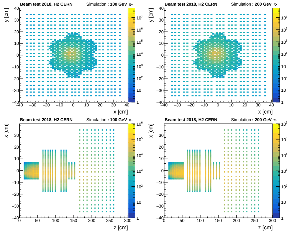
Figure 5.3: Distribution of x vs y coordinates of rechits (top row) and x vs z coordinates of rechits of 100 GeV (left) and 200 GeV (right) pions. Here, Z -axis represents the frequency of events.
