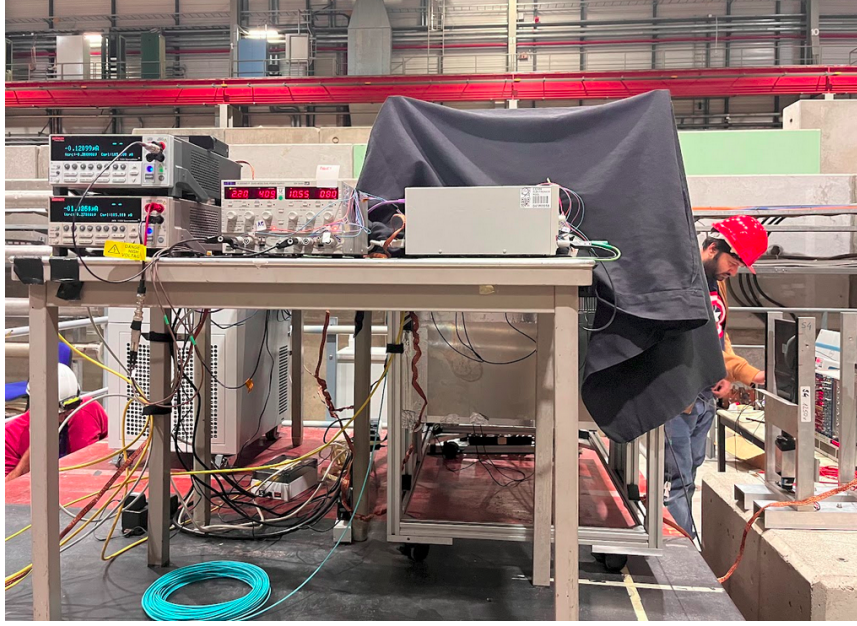
Figure 6.48: Picture of the HGCal beam test setup at H4 beamline facility of SPS.
