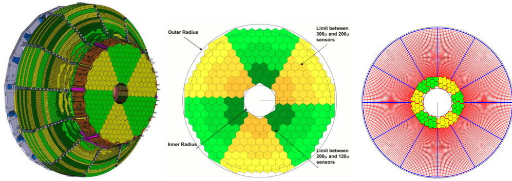
Figure 3.12: The above is showing the image of 3D view of 1 HGCal endcap (left most), a sampling layer of CE-E (middle) and that for CE-H (right most) [94].
