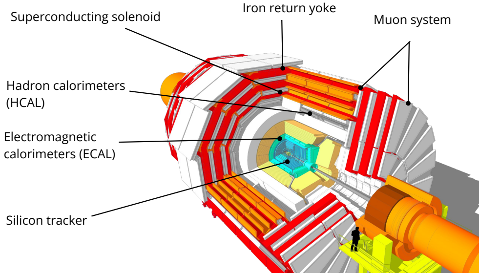
Figure 3.3: Schematic view of CMS detector highlighting different subsystems [69].
