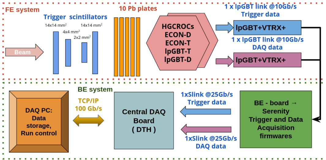
Figure 6.47: Schematic of setup used for September 2023 beam test with HGCal readout chain.
