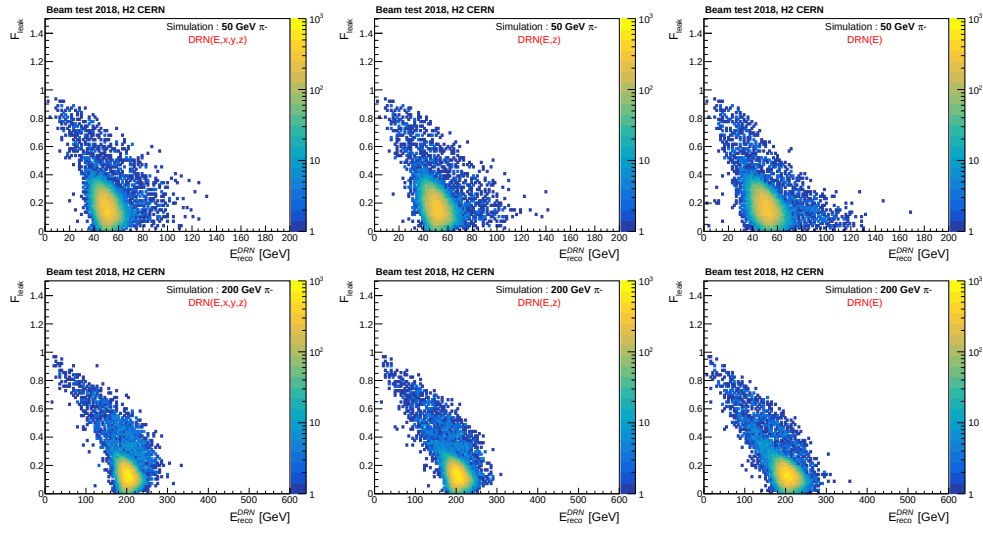
Figure 5.52: Reconstructed energy as a function of F_{\text{leak}} for DRN(E,x,y,z), DRN(E,z) and DRN(E) from left to right, respectively, for 50 and 200 GeV pions. DRN(E) struggles with energy prediction for high F_{\text{leak}} due to lack of spatial data in contrast to DRN(E,x,y,z) and DRN(E,z) utilizing spatial information.
