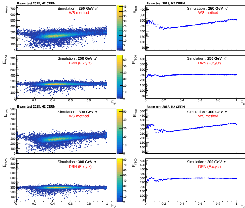
Figure A.18: Energy reconstructed using WS method (top panel) and DRN(E,x,y,z) model (lower panel) for pions of energy 250 and 300 GeV (in the left column) as a function of fraction of energy carried by \pi^0 s in a given shower is shown. The right column shows the profile plots created after calculating the mean of reconstructed energy for different bins in F_{\pi^0} .
