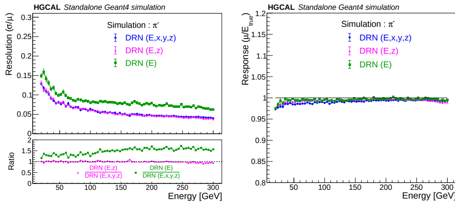
Figure 5.65: Resolution (left) and response (right) predicted by DRN(E), DRN(E,z) and DRN(E x y z) in the full HGCal setup for simulated validation dataset.
