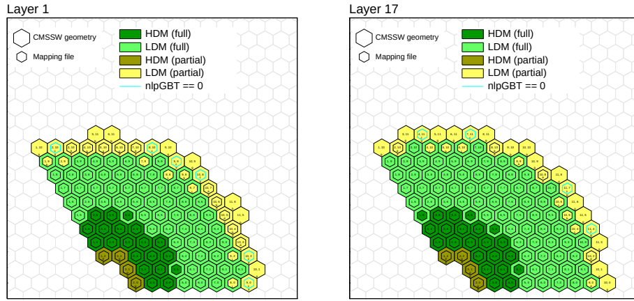
Figure 6.13: Comparison of module types and locations in CMSSW reference (larger hexagons) and a baseline updated (smaller hexagons) HGCal geometries. The number in the hexagons are the (u,v) coordinates for that module.
