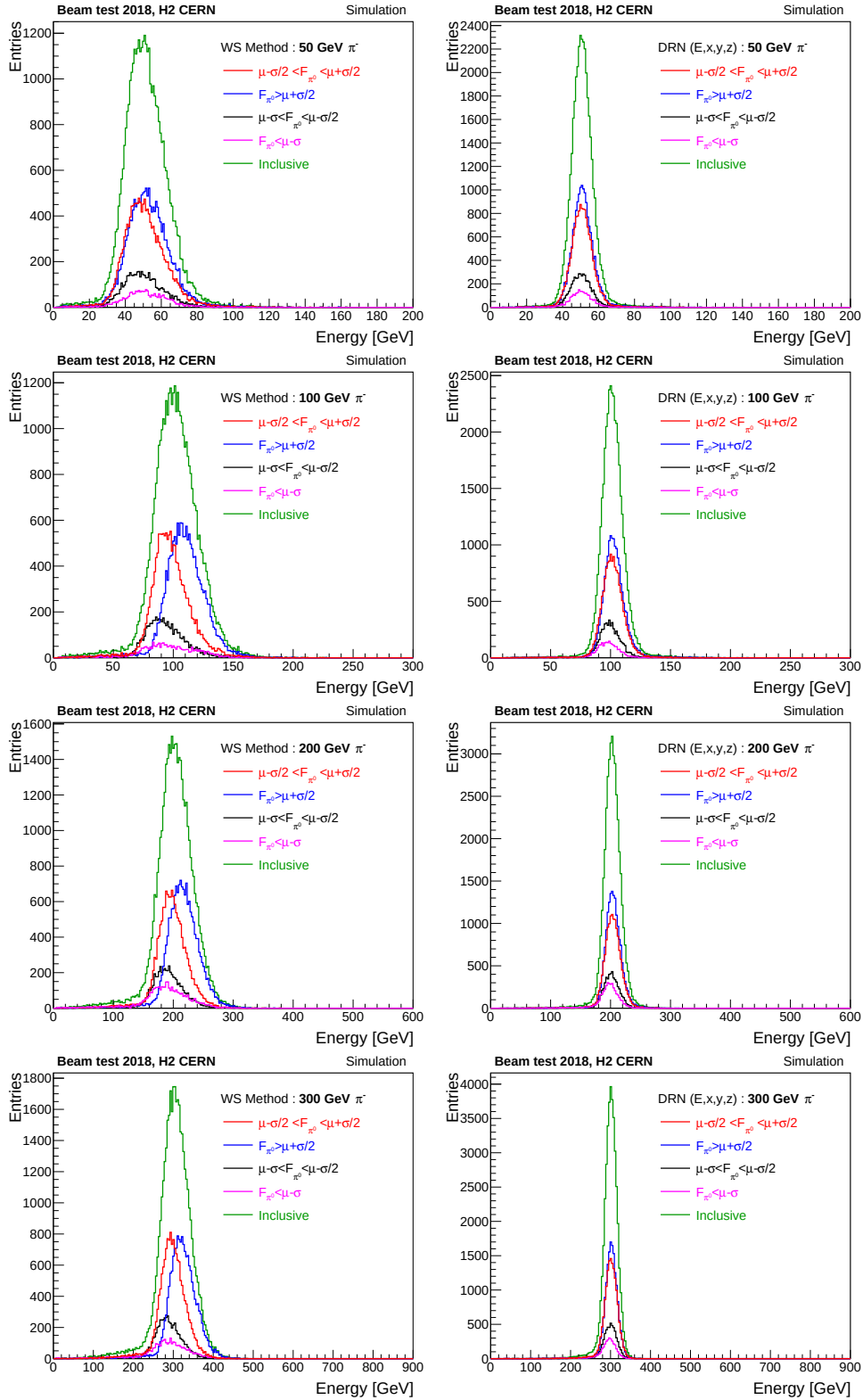
Figure 5.57: This figure illustrates performance of DRN and WS method in terms of reconstructing the energy for different events falling into different categories for 50, 100, 200 and 300 GeV pions. "Inclusive" line represents the energy predictions for all events.
