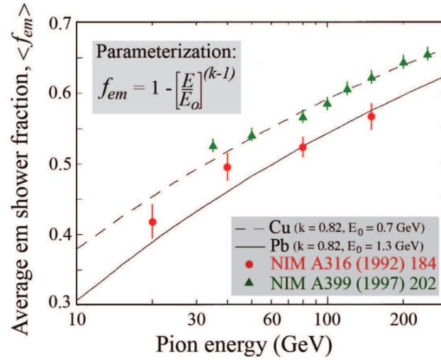
Figure 2.17: The variation of f_{em} with respect to the energy of hadrons in hadronic showers [45].
