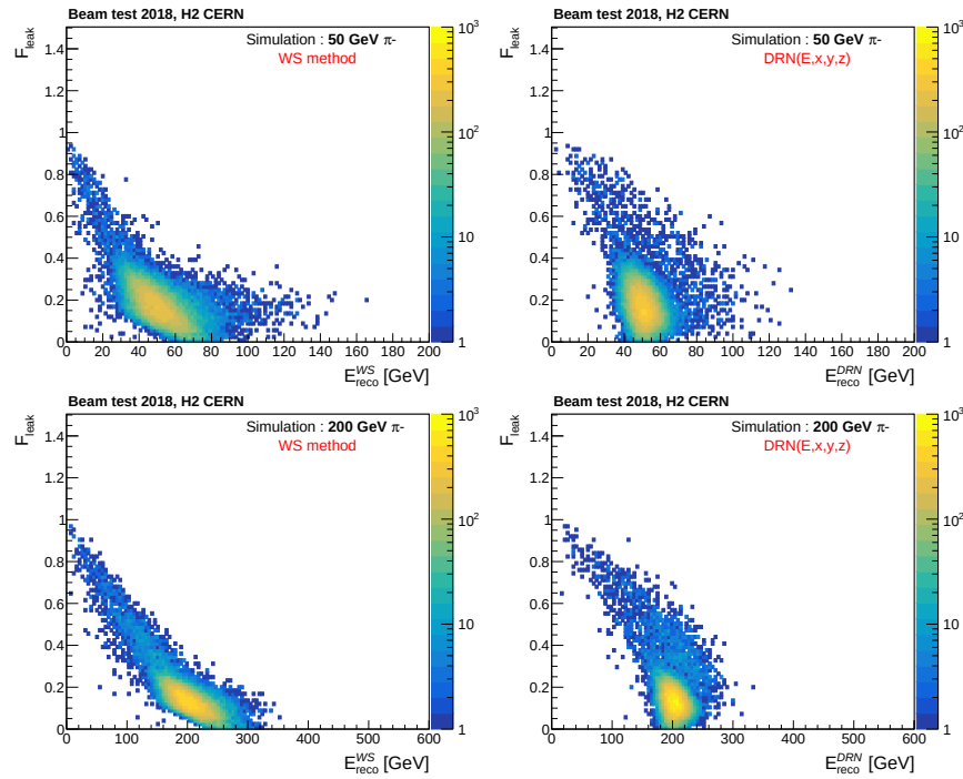
Figure 5.51: Reconstructed energy using WS method (left) and DRN( E,x,y,z ) (right), as a function of F_{leak} for 50 and 200 GeV pions. As F_{leak} increases, using WS method results in E_{reco} that reduces, and diverges from the true incident pion energy. Conversely, the bulk of E_{reco} distribution with DRN remains stable relative to F_{leak} .
