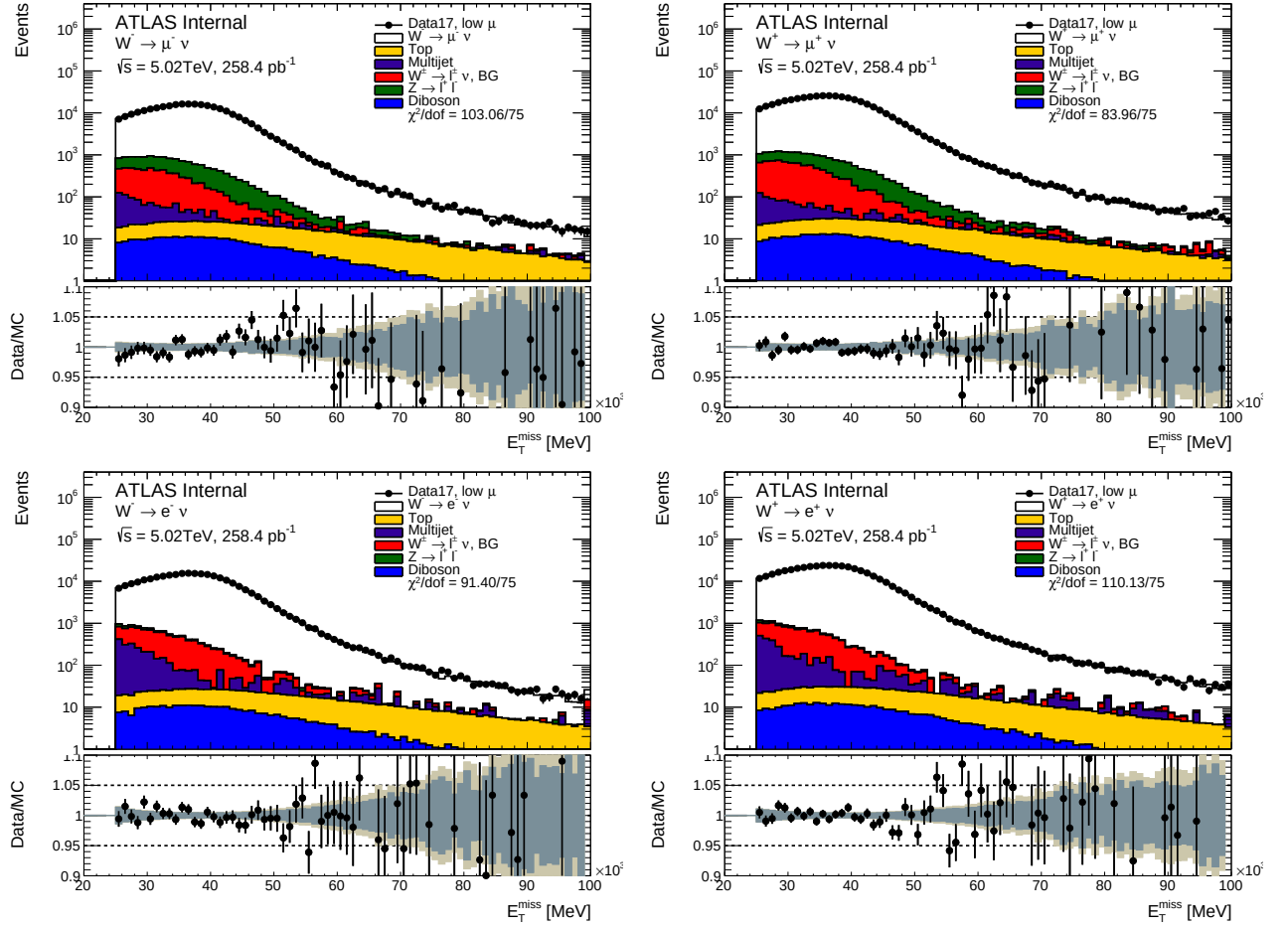
Figure 8.20: \vec{E}_T^{\text{miss}} distribution in the muon and electron channel for the \sqrt{s} = 5 \text{ TeV} dataset.
