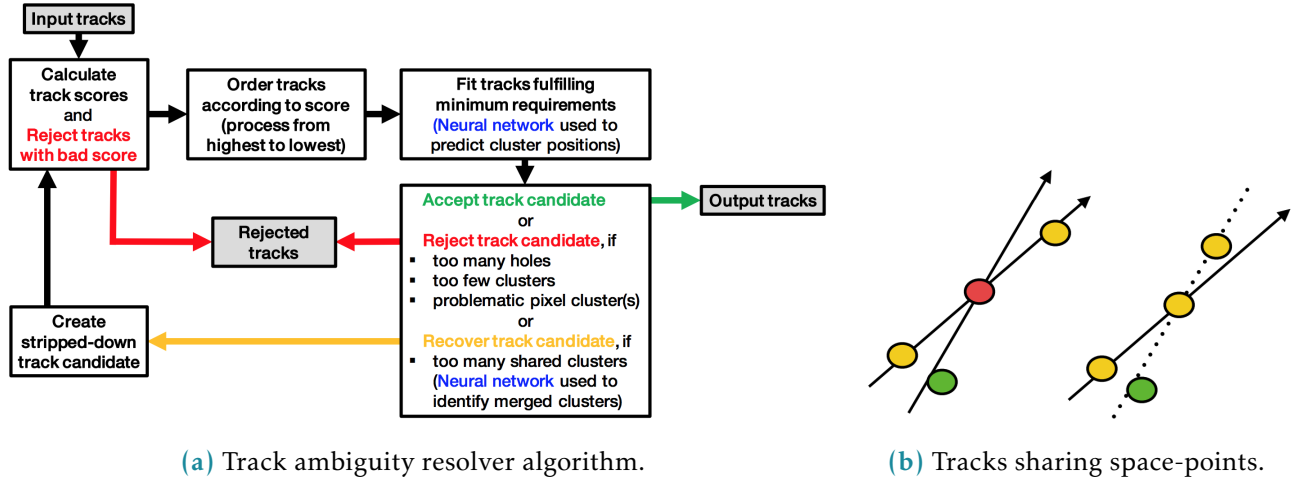
Figure 6.2: Ambiguity solving process [117].
