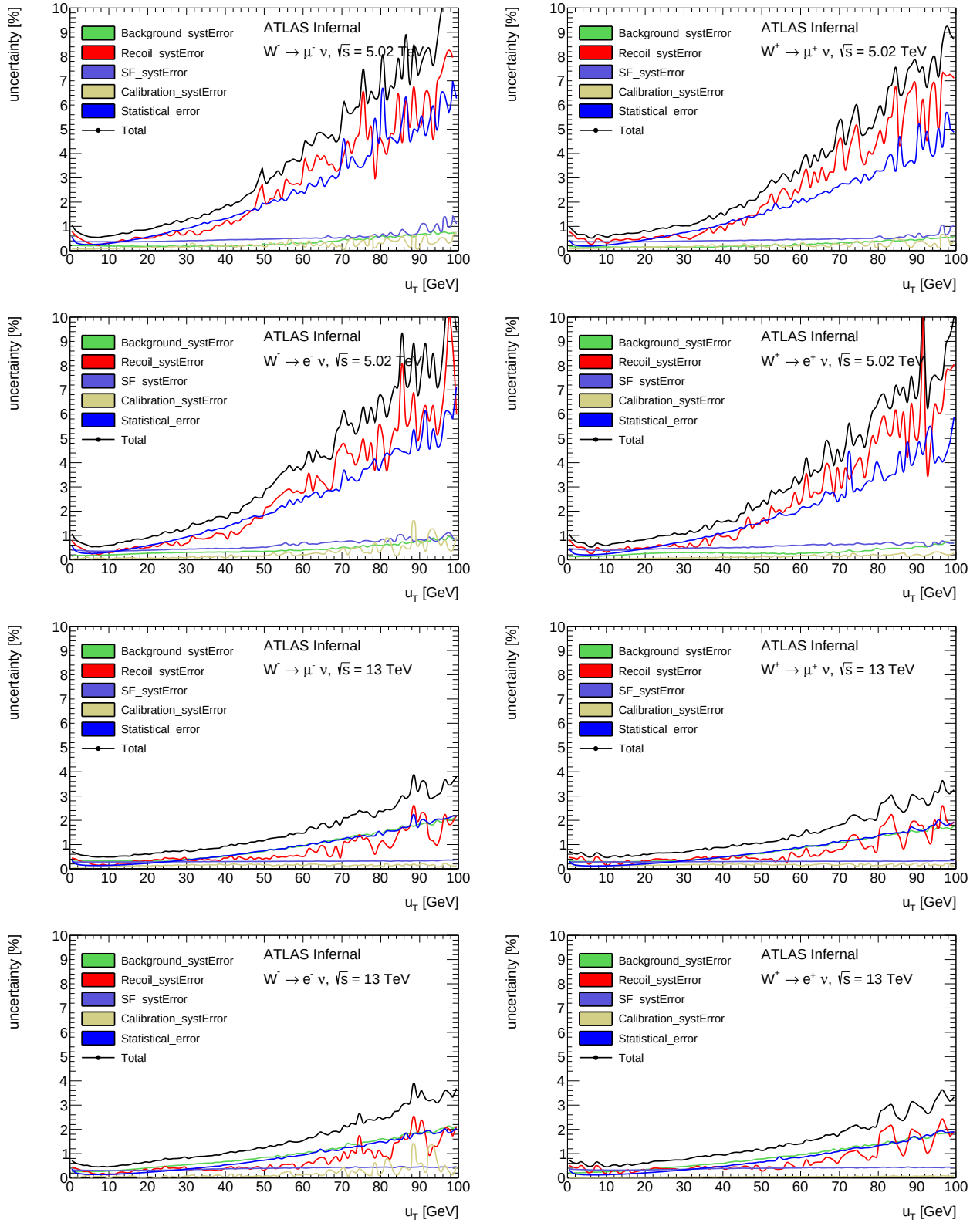
Figure 10.22: W transverse momentum systematic error breakdown in the muon and electron channel for the \sqrt{s} = 5 TeV and \sqrt{s} = 13 TeV datasets.
