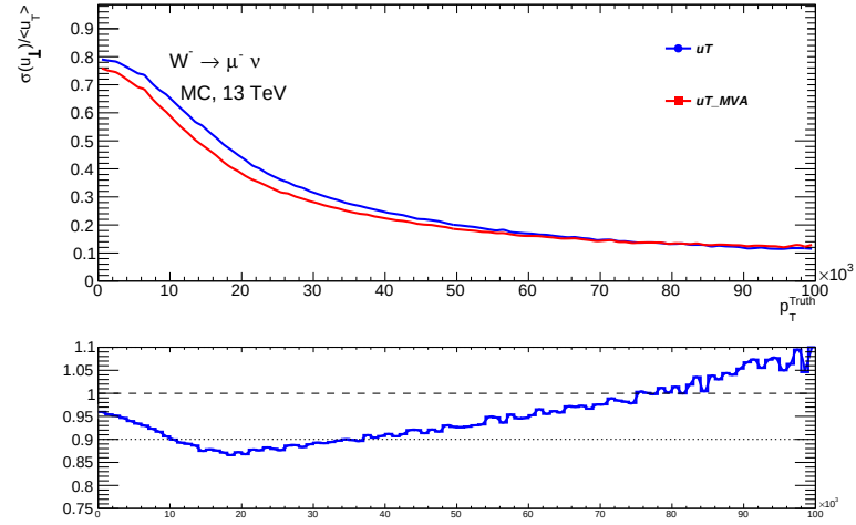
Figure 10.9: Normalized \frac{u_{\perp}}{\langle u_T \rangle} as a function of p_T^{truth} .
