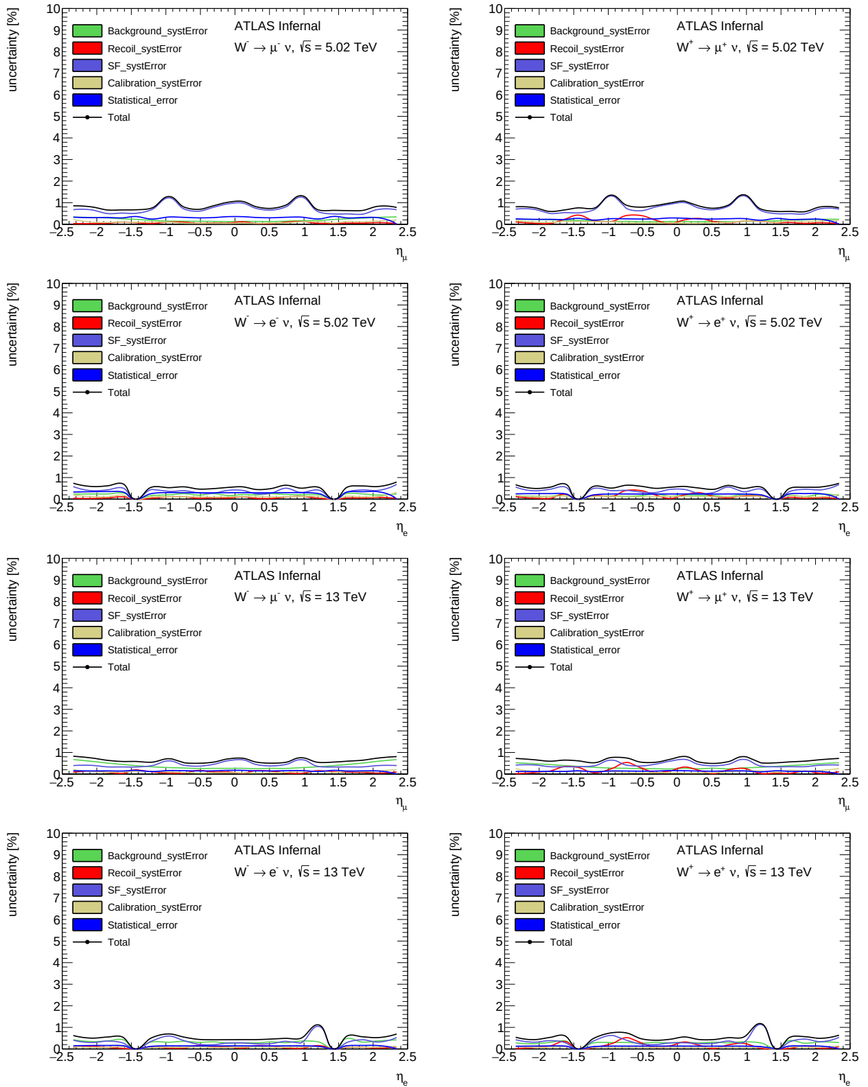
Figure 10.20: Lepton pseudorapidity systematic error breakdown in the muon and electron channel for the \sqrt{s} = 5 TeV and \sqrt{s} = 13 TeV datasets.
