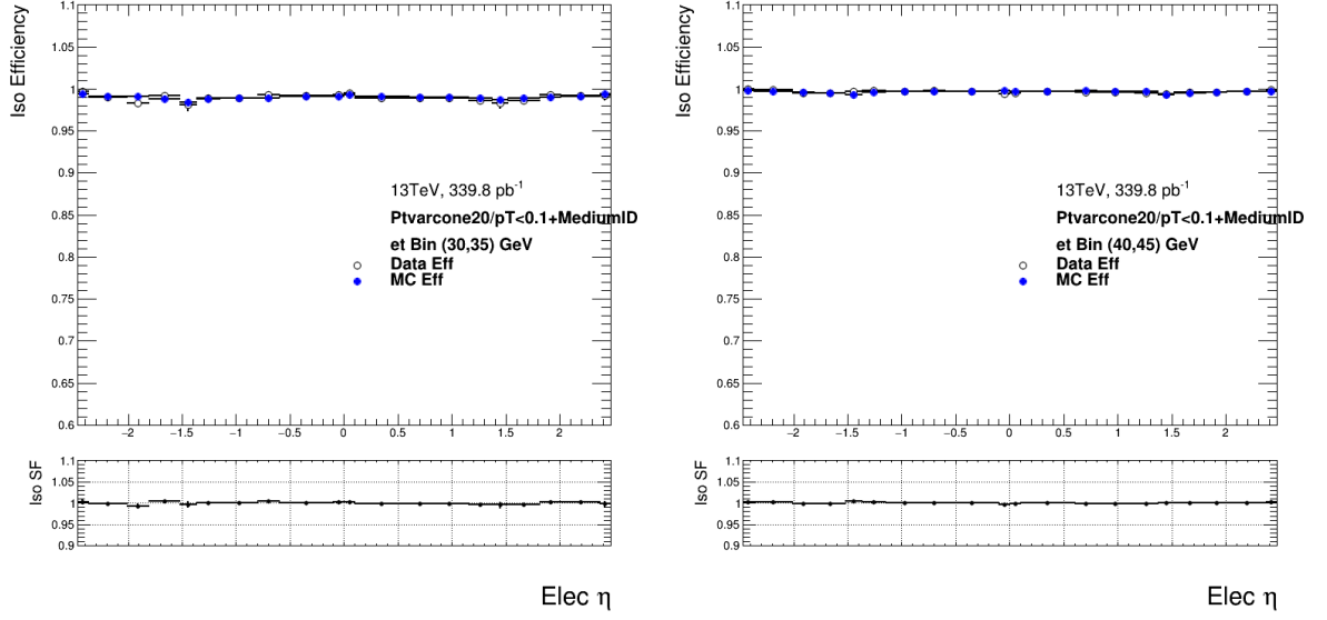
Figure 7.10: Electron isolation efficiencies (top panels) and scale factors (lower panels) for the pt-varcone20/p_T^e < 0.1 working point using 13 TeV 339 pb -1 low-pileup data as function of \eta in bins of p_T [138].
