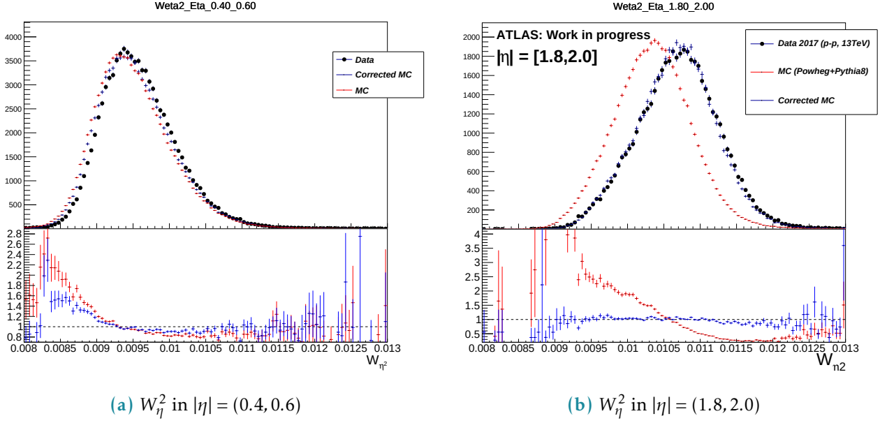
Figure 5.13: W_\eta^2 in the barrel and in the end-cap, Data, MC, reweighted MC
