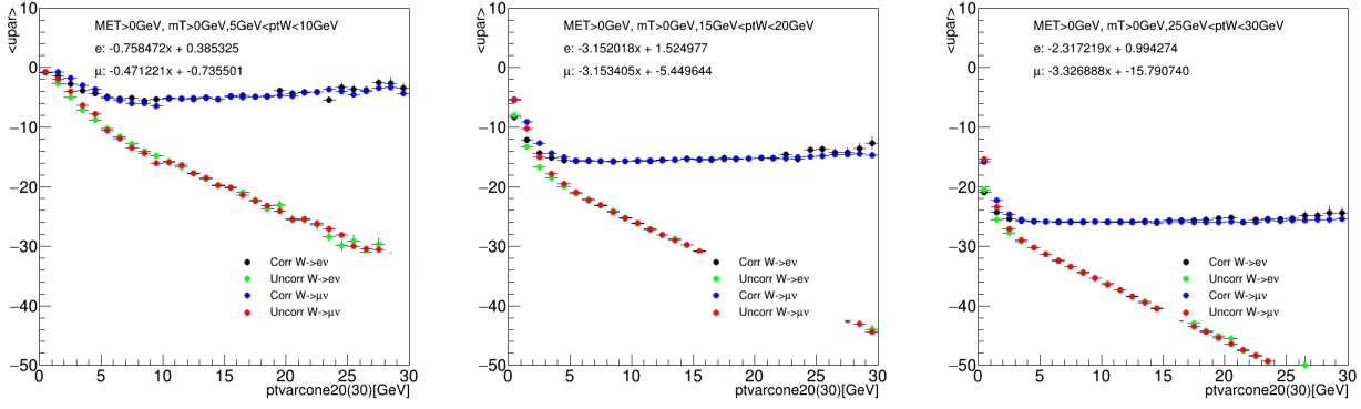
Figure 8.3: \langle u_{\perp}^{\ell} \rangle as a function of pt_{cone20} , before and after correction using data samples at \sqrt{s} = 13 TeV.
