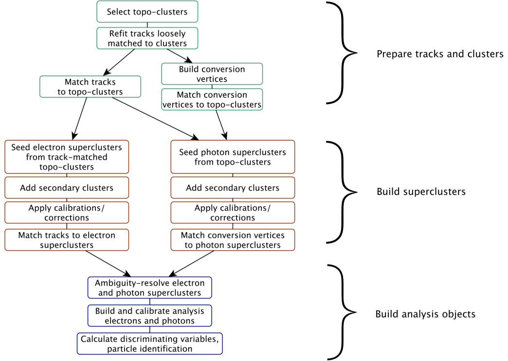
Figure 6.7: The algorithm scheme for topocluster reconstruction.
