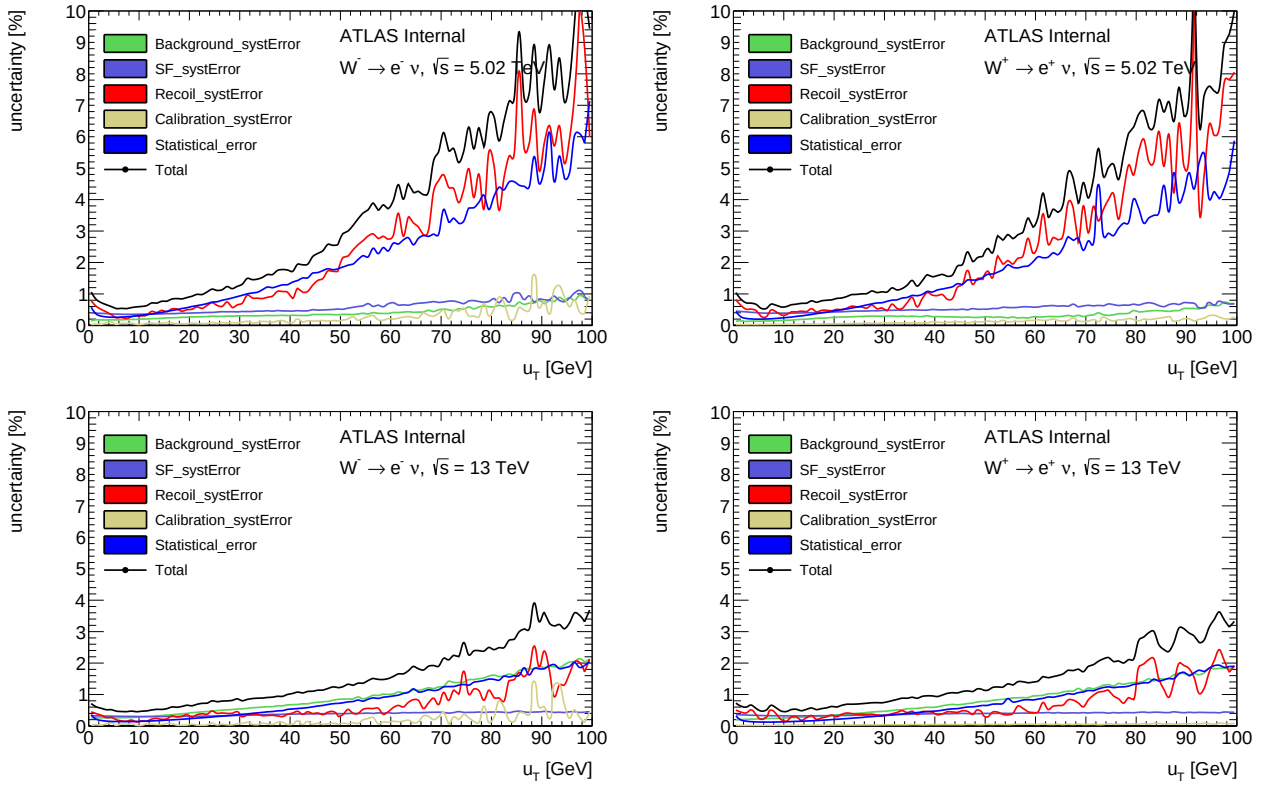
Figure 9.11: Breakdown of systematic uncertainties for 5 (a,b) and 13 (c,d) TeV in the electron channel at the reconstructed level.
