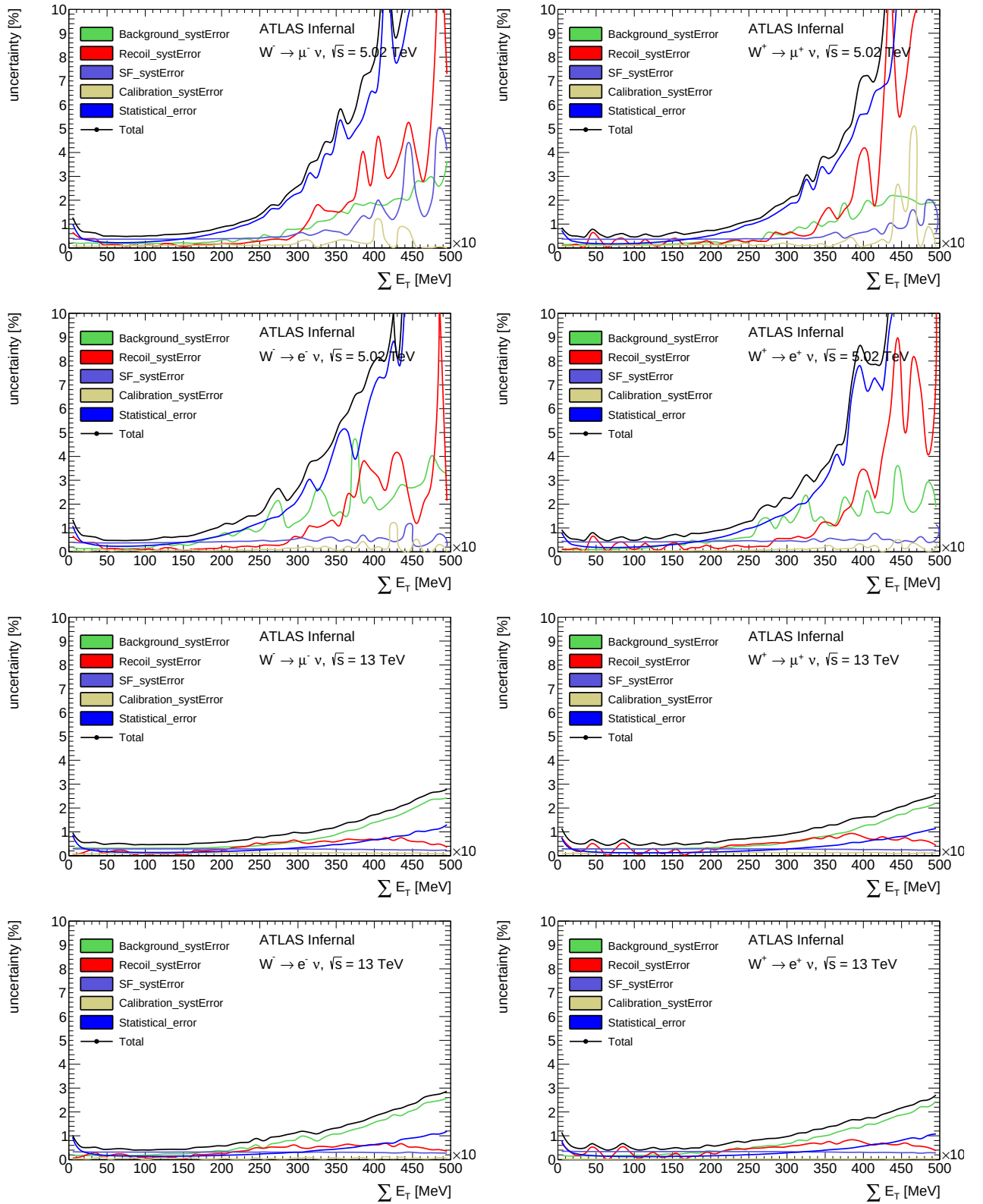
Figure 10.17: \sum E_T systematic error breakdown in the muon and electron channel for the \sqrt{s} = 5 TeV and \sqrt{s} = 13 TeV datasets.
