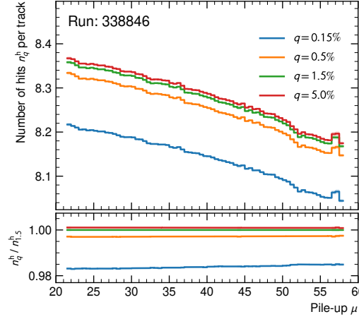
Figure 4.6.: The number of hits per track for different noise thresholds q for run 338846 as a function of the number of pile-up interactions. The shaded bands indicate the statistical uncertainty.
