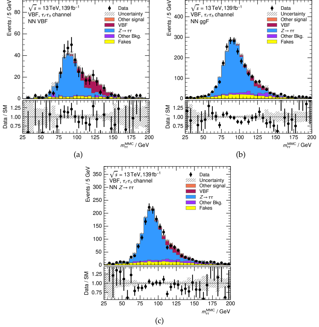
Figure B.7.: Exclusive VBF signal region categories as defined by the NN output for the \tau_{lep}\tau_{had} channel. By definition, the categories are designed to increase the fraction of events from VBF (a), ggF (b), and Z \rightarrow \tau\tau processes (c). The hatched band and the error bars indicate statistical uncertainties of the background expectation and measured data, respectively.
