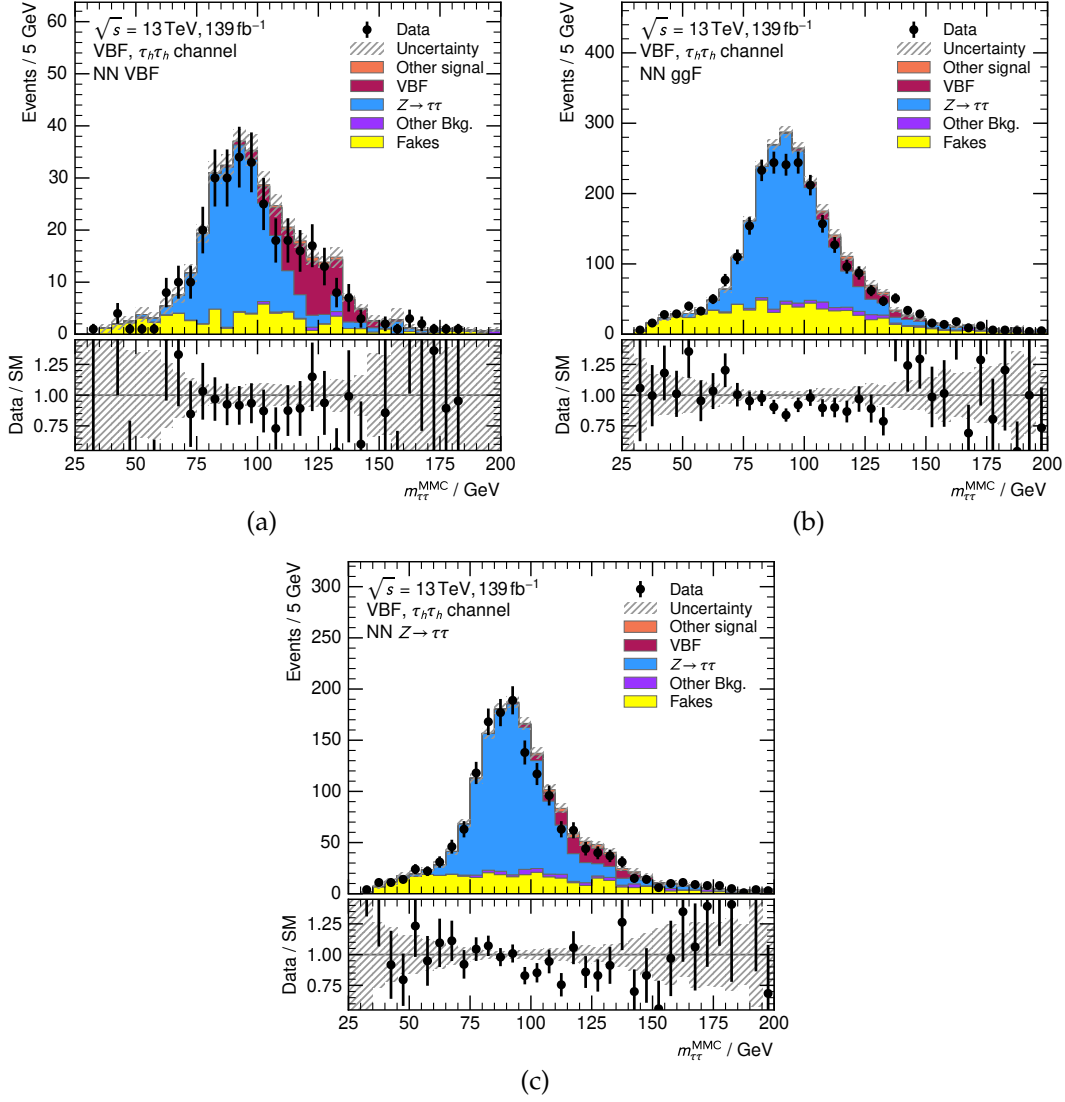
Figure B.8.: Exclusive VBF signal region categories as defined by the NN output for the \tau_{had}\tau_{had} channel. By definition, the categories are designed to increase the fraction of events from VBF (a), ggF (b), and Z \rightarrow \tau\tau processes (c). The hatched band and the error bars indicate statistical uncertainties of the background expectation and measured data, respectively.
