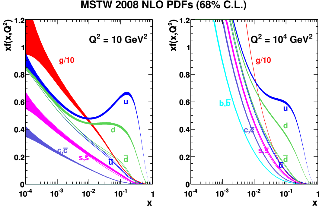
Figure 2.2.: Scaled parton distribution functions for gluons, and valance and sea quarks computed at next-to-leading order. The diagrams show the PDF f(x, Q^2) multiplied by the momentum fraction x of the parton. The PDFs are displayed for two different scales Q^2 [22, 23].
