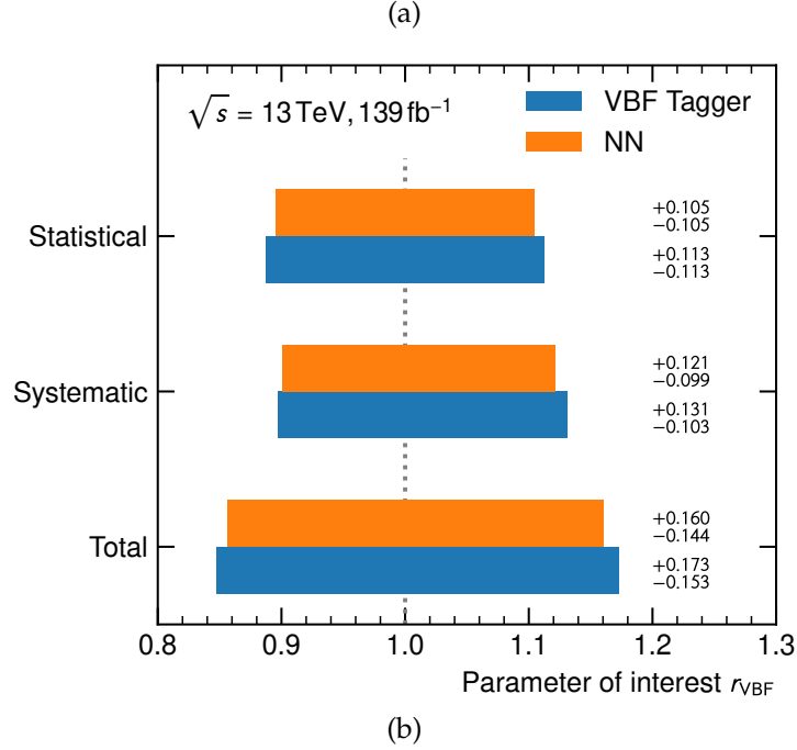
Figure 5.13.: Comparison of the sensitivity between VBF Tagger and NN for each parameter of interest in a 3-POI fit (a) and a decomposition of the uncertainties for the r_{\text{VBF}} parameter (b). The NN-based analysis achieves an approximately 8 % smaller expected uncertainty on the VBF cross section measurement. The fit is performed on an Asimov dataset, and the central value is exactly unity.
