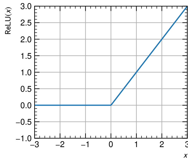
Figure 2.13.: Illustration of the rectified linear unit function \text{ReLU}(x) as a commonly used activation function in neural networks in the range x \in [-3, 3] .
