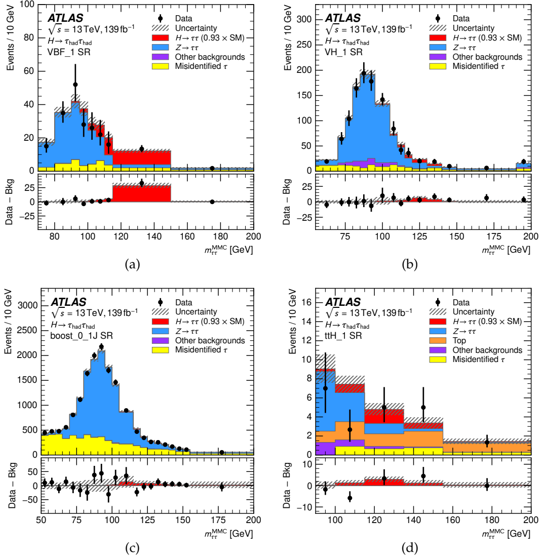
Figure B.11.: Mass m_{\tau\tau}^{\text{MMC}} distributions in selected signal regions of the \tau_{\text{had}}\tau_{\text{had}} channel with the all nuisance parameters set to the value that maximizes the likelihood function [84]. The hatched band and the error bars indicate total uncertainty of the background expectation and statistical uncertainty measured data, respectively.
