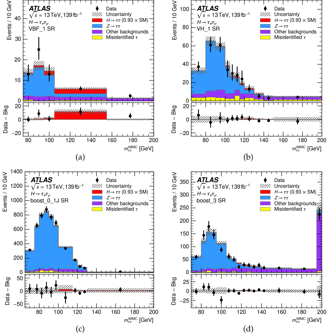
Figure B.9.: Mass m_{\tau\tau}^{\text{MMC}} distributions in selected signal regions of the \tau_e \tau_\mu channel with the all nuisance parameters set to the value that maximizes the likelihood function [84]. The hatched band and the error bars indicate total uncertainty of the background expectation and statistical uncertainty measured data, respectively.
