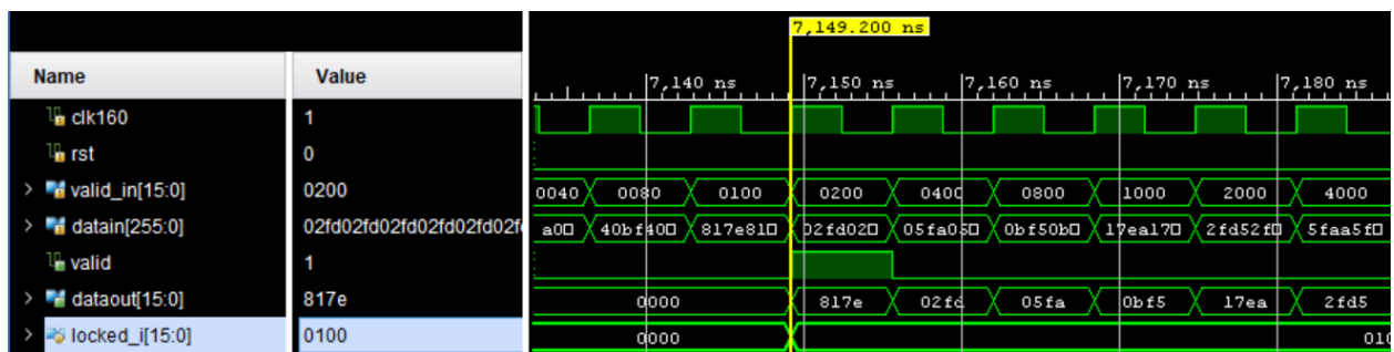
Figure 9: Simulation example of channel getting locked at 7.149 ns
