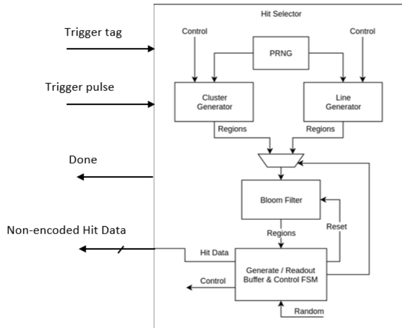
Figure 14: Elaborated architecture of Hit Generator Unit (Picture Credit: Tony)
