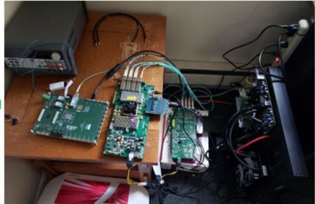
Figure 27: Left: Schematic diagram of the FELIX setup [22]. Right: FELIX hardware setup at UW
