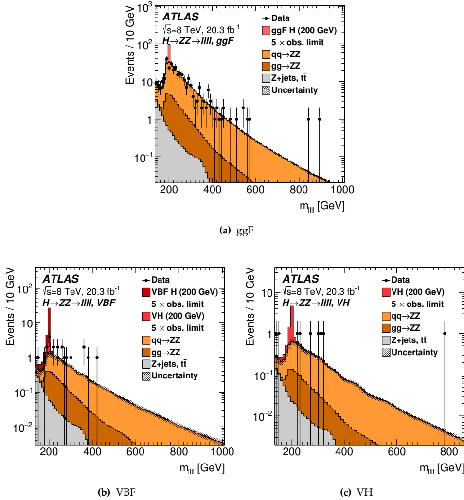
Figure 7.7: Post-fit m_{4\ell} distributions for m_H = 200 GeV for the, (a) ggF, (b) VBF and (c) VH categories. The expected signal for each category is normalised to a cross-section corresponding to five times the observed limit. No significant excess from the expected background is observed.
