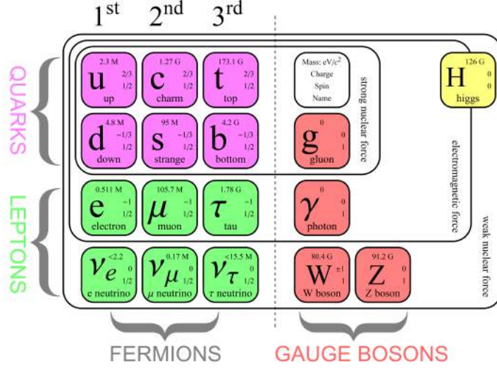
Figure 1.1: The Standard Model particles. Figure from [1]
