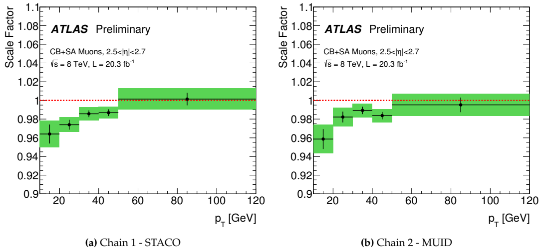
Figure 4.5: Reconstruction efficiency scale factors for the (a) Chain 1 and (b) Chain 2 reconstruction algorithms.
