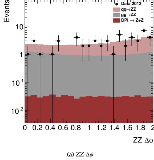
Figure 6.4: Distribution of the observable \Delta\phi for the signal and background events which pass the selection cuts. For the DPI sample \sigma_{\text{eff}} = 15\text{mb} is assumed. Reasonable agreement between data and MC is observed.
