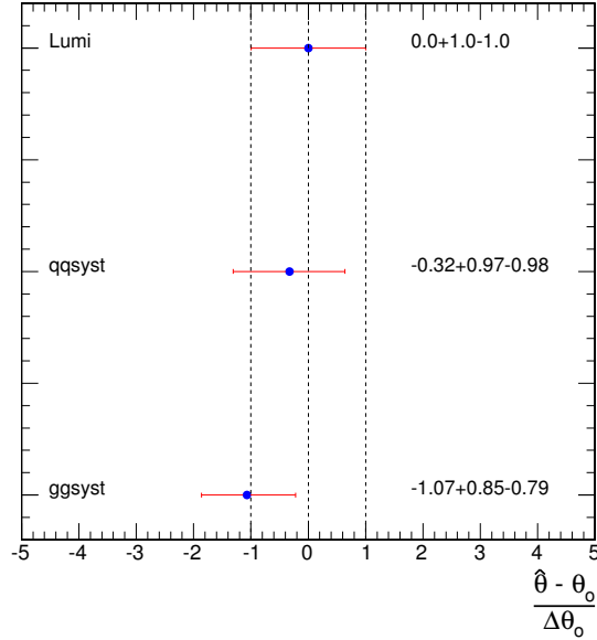
Figure 6.8: Nuisance parameter pulls for the background nuisance parameters and luminosity.
