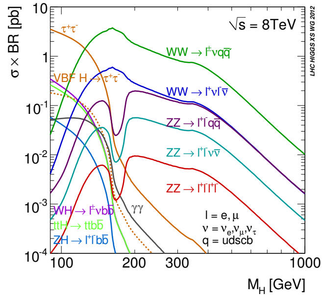
Figure 1.5: Standard Model Higgs boson production cross section times branching ratio at 8 TeV . Figure from [19].
