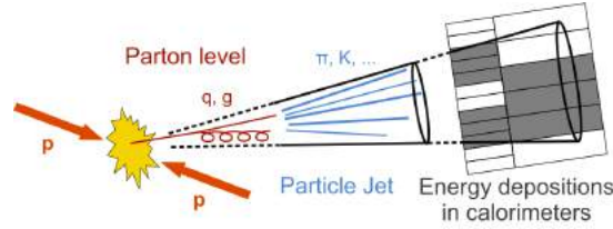
Figure 3.5: Jet production and energy deposit. Figure from [62]
