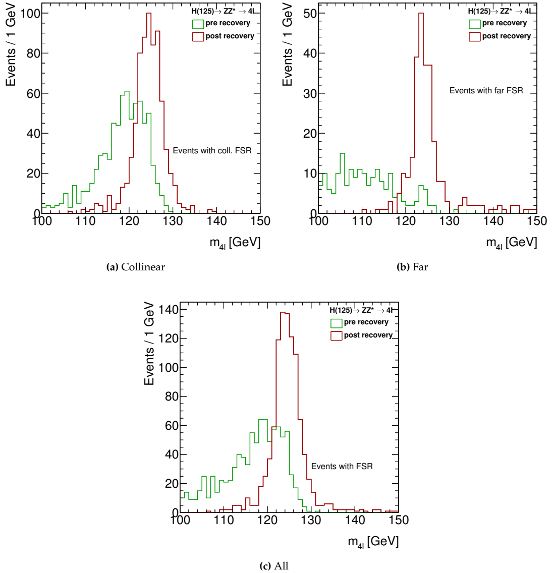
Figure 5.10: MC invariant mass distribution m_{4\ell} of simulated Higgs 125 GeV decaying to four leptons, for events with an identified FSR photon, before (green) and after (red) the FSR correction in case of (a) Collinear FSR, (b) Far FSR, (c) all events.
