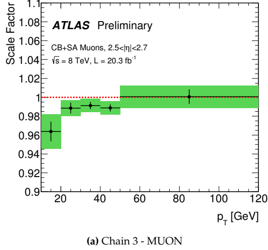
Figure 4.6: Reconstruction efficiency scale factors for the Chain 3 reconstruction algorithm.
