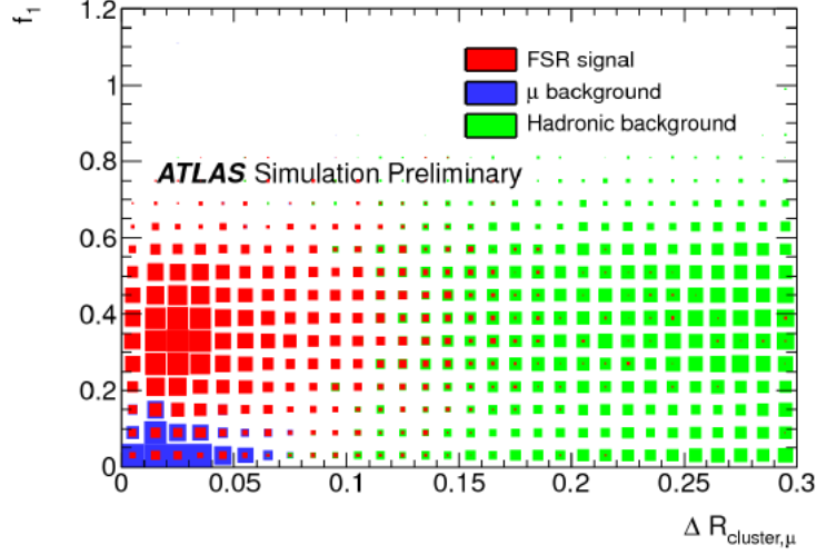
Figure 5.1: Correlation plots of discriminants f_1 , which is the ratio of the photon energy absorbed in the first layer of the calorimeter over total, and \Delta R (cluster, \mu ) with E_T (EM cluster) > 1.3 GeV. Figure from [73]
