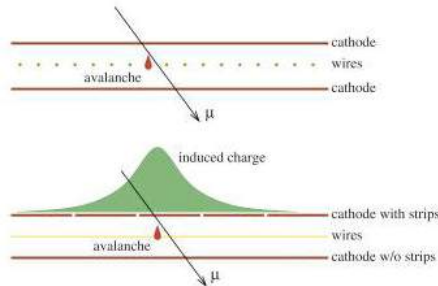
Figure 2.18: Layout of a CSC unit. Figure from [53]
