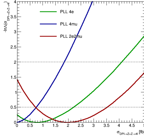
Figure 6.10: Distribution of the profile likelihoods for all the individual channels that are included in the fit with the 1\sigma (dashed line at 0.5) and 2\sigma (dashed line at 2) uncertainty range.
