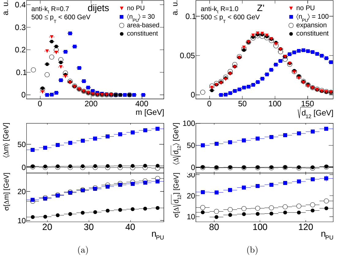
Figure 3.11: Performance of the Constituent Subtraction for jets clustered with the anti- k_t algorithm for (a) the jet mass in dijet events and (b) the \sqrt{d_{12}} variable in Z' \rightarrow t\bar{t} events. Red triangles show distribution without pileup, blue squares show the uncorrected distribution with pileup, open and closed circles show distributions corrected by the shape-expansion and Constituent Subtraction method, respectively. The n_{PU} dependence of mean and standard deviation are shown in the lower panel. [2]
