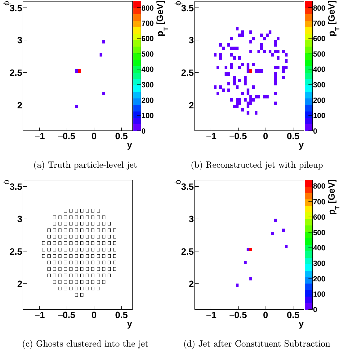
Figure 3.9: Illustration of the Constituent Subtraction method on an example anti- k_t R = 0.7 jet from PYTHIA8 dijet simulation at particle level when overlaid with 25 pileup events. The p_T of the jet constituents in the y - \phi space is shown for (a) jet without pileup, (b) jet with pileup, (c) ghosts clustered into the jet, and (d) corrected jet.
