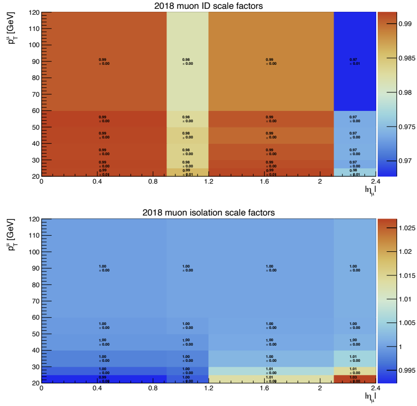
Figure E.5: The figure shows the ratio of muon efficiencies in 2018 data and simulation. The resulting scale factors for both the identification (top) and isolation (bottom) efficiencies are applied per muon in simulation in bins of p_T and absolute \eta .
