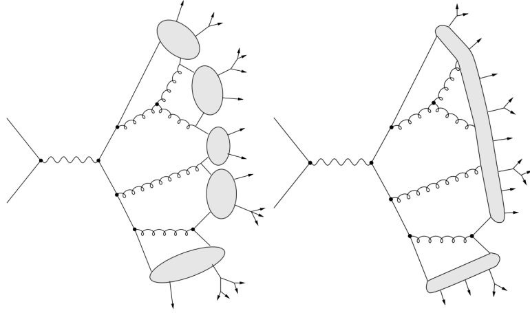
Figure 4.3: An illustration of the two hadronization models. The cluster model is shown on the left and the Lund string model is depicted on the right [66].
