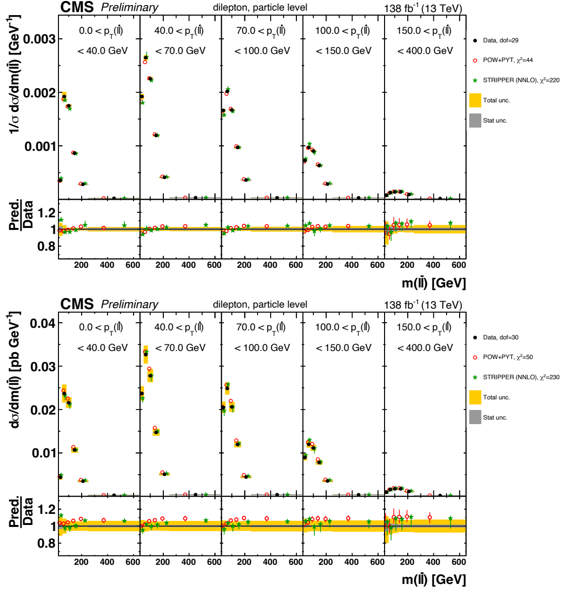
Figure 8.51: Differential t\bar{t} cross sections measured as functions of the invariant mass of the \ell\bar{\ell} system, m(\ell\bar{\ell}) , in ranges of the transverse momentum of the \ell\bar{\ell} system, p_T(\ell\bar{\ell}) , for both normalized (top) and absolute (bottom) measurements performed in the fiducial phase space at particle level. For further details see Figure 8.28.
