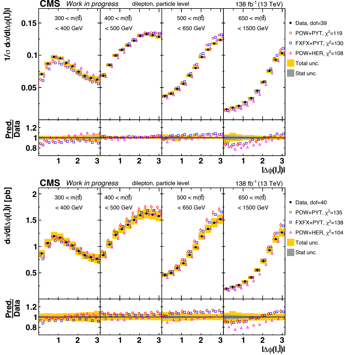
Figure 8.21: Differential t\bar{t} cross sections measured as functions of the absolute value of the azimuthal angle between the lepton and the anti-lepton, |\Delta\phi(\ell, \bar{\ell})| , in ranges of the invariant mass of the t\bar{t} system, m(t\bar{t}) , for both normalized (top) and absolute (bottom) measurements performed in the fiducial phase space at particle level. For further details see Figure 8.1.
