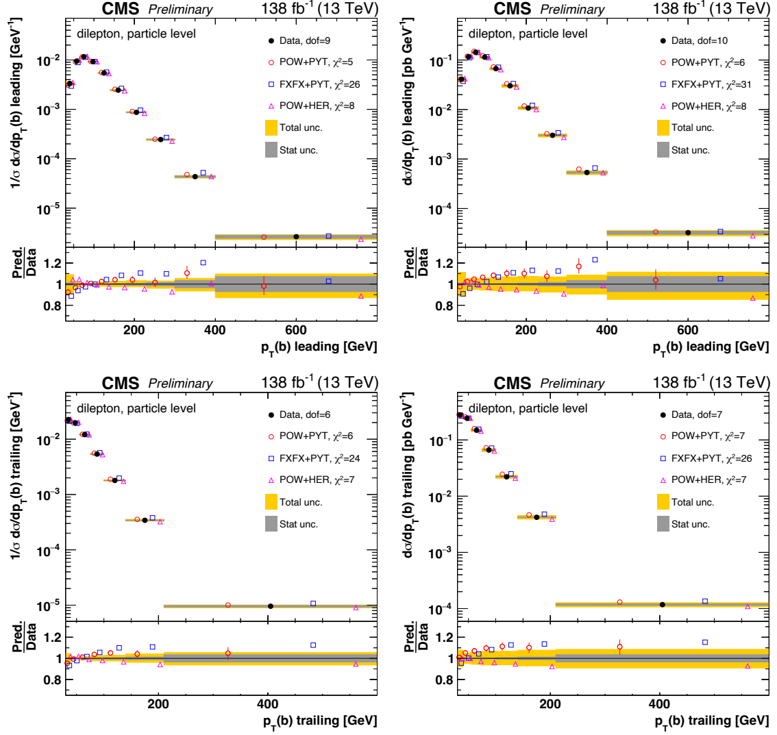
Figure 8.16: Differential t\bar{t} cross sections measured as functions of the transverse momentum of the leading b quark, p_T(b) leading, in the top row and the transverse momentum of the trailing b quark, p_T(b) trailing, in the bottom row. The measurements are performed in the fiducial phase space at particle level. The left and right columns show normalized and absolute cross sections, respectively. For further details see Figure 8.1.
