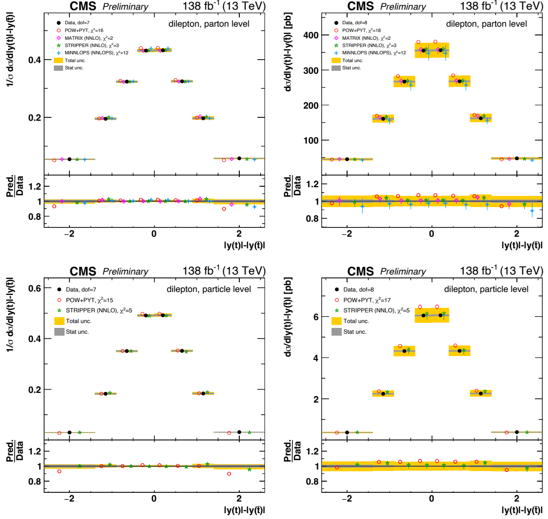
Figure 8.32: Differential t\bar{t} cross sections measured as functions of the difference in absolute value of rapidity of the top and anti-top, |y(t)| - |y(\bar{t})| , in the full phase space at parton level (top row) and in the fiducial phase space at particle level (bottom row). The left and right columns show normalized and absolute cross sections, respectively. For further details see Figure 8.28.
