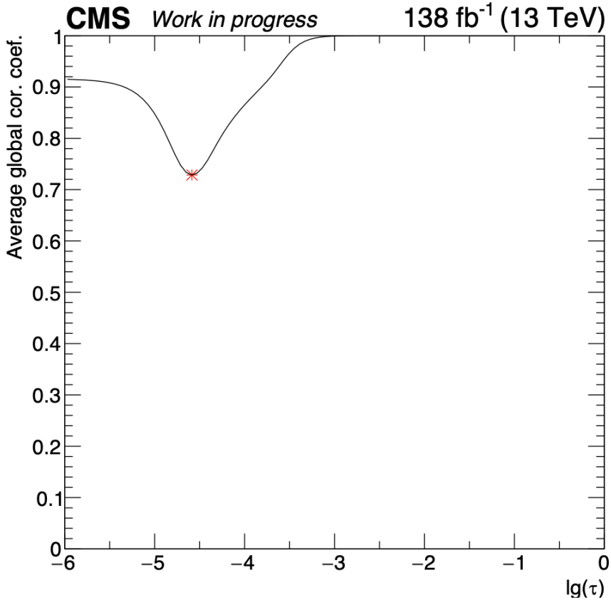
Figure 6.3: The optimal choice of \tau is shown (red star) for the single-differential measurement of the transverse momentum of the top, p_T(t) , at parton level in the full phase space. The average global correlation coefficients are also computed for different points of \log \tau .
