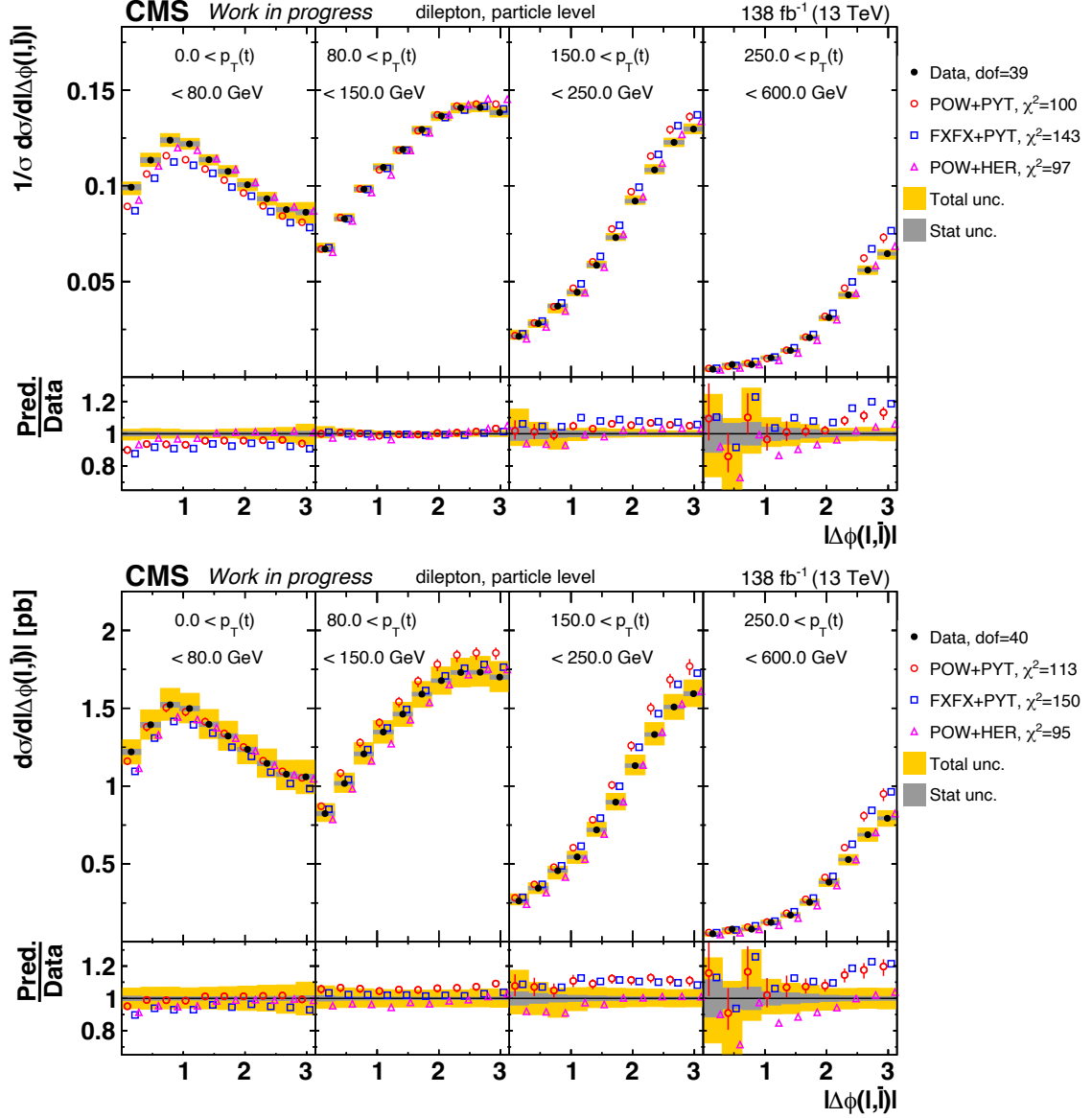
Figure 8.22: Differential t\bar{t} cross sections measured as functions of the absolute value of the azimuthal angle between the lepton and the anti-lepton, |\Delta\phi(\ell, \bar{\ell})| , in ranges of the transverse momentum of the top, p_T(t) , for both normalized (top) and absolute (bottom) measurements performed in the fiducial phase space at particle level. For further details see Figure 8.1.
