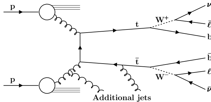
Figure 1.1: An exemplary Feynman diagram of t\bar{t} plus additional jet production in pp collisions is shown for the signal process studied in this work, where the two W bosons both decay to leptons, constituting the dilepton channel.
