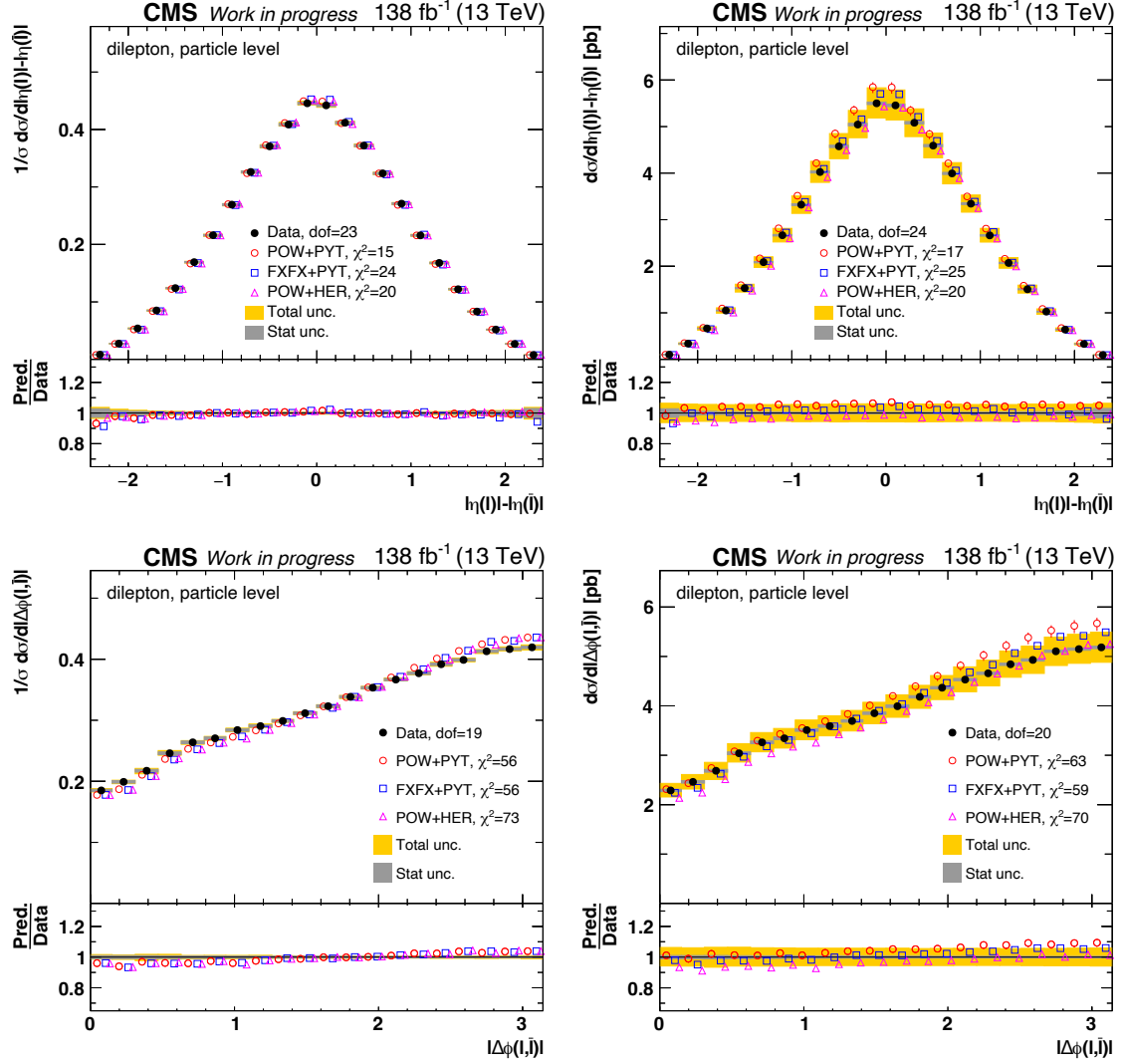
Figure 8.18: Differential t\bar{t} cross sections measured as functions of the difference in absolute pseudorapidity of the lepton and absolute pseudorapidity of the anti-lepton, |\eta(\ell)| - |\eta(\bar{\ell})| , in the top row and the absolute value of the azimuthal angle between the lepton and the anti-lepton, |\Delta\phi(\ell, \bar{\ell})| , in the bottom row. The measurements are performed in the fiducial phase space at particle level. The left and right columns show normalized and absolute cross sections, respectively. For further details see Figure 8.1.
