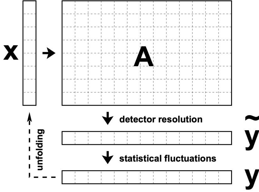
Figure 6.2: A schematic overview illustrating the problem of unfolding for a given observable [126]. Here \mathbf{y} represents the observed number of events at detector level, including statistical fluctuations, \tilde{\mathbf{y}} is the expected number of events at detector level, \mathbf{A} is the response matrix and \mathbf{x} is the estimator of the true spectrum.
