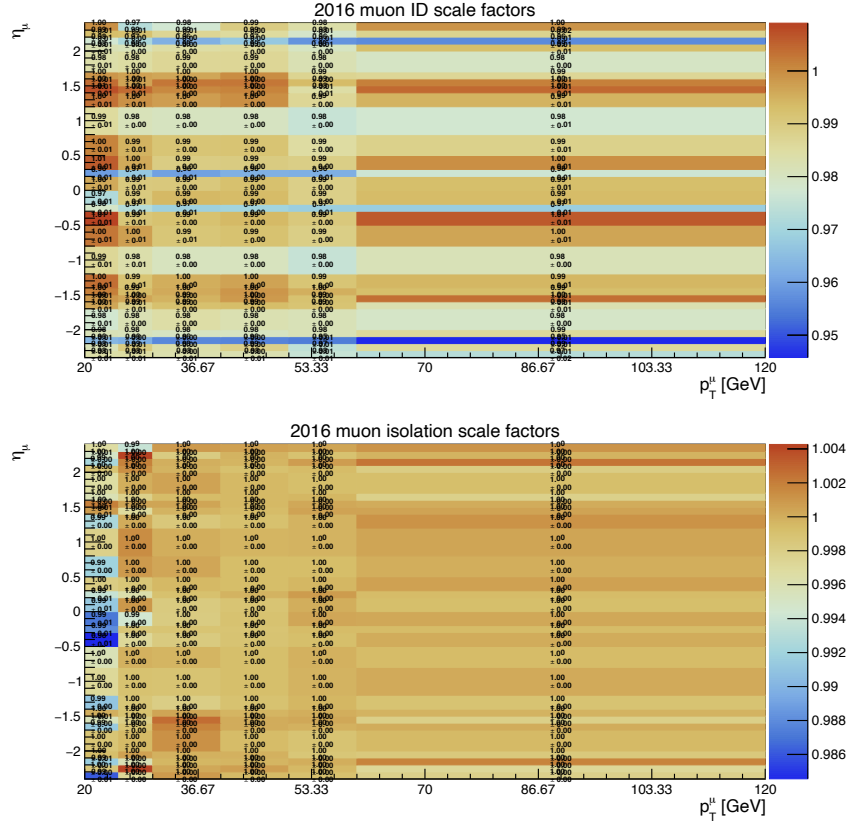
Figure E.1: The figure shows the ratio of muon efficiencies in 2016 data and simulation. The resulting scale factors for both the identification (top) and isolation (bottom) efficiencies are applied per muon in simulation in bins of p_T and \eta .
