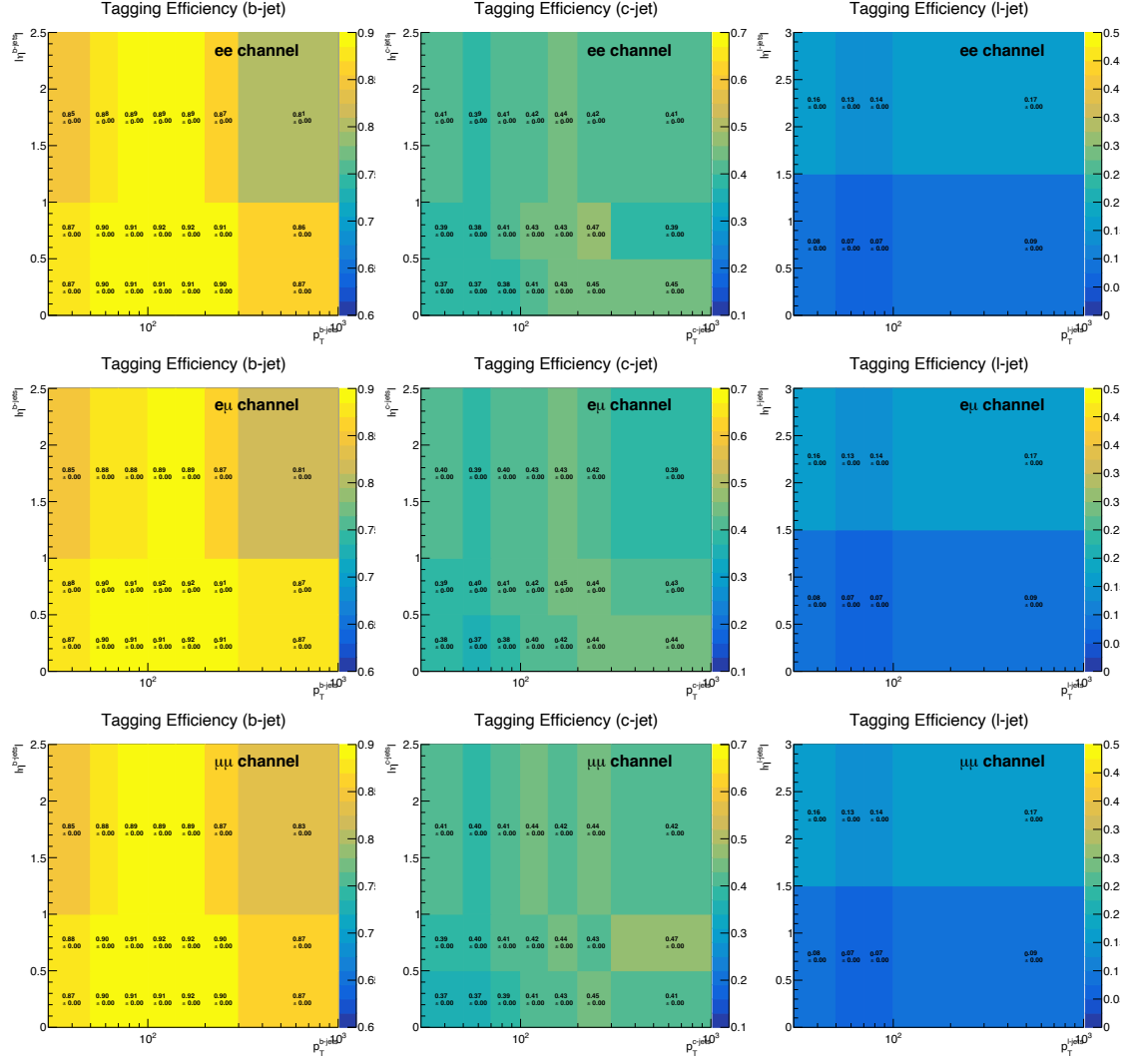
Figure F.3: The b-tag efficiency and mistag rates are computed in bins of jet p_T and \eta and are shown for 2018 in the e^\pm e^\mp (top row), e^\pm \mu^\mp (middle row) and \mu^\pm \mu^\mp (third row) channels. The b-tagging efficiency is shown in the first column while the mistag rates for c- and light-jets are shown in the second and third column, respectively.
