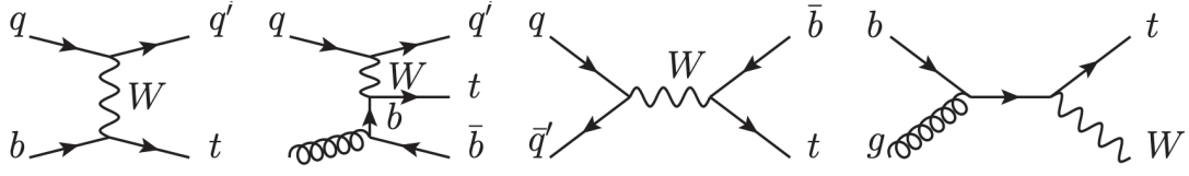
Figure 2.5: Feynman diagrams of single top production at leading order [28].
