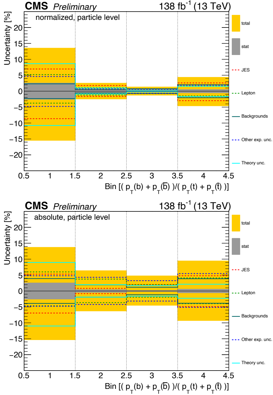
Figure J.30: The figure shows the uncertainty contributions of the differential t\bar{t} cross section measured as a function of the ratio of the scalar sum of p_T of b and p_T of anti- b over the scalar sum of p_T of top and p_T of anti-top, (p_T(b) + p_T(\bar{b})) / (p_T(t) + p_T(\bar{t})) , for both normalized (top) and absolute (bottom) measurements performed in the fiducial phase space at particle level.
