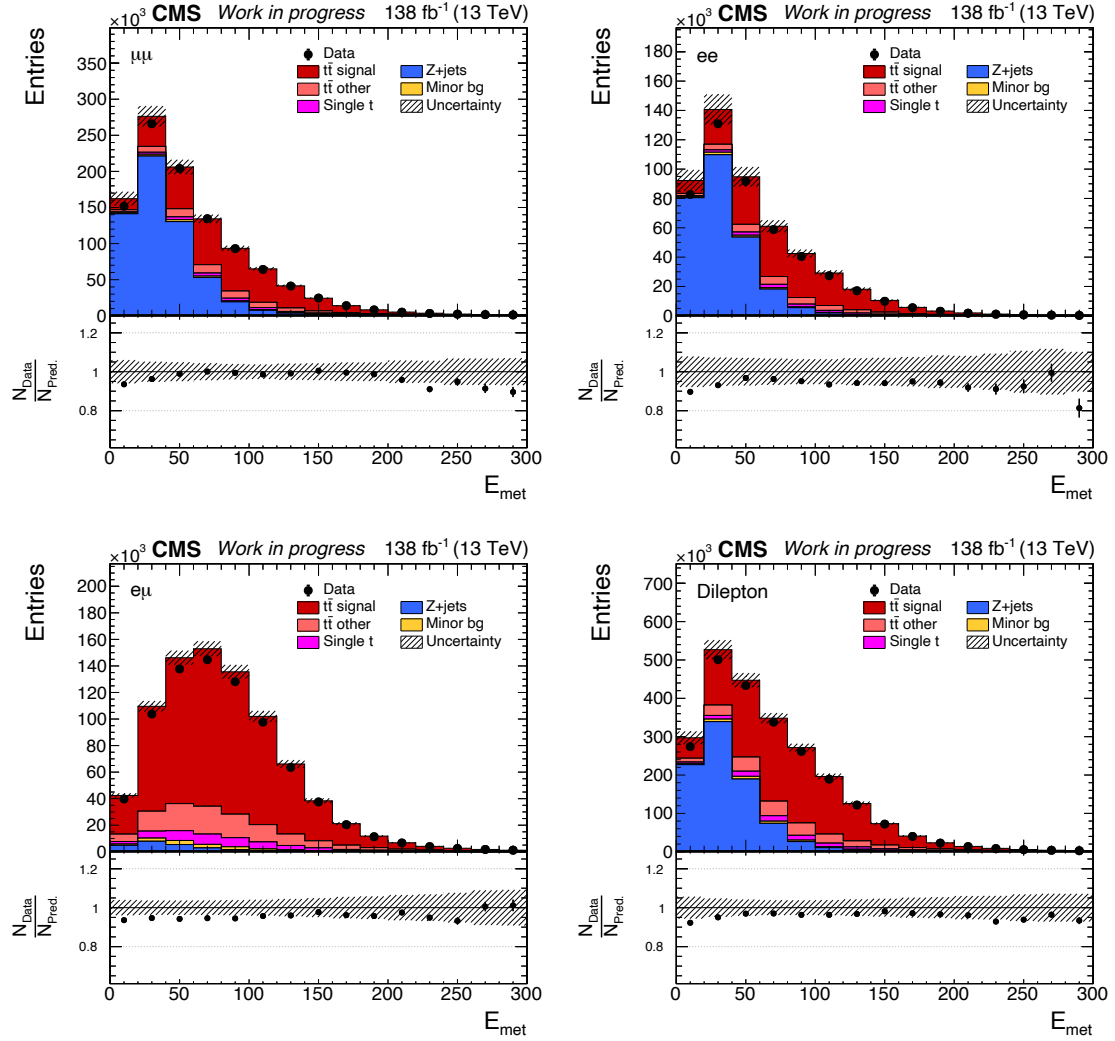
Figure 5.9: Distributions of the missing transverse energy, E_{\text{T}}^{\text{miss}} , are shown separately for the \mu^\pm\mu^\mp (top left), e^\pm e^\mp (top right), e^\pm\mu^\mp (bottom left) and combined channels (bottom right) at step 5 in the selection cutflow, after requiring at least two jets. See Figure 5.7 for further details.
