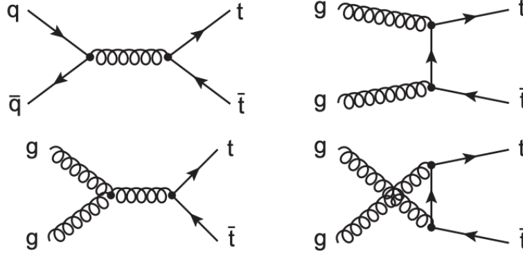
Figure 2.3: Feynman diagrams of top pair production at leading order for quark-anti-quark annihilation (top left) and gluon-gluon fusion in the s-channel (bottom left), t-channel (top right) and u-channel (bottom right) [35].
