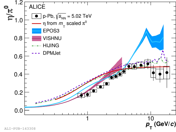
FIGURE V-20: The \eta/\pi^0 ratio in p-Pb collisions at \sqrt{s_{NN}} = 5.02 TeV [323] compared to EPOS3 [348] (blue band), VISHNU [349] (violet band), HIJING [100] (green dot-dashed line) and DPMJET [350] (dark blue dashed line) models as well as m_T scaling predictions (red solid line).
