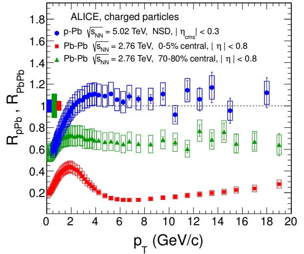
FIGURE II-8: Nuclear modification factor as a function of p_T for 0 – 5% central (red squares) and 70 – 80% central (green triangles) Pb-Pb collisions at \sqrt{s_{NN}} = 2.76 TeV and for p-Pb collisions (blue dots) at \sqrt{s_{NN}} = 5.02 TeV. The color bands at unity are normalization uncertainties [51].
