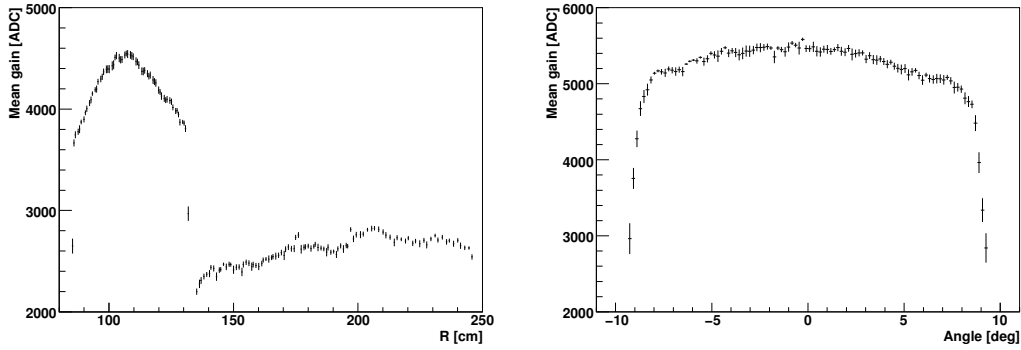
FIGURE IV-19: Radial (left) and azimuthal (right) systematics of gain variation within one sector. The step observed in the radial variation is due to the IROC-OROC transition.
