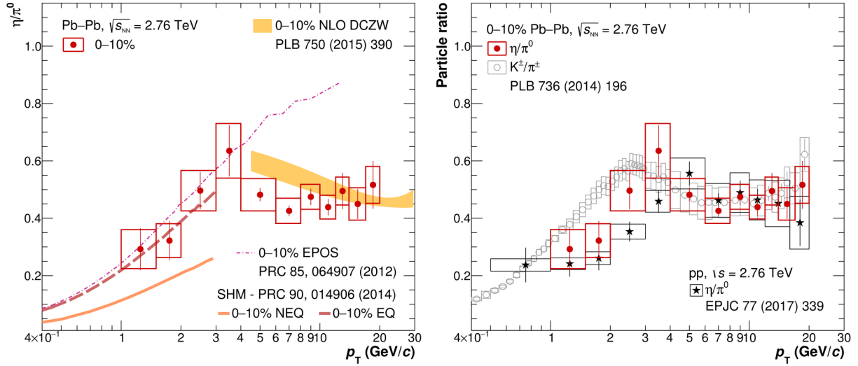
FIGURE V-21: Left: The \eta/\pi^0 ratio for the 0-10% most central Pb-Pb collisions at \sqrt{s_{NN}} = 2.76 TeV [324] compared to EPOS [351] (dot-dashed line), SHM [354, 355, 356] (EQ - dashed line, NEQ - solid line) models and NLO pQCD calculations [358] (orange band). Right: The same ratio (full circles) compared to a corresponding result in pp collisions (stars) and to the K^\pm/\pi^\pm measurement in the same centrality class, system and energy [359] (open circles).
