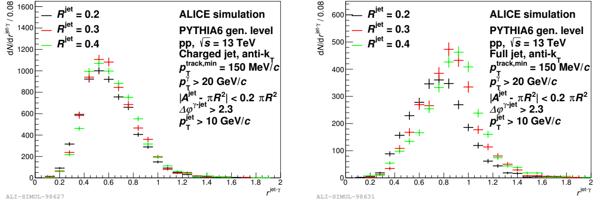
FIGURE VI-8: Photon-jet transverse momentum balance for jets reconstructed with different resolution parameter R^{\text{jet}} = 0.2, 0.3 and 0.4 for charged (left) and full (right) jets.
