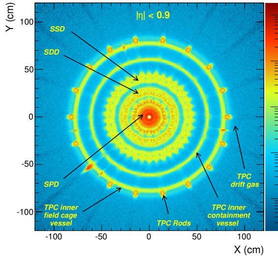
FIGURE IV-26: Distribution of the reconstructed photon conversion points for |\eta| < 0.9 in the plane transverse to the beam [303].
