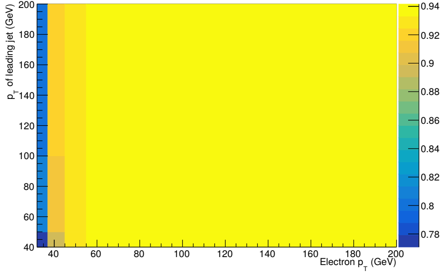
Figure C.2: Electron trigger scale factors in dependence of electron and leading jet p_T . The scale factors are calculated using 2017 single muon data samples and simulated dileptonic t\bar{t} events.
