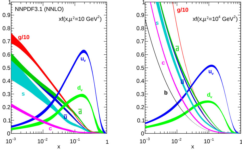
Figure 3.2: The Neural Network Parton Distribution Function (NNPDF) set. Shown are the NNPDF3.1 sets at next-to-next-to-leading order (NNLO) for valence quarks, sea quarks, and gluons for the momentum transfers 10 \text{ GeV}^2 (left) and 10^4 \text{ GeV}^2 (right). The gluon distribution, scaled by a factor of 1/10 , is dominant for low proton momentum fraction values x . Taken from Ref. [84].
