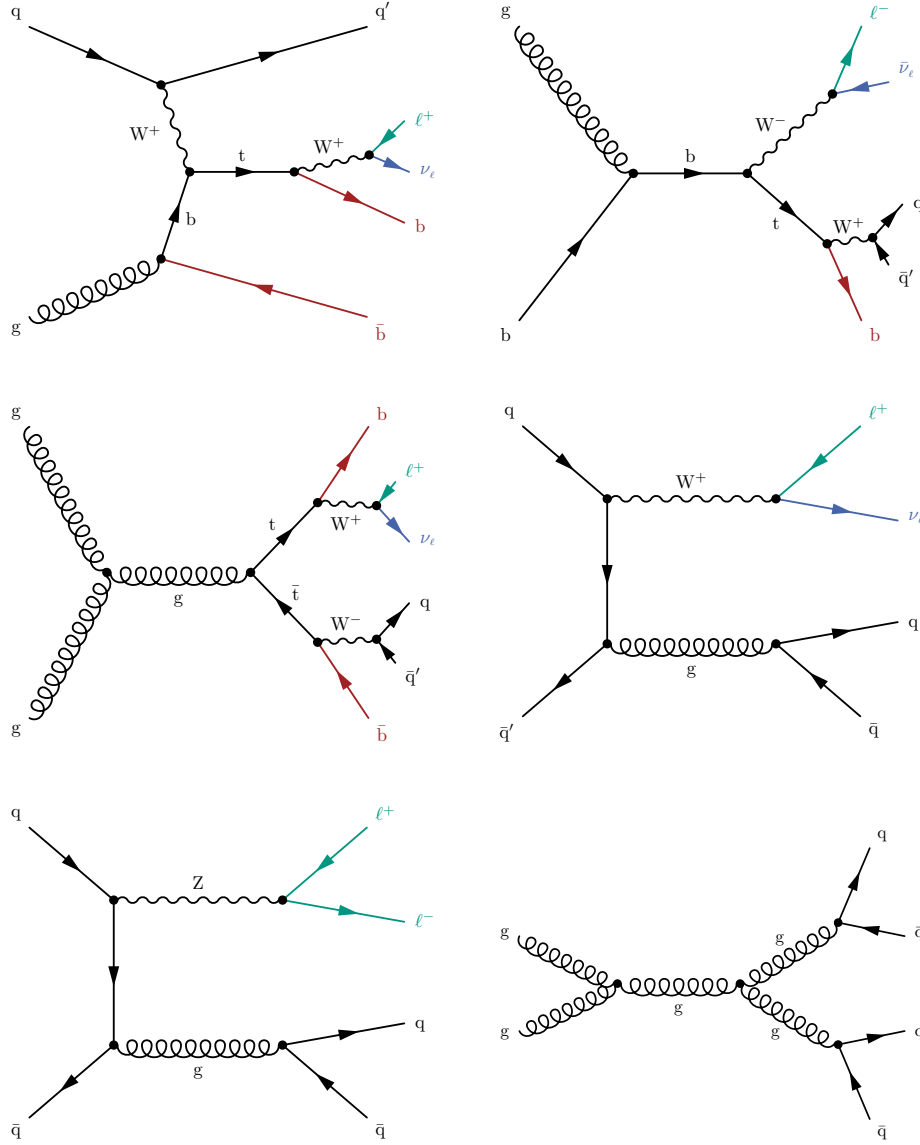
Figure 5.3: Background processes for s-channel single top quark production. LO Feynman diagrams for all relevant background processes that can mimic the final state of the signal process are shown: the t -channel and tW single top quark production modes (top left and top right), t\bar{t} production, which is the dominant background (center left). Minor background contributions are the production of W and Z bosons in association with jets (center right and bottom left), and QCD multijet production (bottom right).
