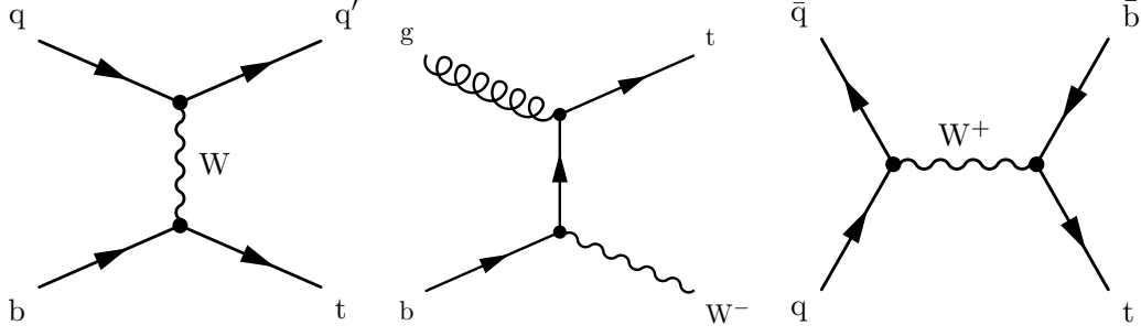
Figure 1.4: Single top quark production. Single top quarks are produced via electroweak interaction. The dominant production mode at the LHC is the t -channel process (left), where the top quark is produced together with a light-flavored quark in forward direction, followed by the production of a single top quark with a W boson (center), called tW process. The rarest production mode is the production of a top quark with a bottom quark via the s channel (right).
