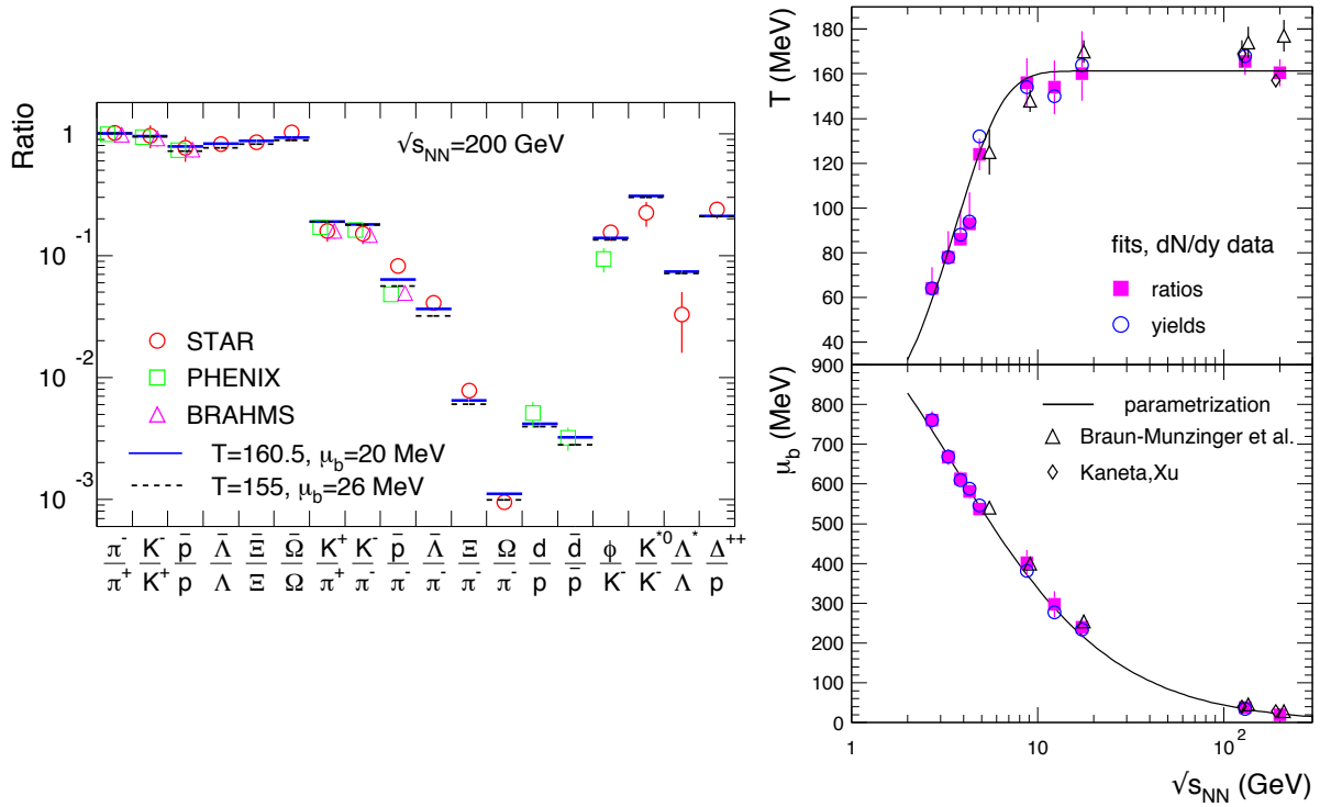
Figure 2.1: Results of Thermal Fits in Heavy Ion Experiments - Left: results of a thermal fit to particle ratios measured at RHIC, for Au–Au collisions at \sqrt{s_{NN}} = 200 GeV. Right: Temperature and Baryon Chemical Potential extracted from thermal fits for a selection of SPS and RHIC collision energies. [61]
