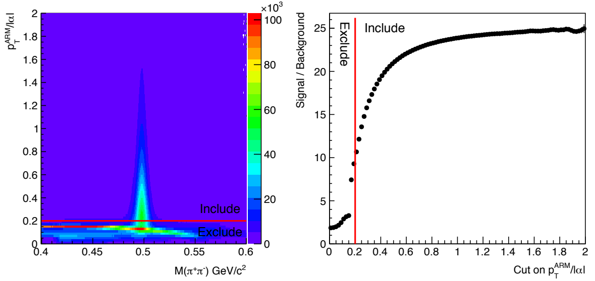
Figure 4.13: Distribution of K_S^0 with Armenteros-Podolanski Variables in Pb-Pb - Left: invariant mass of K_S^0 candidates against p_T^{\text{ARM}}/|\alpha| . Right: estimated signal to background ratio of K_S^0 candidates as a function of the Armenteros-Podolanski cut chosen.
