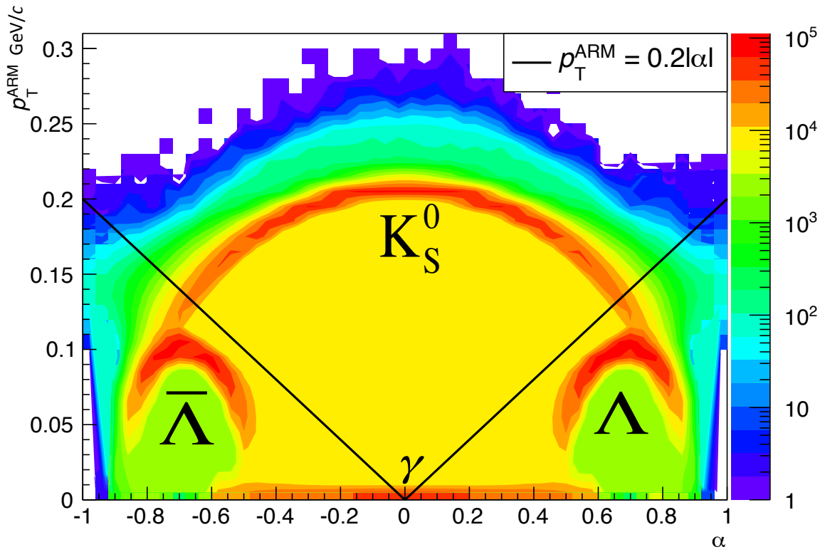
Figure 4.12: Armenteros-Podolanski Diagram for K_S^0 Candidates - Plot of p_T^{\text{ARM}} against \alpha for V0s satisfying all other K_S^0 cuts, before any invariant mass selection. The symmetrical central ellipse is the K_S^0 , while the \Lambda and \bar{\Lambda} are off-centre due to the asymmetric mass of their decay products. The peak at very low p_T^{\text{ARM}} is due to \gamma conversions, and does not enter the invariant mass range used for fitting. The line indicates the cut used; all V0s below this line are rejected as K_S^0 candidates.
