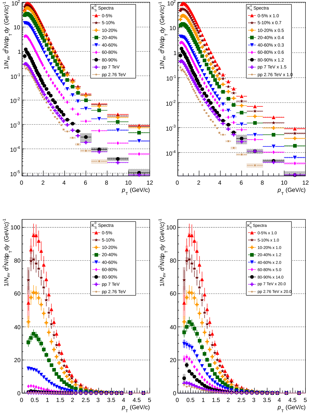
Figure 5.1: K_S^0 Spectra - The fully corrected spectra of K_S^0 , shown in log scale (top) and linear scale (bottom). The right hand plots have a scaling factor applied, to more clearly separate the spectra while leaving the centrality ordering unchanged.
