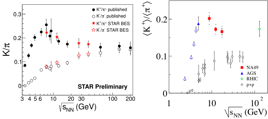
Figure 1.8: K/\pi Ratio at SPS, AGS and RHIC - Left: charged kaon to pion ratios measured by STAR at RHIC as a function of beam energy [45]. Right: charged K^+/\pi^+ ratio as a function of beam energy measured in Pb–Pb and pp collisions at SPS, AGS and RHIC [46]
