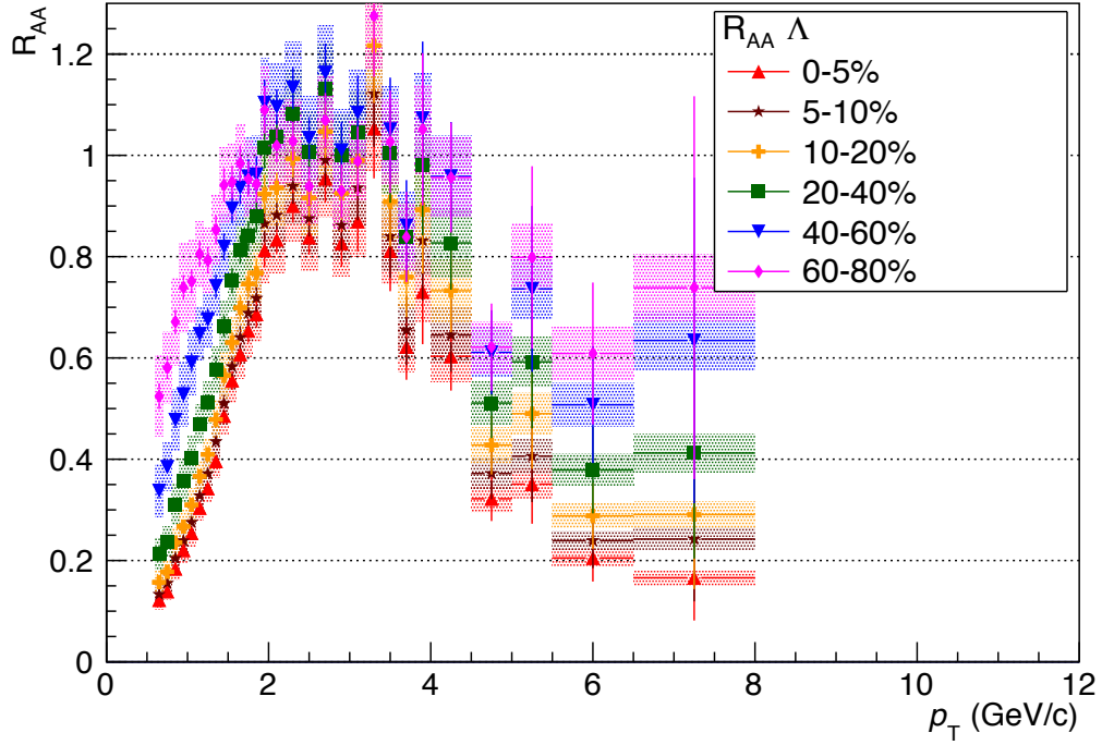
Figure 5.13: \Lambda R_{AA} - R_{AA} of \Lambda for all measured centrality bins. Statistical errors are indicated by the lines, while systematic errors are represented by the hatched areas.
