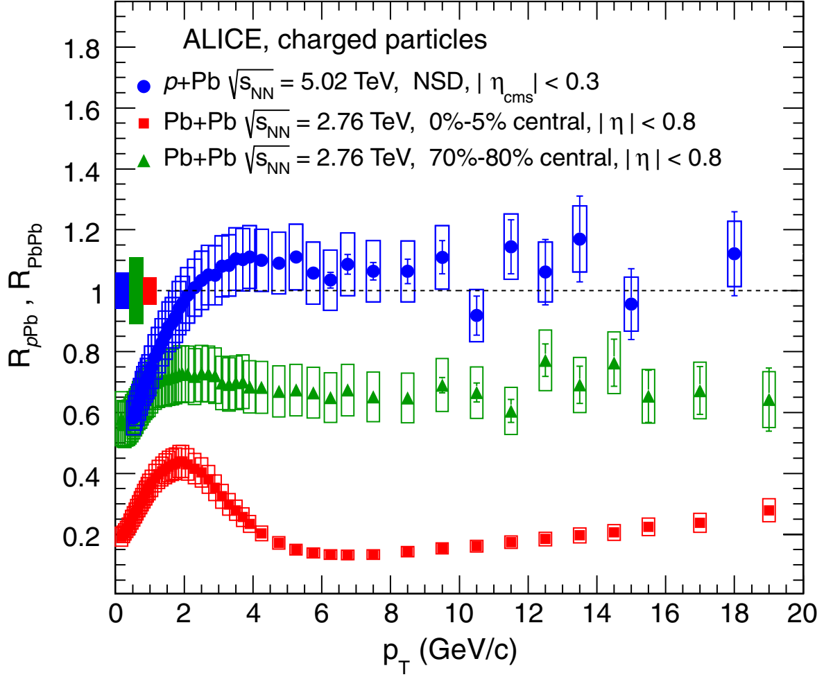
Figure 6.6: R_{pPb} as Measured in ALICE, Compared to R_{AA} - R_{AA} measurements for charged particles at ALICE, compared with the equivalent measurement, R_{pPb} , in p-Pb collisions [169]. Systematic uncertainties are indicated by the boxes.
