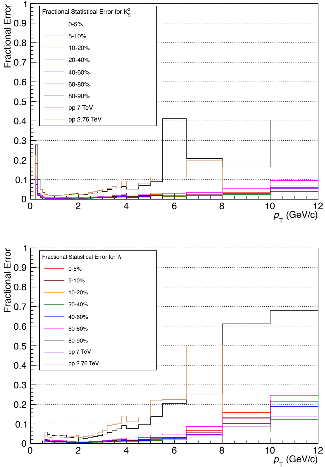
Figure 4.26: Fractional Statistical Errors on \Lambda and K_S^0 Spectra. - The statistical uncertainties of the corrected K_S^0 (top) and \Lambda (bottom) spectra, expressed as a fraction of the corrected spectra. Colours indicate different centralities and colliding systems.
