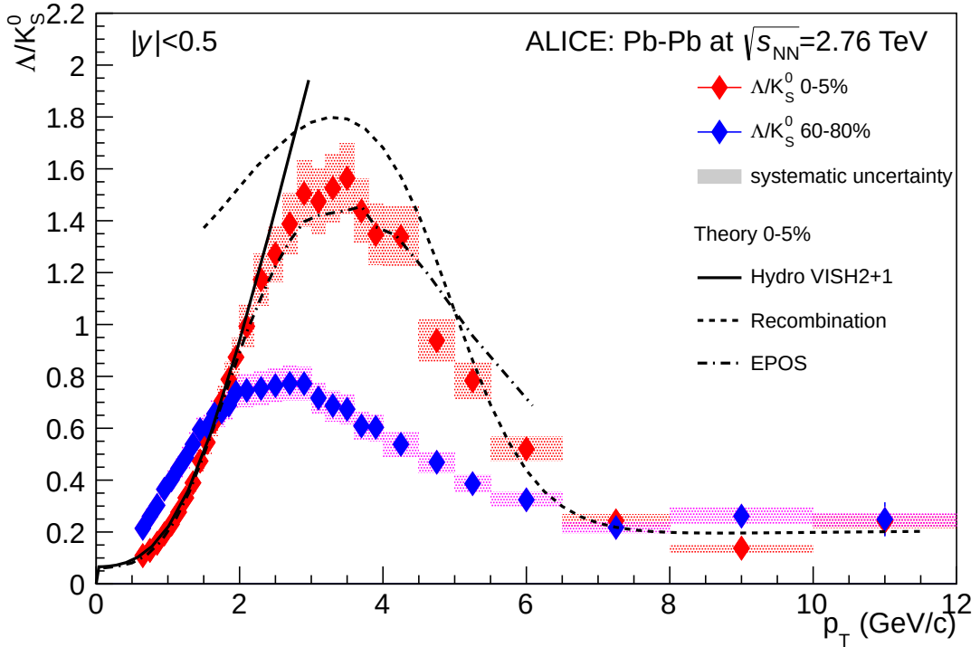
Figure 5.7: \Lambda/K_S^0 Ratio Compared with Theory - The \Lambda/K_S^0 ratio, as measured in 0-5% and 60-80% centrality bins, as compared to theoretical predictions for the 0-5% centrality.
