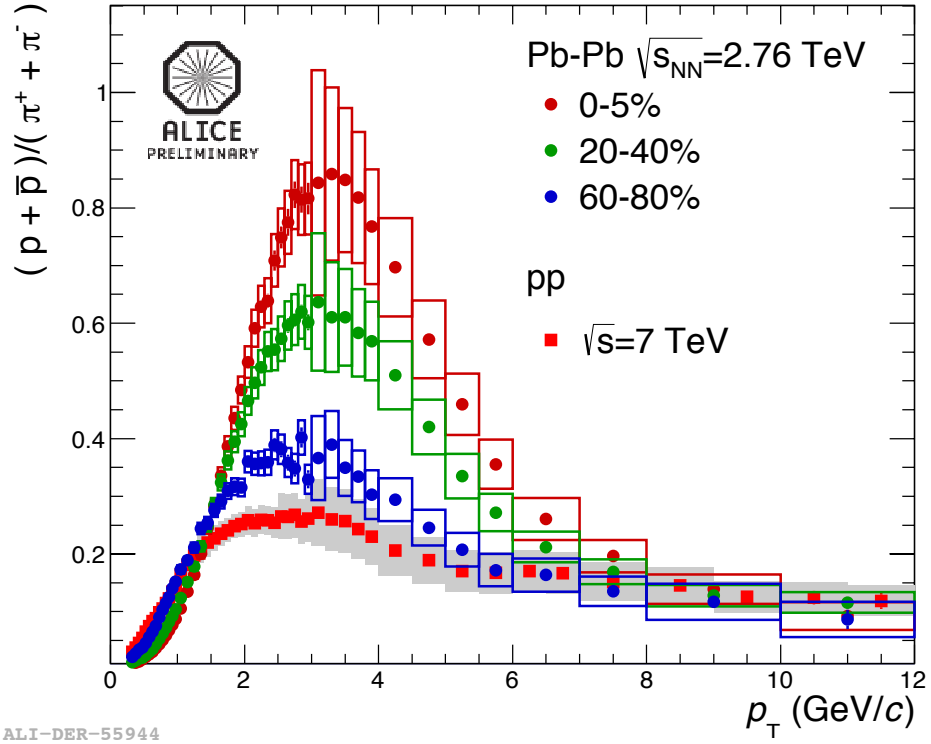
Figure 5.11: p/\pi Ratio Measured by ALICE - The ratio of protons and their antiparticles to charged pions, for selected centralities in Pb-Pb collisions, and pp collisions at \sqrt{s} = 7 TeV [162].
