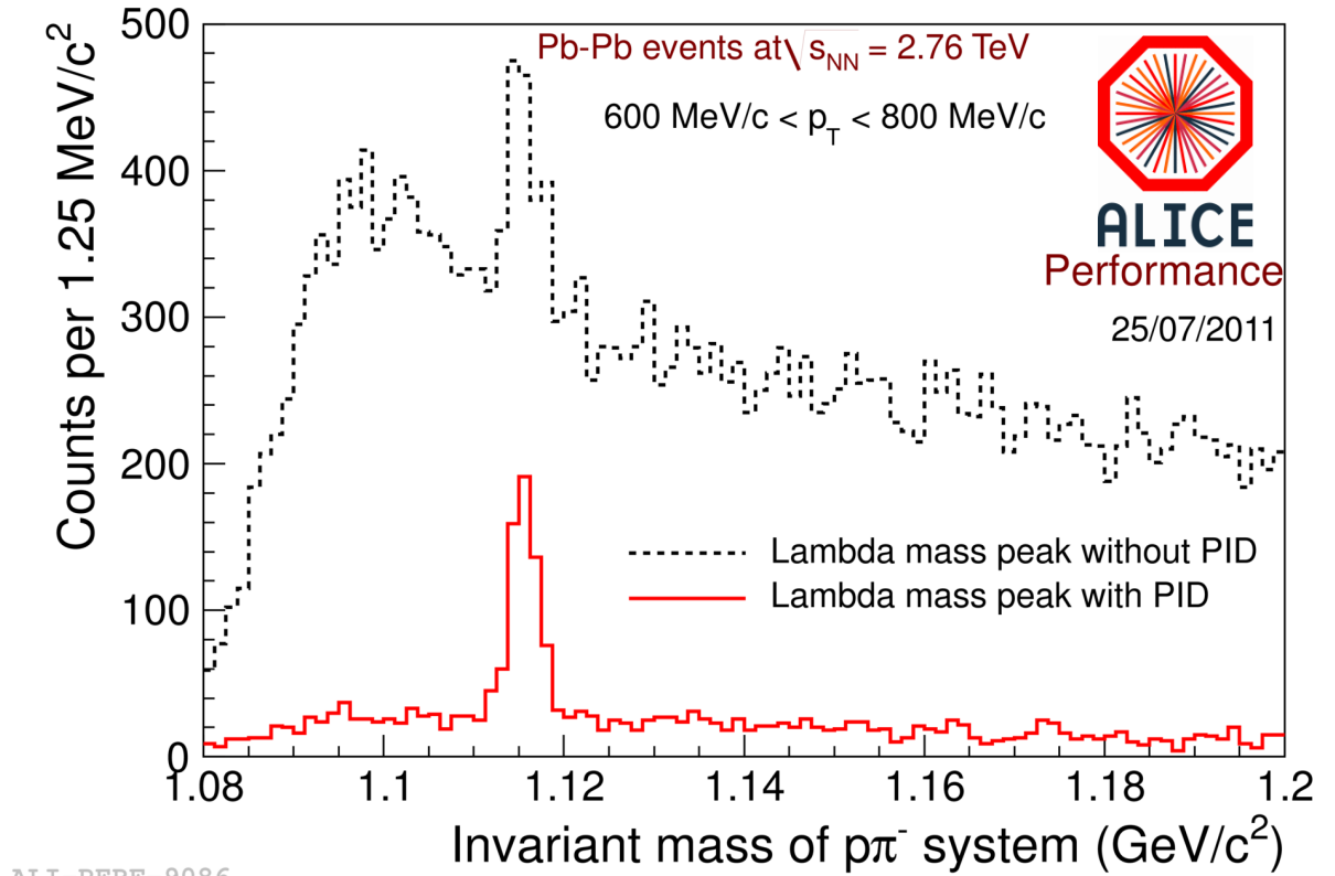
Figure 4.10: Invariant Mass of \Lambda candidates - Invariant mass of \Lambda candidates for 0.6 \text{ GeV}/c < p_T < 0.8 \text{ GeV}/c , with and without PID [152].
