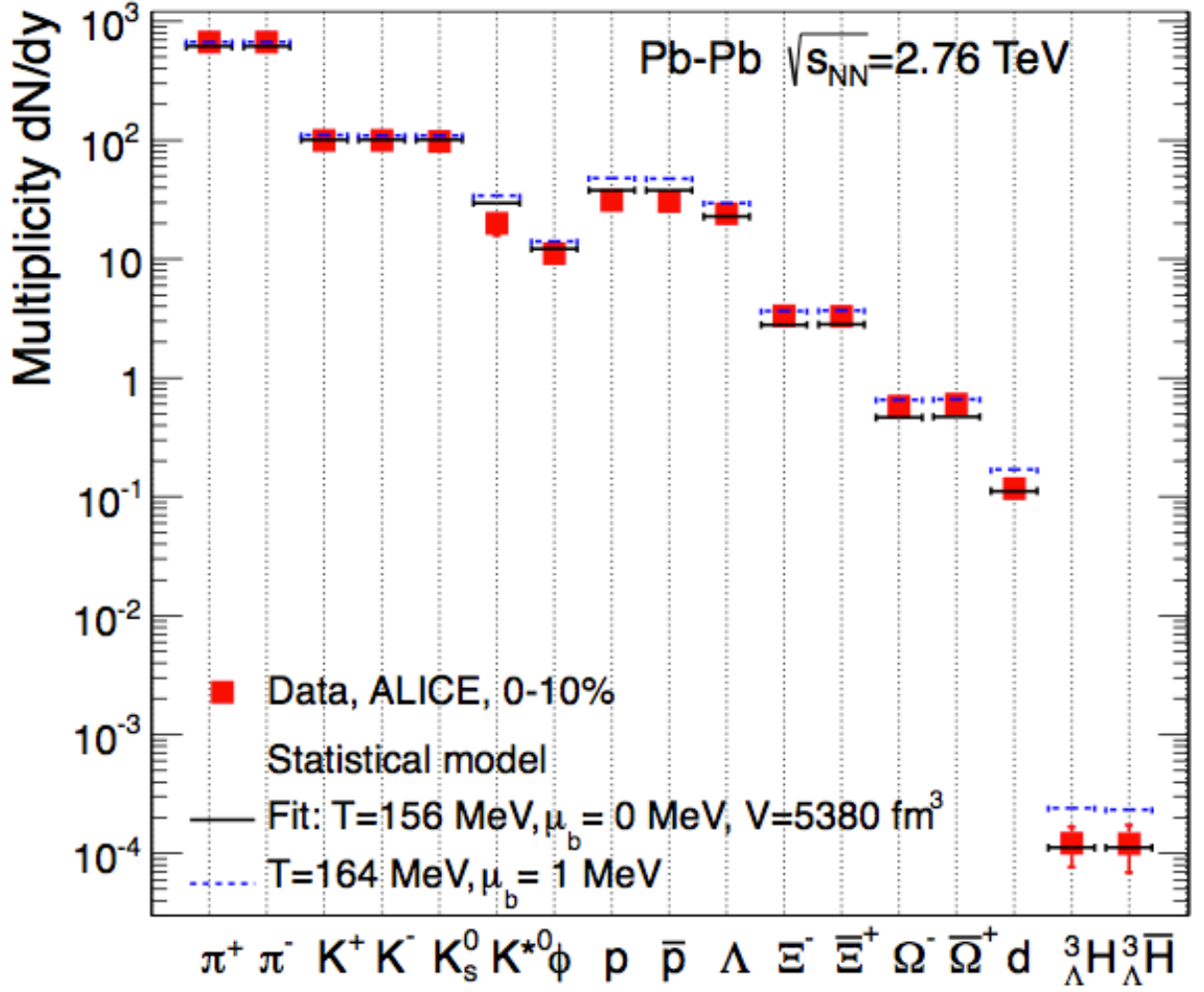
Figure 5.16: Thermal Fit to ALICE 0-10% Data - Thermal fit to central ALICE data, taken from [3]
