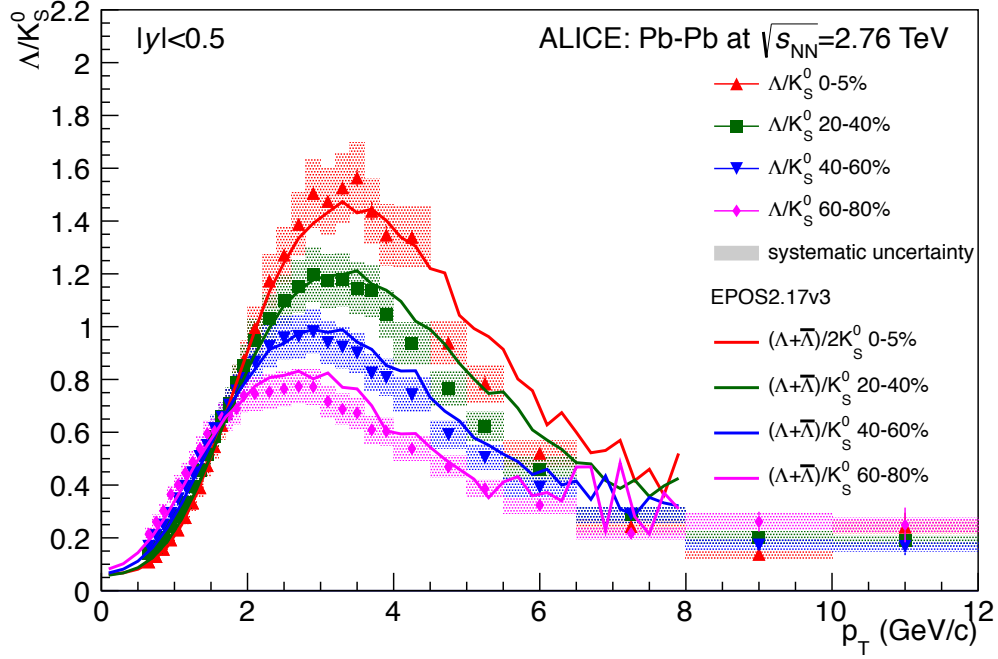
Figure 5.9: \Lambda/K_S^0 Ratio Compared with the EPOS Model - The \Lambda/K_S^0 ratio for selected centralities, as compared to the predictions from the EPOS model for matching centralities.
