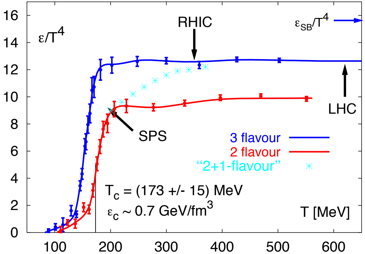
Figure 1.5: Lattice Predictions of Energy Density - Energy density of QCD medium as calculated with Lattice QCD. Also shown is the prediction from the ideal gas model, \epsilon_{SB} . The critical temperature depends slightly on the number of light quark flavours considered. [19]
