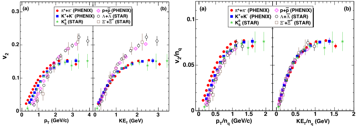
Figure 2.8: \nu_2 Measured in RHIC - Elliptic flow as measured in \sqrt{s_{NN}} = 200 GeV Au–Au collisions at RHIC for various particle species [123]. Within each panel, the left plot is shown as a function of p_T and the right as a function of transverse kinetic energy. The right panel has been scaled to the number of valence quarks.
