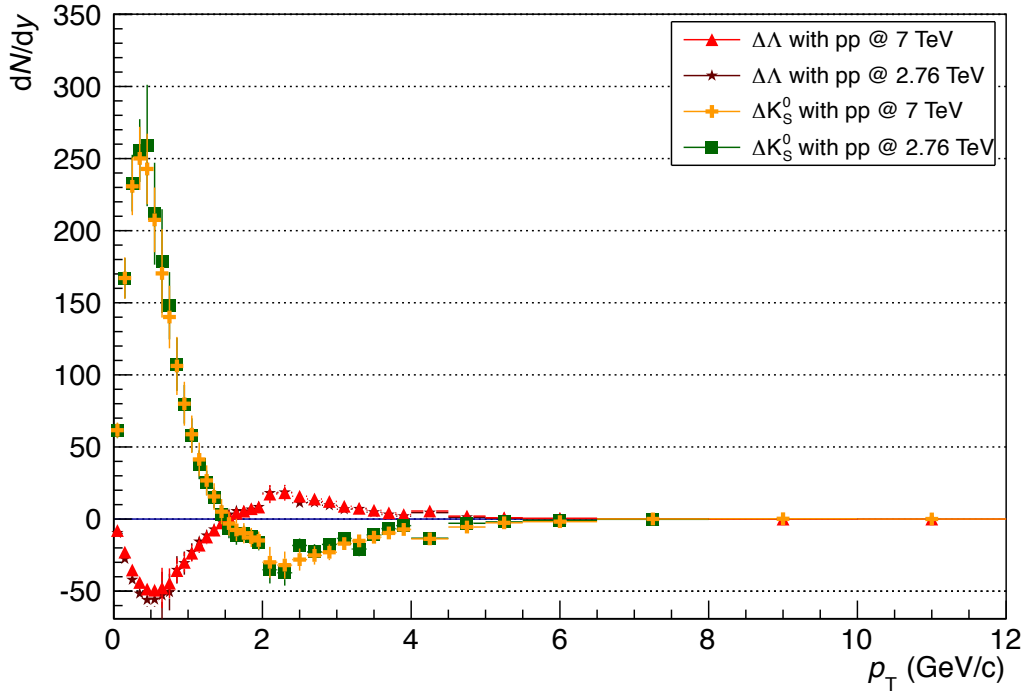
Figure 6.4: \Delta\Lambda and \Delta K_S^0 Required to Change pp-like \Lambda/K_S^0 Ratio to Pb–Pb-like. - \Delta\Lambda and \Delta K_S^0 calculated under the assumption that the other particles distribution is unchanged between pp and Pb–Pb, and that there are 1000 \Lambda particles.
