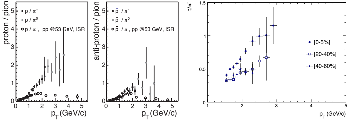
Figure 1.11: p(\bar{p})/\pi Ratio at RHIC - (Anti-)proton to pion ratio measured in Au–Au collisions at RHIC. Left and Centre: p/\pi and \bar{p}/\pi ratio measured by PHENIX in 0-10% most central \sqrt{s_{NN}} = 130 GeV Au–Au collisions [56]. Also shown are similar measurements in pp collisions at \sqrt{s} = 53 GeV. Right: \bar{p}/\pi ratio measured by STAR in \sqrt{s_{NN}} = 200 GeV Au–Au collisions for a selection of centralities [57].
