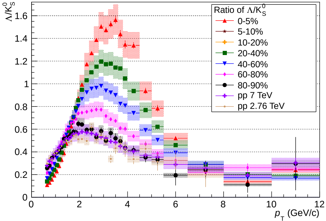
Figure 5.5: \Lambda/K_S^0 Ratio - The \Lambda/K_S^0 ratio for Pb–Pb and pp collisions. Only selected centralities shown for clarity.
