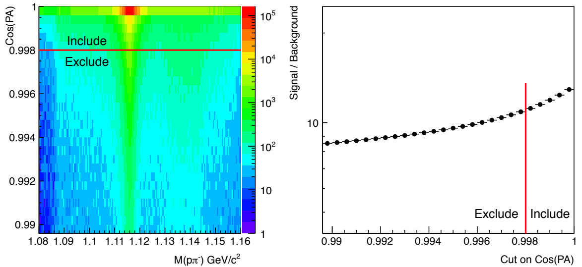
Figure 4.3: Distribution of \Lambda with Cosine of Pointing Angle in 7 TeV pp - Left: invariant mass of \Lambda candidates against cosine of pointing angle. Right: estimated signal to background ratio of \Lambda candidates as a function of the cosine of pointing angle cut chosen.
