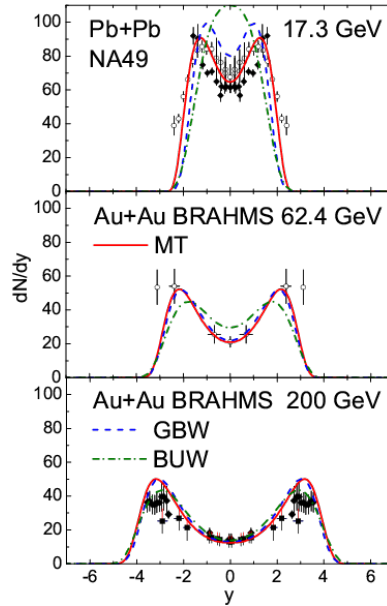
Figure 1.6: Baryon Transport at RHIC and the SPS - Net baryon number as a function of rapidity as measured in \sqrt{s_{NN}} = 17.3 GeV Pb–Pb collisions at the SPS, and \sqrt{s_{NN}} = 62.4 GeV and 200 GeV Au–Au collisions at RHIC [25].
