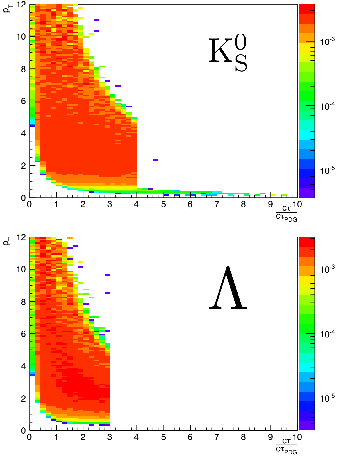
Figure 4.22: Efficiency for Reconstructing a K_S^0 or \Lambda with a Given c\tau and p_T . - 2D efficiency in c\tau and p_T for K_S^0 (top) or \Lambda (bottom) in \sqrt{s} = 2.76 TeV pp collisions. The large empty region to the right of each plot is due to the lifetime cut, and that in the bottom left is due to the decay length cut.
