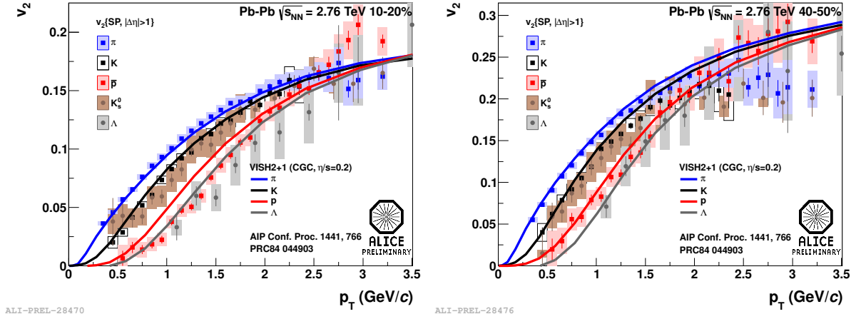
Figure 2.6: \nu_2 Measured in ALICE - Elliptic flow as measured by ALICE for various particle species, along with model predictions [97].
