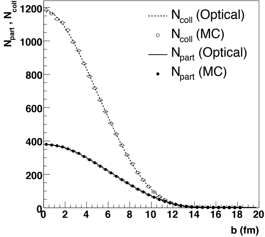
Figure 2.4: Glauber Model Predictions - Glauber model predictions for the number of participants N_{\text{part}} and binary collisions N_{\text{coll}} in Au–Au collisions against impact parameter. The optical (smooth density) approximation and Monte Carlo methods are notably similar. Calculated with \sigma_{NN}^{\text{inel}} = 42 mb, and thus d_{\text{inel}} = \sqrt{\sigma_{NN}^{\text{inel}}/\pi} = 1.2 fm [65].
