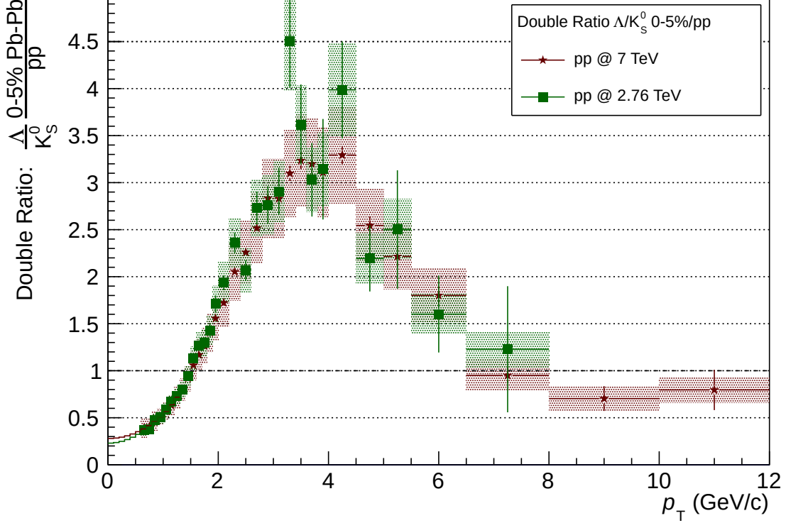
Figure 6.3: Double Ratio of \Lambda/K_S^0 (0-5% Pb-Pb)/(pp) - The \Lambda/K_S^0 ratio in 0-5% Pb-Pb collisions is divided by that measured in pp at \sqrt{s} = 2.76 TeV and 7 TeV. Statistical uncertainties are indicated by the error bars and systematic uncertainties by the shaded areas. Both a suppression region at low p_T and an enhancement region at intermediate p_T can be clearly resolved.
