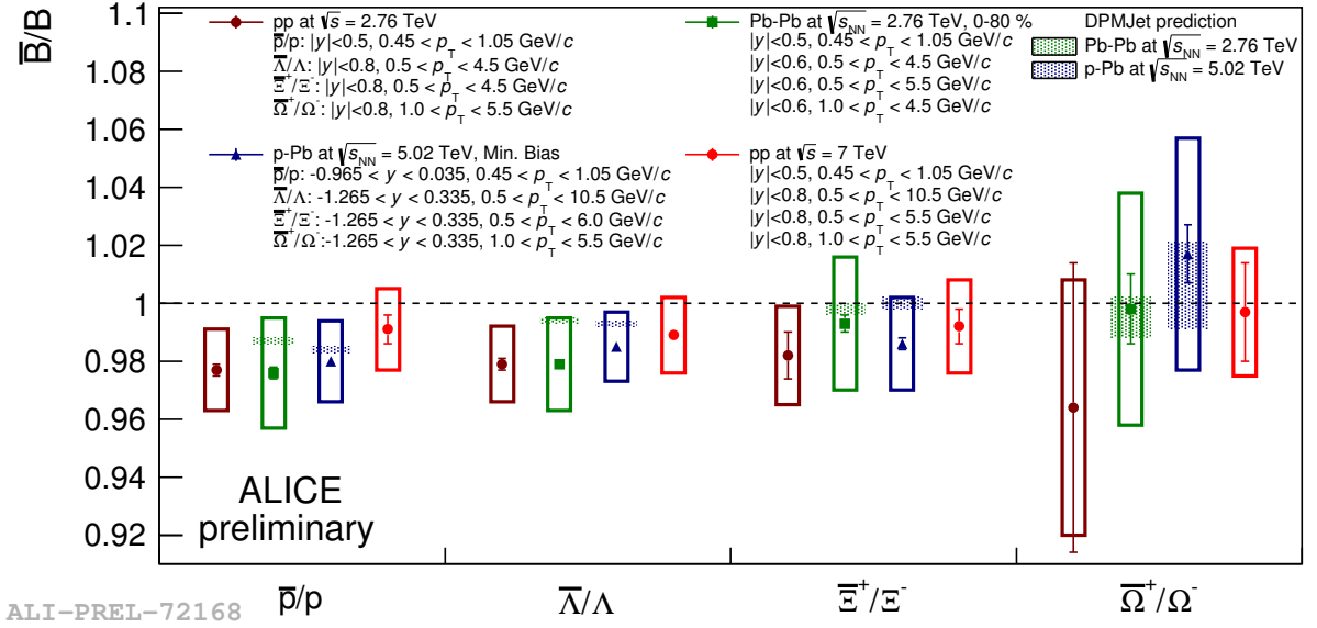
Figure 1.9: Antibaryon to Baryon Ratios at ALICE - Midrapidity antibaryon to baryon ratios as measured in pp, p-Pb and Pb-Pb collisions with ALICE at the LHC [48, 49]
