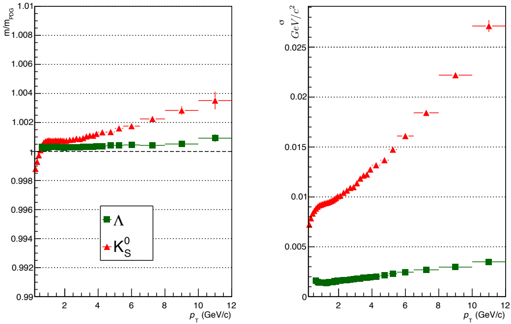
Figure 4.16: Mass and Peak Width from Fitting the Invariant Mass Distributions - Results for the peak centre, m , normalised to PDG mass, and peak width, \sigma , of the Gaussian fit to the invariant mass distribution in Pb–Pb collisions for 0–90% centrality.
