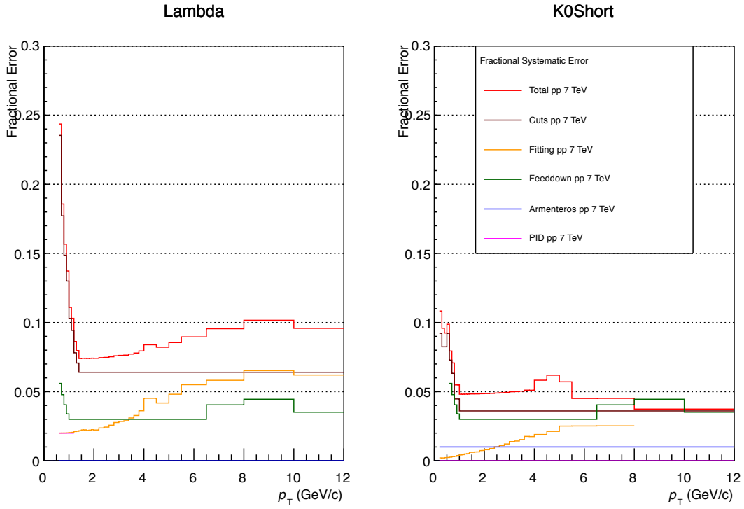
Figure 4.29: Systematic Errors for pp Collisions at \sqrt{s} = 7 TeV - Breakdown of sources of systematic error for pp collisions at \sqrt{s} = 7 TeV.
