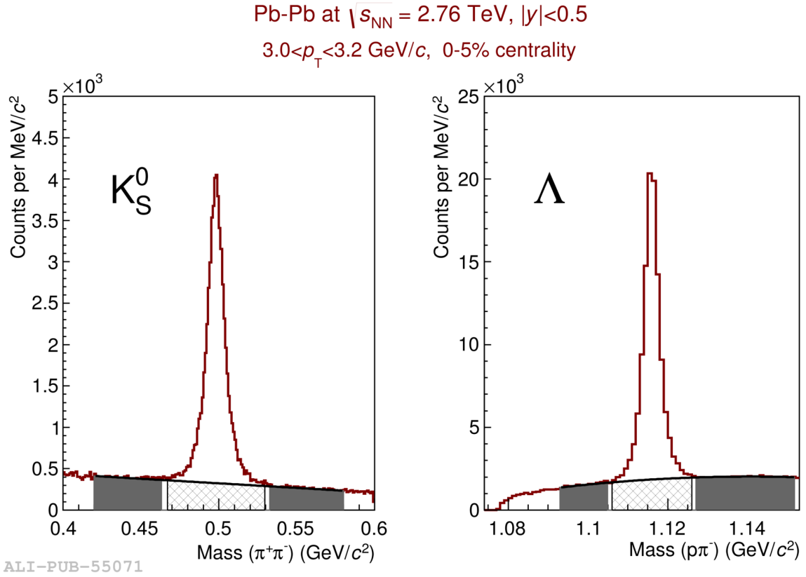
Figure 4.15: \Lambda and K_S^0 Candidates' Invariant Mass - Distribution of invariant mass for \Lambda and K_S^0 candidates from Pb-Pb collisions in 0-5% centrality interval, 3.0 < p_T < 3.2 GeV/c. The region fitted for the background is shaded in grey, and the extrapolated region subtracted from the peak indicated by crosshatching [1].
