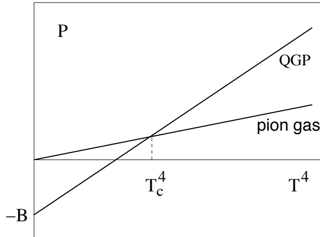
Figure 1.4: Pressure of the Hadron Gas and Quark-Gluon Plasma - Schematic of the pressure-temperature relationship for the Hadronic Gas and Quark-Gluon Plasma phase, using the MIT bag model. [18]
