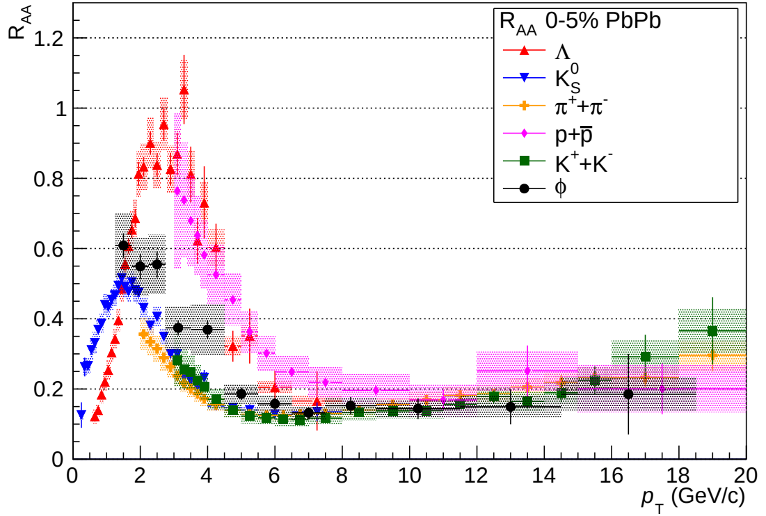
Figure 5.14: R_{AA} of Identified Particles with ALICE - R_{AA} of \Lambda and K_S^0 for the 0-5% centrality bin, with the published ALICE results for the R_{AA} of protons, charged pions and charged kaons [160]. Also shown are results for the phi meson from the Quark Matter 2014 Conference [163]. Statistical errors are indicated by the lines, while systematic errors are represented by the hatched areas.
