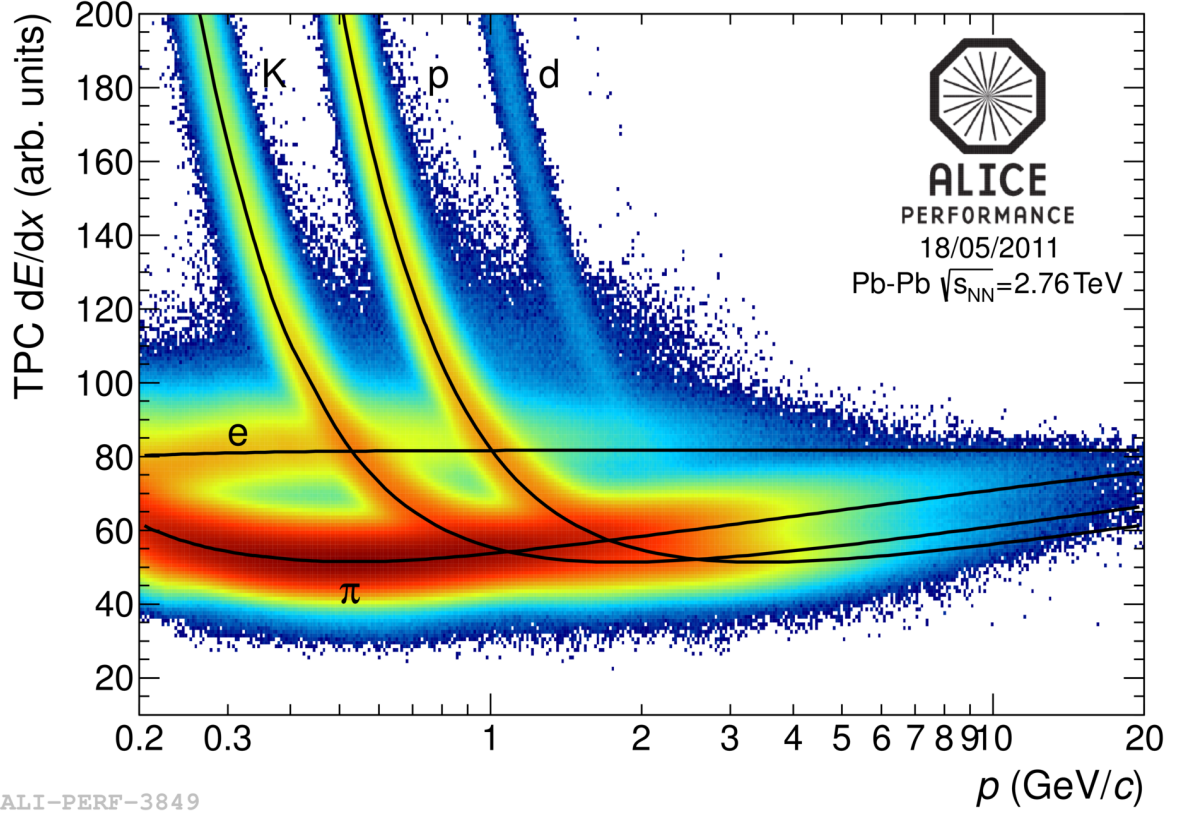
Figure 3.4: Energy Loss in the TPC - Energy Loss vs Momentum as measured in the ALICE TPC in Pb-Pb collisions at \sqrt{s_{NN}} = 2.76 TeV [147].
