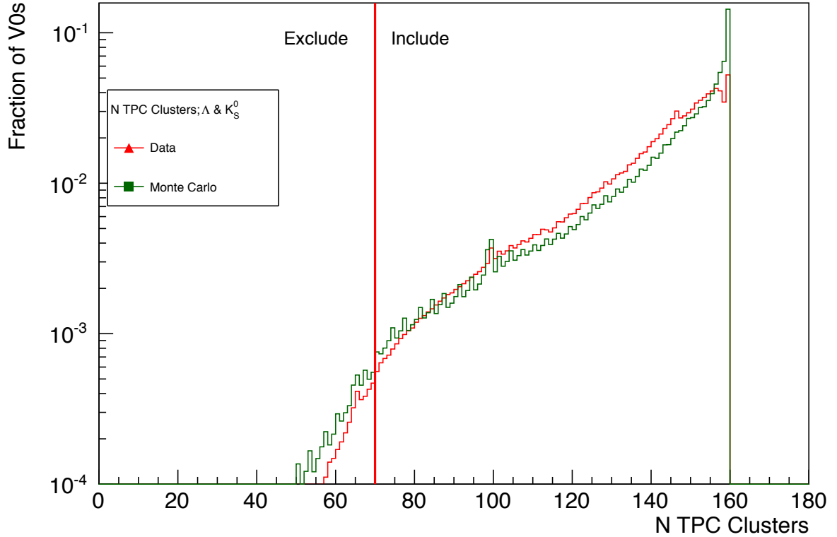
Figure 4.7: Estimated Distribution of K_S^0 and \Lambda with Number of TPC Clusters in Pb-Pb - Comparison of Monte Carlo and Data distributions of \Lambda and K_S^0 with the number of TPC clusters per daughter track. Sideband subtraction is used to estimate distributions.
