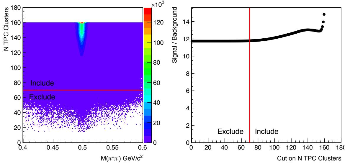
Figure 4.6: Distribution of K_S^0 with Number of TPC Clusters in Pb-Pb - Left: invariant mass of K_S^0 candidates against number of TPC clusters. Right: estimated signal to background ratio of K_S^0 candidates as a function of the TPC cluster cut chosen.
