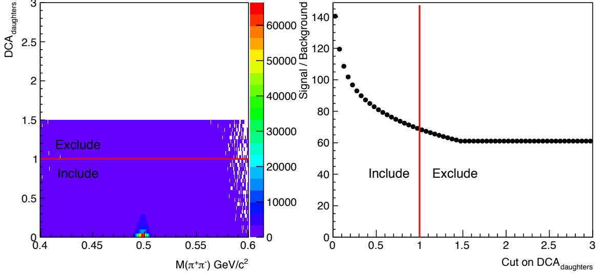
Figure 4.5: Distribution of K_S^0 with DCA between Daughters in 7 TeV pp - Left: invariant mass of K_S^0 candidates against DCA between daughter tracks. Right: estimated signal to background ratio of K_S^0 candidates as a function of the DCA between daughters cut chosen.
