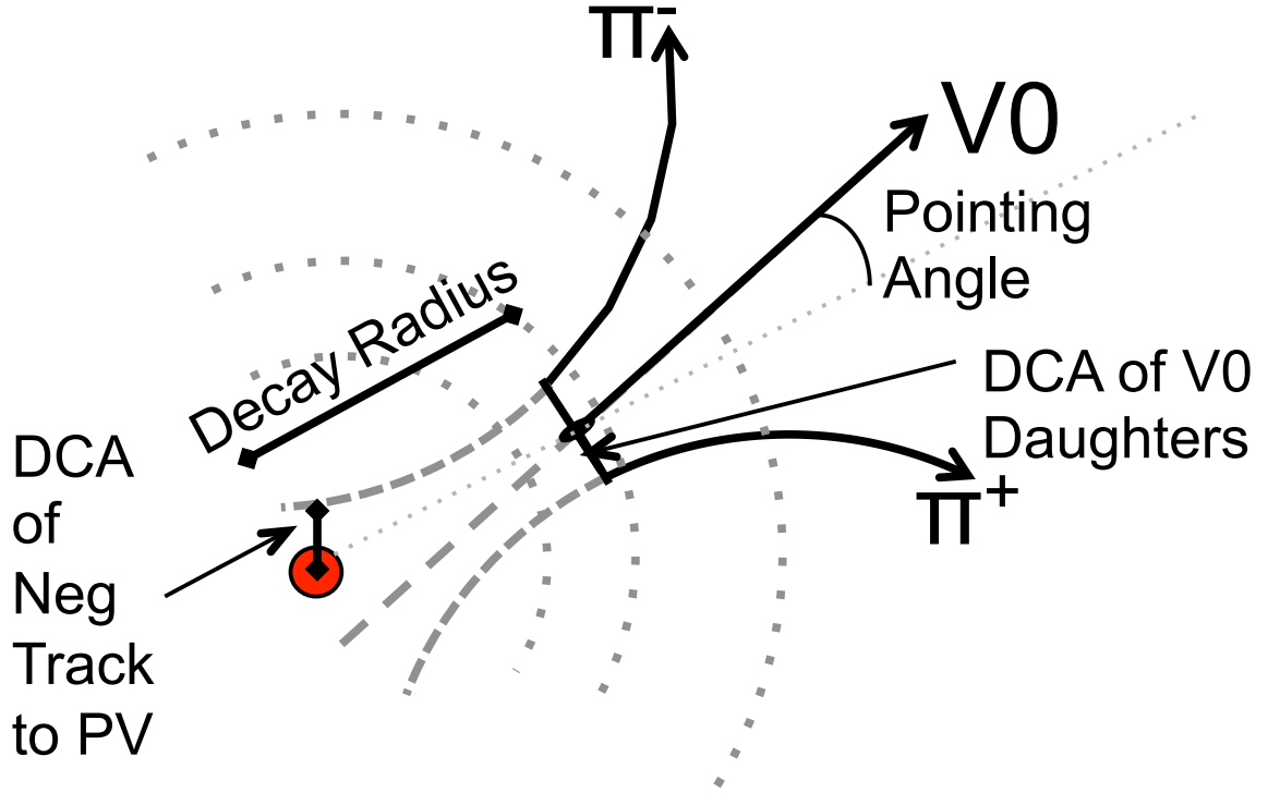
Figure 4.2: Kinematic Cuts - Schematic indicating some kinematic cut variables.
