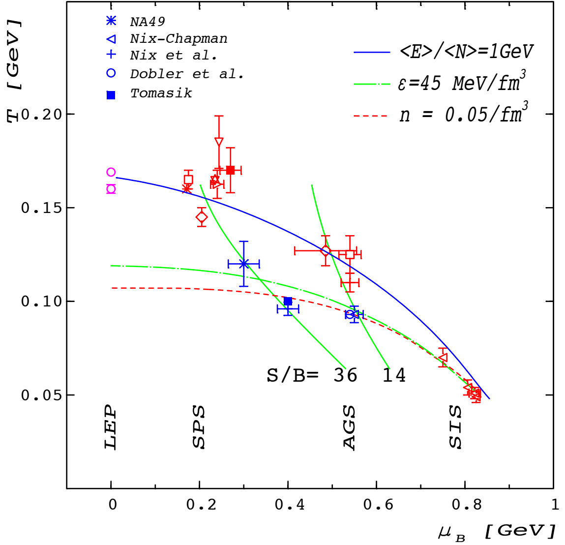
Figure 2.2: Chemical and Kinetic Freezeout Measurements - Chemical and Kinetic Freezeout calculations from SPS and AGS data. The upper red points, and solid fit line indicated chemical freezeout measurements. The lower blue points and dotted lines indicate kinetic freezeout. [64]
