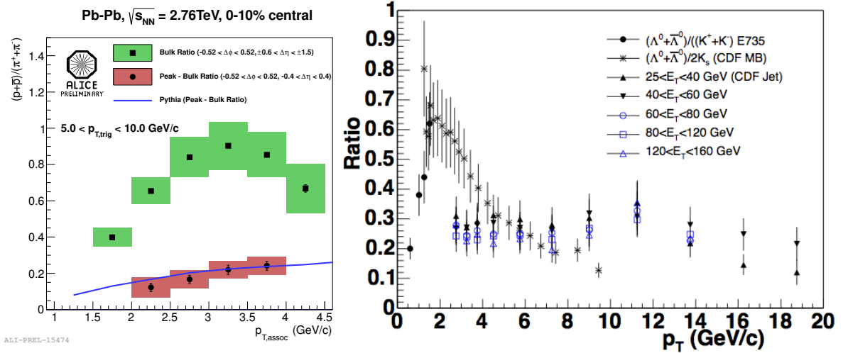
Figure 6.5: Baryon to Meson Ratios Measured in Jet and Bulk - Left: preliminary ALICE results for the p/\pi ratio measured in the bulk region, and in the jet region with bulk values subtracted. Events require a trigger particle with 5 < p_T < 10 GeV/c. Also shown is a comparison to Pythia predictions for the peak-bulk ratio. Right: inclusive \Lambda/K ratios measured by CDF and E735 in p\bar{p} collisions at the Tevatron, compared to values measured in jets at CDF [168].
