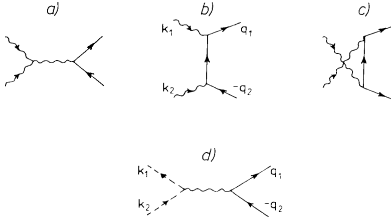
Figure 1.7: Lowest Order QCD Diagrams for s\bar{s} Production - Feynman diagrams for (a-c) gg \rightarrow s\bar{s} and (d) q\bar{q} \rightarrow s\bar{s} [24].
