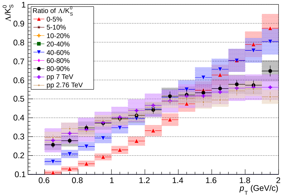
Figure 5.6: \Lambda/K_S^0 Ratio at Low p_T - The low p_T portion of the \Lambda/K_S^0 ratio for Pb-Pb and pp collisions. Only selected centralities shown for clarity.
