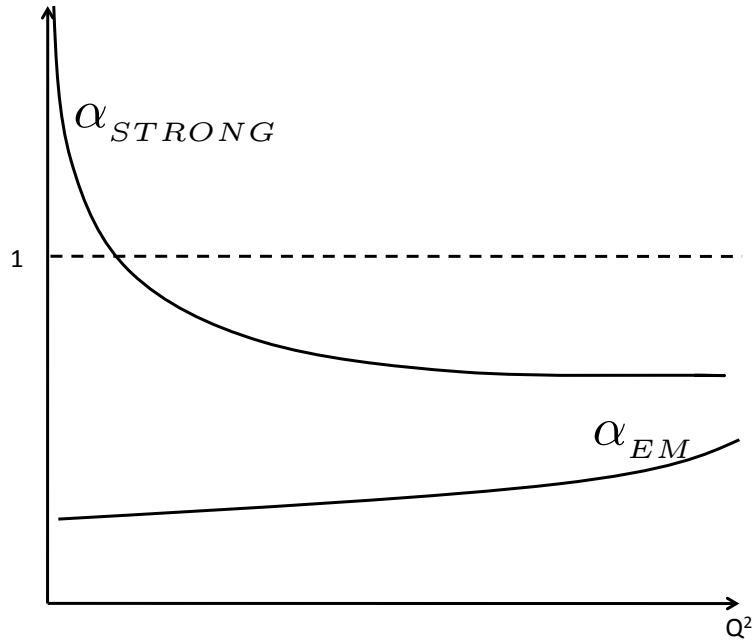
Figure 1.3: Coupling Strength of QCD and QED - Strength of QCD and QED coupling against four-momentum transfer Q^2 . Large four-momentum transfer corresponds to high collision energies or short distance scales.
