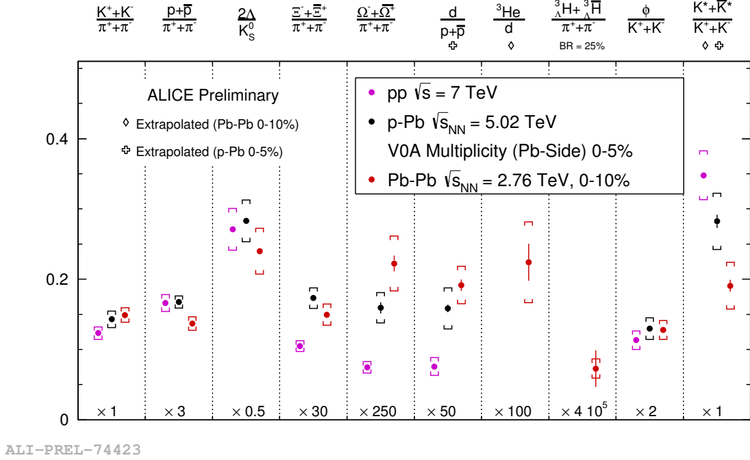
Figure 6.2: Integrated Particle Ratios with ALICE at the LHC - Particle ratios in central p-Pb and Pb-Pb, and all pp collisions. The ratios of protons, \Lambda and \Xi^- to pions show hints of baryon suppression in Pb-Pb collisions [52]. Scale factors, displayed along the bottom axis, are applied to allow comparison of ratios on a common vertical axis.
