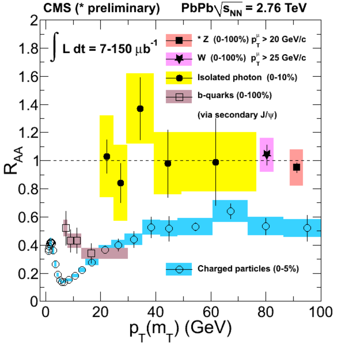
Figure 2.7: R_{AA} as Measured in CMS - R_{AA} of charged particles in central collisions at CMS along with electroweak probes. [31]
