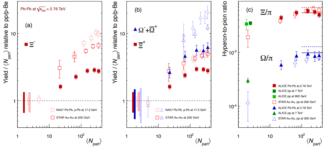
Figure 1.10: Enhancement of Strange Nucleon Production in ALICE - a,b: Relative yield of (multi)-strange baryons in heavy ion collisions, normalised to baseline pp/p-Be collisions and number of participant nucleons. c: ratio of multistrange baryons to pions for A-A and pp collisions at LHC and RHIC energies. Lines indicate thermal model predictions. [50]
