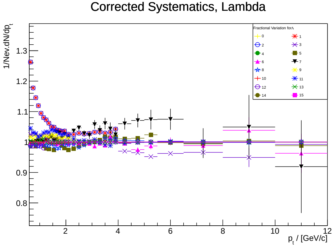
Figure 4.27: Cut Systematics for \sqrt{s} = 7 TeV pp - Variation in corrected yield for different cut combinations. See Table 4.3 for legend key.
