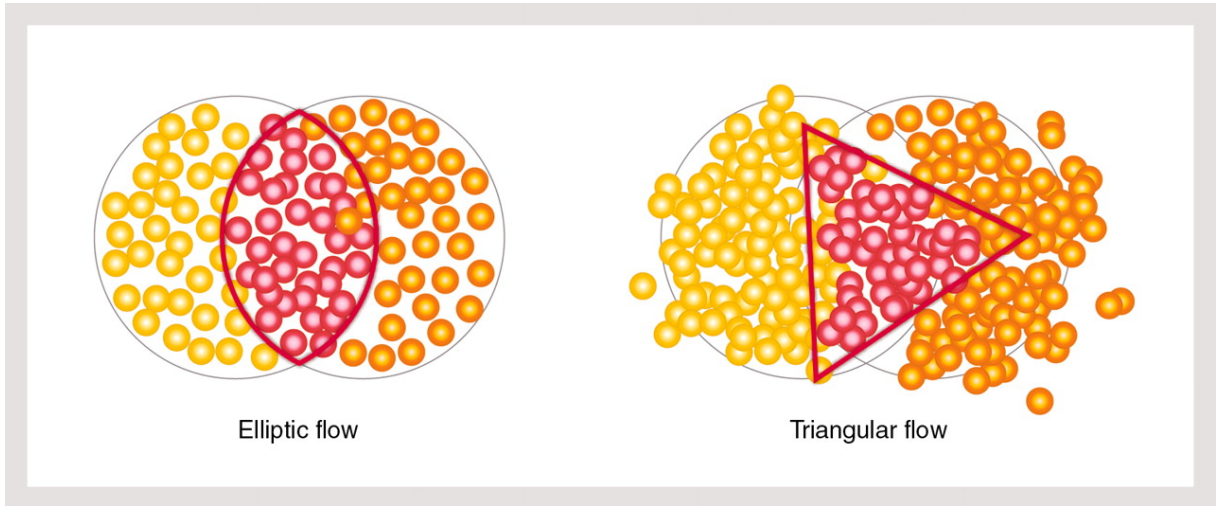
Figure 2.5: Elliptic And Triangular Flow - Schematic of the profile of colliding nuclei, indicating the prevalent flow distribution [87].
