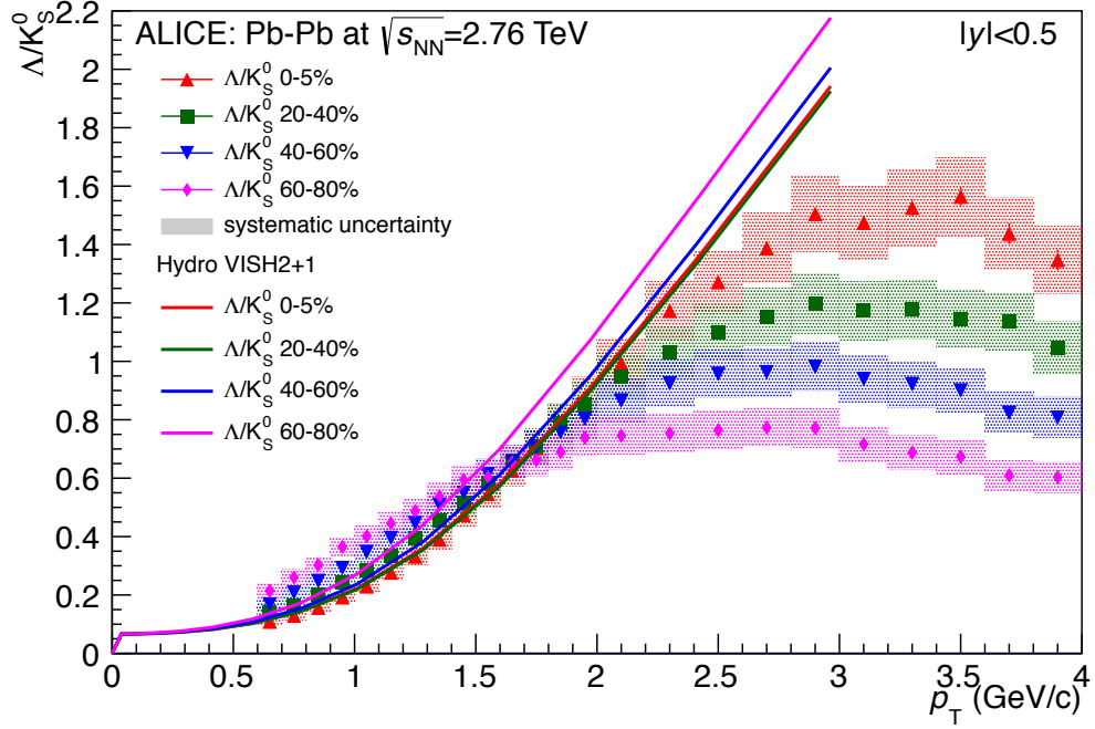
Figure 5.8: \Lambda/K_S^0 Ratio Compared with Hydrodynamical Model - The \Lambda/K_S^0 ratio for selected centralities, as compared to the predictions from the VISH2+1 model for matching centralities.
