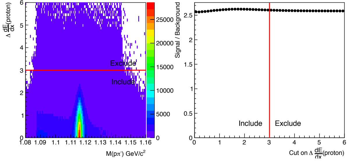
Figure 4.9: Distribution of \Lambda with TPC PID in Pb-Pb - Left: invariant mass of \Lambda candidates against N\sigma deviation of the positive daughter from the ideal proton dE/dx signal in the TPC. Right: estimated signal to background ratio of \Lambda candidates as a function of the PID cut chosen.
