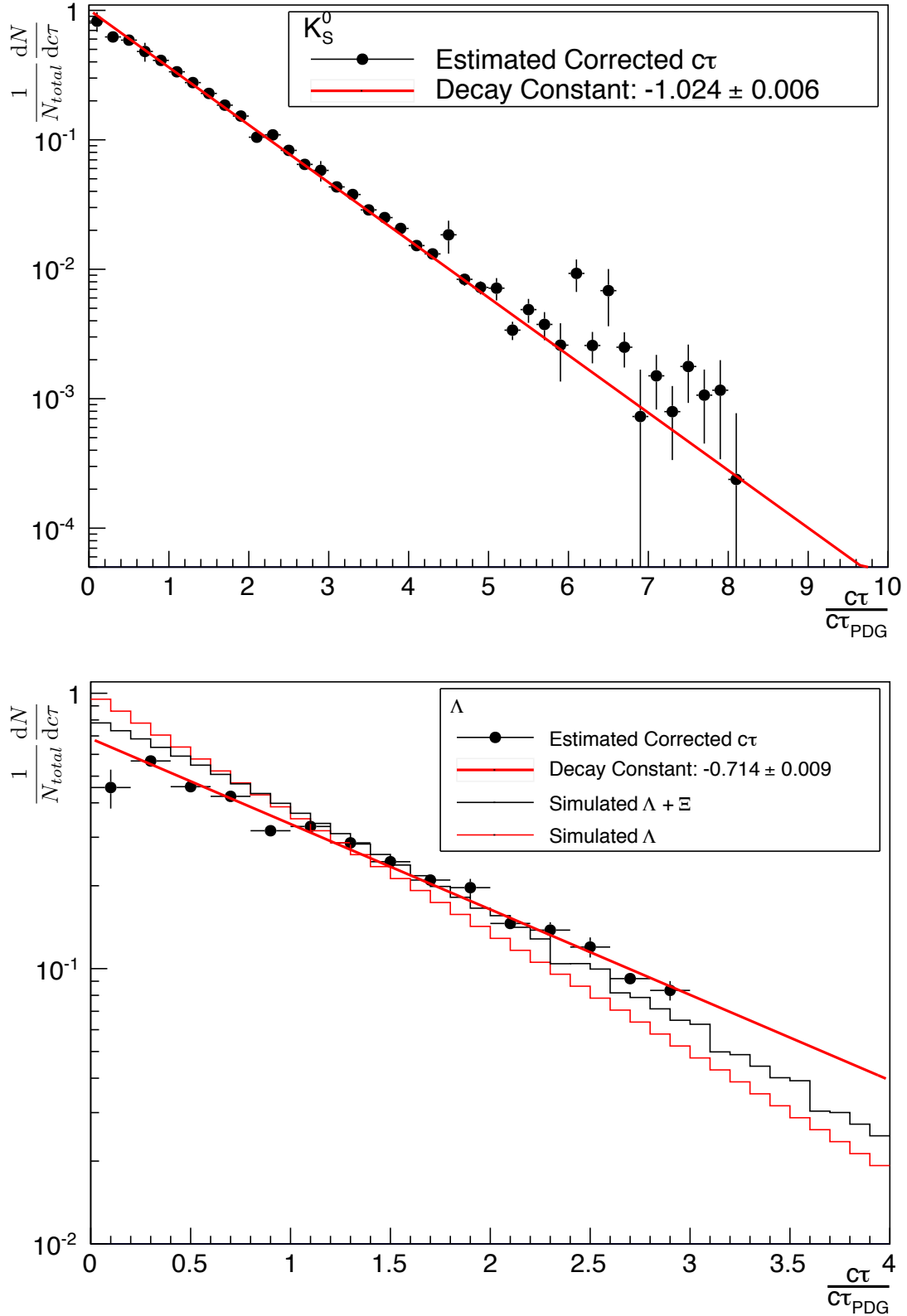
Figure 4.24: Corrected c\tau Distribution for K_S^0 or \Lambda in \sqrt{s} = 2.76 TeV pp collisions - An estimate of the corrected c\tau distribution for K_S^0 (top) or \Lambda (bottom). The red line is an exponential fit to the data points. \Lambda is not feeddown corrected, but does show simulations for a pure \Lambda distribution and a feeddown contaminated \Lambda distribution.
