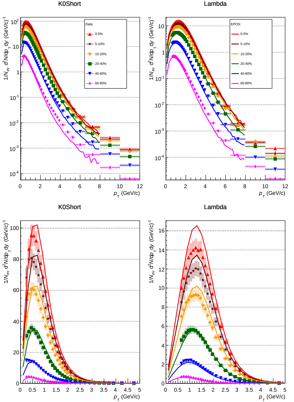
Figure 5.4: \Lambda and K_S^0 Spectra Compared to EPOS 2.17v3 Model - The fully corrected spectra of K_S^0 (left) and \Lambda (right), shown in log scale (top) and linear scale (bottom) compared to the EPOS model.
