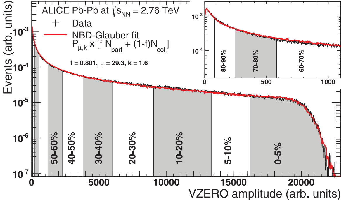
Figure 3.5: Centrality Bins in ALICE - Charged particle multiplicity as measured with the VZERO scintillators in ALICE, compared with a Glauber Model fit [4].
