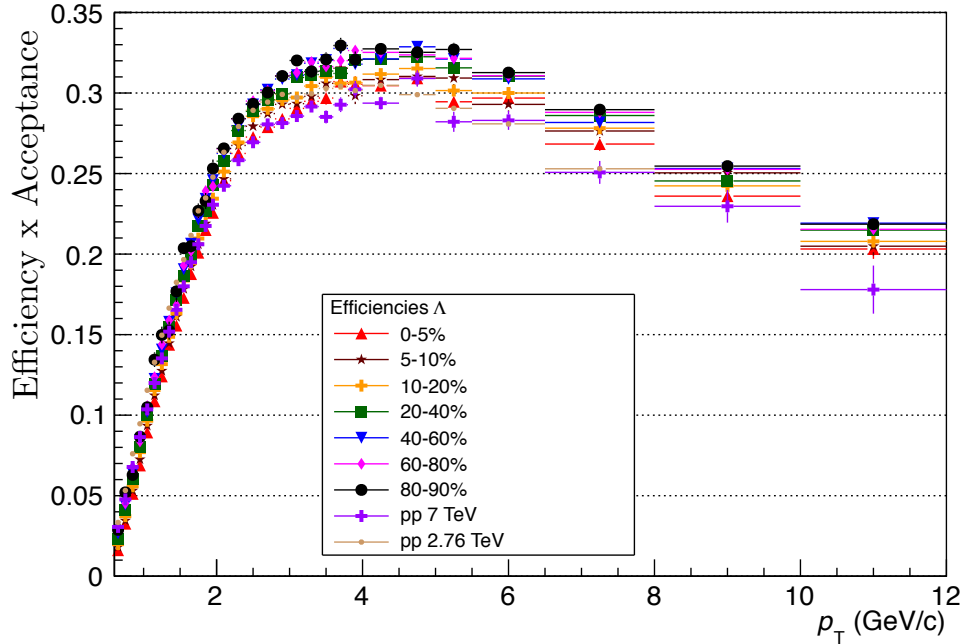
Figure 4.18: \Lambda Efficiencies - Efficiency and Acceptance for reconstructing a \Lambda in this analysis. Markers indicate different centrality bins and colliding systems, as detailed in the legend.
