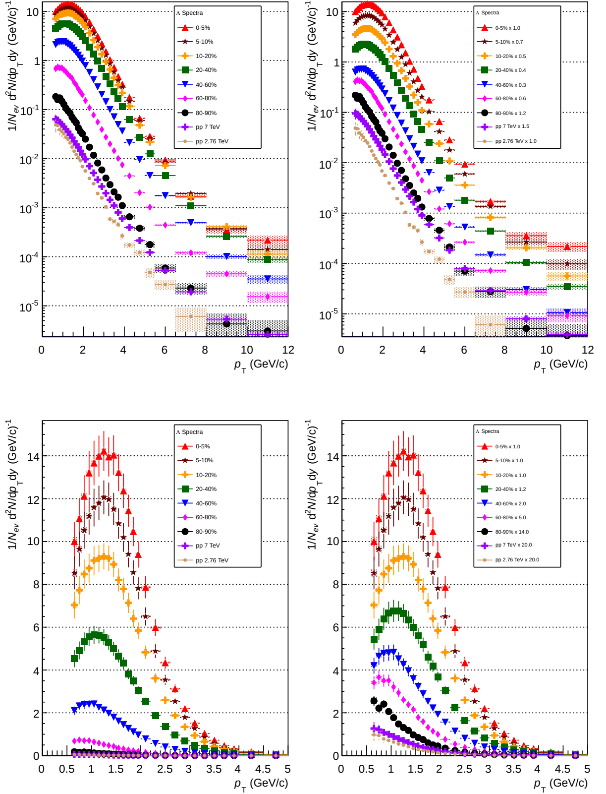
Figure 5.2: \Lambda Spectra - The fully corrected spectra of \Lambda , shown in log scale (top) and linear scale (bottom). The right hand plots have a scaling factor applied, to more clearly separate the spectra while leaving the centrality ordering unchanged.
