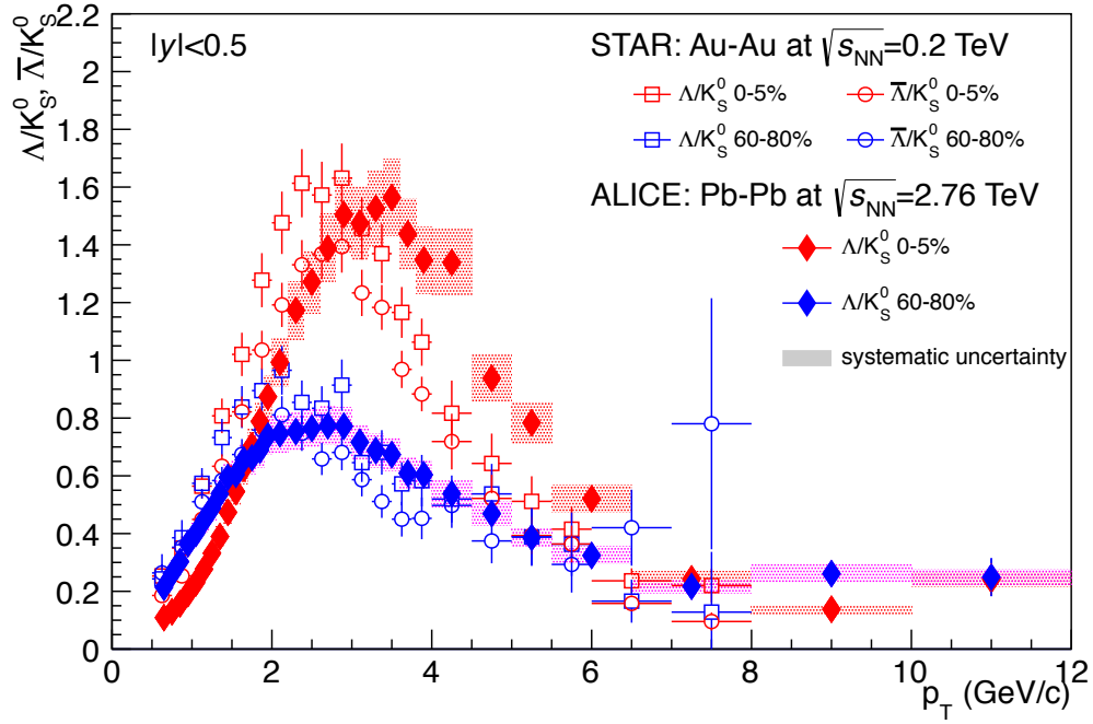
Figure 5.10: \Lambda/K_S^0 Ratio Compared with STAR - \Lambda/K_S^0 measured in this analysis compared with similar ratios measured at STAR [161].
