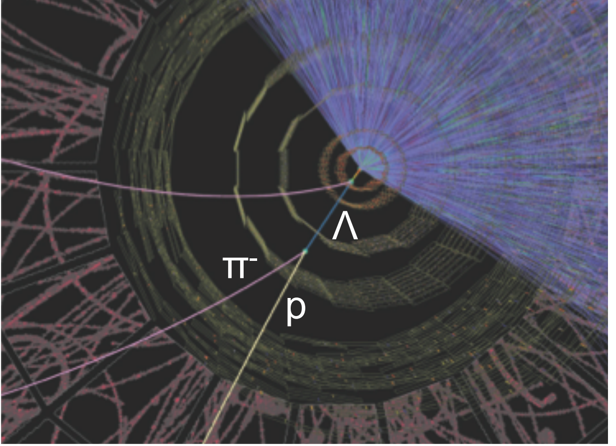
Figure 4.1: Simulated \Lambda decay in ALICE - Example of a \Lambda decay from Pb–Pb 5.5 TeV Hijing MC Event. For clarity, not all tracks are shown. [131]
