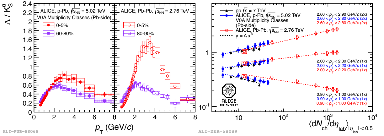
Figure 6.7: \Lambda/K_S^0 Ratio Results in pp, p-Pb and Pb-Pb Collisions - Left: the \Lambda/K_S^0 ratio in central and peripheral collisions in p-Pb, \sqrt{s_{NN}} = 5.02 TeV, and Pb-Pb collisions at \sqrt{s_{NN}} = 2.76 TeV. Right: value of the \Lambda/K_S^0 ratio at selected p_T for different colliding systems plotted against charged particle multiplicity. [171]
