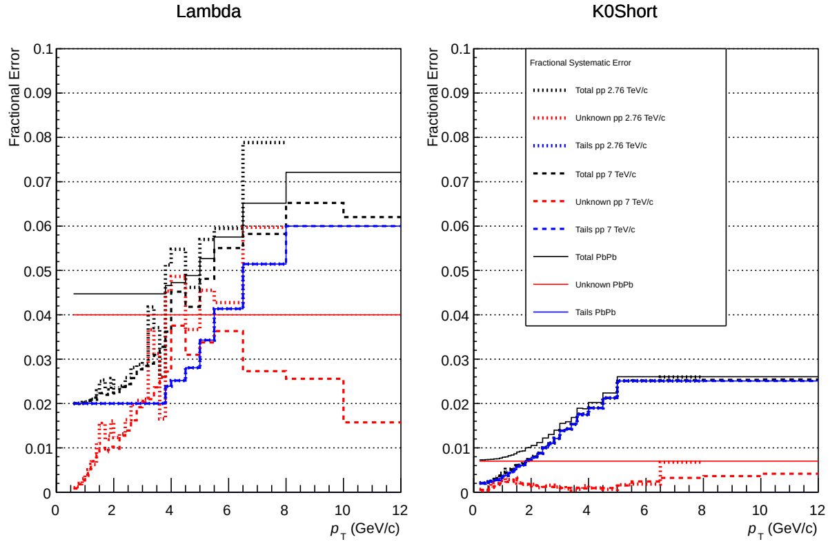
Figure 4.28: Fitting Systematics - Fractional errors associated with the fitting routine; for \Lambda on the left and K_S^0 on the right. ‘Tails’ indicates that part of the error associated with signal misidentified as background, and ‘Unknown’ all other. The ‘Total’ is the quadratic sum of the two.
