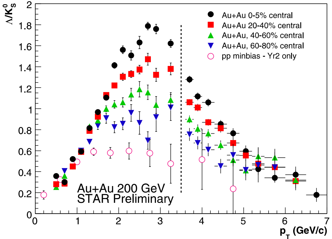
Figure 1.12: The \Lambda/K_S^0 Ratio Measured at STAR - The \Lambda/K_S^0 ratio as measured in \sqrt{s_{NN}} = 200 GeV Au–Au collisions at STAR [58]. Results to the right of the dotted line have had their statistics improved by including the 2004 Au–Au run.
