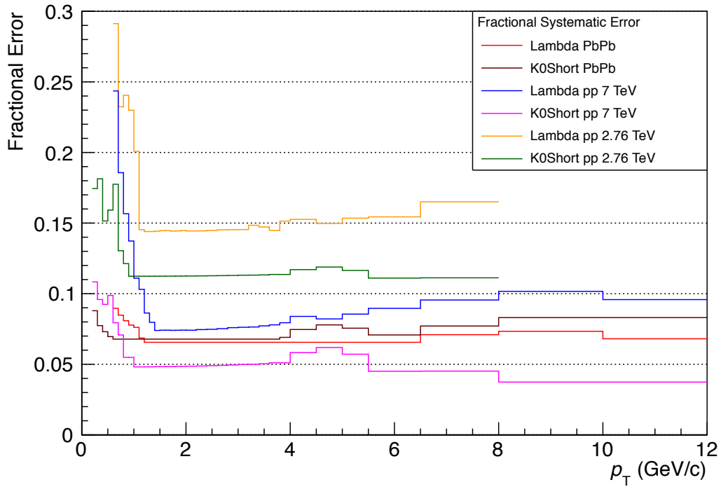
Figure 4.30: Systematic Errors - Total systematic errors for all particles and collision systems.
