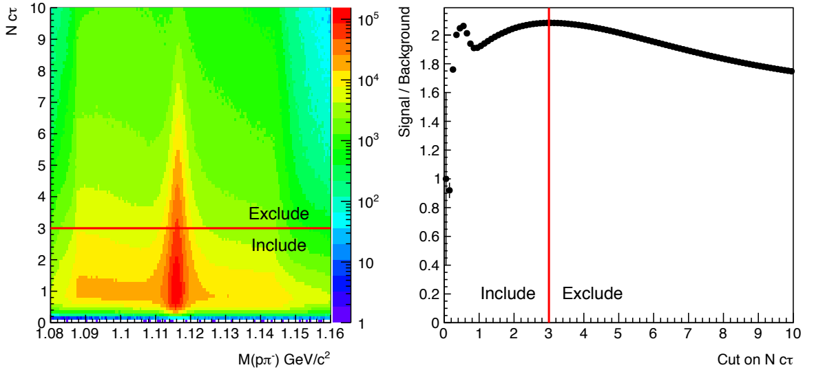
Figure 4.8: Distribution of \Lambda with Lifetime in Pb–Pb - Left: invariant mass of \Lambda candidates against lifetime as a multiple of PDG \Lambda lifetime. Right: estimated signal to background ratio of \Lambda candidates as a function of the lifetime cut chosen.
