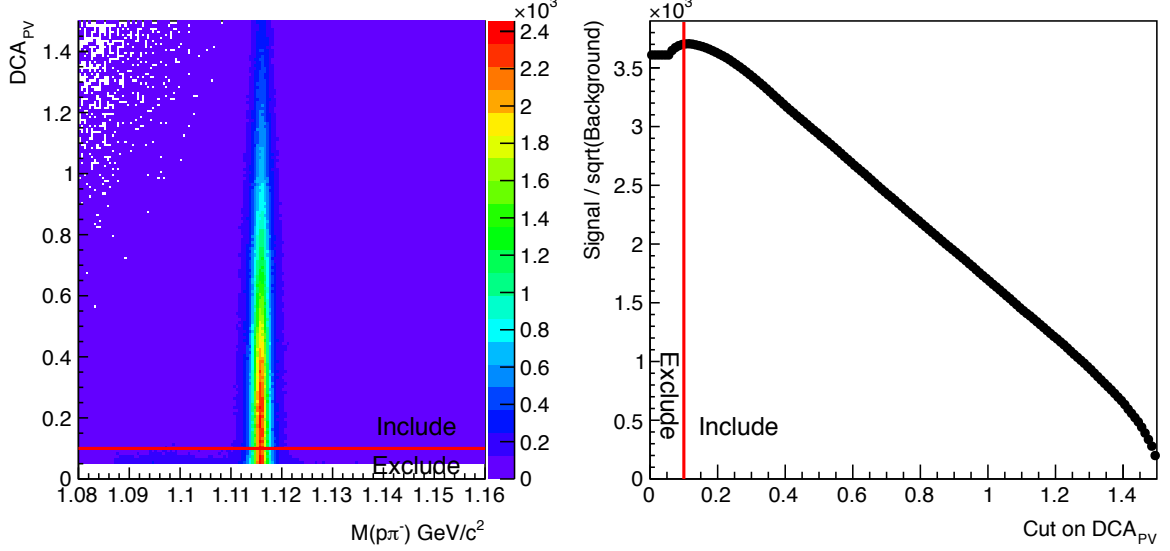
Figure 4.4: Distribution of \Lambda with DCA to Primary Vertex in 7 TeV pp - Left: invariant mass of \Lambda candidates against DCA of daughter tracks to primary vertex. Right: estimated significance of \Lambda candidates above background as a function of the DCA to primary vertex cut chosen.
