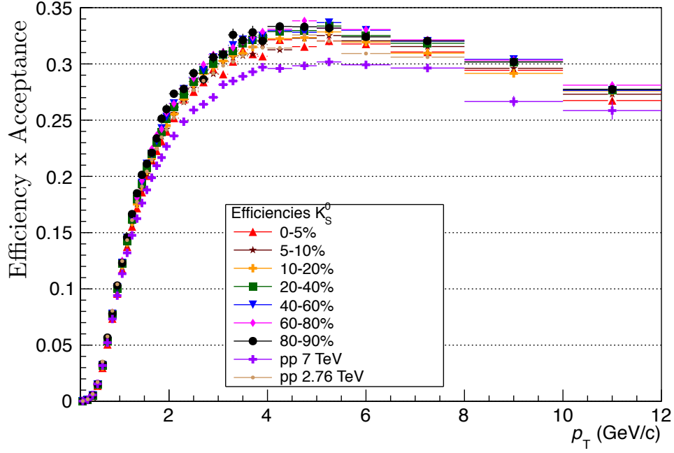
Figure 4.17: K_S^0 Efficiencies - Efficiency and Acceptance for reconstructing a K_S^0 in this analysis. Markers indicate different centrality bins and colliding systems, as detailed in the legend.
