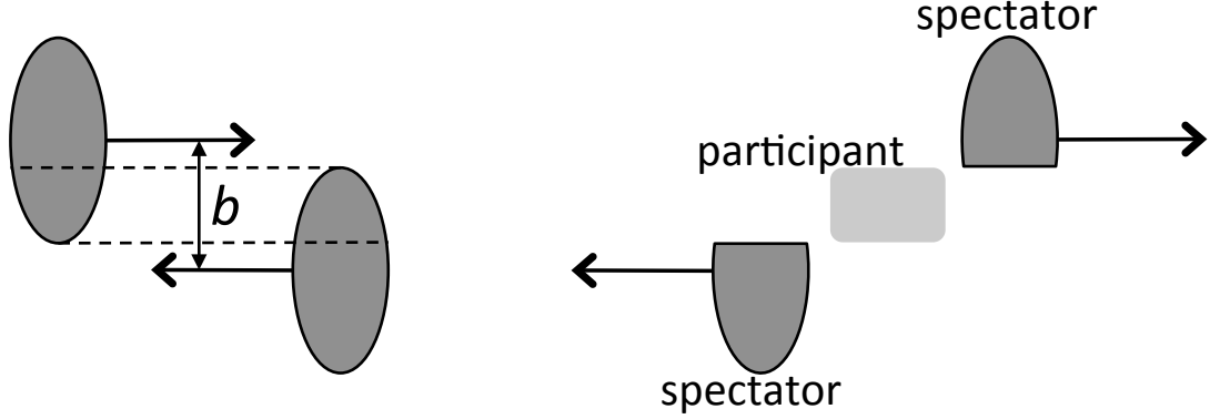
Figure 2.3: Impact Parameter of Colliding Nuclei - Geometry of colliding nuclei with impact parameter \mathbf{b} indicated on the left hand diagram. This determines the ‘participant’ and ‘spectator’ nuclei for the collision, as shown on the right hand side.
