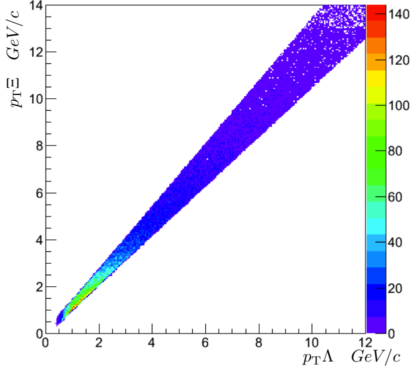
Figure 4.20: Feeddown Matrix - Matrix relating the p_T distribution of \Xi^- to the p_T distribution of their \Lambda daughters for 0-5% centrality Pb-Pb Monte Carlo simulations.
