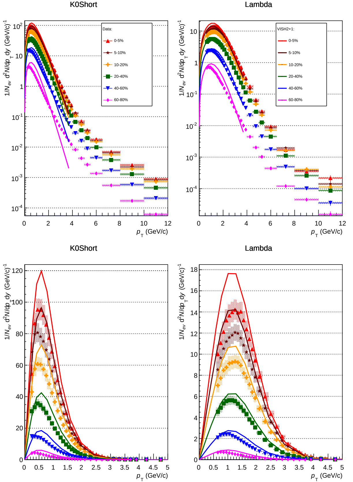
Figure 5.3: \Lambda and K_S^0 Spectra Compared to Vish2+1 Model - The fully corrected spectra of K_S^0 (left) and \Lambda (right), shown in log scale (top) and linear scale (bottom) compared to the Vish2+1 hydrodynamical model.
