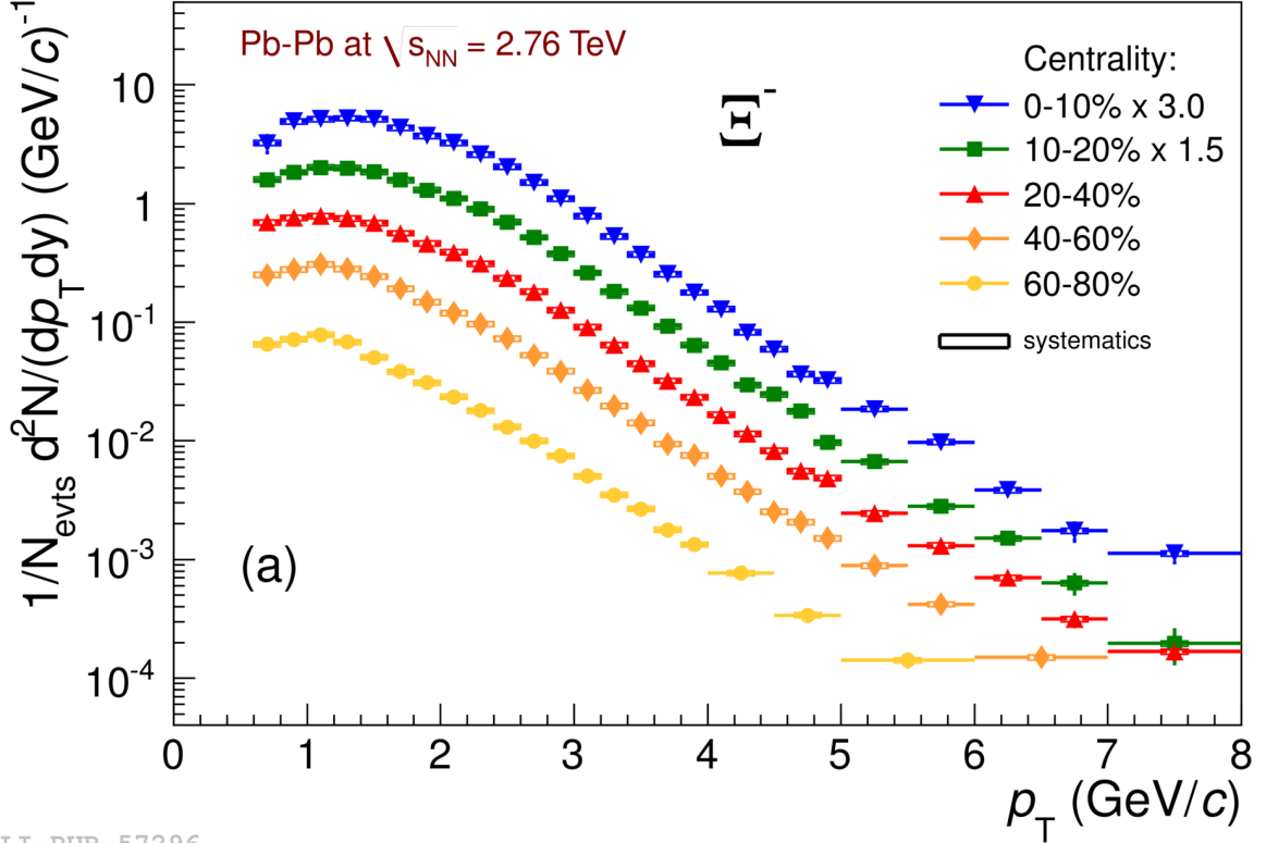
Figure 4.19: \Xi^- Spectra - p_T spectra of \Xi^- from \sqrt{s_{NN}} = 2.76 TeV Pb-Pb collisions [158].
