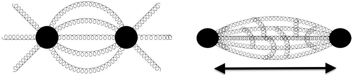
Figure 1.1: Schematic of Quark-Gluon Interactions - Schematic indicating gluon field lines as two quarks are separated.
