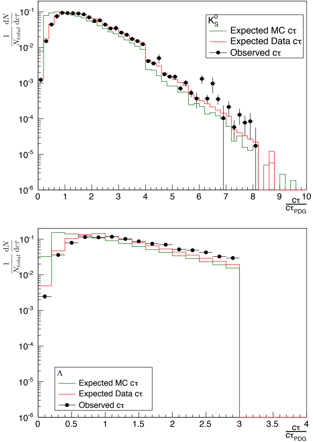
Figure 4.23: Expected Measured c\tau Distributions for K_S^0 and \Lambda in \sqrt{s} = 2.76 TeV pp Collisions - The c\tau distribution one would expect to measure for an ideal initial c\tau and a data-like (red) or Monte-Carlo-like (green) p_T distribution. The calculated efficiency has been used to convert the ideal c\tau - p_T distribution to an observed distribution. The markers show the measured c\tau distribution which is consistent with the expectation for a data-like p_T distribution. Sharp drops in the distribution are due to applied kinematic cuts. Results for K_S^0 shown in top plot, \Lambda in bottom plot. Note that \Lambda results are not feeddown corrected.
