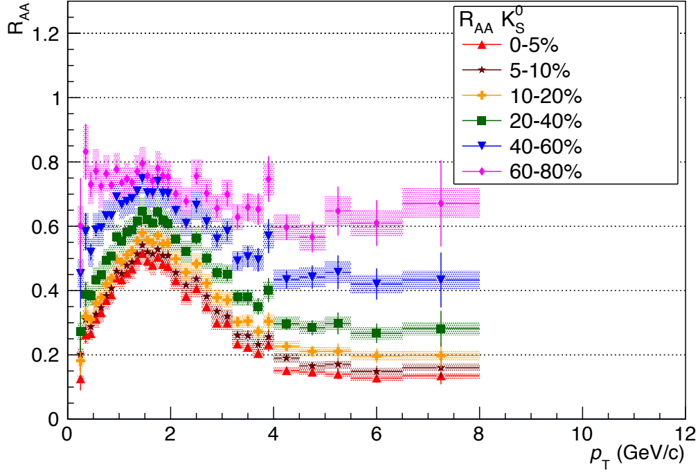
Figure 5.12: K_S^0 R_{AA} - R_{AA} of K_S^0 for all measured centrality bins. Statistical errors are indicated by the lines, while systematic errors are represented by the hatched areas.
