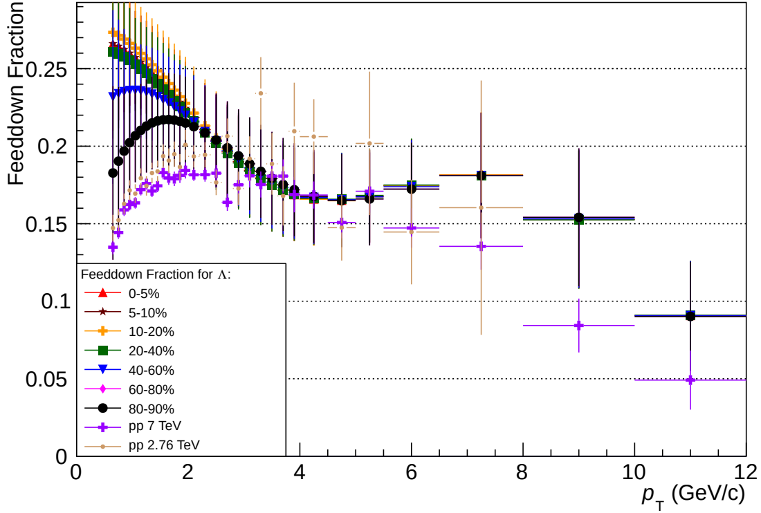
Figure 4.21: Feeddown as a Fraction of \Lambda Spectra - The estimated fraction of \Lambda entering our analysis from \Xi^- + \Xi^0 decay. Markers indicate different centralities and colliding systems.
