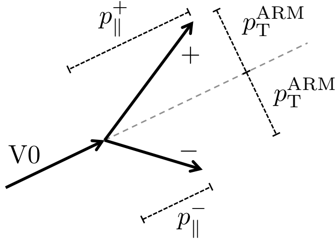
Figure 4.11: Schematic of Momentum Projections Used in Armenteros-Podolanski Diagram - The projection of the positive and negative daughters momentum perpendicular and parallel to the V0's momentum are indicated. The perpendicular components are equal and opposite to satisfy conservation of momentum, and the relative magnitudes of the projections are determined by the Lorentz boost of the V0 and the decay angle relative to the boost in the V0 rest frame.
