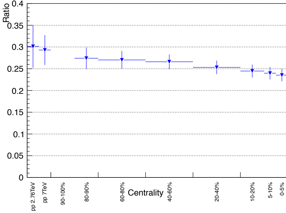
Figure 6.1: Ratio of p_T -integrated \Lambda/K_S^0 Yields. - Yields of \Lambda and K_S^0 are integrated from p_T = 0 upwards using the blastwave & Tsallis fits discussed in Section 5.6. These integrated yields are then divided to give the total \Lambda/K_S^0 ratio.
