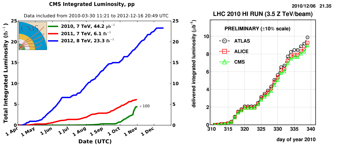
Figure 3.2: Integrated Luminosity at the LHC - Left: integrated luminosity of pp collisions as recorded by the CMS experiment at the LHC for 2010, 2011 and 2012 [138]. A considerable year-on-year increase in the integrated luminosity can be observed. Right: integrated luminosity of Pb–Pb collisions for the 2010 run studied in this work [139]. The luminosity can be seen to increase as the run continues.
