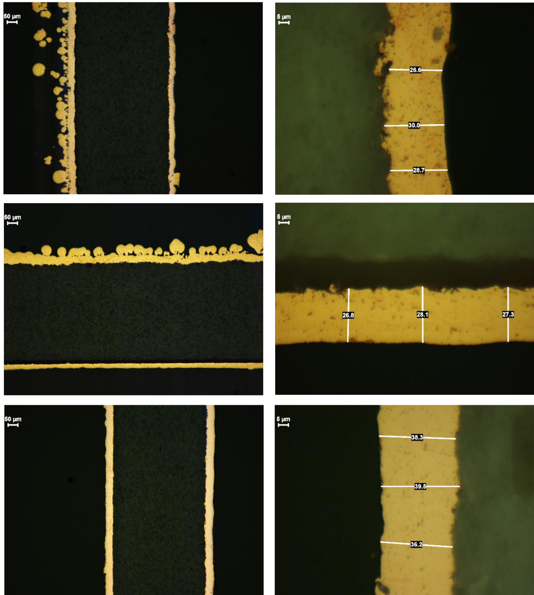
Figure 8.16: The microscope picture of a sectioned copper coated box. Uniformity of the coating is very good and the thickness is measured to be approximately 30 \mu\text{m} .
