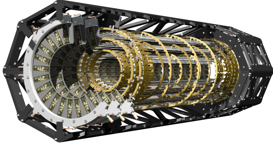
Figure 3.5: 3D model of the pixel detector consisting of barrel and end-cap layers[60].
