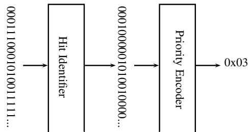
Figure 10.7: A block diagram of the Hit Locator data-flow. The data goes from left to right, the Hit Identifier reduces all clusters to a width of 1 which the priority encoder can process. The Priority encoder then reports the location of the first hit.
