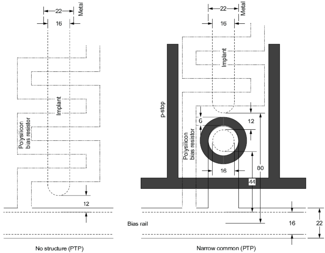
Figure 5.19: The punch through protection structure. The schematic on the right shows the bias rail extended to be around 12 \mu\text{m} away from the implant which facilitate the PTP functionality[39].
