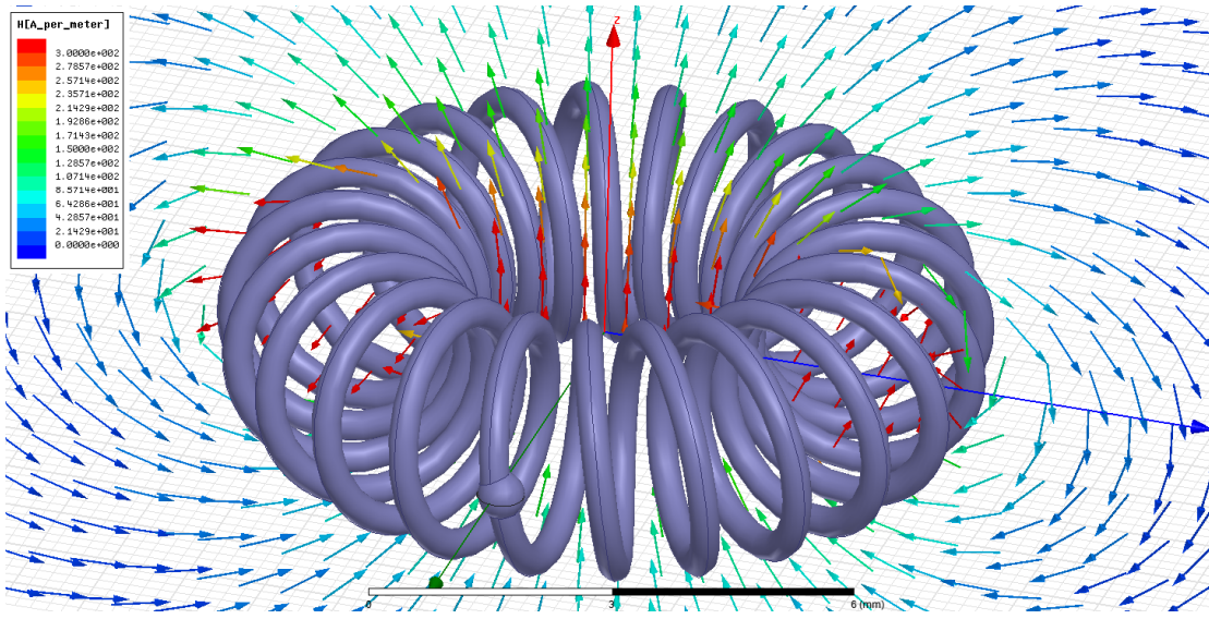
Figure 8.22: A model of a toroid coil with the simulated magnetic field.
