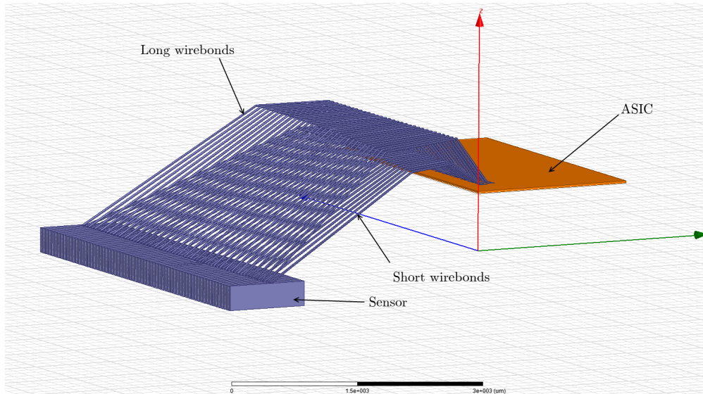
Figure 8.17: A model of the wire-bonds drawn with HFSS[45]. The wire-bond geometry is \sim 4.5 mm in length, the bond angle is \sim 12^\circ and the diameter is 25\text{ }\mu\text{m} .
