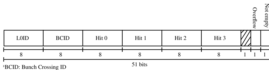
Figure 10.4: The R3 DCL packet structure.
