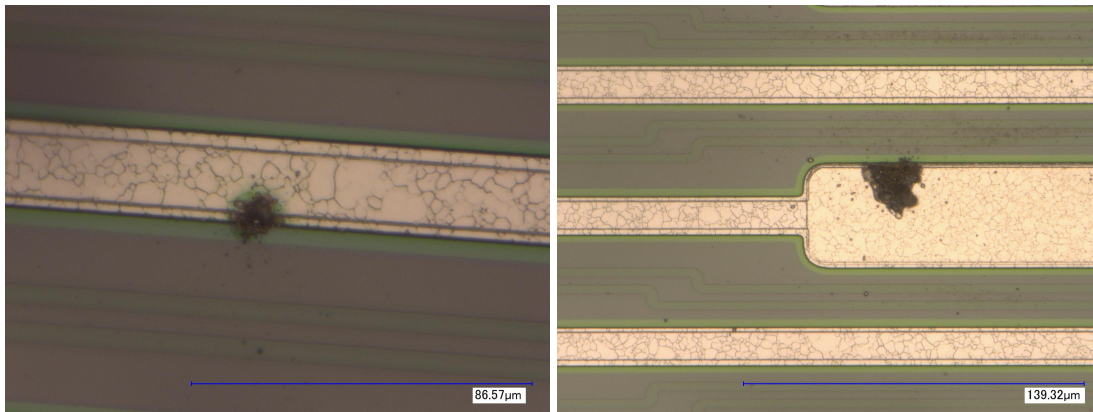
Figure 6.10: The damage on the metal strip due to a large amounts of charge injected into the sensor. Left: damage on the strip track. Right: damage on the bond pad.
