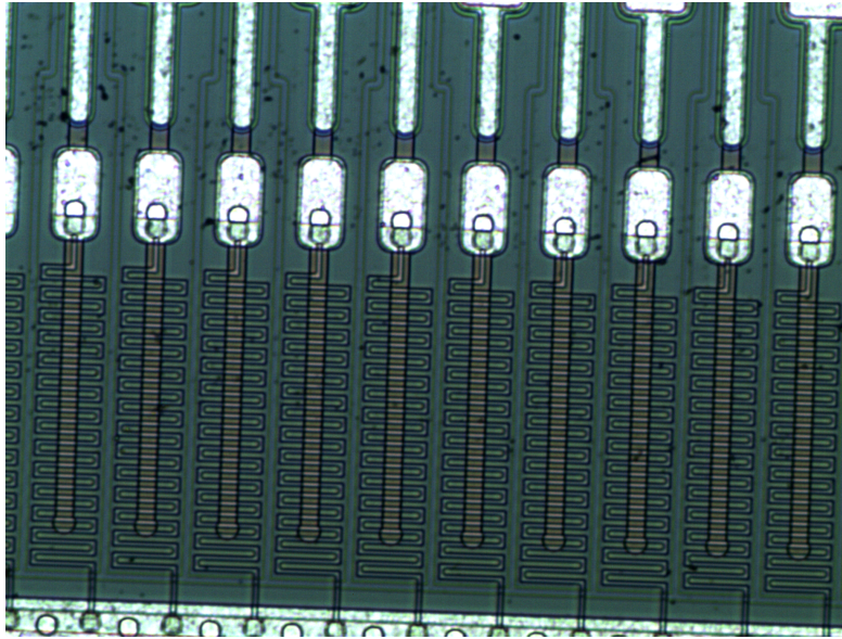
Figure 5.13: An image showing the polysilicon bias resistors connecting the implants to the bias ring.
