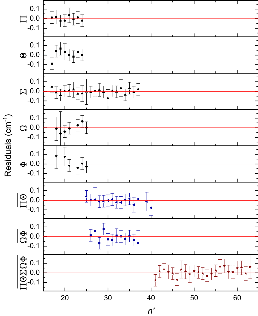
Figure 6.7: Residuals for each Rydberg series obtained by the global fit of method3: a global fit to all series for which the ionization energy with respect to the second excited state was a shared fit parameter.
