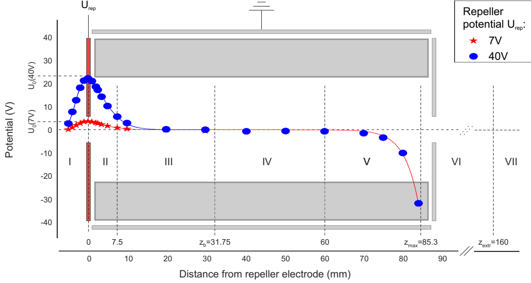
Figure 4.26: Longitudinal potential inside the LIST cavity as a function of the distance to the repeller electrode calculated by the CPO © program. Ranges on the longitudinal axis, which are discussed in the text, are indicated by the Roman numbers. The potential defined by Equation (4.6) is fitted to the simulated data
