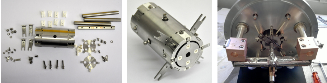
Figure 4.6: Left: Overview of the LIST1 components. Center: assembled LIST. The repeller electrode, the LIST chamber, the LIST holder and the RF-contacts are visible. Right: LIST 1 installed into an ISOLDE target.
