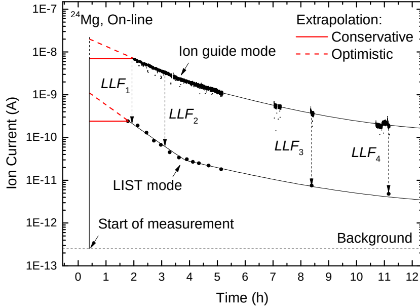
Figure 4.23: On-line measurement of the LIST1 laser ionization efficiency in ion guide mode and LIST mode using a 0.11\ \mu\text{g} sample of natural magnesium. The sample was evaporated over 12 h. Four different LIST loss factors, LLF_1 to LLF_4 , were extracted at different times of the measurement and are listed in Table 4.2.
