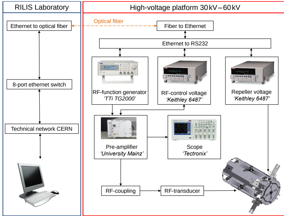
Figure 4.13: Illustration of the remote control system of the LIST. Glass fibers were passed from the RILIS laboratory to the HV-cage for remote control of the electronics. The RF-function generator, the RF-control supply and the repeller voltage supply are integrated and controlled via the technical network of CERN.
