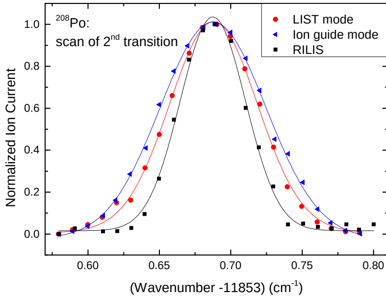
Figure 4.24: Comparison of the resonances of the second intermediate step of the polonium (Po) scheme ( 50934.89\text{ cm}^{-1} , 6p^3(^4S^\circ)7p ) obtained in LIST mode , ion guide mode and in standard RILIS mode , respectively. The transition was scanned by tuning a narrow band Ti:Sa laser across the resonance and fitted by a Voigt profile. Ion intensities were normalized for better comparison.
