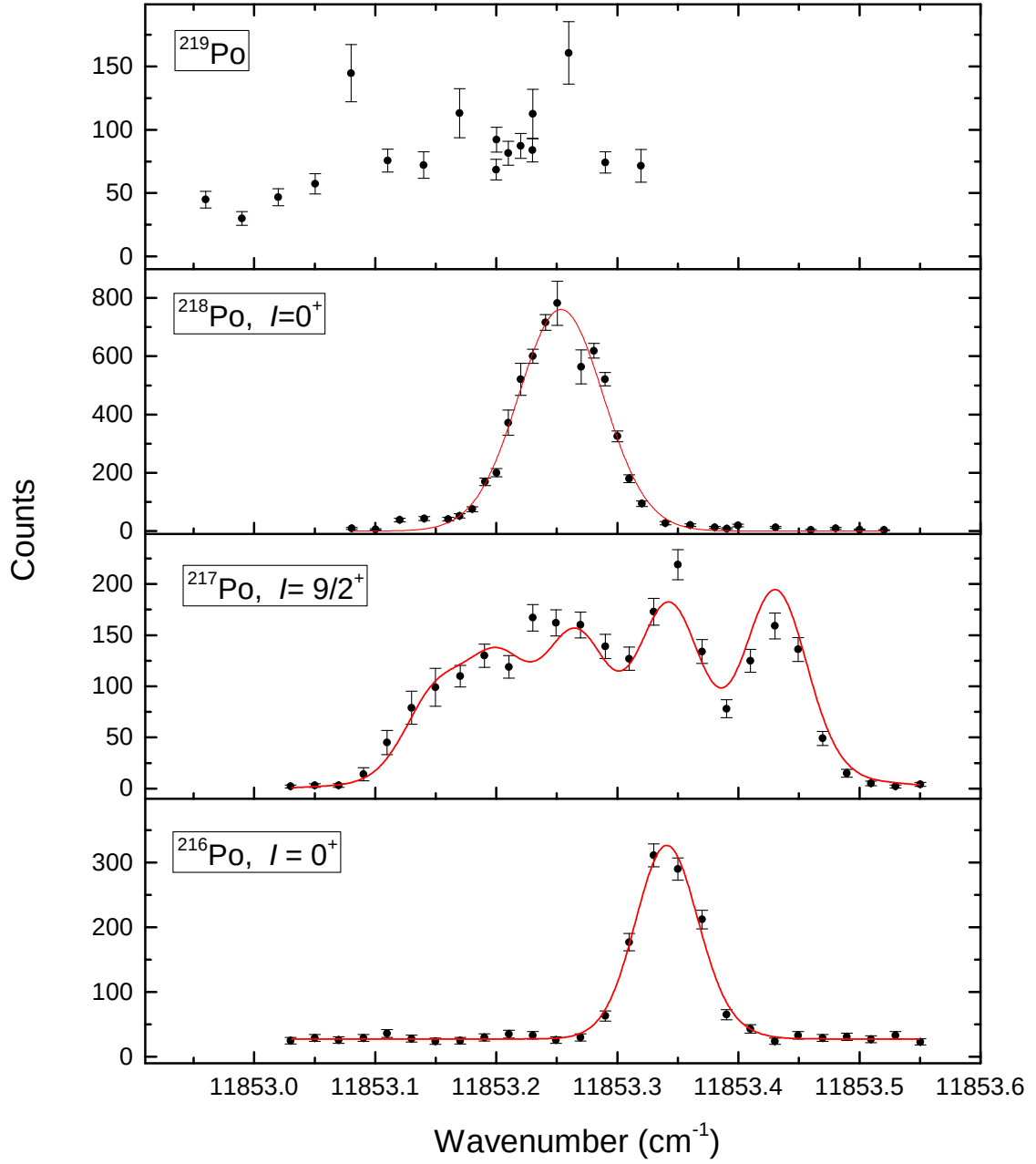
Figure 7.6: Laser spectra of the neutron-rich ^{116,117,118,119}\text{Po} isotopes. Uncertainties are given by the standard deviation. The red curves are the fits to the data [156]. The spectrum of ^{219}\text{Po} was analyzed by T.E. Cocolios [40].
