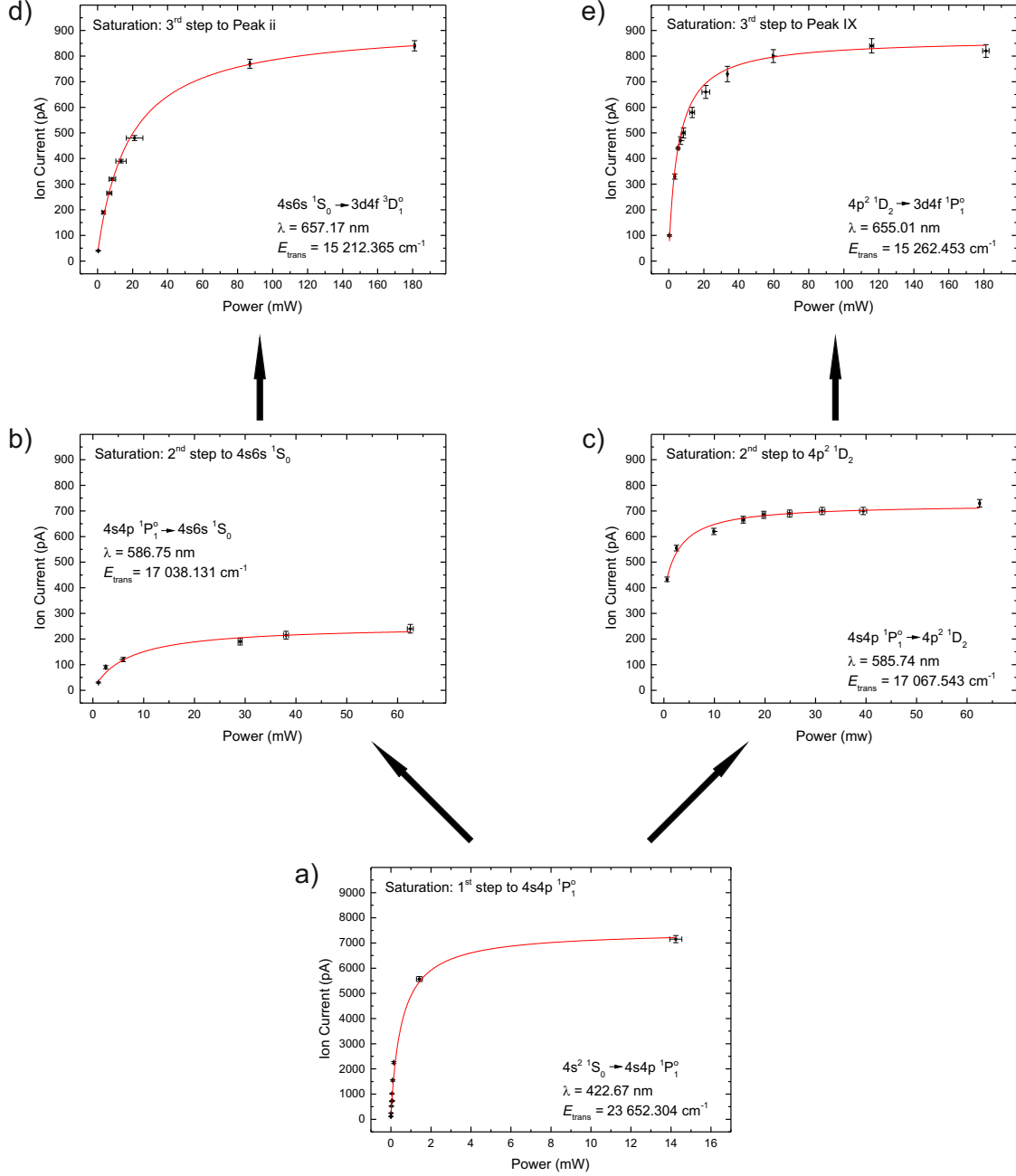
Figure 5.6: Saturation curves for the atomic transitions used in the new calcium schemes.
