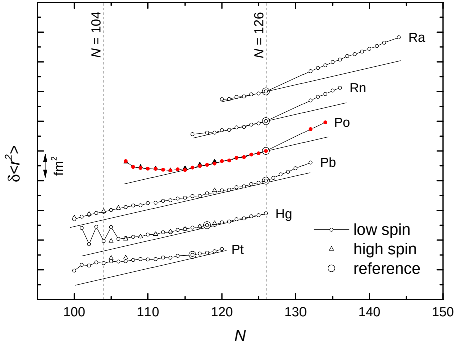
Figure 7.1: Changes in mean square radii, \delta \langle r^2 \rangle_{A,A'} , for even- Z isotopes in the lead-region ( Z = 82 ): platinum ( _{78}\text{Pt} ) [101], mercury ( _{80}\text{Hg} ) [171], lead ( _{82}\text{Pb} ) [6, 47, 50, 53], polonium ( _{84}\text{Po} ) [39, 159], radon ( _{86}\text{Rn} ) and radium ( _{88}\text{Ra} ) [64]. The reference isotopes are indicated by the large circles.
