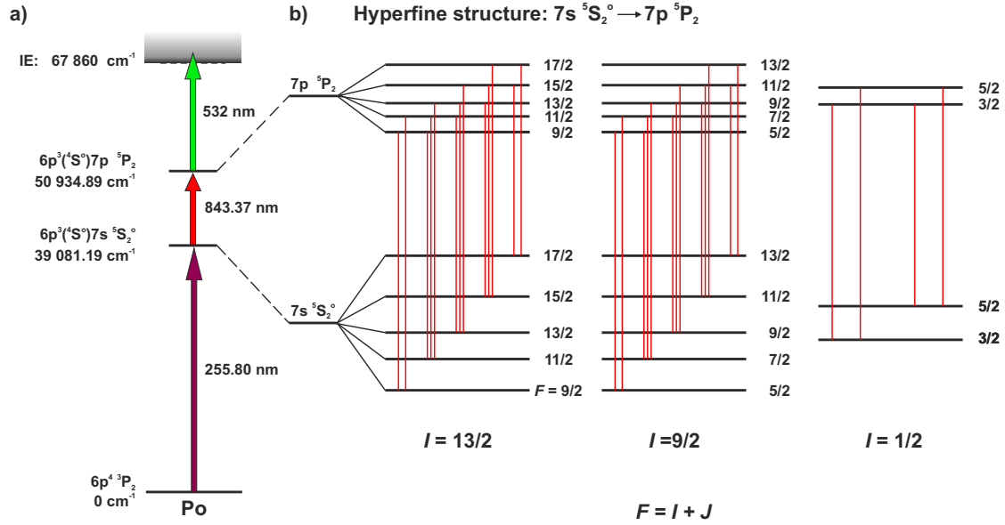
Figure 7.2: a) Three-step laser ionization scheme for polonium. b) Zoom on the possible hyperfine levels for nuclear spins I^\pi = 13/2^+, 9/2^+, 1/2^- with total angular momentum F and corresponding transitions (red solid lines) for the studied transition from the 7s\ ^5S_2^o state to the 7p\ ^5P_2 state. The hyperfine structure is not to scale.
