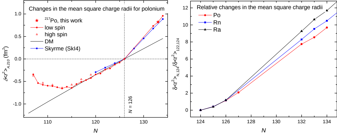
Figure 7.7: Left: changes in mean square charge radii, \delta\langle r^2 \rangle_{A,210} , for polonium isotopes with respect to the reference isotope, ^{210}\text{Po} . ^{217}\text{Po} (star) is shown among the other isotopes (low spin, circle; high spin, triangle) measured during the previous runs at ISOLDE [39, 159]. The predictions from the droplet model (DM) [8] and the SkI4-parametrization of the Skyrme-Hartree-Fock model [71, 72] are given by the black line and the blue squares, respectively. Right: comparison of the relative changes in the mean square charge radii, \delta\langle r^2 \rangle_{N,124} / \delta\langle r^2 \rangle_{122,124} , of Po (this work and [39, 159]), Rn, and Ra [64]. The connections between the data are to guide the eyes only.
