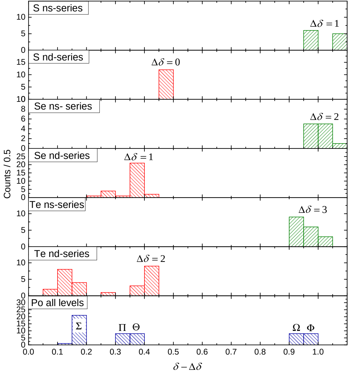
Figure 6.8: Histograms of the distributions of the quantum defects of the Rydberg levels of polonium (Po) and the electron levels found in literature for sulphur (S), selenium (Se) and tellurium (Te). The quantum defects are substituted by \delta - \Delta\delta for a better comparison and the calculated \Delta\delta -values are given in the corresponding histograms. For Rydberg levels, \delta - \Delta\delta values can be identified with the \delta' -values: \delta_{\text{Po}} - \Delta\delta_{\text{Po}} \equiv \delta'_{\text{Po}} . A general trend is observed that \delta - \Delta\delta values of the ns-series (green) tend to be \approx 1 , while the \delta - \Delta\delta values of nd-series (red) tend to accumulate between 0.05 and 0.5. Correspondingly, it can be thus assumed that the Rydberg series \Omega and \Phi of polonium are ns-series and \Sigma , \Pi and \Theta of polonium are nd-series. The \Delta\delta values increase by +1 from sulphur to selenium and to tellurium following the increase of the periods of the homologous elements. Polonium ns-levels should thus have \Delta\delta = 4 and polonium nd-levels should have \Delta\delta = 3 .
