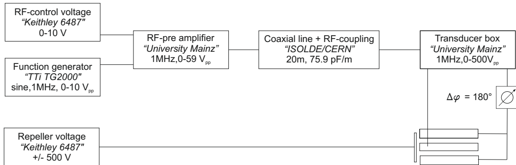
Figure 4.8: A schematic of the electronic supplies and the RF-transmission system from the high-voltage cage to the LIST. The RF-supply system consists of a function generator, a DC-control unit, a pre-amplifier, a radiation hard coaxial line including the RF-coupling and a transducer box. The DC-voltage for the repeller is provided by a power supply and transmitted through a standard feed-through to the target.
