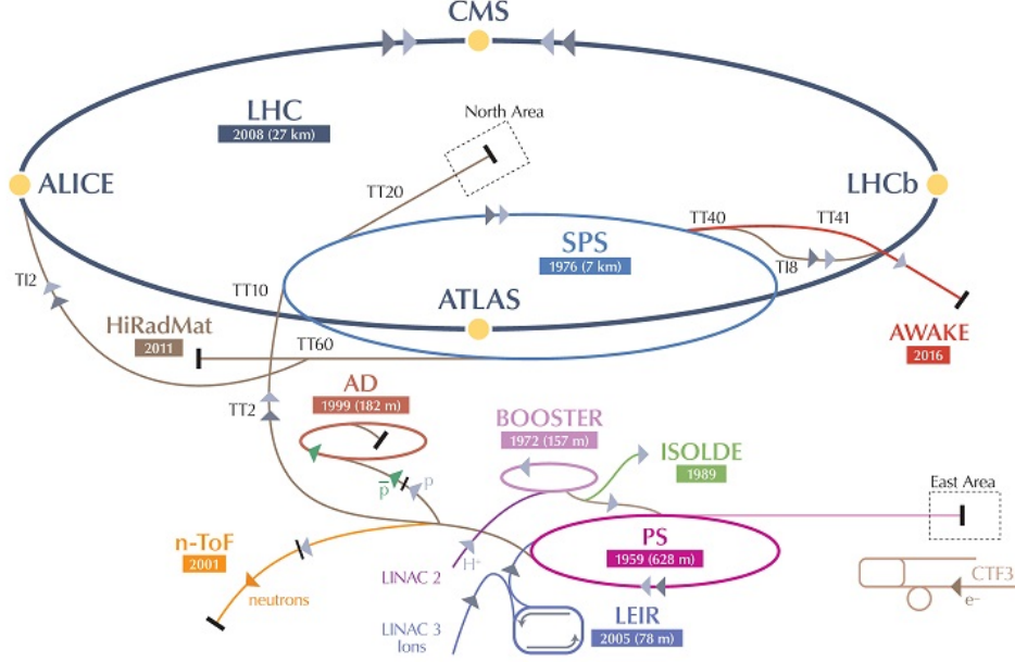
Figure 3.3: An illustration of the CERN accelerator complex with all major facilities. The proton bunches are accelerated by the LINAC 2 and Booster (in the text referred to as the Proton Synchrotron Booster, PSB) to 1.4 GeV before they are sent to ISOLDE [30].
