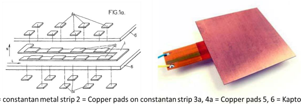
Figure 52: Thin integrated circuit heat flux sensor (Thery and Raucoules, 2006).
