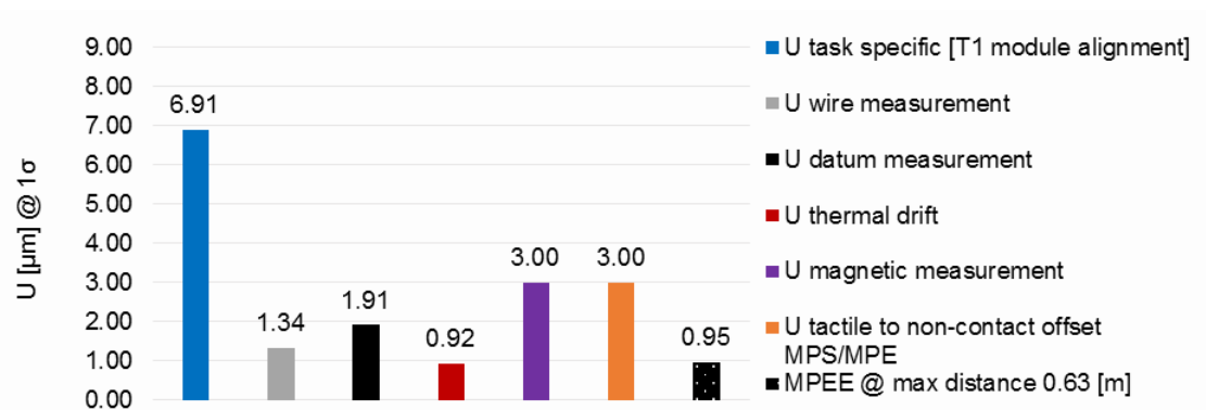
Figure 89: Final alignment uncertainty of magnetic axis alignment measurements using the three spheres datum of CLIC T1 assembly and respective quadratic contributors
