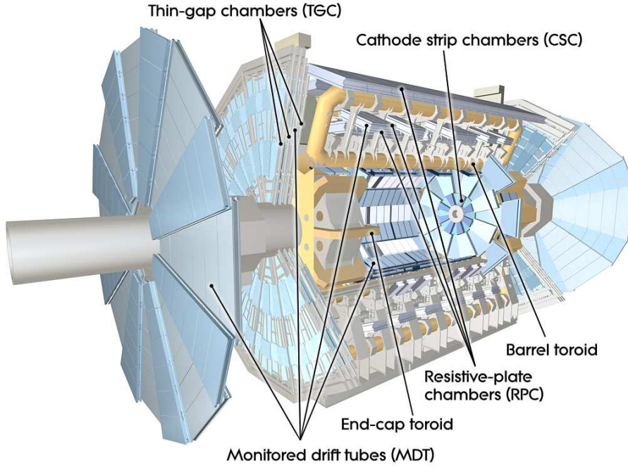
Figure 3.7: Cut-away view of the ATLAS muon spectrometer.
