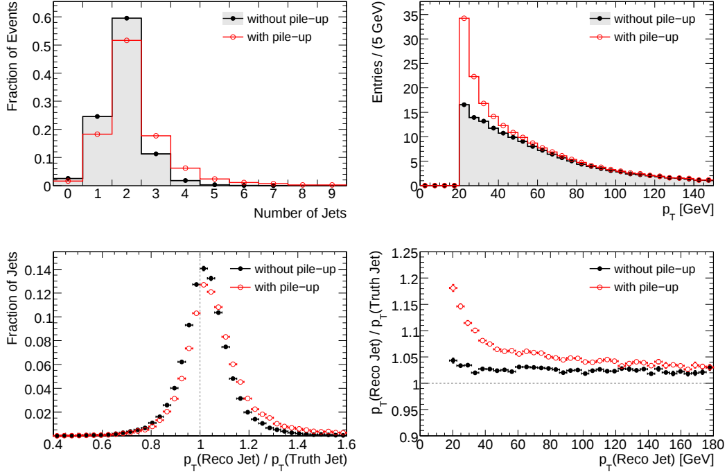
Figure 6.6: Jet multiplicity (top left) and p_T distribution scaled to 1\text{ fb}^{-1} (top right) in H \rightarrow WW events without and with pile-up. The bottom plots show the distribution (left) and p_T dependence (right) of the ratio of the reconstructed and the true jet transverse momentum.
