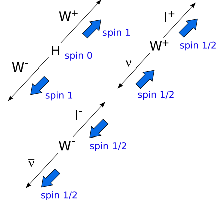
Figure 5.2: Illustration of the spin correlation in H \rightarrow WW \rightarrow l\nu l\nu decays. For Higgs masses close to the threshold m_H \approx 2m_W , the W bosons are produced virtually at rest and the two charged leptons tend to be emitted into the same direction.
