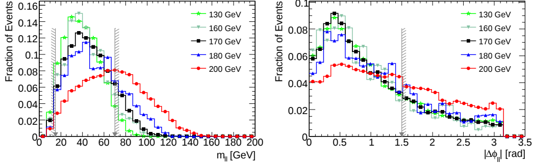
Figure 5.22: Distributions of the invariant mass of the lepton pair (left) and of the azimuthal angle between the two leptons (right) for different Higgs boson masses. The gray arrows indicate the cut values.
