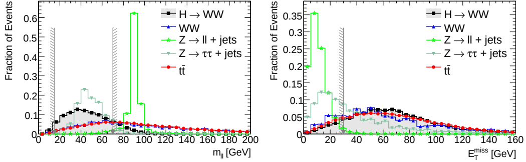
Figure 5.11: Distributions of the di-lepton invariant mass m_{ll} (left) and the missing transverse energy (right). The gray arrows indicate the cut values.
