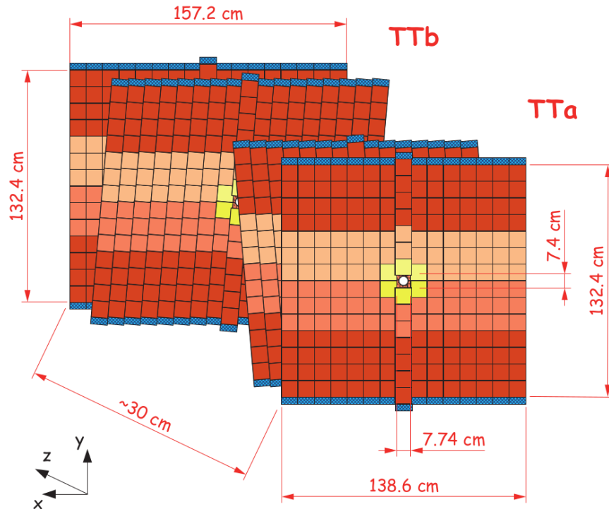
Figure 2.6: A schematic overview of the TT station, where the four layers forming the “ xuvx ” configuration.
