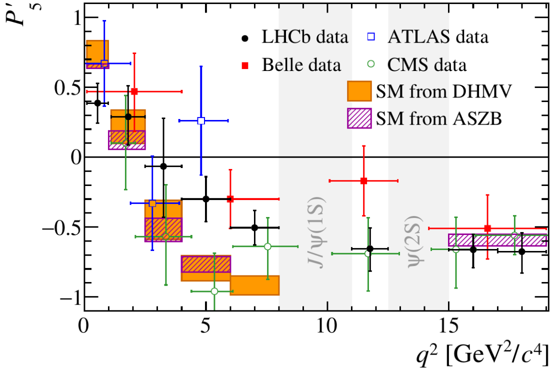
Figure 1.7: A collection of P_5' measurements from several collaborations, where the coloured band represents the SM predictions [34–37].
