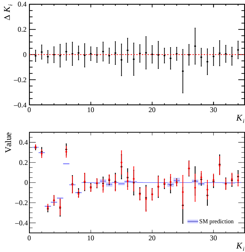
Figure 4.33: (Top) Distribution of \Delta K_i \equiv K_i^{\text{default}} - K_i^{\chi^2} , where the uncertainties are obtained from error propagation; it must be noted that for simplicity correlations are not included in the error determination of \Delta K_i . (Bottom) Comparison of moments obtained with the default method (black markers) and the \chi^2 fit (red markers). The SM predictions are also illustrated by the blue solid line, with the light-blue band corresponding to the uncertainty of the SM predictions [1].
