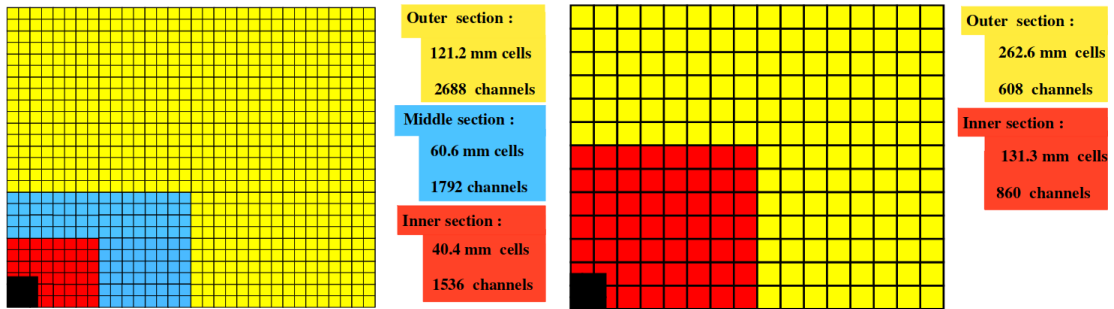
Figure 2.10: The segmentation of ECAL (left) and HCAL (right) [79].
