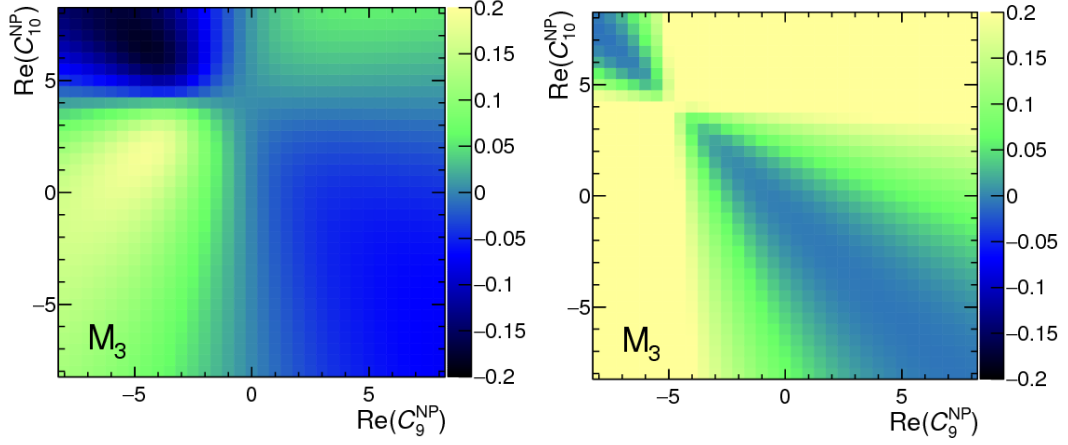
Figure 1.10: Dependence of K_3 (convention used between [44] and this thesis is K_i \equiv M_i ) with variations in \text{Re}(C_{10}^{\text{NP}}) and \text{Re}(C_9^{\text{NP}}) , in 1 < q^2 < 6 \text{ GeV}^2/c^4 (left) and 15 < q^2 < 20 \text{ GeV}^2/c^4 (right) regions.
