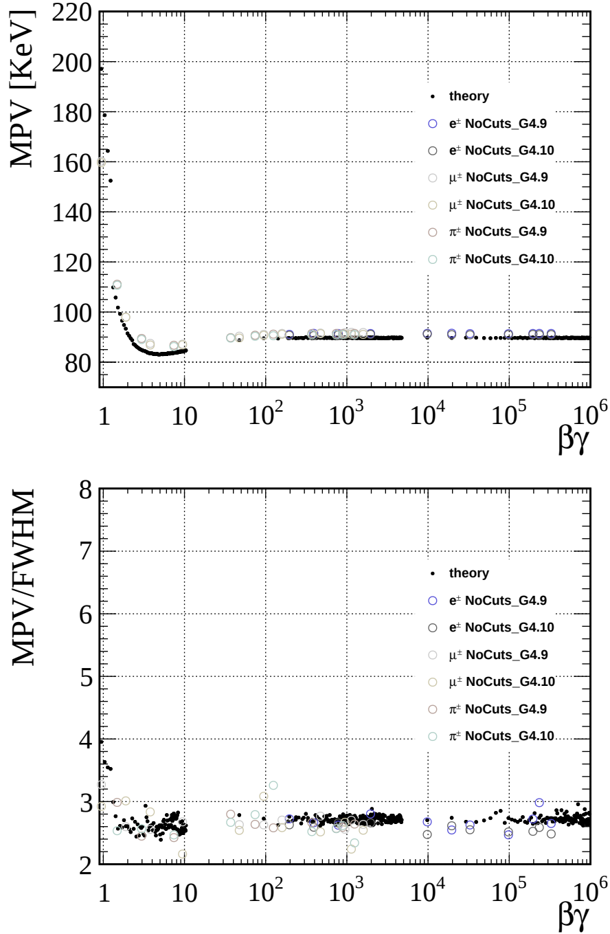
Figure 3.3: Summary of MPV (top) and MPV/FWHM (bottom) from the energy deposits using NoCuts, between GEANT4.9.6P04 and GEANT4.10.3P02 versions.
