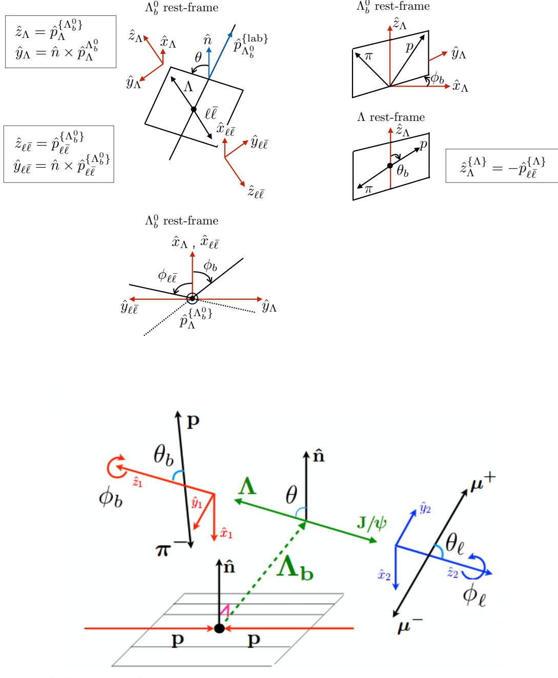
Figure 1.9: Pictorial representation of angles, describing \Lambda_b^0 \rightarrow \Lambda(\rightarrow p\pi^-)\mu^+\mu^- (top) [44] and \Lambda_b^0 \rightarrow \Lambda(\rightarrow p\pi^-)J/\psi(\rightarrow \mu^+\mu^-) (bottom, adopted and modified by Ref. [47]) decay. The angular definition for both decays is identical.
