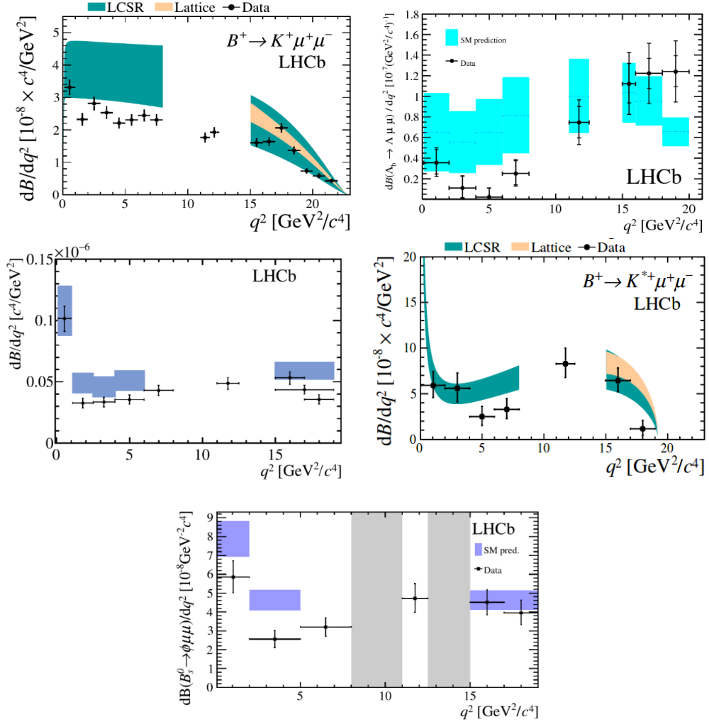
Figure 1.6: A collection of \mathcal{B} measurements in several bins of q^2 . The measurements are compared with the SM predictions (coloured bands), for B^+ \rightarrow K^+ \mu^+ \mu^- [29], \Lambda_b^0 \rightarrow \Lambda \mu^+ \mu^- [27], B^0 \rightarrow K^{*0} \mu^+ \mu^- [30], B^+ \rightarrow K^{*+} \mu^+ \mu^- [29], B^0 \rightarrow \phi \mu^+ \mu^- [28]. The SM prediction of the \mathcal{B} for \Lambda_b^0 \rightarrow \Lambda \mu^+ \mu^- has significantly improved [31], due to improvements in the calculations of the form factors in the context of Lattice QCD.
