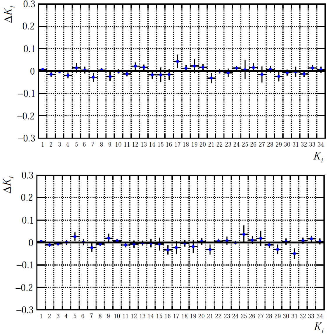
Figure 4.21: Distribution of the differences ( \Delta K_i \equiv K_i^{\text{Uniform}} - K_i^{\text{MC/eff}} ) of the K_i moments extracted from the 6D uniform distribution and the MC additionally weighted by the inverse of the efficiency model, using 2011 + 2012 MC samples of the DD (top) and LL (bottom) category.
