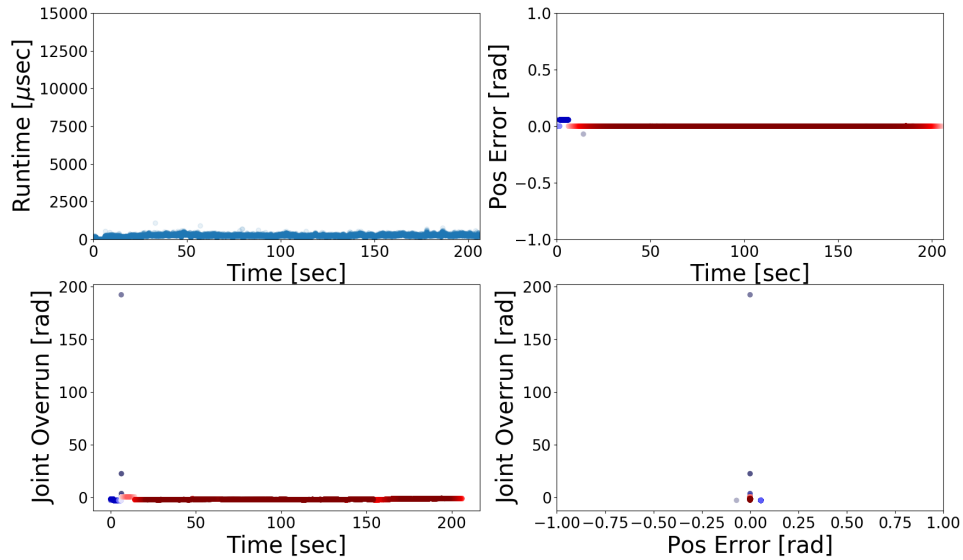
Figure 2.10: Evaluation of KDL Levenberg-Marquardt solver
