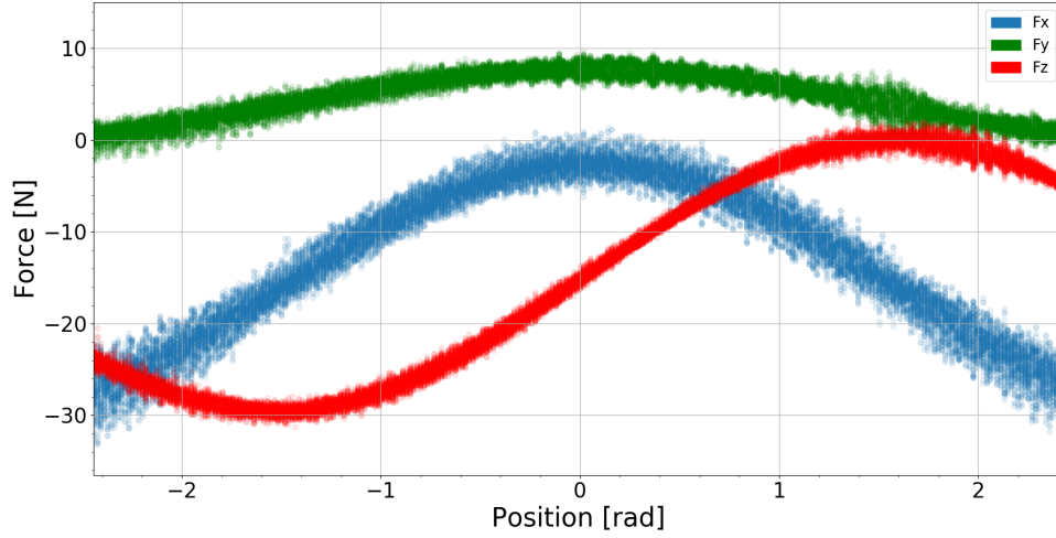
Figure 3.8: The noisy readings of the force values in the sensor coordinate system
