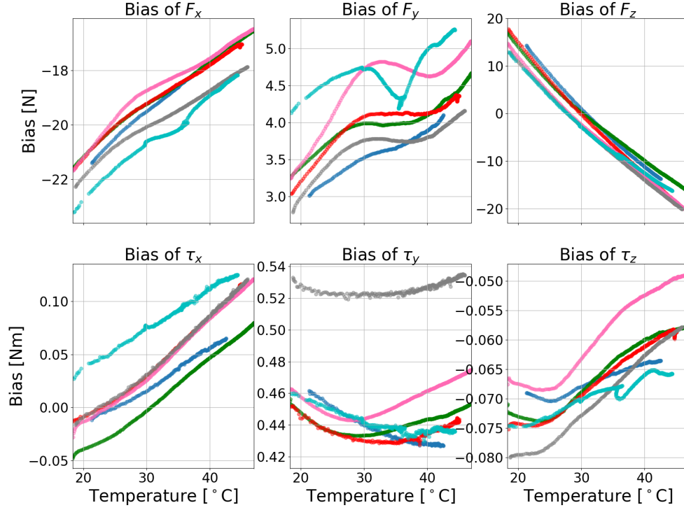
Figure 3.17: The relationship of biases and temperature
