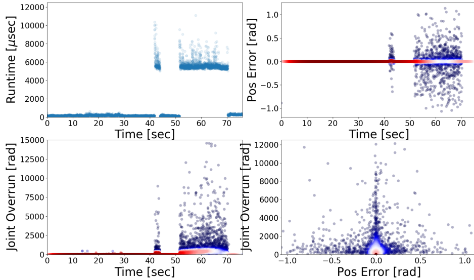
Figure 2.9: Evaluation of KDL Newton-Rhapson solver
