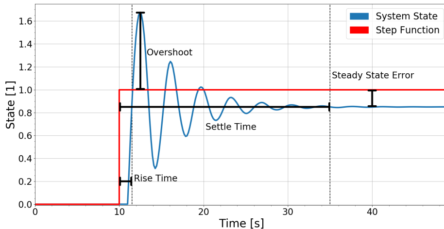
Figure 2.11: Closed-loop response of a poorly tuned PID controlled system
