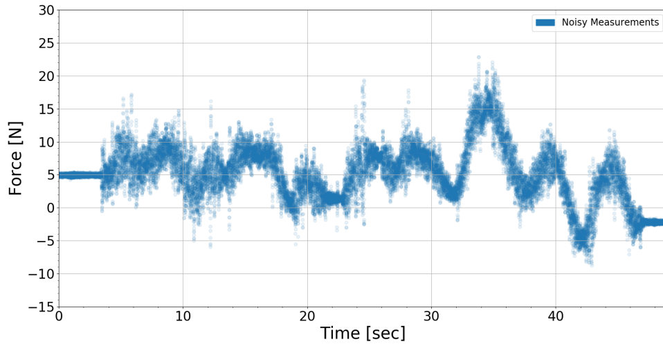
Figure 3.1: The F_z component in the Sensor Coordinate system There is no contact force present
