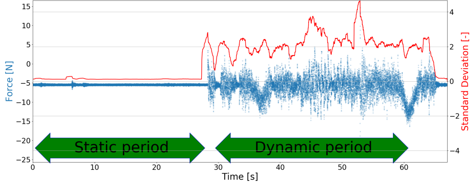
Figure 3.3: The signal in Static and dynamics measurement, with the standard deviation plotted
