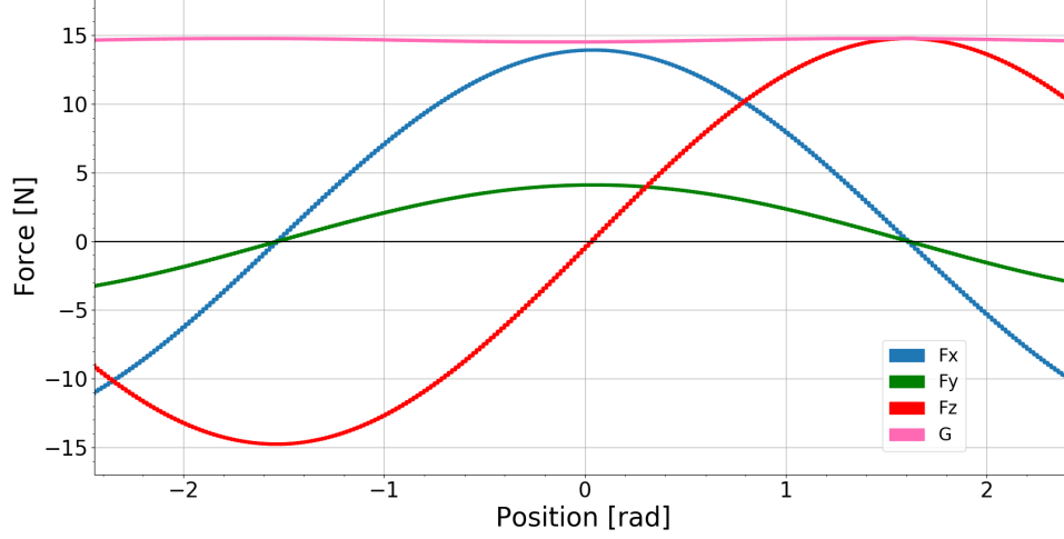
Figure 3.10: The 4 functions compensated for bias
