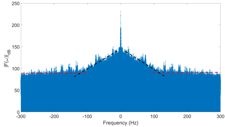
Figure 3.2: The Fourier transformation of noise during movement. Black line shows pink noise. The red line shows white noise.
