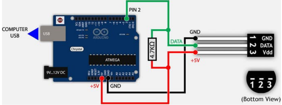
Figure 3.15: The temperature sensor set-up (17)
