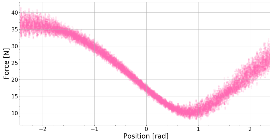
Figure 3.9: The second norm of the force readings
