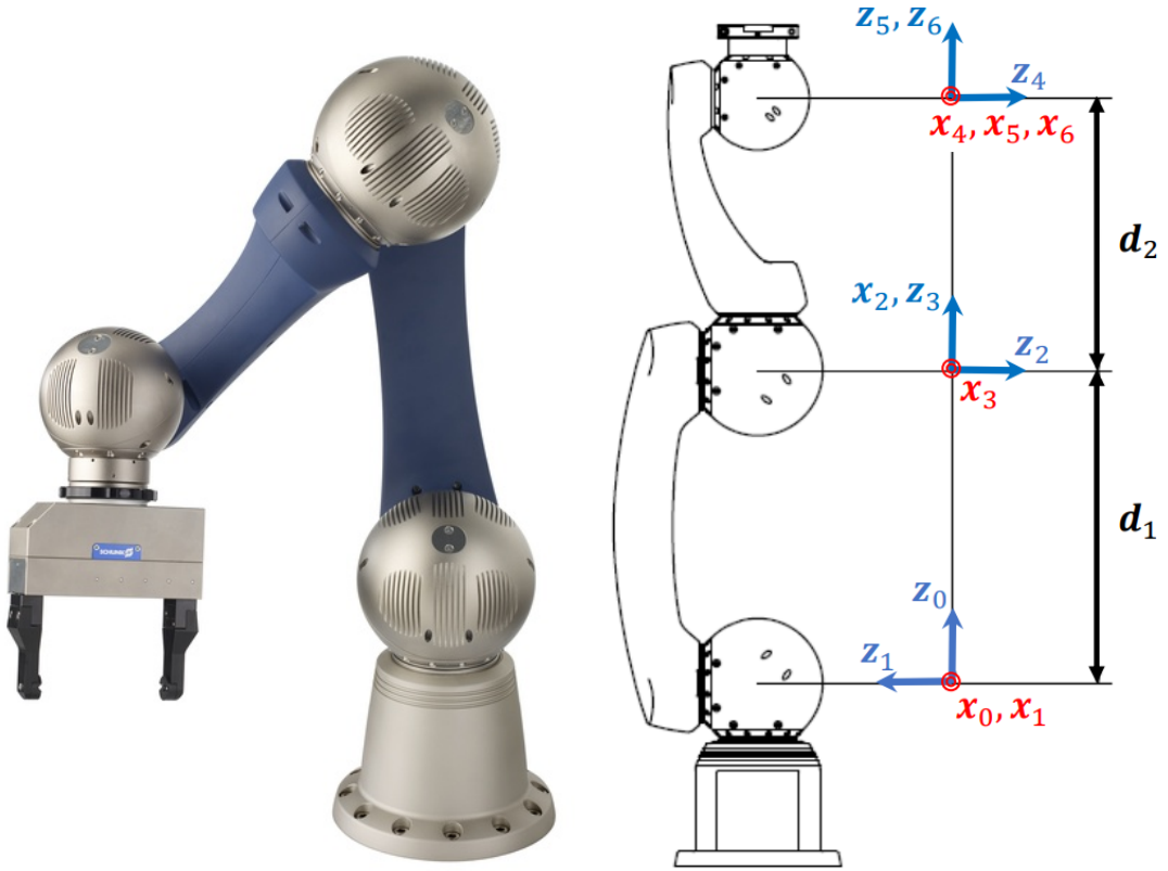
Figure 2.3: The Schunk Powerball robot and the attached Joint Coordinate Frames (12)
