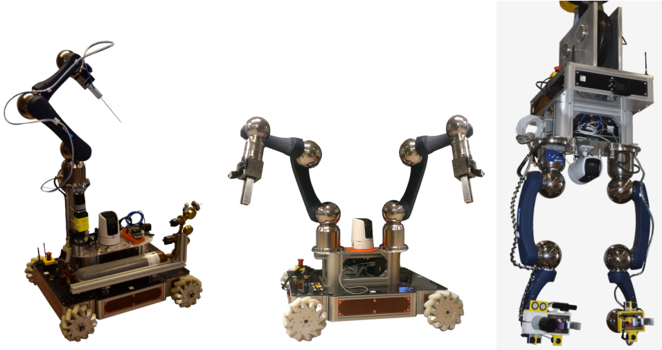
Figure 1.3: Different configurations of the CERNBot
