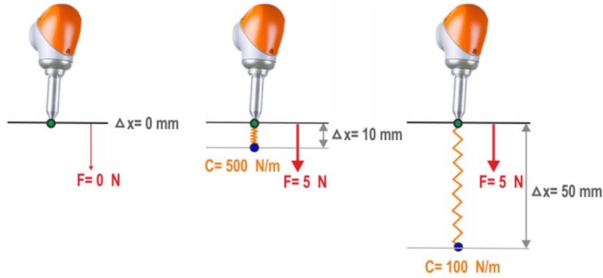
Figure 4.2: Examples for calculating the force exerted by the end-effector
