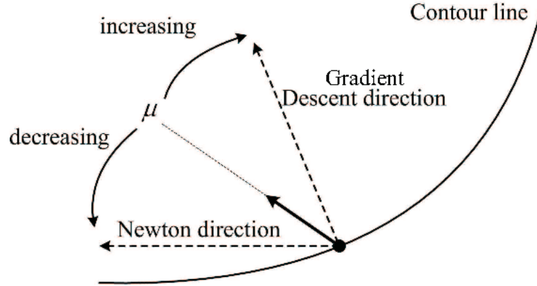
Figure 2.6: The dependence of the steps on the \lambda (here \mu ) parameter
