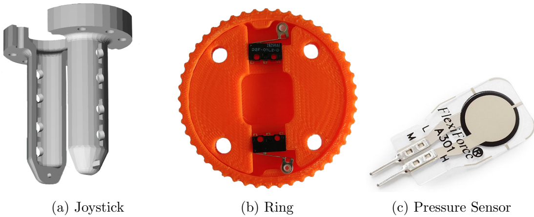
Figure 4.4: The components of the teleoperation end-effector
