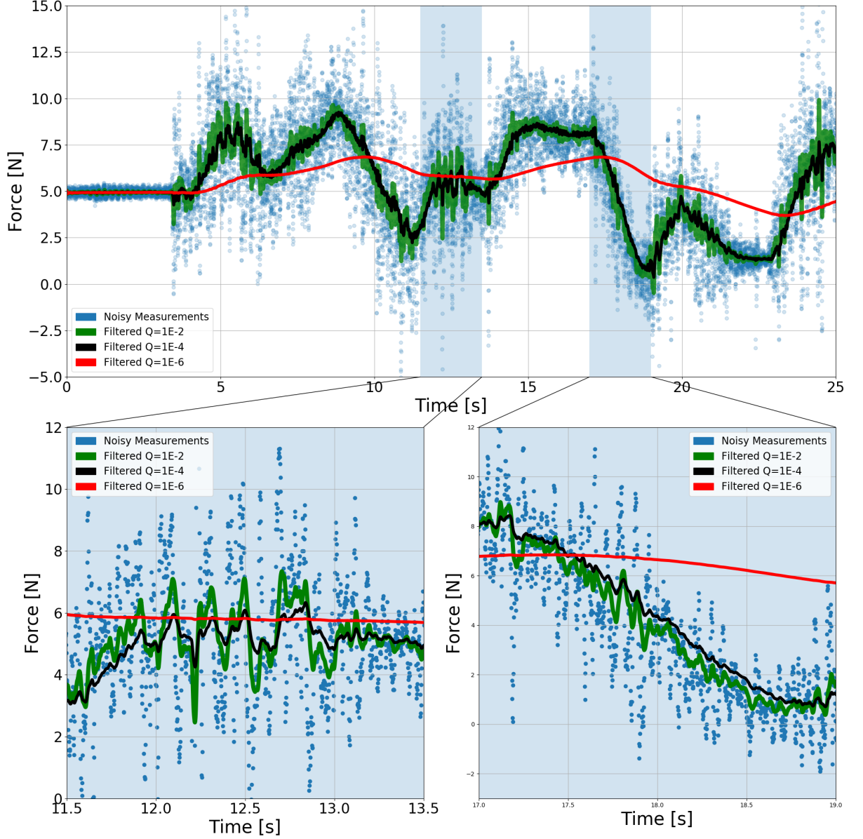
Figure 3.5: The effect of different Q values on the Kalman Filtering of F_x
