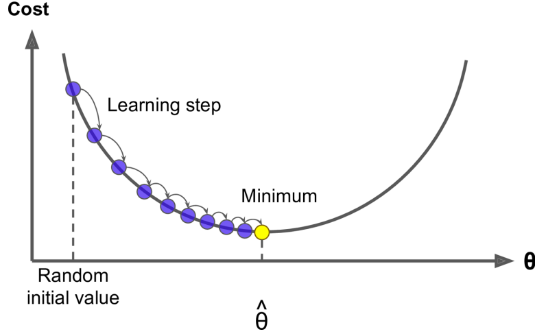
Figure 2.5: The Gradient Descent Method
