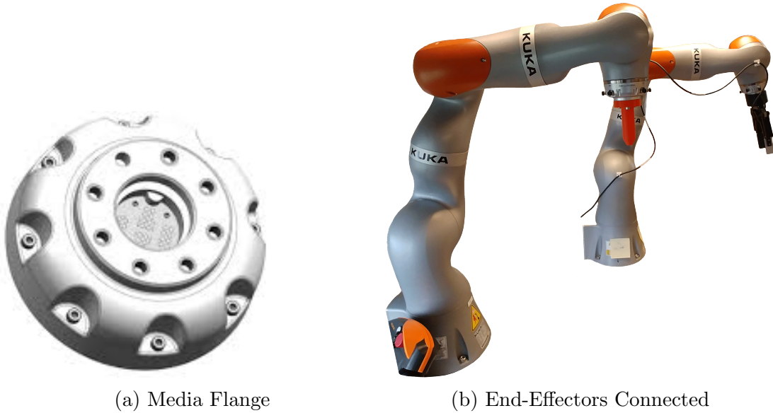
Figure 4.3: Different end-effectors can be interfaced with the robot through the media flange
