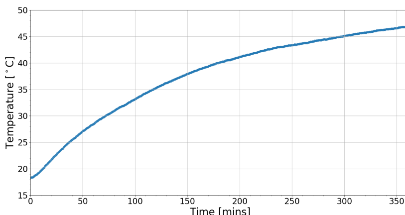
Figure 3.14: The temperature of the Force-Torque sensor
