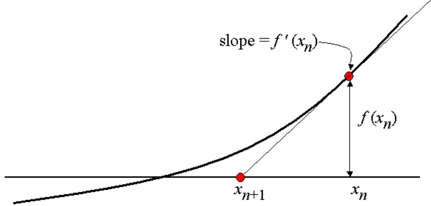
Figure 2.4: The Newton Method
