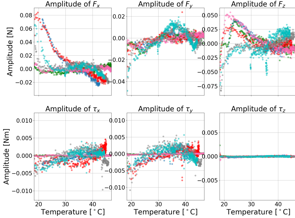
Figure 3.16: The relationship of standardized amplitudes and temperature
