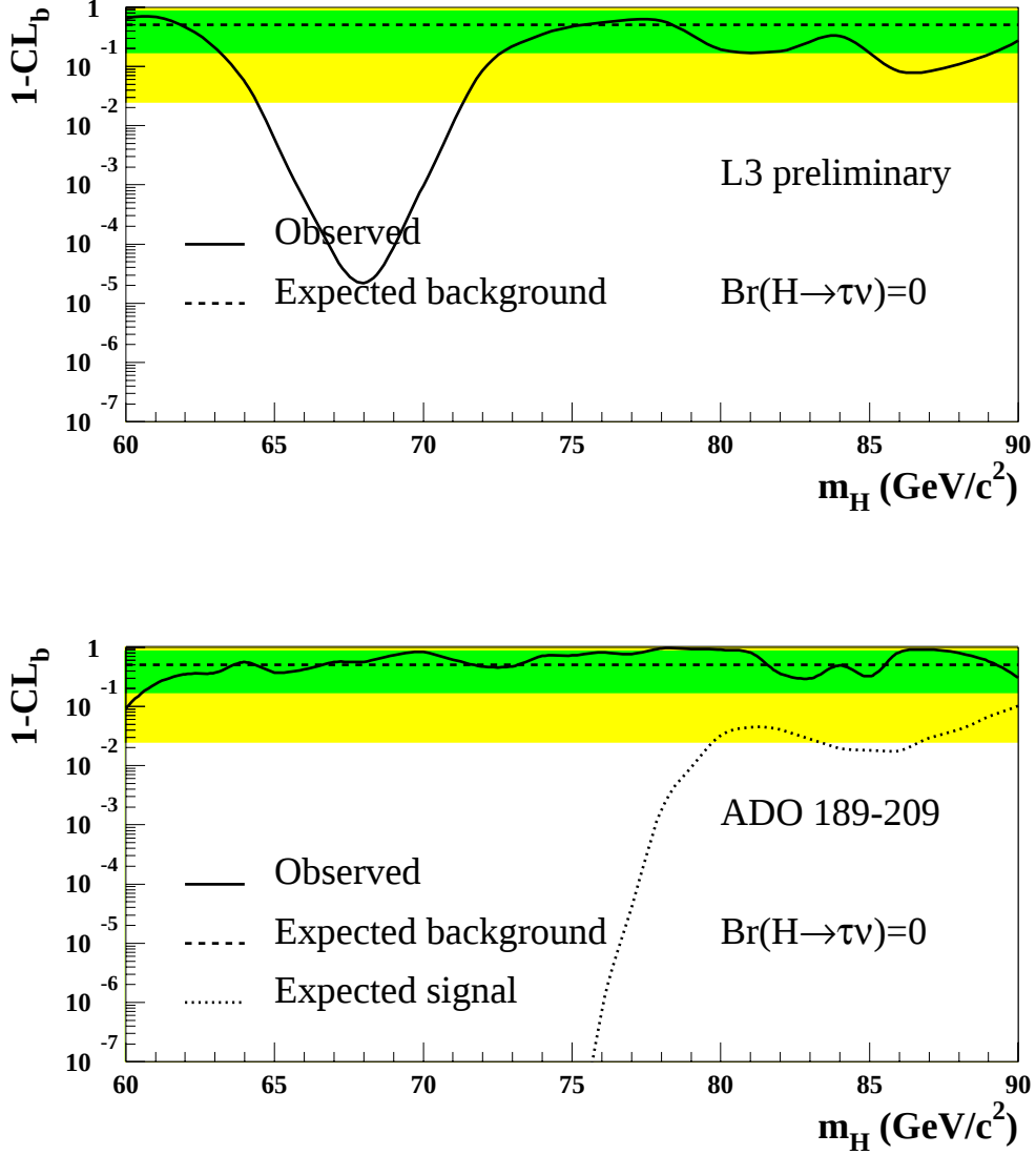
Figure 1: The confidence level 1 - CL_b as a function of m_{H^\pm} , for the branching ratio B(H^+ \rightarrow \tau^+ \nu) = 0 (top : L3 alone, bottom : ADO combination). The straight horizontal line at 50% and the shaded bands represent the mean result and the symmetric 1\sigma and 2\sigma probability bands expected in the absence of a signal. The solid curve is the observed result and the dotted curve shows the median result expected for a signal when tested at the “true” mass.
