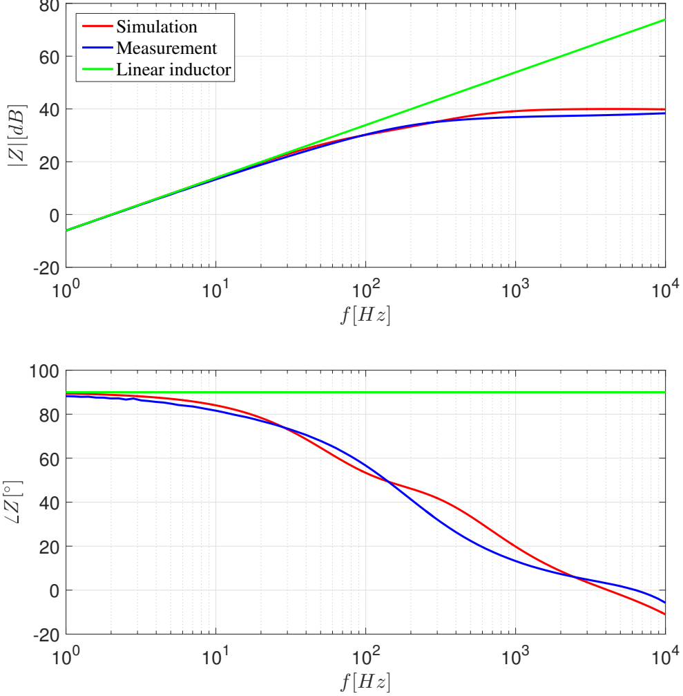
Figure 6.6: Comparison between measurements and simulations
