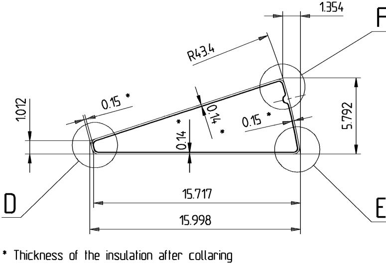
Figure 3.3: Insulation around copper wedges
