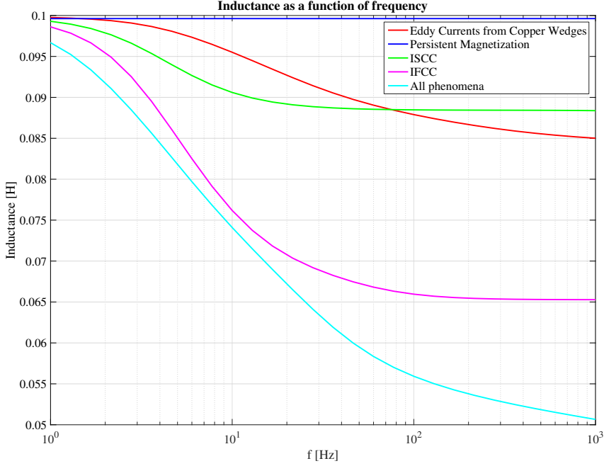
Figure 5.25: L vs \Omega from COMSOL model of MB, isolating various effects to study contribution on magnetization at 1 kA
