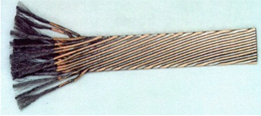
Figure 2.5: Rutherford cable [13]
