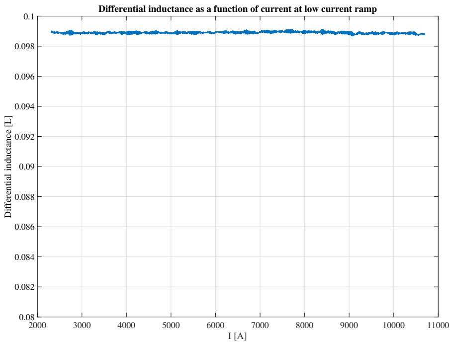
Figure 5.21: Calculation of Differential Inductance from Measurement of Current ramp from LHC during operation
