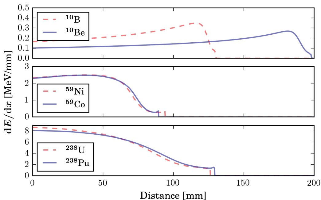
Figure 6.8: Energy loss of ^{10}\text{Be} , ^{10}\text{B} , ^{59}\text{Ni} , ^{59}\text{Co} , ^{238}\text{U} and ^{238}\text{Pu} , as a function of distance in \text{CF}_4 gas, from the SRIM code calculations. It is seen that the separation becomes worse with increasing Z number, from ^{10}\text{Be} - ^{10}\text{B} to ^{59}\text{Ni} - ^{59}\text{Co} . The unexpectedly good separation between the heavier nucleus is likely due to bad accuracy in the SRIM calculations for heavy ions.
