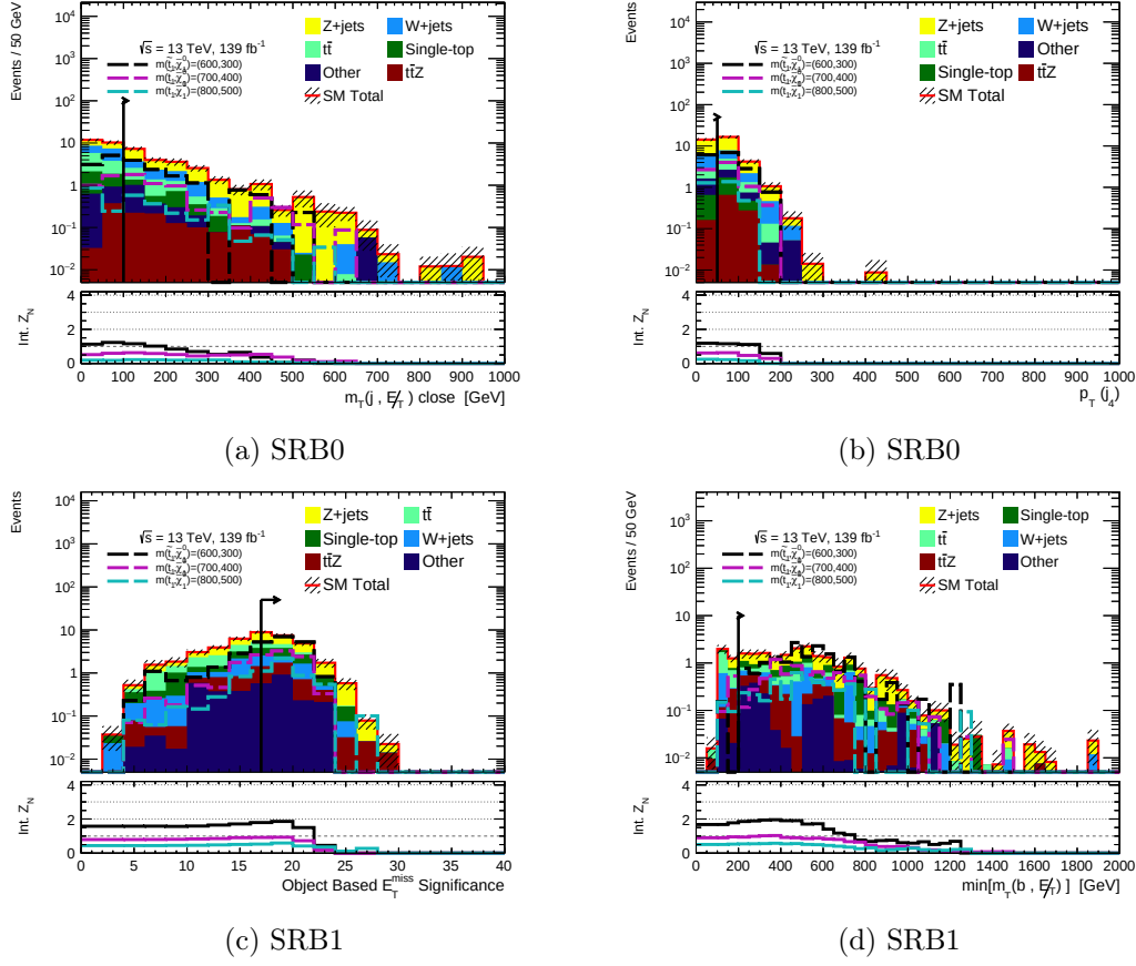
Figure 4.13: N-1 plots of the m_{T, \text{close}}^j (a) and p_T^{\text{jet}_4} (b) selections of SRB0 and of \mathcal{S} (c) and m_{T, \text{min}}^b (d) for SRB1. The stacked contributions from the SM background are shown with the expected signal yields of representative models overlaid with dashed lines. The shaded band indicates the statistical uncertainty on the background expectation and the lower panel shows the integrated significance for the considered signal models. Overflow events are added to the rightmost bin.
