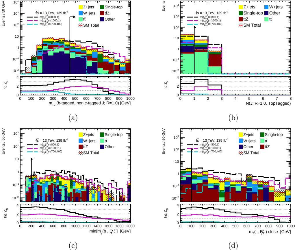
Figure 4.12: N-1 plots of the m_{T2}(J_{R=1.0}^b, c) (a), N_{\text{tops}}^{\text{DNN}}(R = 1.0) (b), m_{T, \min}^b (c) and m_{T, \text{close}}^j (d) variables used in the definition of SRA. The stacked contributions from the SM background are shown with the expected signal yields of representative models overlaid with dashed lines. The shaded band indicates the statistical uncertainty on the background expectation and the lower panel shows the integrated significance for the considered signal models. Overflow events are added to the rightmost bin.
