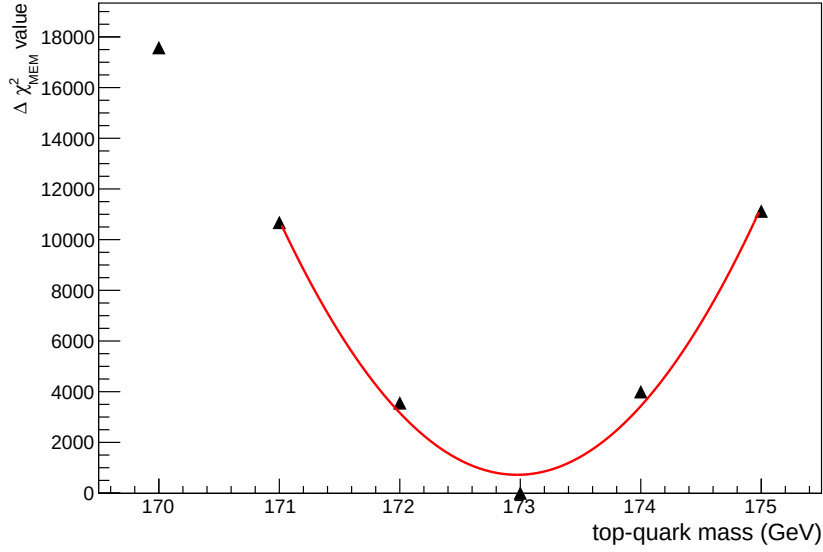
Figure 5.11: \Delta\chi^2_{\text{MEM}} curve obtained for 4000 generator-level events created in Mad-Graph with m_t = 173 GeV fitted with a quadratic function. Minimising this function results in a top-quark mass of 172.97 \pm 0.02 GeV.
