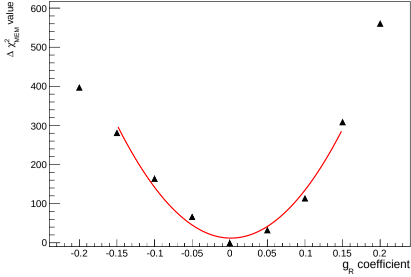
Figure 6.6: Obtained \Delta\chi^2_{MEM} curve using all simulated samples after requiring the -\ln(\mathcal{L}_{MEM}) variable obtained at g_R = 0 to be smaller than 63.87.
