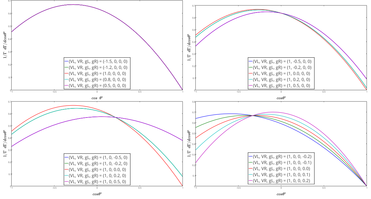
Figure 1.2: Influence of varying a single coupling coefficient on the \cos \theta^* distribution. From upper left to upper right the considered coupling constants are V_L , V_R , g_L and g_R , respectively.
