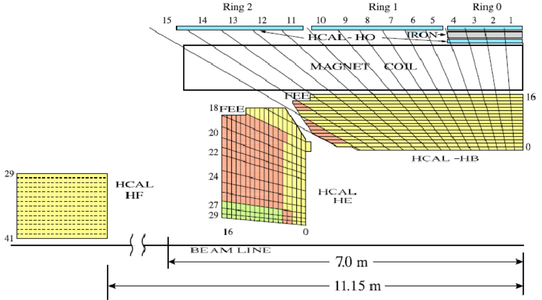
Figure 2.7: Layout of the hadronic calorimeter [65].
