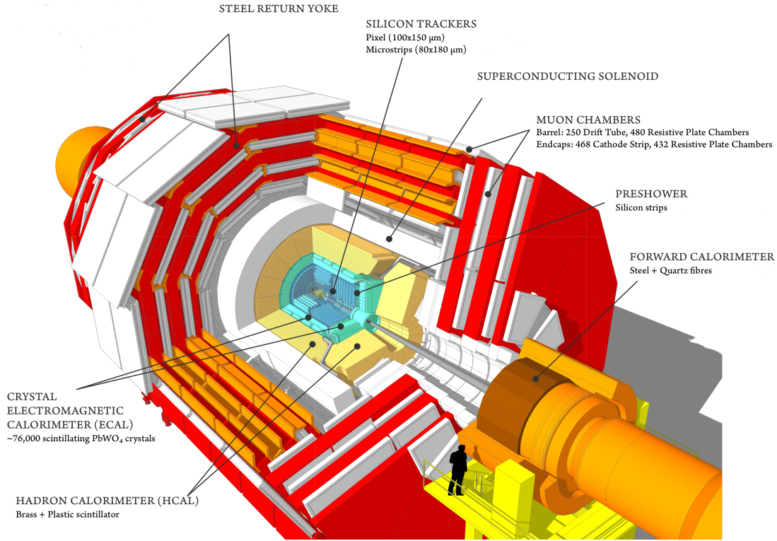
Figure 2.4: CMS layout with all subdetectors clearly visible [60].
