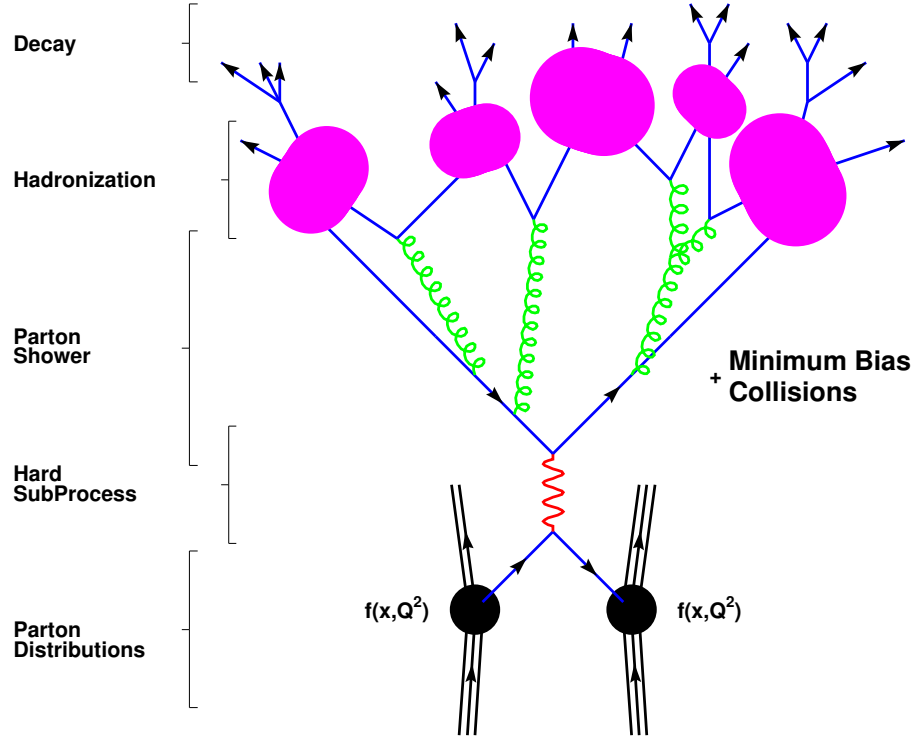
Figure 3.1: Schematic overview of the consecutive steps of the event generation process [72].
