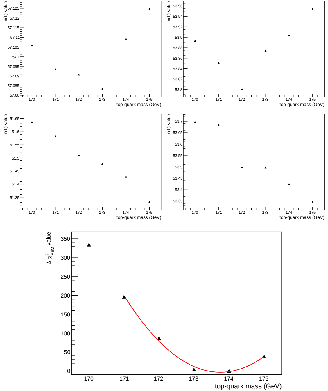
Figure 5.12: Individual event probabilities for the measurement of the top-quark mass (upper two rows) using reconstructed events, which get combined in the overall likelihood (last row) from which the most optimal value of the top-quark mass is extracted.
