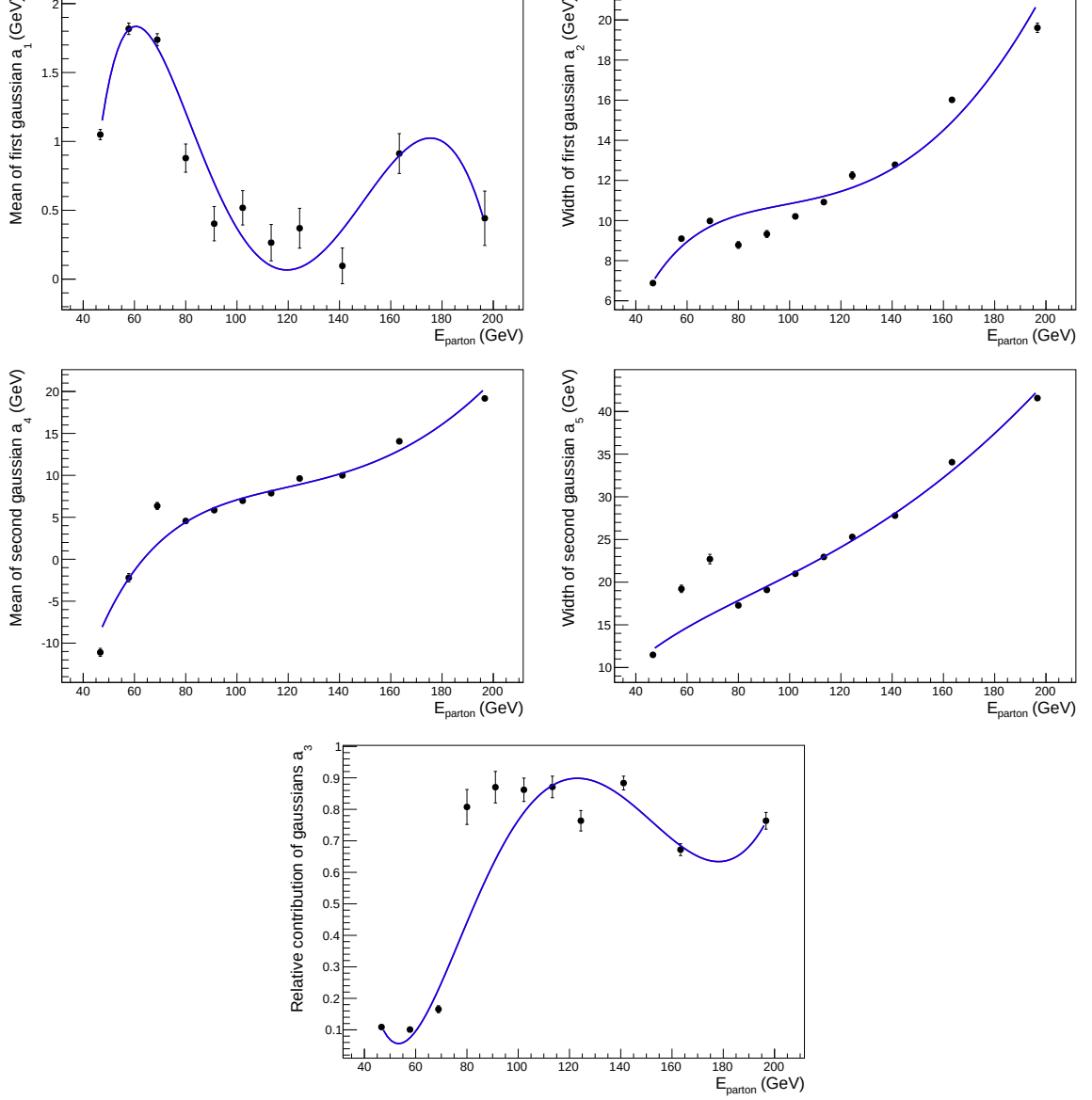
Figure 5.7: Obtained shape for the five E -dependent parameters describing the double-Gaussian jet transfer function for the b-flavoured jets. The two upper parameters correspond to the narrow Gaussian while the two middle ones are related to the broad Gaussian, for which the mean is consistently given on the left and the width on the right. The bottom parameter depicts the relative contribution of the two Gaussian distributions. Each parameter has been fitted with the corresponding parametrisation given in Table 5.1.
