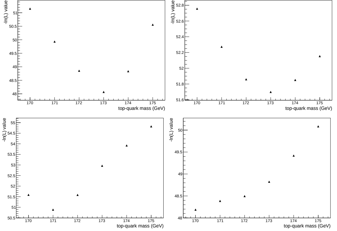
Figure 5.10: Individual event probabilities for the measurement of the top-quark mass using generator-level events.
