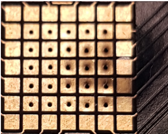
Figure 7.8: Copper pixel sensor burn marks due to the MC40 proton beam.
