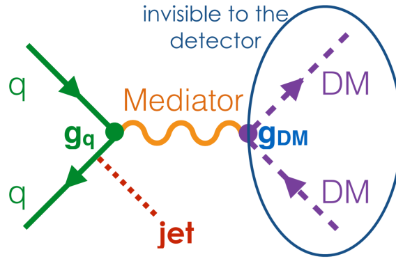
Figure 2.9: A typical monojet signature arising from initial state radiation from a quark that collides with another quark, forming a mediator that decays to dark matter candidates. The jet is detected and influenced via recoiling off the dark matter, which is undetected. No coupling between the jet and dark matter is required, allowing generic probing of dark matter models.
