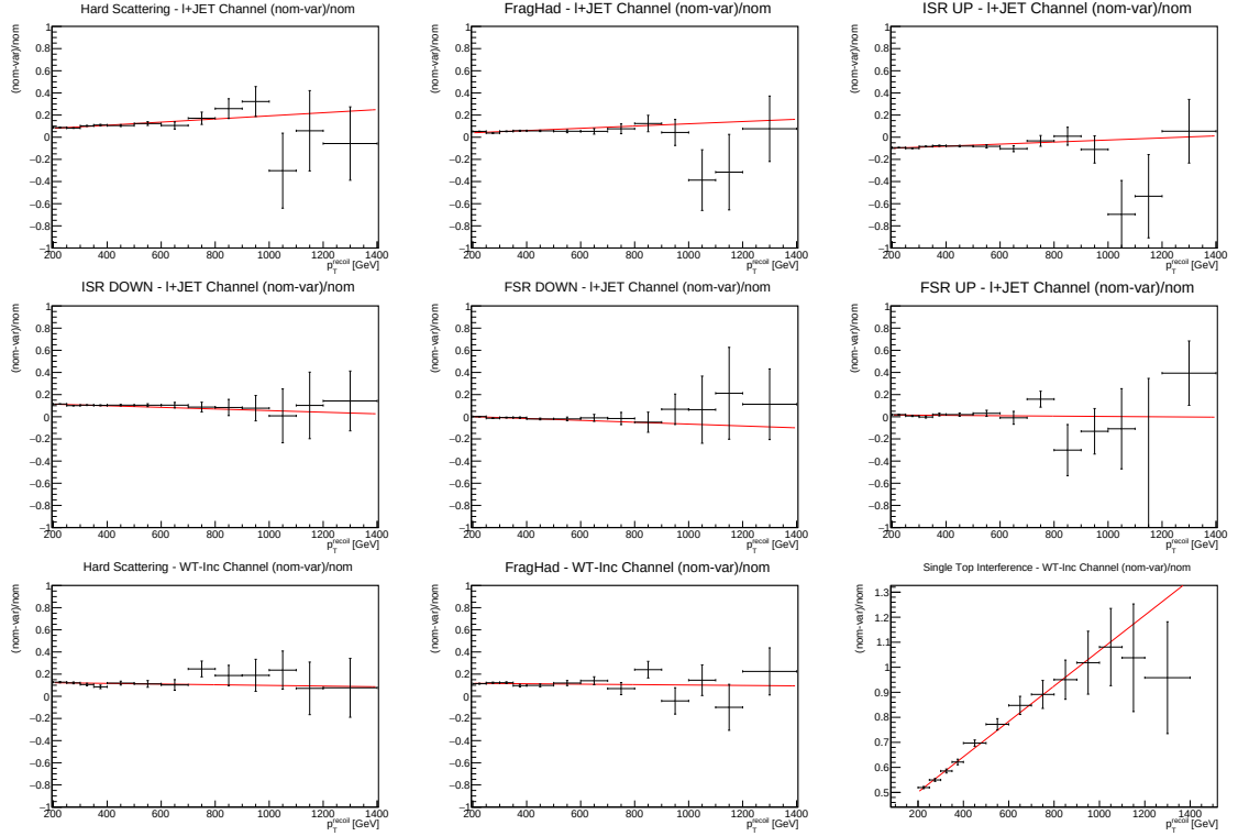
Figure 6.3: Individual systematic uncertainties fitted with a linear fit for both t\bar{t} and single- t systematics. Shown for the l+\text{jet} channel for t\bar{t} and for the Wt -inclusive channel for single- t , the dominant channels of t\bar{t} and single- t respectively in the monojet analysis. Hard Scattering is the uncertainty associated with the scattering between partons, FragHad is the uncertainty associated with hadronization of the final state particles, ISR/FSR is uncertainty in initial/final state radiation. Single top interference is the uncertainty in the single- t case associated with production of a t\bar{t} pair.
