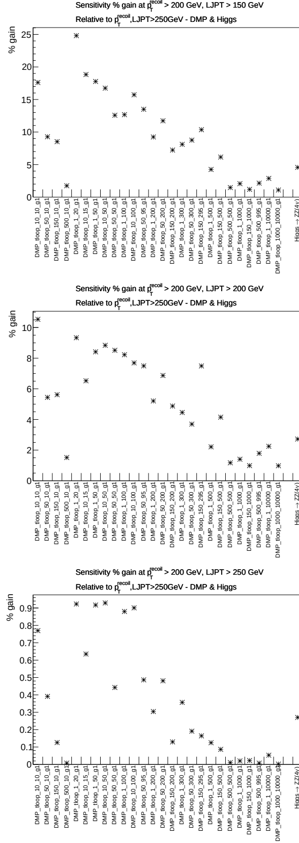
Figure 4.8: Global sensitivity gain estimate when lowering P_T^{\text{recoil}} and leading jet p_T thresholds for Higgs → invisible and pseudoscalar WIMP models (DMP_tloop_x_y_g1 = pseudoscalar WIMP with a WIMP mass = x GeV and mediator mass = y GeV). A significant increase compared to the previous analysis thresholds, up to 25% for some with the P_T^{\text{recoil}} threshold = 200 GeV, and leading jet p_T threshold = 150 GeV.
