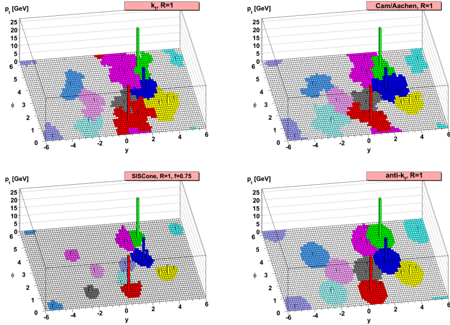
Figure 3.13: Jets formed for an example event with the anti- k_t algorithm, and other jet clustering algorithms [49].
