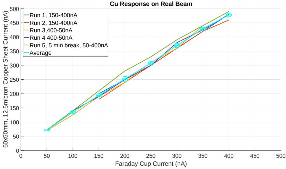
Figure 7.2: Current measured across a copper sheet placed in the MC40 proton beam at various beam currents, showing a linear response.
