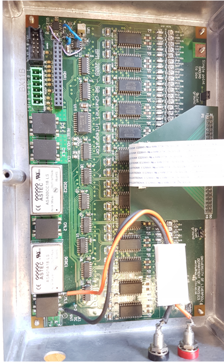
Figure 7.4: Integrator board to readout sensor.
