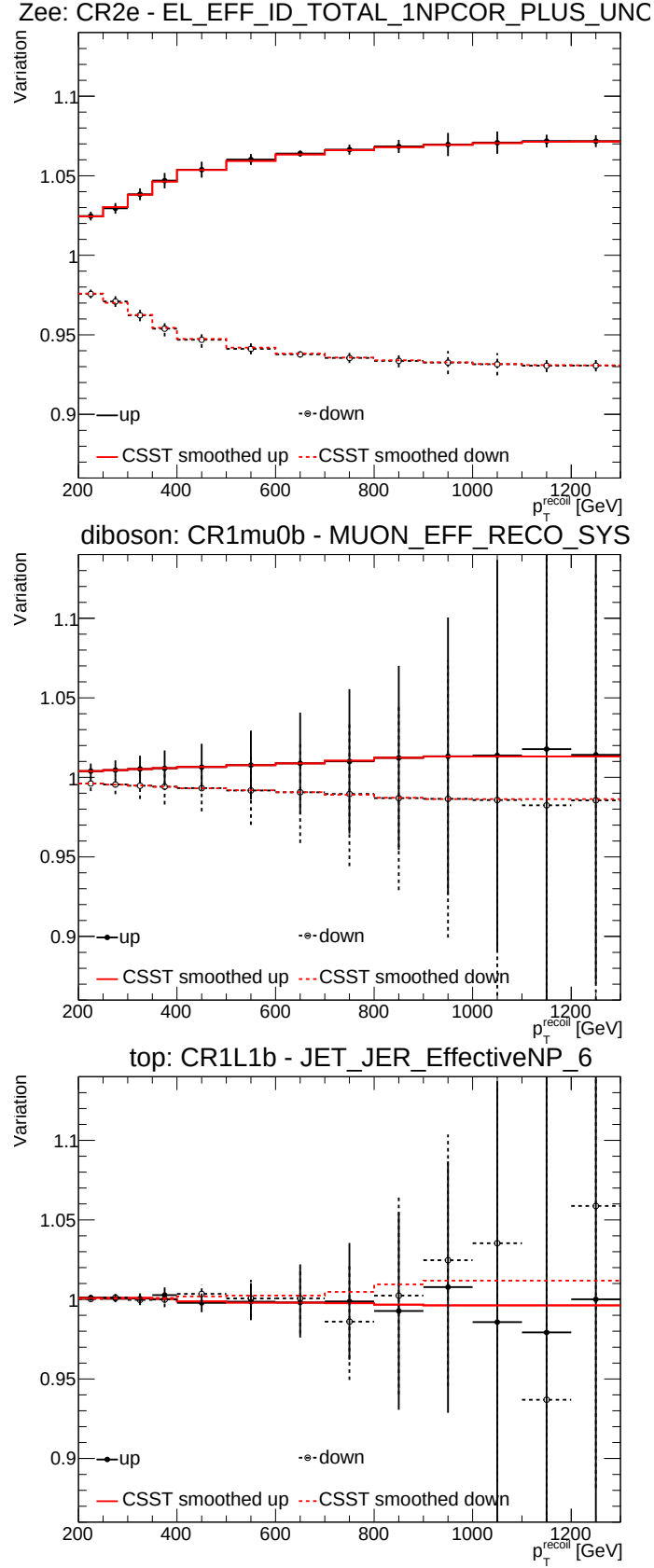
Figure 6.1: Example experimental systematic uncertainty variations of processes with limited MC statistics without (black) and with (red) smoothing applied. From top to bottom, the uncertainty on the: electron identification efficiency scale factors in CR2e, muon reconstruction efficiency in CR1mu0b, jet energy resolution in CR1L1b.
