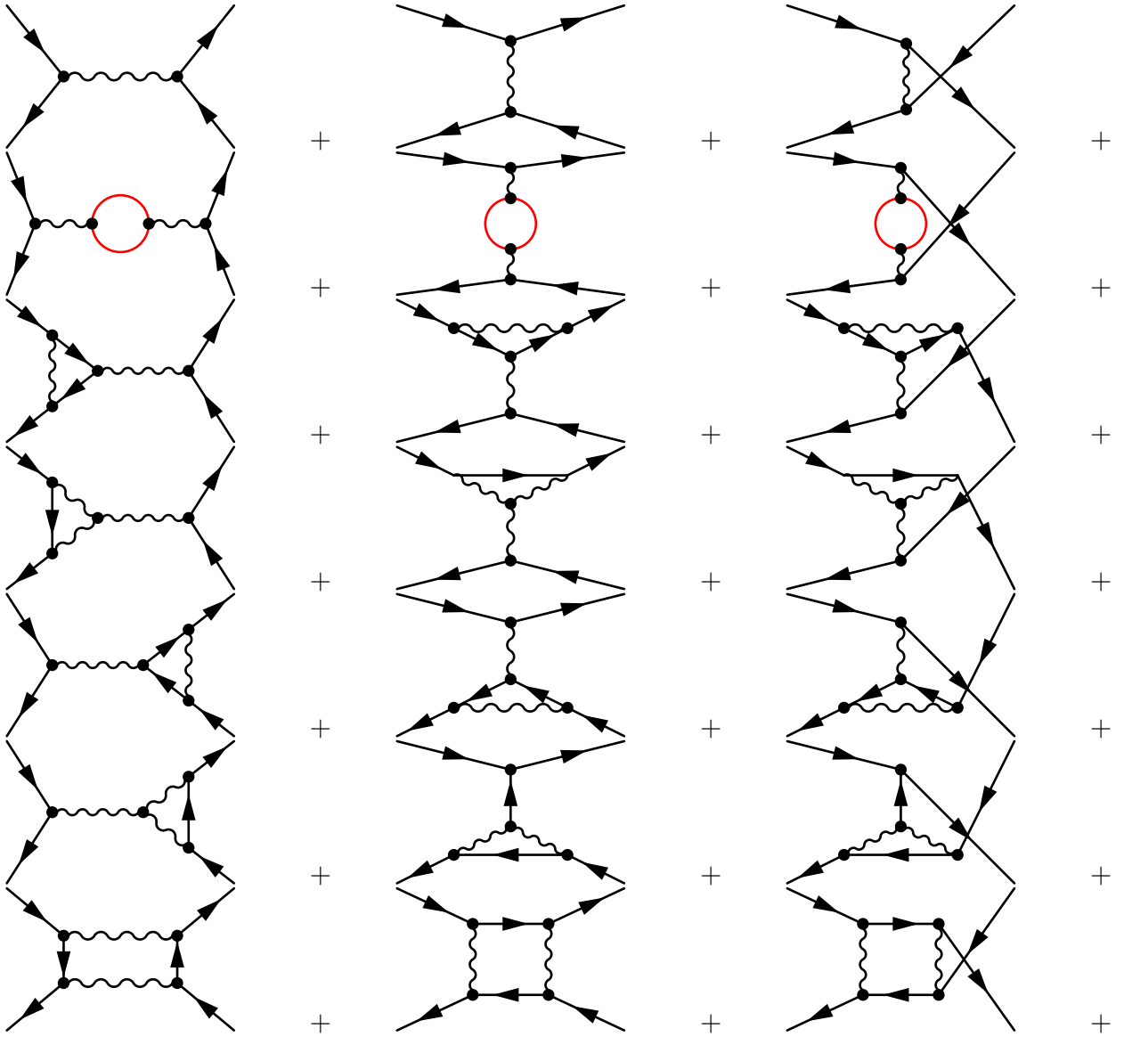
Figure 2.4: Two incoming fermionic fields interacting and producing two outgoing fermionic fields; all Feynman diagrams at leading (two vertices) and next-to-leading order (four vertices). The first, second and third columns represent s-channel, t-channel and u-channel processes respectively. u-channel diagrams are only involved where the 2 final state fields are indistinguishable (e.g. in the case of e^-e^- \rightarrow e^-e^- ). Vertices are represented by a dot; importantly the crossing of the outgoing fermionic fields in the u-channel does not involve a vertex. Diagrams with two plain red lines in them represent the sum of two Feynman diagrams, one where both red lines are bosonic fields and one where both red lines are fermionic fields.
