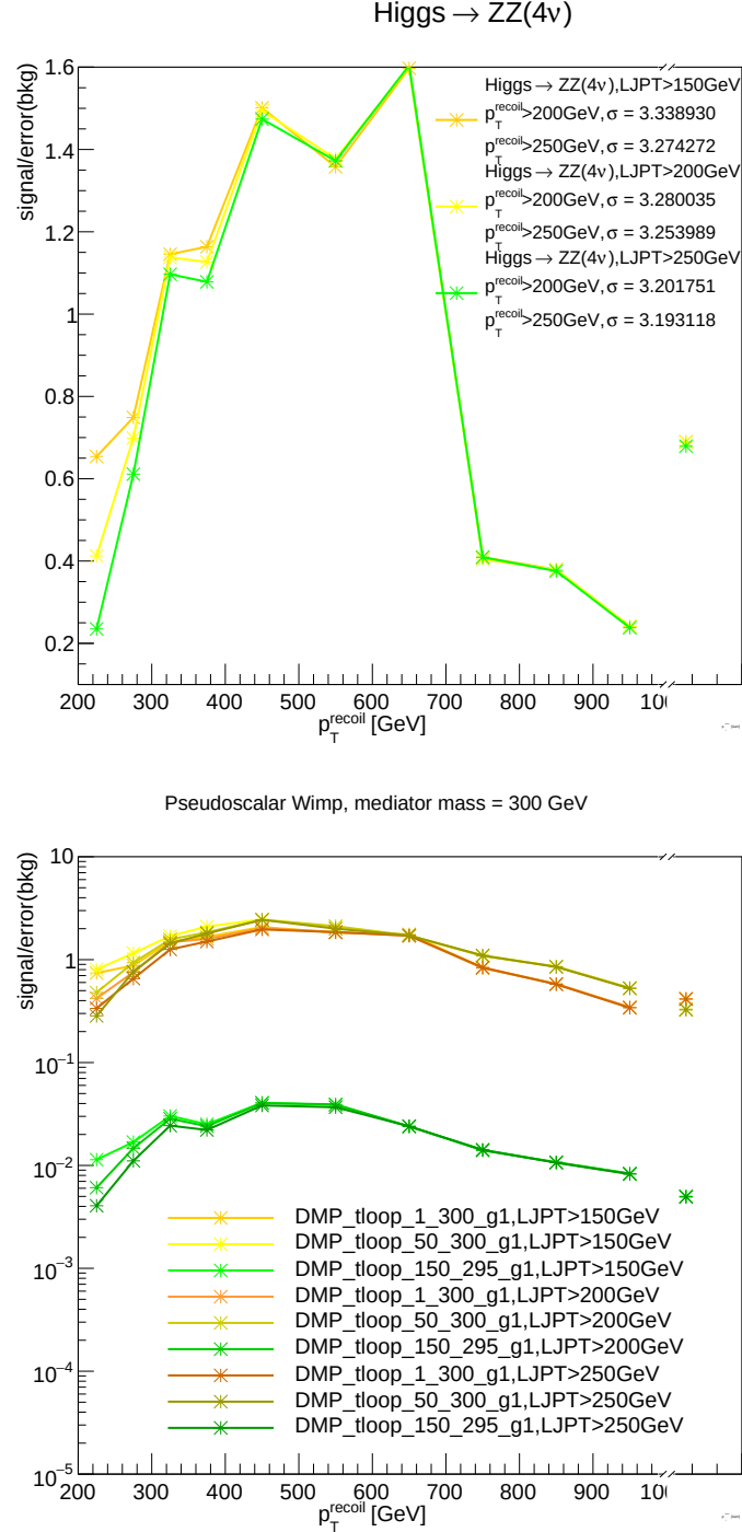
Figure 4.7: Sensitivity estimate per bin when lowering P_T^{\text{recoil}} and leading jet p_T thresholds for Higgs \rightarrow invisible (top) and three example pseudoscalar WIMP models (bottom) (DMP_tloop_x_y_g1 = pseudoscalar WIMP with a WIMP mass = x GeV and mediator mass = y GeV). The sensitivity in the new P_T^{\text{recoil}} = 200\text{--}250 GeV bin can be seen to be comparable to the 250–300 GeV bin when also lowering the leading jet p_T threshold for many samples.
