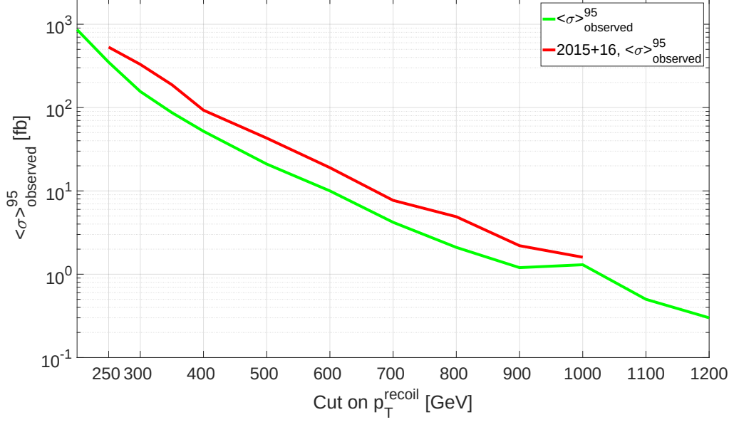
Figure 6.15: Observed 95% confidence level upper limit on the visible cross section, defined as the product of cross section, acceptance and efficiency, \langle \sigma \rangle_{obs}^{95} , for the inclusive selections. The red curve shows the previous version of the monojet analysis, while the green is the current.
