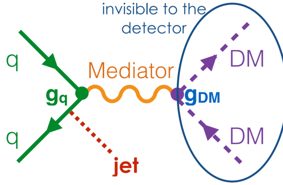
Figure 1.1: A typical monojet signature arising from initial state radiation from a quark that collides with another quark, forming a mediator that decays to dark matter candidates. The jet is detected and influenced via recoiling off the dark matter which is undetected. No coupling between the jet and dark matter is required, allowing probing of generic dark matter models.
