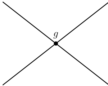
Figure 2.1: Four fields interacting at a vertex with coupling g .
