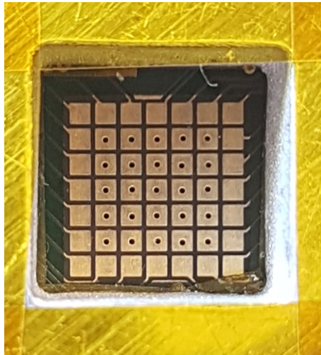
Figure 7.3: Pixel sensor attached to collimator.
