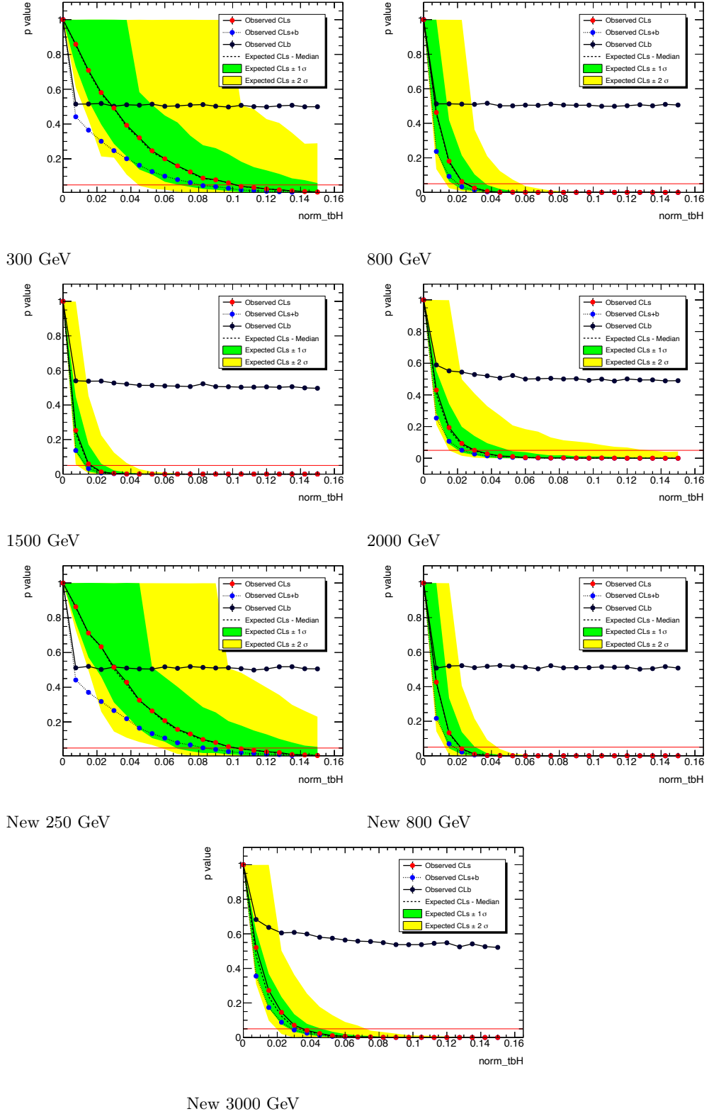
■ Figure 4.14 P-value for different cross-sections, produced by Toy Monte Carlo for all signal masses. The label norm_tbH corresponds to the cross-section in [pb].
