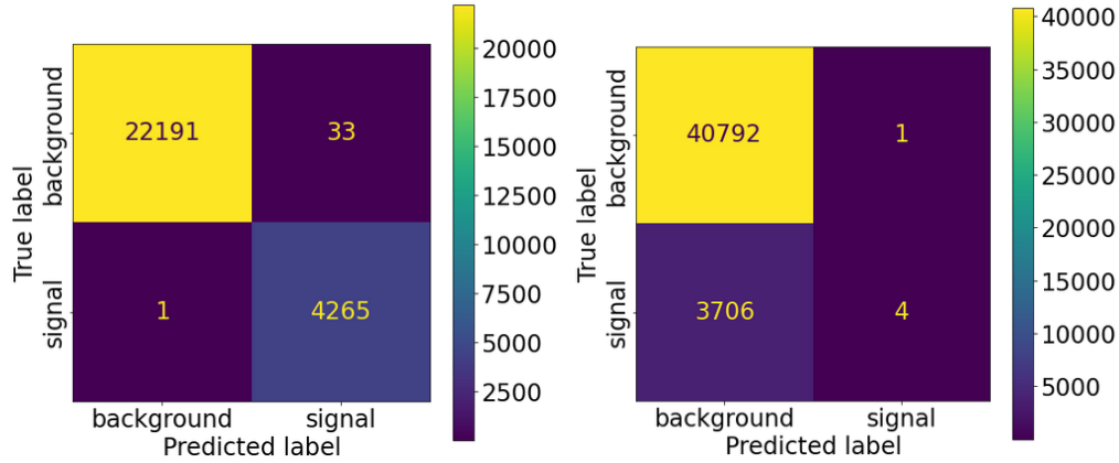
■ Figure 3.3 Confusion matrix for v5 data (left) and v8 data (right)
