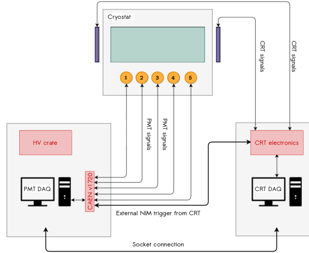
Figure 3.15.: Schematic description of the CRT and PMT-DAQ communication.
