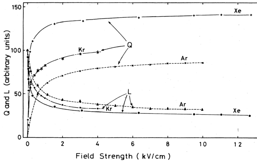
Figure 2.4.: Variation of relative scintillation light, L, and collected ionization charge, Q, as a function of the electric drift field strength produced by electrons with energy in the range (0.976, 1.05) MeV, using various noble gases. Triangle point represent data obtained in LAr in the drift field range reaching up to 10 kV/cm. The plot is taken from Ref. [125].
