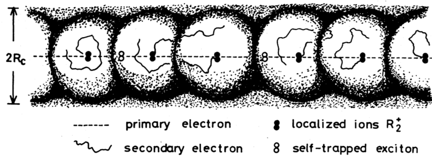
Figure 2.1.: Illustration of the track structure and the Coulomb clouds determined by the ionization process of an incident electron; the Coulomb attraction radius R_C is reported. The illustration is taken from Ref. [125].
