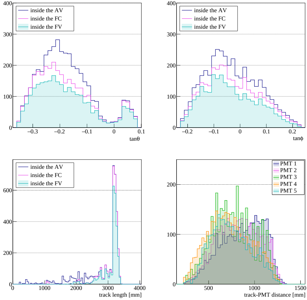
Figure 3.28.: Distributions showing the track topology identified as a consequence of the CRT selection, corresponding to muon-like events crossing the FC volume. Top: Angular distributions in terms of the \theta (left) and \phi (right) angles. Bottom: Distributions of the track length in the three fiducial volumes defined in Sec. 3.3.1 (left) and of the minimum approach distance between the muon-like event's track and each photo-cathode surface, of events inside the FC volume (right).
