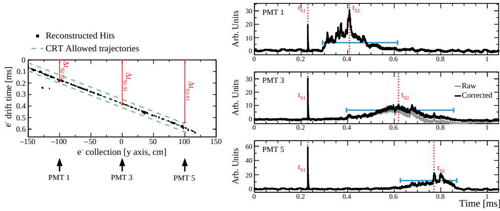
Figure 6.5.: Left: Example of a CRT trigger event crossing the LAr AV of the WA105 DP demonstrator demonstrator. The track reconstruction in the anode plane is shown on the left (black line) within the CRT reconstructed track (cyan lines). Right: The waveforms detected by PMT-1, PMT-3, and PMT-5 are shown on the right, after the pedestal subtraction and inverting the sign of the S1 and S2 peaks; the correction of the raw PB waveform is visible in the middle-right plot [223].
