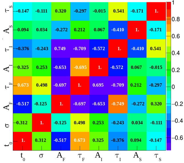
Figure 4.3.: Correlation matrix of the parameters needed in Eq. (4.1b) to reproduce the scintillation time profile. The color scale represents the intensity of the correlation.
