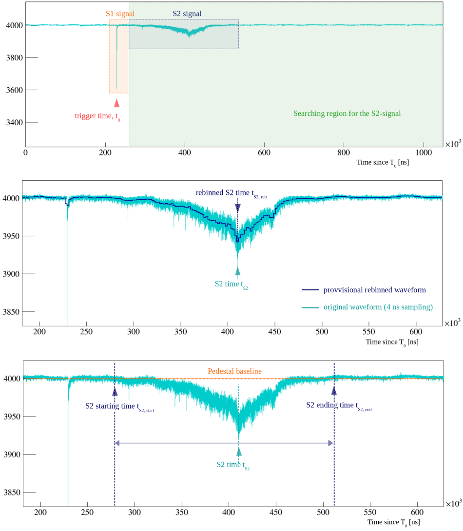
Figure 6.3.: Description of the S2-algorithm steps from the example of a single-event waveform detected by a NB PMT. Top: Definition of the region of interest for the searching of the S2-minimum. Middle: Identification of the S2-minimum in a rebinned and un-rebinned waveform. Bottom: Definition of the characteristic quantities defining the electroluminescence signal retrieved by the S2-algorithm.
