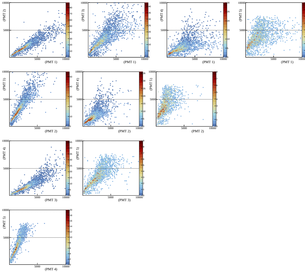
Figure 3.29.: Correlation of the integrated S1 charge over 4 \mu s collected by each PMT with respect to each of the others PMTs, after applying the complete CRT cut sequence.
