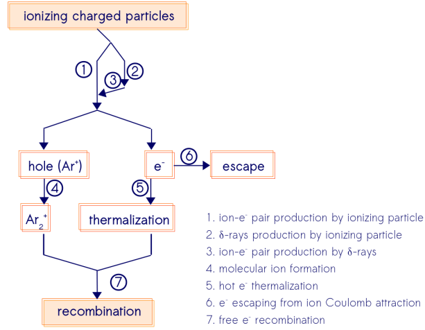
Figure 2.2.: Scheme summarizing the general reactions occurring in noble gases excited by ionizing charged particles; re-adapted from Ref. [125].
