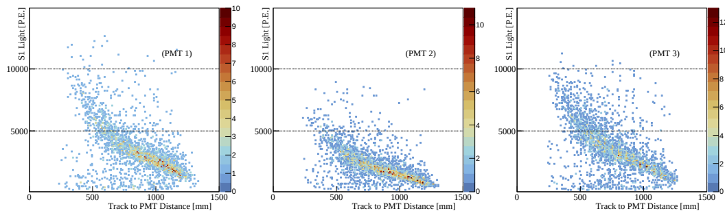
Figure 5.1.: 2-D distributions of the S1 light, integrated over 4 \mu\text{s} , as a function of the minimum approach distance. The typical muon-like event selection for track triggered by the CRT panels is applied; only muons inside the FC volume are accepted.
