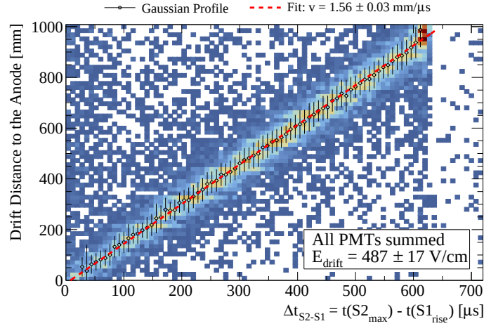
Figure 6.6.: Measurement of the drift velocity, based on the CRT track reconstruction, performed in presence of a 0.485 kV/cm drift field [223].
