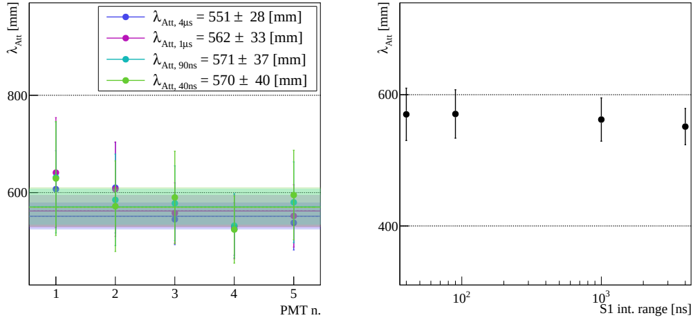
Figure 5.4.: Left: Measurement of the attenuation length measured by the five PMTs in the four integration time ranges: 40 ns in green, 90 ns in cyan, 1 \mu s in magenta, and 4 \mu s in blue. Right: The average on the five PMTs is reported as a function of the integrated charge range.
