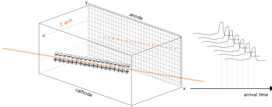
Figure 1.3.: Schematic description of the TPC operation principles. The orange line represents the track of the crossing particles producing ionization electrons and positive ions drifted by the electric field. The 2-D reconstruction of the track projection takes place in the anode plane; the arrival time of the drifted electrons gives the z-coordinate of the track.
