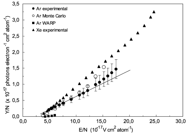
Figure 2.8.: Electroluminescence yield as a function of reduced electric field produced in Argon from measurements (full dots from Ref. [197] and Ref. [199]) and simulations (empty dots from Ref. [200]). The plot is taken from Ref. [197].
