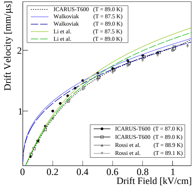
Figure 2.5.: Summary of the studies related to the drift velocity measurement in LAr. Colored lines represent the drift velocity parameterization as a function of the drift field and temperature given in Ref. [169] (Walkoviak) and Ref. [174] (Li). The points correspond to the measurements performed by ICARUS-T600 (Ref. [170] and [171]), and Rossi et al., [173].
