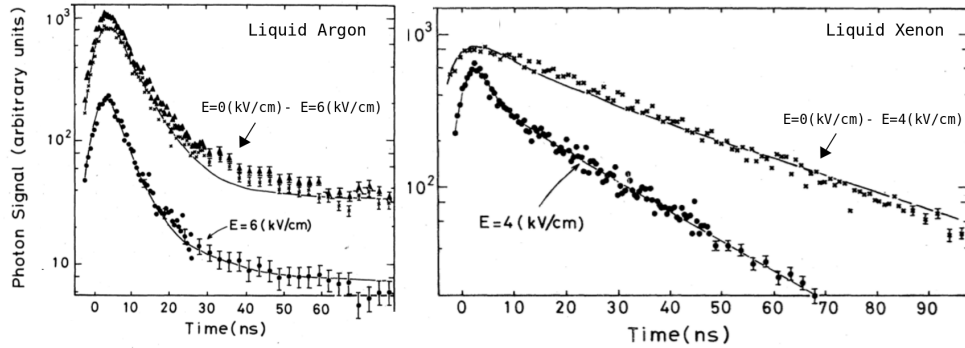
Figure 4.25.: Scintillation time profile measured, without (triangles) and with (full-dots) an applied electric field; the difference curve between the two represents the recombination contribution ( \times ); the results referred to LAr are shown on the left and the ones referred to LXe on the right. The plots are taken from Ref. [125].
