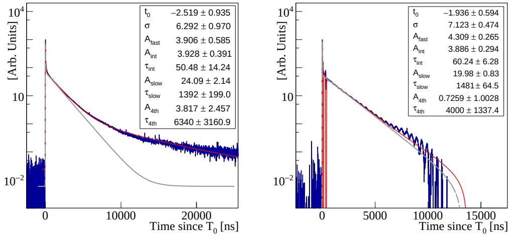
Figure 4.10.: Scintillation time profile showed up to 25\ \mu\text{s} for an NB PMT ( left ) and up to 12\ \mu\text{s} for an PB PMT ( right ). For the NB PMT a fourth exponential is needed to reproduce correctly the data in the whole range; the four-exponential function is drawn in red . The three-exponential function ( grey -line) after \sim 5\ \mu\text{s} is no longer able to reproduce the data. Otherwise, in the PB PMT the three-exponential function is still valide to reproduce the time profile.
