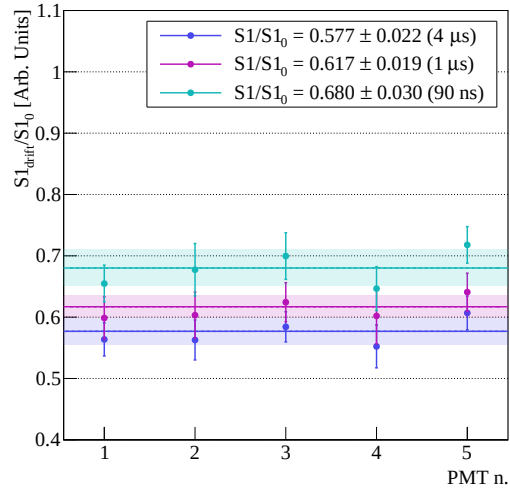
Figure 4.16.: Measurement of the S_{1,\text{drift}}/S_{1,0} ratio PMT-by-PMT obtained integrating the S1-charge in 90 ns (cyan), 1 \mu\text{s} (magenta), and in 4 \mu\text{s} (blue).
