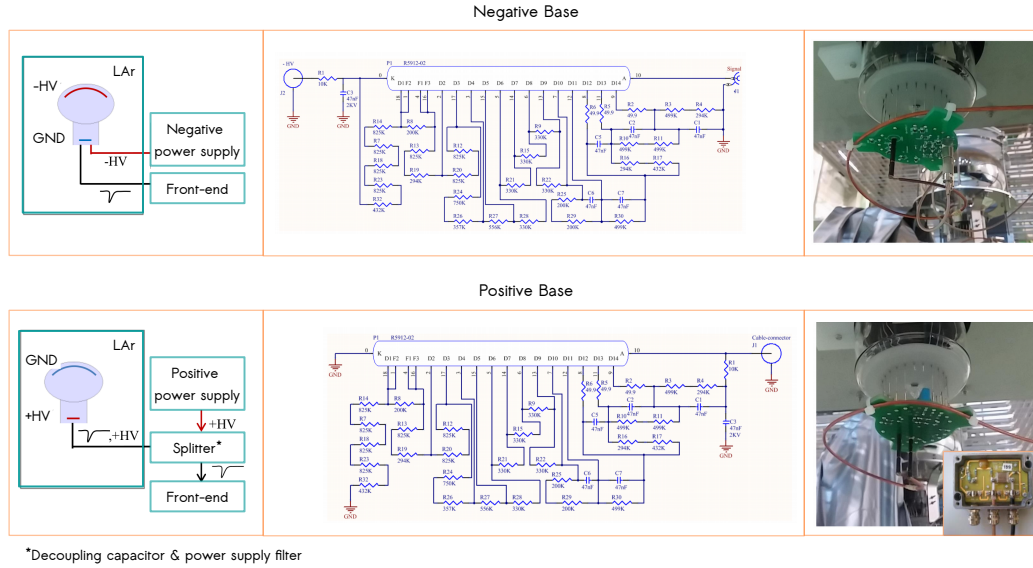
Figure 3.8.: Schematic description ( left ), dynodes diagram ( middle ), and two pictures ( right ) of the negative base (NB) ( top ) and the positive-base (PB) ( bottom ) configurations installed in the WA105 DP demonstrator.
