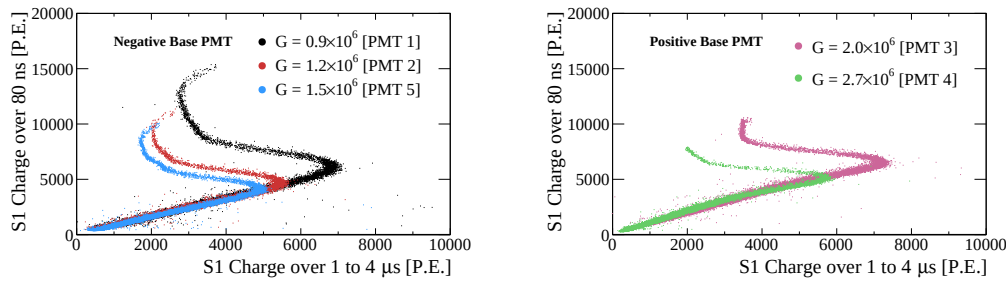
Figure 3.22.: Typical correlation of the integrated S1-charge over 80 ns (y-axis) and in the [1; 4] \mu\text{s} range (x-axis), both expressed in P.E.; given the shape of the correlation the effect has been named comet-effect . The effect is visible in both base configurations, NB on the left and PB on the right ; the result is related to the PMTs operation with gain of \sim 10^6 .
