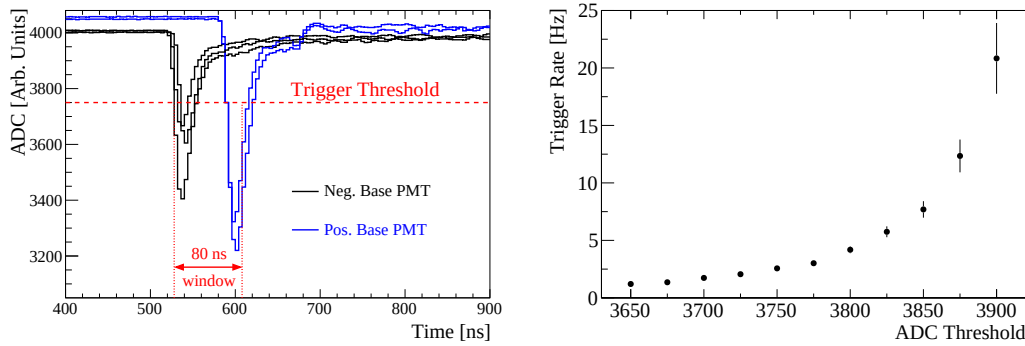
Figure 3.16.: Left: PMT self-trigger configuration illustrated considering the waveforms detected in one raw event. Right: Trigger rate shown as a function of the ADC threshold set to the five PMTs.
