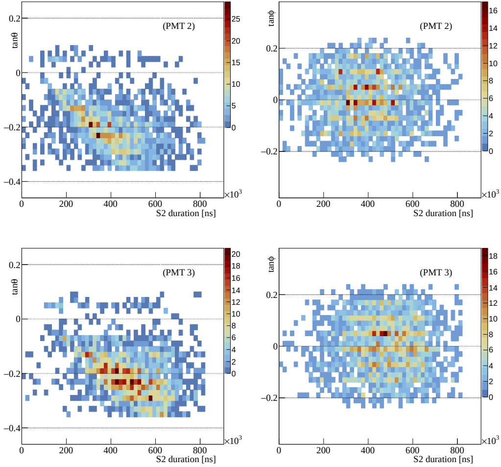
Figure A.9.: Correlation of the S2 duration with the track topology expressed in terms of the \tan\theta ( left ) and \tan\phi ( right ) distributions; as an example, results from PMT-2 and PMT-3 are shown, the behavior is confirmed by all PMTs.
