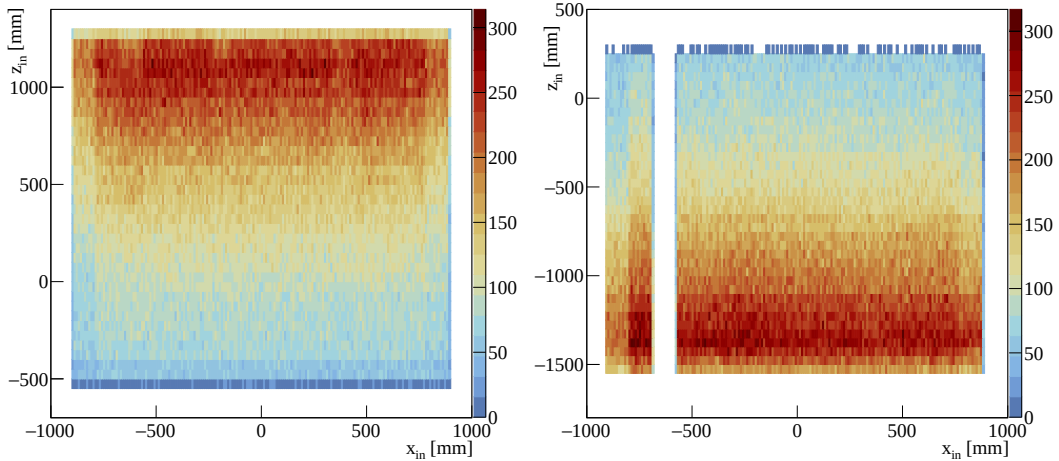
Figure 5.6.: CRT-maps corresponding to the upper panel ( wall-side , on the left ) and the lower panel ( door-side , on the right ) obtained from \sim 61 hours of data taking in CRT-shifted geometry.
