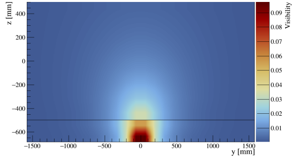
Figure 5.11.: Photon visibility in the y-z plane (at x = 0 ) for PMT-3. The loss of visibility due to photon absorption by the cathode is visible at z = -500 mm [223].
