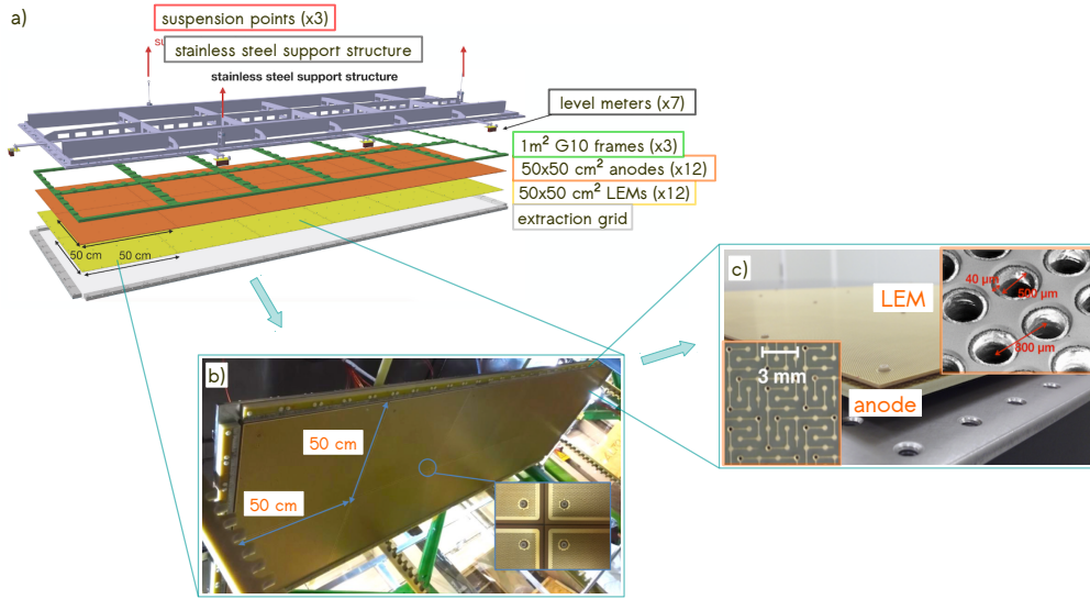
Figure 3.4.: Schematic view of CRP and main constituent components (a), bottom view of the twelve 50×50 cm 2 LEM units (b), and zoom of the anode and LEM structures (c). The images are taken from [78].
