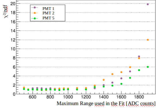
Figure 3.20.: \chi^2 minimization developed to identify a common cut rejecting all the events saturating the PMT response. For this specific purpose, the S1-amplitude is expressed in ADC counts.
