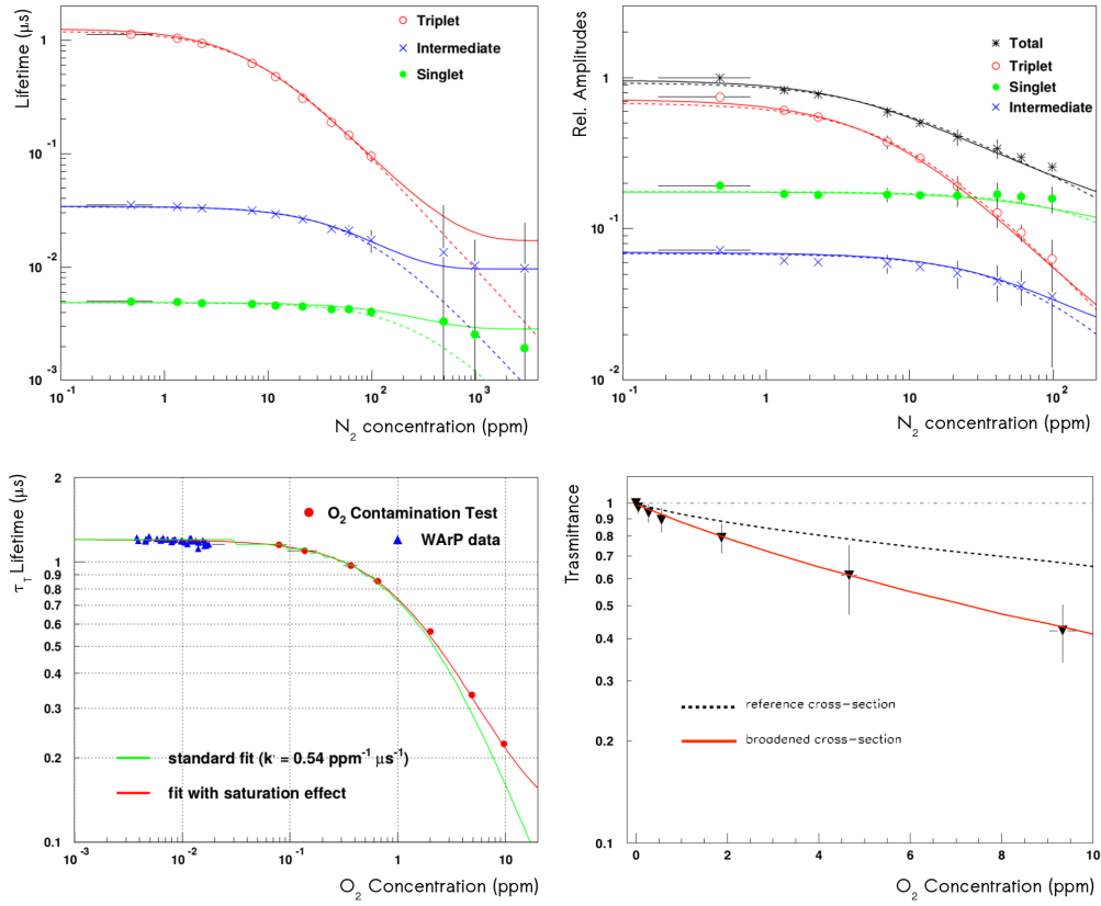
Figure 2.6.: Values of the \tau_1 decay times in presence of N_2 (top-left) and O_2 (bottom left) impurities studied at different concentrations. According to Eq. (2.19b), also the relative probability amplitudes are affected by the presence of impurities; the effect of N_2 is reported in the (top-right). In the (bottom-right), the effect of increasing O_2 concentrations on the VUV photon transmittance is reported. The plots are taken from Ref. [152] and [143].
