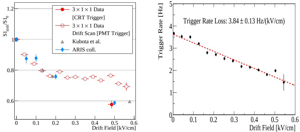
Figure 4.17.: Left: Measurement of the S_{1,\text{drift}}/S_{1,0} ratio in the data of the drift field scan using the PMT self-trigger. Right: Measurement of the PMT self-trigger rate as a function of the drift field strength for the same set of data.
