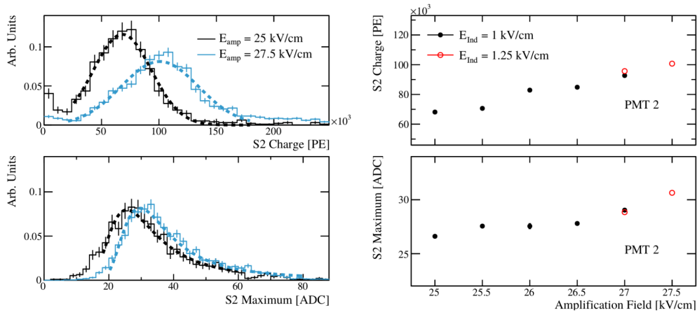
Figure 6.9.: Left: Reconstructed S2-charge ( top ) and S2-amplitude ( bottom ) spectra, under two different amplification field strengths; as an example, results from PMT-2 are reported. Right: Both observables are shown as a function of the amplification field, for PMT-2, in two different induction field conditions [223].
