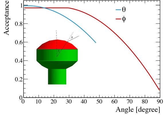
Figure 5.5.: Characteristic dependence of the PMT acceptance with the incident angles of the VUV photons [223].
