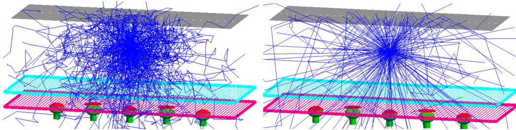
Figure 5.10.: Description of the light propagation inside the WA105 DP demonstrator when the simulated Rayleigh scattering length is of 20 cm ( left ) or 163 cm ( right ) [223].
