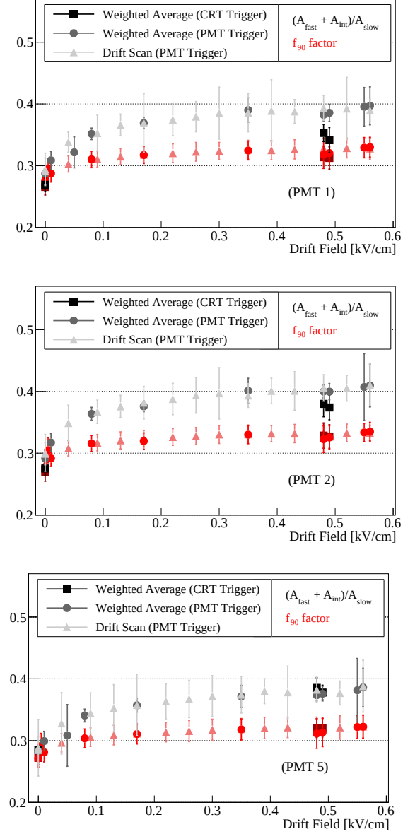
Figure 4.20.: Comparison of the f_{90} factor (red points) and the (A_{fast} + A_{int})/A_{slow} ratio (in grey) dependences with the drift field strength measured in the NB PMTs.
