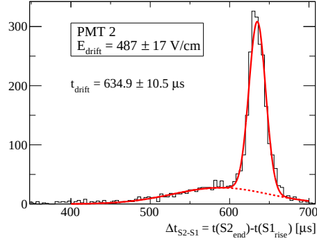
Figure 6.7.: Measurement of the drift velocity, including data triggered by the PMT self-trigger, considering a muon-like event selection based on the track reconstruction in the anode-plane [223].
