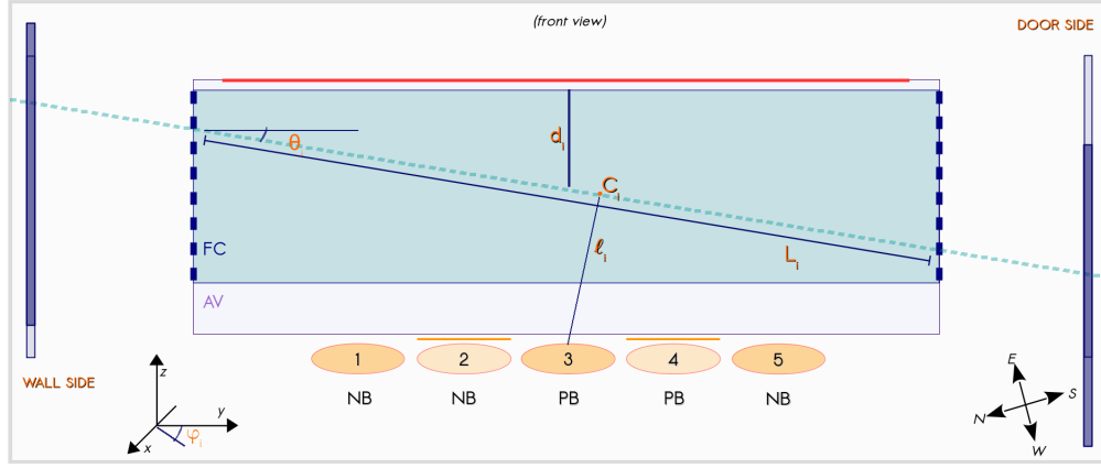
Figure 3.11.: Descriptive sketch (not scaled) of the track reconstruction given by the CRT external system trigger; the two CRT geometries are reported.
