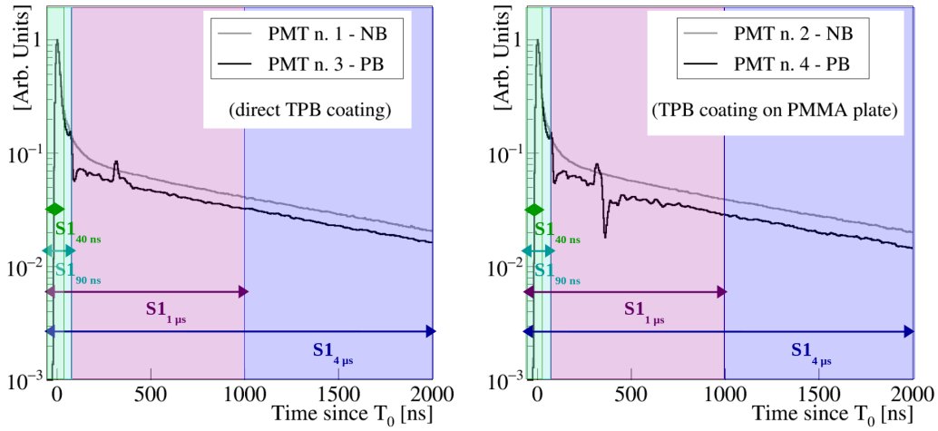
Figure 3.31.: Average waveforms of the NB (in grey) and PB (in black) PMTs, in the two WLS configurations. In both cases, the colored rectangles correspond to the integration ranges: 40 ns (green), 90 ns (cyan), 1 \mu s (magenta), and 4 \mu s (dark blue). Left: PMTs with TPB direct coating. Right: PMTs with the TPB coating on the PMMA plate.
