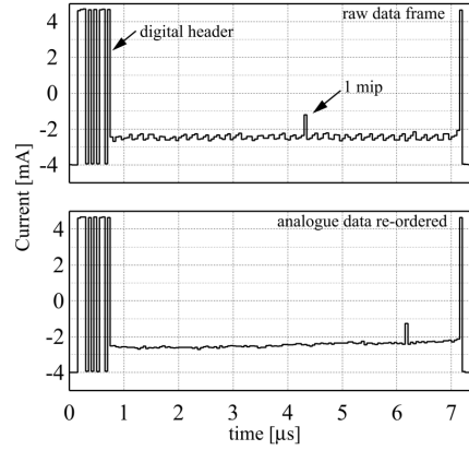
Figure 2.4: An example APV data frame[57] (top) and the same frame if the data are re-ordered by channel number (bottom). The frame is started with a 12 bit header followed by 128 channels of unordered analogue data while a tick mark indicates the start of the next cycle. Pedestals are clearly visible on each APV channel while the re-ordered data show there is a slight baseline droop across the chip.
