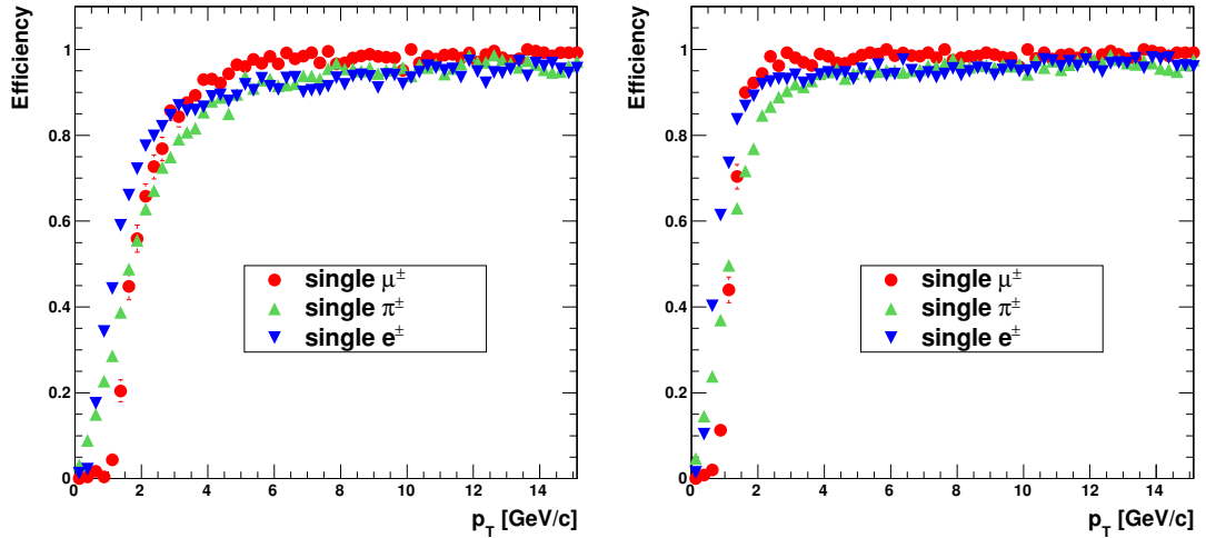
Figure 4.7: p_T discrimination performance for single \mu^\pm , \pi^\pm and e^\pm tracks using a stacked layer at 25 cm in the untilted configuration with a 2 mm sensor separation; Left: for a correlation window of 3 pixels, Right: for a correlation window of 5 pixels.
