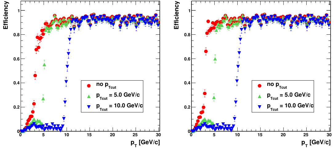
Figure 4.22: p_T discrimination performance using a double stack geometry for single \pi^\pm tracks where; Left: the individual stacks use a tight correlation window of 3 pixels, and Right: the individual stacks use a loose correlation window of 5 pixels.
