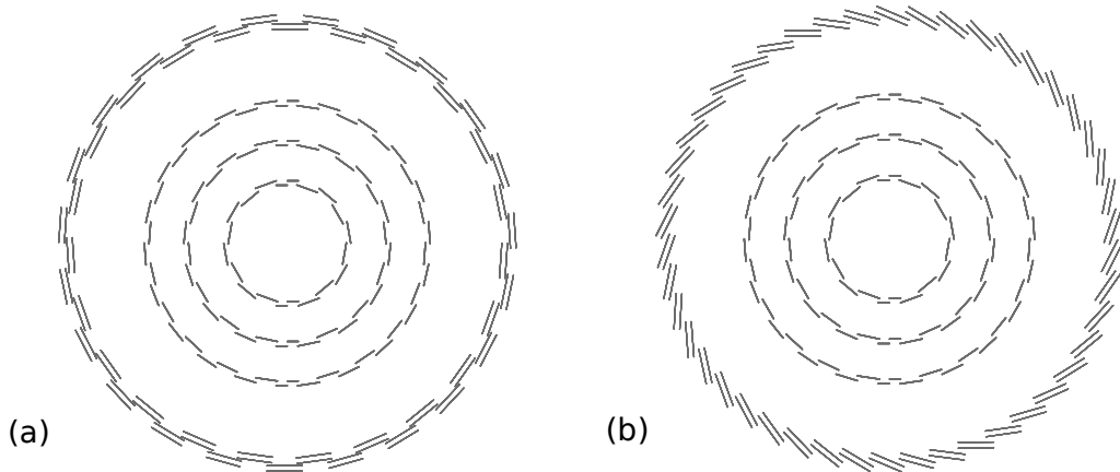
Figure 3.10: An r - \phi view of the current CMS pixel sensor arrangement and one stacked pixel layer; (a) illustrates the stacked sensor ladders arranged in an in-out layout, (b) demonstrates the tilted arrangement of stacked sensor ladders in r - \phi .
