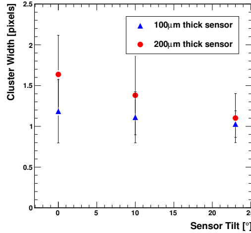
Figure 3.12: Simulated variation of cluster width in r - \phi as a function of sensor thickness and sensor tilt angle relative to the normal of the radial axis. A tilt of 23^\circ is equivalent to the Lorentz angle for electrons in current CMS pixel sensors operating under a bias voltage of V_{bias}=150 V. Results are for p_T=4 GeV/c muon tracks impinging on a pixel layer at 25 cm with 100\mu\text{m} pitch in r - \phi .
