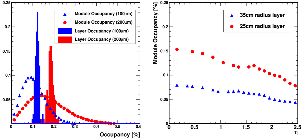
Figure 4.1: Left: Layer and module occupancy distributions for a layer at 25 cm. Right: Average module occupancy as a function of module position in \eta for layers at 25 cm and 35 cm. Results are for SLHC pileup conditions (minimum bias events with an average pileup of 400 interactions per bunch crossing) and untilted sensors.
