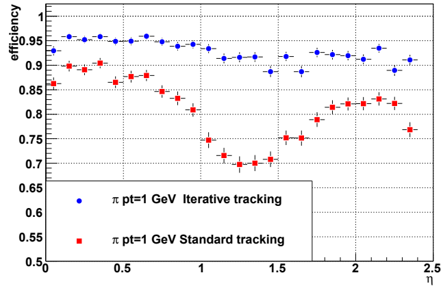
Figure 1.13: Track reconstruction efficiency for p_T=1\text{ GeV}/c pions as a function of pseudorapidity[32]. The two efficiencies are from two different tracking algorithms. The Iterative Tracking algorithm allows recovery of pions which interact in the high material regions by reconstructing tracks using looser criteria and better seeding without the expected increase in fake rate or reconstruction time.
