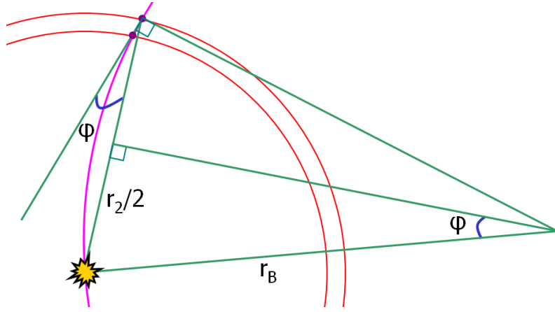
Figure 3.5: Determination of track transverse momentum by reconstruction of the crossing angle \phi using a pair of closely separated layers at radii r_1 and r_2 . [62]
