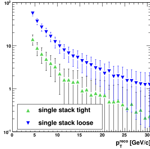
Figure 4.26: Average distribution of combinatorial fake tracks per event under SLHC conditions as a function of their reconstructed transverse momenta for both tight (3 pixel) and loose (5 pixel) individual stack correlation cuts. The p_T cut is set at 4 GeV/c.
