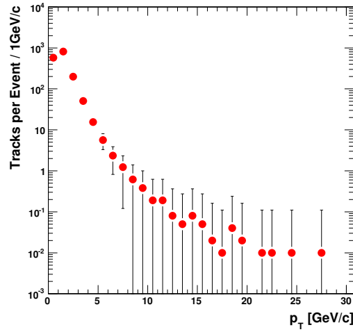
Figure 4.17: The p_T spectrum (normalised per event) for all minimum bias particles that generate stubs in a stacked layer placed at a radius of 25 cm with 1 mm sensor separation under SLHC conditions. Over 80% of generated stubs are from tracks with transverse momentum below 2\text{ GeV}/c .
