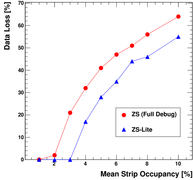
Figure 2.12: Fraction of triggers blocked by the tracker readout system due to rate throttling, as a function of the simulated event occupancy[72].
