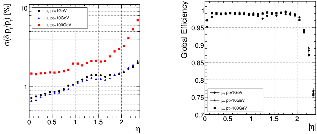
Figure 1.12: Left: Transverse momentum resolution of single muons (at p_T=1,10 and 100\text{ GeV}/c ) in the SST as a function of pseudorapidity[11], and Right: Track reconstruction efficiency for muons (at p_T=1,10 and 100\text{ GeV}/c ) as a function of pseudorapidity[11].
