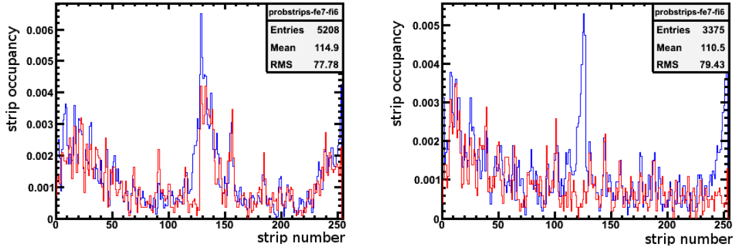
Figure 2.13: Average strip occupancy for a pair of APVs from a single fibre for low (Red) and high (Blue) trigger rates. There is a clear channel dependence. The figure on the right demonstrates that copper shielding between modules and the power bus[73] does not reduce the noise at high trigger rates[74].
