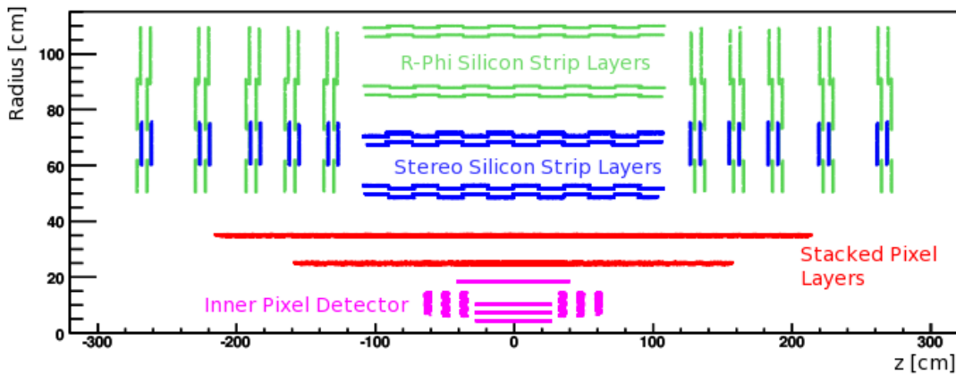
Figure 3.16: The concept tracker geometry, providing coverage over the range |\eta| < 2.5 . The simulated geometry also includes inactive material including cabling and cooling services, structural support and readout electronics, all of which are not displayed here.
