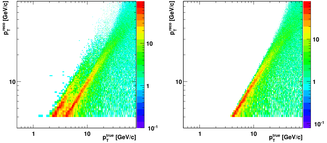
Figure 4.29: Distribution of Monte-Carlo track transverse momentum ( p_T^{\text{true}} ) and measured transverse momentum ( p_T^{\text{reco}} ) for single e^\pm tracks reconstructed by the double stack and passing the 4 GeV/c p_T cut. Left: for all tracks, and Right: for tracks only originating from the beam spot. The individual stacks use a tight correlation window of 3 pixels.
