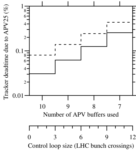
Figure 2.8: Tracker deadtime as a function of the control loop size and the maximum number of APV buffers available when operating in deconvolution mode. The deadtime calculated when the real APV is used is given by the dashed line. The solid line indicates the deadtime when the simulated APV is used[69]. The simulated APV offers increased efficiency since the buffer counter can be decreased as soon as the internal pipeline FIFO is cleared while the FPGA must wait for the detection of the three APV frame start bits (Figure 2.4) when using the real APV.
