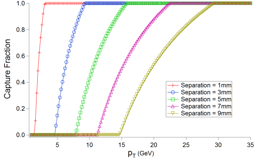
Figure 3.7: p_T discrimination performance of an ideal stacked pixel layer using a toy Monte-Carlo simulation[62]. Results are for a layer at 10 cm with pixel dimensions of 20 \times 50 \mu\text{m}^2 ( r\phi \times z ) and a search window of \pm 1 pixel.
