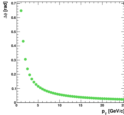
Figure 4.16: \phi difference ( \Delta\phi ) between the straight line projection of a stub (at radius 25 cm) from the origin to the calorimeter surface and the true impact point of the track at the ECAL as a function of p_T for the barrel region only. For tracks with p_T < 6.5 GeV/c, the resolution is larger than that of a trigger tower.
