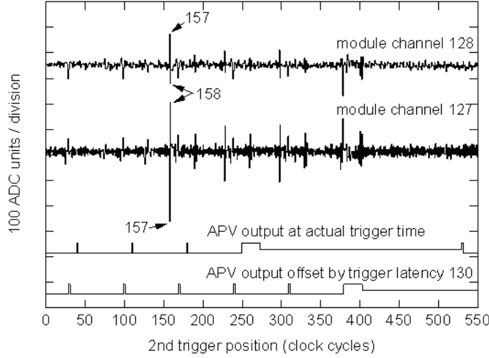
Figure 2.14: Pedestal fluctuations on the most affected APV channels showing a dependence on the spacing between two triggers (where the first trigger occurs at -3)[74]. After taking the L1 latency into account, it can be seen that the noise coincides with the readout operation of the first trigger, including the APSP sample and hold stage and the APV digital header at \sim 380 clock cycle spacing. The large fluctuations at \sim 158 clock cycle spacing correspond to the APSP readout of the first triggered pipeline sample.
