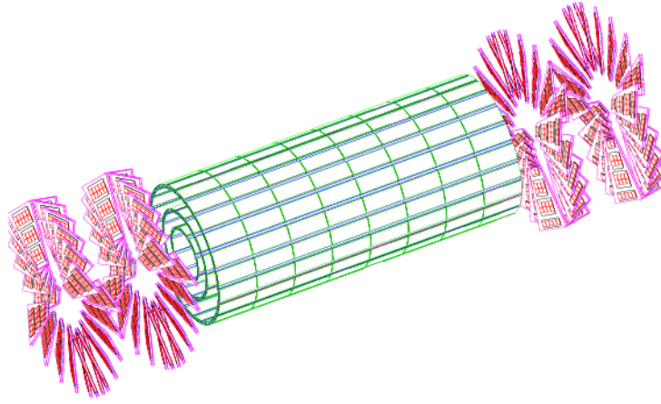
Figure 1.15: Layout of the CMS Pixel Detector[11].
