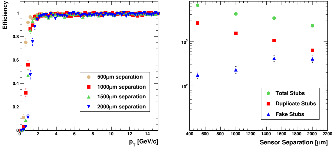
Figure 4.6: Left: p_T discrimination performance of a stacked layer for single \mu^\pm tracks and, Right: Average number of generated stubs per event under SLHC pileup conditions as a function of sensor separation where the correlation window is widened with sensor separation. Results are for a stacked layer at 25 cm in the untilted configuration. Compared to Figure 4.4, the p_T discrimination curve does not change with sensor separation, however the total number of stubs including duplicates and fakes does increase with sensor separation.
