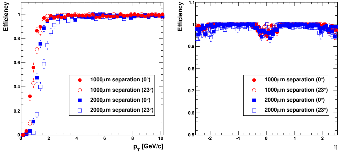
Figure 4.10: Left: p_T discrimination performance comparison of untilted and tilted sensors in a stacked layer at 25 cm. Right: Efficiency vs. \eta comparison of untilted and tilted sensors for tracks with p_T > 2 GeV/c using a stacked layer at 25 cm. Results are for single \mu^\pm events and identical correlation cuts. The dip at \eta=0 is due to non overlapping stacked modules in the central region.
