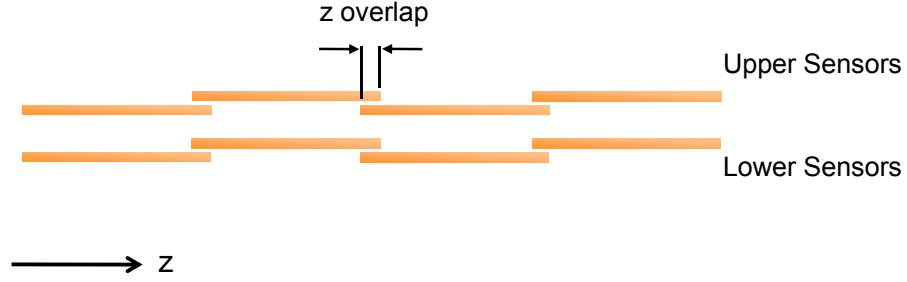
Figure 3.13: An overview of the sensor layout in r - z , demonstrating the overlaps between sensors in z .
