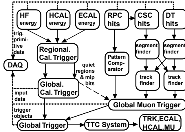
Figure 1.17: Control flow diagram of the L1 Trigger System[34].
