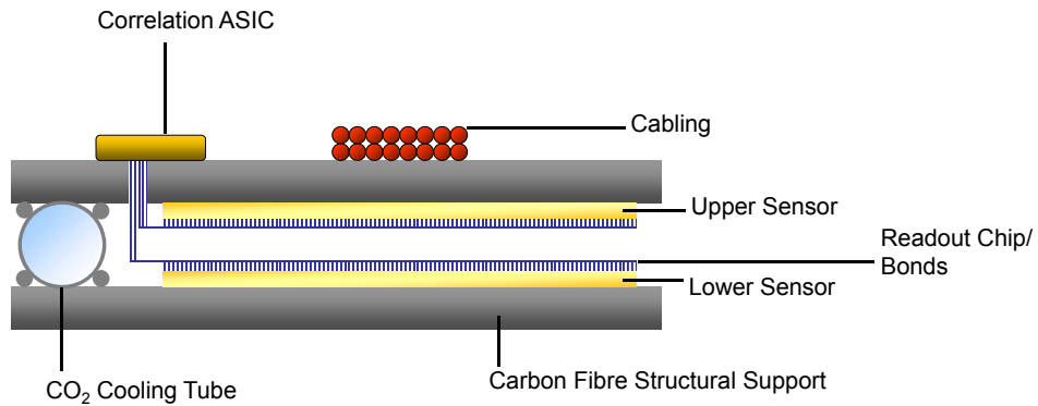
Figure 3.8: Strawman module layout in r - \phi as used in simulations including cooling, cabling and structural support.
