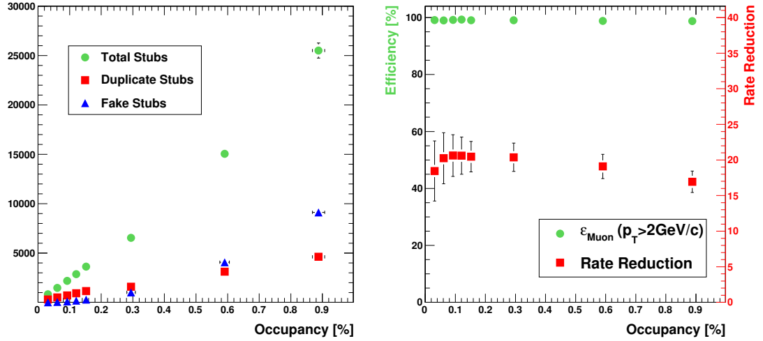
Figure 4.14: Left: Average number of generated stubs per event and, Right: Trigger efficiency for muons with p_T > 2 \text{ GeV/c} (left scale) and rate reduction factor (right scale) under SLHC pileup conditions as a function of average layer occupancy. Results are for a stacked layer at 25 cm in the untilted configuration and a sensor separation of 1 mm.
