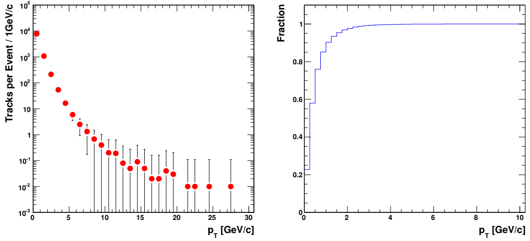
Figure 3.4: The p_T spectrum (normalised per event) for all minimum bias particles that leave hits in a sensitive layer placed at a radius of 25 cm and at an average pileup of 400 p-p interactions per event. The right hand plot indicates, as a fraction of all tracks, the number of tracks with transverse momentum less than the given p_T . Events were simulated within a magnetic field of 4 T and a coverage of |\eta| < 2.5 .
