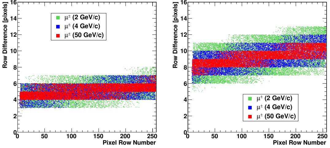
Figure 3.21: Pixel row difference (row difference between hit pixels on the upper and lower sensors) as a function of the hit pixel row on the upper sensor for 50, 4 and 2 GeV/c \mu^\pm for a stacked layer at 25 cm in a tilted configuration using a 1 mm separation (left) and 2 mm separation (right). In order to correlate hits efficiently, an offset as a function of the active pixel row must be applied. This offset is also dependent on the sensor separation, sensor width, sensor tilt and layer radius.
