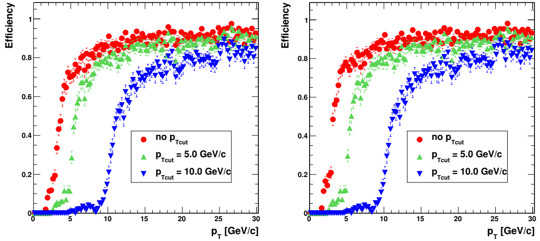
Figure 4.23: p_T discrimination performance using a double stack geometry for single e^\pm tracks where; Left: the individual stacks use a tight correlation window of 3 pixels, and Right: the individual stacks use a loose correlation window of 5 pixels.
