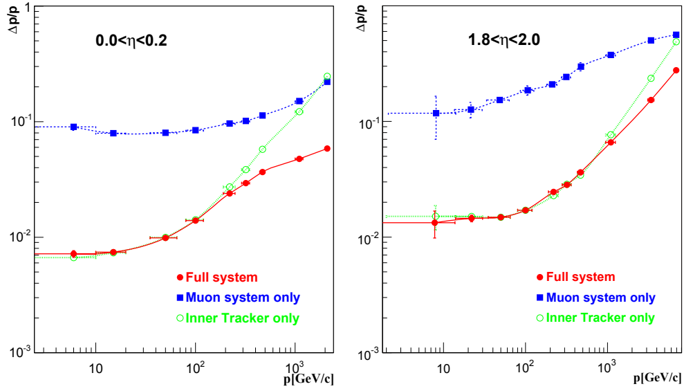
Figure 1.8: Muon momentum resolution as a function of momentum, using either the muon system only, the tracker only or the combined muon-tracker system in the barrel region 0 < |\eta| < 0.2 (left) and endcap region 1.8 < |\eta| < 2.0 (right)[11].
