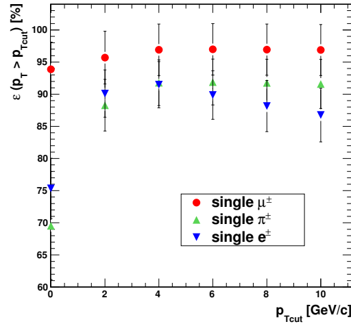
Figure 4.24: Global trigger efficiency for \mu^\pm , \pi^\pm and e^\pm tracks with reconstructed transverse momenta greater than p_{Tcut} , as a function of the p_T cut. Efficiencies, as defined as in equation (4.11), are calculated using tracks with Monte Carlo transverse momentum p_T > p_{Tcut} and a Monte Carlo track distribution flat in p_T from 0 to 50 GeV/c. In this case, the individual stacks use a tight correlation window of 3 pixels.
