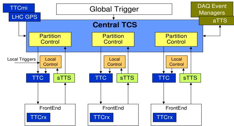
Figure 2.1: An overview of the Trigger Control System including the Trigger, Timing & Control (TTC) network and Trigger Throttling System (sTTS)[50]. Individual partitions can be controlled by a Local Trigger Controller (LTC) which provides the same functionality as the Global Trigger Controller except it can obtain triggers from the relevant local subdetector. In this way, partitions can be operated separately if the central TCS is down for maintenance.
