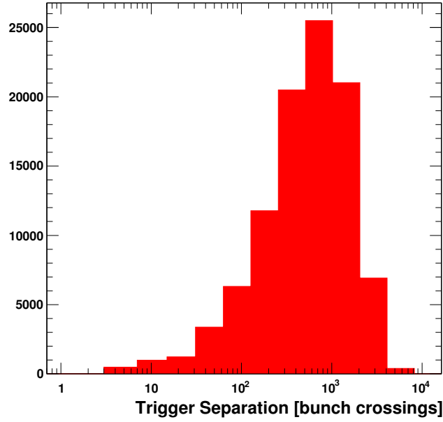
Figure 2.11: Throttled trigger distribution as measured by the APVe during a integration run with the GTC configured to generate pseudo-random Poisson triggers at a mean rate of 100 kHz.
