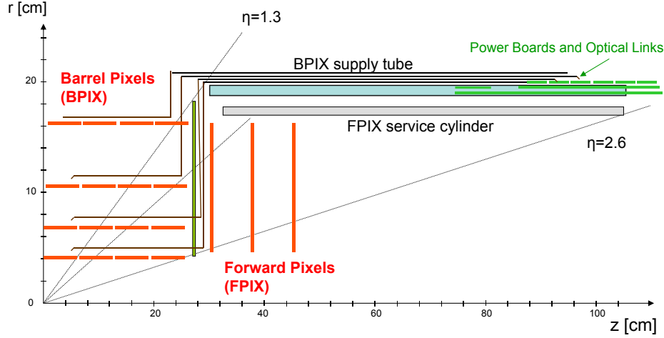
Figure 1.19: Proposed Phase I pixel upgrade. The new pixel system will comprise 4 barrel layers and 3 endcap disk pairs, lighter mechanics and cooling and more inactive material will be placed outside of the tracker coverage.
