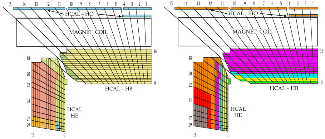
Figure 1.20: Readout segmentation in the current HCAL (left) and proposed Phase I HCAL (right)[44]. Energy deposition per tower will be measured at 4-7 different depths using Silicon Photo Multipliers. The number of segments is limited by the readout bandwidth of the upgraded HCAL which is set by the fixed volume for cabling.
