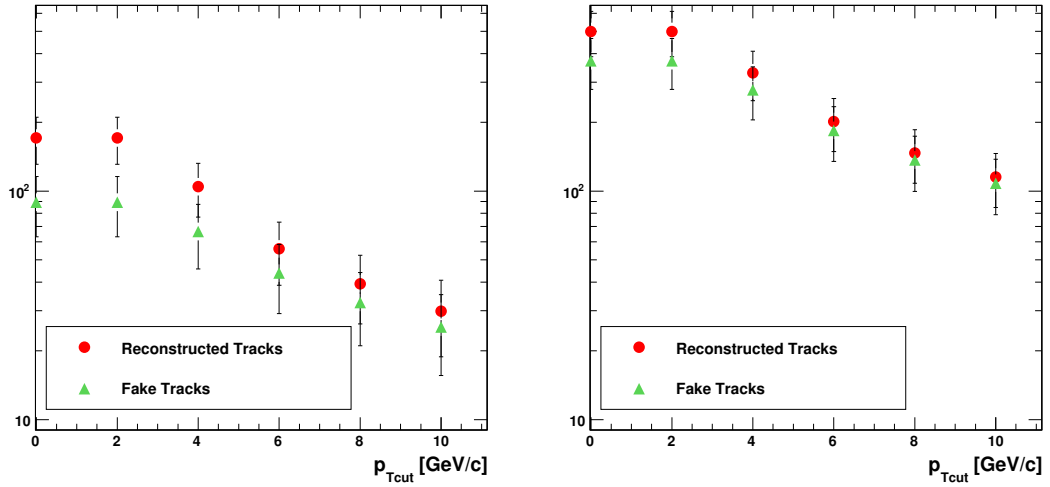
Figure 4.25: Average number of total and fake reconstructed tracks per event under SLHC conditions as a function of the p_T cut where; Left: the individual stacks use a tight correlation window of 3 pixels, and Right: the individual stacks use a loose correlation window of 5 pixels. The number of combinatorial fake tracks per event dominate the rate.
