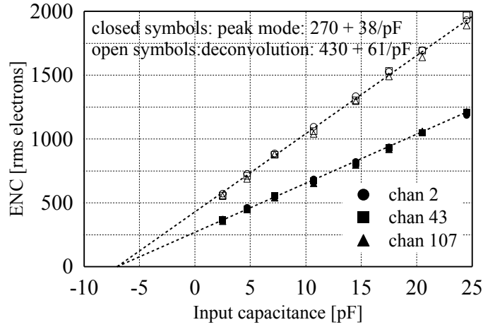
Figure 2.3: Measured noise dependence on input capacitance for the APV25 in peak mode and deconvolution mode[30].
