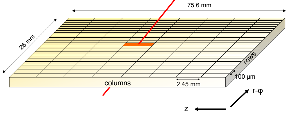
Figure 3.15: A schematic of the sensor layout and dimensions. Pixel rows are defined along the r\text{-}\phi axis and columns along z .
