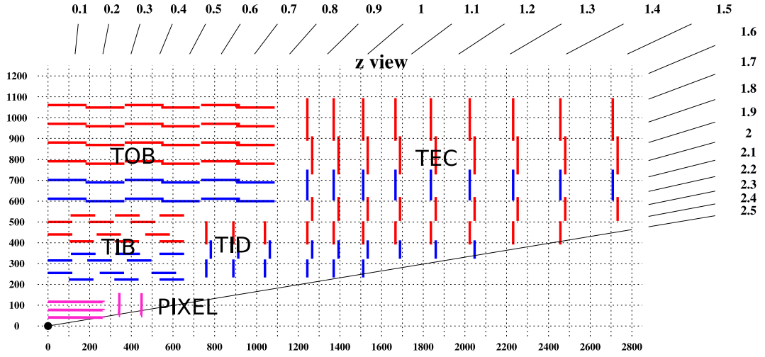
Figure 1.11: Schematic of the CMS Tracker. A quarter section is displayed with the interaction point at the bottom-left corner. The SST is made up of individual modules - indicated here by the straight red and blue lines. Each module consists of either 1 or 2 silicon sensors as well as associated readout electronics. The blue modules are double sided so that a stereo r - \phi and r - z measurement can be performed. The red modules are single sided. Scale is in mm, with units of pseudorapidity indicating the angular coverage[11].
