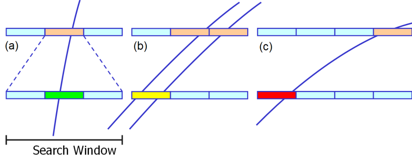
Figure 3.6: Reconstruction of the track crossing angle using a stacked pixel layer[62]. A high p_T track will intersect the layer virtually perpendicular to the sensor. In this case (a), the hits fall within the search window and the correlation reveals a high p_T track. Tracks with lower transverse momenta intersect the layer at shallower angles and hence may (b) either pass or fail the correlation depending on the impact point on the sensor or (c) or always fail the correlation if the angle of incidence is too small.
