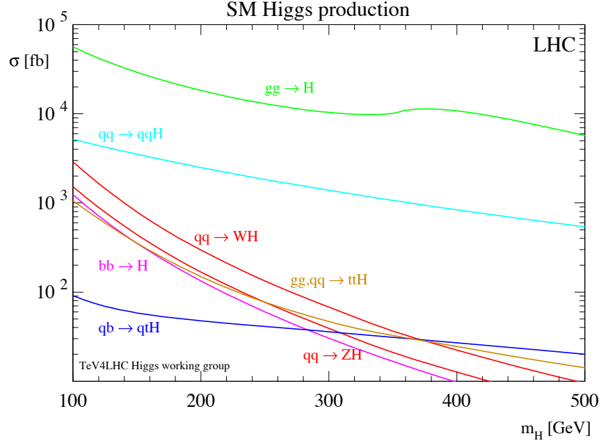
Figure 1.3: Standard Model Higgs production cross sections for pp collisions at the LHC where \sqrt{s}=14 TeV[17].
