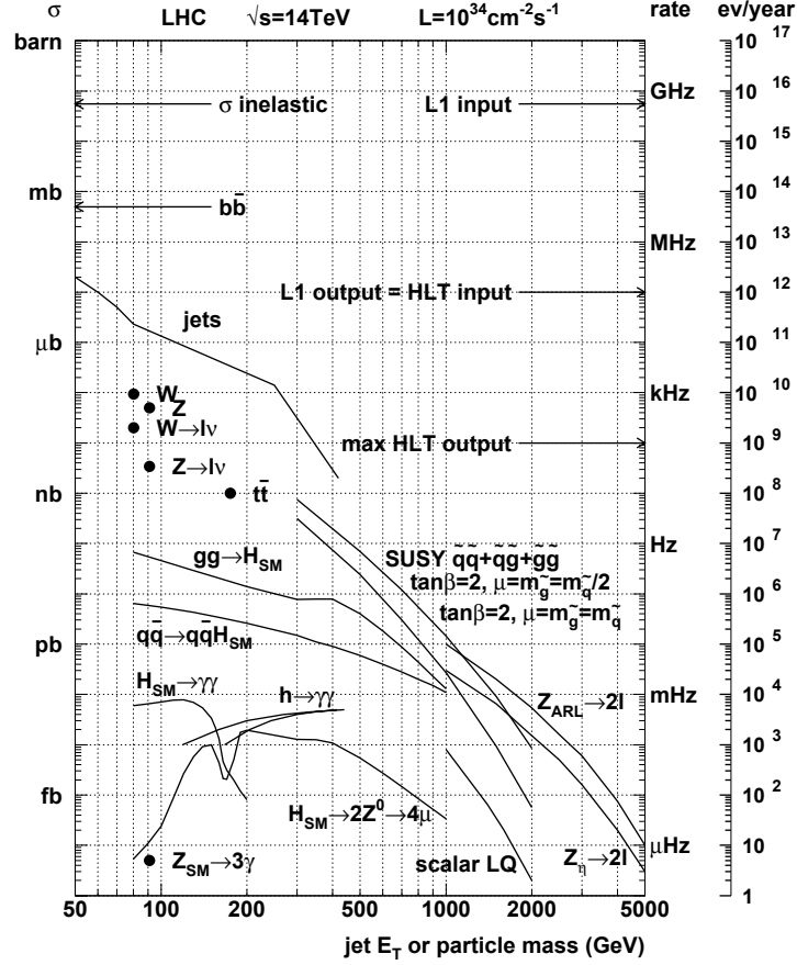
Figure 1.16: Inclusive proton-proton cross-sections as a function of particle mass (or jet E_T ) for some physics processes at LHC at 10^{34}\text{cm}^{-2}\text{s}^{-1} . Rates are provided on the right hand scale[34].
