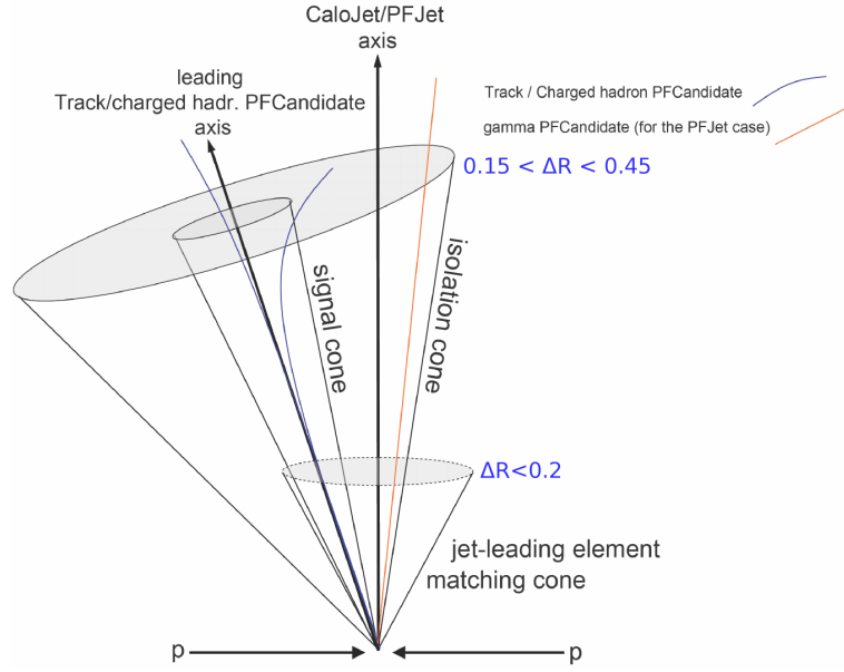
Figure 3.3: The \tau -jet HLT isolation cone algorithm[79]. The leading track within a cone of \Delta R < 0.2 about the L1 \tau -jet axis is identified and an isolation requirement is performed within the annulus 0.15 < \Delta R < 0.45 (variable) of the track. The leading track p_T cut is luminosity and algorithm dependent but is \sim 5 \text{ GeV} during pixel isolation and \gtrsim 15 \text{ GeV} after full track reconstruction[80].
