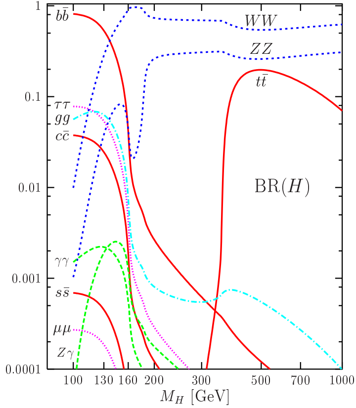
Figure 1.4: The decay branching ratios of the Standard Model Higgs boson as a function of M_H [19].
