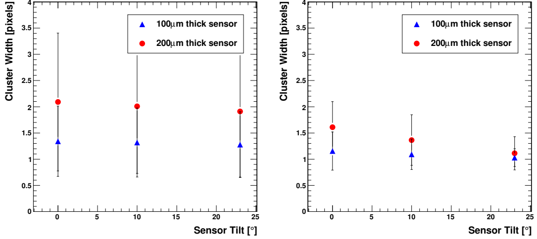
Figure 4.3: Cluster width r\text{-}\phi in as a function of sensor tilt and sensor thickness for a layer at 25 cm; Left: for minimum bias events, Right: for minimum bias events but where tracks have transverse momentum p_T > 2 \text{ GeV}/c .
