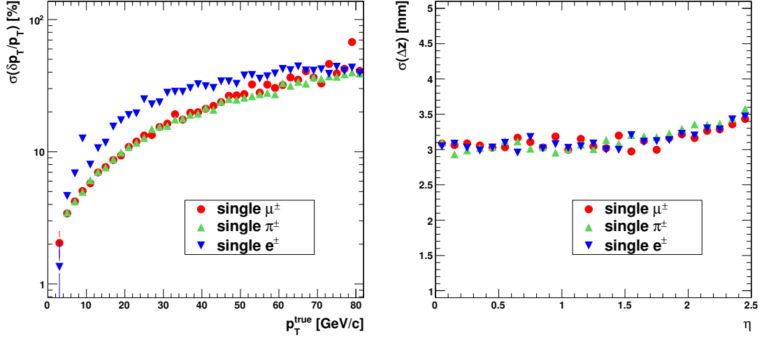
Figure 4.32: Left: Transverse momentum, and Right: z vertex (rms) resolutions for reconstructed \mu^\pm , \pi^\pm and e^\pm tracks using a double stack layer. Results are for real tracks passing the 4 GeV/c p_T cut and a tight correlation window of 3 pixels for the individual stacks.
