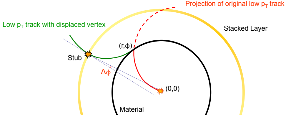
Figure 4.8: Origin of low transverse momentum background in pion events. Interactions with material in the inner detector can give rise to low p_T tracks that pass the correlation due to their displaced vertex. In this case, the reconstructed track crossing angle relative to the normal of the layer ( \Delta\phi ) is small enough to generate a stub even though the p_T of the original track would not have passed the correlation.
