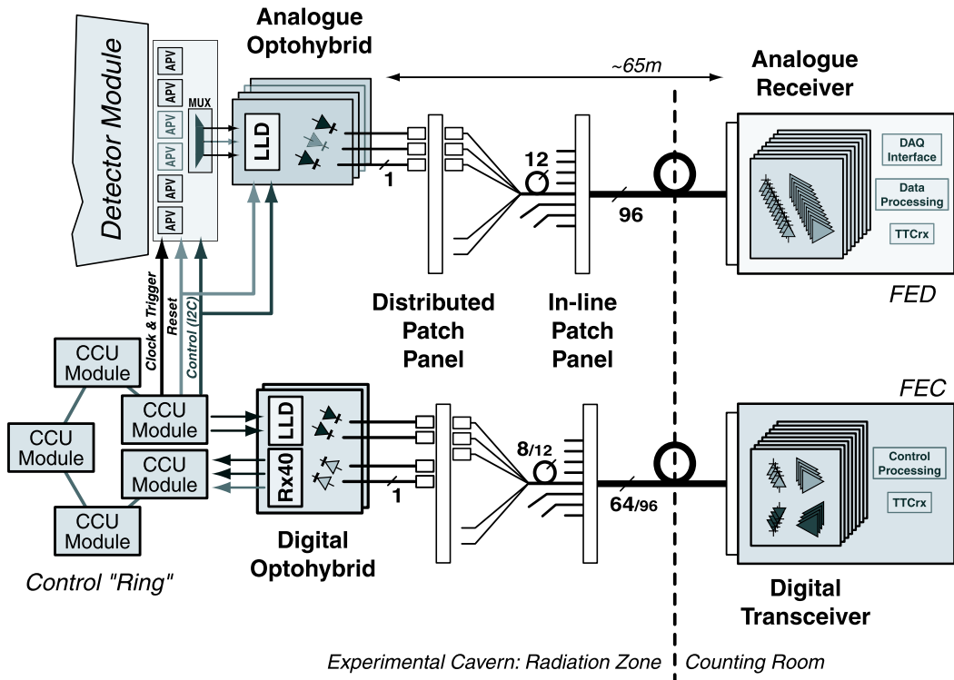
Figure 2.2: The CMS Tracker Front End control and readout architecture[55].
