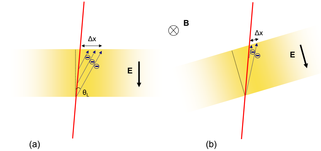
Figure 3.11: Illustration of the effect of Lorentz drift in sensors where electrons are the majority charge carrier; (a) in the untitled sensor case, (b) where the sensor is tilted to coincide with the drift angle. In the tilted case, the resulting signal spread ( \Delta x ) is smaller than it is for untitled sensors. The direction of the magnetic field ( \mathbf{B} ) is into the page.
