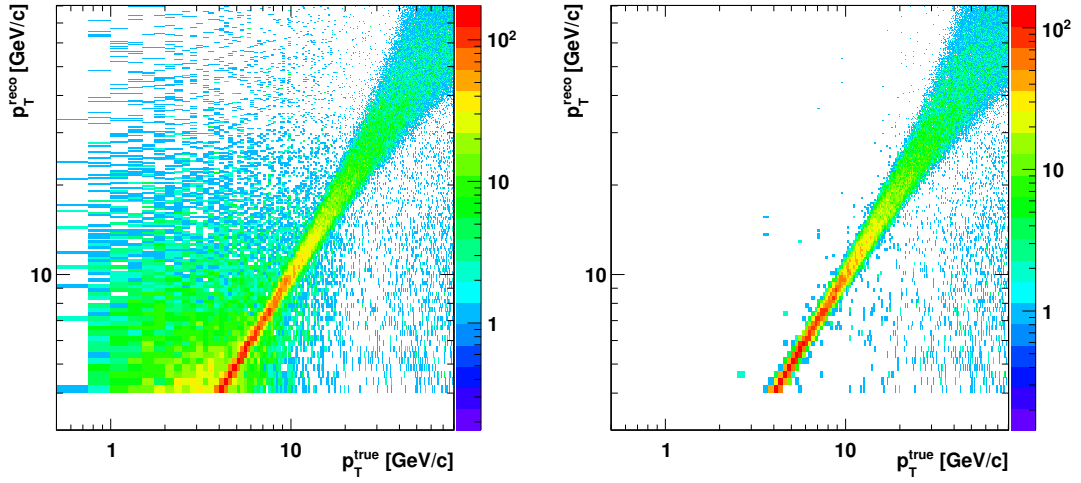
Figure 4.28: Distribution of Monte-Carlo track transverse momentum ( p_T^{\text{true}} ) and measured transverse momentum ( p_T^{\text{reco}} ) for single \pi^\pm tracks reconstructed by the double stack and passing the 4 GeV/c p_T cut. Left: for all tracks, and Right: for tracks only originating from the beam spot. The individual stacks use a tight correlation window of 3 pixels.
