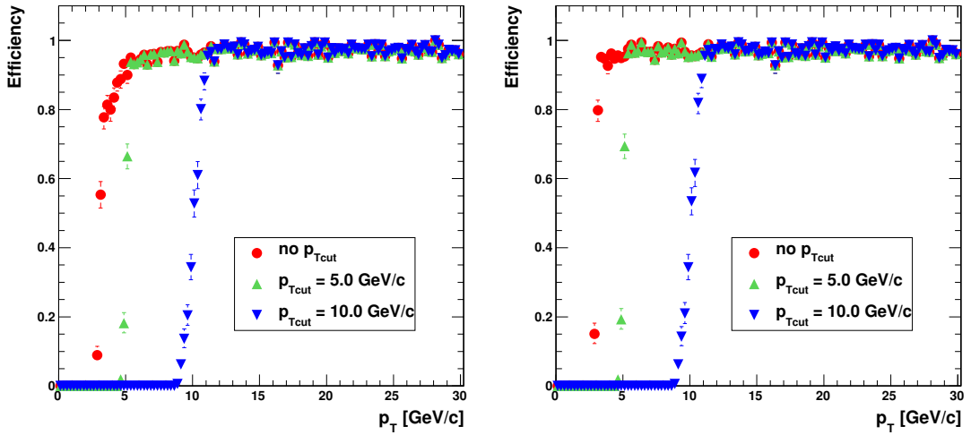
Figure 4.21: p_T discrimination performance using a double stack geometry for single \mu^\pm tracks where; Left: the individual stacks use a tight correlation window of 3 pixels, and Right: the individual stacks use a loose correlation window of 5 pixels. The performance is shown when no cut is placed on the reconstructed transverse momentum and then when a cut of p_T=5,10 GeV/c is used.
