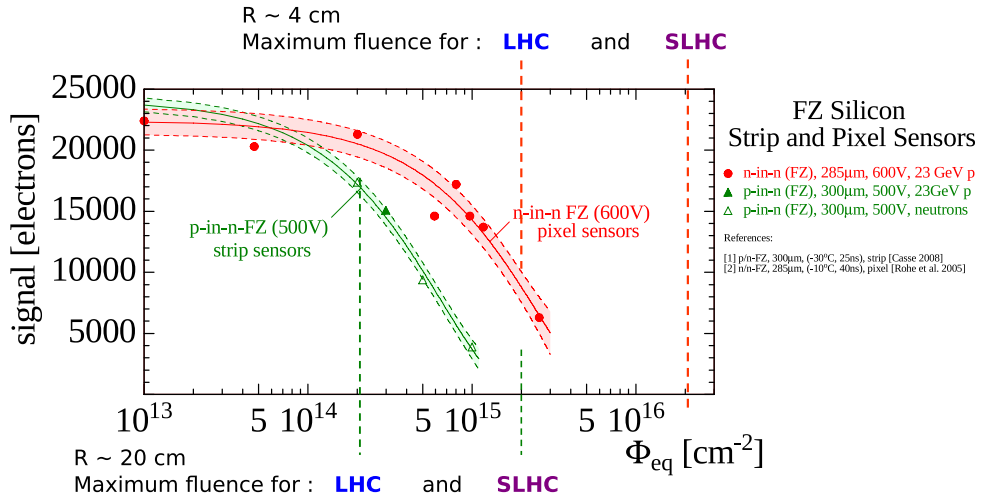
Figure 1.21: Signal performance of the current strip ( p^+ -on-n) sensors and pixel ( n^+ -on-n) sensors with fluence[45]. The current pixel sensor technology could be used at radii greater than 20 cm and provide sufficient signal for \sim 10 years at 10^{35} \text{ cm}^{-2} \text{ s}^{-1} . The exact performance will be determined by sensor parameters such as thickness and operation voltage, and the channel noise which is dependent on the sensor pitch, the leakage current and the performance of the readout electronics.
