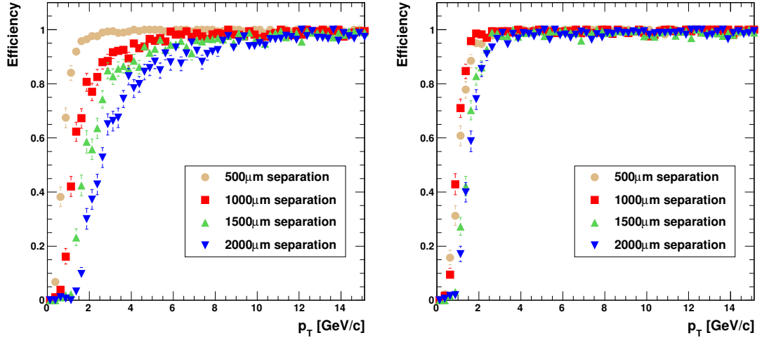
Figure 4.9: p_T discrimination performance for single \mu^\pm tracks using a stacked layer at 25 cm in the tilted configuration; Left: for a fixed 3 pixel correlation cut, Right: for variable correlation cuts.
