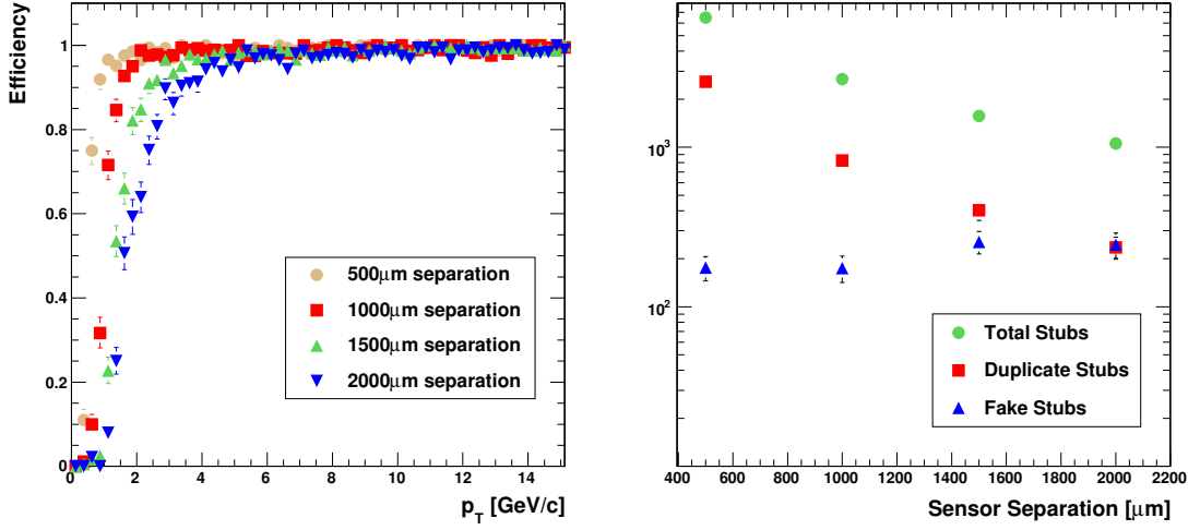
Figure 4.4: Left: p_T discrimination performance of a stacked layer for single \mu^\pm tracks at various sensor separations and a fixed 3 pixel row correlation window, Right: Average number of generated stubs per event under SLHC pileup conditions as a function of sensor separation. Results are for a stacked layer at 25 cm in the untilted configuration. Column window is 2 pixels for sensor separations of 1000 \mu\text{m} and less while a 3 pixel window is used for larger separations.
