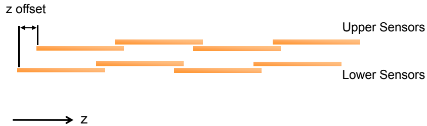
Figure 3.14: An overview of the sensor layout in r - z , demonstrating an applied offset between the upper and lower sensor layers to compensate for the increasing angle of incidence with \eta .
