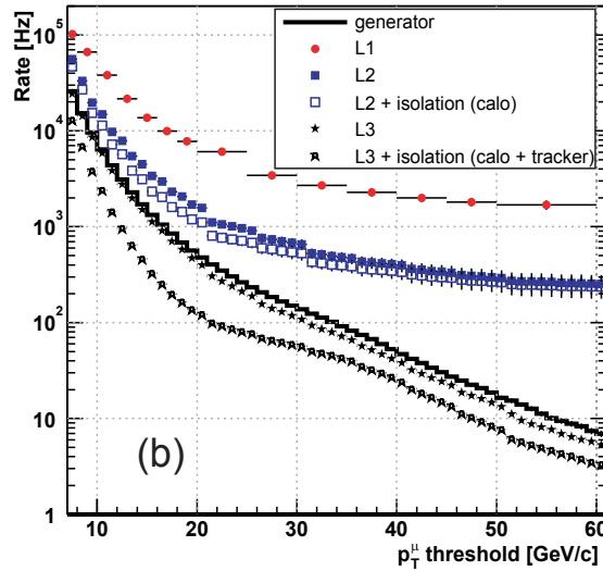
Figure 3.1: The HLT single-muon trigger rate as a function of applied p_T threshold at 10^{34}\text{cm}^{-2}\text{s}^{-1} [35]. At L3, the addition of tracking information to the trigger allows a significant rate reduction over the L1 and L2 rates due to the improved momentum resolution, especially at high transverse momenta.
