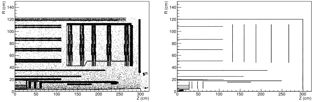
Figure 3.19: Distribution of vertices from electron bremsstrahlung for the Full (left) and Fast (right) simulations demonstrating the comparative interaction geometries.
