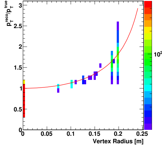
Figure 4.30: Relationship between ratio of reconstructed to true track transverse momentum p_T^{\text{reco}}/p_T^{\text{true}} to track vertex radius for single electron events. The p_T of the original electrons starting from the beam spot are well reconstructed although due to bremsstrahlung the transverse momentum can be underestimated. Electrons from photon conversions are reconstructed with increased p_T depending on the radius of their conversion vertex. An analytical calculation of the ratio (red curve) demonstrates good agreement.
