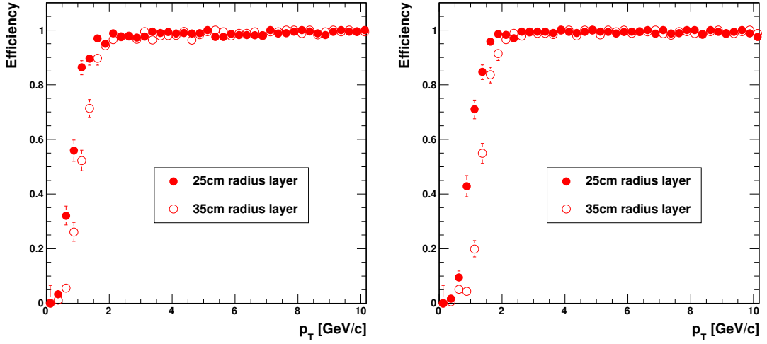
Figure 4.12: p_T discrimination performance for single \mu^\pm tracks using stacked layers at 25 cm and 35 cm; Left: in the untitled configuration, Right: when the sensors are tilted.
