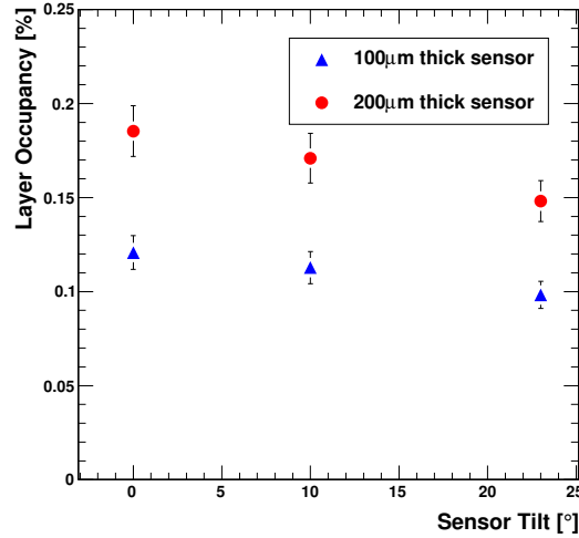
Figure 4.2: Average layer occupancy as a function of sensor tilt and sensor thickness for a layer at 25 cm. Results are for minimum bias events with an average pileup of 400 interactions per bunch crossing.
