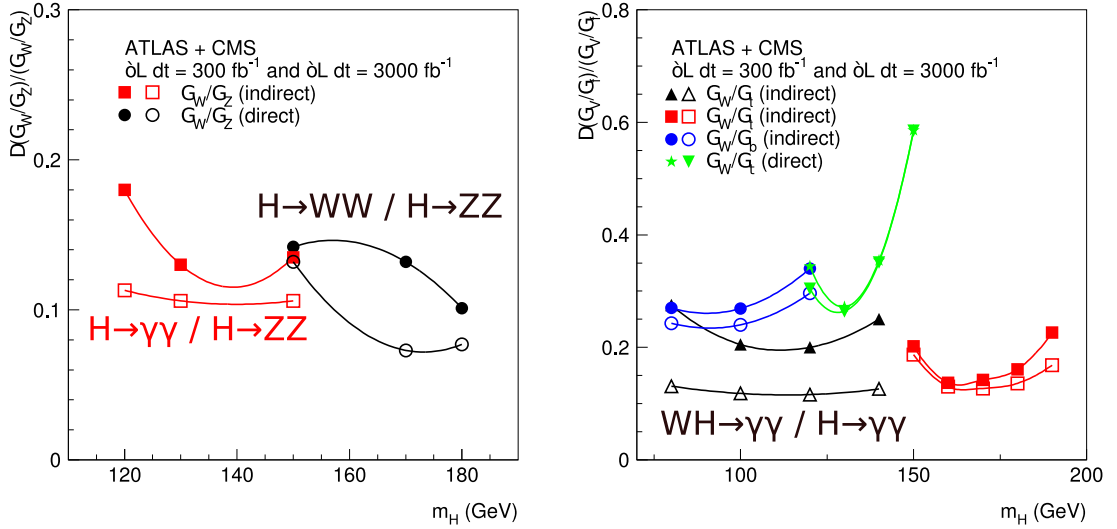
Figure 1.6: Expected uncertainties on the measured ratios of the Higgs widths to final states involving bosons only (left) and bosons and fermions (right), as a function of the Higgs mass for 300 \text{ fb}^{-1} (closed symbols) and 3000 \text{ fb}^{-1} (open symbols) integrated luminosity per experiment. The increased statistics will benefit the H \rightarrow \gamma\gamma and H \rightarrow WW channels the most, mainly improving the ratio of the HWW to HZZ and HWW to Ht\bar{t} couplings, either directly or indirectly (through the W loop in H \rightarrow \gamma\gamma ). The other couplings see limited improvement due to theoretical uncertainties on the absolute production cross sections at high M_H although this may improve in the future[24].
