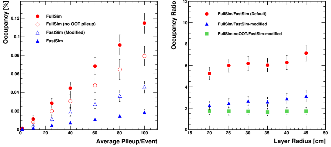
Figure 3.20: Left: Occupancy dependence on the average pileup per event for a stacked pixel layer at 25 cm and 200 \mu\text{m} thickness, Right: Variation of the FullSim to FastSim occupancy ratio as a function of stacked pixel layer radius where sensor parameters and layer coverage remain the same at each radius. The figures denoted by FastSim-default are provided by the default configuration of the Fast Simulation package. FastSim-modified indicates the results for the Fast Simulation where the minimum track p_T cut has been reduced to 50 MeV/c and looping tracks are fully propagated. FullSim-noOOT refers to occupancies generated by the Full Simulation where out-of-time pileup is not included in the event.
