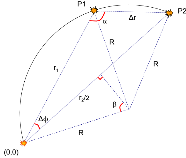
Figure 4.19: The three point reconstruction using two stub positions P1(r_1, \phi_1) , P2(r_2, \phi_2) and the assumed vertex position (0,0) . Using circle theorems, 2\pi - 2\beta = 2\alpha .
