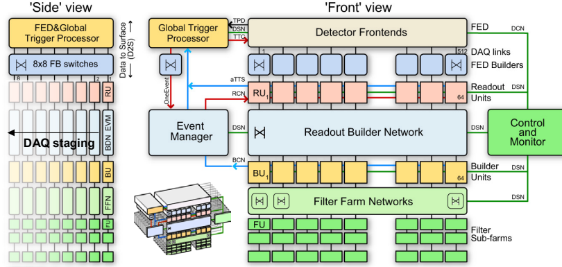
Figure 1.18: Overview of the CMS Trigger and Data Acquisition System[37]. Indicated are the Reader Units (RUs), Builder Units (BUs) and Filter Units (FUs) as well as the Detector Control Network (DCN) and DAQ Service Network (DSN) used by the Run Control/Monitor System (RCMS) for managing the DAQ. On the left, the ‘side’ view illustrates the principle of DAQ staging where ‘slices’ of the ‘front view’ DAQ will be gradually added until the full system is realised.
