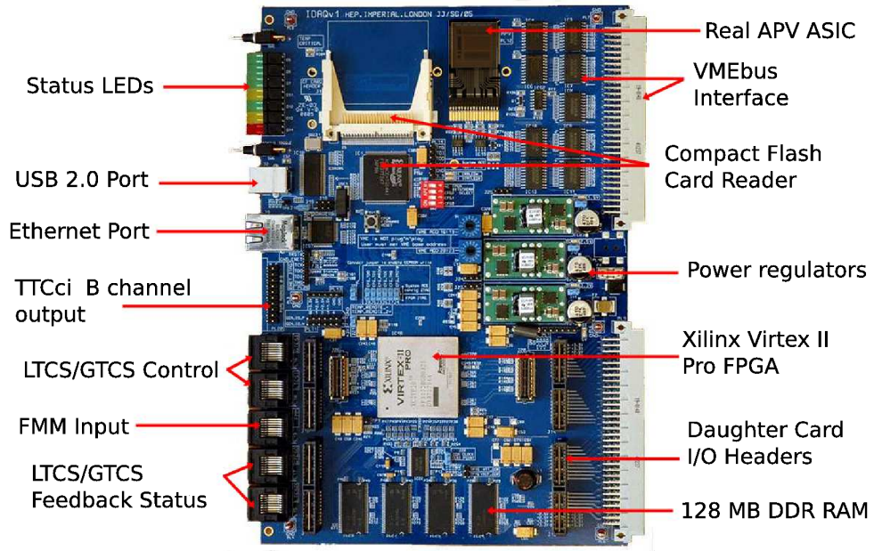
Figure 2.7: Layout of the APVE IDAQ card.
