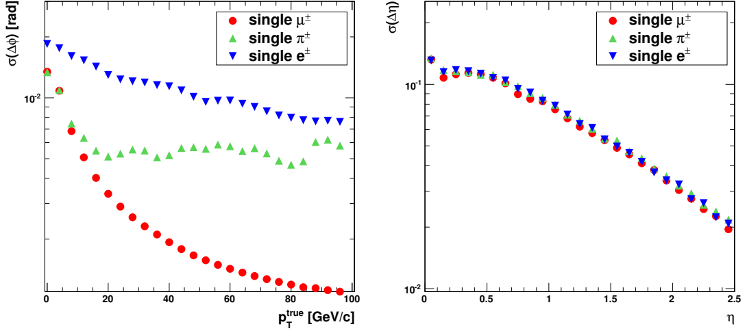
Figure 4.31: Left: \Delta\phi , and Right: \Delta\eta (rms) resolutions at the ECAL surface for reconstructed \mu^\pm , \pi^\pm and e^\pm tracks using a double stack layer. Results are for real tracks passing the 4 GeV/c p_T cut and a tight correlation window of 3 pixels for the individual stacks.
