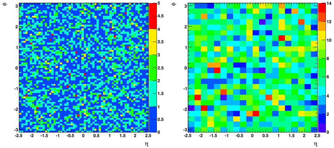
Figure 4.15: Distribution of stubs in; Left: approximate \eta - \phi trigger towers ( \Delta\eta\Delta\phi = 0.087 \times 0.087 ) or Right: approximate \eta - \phi ECAL trigger regions ( 3 \times 3 towers).
