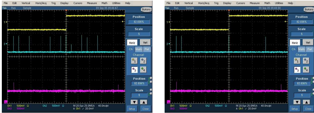
Figure 2.10: Examples of the APVe Ready to Out-Of-Sync output status (Yellow) transition[62]. The error occurs when no cyclical BC0 (Magenta) is detected at the APVe input. It can be seen that a L1A signal (Cyan) is received by the APVe instead.
