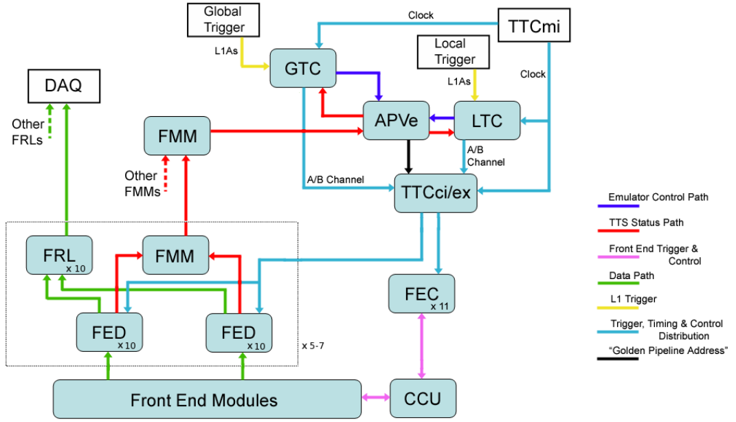
Figure 2.6: The Silicon Strip Tracker Readout and Control System and its interaction with the TCS (one partition). The marked region consisting of the FEDs, FMMs and FRLs is repeated 5-7 times depending on the partition size. There will be approximately 96-134 FEDs, 11 FECs, 5-7 FMMs and 50-70 FRLs per Tracker partition in the final system. All off-detector components are accessible via VMEbus and can therefore be controlled by RCMS and DCS through XDAQ.
