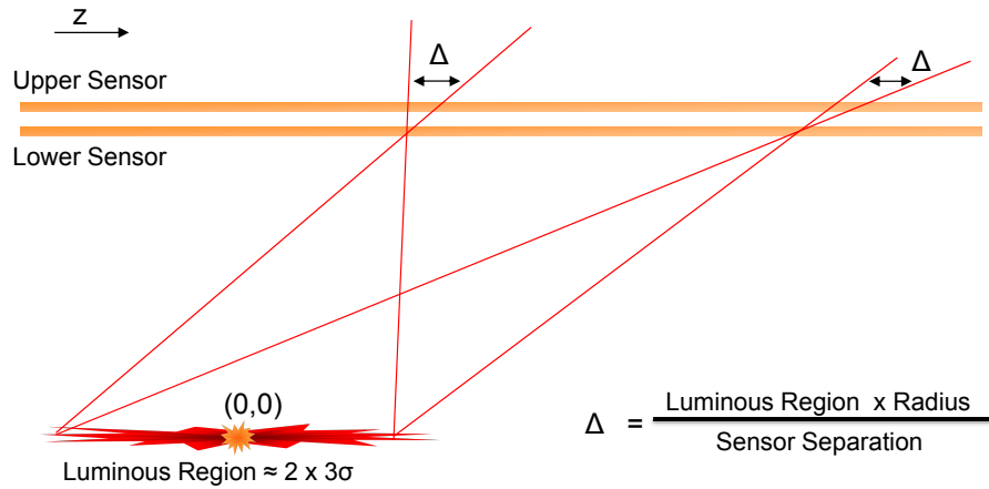
Figure 3.9: Illustration demonstrating the effect of the size of the luminous region on the spread of hit positions ( \Delta ) in a stacked layer.
