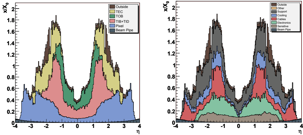
Figure 1.14: Tracker material budget in radiation lengths as a function of pseudorapidity by subdetector (left) and by material type (right)[26]. The majority of the material is taken up by cabling, cooling equipment, electronics and support structures.
