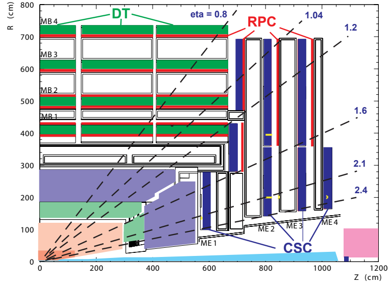
Figure 1.9: One quarter r-z section view of the CMS muon system for low luminosity running. RPC and CSC coverage will be extended after initial operation[11].
