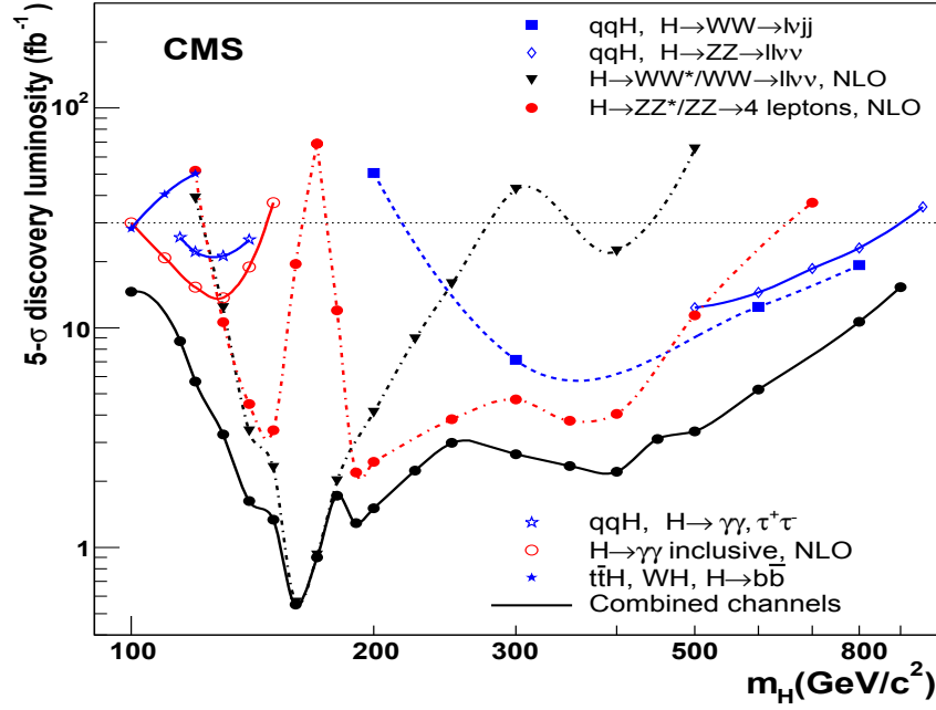
Figure 1.5: The required integrated luminosity needed to achieve a 5\sigma discovery signal in CMS using various detection channels as a function of M_H [19].
