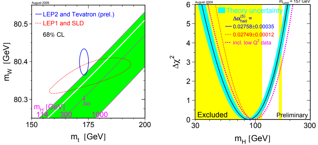
Figure 1.2: Left: Indirect constraints on M_W and m_t based on LEP-I and SLD data (dashed contour) and the direct measurements from the LEP-II and Tevatron experiments (solid contour) at 68% confidence. The shaded region corresponds to the dependence of M_H on these parameters.
