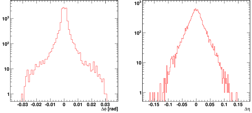
Figure 4.20: Distribution of; Left: \Delta\phi and Right: \Delta\eta difference between stubs on a stacked layer at 25 cm and another at 35 cm using single \mu^\pm tracks with p_T > 2 \text{ GeV}/c .
