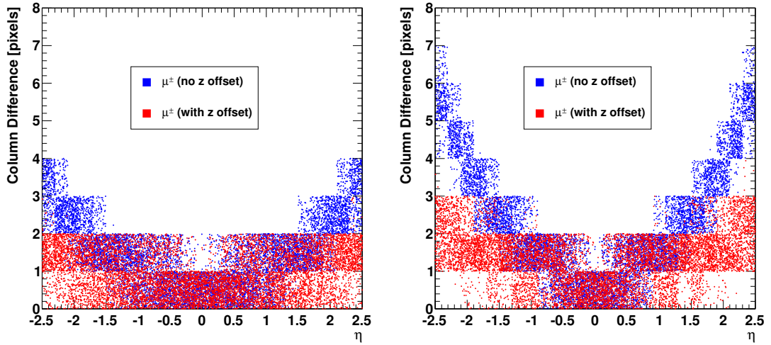
Figure 3.23: Pixel column difference (column difference between hit pixels on the upper and lower sensors) as a function of \eta for 50 GeV/c \mu^\pm for a stacked layer at 25 cm in a tilted configuration using a 1 mm separation (left) and 2 mm separation (right). The blue distribution is for a stacked layer geometry which does not implement the z offset described in 3.3.1. Efficient correlation would require the matching of columns as a function of module position and at high \eta hit data must be transferred between modules. The red distribution is for a stacked layer geometry which implements the z offset so that the correlation window can be kept fixed to within 2-3 pixels depending on the sensor separation.
