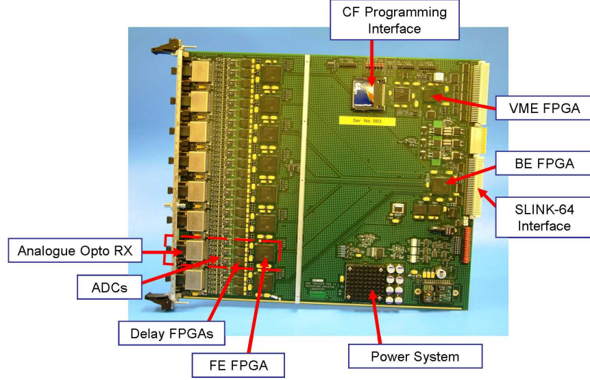
Figure 2.5: Layout of the CMS Silicon Strip Tracker FED. Modified from [62].
