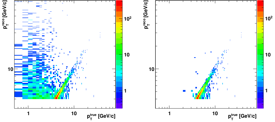
Figure 4.27: Distribution of Monte-Carlo track transverse momentum ( p_T^{\text{true}} ) and measured transverse momentum ( p_T^{\text{reco}} ) for minimum bias particles under SLHC conditions reconstructed by the double stack and passing the 4 GeV/c p_T cut. Left: for all tracks, and Right: for tracks only originating from the beam spot. The individual stacks use a tight correlation window of 3 pixels.
