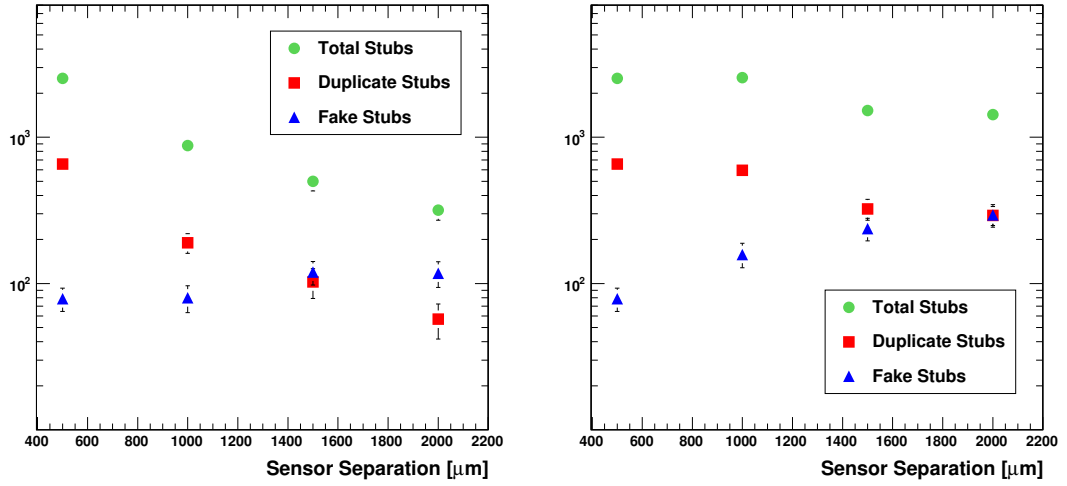
Figure 4.11: Average number of generated stubs per event under SLHC pileup conditions as a function of sensor separation; Left: for fixed correlation cuts, Right: for variable correlation cuts. Results are for a stacked layer at 25 cm in the tilted configuration.
