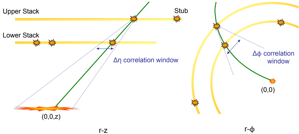
Figure 4.18: The double stack reconstruction method. Stubs from the inner stacked pixel layer which fall within a \Delta\eta\Delta\phi window of a seed stub in the outer layer are correlated.
