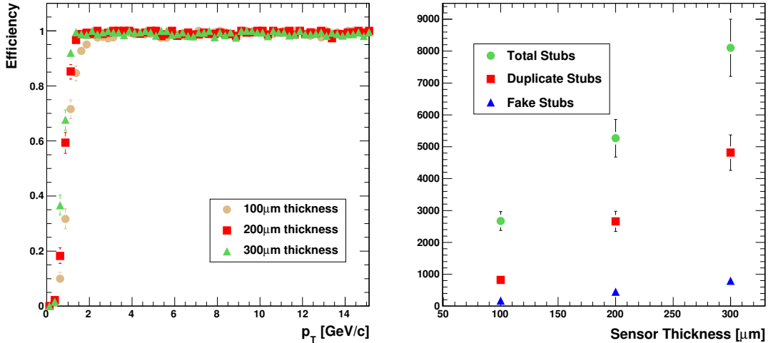
Figure 4.13: Left: p_T discrimination performance of a stacked layer for single \mu^\pm tracks and, Right: Average number of generated stubs per event under SLHC pileup conditions as a function of sensor thickness. Results are for a stacked layer at 25 cm in the untilted configuration and a sensor separation of 1 mm.
