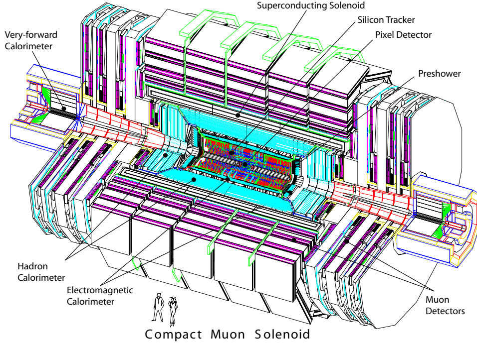
Figure 1.7: Schematic of the CMS Detector[11].
