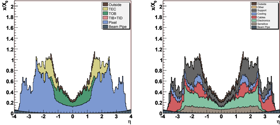
Figure 3.18: Material contribution of the tracker in radiation lengths as a function of pseudorapidity by subdetector (left) and by material type (right).
