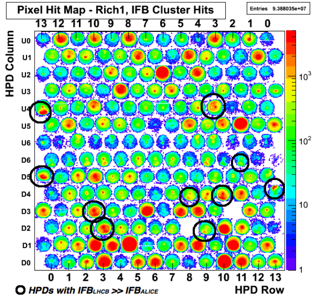
Figure 4.21: ALICE/PHYSICS run pairs: large cluster hit-map for one run. High IFB_{PHYSICS} deviations are circled in black.
