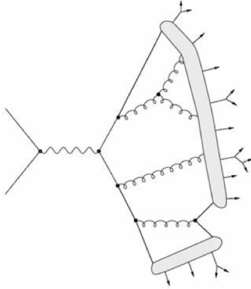
Figure 5.3: The Lund string model applies a colour-confinement string, which stretches between a quark/anti-quark pair. Gluons appear as kinks in the string.
