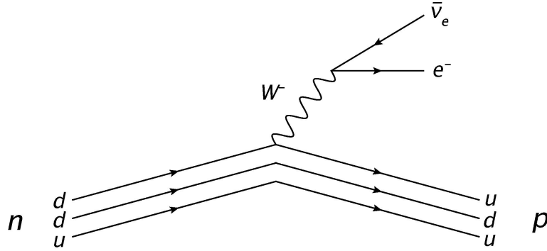
Figure 2.2: Quark-level Feynman diagram of beta decay, where the (u, d)_L doublet couple to the W^- , which in turn emits a (e^-, \bar{\nu}_e)_L doublet.
