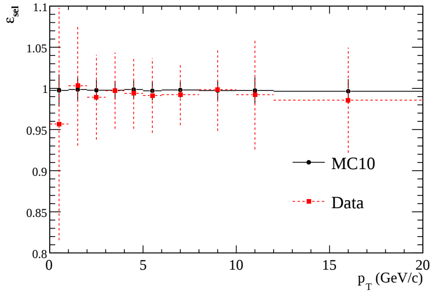
Figure 7.6: Ratio of fit-extracted signal yields with \chi_{vtx}^2 < 8 to signal yields without \chi_{vtx}^2 < 8 for 2010 data sample (red dashed) and MC10 (black solid). A tight cut is applied on the B^\pm lifetime \tau > 0.4 ps to compensate for increased background levels when removing the \chi_{vtx}^2 < 8 cut.
