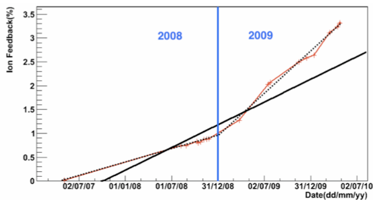
Figure 4.16: Timeline of HPD with developed ion feedback. Increase in vacuum degradation is evident from 2009.
