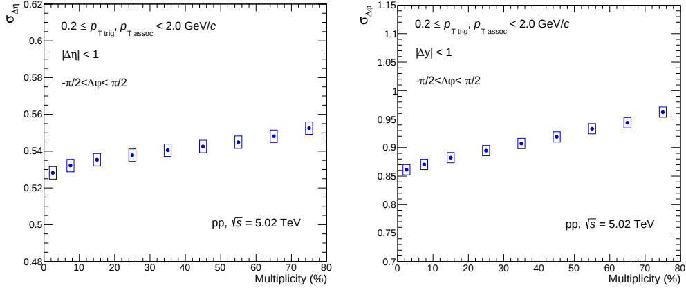
FIGURE 5.27: Balance function width \sigma_{\Delta\eta} (left) and \sigma_{\Delta\phi} (right) of charged particles in pp collisions at \sqrt{s} = 5.02 \text{ TeV} as a function of multiplicity class
