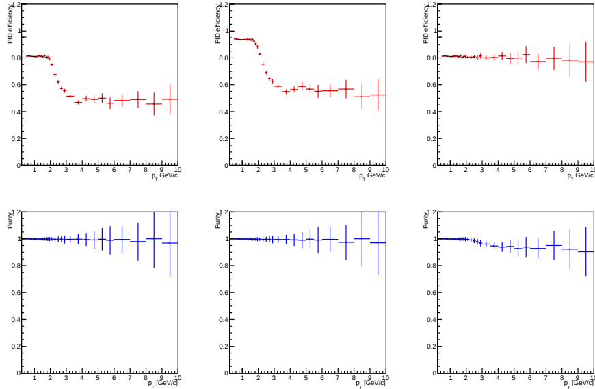
FIGURE 5.20: PID efficiencies and purities for pions reconstructed in the first (left), second (middle) and third (right) PID strategy variation
