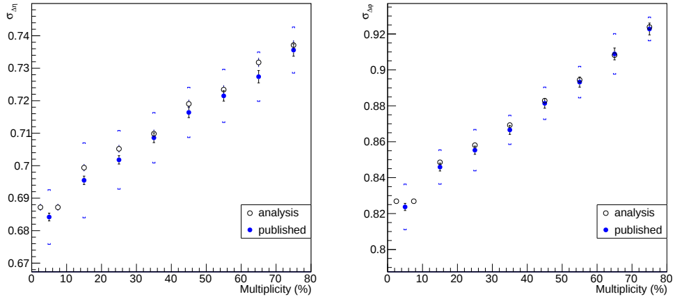
FIGURE 5.28: Comparison between the balance function width in \Delta\eta (left) and \Delta\phi (right) in repeated analysis at \sqrt{s} = 7 \text{ TeV} and published results for charged particles at \sqrt{s} = 7 \text{ TeV}
