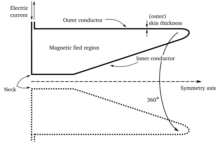
Figure 5.1: Cross-sectional schematic view of a magnetic horn.
