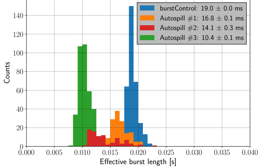
Figure 3.17: Distribution of the effective burst length for each extracted burst during the successful spill optimization with Austopill. The average of each histogram is reported in the legend.
