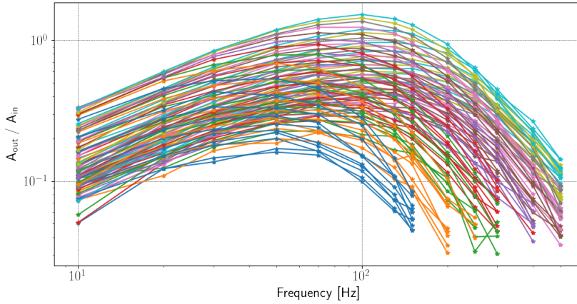
Figure 4.28: Overview of all the obtained transfer functions from the V_{ss} \times \xi parameter scan.
