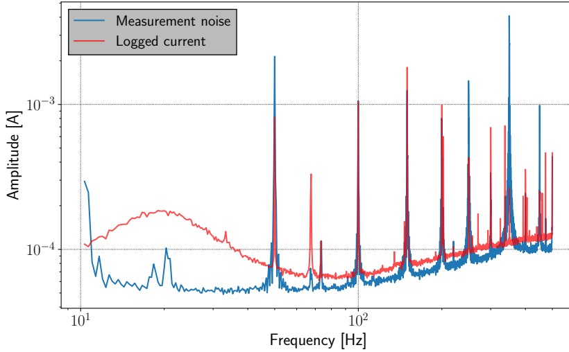
Figure 4.21: Average spectrum of the DCCT measurement noise (blue) compared with the average spectrum of the logged ripple currents during operation (red).
