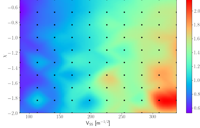
Figure 4.34: Interpolated 2D map of the pole of the transfer function for the V_{ss} \times \xi parameter scan. The color code indicates the position of the pole normalized by the one of the current SPS working point.
