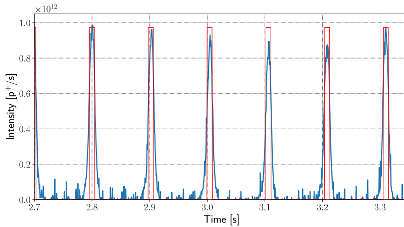
Figure 3.12: Measured spill (blue) obtained by demanding 9 ms as burst length, superimposed with a 9 ms square wave (red) for reference.
