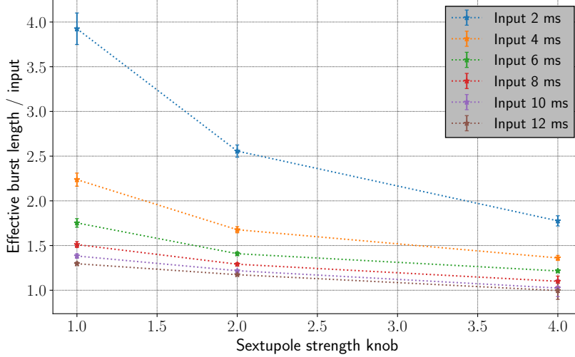
Figure 3.31: Effective burst length to demanded burst length ratio as a function of the sextupole strength scaling factor (where 1 is the nominal strength). The reported set of points are grouped according to the same demanded burst length, as indicated in the legend.
