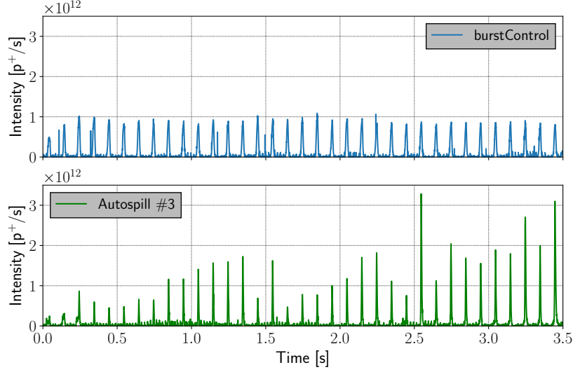
Figure 3.20: Top: spill created with the burstControl application as initial condition for the iterative optimization. Bottom: spill obtained at the third iteration of the Autospill, with the successfully optimized burst length.
