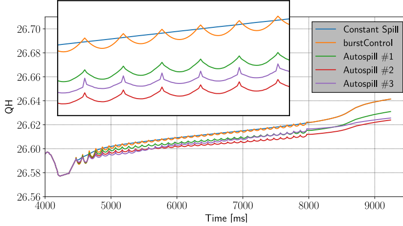
Figure 3.16: Flat-top tunes of a successful burst extraction spill optimization. The small plot shows a zoom of the tune functions of each optimization step.
