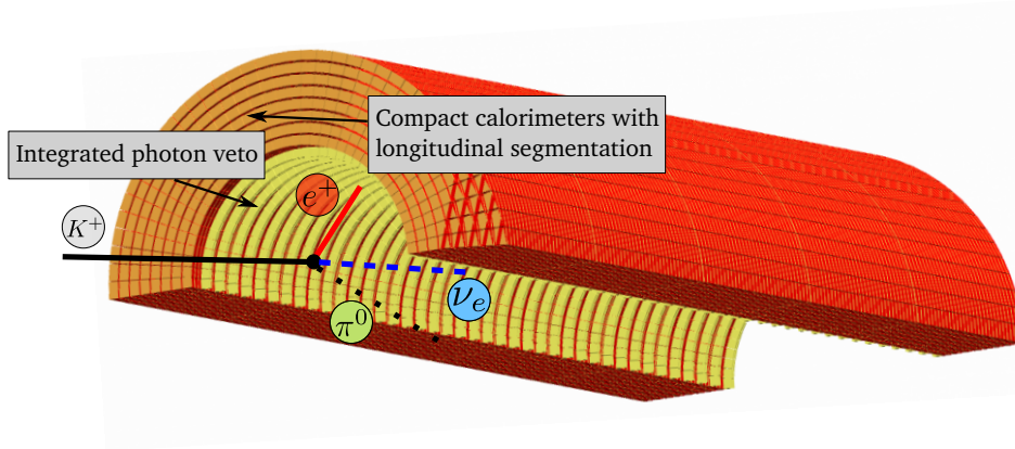
Figure 2.2: Sketch of a sector of the ENUBET instrumented decay tunnel.
