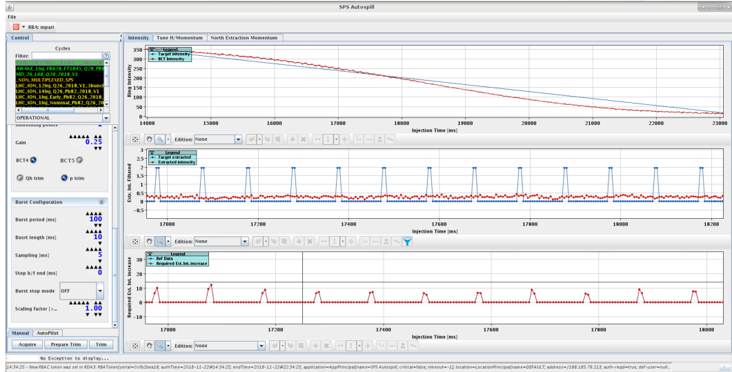
Figure 3.15: Screenshot of the upgraded Austospill application used during the last burst extraction tests at the SPS.
