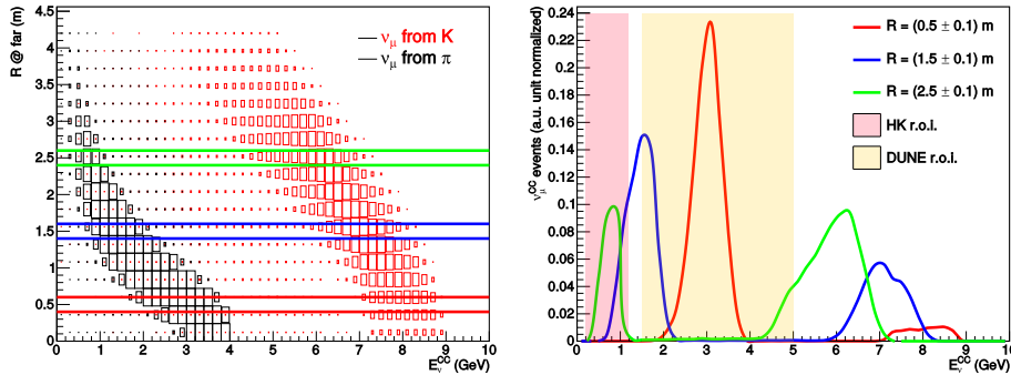
Figure 2.4: Left: correlation of \nu_{\mu}^{CC} energy with the radial distance from the beam axis at the neutrino detector. Right: energy distributions for the corresponding radial ranges selected from the left plot. From [25].
