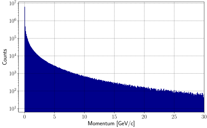
Figure 5.11: Momentum distribution of the all the secondary particles produced by the protons interaction on the target, for a number of protons of target of 10'000.
