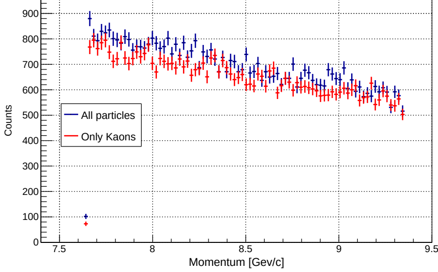
Figure 5.13: Comparison of the momentum distribution of the selected K^+ with the particle cut option (red) or without (blue).
