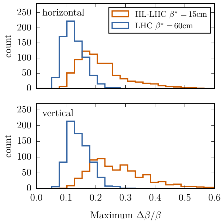
Figure 4.6.: Peak \beta -beating distribution after one iteration of global optics correction.
