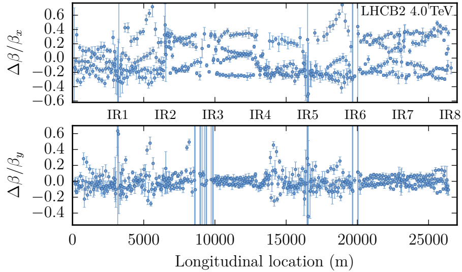
Figure B.18.: Beta-beating for beam 2 for ATS optics with \beta^* = 10 cm.
