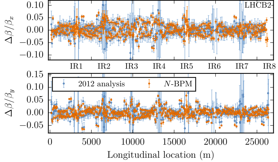
Figure B.3.: \beta -beating for Beam 2 after local and global corrections at \beta^* = 60 cm.
