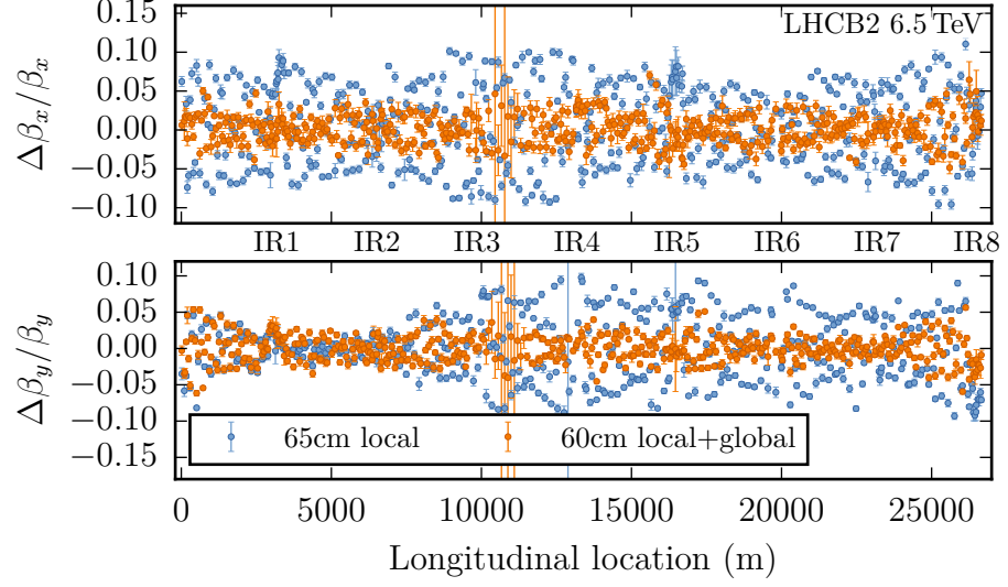
Figure B.7.: \beta -beating after local and global optics corrections along the machine for beam 2 at a \beta^* of 60 cm.
