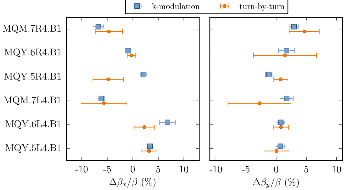
Figure 2.14.: Comparison of the measured \beta -functions using k-modulation and turn-by-turn measurements for magnets in IR4 for beam 1 at 450 GeV.
