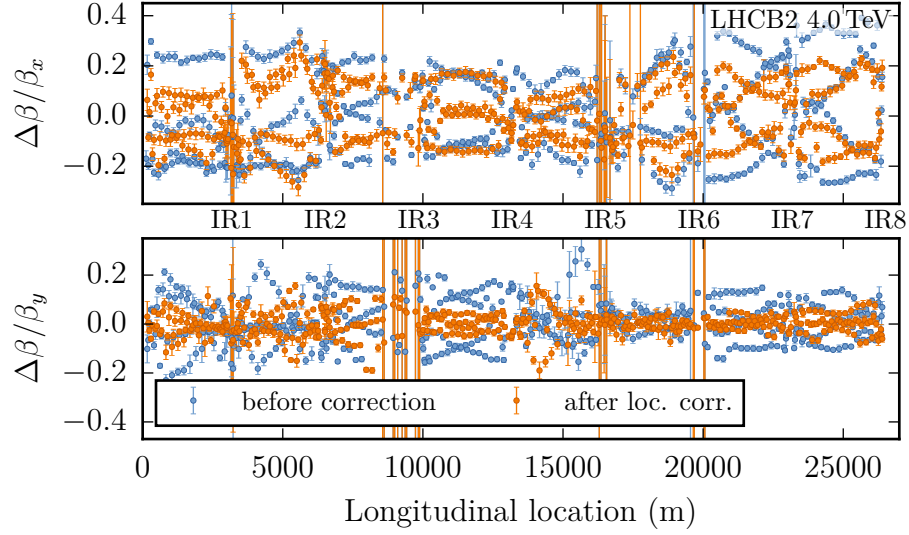
Figure B.17.: Beta-beating for beam 2 for ATS optics with \beta^* = 20 cm, before and after local corrections.
