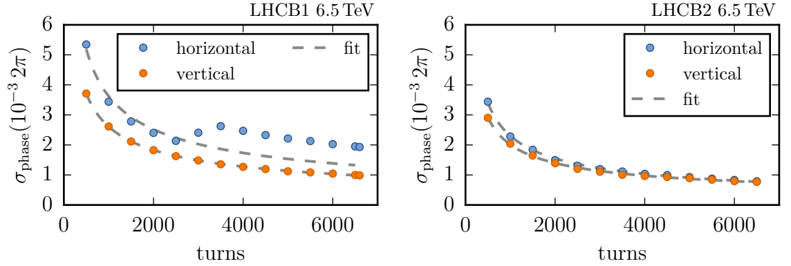
Figure 3.18.: Average precision of the measured phase advance for different number of turns used in the analysis for beam 1 (left) and beam 2 (right). The fit was done with a function proportional to 1/\sqrt{\text{turns}} , and for beam 1 horizontally only the first five data points were used for the fit.
