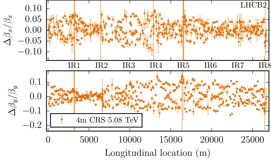
Figure B.13.: Beta-beating for beam 2 during the CRS at an energy of 5.08 TeV and a \beta^* of 4m in IP1 and IP5.
