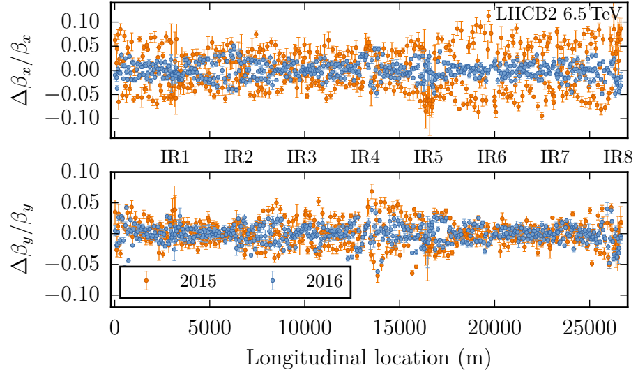
Figure B.12.: \beta -beating for beam 2 at \beta^* = 40 cm after corrections in 2015 and 2016.
