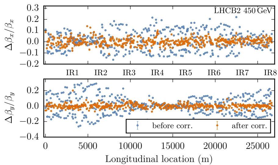
Figure B.2.: \beta -beating at injection for beam 2 before and after optics correction.
