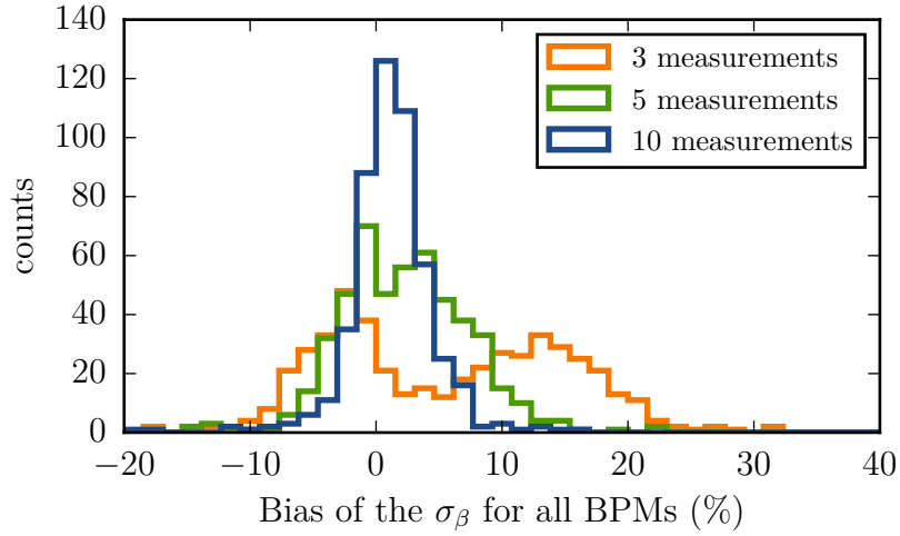
Figure 2.6.: The distribution shows for all BPMs the mean of the deviation of the derived uncertainty of the \beta -function compared to the calculated error bar from the known phase uncertainty.
