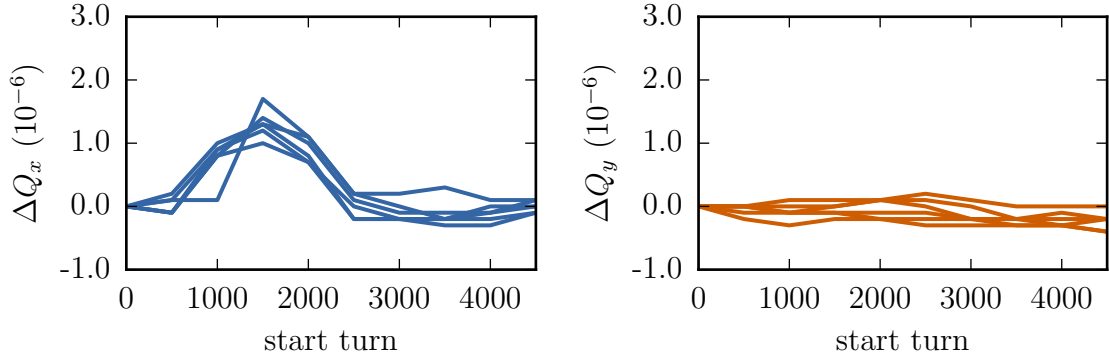
Figure 3.13.: Measured deviation of the ac dipole tune when 2000 turns out of 6600 were analyzed, starting from different turn numbers. The plots show six different measurements at a \beta^* of 80 cm.
