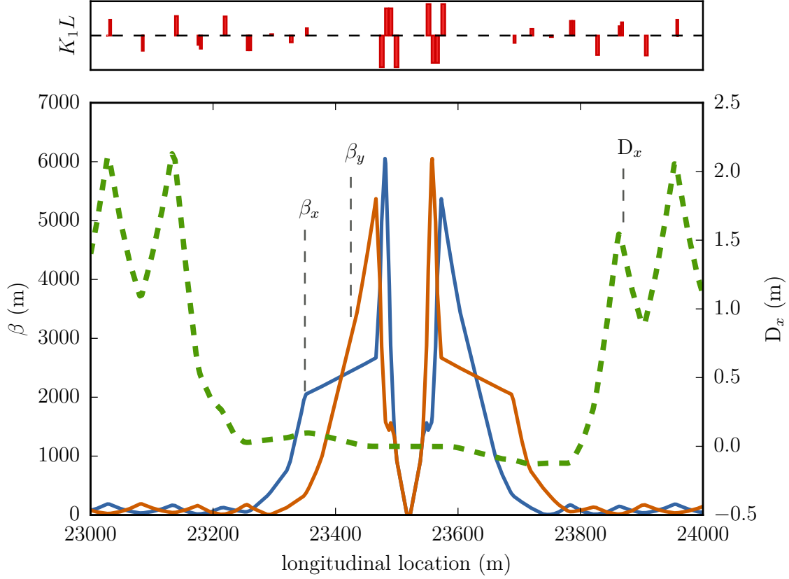
Figure 1.11.: \beta -function and horizontal dispersion in IR1 for a \beta^* of 40 cm. The top graph indicates the position of quadrupole magnets and their integrated field gradient ( K_1L ). The IP is surrounded by the final focusing triplet magnets.
