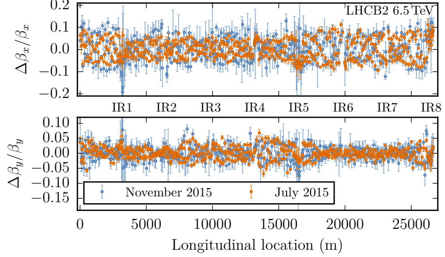
Figure B.11.: Repeated measurement of the \beta -beating for beam 2 at a \beta^* of 40 cm after a time period of 4 months.
