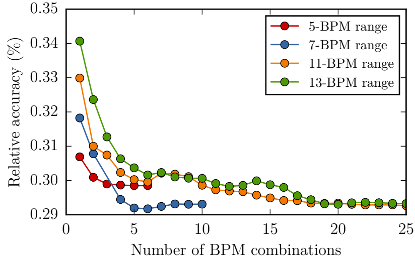
Figure 2.20.: Accuracy of the derived horizontal \beta -functions from simulations for different ranges of BPMs and different amount of BPM combinations.
