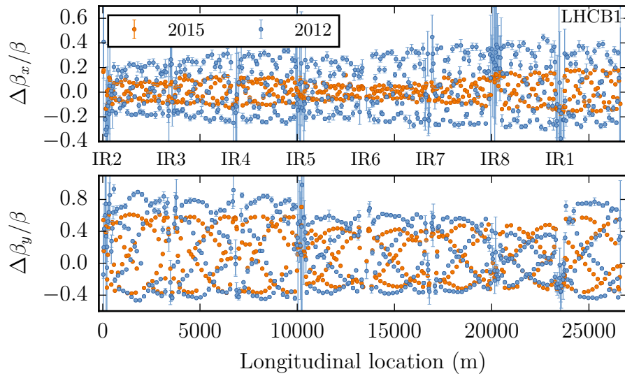
Figure B.10.: \beta -beating before optics corrections for beam 1 at a \beta^* of 60 cm (2012) and 65 cm (2015).
