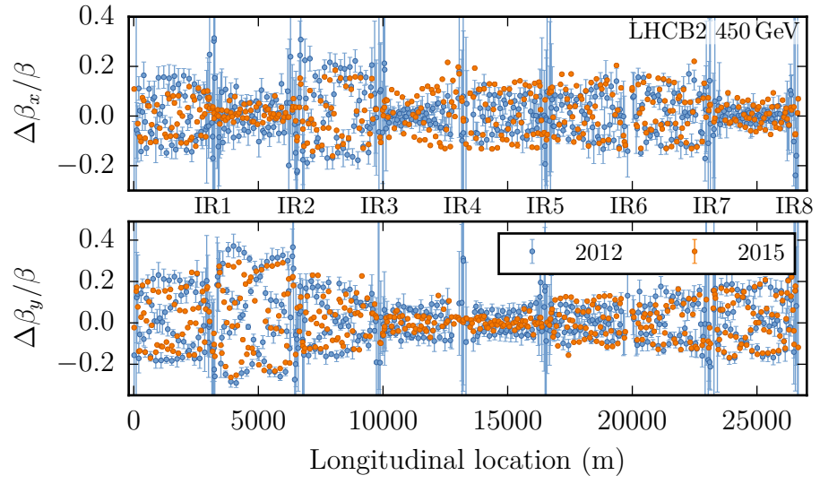
Figure B.1.: \beta -beating at injection for beam 2 in 2015 in comparison to 2012.
