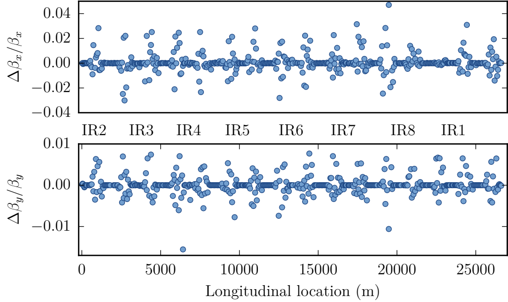
Figure 2.10.: Relative deviation of the computed \beta -function for a measurement of beam 1 at a \beta^* of 80 cm, between using either a model with the nominal setting of MQT magnets, or the real setting of the magnets during the measurement.
