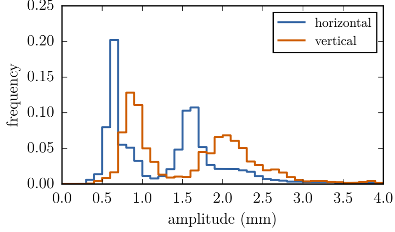
Figure 3.17.: Distribution of the beam oscillation amplitudes during TbT measurements at all BPMs for low- \beta^* optics in 2015. The two peaks in this distribution are due to the fact that most of the BPMs are located in the arcs where the \beta -function alternates between 30 m and 170 m at the BPM positions.
