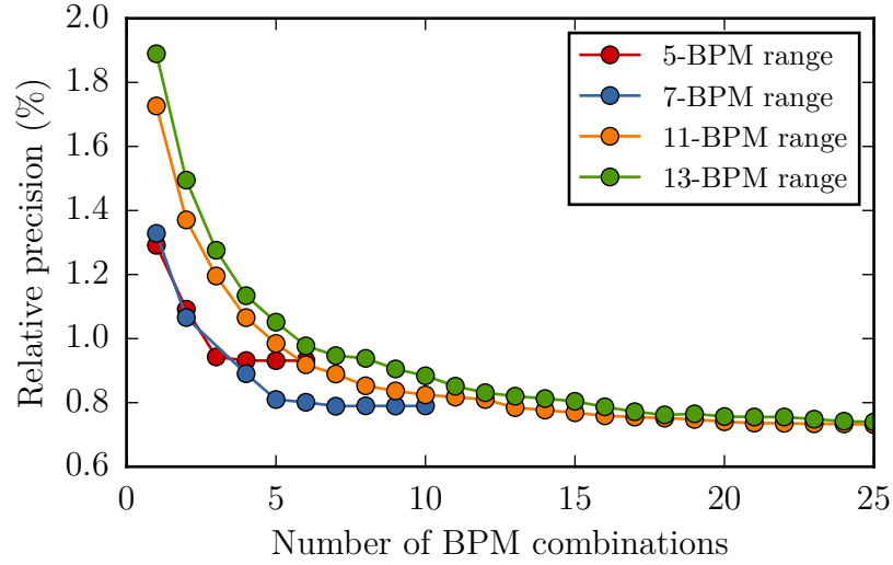
Figure 2.19.: Precision of the derived horizontal \beta -functions from simulations for different ranges of BPMs and different amount of BPM combinations.
