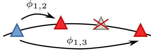
Figure 2.2.: In the arcs the phase advance between two consecutive BPMs is about \pi/4 . If the blue BPM is probed, it is better to skip the grey BPM and use the two red BPMs. The resulting phase advances are approximately \phi_{1,2} = \pi/4 and \phi_{1,3} = 3\pi/4 , which is the optimum according to Eq. (2.1).
