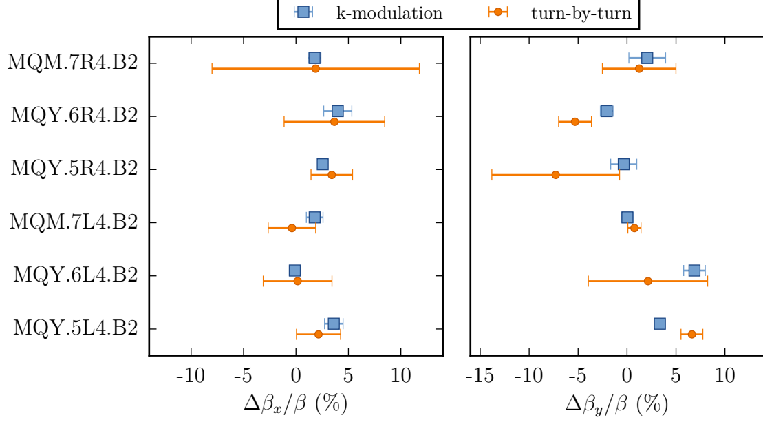
Figure 2.15.: Comparison of the measured \beta -functions using k-modulation and turn-by-turn measurements for magnets in IR4 for beam 2 at 450 GeV.
