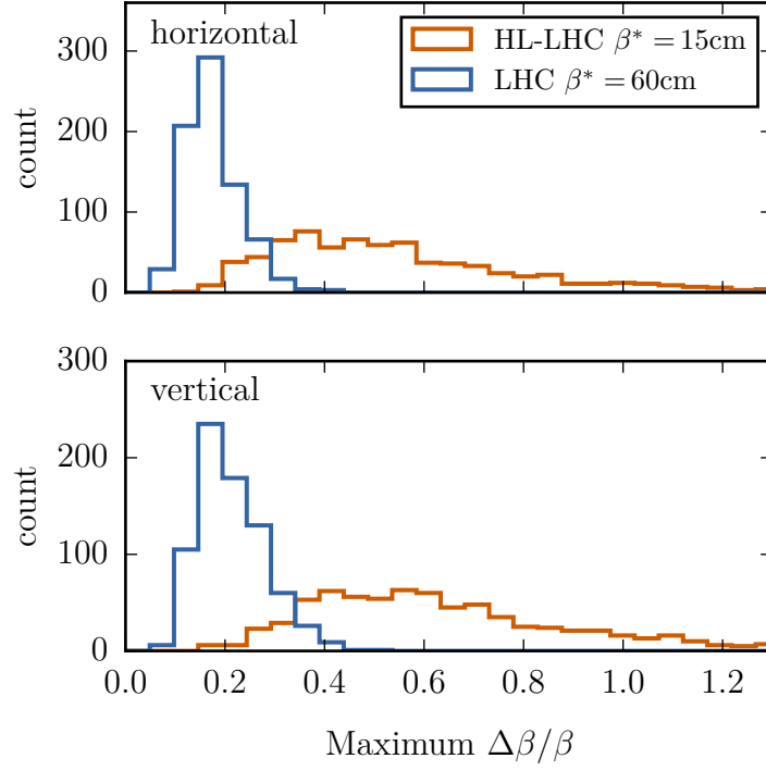
Figure 4.5.: Peak \beta -beating distribution before optics correction.
