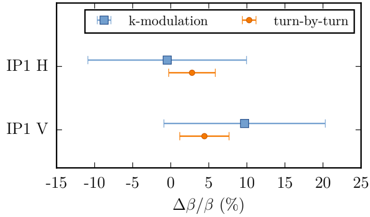
Figure 2.16.: Comparison of the measured \beta -functions using k-modulation and turn-by-turn measurements in IP1 for beam 1 at 6.5 TeV.
