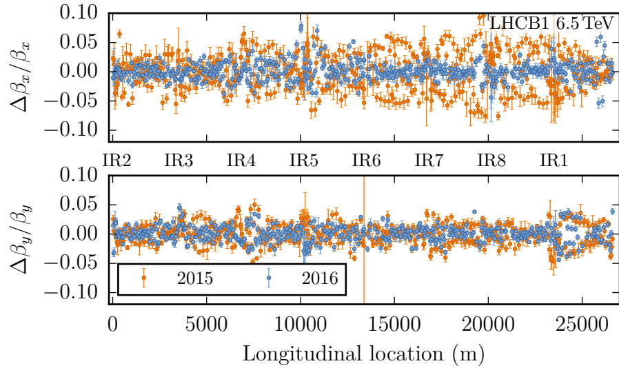
Figure 3.9.: \beta -beating for beam 1 at \beta^* = 40 cm after corrections in 2015 and 2016.
