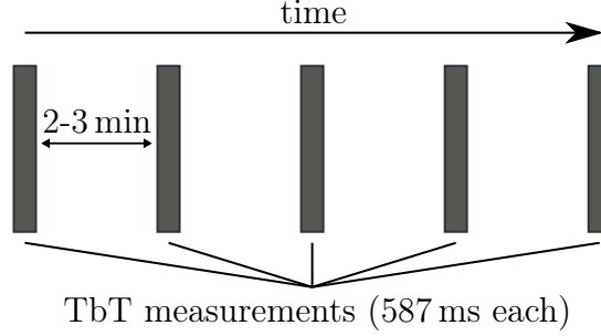
Figure 3.12.: Illustration of the time scale for a set of TbT measurements. Taking at least five measurements is recommended, based in the observations in Section 2.1.1. Additional measurement sets with different rf settings can be performed for probing off-momentum effects.
