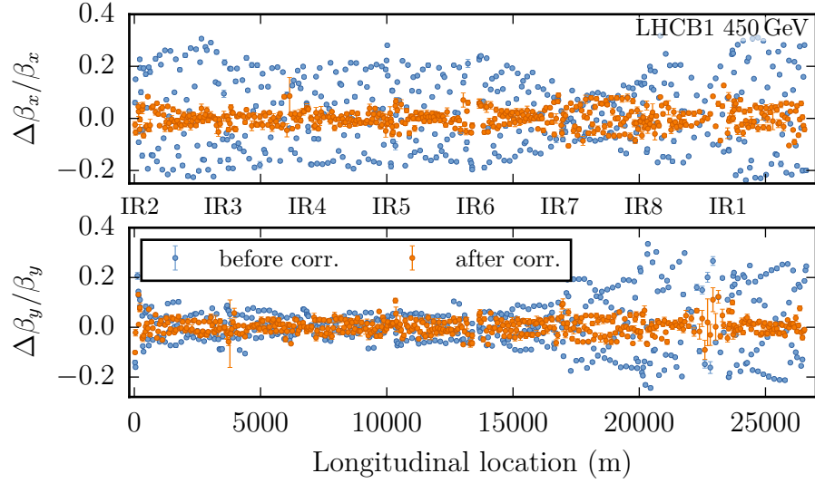
Figure 3.4.: \beta -beating at injection for beam 1 before and after optics correction. Both measurements were analyzed with the N -BPM method.
