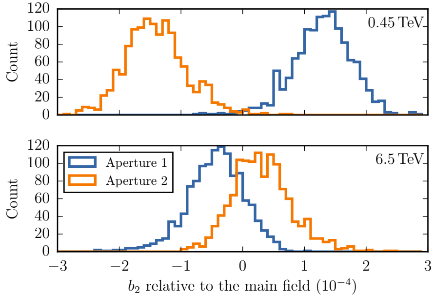
Figure 2.7.: Distribution of the b_2 component for the LHC main dipole magnets, separately for both apertures, at 450 GeV and 6.5 TeV.
