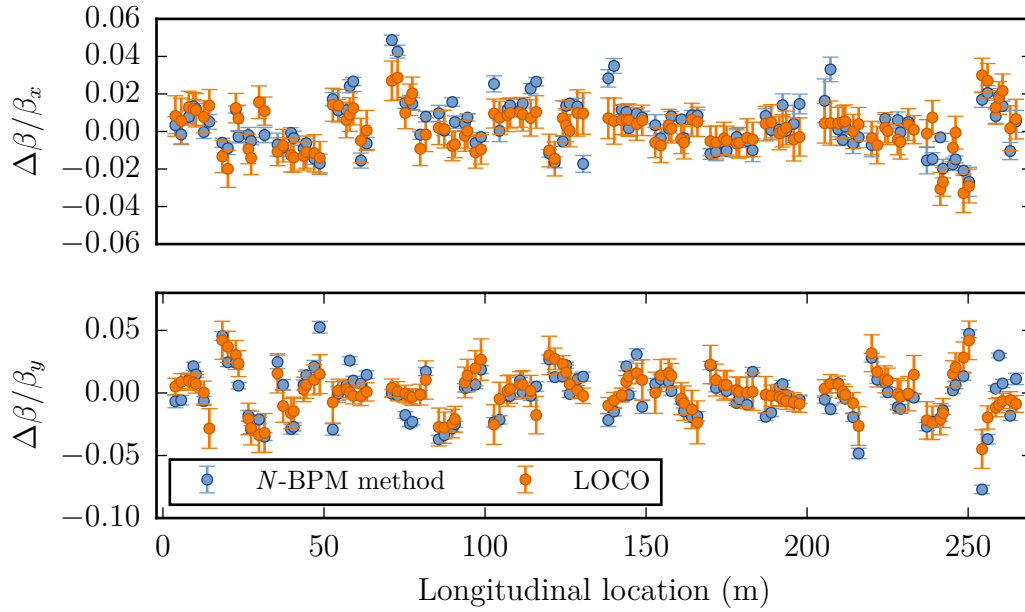
Figure 2.23.: Comparison of the \beta -beating as derived from BPM turn-by-turn data using the phase of the betatron oscillation ( N -BPM method with an 11-BPM range) to the \beta -beating from LOCO.
