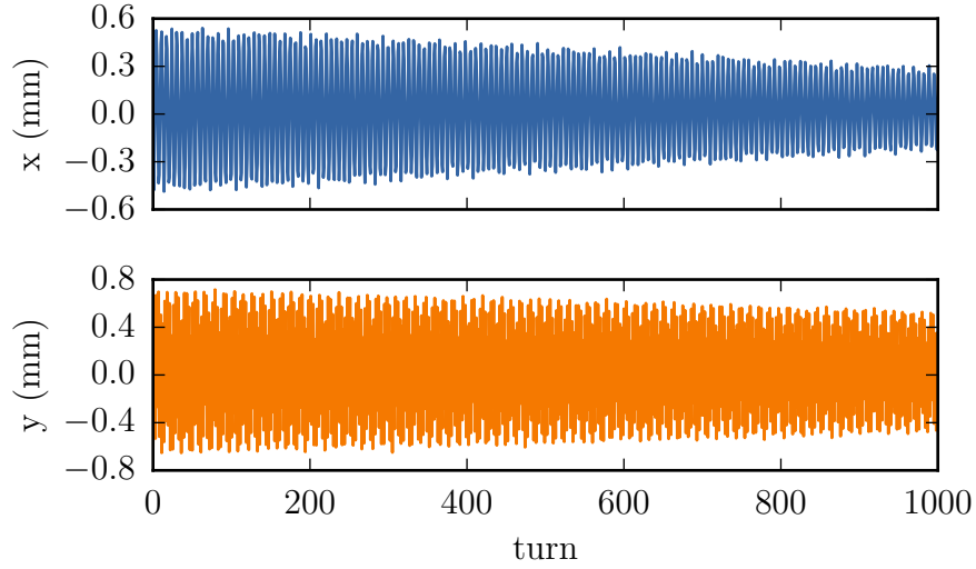
Figure 2.21.: Turn-by-turn oscillations at BPMs where \beta = 12.7 m.
