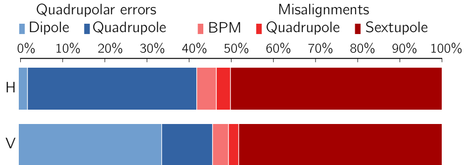
Figure 2.18.: Contribution of the uncertainties from Table 2.5 to the total variance of the derived \beta -function. The average value over all BPMs is shown for the case of probing the middle BPM of neighboring BPMs, as it is the combination which has the smallest systematic error. The top bar is for the horizontal plane (H) and the bottom one for the vertical plane (V). Quadrupolar errors are shown in blue and misalignment uncertainties in red.
