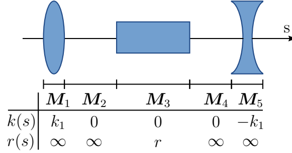
Figure 1.5.: Illustration of a typical segment in an accelerator of a focusing quadrupole followed by a dipole and a defocusing quadrupole. The transfer matrices M_1 to M_5 denote the regions where constant magnetic fields along the longitudinal axis are assumed.
