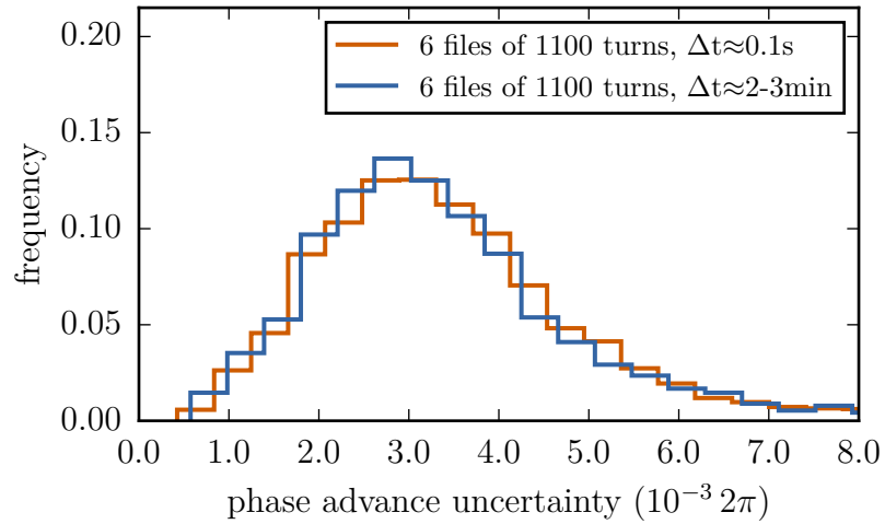
Figure 3.15.: Uncertainties of the measured betatron phase advances calculated from six measurement files of 1100 turns from one ( \Delta t \approx 0.1 s) or multiple ( \Delta t \approx 2-3 min) beam excitations for beam 1 at a \beta^* of 80 cm.
