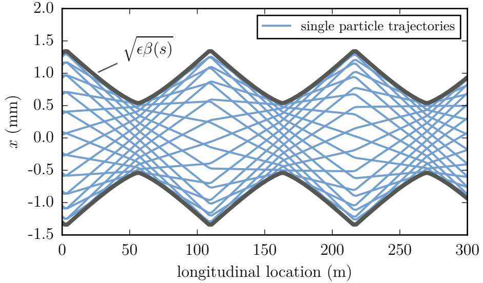
Figure 1.6.: Particle trajectories computed from Eq. (1.13). The maximum amplitude \sqrt{\epsilon\beta(s)} defines an envelope for all particles with emittance \epsilon .
