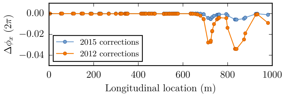
Figure 3.22.: Resulting deviations of the betatron phase for local corrections in IR1 of beam 1 which were used in 2012 and 2015.
