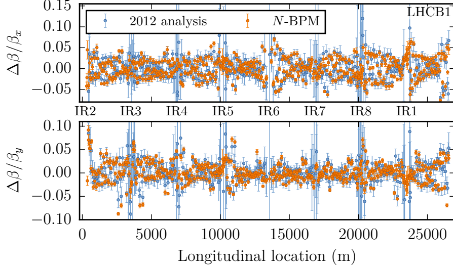
Figure 3.1.: \beta -beating for Beam 1 after local and global corrections at \beta^* = 60 cm.
