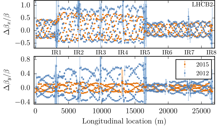
Figure 3.21.: \beta -beating before optics corrections for beam 2 at a \beta^* of 60 cm (2012 at 4 TeV) and 65 cm (2015 at 6.5 TeV).
