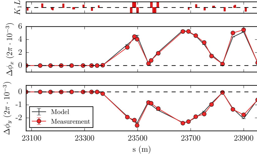
Figure 1.15.: The simulated measurement of the phase advance deviation between consecutive BPMs is shown for one IR. On the top of the plot the position of quadrupole magnets is illustrated with the two triplets around the center where the IP is. An artificial error in a magnet results in a periodic deviation of the phase advances starting at that magnet position (red line). The gradients in the lattice model in MAD-X are adjusted to reproduce the observed deviations (black line). Applying these gradients with negative sign will correct these deviations.
