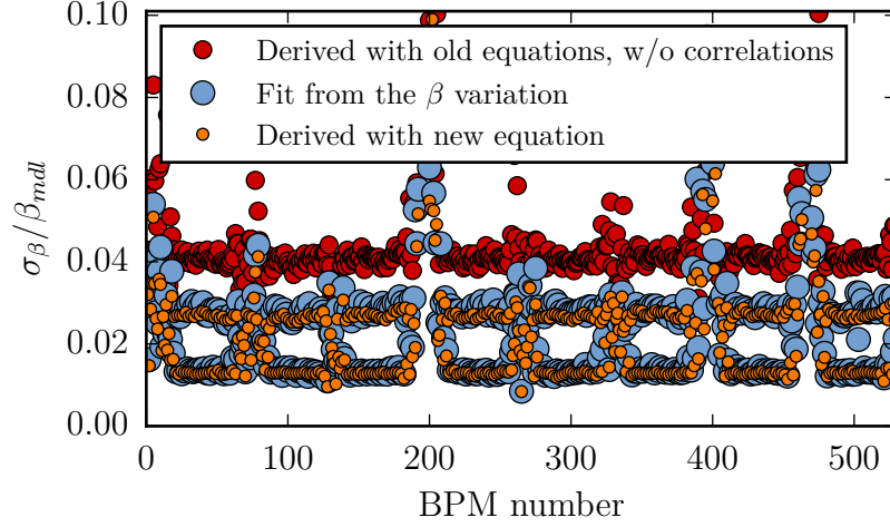
Figure 2.4.: Relative uncertainty of the \beta -function derived in the error propagation compared to a fit of the variation of calculated \beta -functions.
