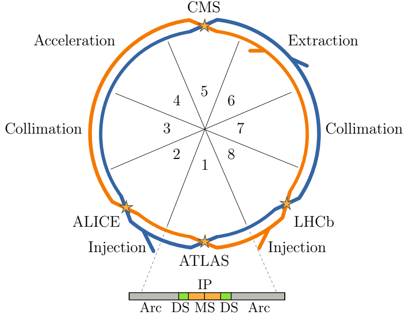
Figure 1.9.: Layout of the LHC illustrating the eight octants. In each octant the purpose of its IR is shown. The crossing of beam 1 (blue) and beam 2 (orange) is indicated in the four experimental insertions. For octant 1 the sequence of arcs, dispersion suppression (DS) and matching section (MS) with the interaction point (IP) in the center, is shown.
