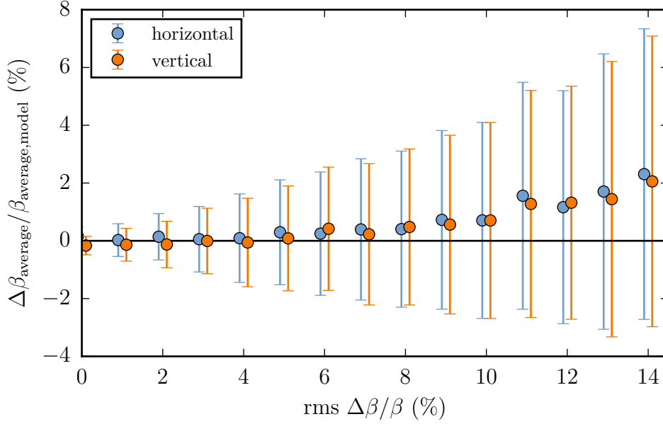
Figure 1.14.: The relative deviation of the average \beta -function from the model value is shown for different lattices where quadrupole errors were introduced for the LHC optics with \beta^* = 40 cm. The data has been binned in steps of 1% according to the rms \beta -beating.
