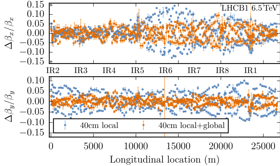
Figure B.4.: \beta -beating after local and global optics corrections along the machine for beam 1 at a \beta^* of 40 cm.
