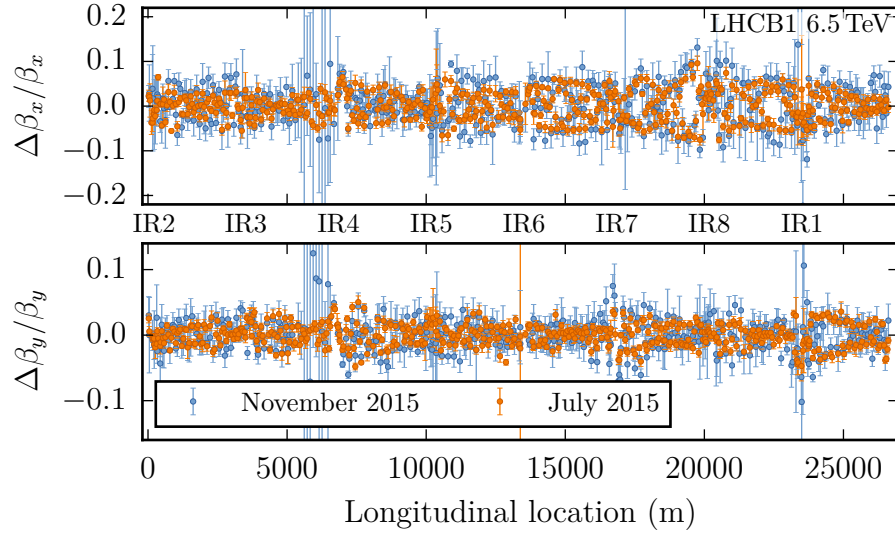
Figure 3.20.: Repeated measurement of the \beta -beating for beam 1 at a \beta^* of 40 cm after a time period of 4 months.
