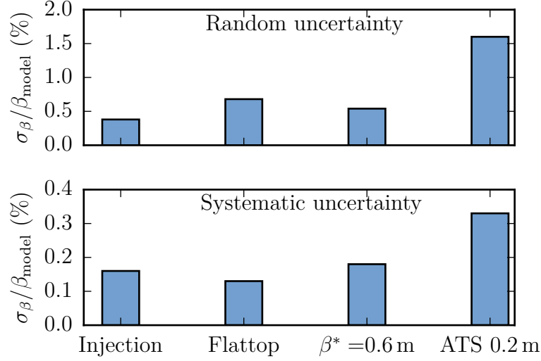
Figure 4.4.: Average relative uncertainty of the measured \beta -functions. Injection measurements are performed at 450 GeV, while all other measurements are at 4 TeV.
