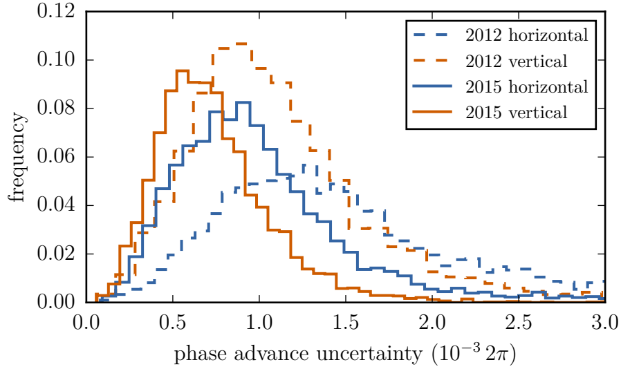
Figure 3.16.: Uncertainties of the measured betatron phase advances for both beams for optics with \beta^* = 60 cm (2012) and \beta^* = 80 cm (2015).
