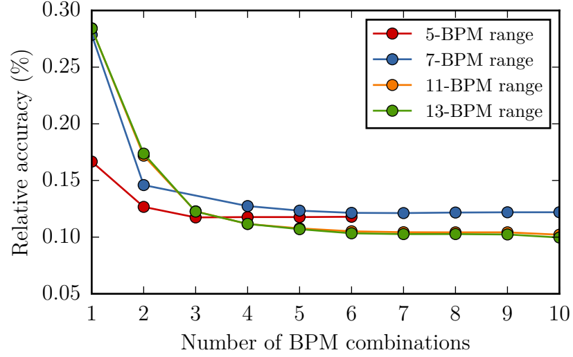
Figure 2.12.: Accuracy of the derived \beta -functions from simulations for different ranges of BPMs and different amount of BPM combinations. The oscillation amplitude was 1 mm in the arcs and a Gaussian noise of 200 \mu\text{m} was applied.
