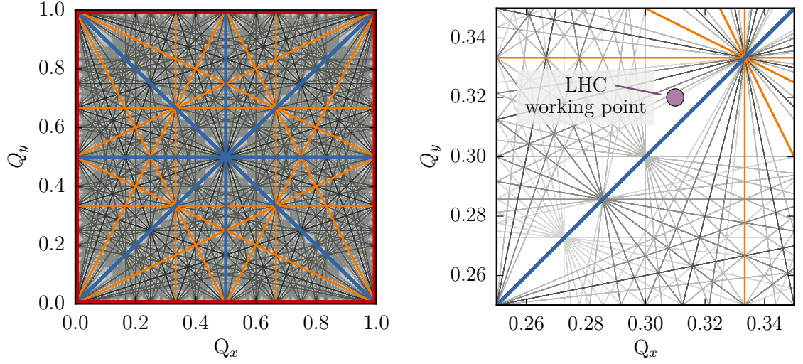
Figure 1.8.: Full tune diagram (left) and a zoom around the LHC working point (right) for resonances up to the 12 th order. The first order (red), second order (blue) and third order (orange) resonances are highlighted with colors. Higher order resonances are drawn with decreasing line widths and brighter gray tones.
