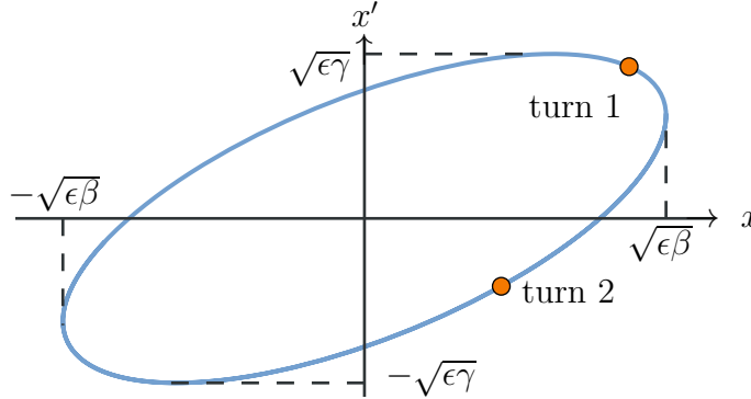
Figure 1.7.: The phase space ellipse defines the possible configurations of transverse position and angle for a particle with emittance \epsilon . It is specified at a certain location in the accelerator by the local optical functions.
