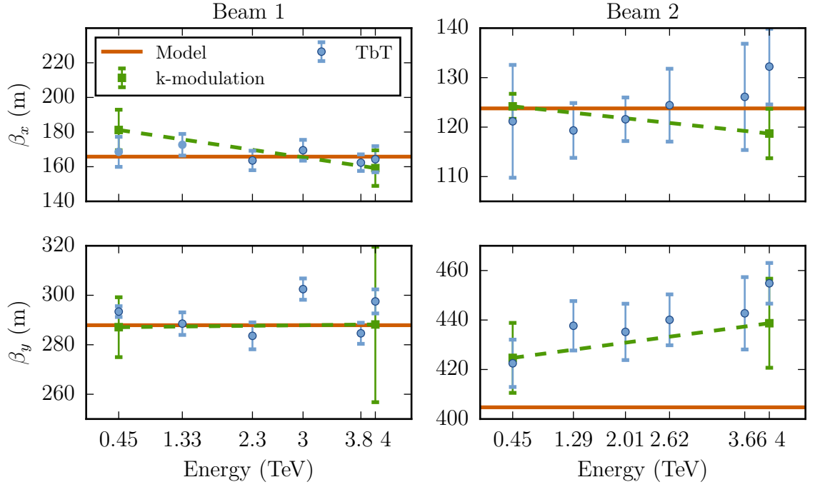
Figure 3.10.: Measured \beta -function at the wire scanners during the energy ramp. \beta values from a k-modulation measurement at 0.45 TeV and 4 TeV are shown as a comparison. The dashed line connects the two points from the k-modulation measurement at injection and top energy.
