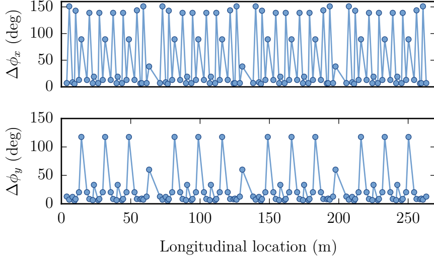
Figure 2.17.: Phase advances of consecutive BPMs in the nominal model. Many phase advances close to 0^\circ impair the calculation of \beta -functions when using only neighboring BPMs.
