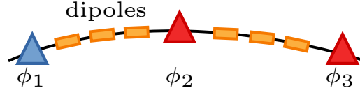
Figure 2.8.: The \beta -function is derived at the BPM with phase \phi_1 . The phase advances to two other BPMs are used, with \phi_{12} = \phi_2 - \phi_1 and \phi_{13} = \phi_3 - \phi_1 .
