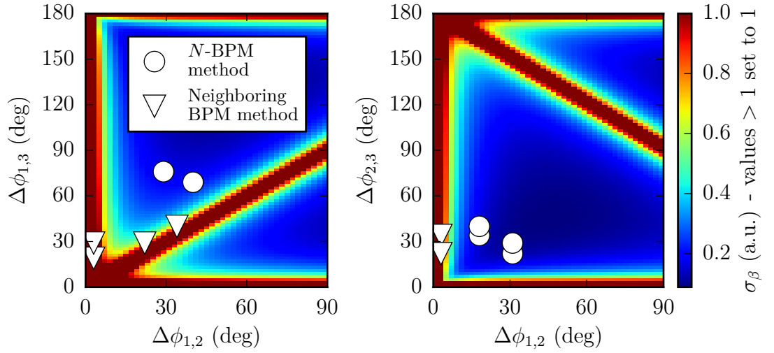
Figure 2.1.: Expected error of a measured \beta -function at position s_1 , depending on the phase advances to the other two BPMs. The six used phase advances (three BPM combinations each, for the horizontal and vertical plane) for a BPM position in IR4 from the neighboring BPM method are indicated by triangles. When an increased range of 7 BPM is used ( N -BPM method), 15 different combinations of phase advances are possible per plane, including the ones that are indicated by triangles. Six better suited combinations from the range of 7-BPMs are indicated by circles.
