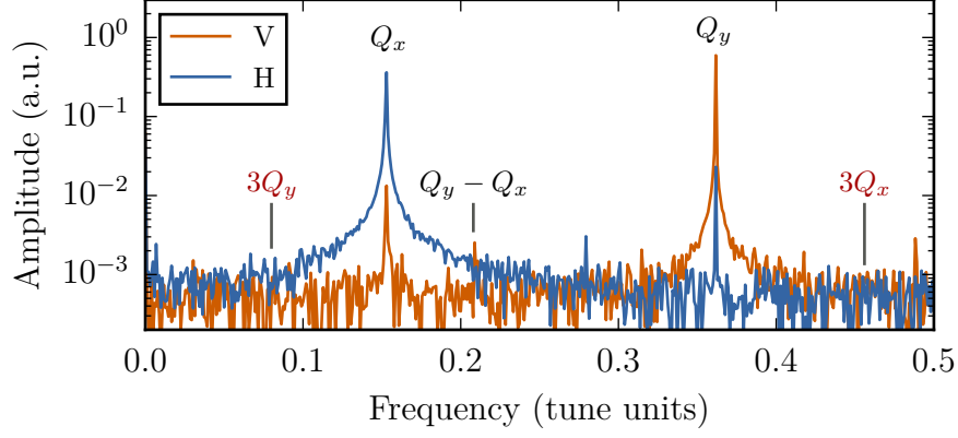
Figure 2.22.: Frequency spectrum of the horizontal (H) and vertical (V) turn-by-turn oscillations. The two peaks correspond to the tunes Q_x = 18.15 and Q_y = 8.36 . No additional lines which correspond to cubic distortions at 3Q_x and 3Q_y are visible.
