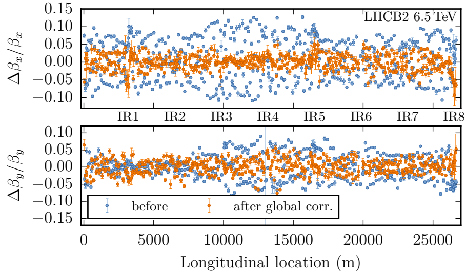
Figure B.9.: \beta -beating after local and global optics corrections along the machine for beam 2 at a \beta^* of 80 cm.
