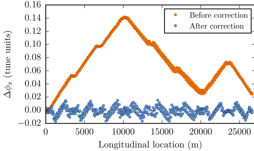
Figure 2.9.: Illustration of the betatron phase deviation due to the dipole b_2 components and after an arc-by-arc correction with MQT magnets. The slope of the phase deviation changes when the beam changes from the inner to the outer aperture after an interaction point.
