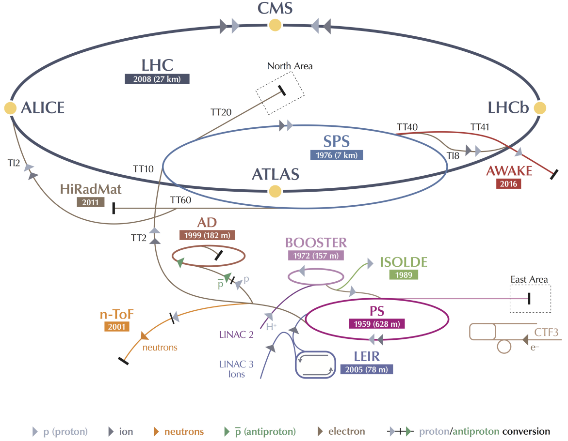
Figure 1.1.: Illustration of the CERN accelerator complex. Colored arrowheads indicate the possible paths of different particles. © CERN [13].
