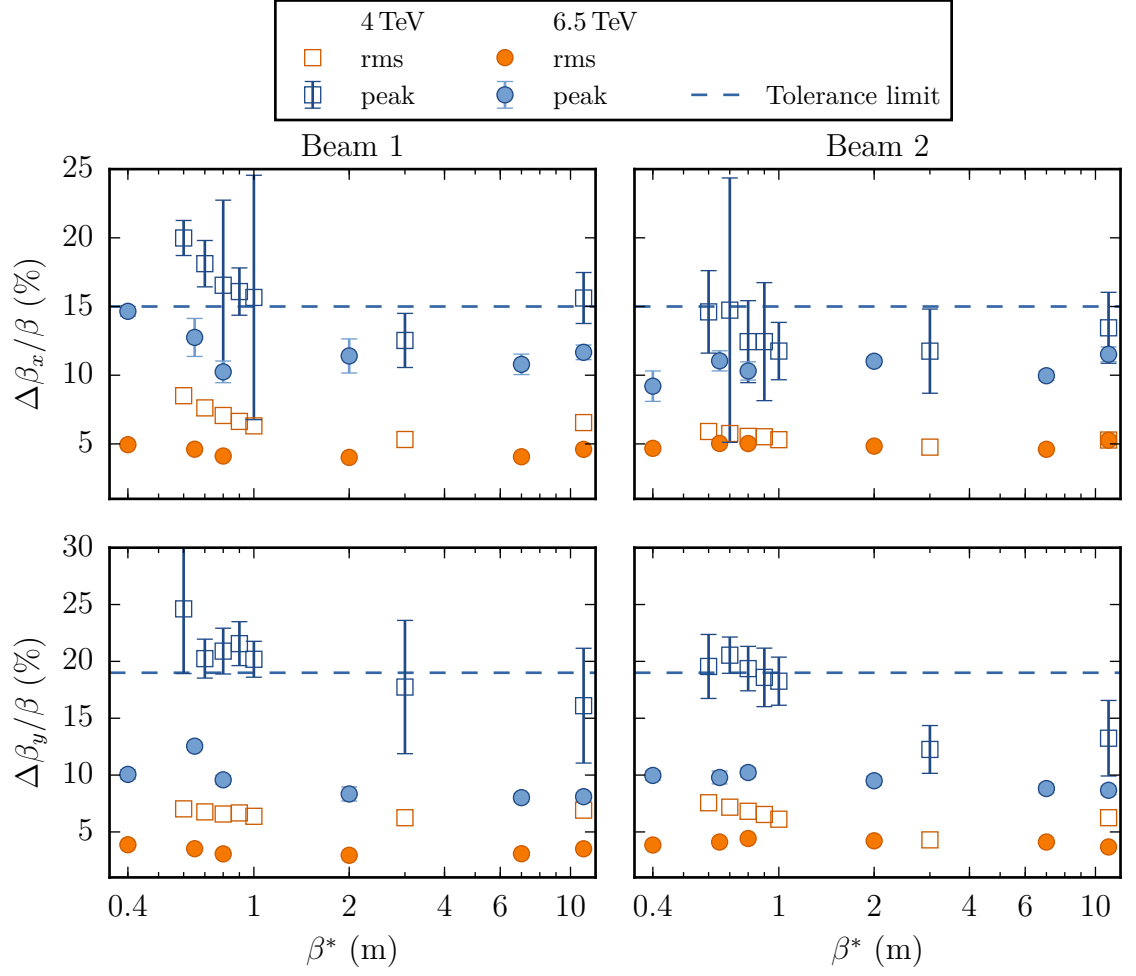
Figure 3.6.: Measured peak and rms \beta -beating along the \beta^* squeeze after local optics corrections have been incorporated. The maximum tolerable peak \beta -beating according to Table 1.2 is indicated as well.
