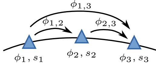
Figure 1.13.: Illustration of the \beta -function measurement from phase. The phase advances \phi_{i,j} in between three positions s_i are needed to derive the \beta -functions at those positions.
