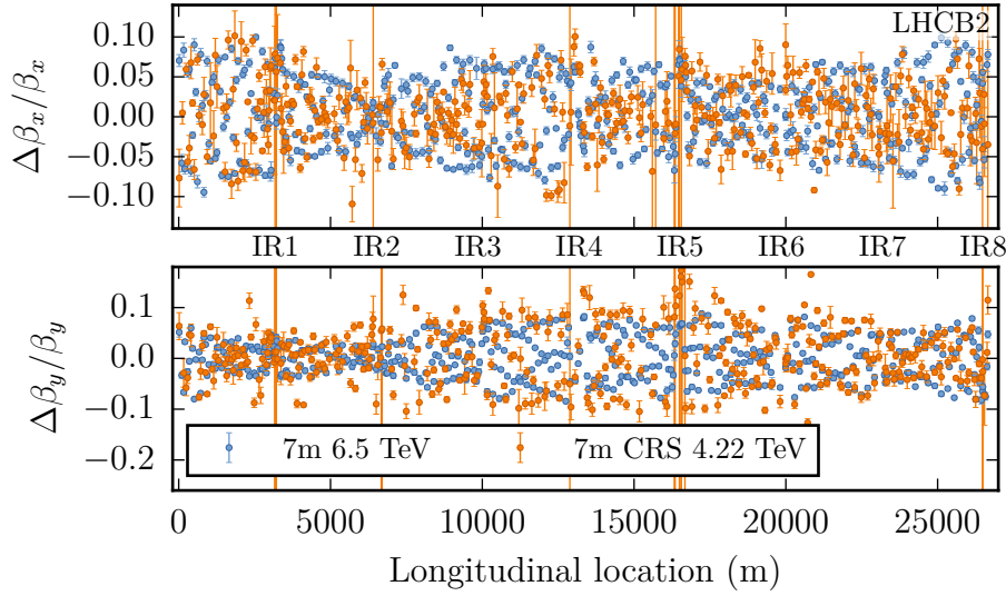
Figure 3.11.: \beta -beating for beam 2 during the CRS at an energy of 4.22 TeV and a \beta^* of 7 m in IP1 and IP5 in comparison to a static measurement at 6.5 TeV with the same \beta^* .
