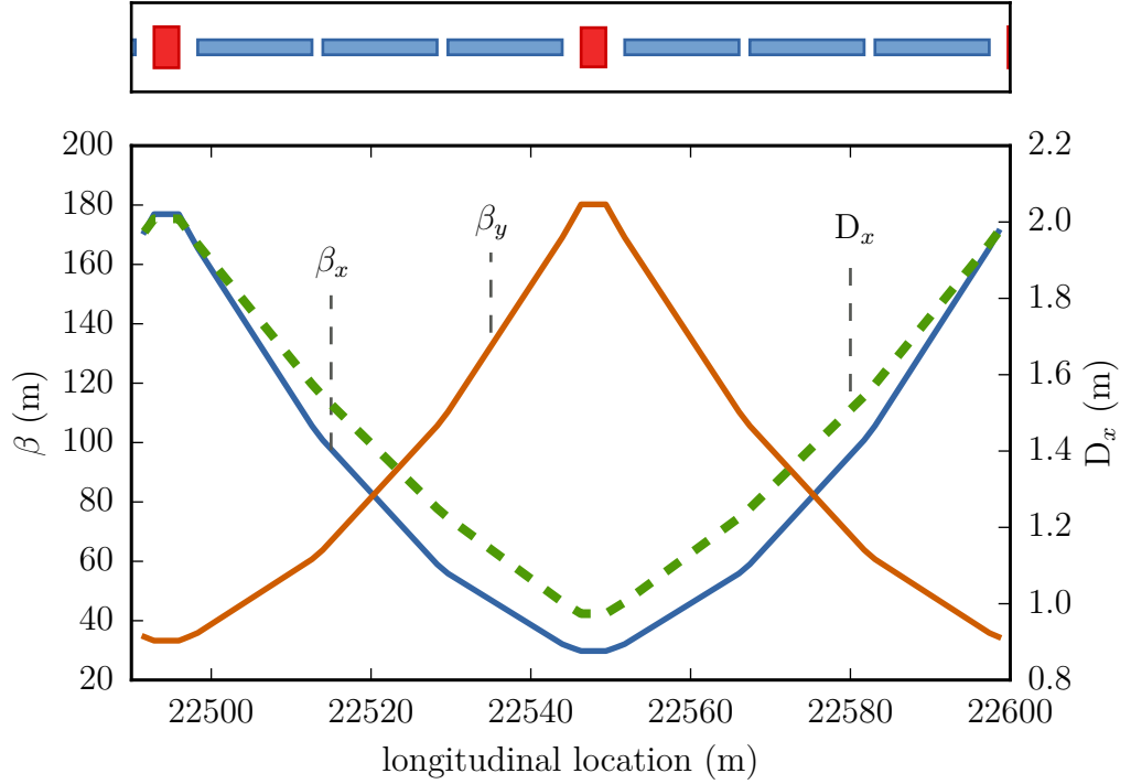
Figure 1.10.: \beta -function and horizontal dispersion in an LHC arc FODO cell. The top graph indicates the position of dipole (blue) and quadrupole (red) magnets.
