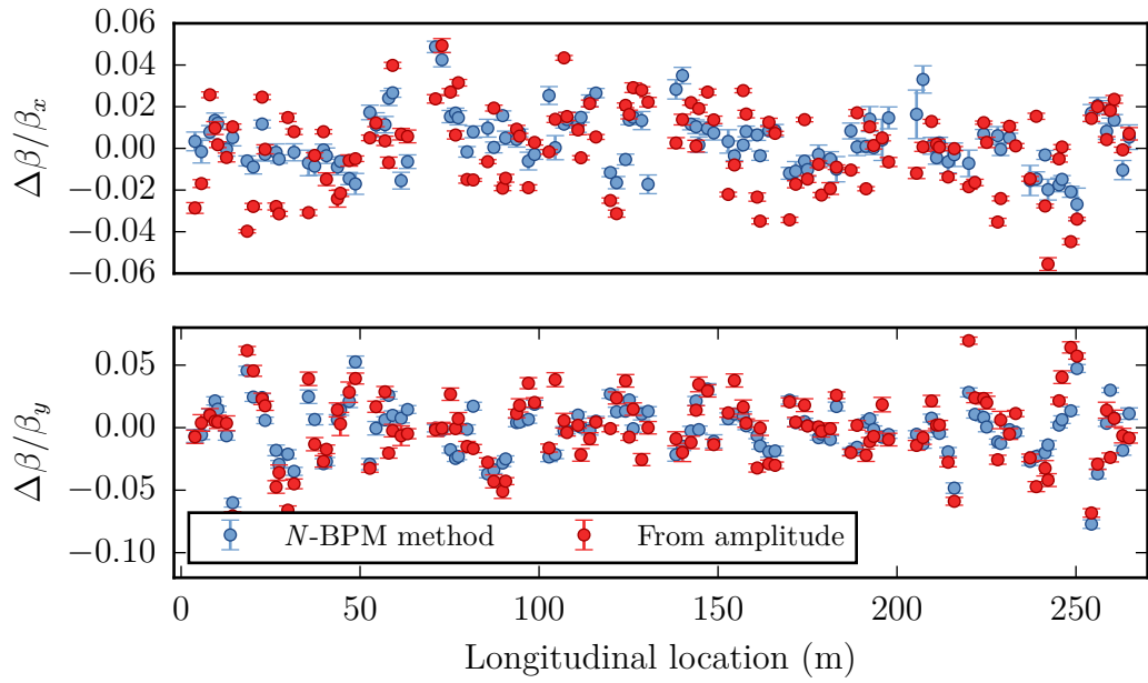
Figure 2.24.: Comparison of the \beta -beating as derived from BPM turn-by-turn data using either the amplitude information or phase of the betatron oscillation ( N -BPM method).
