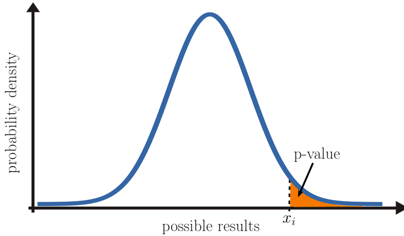
Figure A.1.: Illustration of the p-value for the observed result x_i , where a more extreme results would be larger than x_i .
