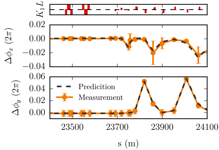
Figure 4.3.: Deviation of the propagated phase advance in SbS after local corrections for ATS optics for beam 1 at \beta^* = 20 cm. For successful corrections a flat line would be expected, cf. Section 1.3.1. Due to a wrong magnet setting in the corrections, the actual prediction of the phase deviation differs from this expectation. However, it is in excellent agreement with the measurement.
