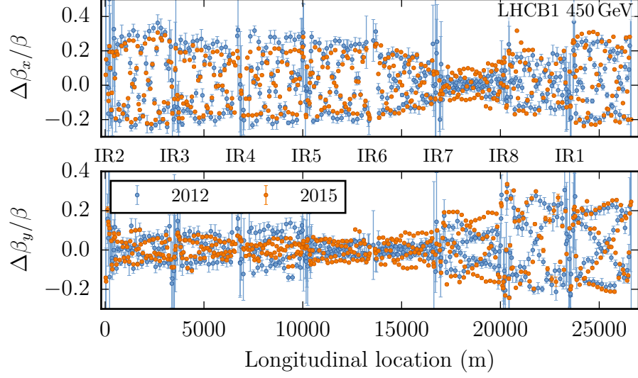
Figure 3.3.: \beta -beating at injection for beam 1. The measurement from 2015 was analyzed with the N -BPM method, while the one from 2012 used the previous neighboring BPM method.
