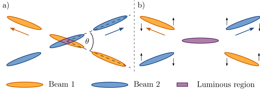
Figure 4.1.: Illustration of bunch crossings at an IP. In a) the effect of the crossing angle \theta between the beams is shown, which reduces the luminous region where particle collisions occur. The luminous region becomes smaller for larger crossing angles. In b) the same setting is shown with additional crab cavities before and after the crossing. The transverse deflection of the bunches allows effectively for head-on collisions and compensates the luminosity reduction due to the crossing angle.
