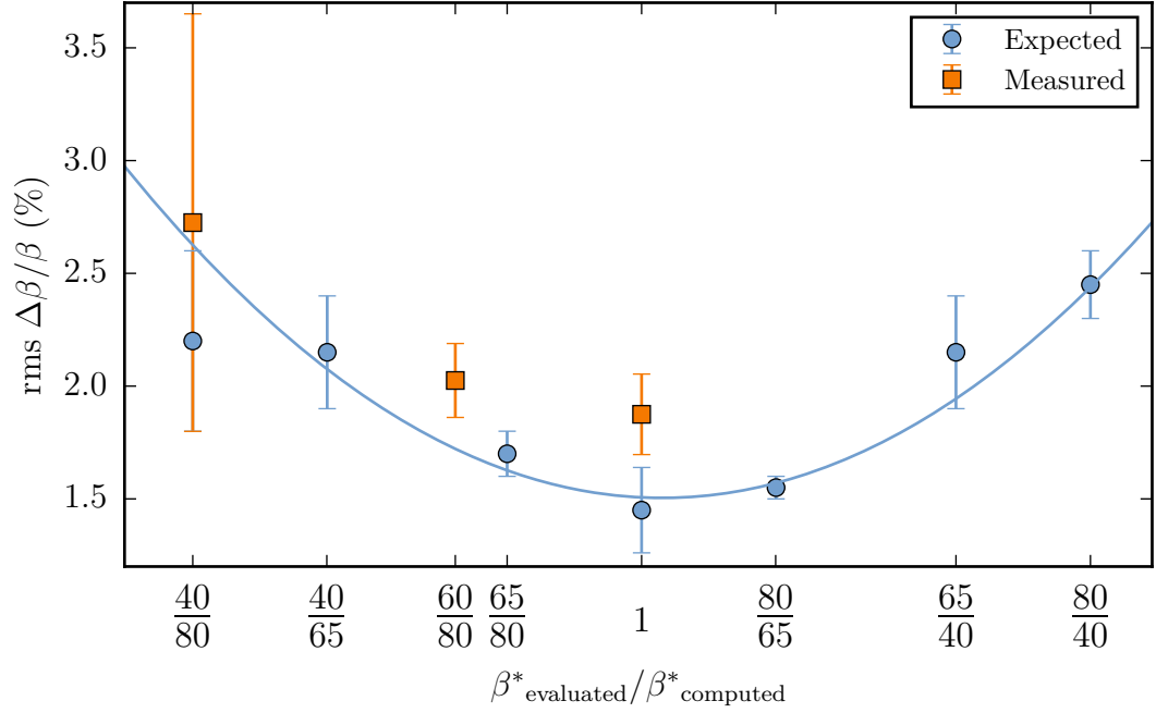
Figure 3.7.: The expected rms \beta -beating is shown for different \beta^* after evaluating different global corrections which have been computed from measurements at a \beta^* of either 80 cm, 65 cm or 40 cm. A fit with a parabola in a logarithmic horizontal axis is shown. The expected \beta -beating at \beta^*_{\text{evaluated}}/\beta^*_{\text{computed}} = 1 includes the three cases of evaluating the global correction for the same optics from which they were computed. The measured rms \beta -beating is shown for the three cases of applying the global corrections computed at \beta^* = 80 cm to the three optics with a \beta^* of 80 cm, 60 cm and 40 cm.
