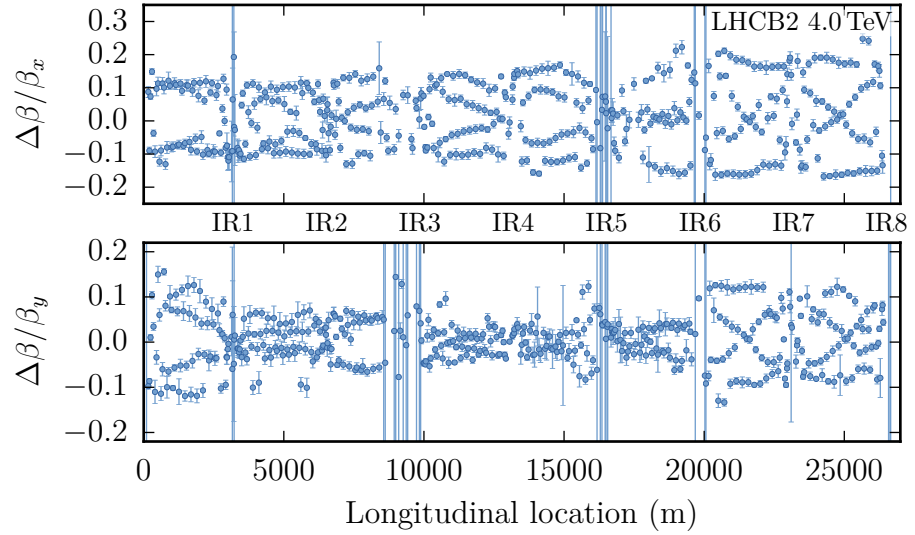
Figure B.16.: Beta-beating for beam 2 for ATS optics with \beta^* = 40 cm.
