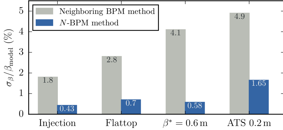
Figure 3.2.: Average uncertainty of the measured \beta -functions for different measurements from 2012.
