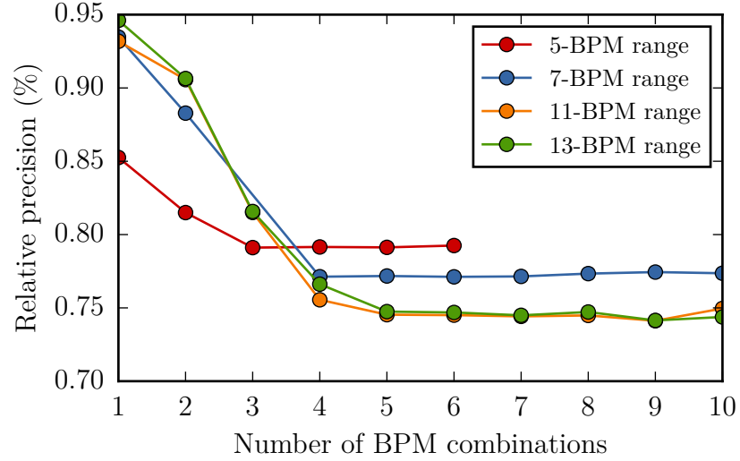
Figure 2.13.: Precision of the derived \beta -functions from simulations for different ranges of BPMs and different amount of BPM combinations. The oscillation amplitude was 1 mm in the arcs and a Gaussian noise of 200 \mu\text{m} was applied.
