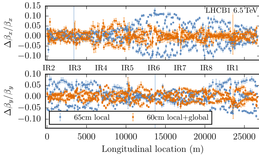
Figure B.6.: \beta -beating after local and global optics corrections along the machine for beam 1 at a \beta^* of 60 cm.
