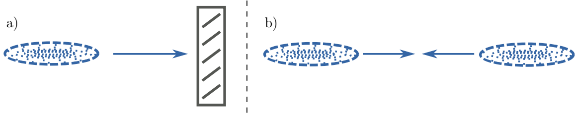
Figure 1.2.: Illustration of a collision experiment where particles either collide a) with other particles which are in rest (fixed target), or b) head on with particles of same momentum.
