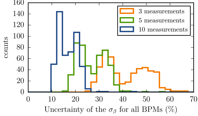
Figure 2.5.: The distribution shows for all BPMs the width of the deviation of the derived uncertainty of the \beta -function compared to the calculated error bar from the known phase uncertainty.
