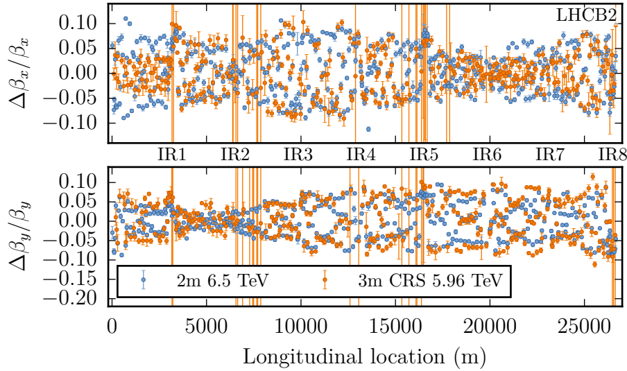
Figure B.14.: Beta-beating for beam 2 during the CRS at an energy of 5.96 TeV and a \beta^* of 3m in IP1 and IP5 in comparison to a static measurement at 6.5 TeV with a \beta^* of 2m.
