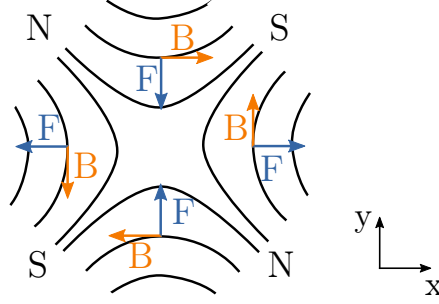
Figure 1.4.: Magnetic field lines of a quadrupole magnet. The resulting force is indicated for a positively charged particle moving perpendicular into the drawing plane. Particles with a transverse offset from the quadrupole center will be focused in the vertical plane and defocused in the horizontal plane.
