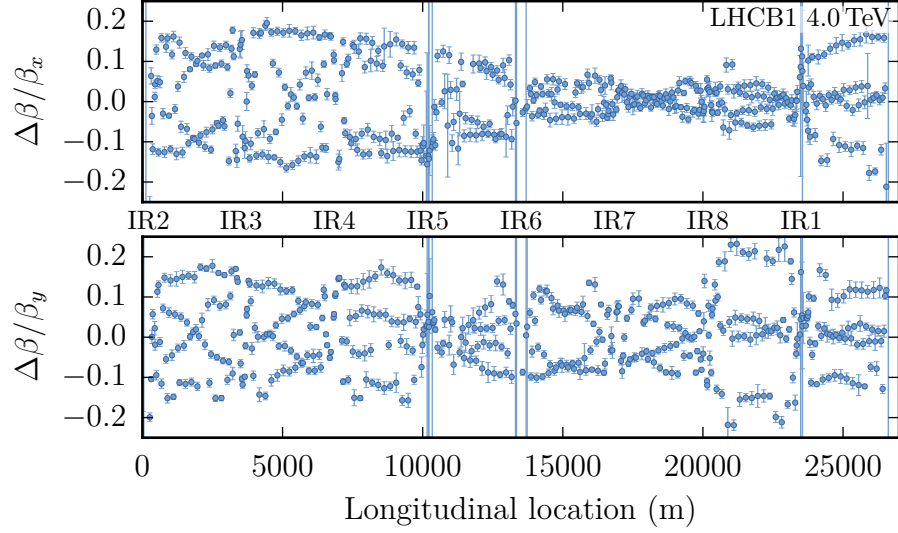
Figure B.15.: Beta-beating for beam 1 for ATS optics with \beta^* = 40 cm.
