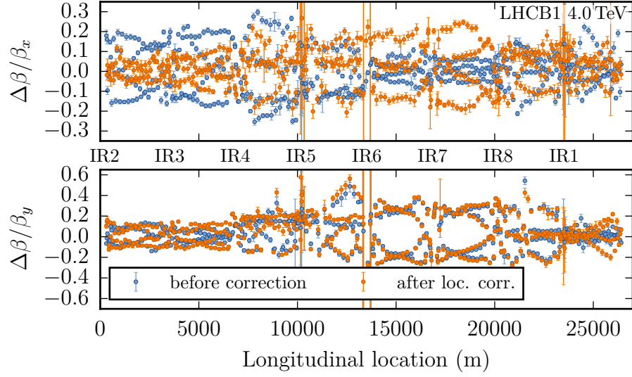
Figure 4.2.: Beta-beating for beam 1 for ATS optics with \beta^* = 20 cm, before and after local corrections.
