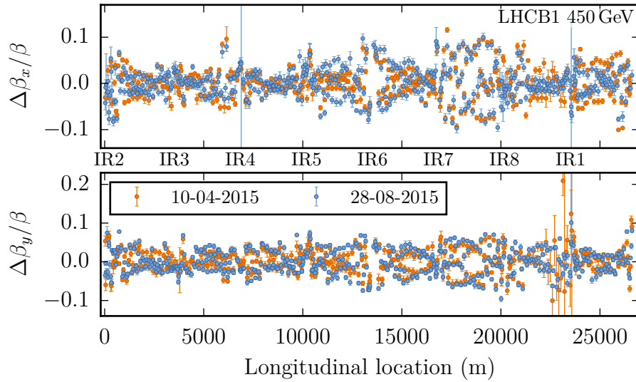
Figure 3.19.: Repeated measurement of the \beta -beating for beam 1 at injection after a time period of 4 months.
