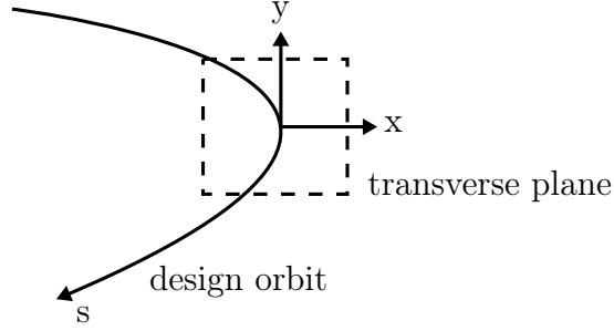
Figure 1.3.: Schematic of the Frenet-Serret coordinate system, which is used to describe the particle motion in an accelerator in the vicinity of a design orbit.
