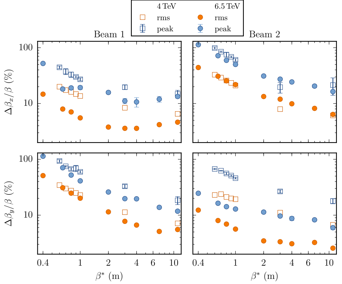
Figure 3.5.: Measured peak and rms \beta -beating before optics corrections. Values are given for different \beta^* along the squeeze. Measurements at 4 TeV were performed in 2012, and at 6.5 TeV in 2015.
