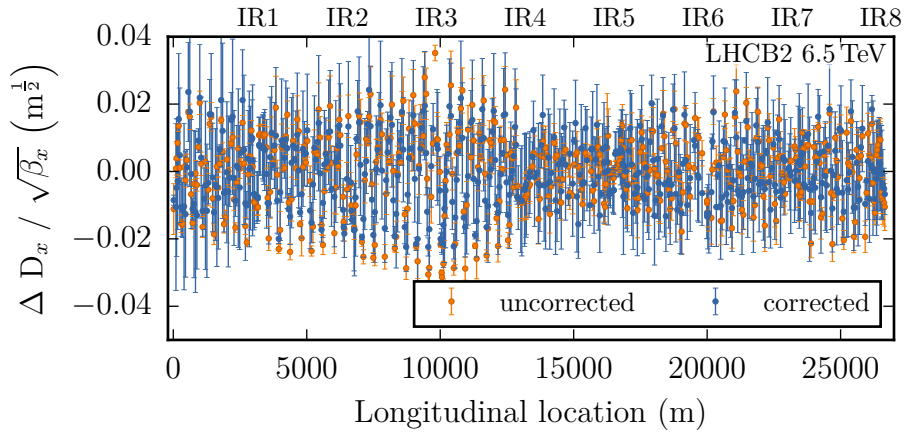
Figure 3.8.: Normalized dispersion before and after global corrections for beam 2 and \beta^* = 80 cm.
