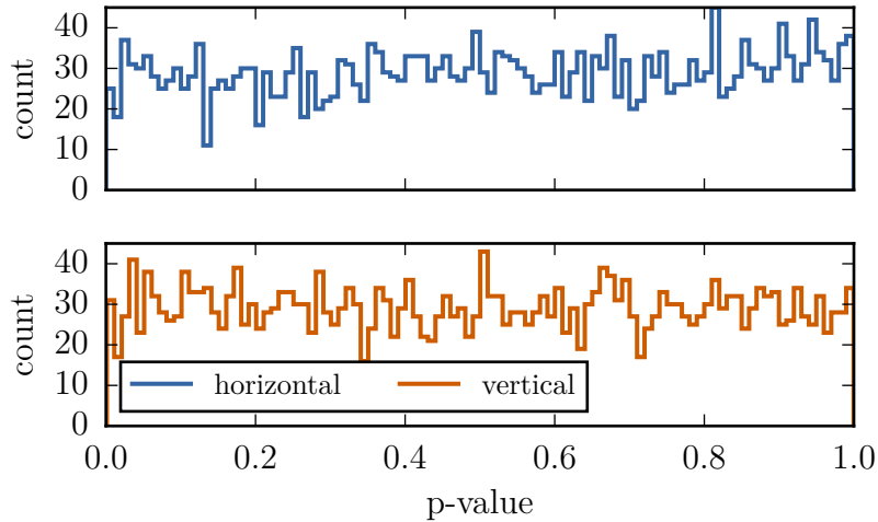
Figure 3.14.: Distribution of the p-values for a linear regression of the measured phase advances from six consecutive TbT analysis of 1100 turns each. The data was generated by splitting a measurement of 6600 turns into six pieces. The plot shows the case of a \beta^* of 80 cm for beam 1.
