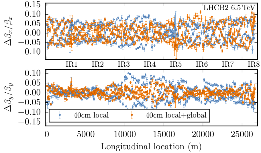
Figure B.5.: \beta -beating after local and global optics corrections along the machine for beam 2 at a \beta^* of 40 cm.
