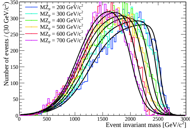
Figure 9.11: Event invariant mass spectra for various Z' masses.
