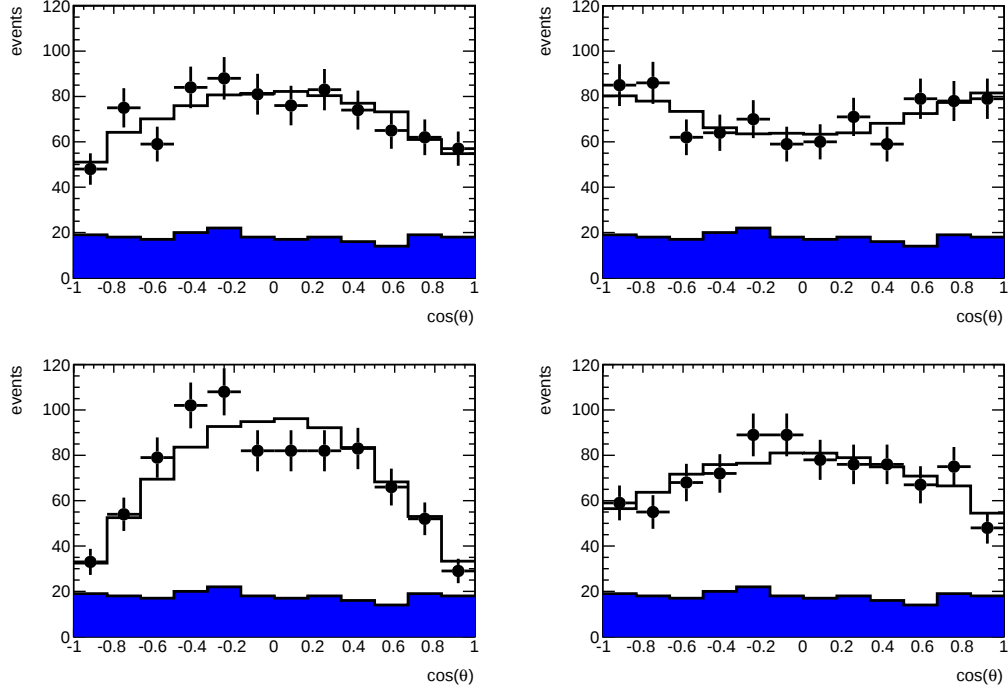
Figure 5.9: Example simulated events superimposed on reference histogram scaled to 100 \text{ fb}^{-1} for the four different coupling types. The ZZ background is added to the signal histogram, and is shown overlayed in blue. Clockwise from top left: Standard Model, CP Odd, CPV, CP Even.
