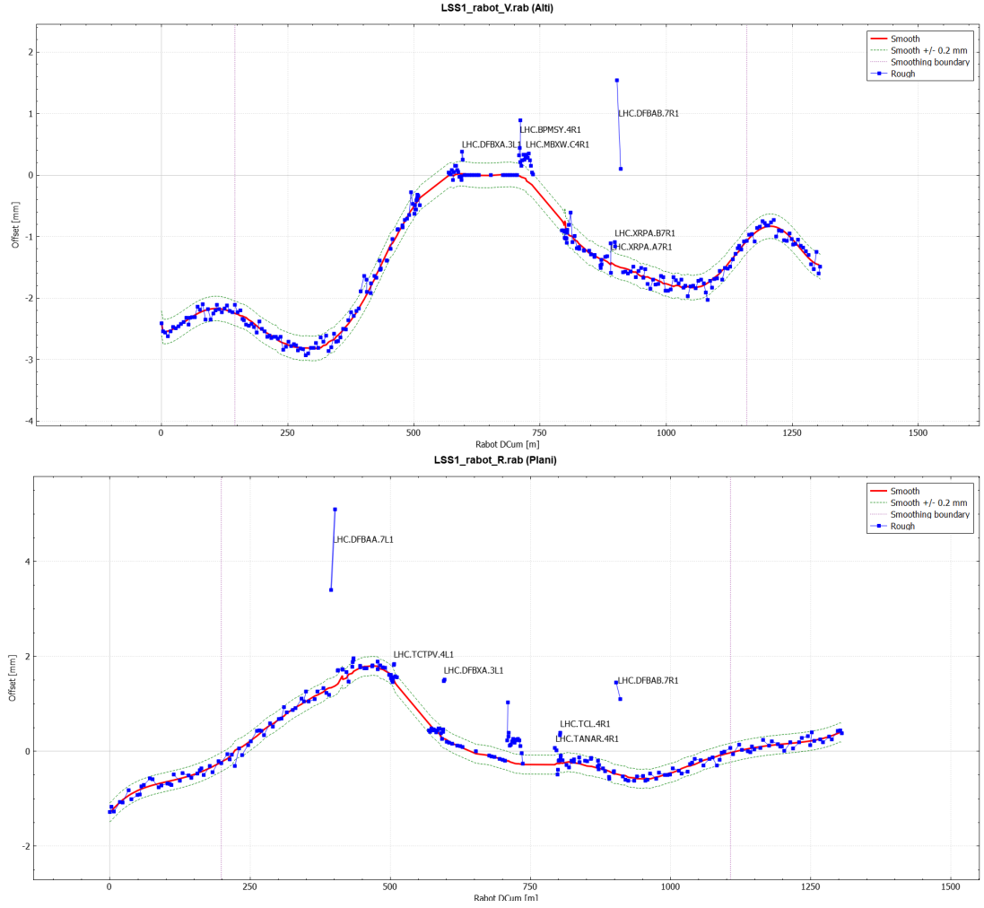
Figure A.5: Vertical ( top ) and horizontal ( bottom ) positions of LHC elements as measured during the 2022 laser survey campaigns. ATLAS collision point is located around 650 m.
