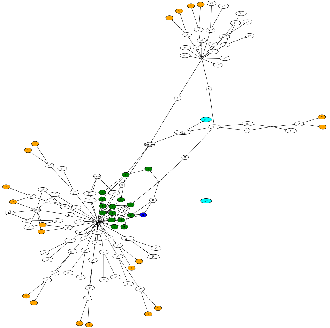
Figure 4.2: Single diffractive di-jet event generated by Pythia 8. All generated particles are shown, with lines indicating the mother-daughter relation. The reconstructed jets are represented as bulbs named “system”; lines directly connected to these bulbs indicate which final state particles were used for their reconstruction.
