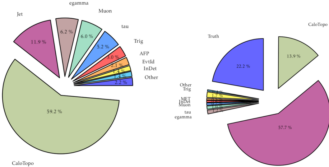
Figure 4.3: Structure of ATLAS STD6 derivation designed to be used in the low- \mu diffractive analyses: the data are on left and Monte Carlo on right .
