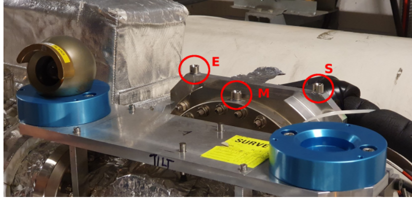
Figure B.1: Survey measurement of the positions implemented in 2019: inlet (E – fr. entrée ), middle (M – milieu ) and outlet (S – sortie ) reference points positioned along the top surface of the Roman Pot. This configuration enabled precise tracking of pot rotation through multiple measurement positions, with coordinates recorded relative to the beam pipe centre.
