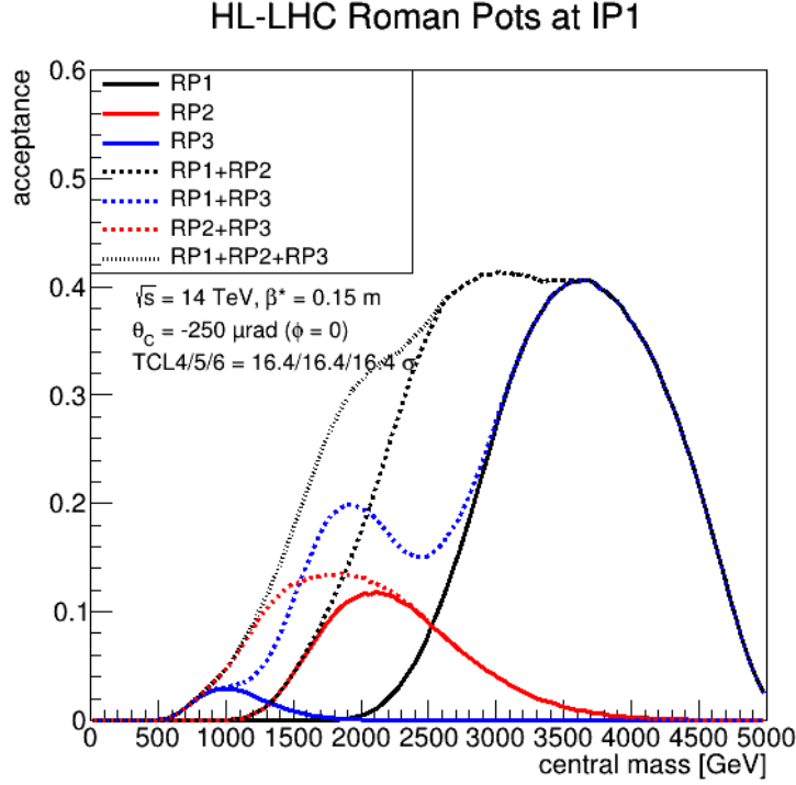
Figure C.4: Mass acceptance for various combinations of stations near IP1 for the horizontal crossing angle with \phi=0 .
