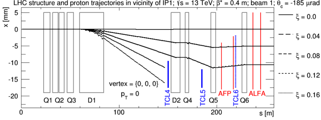
Figure A.1: The LHC beam-line in the vicinity of the ATLAS collision point. Proton trajectories are plotted for LHC Run 2 optics: \sqrt{s} = 13 TeV, \beta^* = 0.4 m and \theta_C = -185 \mu rad. From [94].
