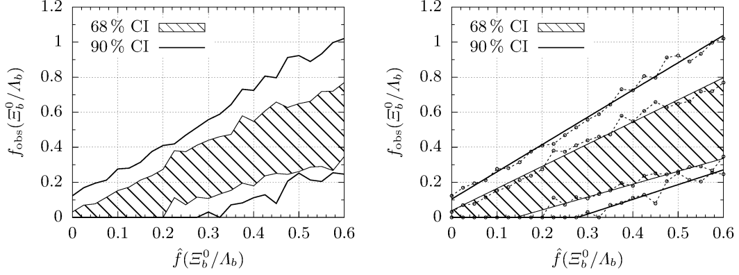
Fig. S.2. Frequentist CIs using the shortest method. Interval boundaries are estimated by finding the shortest intervals in f_{\text{obs}}(\Xi_b^0/\Lambda_b) with a coverage of 68 % and 90 % at 25 different \hat{f}(\Xi_b^0/\Lambda_b) positions. The boundaries (left) are smoothed with linear functions (right).
