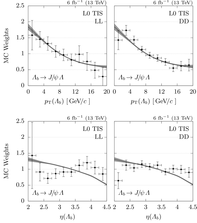
Fig. 4.12. Averaged fit results of weights for \Lambda_b \rightarrow J/\psi \Lambda (simultaneously for LL and DD tracks) and \Lambda_b \rightarrow D^0 p K^- events (taken from Ref. [74]).
