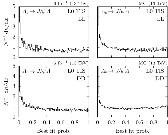
Fig. D.2. Fit probability of LL and DD tracks (top and bottom), and for recorded data (left) and truth-matched, simulated events (right).
