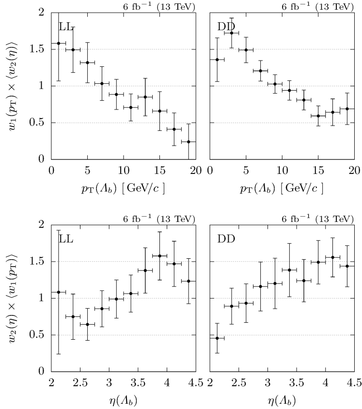
Fig. 4.10. Product of w_1(p_T) and the mean of w_2(\eta) (top) and vice versa (bottom) for LL (left) and DD (right) tracks.
