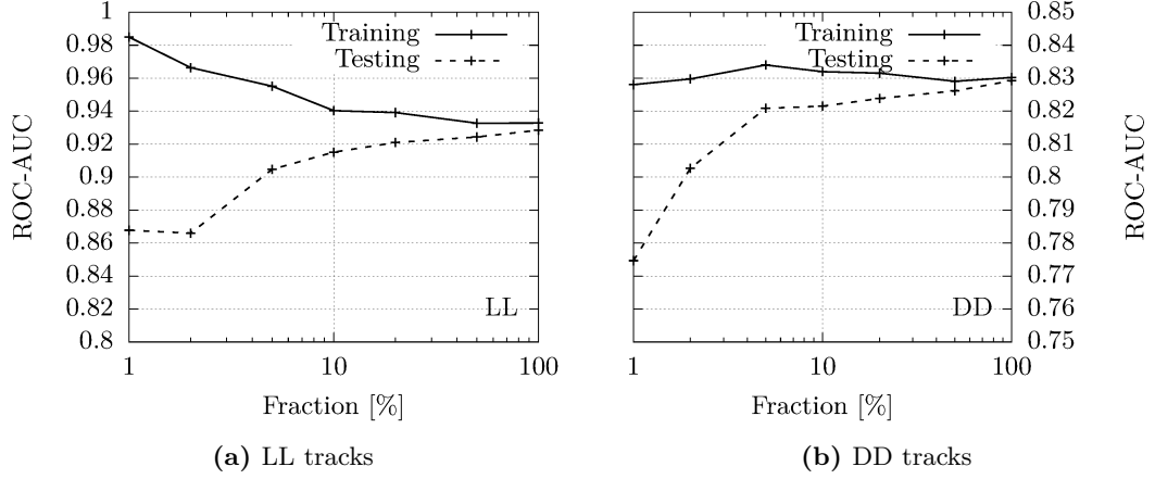
Fig. 5.8. Convergence of the SVMs ( A classifier) given by the ROC-AUC values for different sample sizes where a sample size of 100 % corresponds to the size of the full trainings set. The ROC-AUC is evaluated via a 5-fold cross-validation scheme on the training set (solid line) and testing folds (dashed line).
