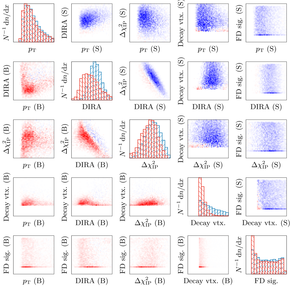
Fig. 5.13. Marginal and linear correlation distributions of the feature space ( \Lambda classifier) before applying PCA transformation for LL tracks. In the correlation distributions misclassified events are color-coded in red (signal events classified as background) and blue (background events classified as signal) when using a threshold of zero.
