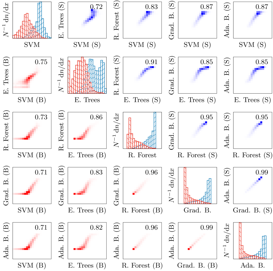
Fig. L.1. Distributions of the responses and correlations of the tier 1.1 \Lambda classifiers for LL tracks, separated for signal (S) and background (B). On top of the correlation distributions we show the PCC as a measure for the linear correlation.
