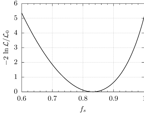
Fig. S.3. Normalized log-likelihood ratio of f_s as estimated by the fitting procedure. The normalization is chose such that intervals using the likelihood ratio method can directly be read off the y -axis.
