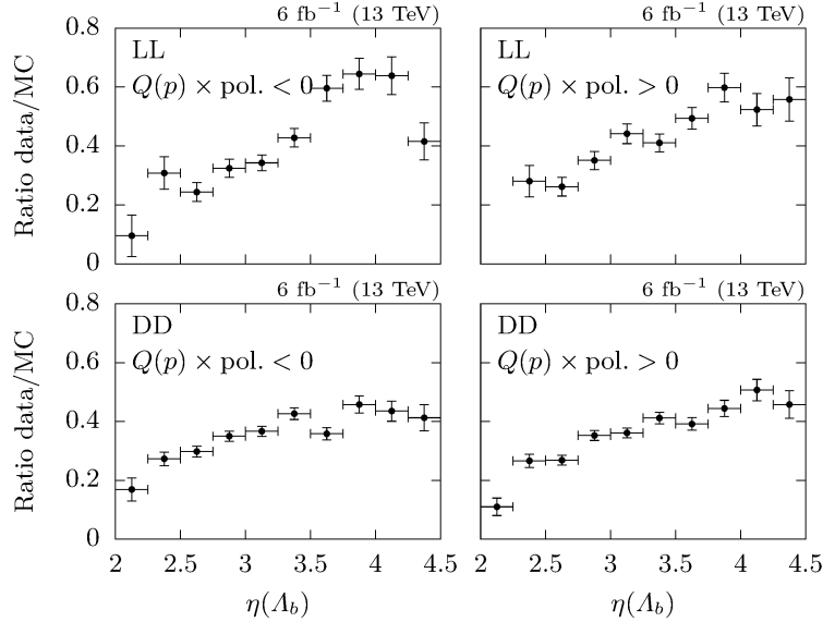
Fig. F.4. Samples split w.r.t. the sign of the product of proton charge and magnet polarity.
