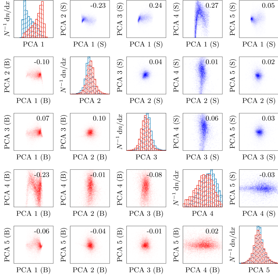
Fig. L.4. Distributions of the responses and correlations of the tier 1.1 \Lambda classifiers for DD tracks after PCA transformation, separated for signal (S) and background (B). On top of the correlation distributions we show the PCC as a measure for the linear correlation.
