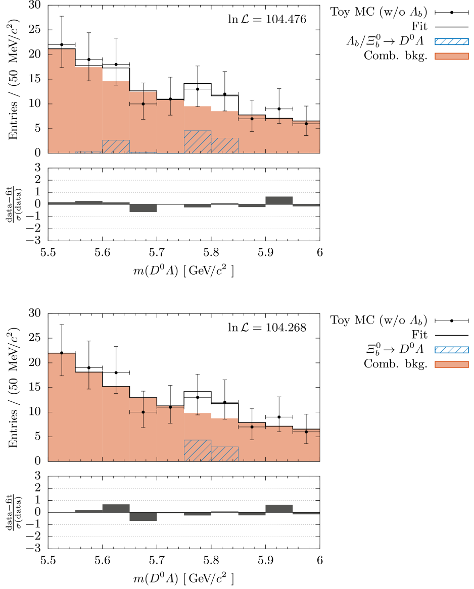
Fig. P.11. Example of a distribution (data points) that was generated as part of the pseudo-experiment to test the validity of the signal yield significance of the \Lambda_b \rightarrow D^0 \Lambda mode. During generation this mode was kept disabled (null hypothesis). The distribution is fitted twice, first with the \Lambda_b signal component enabled (top) and once with disabled \Lambda_b signal component (bottom). The difference in the log-likelihood values is then used to benchmark the null-hypothesis.
