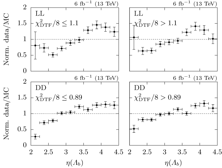
Fig. F.2. Ratios of recorded data and simulated events, parametrized in \eta(\Lambda_b) for lower and upper 50 % quantiles of \chi^2_{\text{D}_{\text{TF}}}/\text{DoF} .
