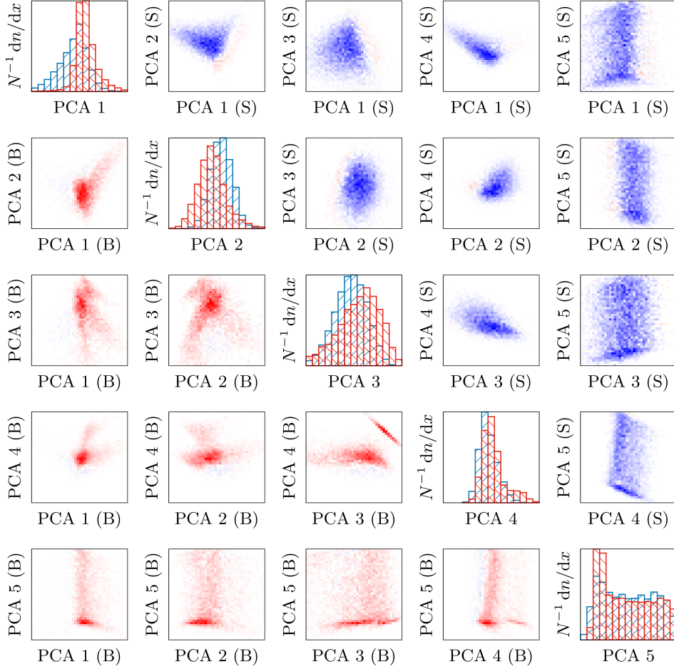
Fig. 5.15. Marginal and linear correlation distributions of the PCA components ( \Lambda classifier) for LL tracks. In the correlation distributions misclassified events are color-coded in red (signal events classified as background) and blue (background events classified as signal) when using a threshold of zero.
