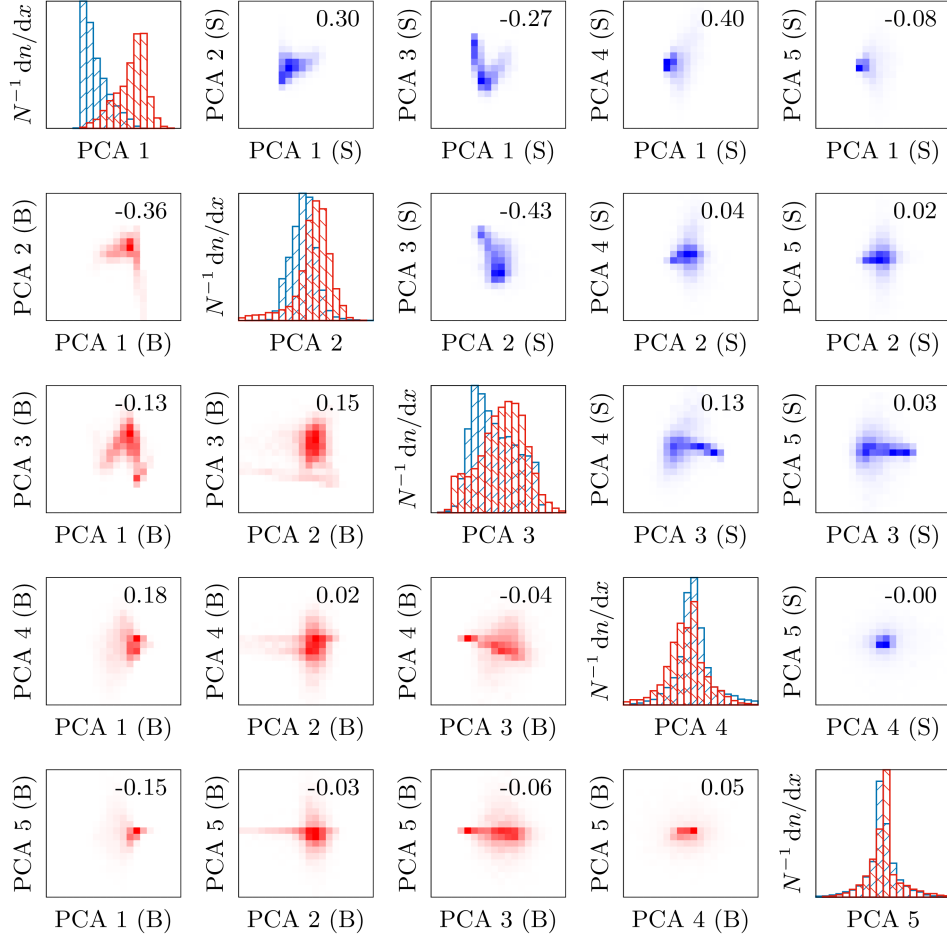
Fig. L.3. Distributions of the responses and correlations of the tier 1.1 \Lambda classifiers for LL tracks after PCA transformation, separated for signal (S) and background (B). On top of the correlation distributions we show the PCC as a measure for the linear correlation.
