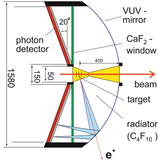
Figure 3.3: Schematic layout of the RICH detector. The Cherenkov light of the positron is reflected at the mirror and focused to a ring on the readout pads.
