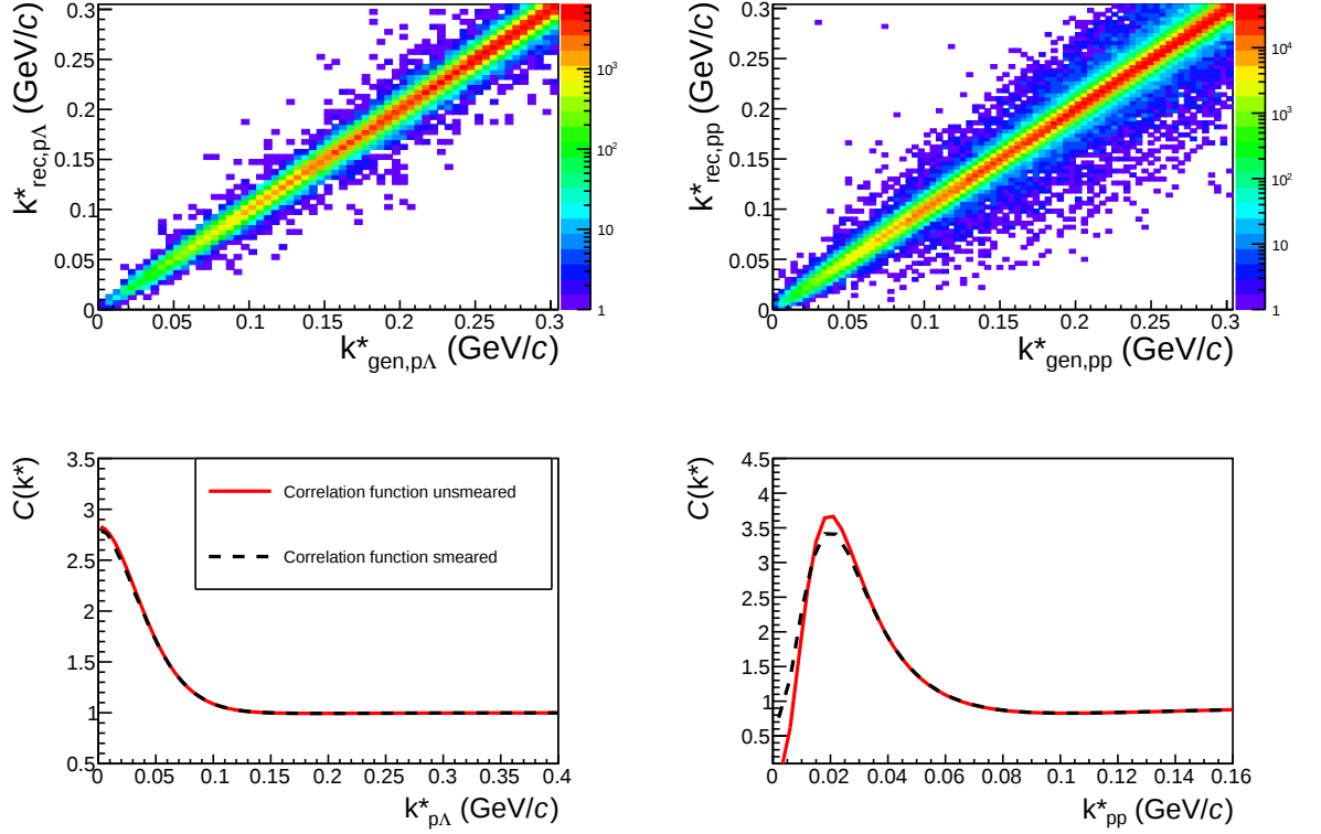
Figure 6.29: Top: Resolution matrices for p - \Lambda and p - p . Bottom: Influence of the momentum resolution on the correlation functions.
