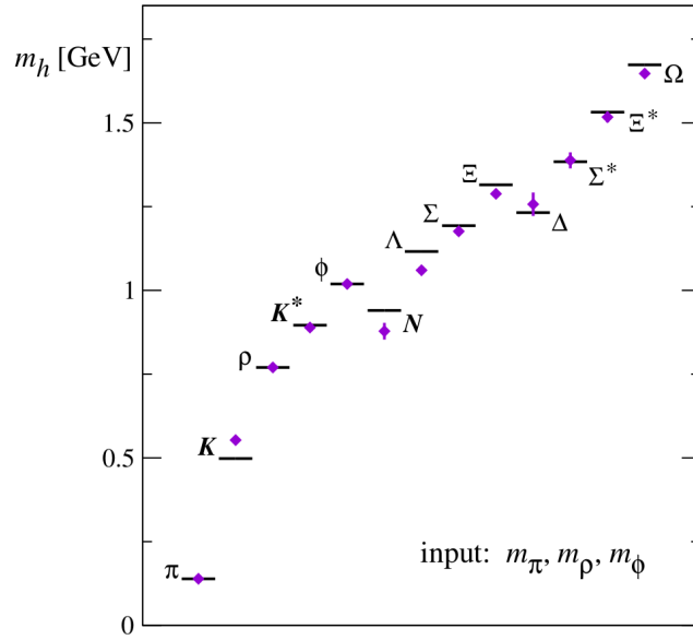
Figure 1.2: Comparison of predictions from lattice QCD (points) to experimental results (horizontal lines). Taken from [Lus03].
