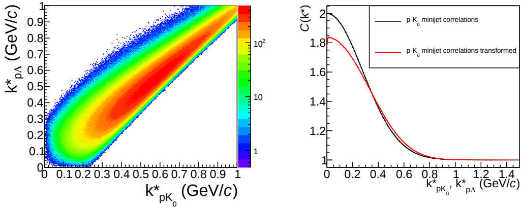
Figure 6.3: Results from a Toy Monte Carlo study. Left: Matrix presenting the correlation between k^* of an initial momentum p - K_S^0 transformed to p - \Lambda . Right: A broad simulated mini-jet background present in p - K_S^0 survives the transformation to the p - \Lambda momentum basis.
