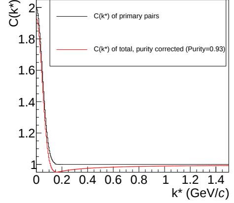
Figure 6.15: For lower purities (Purity=0.93) residual correlations from impurities start to play a role. The two correlation functions do not coincide anymore.
