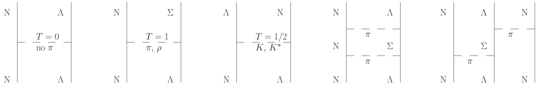
Figure 1.11: Feynman diagrams to describe the \Lambda N interaction. Taken from [GHM16].
