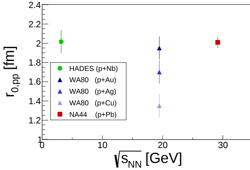
Figure 4.29: Comparison of the extracted source radius to measurements of other radii from p+A collisions.
