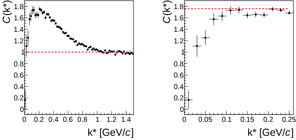
Figure 6.9: Left: The \bar{\Lambda} - \Lambda correlation function. Also for this pair a strong contribution from mini-jets is visible, showing up as a broad correlation signal starting at k^* \sim 1 GeV/c. Right: Same correlation function zoomed to small relative momenta. One can see a correlation signal having femtoscopic signatures on top of the mini-jet background.
