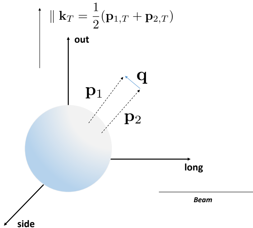
Figure 2.13: Definition of the longitudinally-comoving-system. The “long” component is aligned with the beam direction, “out” is parallel to the pair transverse momentum and “side” perpendicular to the other two directions.
