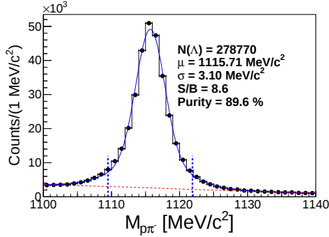
Figure 4.4: p-\pi^- invariant mass spectrum for combination 2 of topological cuts.
