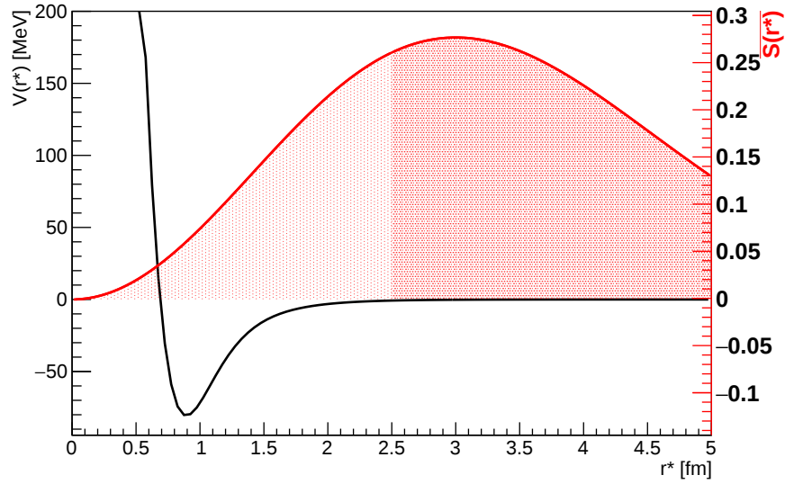
Figure 2.9: The black function represents a typical short range nuclear potential and the red function corresponds to a pair distribution according to Eq. (2.29) for r_0 = 1.5 fm. A fraction of pairs is produced within the range of the potential and the rest in a region where it vanishes. This plot demonstrates that at some point the assumption of the asymptotic form of the wave function breaks down if the potential strength becomes non-negligible.
