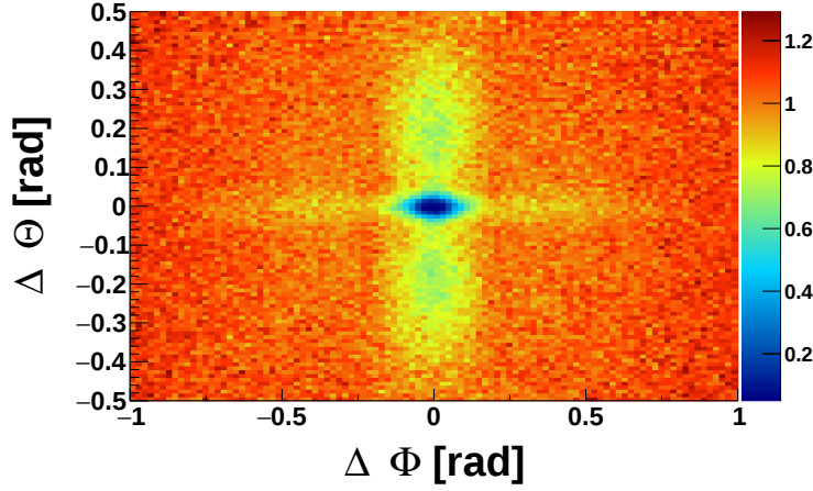
Figure 4.7: Experimental correlation function in (\Delta\phi, \Delta\Theta) for p-p pairs.
