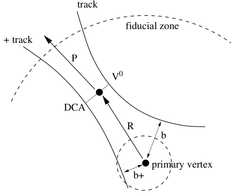
Figure 6.2: Sketch of a V0 decay and its vertex selection taken from [Cor+06]. Only V0 vertices inside a fiducial volume are kept and the daughter tracks have to have some minimum impact parameter to the primary vertex. The distance of closest approach of the daughter tracks should not exceed a maximum value.
