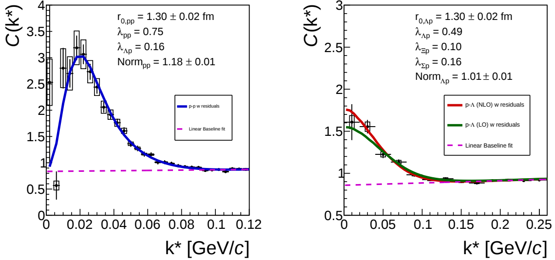
Figure 6.33: Simultaneous fit of the p-p and p-\Lambda pair with updated \lambda parameter, where the NLO expansion (red line) is used for the scattering parameter. After the fit is performed the LO parameter set (green line) is plugged in.
