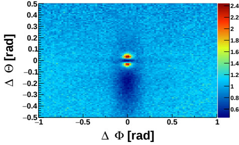
Figure 4.10: Experimental correlation function in (\Delta\phi, \Delta\Theta) for \pi^- - \pi^+ pairs..
