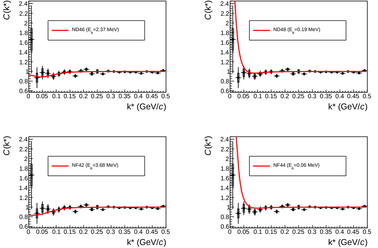
Figure 6.36: Comparison of the influence of the scattering parameters of Tab. 6.7 on the theoretical \Lambda - \Lambda correlation function.
