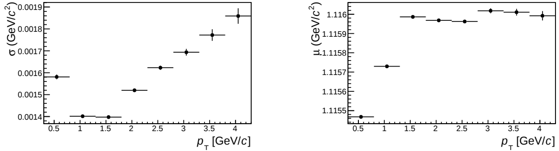
Figure 6.5: The resulting mean and variance of the \Lambda signal as a function of p_T .
