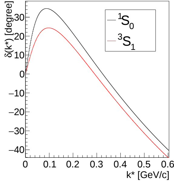
Figure 1.12: Phaseshift of Usmani potential of the form given in Eq. (1.10)
