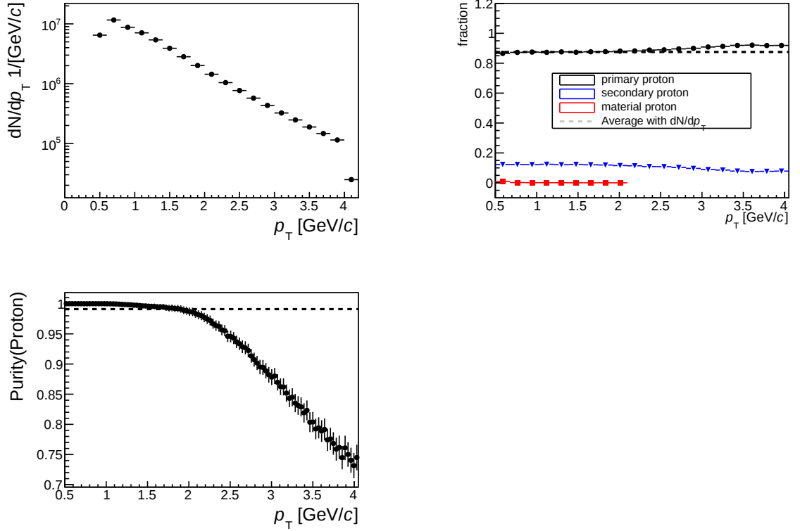
Figure 6.21: The fractions of protons as a function of p_T obtained from the template fitting method. The purity is extracted from Pythia. The averages of the quantities are obtained by using the production probability dN/dp_T of protons.
