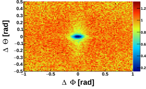
Figure 4.8: Experimental correlation function in (\Delta\phi, \Delta\Theta) for \pi^- - \pi^- pairs.
