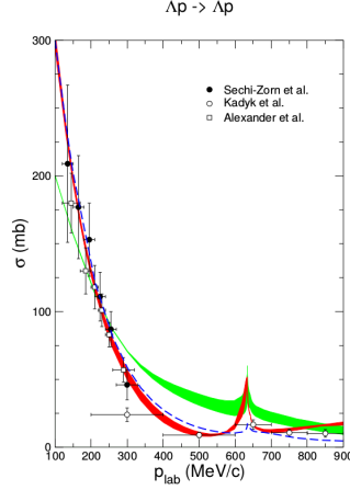
Figure 1.9: A comparison of the measurement of the elastic \Lambda p cross section to calculations from an chiral effective field theory prediction. The green band is for the leading order expansion whereas the red band represents the next-to-leading-order expansion. Taken from [Hai+13].
