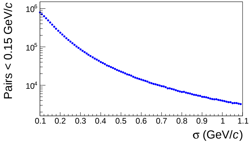
Figure 2.14: Number of proton pairs in the femtoscopy region k^* < 150 MeV/c as a function of the Gaussian momentum production width of the protons. The pair statistics in the femtosopic range is highly non-linear.
