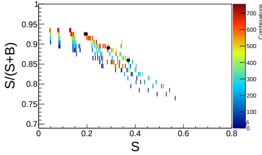
Figure 4.2: Purity as a function of the remaining signal for different topological cut selections. The black circles show the selected cuts.
