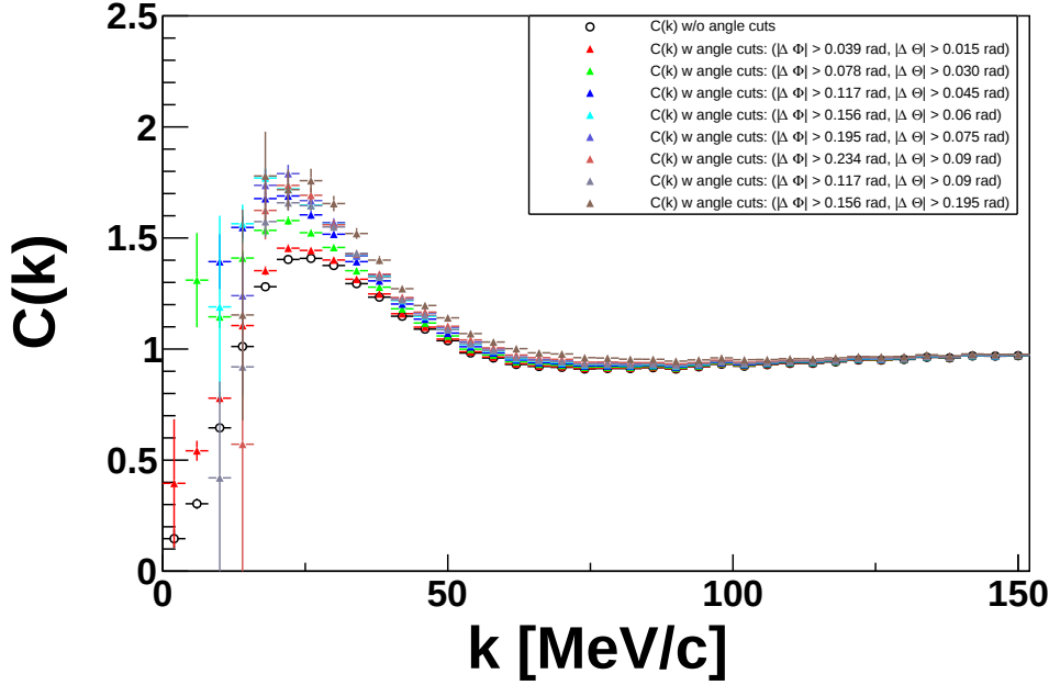
Figure 4.11: Experimental correlation p - p function with different cut selections on (\Delta\phi, \Delta\Theta) to reject close pairs.
