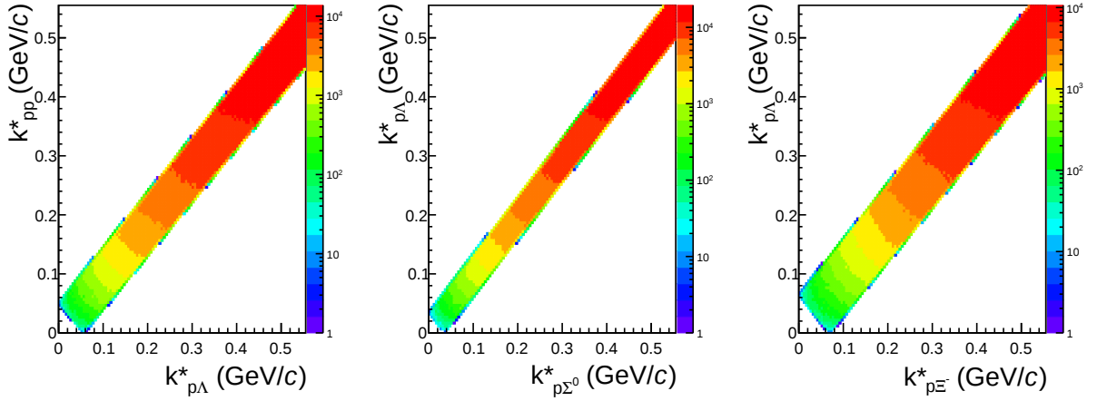
Figure 6.25: Transformation matrix M for p - \Lambda decaying into pairs of p - p (left) and p - \Sigma^0 (middle) p - \Xi^- (right) decaying in pairs of p - \Lambda .
