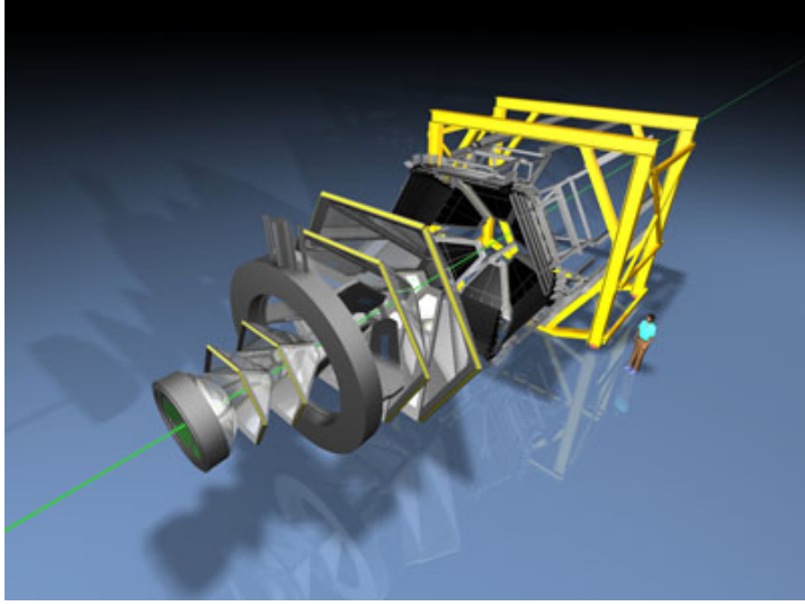
Figure 3.1: Setup of the HADES detector. The green line indicates the beam.
