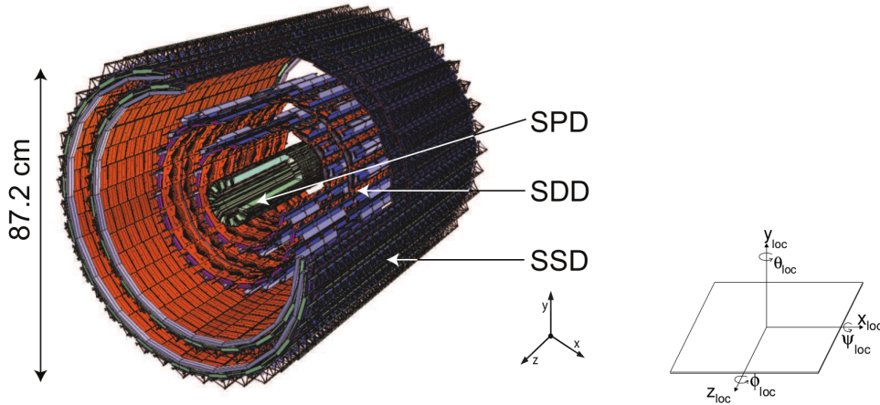
Figure 5.2: The structure of the Inner Tracking System (ITS) with its six layers SPD (two innermost), SDD (two intermediate), SSD (two outermost) [Aam+10].
