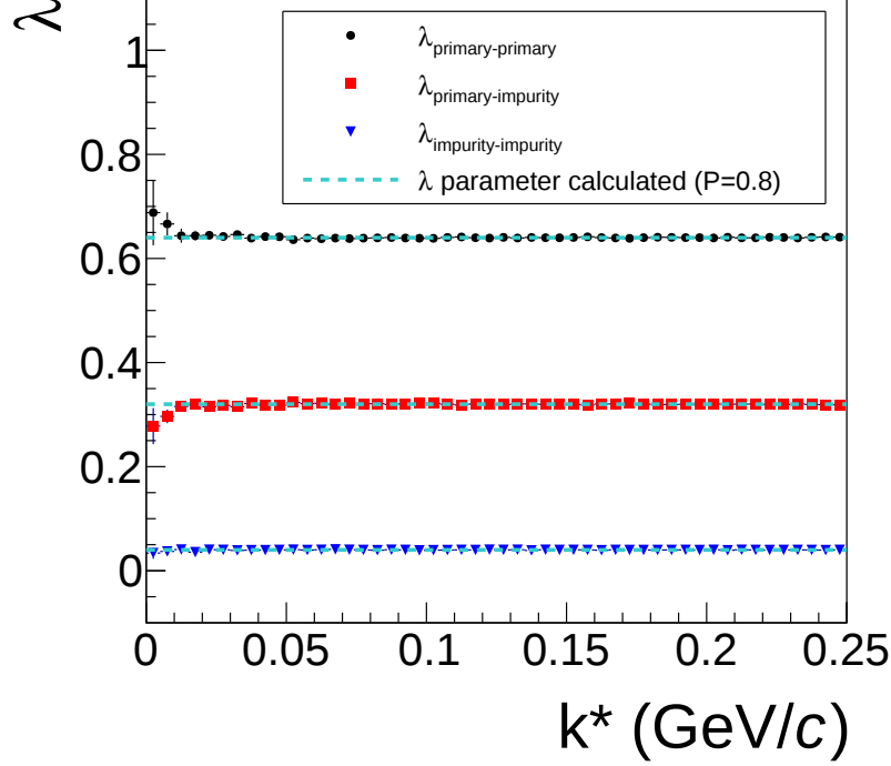
Figure 6.17: Comparison of the two methods to evaluate the \lambda parameter. The \lambda parameters presented as marker are the parameter using directly their definition. The dotted line shows the parameter by relating them to the single-particle purity \mathcal{P} = 0.8 .
