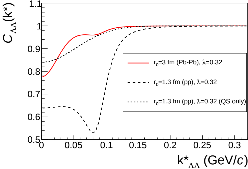
Figure 6.35: The \Lambda - \Lambda correlation function for two different source sizes. For the smaller source size the quantum statistics only correlation function is plotted only for comparison.
