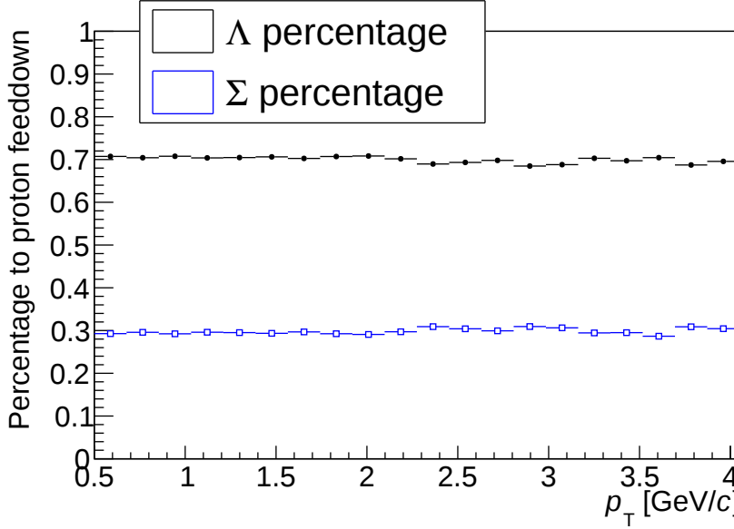
Figure 6.20: Percentage of feed-down to protons from \Sigma^+ and \Lambda as a function of p_T .
