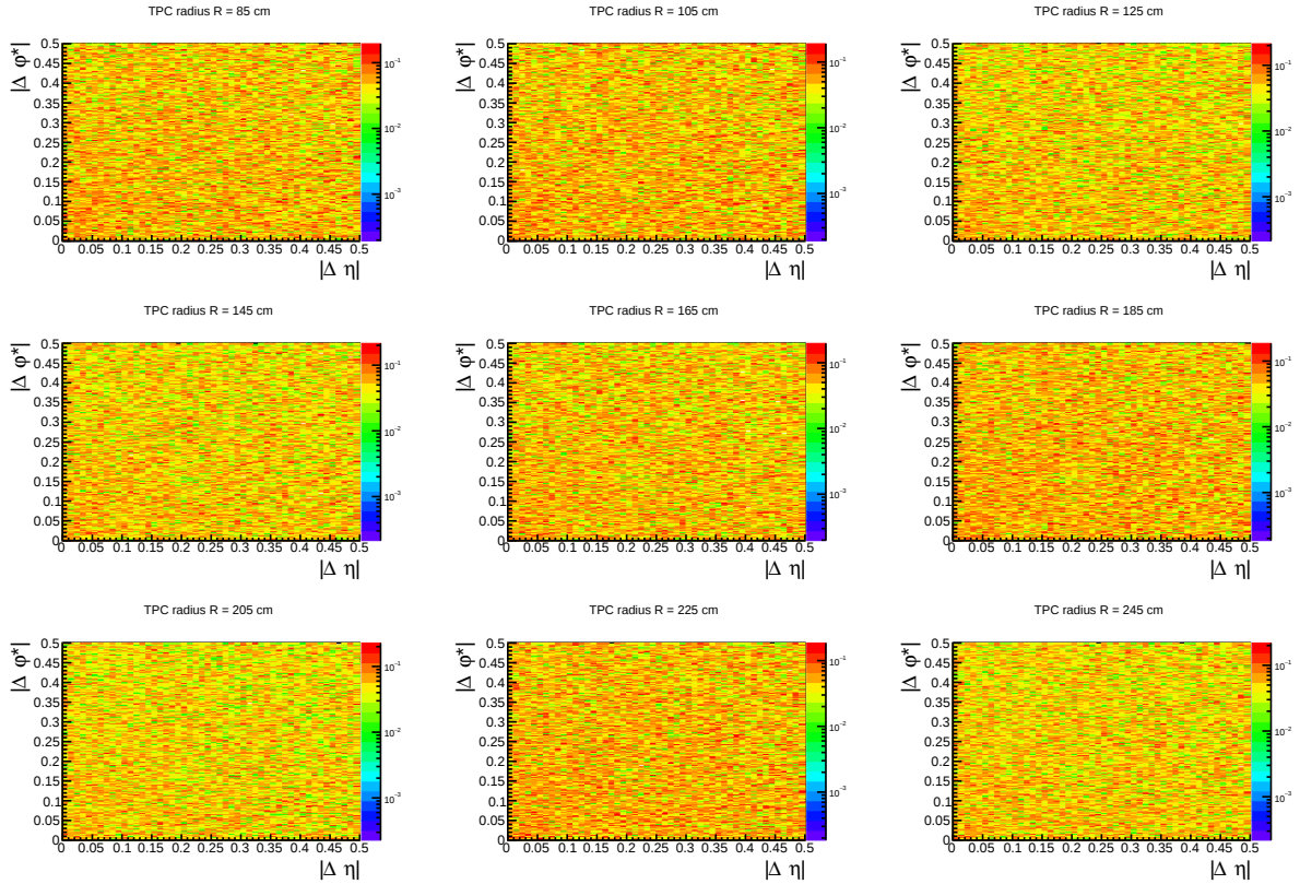
Figure 6.30: Correlation function for p-p in \varphi^*, \eta representation for Pythia simulations at different radii of the TPC. Merging or splitting would be visible at the origin (0,0).
