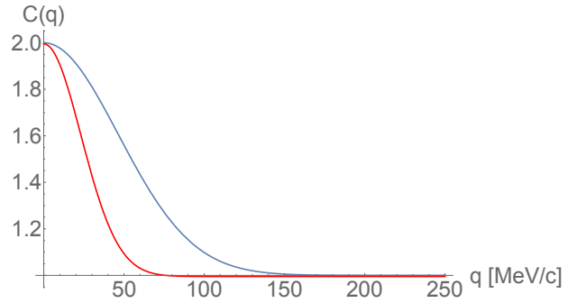
Figure 2.4: Correlation function for two identical bosons. The blue line is the quantum statistics correlation function for a Gaussian source size of r_0 = 1.5 fm and the red one for a source size of r_0 = 3 fm.
