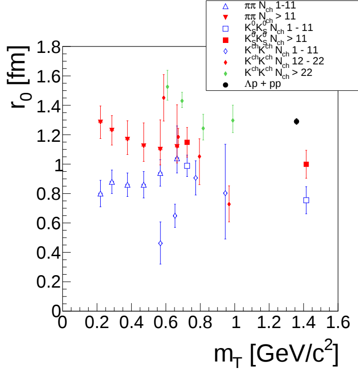
Figure 6.34: Comparison of radii obtained in the pp collision system at 7 TeV. The black point is the radius obtained in this analysis from p - p and p - \Lambda pairs.
