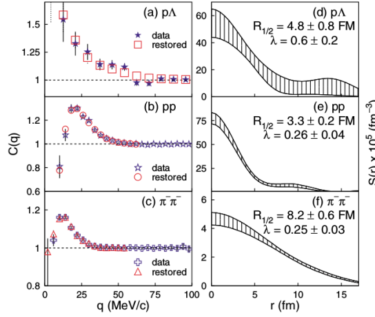
Figure 7.2: Correlation functions for p-p , p-\Lambda and \pi^-\pi^- and the corresponding source images. Taken from [Chu+03].
