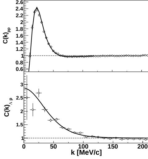
Figure 4.26: Model comparison of the p - p correlation function (top) and p - \Lambda (bottom) to extract the source size.
