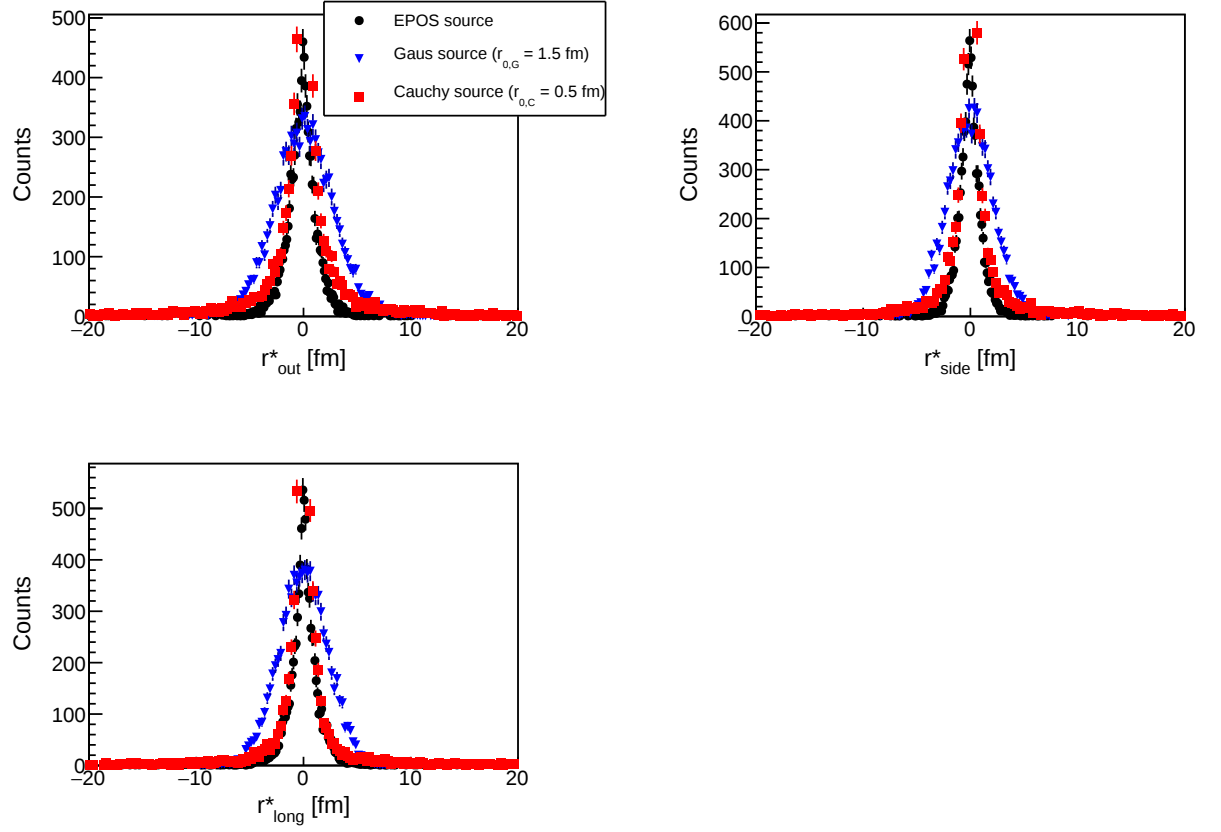
Figure 6.37: Comparison of freeze-out coordinates for p - p pairs predicted by the EPOS model compared to coordinates sampled from a Gaussian and Cauchy p.d.f. The coordinates are shown in cartesian coordinates.
