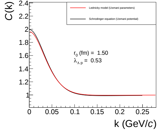
Figure 2.11: Comparison of the Lednicky model and the full solution of the Schrodinger Equation for a source radius of r_0 = 1.5 fm.
