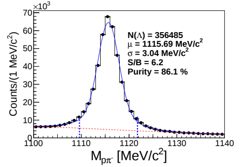
Figure 4.3: p-\pi^- invariant mass spectrum for combination 1 of topological cuts.
