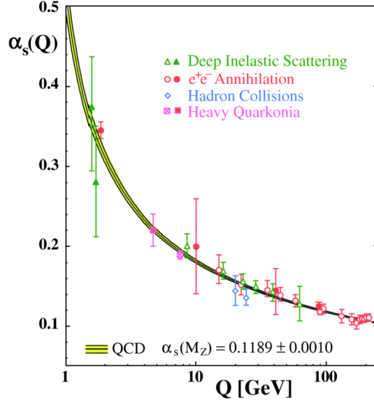
Figure 1.1: Running coupling from QCD compared to measurements. Taken from [Bet07].
