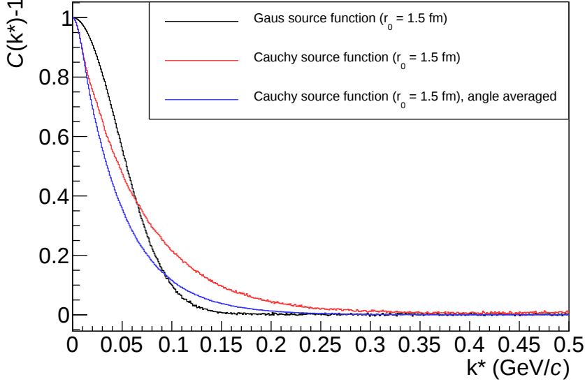
Figure 2.2: Bose-Einstein correlation function for a source size of r_0=1.5 fm calculated for single-particle emitters having a Gaussian and Cauchy shape. The influence on the correlation function is significant. For comparison also the correlation function obtained neglecting the typical angular behavior included in a Cauchy source function is displayed.
