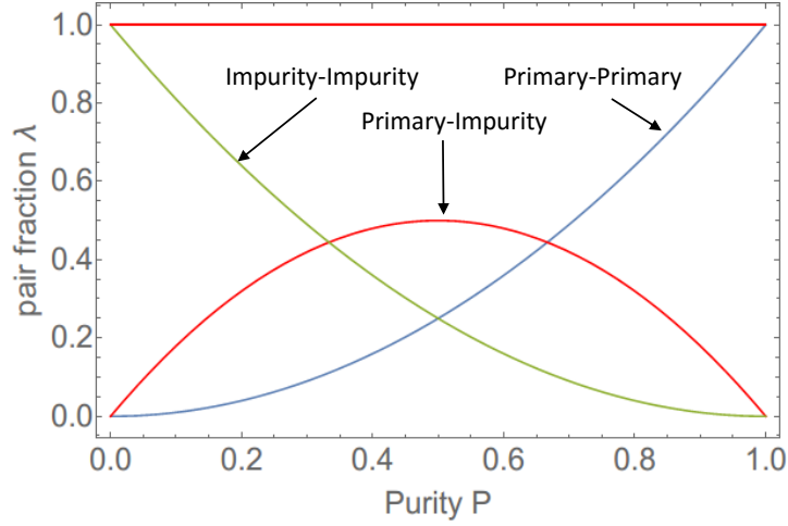
Figure 6.16: Decomposition of the correlation function given in Eq. (6.7) as a function of the single-particle Purity.
