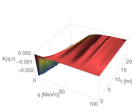
Figure 2.5: Kernel of the Coulomb interaction.
