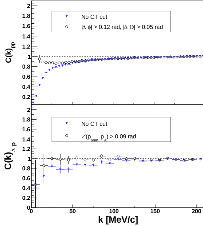
Figure 4.13: Correlation functions for p - p (top) and p - \Lambda (bottom) obtained from UrQMD and GiBUU (see text). One can see that a minimal cut on angles between the particles cures the track merging.
