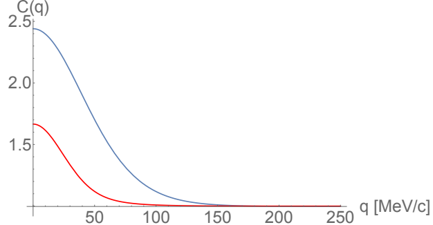
Figure 2.8: Strong interaction correlation function. The blue line is the strong interaction correlation function for a Gaussian source size of r_0 = 1.5 fm and the red one for a source size of r_0 = 3 fm. They were calculated using f_0 = 1.5 fm, d_0 = 2 fm.
