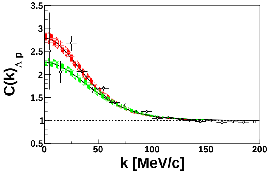
Figure 4.30: Influence of different sets of scattering parameter on the correlation function. The LO and NLO scattering length at a cutoff value of 600 MeV are taken from [Hai+13]. A small bug entered this figure, which is explained in the text.
