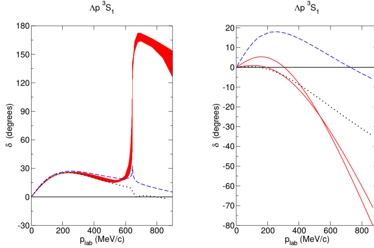
Figure 1.7: Phaseshift of the \Lambda p \ ^3S_1 state for the NLO model as well as Jülich '04 (blue dashed) and NSC97f (black dashed). Taken from [Hai+17].
