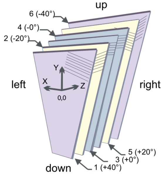
Figure 3.4: Schematic view of the drift chambers oriented at \pm 0^\circ , \pm 20^\circ , \pm 40^\circ .
