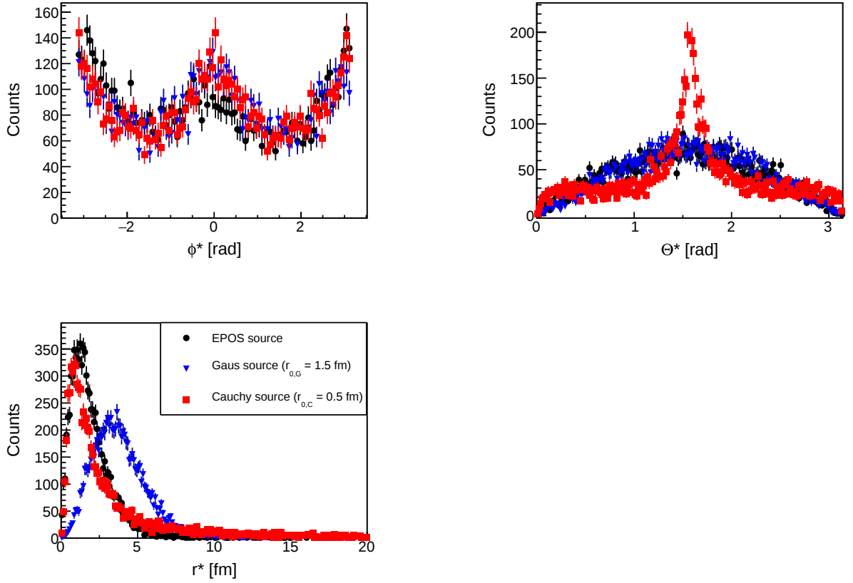
Figure 6.38: Comparison of freeze-out coordinates for p - p pairs predicted by the EPOS model compared to coordinates sampled from a Gaussian and Cauchy p.d.f. The coordinates are shown in spherical coordinates.
