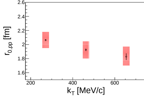
Figure 4.27: The p - p source size as a function of the total transverse momentum k_T .
