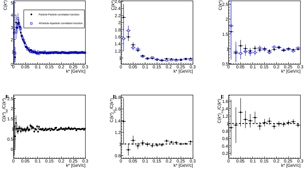
Figure 6.12: Baryon-Baryon and Antibaryon-Antibaryon correlation functions on the top and the corresponding ratios on the bottom. Left: (Anti)proton-(Anti)proton, Middle: (Anti)proton-(Anti)Lambda, Right: (Anti)Lambda-(Anti)Lambda.
