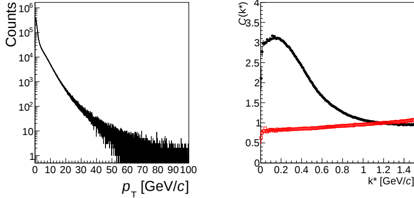
Figure 6.11: Left: Parton transverse momentum in Pythia. Right: Black dots represent the full \bar{p} - p correlation function from Pythia. The red squares show the correlation function obtained by requiring that the \bar{p} - p pair stem from different partons.
