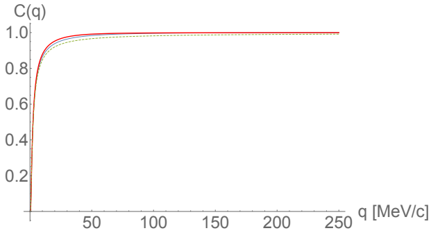
Figure 2.6: Coulomb correlation function. The green dashed line shows just the Gamov factor. The blue line is the Coulomb correlation function for a Gaussian source size of r_0 = 1.5 \text{ fm} and the red one for a source size of r_0 = 3 \text{ fm} .
