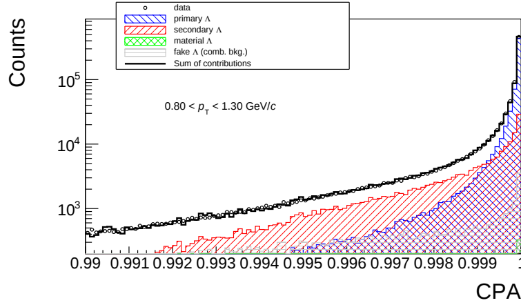
Figure 6.23: Template fit to the cosine pointing angle in a p_T interval.
