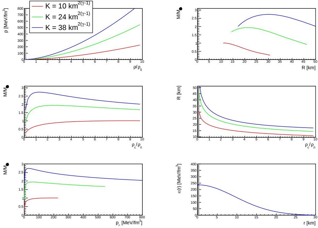
Figure 1.4: Neutron star properties for the EoS of Eq. (1.6) with \gamma = 5/3 . The energy density \epsilon(r) is calculated for the stiffest version of the EoS and the largest reachable neutron star mass.
