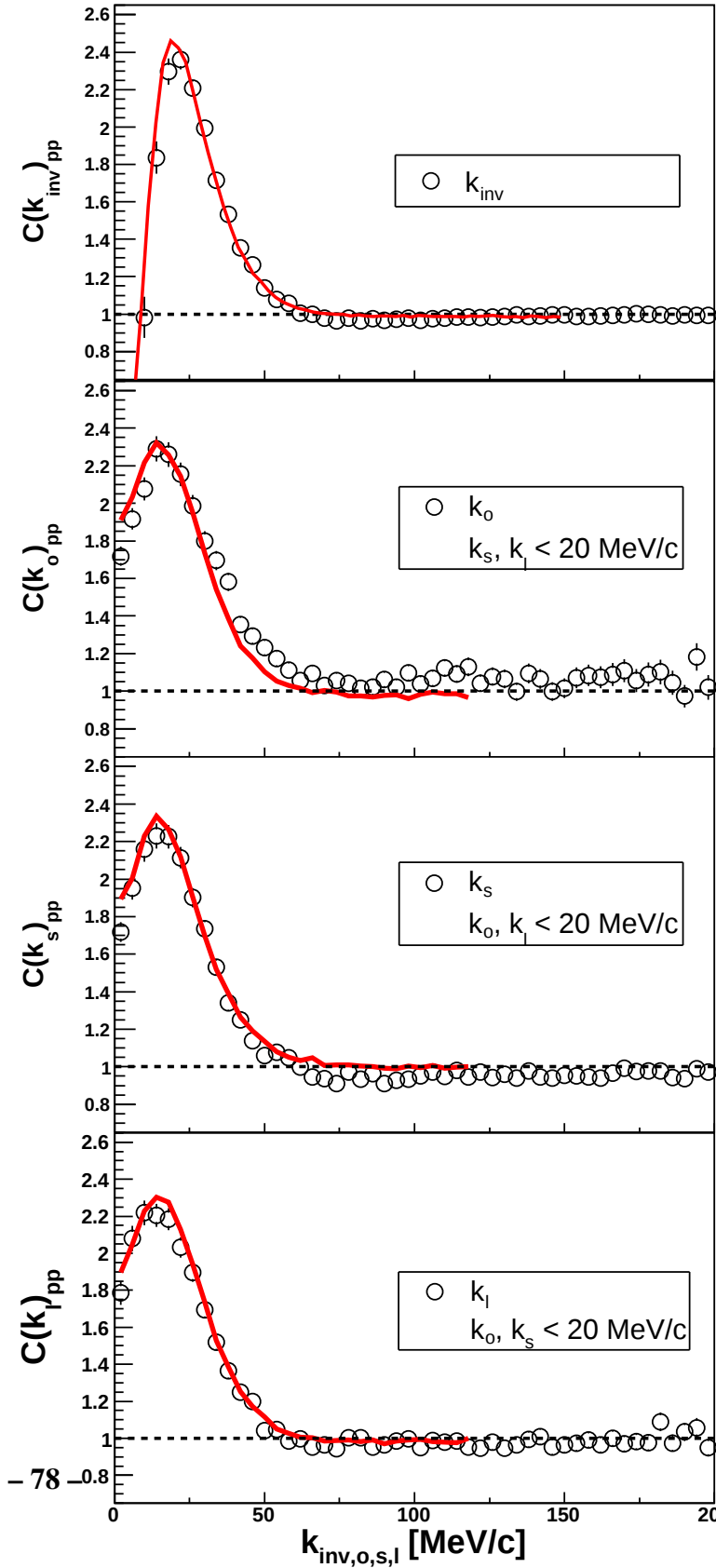
Figure 4.25: Comparison of fully corrected experimental p-p correlations (open circles) to predictions of CRAB (red lines) which use UrQMD as input. The plot at the top is the one-dimensional correlation function. The other three are projections of the 3D correlation function in the LCMS.
