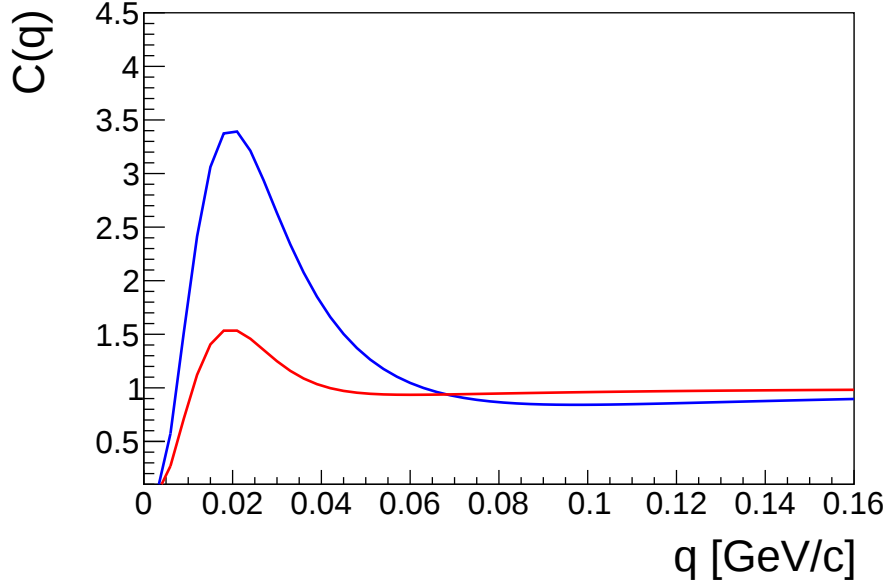
Figure 2.12: Two example plots of proton-proton correlation functions for source sizes of r_0 = 1.5 fm (blue) and r_0 = 3 fm (red). The proton-proton correlation function includes Fermi-Dirac statistics and Coulomb repulsion, which lead to a suppression of the correlation signal below unity for q \approx 0 as well as strong interaction which shows up as a bump structure at q \approx 20 MeV/c.
