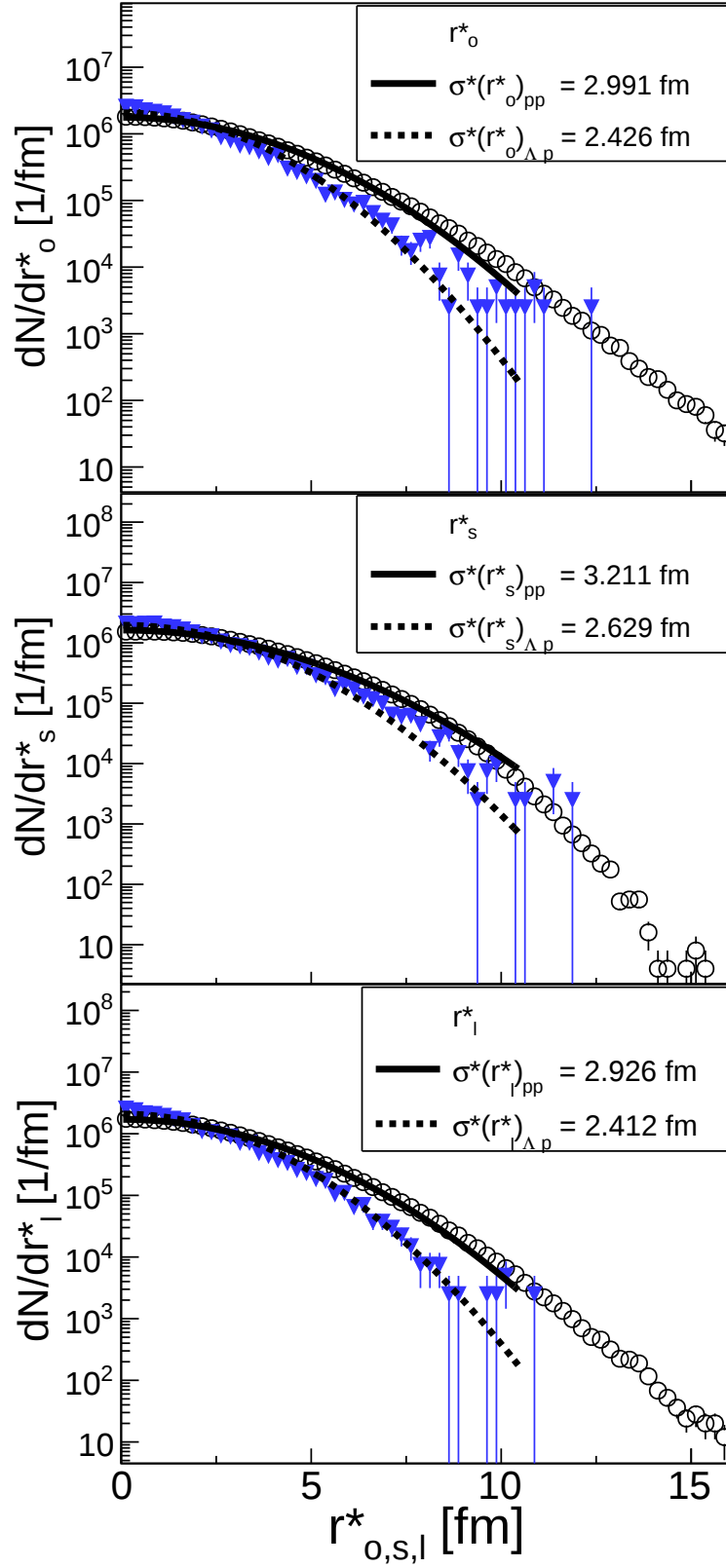
Figure 4.24: The projections in out-side-long direction in the PRF for p-p (open circles) and p-\Lambda (blue triangles) pairs from UrQMD. The p-\Lambda values are scaled to fit on the same plot. The width in every direction is obtained by fitting to it a Gaussian function (solid p-p , dashed p-\Lambda ).
