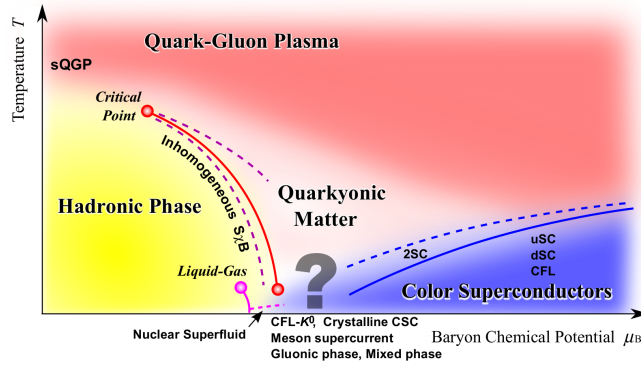
Figure 1.3: Phase diagram of QCD in terms of the temperature T and chemical potential \mu_B . Taken from [FH11].
