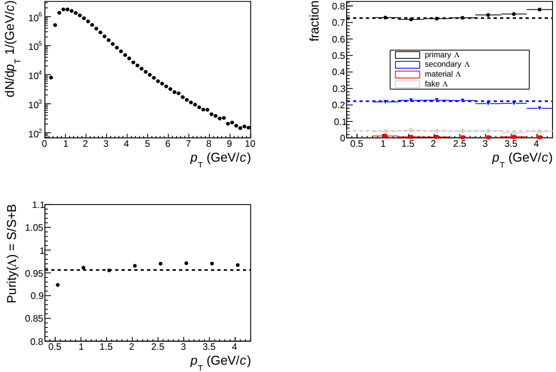
Figure 6.24: The fractions of \Lambda as a function of p_T obtained from a template fitting method. The purity is extracted by fitting the \Lambda invariant mass peaks. The averages of the quantities are evaluated by using the production probability dN/dp_T of \Lambda .
