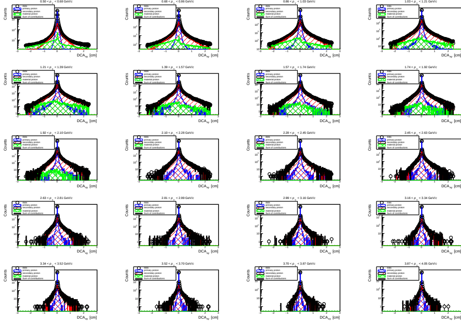
Figure 6.18: Adjusted Monte Carlo Templates from Pythia to the experimental data in the full p_T range.
