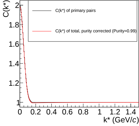
Figure 6.14: The black curve is the correlation function in which one is interested. For high purities (Purity=0.99) the residual correlations are small and one retrieves the correlation function of interest.
