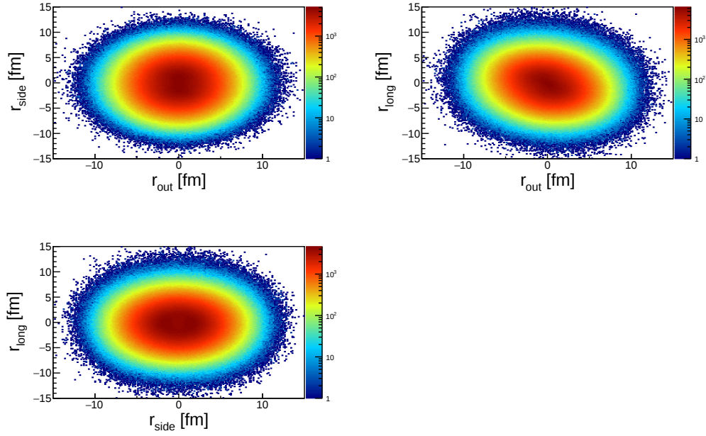
Figure 4.22: Freeze-out coordinates in the out-side-long basis for p-p pairs from UrQMD.
