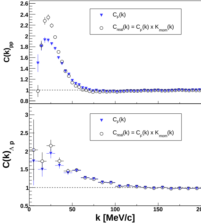
Figure 4.20: Effect of the correction for momentum resolution the measured experimental correlation functions of p - p (top) and p - \Lambda (bottom).
