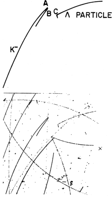
Figure 1.8: A film containing an elastic \Lambda p scattering event. Taken from [Sec+68].
