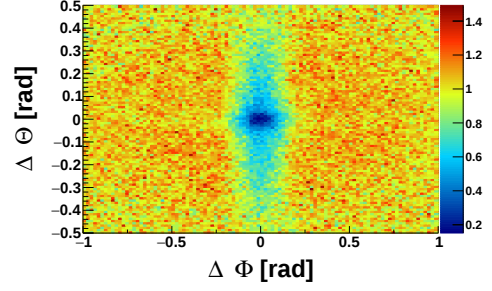
Figure 4.9: Experimental correlation function in (\Delta\phi, \Delta\Theta) for \pi^+ - \pi^+ pairs.
