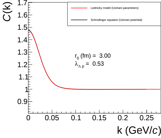
Figure 2.10: Comparison of the Lednicky model and the full solution of the Schrodinger Equation for a source radius of r_0 = 3 fm.
