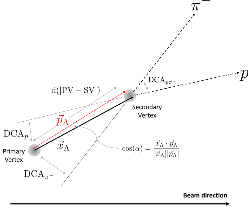
Figure 4.1: Sketch of a \Lambda decay and the explanation of topological selection criteria.
