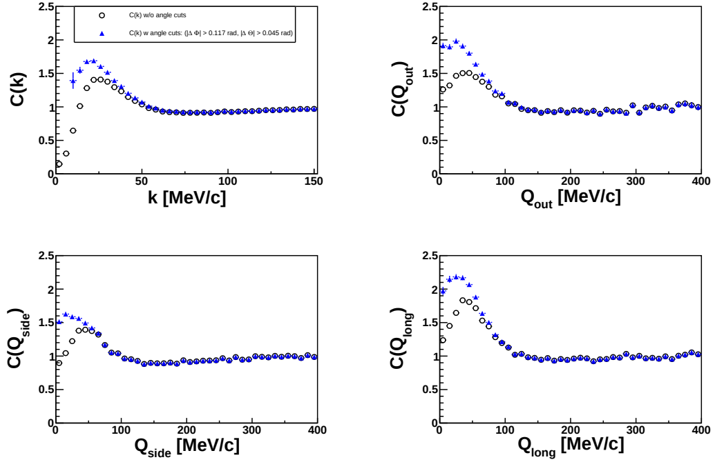
Figure 4.12: Comparison of the p-p correlation function in the k and q_{o,s,l} representation. The reduction of the merging effect is clearly visible.
