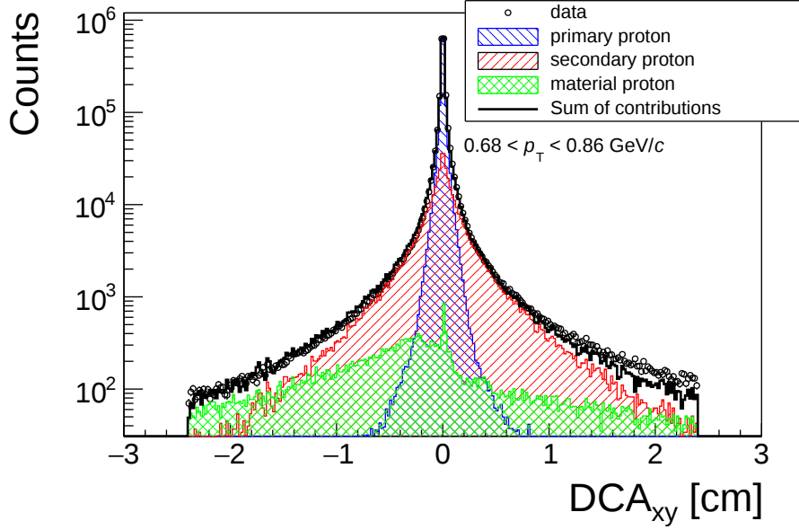
Figure 6.19: Adjusted Monte Carlo Templates from Pythia to the experimental data. Due to the shape of the templates one has a good discrimination of the origin of the protons.
