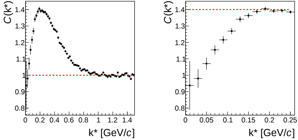
Figure 6.8: Left: Correlation function of the sum of \bar{p} - \Lambda and p - \bar{\Lambda} pairs. Also for this pair a strong contribution from mini-jets is visible, showing up as a broad correlation signal starting at k^* \sim 1 GeV/c. Right: Same correlation function zoomed to small relative momenta. One can see a correlation signal having femtoscopic signatures on top of the mini-jet background.
