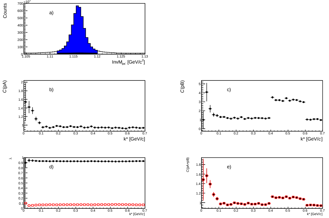
Figure 6.13: Decomposition of the individual correlation signals. The \Lambda signal is divided in signal (blue shaded) and background (black shaded) contributions. The signal correlation function is denoted as p - A and the background function as p - B . With the summation of the individual correlation functions weighted with the \lambda parameter one gets back the red squares of C(pA + pB) . The black dots of C(pA + pB) represent the total correlation function like it would be obtained in the experiment.
