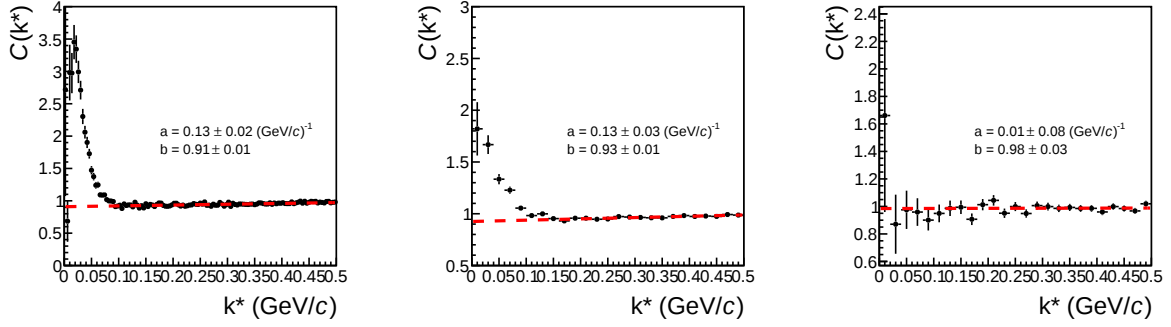
Figure 6.31: Baseline fit (red dashed line) obtained in a non-femtoscopic k^* region with Eq. (6.43).
