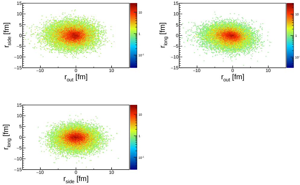
Figure 4.23: Freeze-out coordinates in the out-side-long basis for p-\Lambda pairs from UrQMD.
