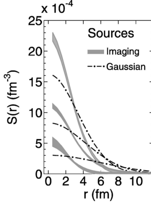
Figure 7.1: The Gaussian source which was fitted to the experimental data is compared to the source extracted from Imaging. Taken from [Ver+02].
