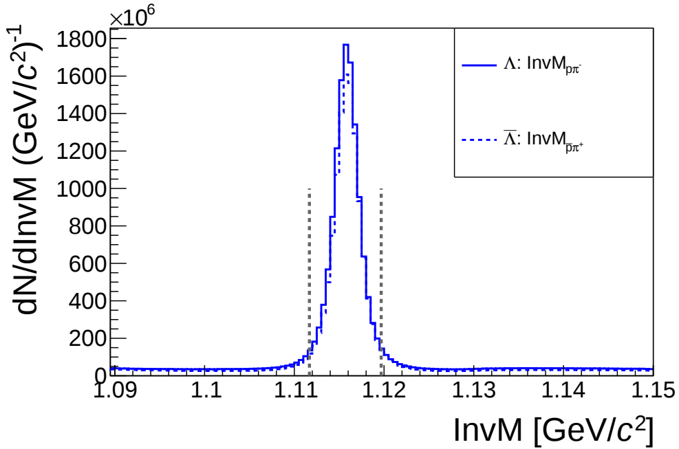
Figure 6.4: Invariant mass distribution of p\pi^- ( \bar{p}\pi^+ ) to obtain the \Lambda ( \bar{\Lambda} ) signal and the selection width used in the analysis.
