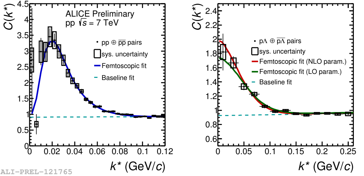
Figure 6.32: Simultaneous fit of the p - p and p - \Lambda pair, where the NLO expansion (red line) is used for the scattering parameter. After the fit is performed the LO parameter set (green line) is plugged in.
