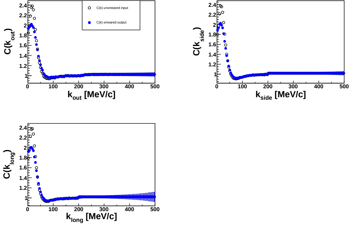
Figure 4.17: Effect of the momentum resolution for k_{o,s,l} projections.
