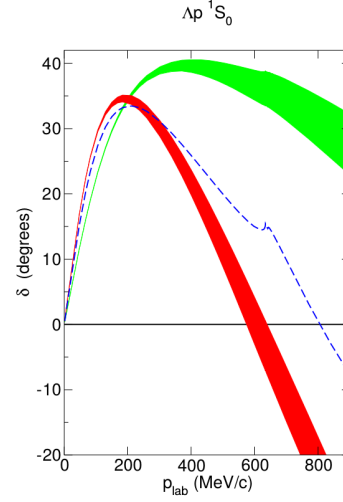
Figure 1.10: Phaseshift calculations from the effective field theory. No data points are available for elastic \Lambda p scattering. Taken from [Hai+13].
