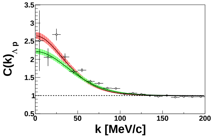
Figure 4.31: Influence of different sets of scattering parameter on the correlation function. The LO and NLO scattering length at a cutoff value of 600 MeV are taken from [Hai+13]. This figure includes the fully correct Lednicky model. See text for details.
