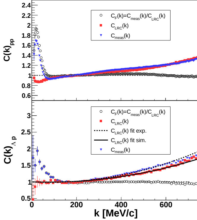
Figure 4.14: Effects of LRC on the correlation function. Top: p-p pairs where UrQMD is used to describe the baseline. Bottom: p-\Lambda pairs where Eq. 4.3 is used to describe LRC. The experimental (dashed) as well as the simulation (solid) correlation function is fitted in k \in [250, 600] MeV/ c to check for any differences at low k .
