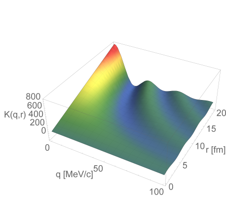
Figure 2.7: Kernel of the strong interaction.
