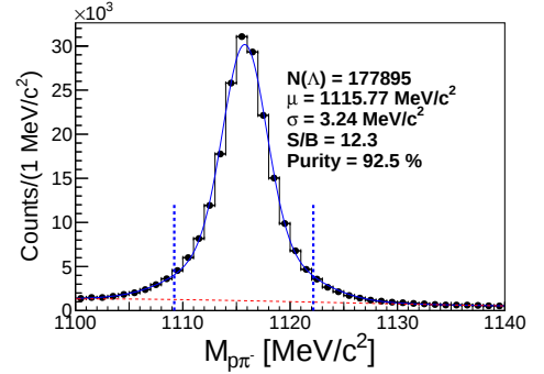
Figure 4.5: p-\pi^- invariant mass spectrum for combination 3 of topological cuts.
