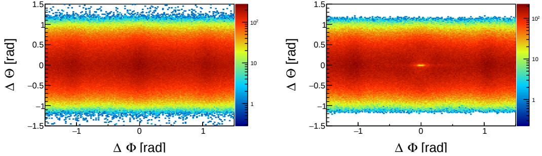
Figure 4.6: Angle correlations of (\Delta\phi, \Delta\Theta) for p - p pairs. The left plot shows p - p pairs after GEANT which filters the pairs for acceptance. The right plot includes also the tracking which introduces a hole in the distribution.
