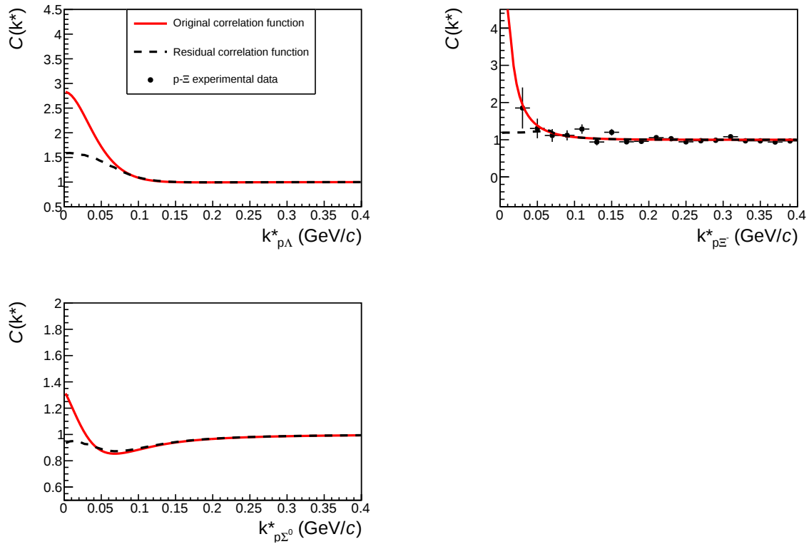
Figure 6.26: Initial correlation functions displayed as red solid lines. The black dashed lines are the residual correlations. Top left: p\Lambda \rightarrow p-p , Top right: p\Xi^- \rightarrow p\Lambda . Bottom left: p\Sigma^0 \rightarrow p\Lambda .
