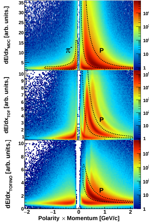
Figure 3.5: Specific energy loss distributions for MDC, TOF and TOFINO as a function of the particles momentum. One can clearly see the different bands corresponding to different particle species.
