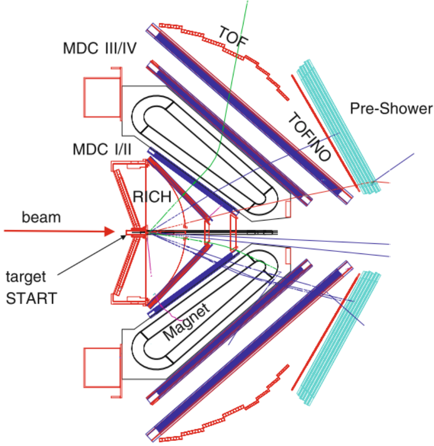
Figure 3.2: Side view of the HADES detector system and its detector components.
