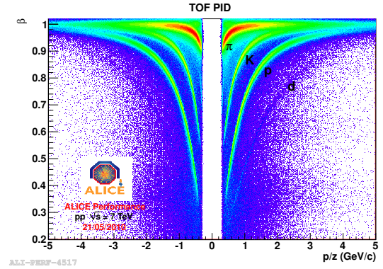
Figure 5.5: The velocity of particles versus their momenta. Different bands develop for the different particle species.
