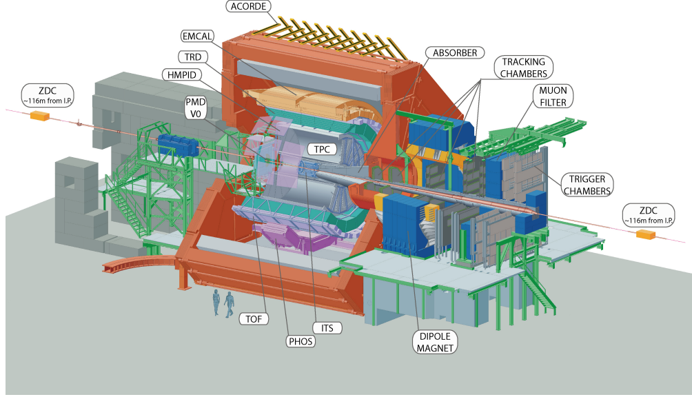
Figure 5.1: The ALICE detector with its individual components [Aam+08].
