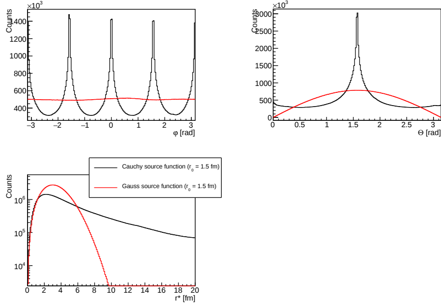
Figure 2.1: Projections of the source functions on r^* , \Theta and \varphi . The red distribution corresponds to a Gaussian and the black to a Cauchy source choice. See text for more details.
