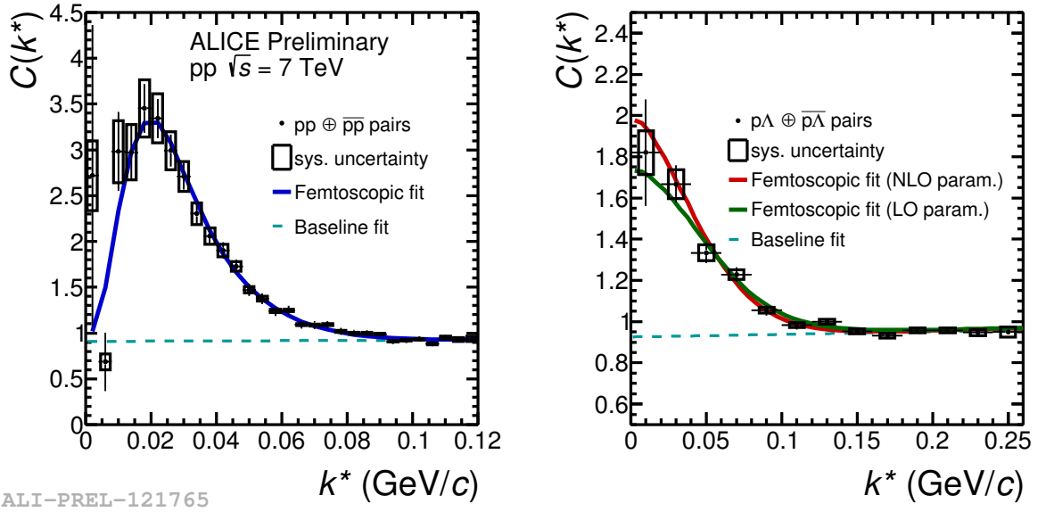
Figure 6.32: Simultaneous fit of the p - p and p - \Lambda pair, where the NLO expansion (red line) is used for the scattering parameter. After the fit is performed the LO parameter set (green line) is plugged in.
