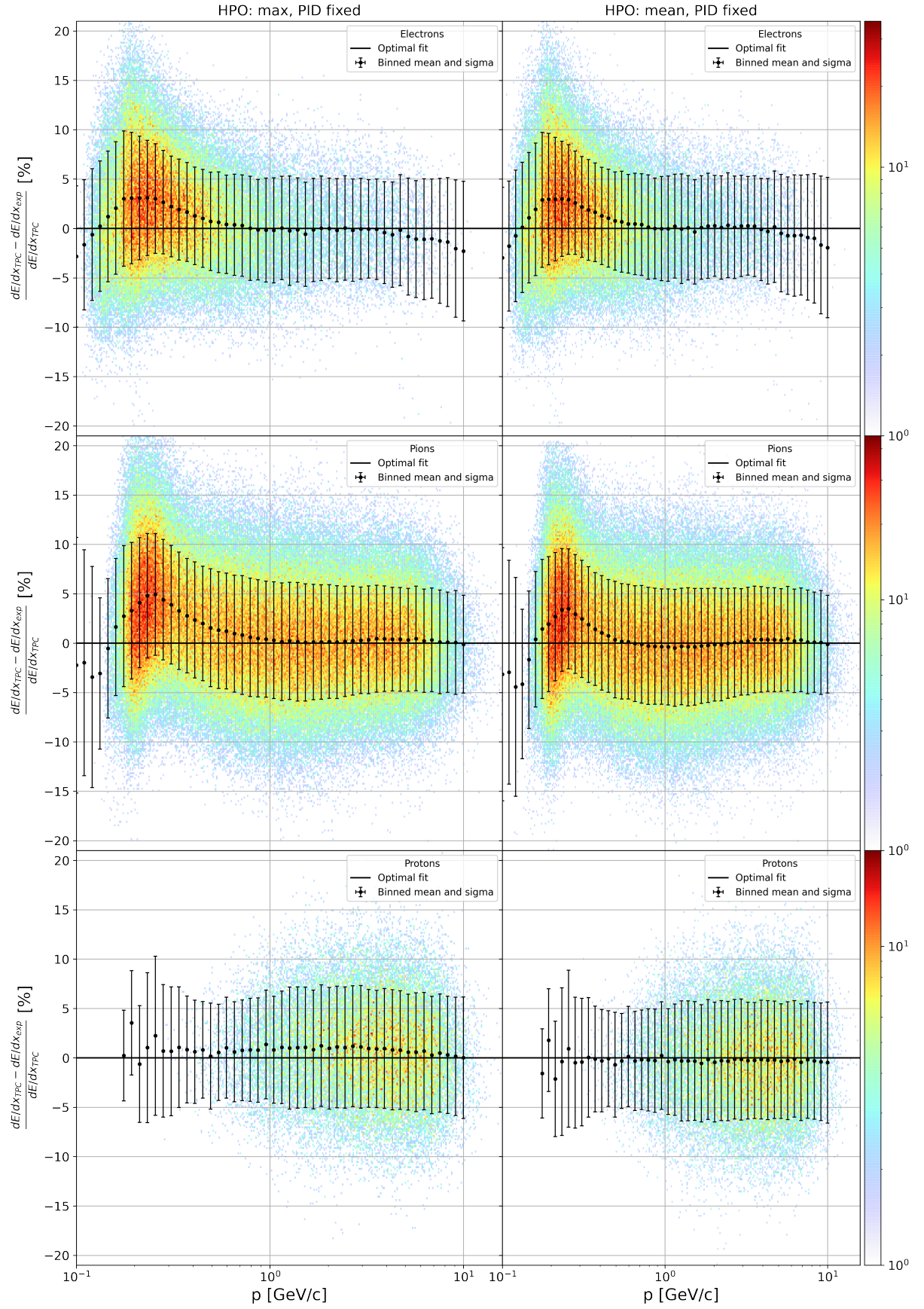
Figure 5.7: Comparison of the HPO performance for fixed particle identities with the Run 2 parameterization for identified electrons, pions and protons.
