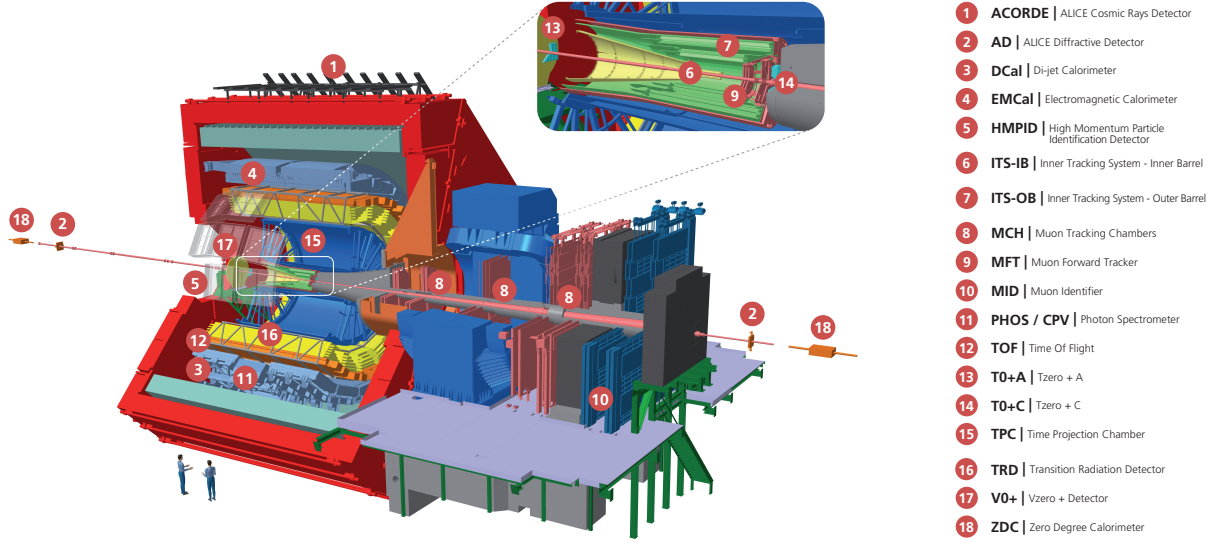
Figure 2.1: Schematic representation of the detector systems for Run 3 of the ALICE experiment, located at IP2 at the LHC.
