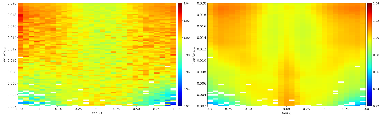
Figure 5.12: Mean corrections for protons in the (\tan(\lambda), 1/(dE/dx_{\text{exp}})) space for the neural network (left) and the spline fit (right).
