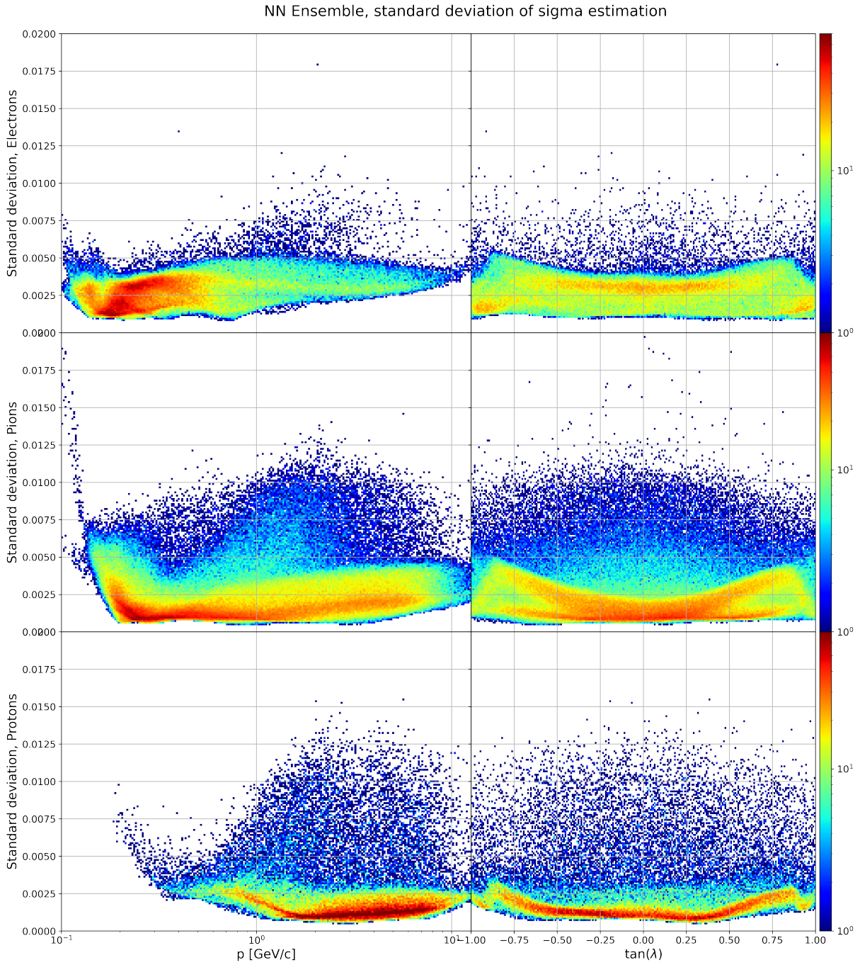
Figure 5.19: Deviation of the sigma estimation produced by a neural network ensemble for momentum and \tan(\lambda) .
