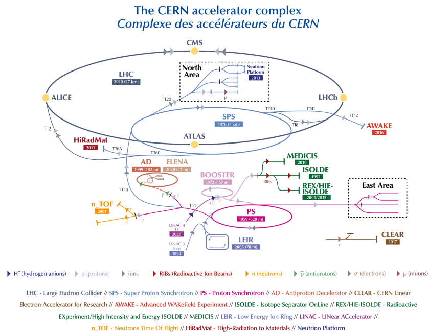
Figure 1.1: Schematic representation of the CERN accelerator complex with the four major experiments ALICE, ATLAS, CMS and LHCb.
