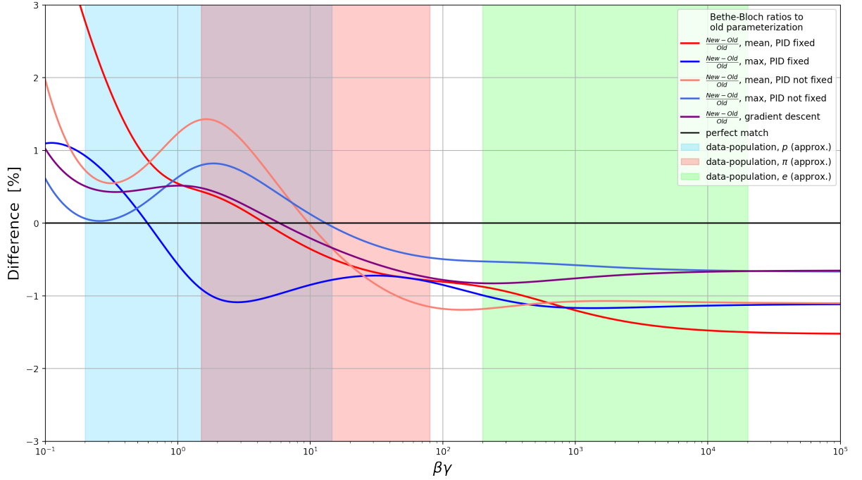
Figure 5.9: Gradient descent method together with the HPO results as a ratio to the Run 2 parametrization.
