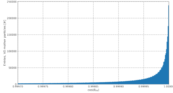
Figure 5.2: Distribution of the \cos(\theta_{PA}) combined for all decays.
