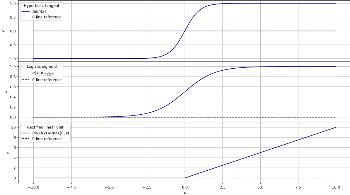
Figure 3.1: Common 1D Activation functions of neurons in a neural network.
