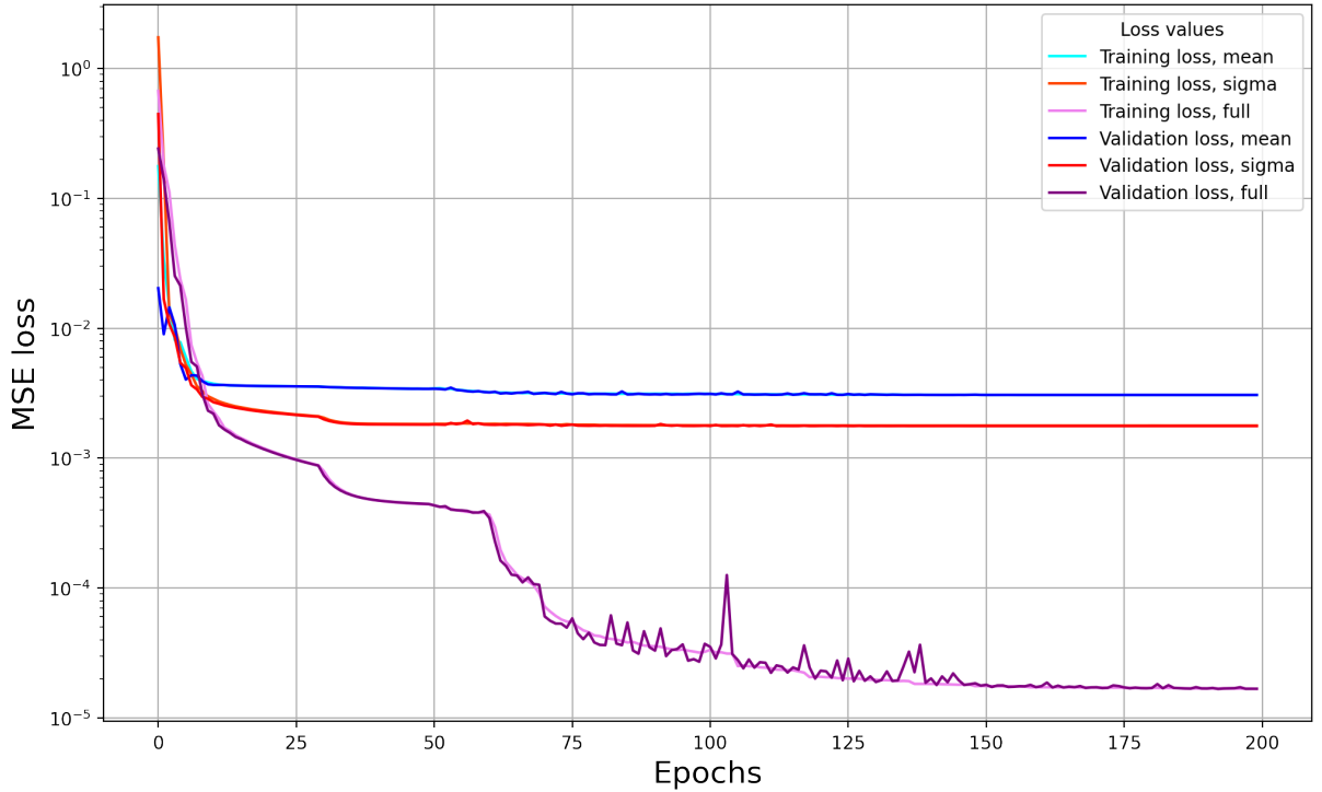
Figure 5.20: Loss scores of the networks trained for the mean and sigma estimation, as well as the full network for the application in O^2 .
