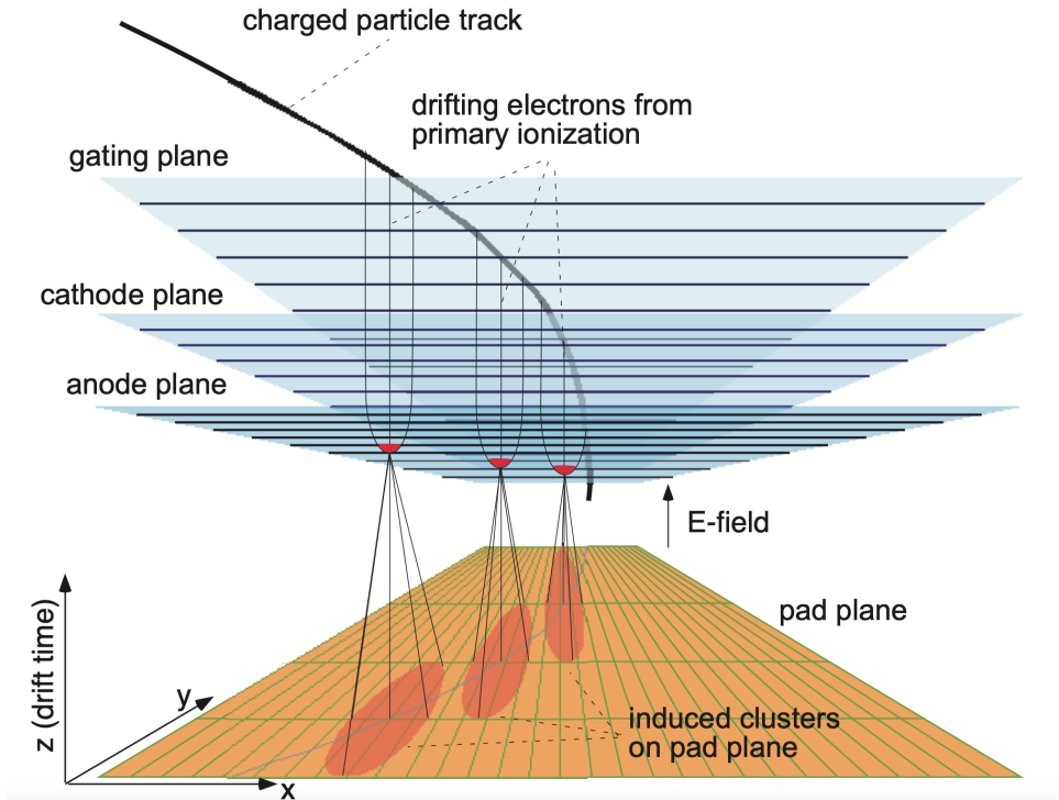
Figure 2.3: MWPC as it was used in the ALICE TPC for Run 2 [4].
