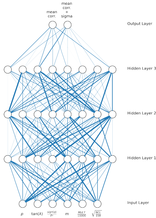
Figure 5.16: Neural network (final architecture) with the connecting weights represented by the line-thickness between adjacent layers.
