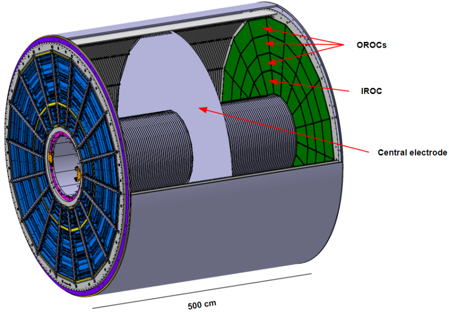
Figure 2.2: 3D representation of the ALICE TPC for Run 3 [2] with annotations.
