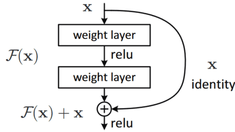
Figure 3.4: A skip connection as implemented in a residual neural network. 2
