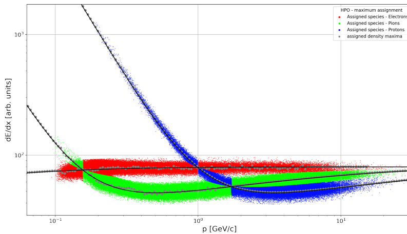
Figure 5.5: Locally assigned particle species and density maxima based on binning in \beta\gamma and dE/dx .
