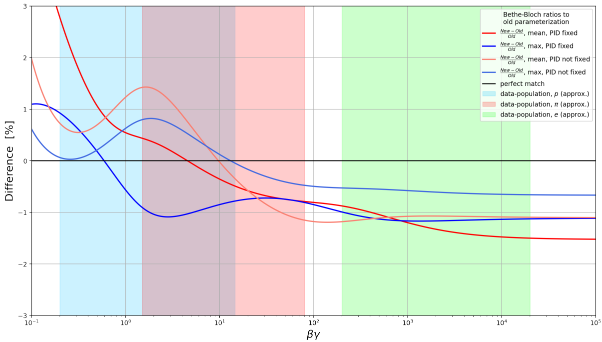
Figure 5.8: Difference in [%] between the Bethe-Bloch parametrization obtained in Run 2 and the parametrizations obtained from the HPO algorithm with different settings.
