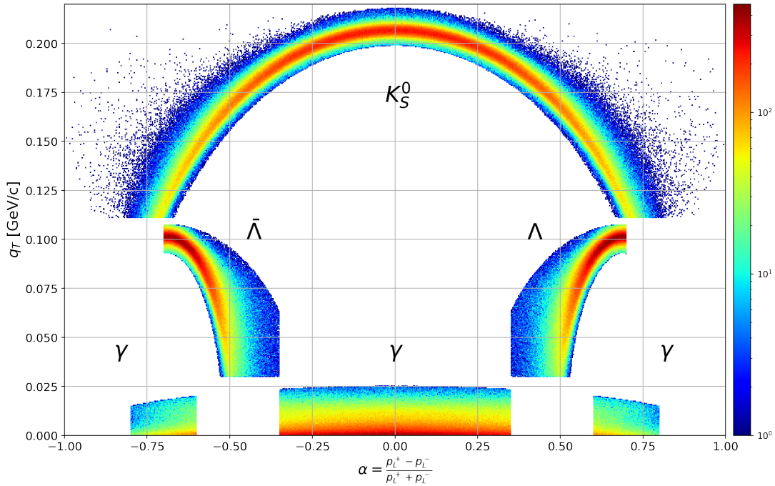
Figure 5.3: Pure V0 selection based on the Armenteros-Podolanski selections for the LHC18b converted dataset together with applied selection criteria on the invariant mass and \cos(\theta_{PA}) (this work).
