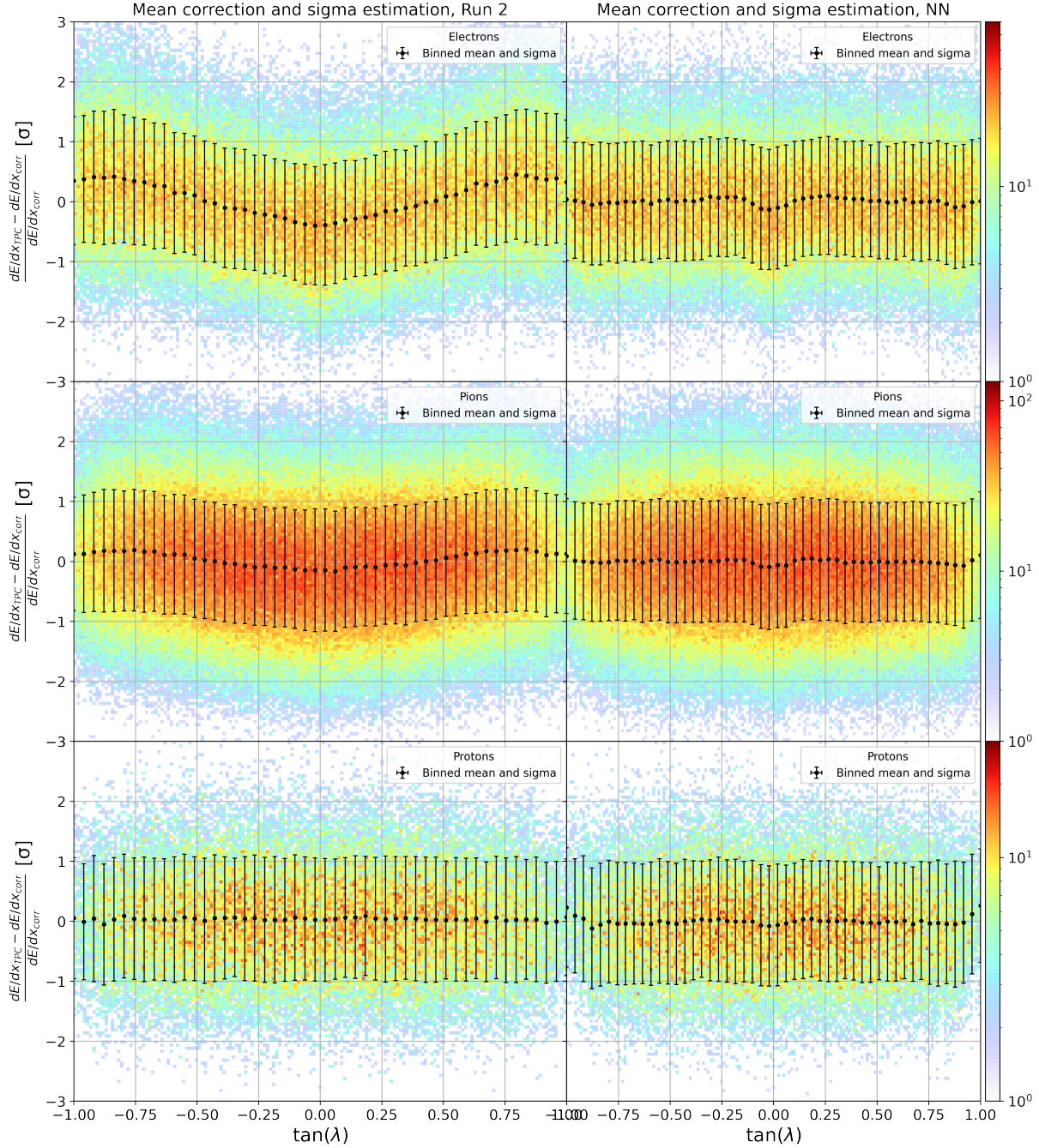
Figure 5.18: N\sigma distributions for identified electrons, pions and protons with the method from Run 2 and the neural network application.
