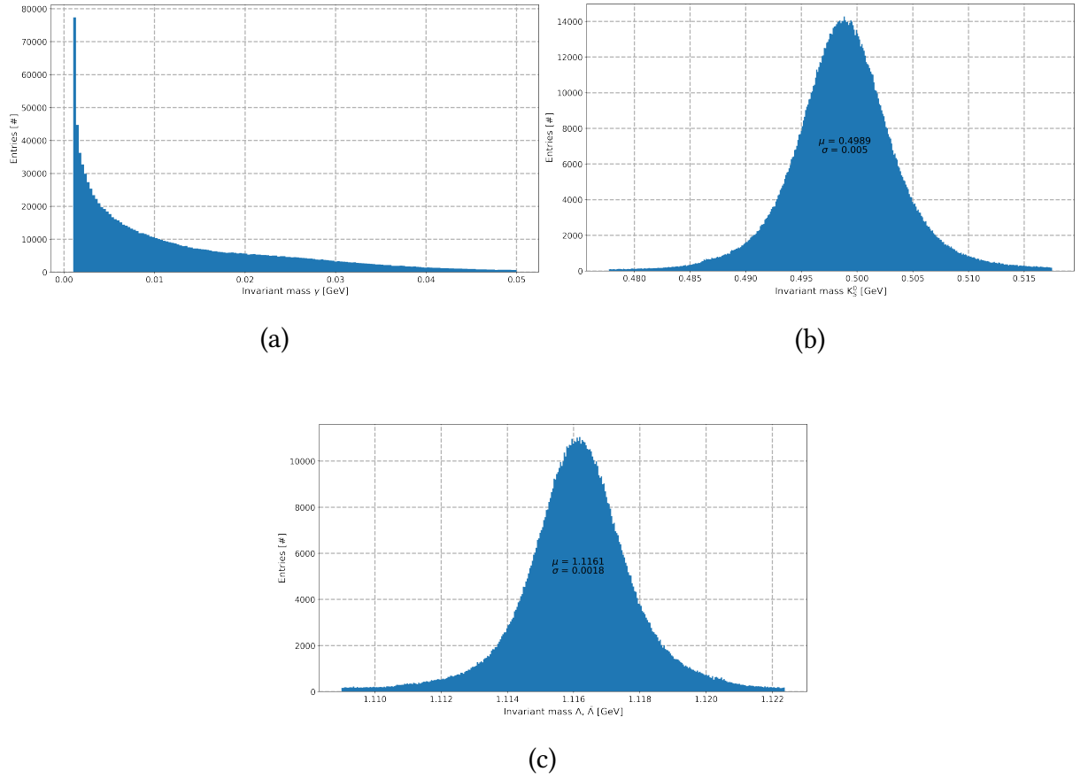
Figure 5.1: Reconstructed invariant mass distributions for \gamma (top left), K_S^0 (top right) and \Lambda / \bar{\Lambda} (bottom center).
