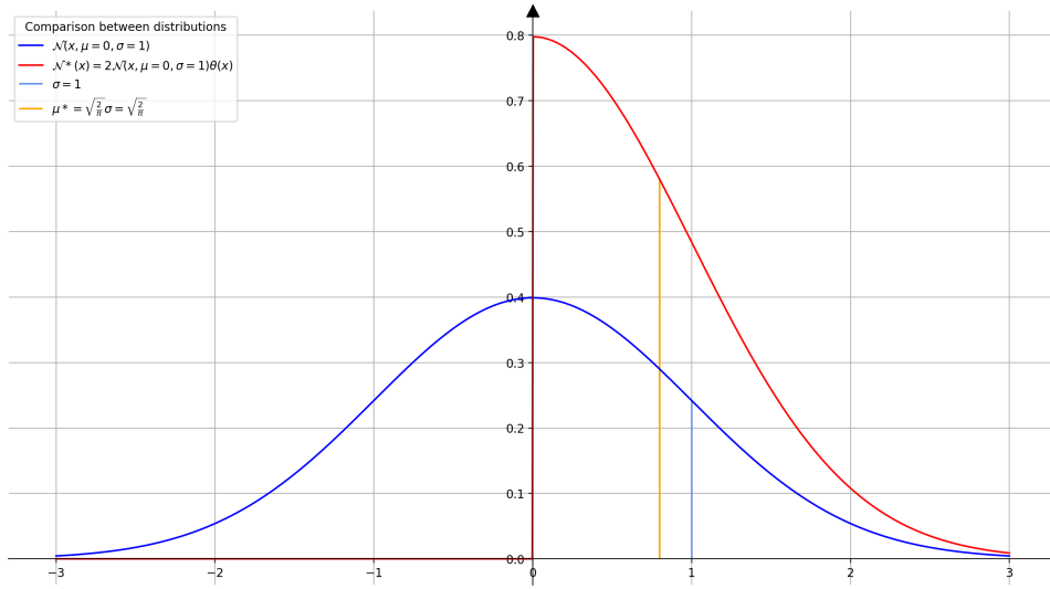
Figure 5.15: Comparison between original Gaussian distribution and the \mathcal{N}^* distribution.
