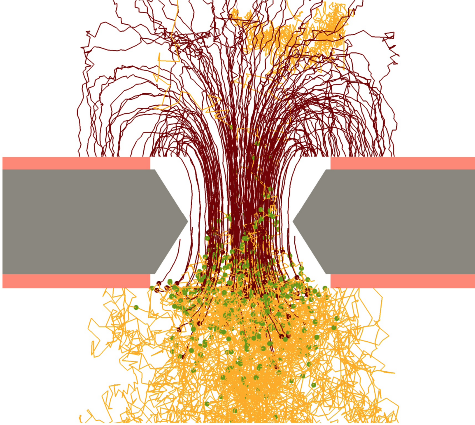
Figure 2.4: Cross-sectional view: Garfield simulation for an electron passing a GEM hole [3].
