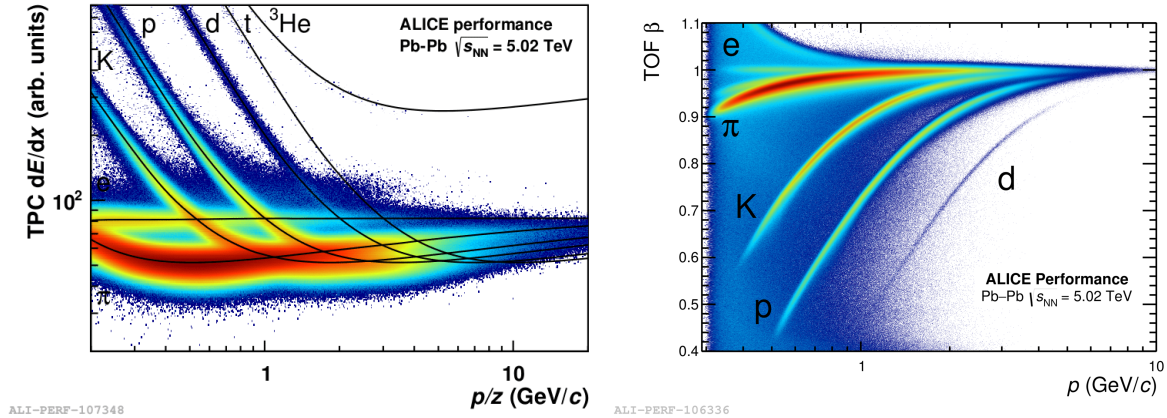
Figure 4.6: Separation power of the TPC (left) and TOF (right) detector
