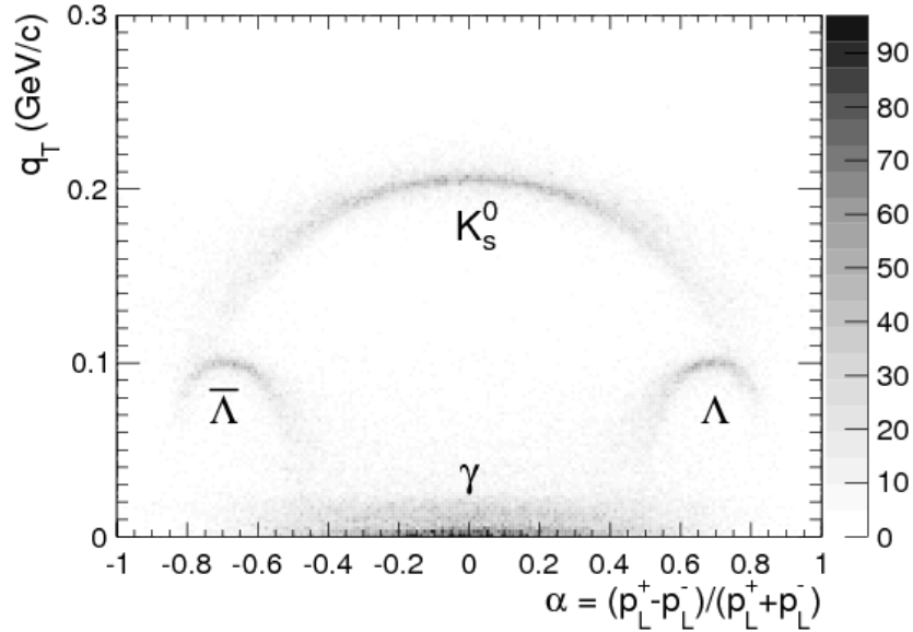
Figure 4.4: Plot of the Armenteros-Podolanski variables with reconstructed mother particles [13].
