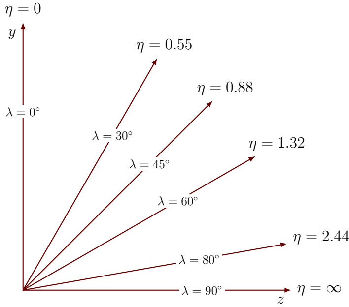
Figure 4.2: Pseudo-rapidity and \tan(\lambda) for different values of \lambda .
