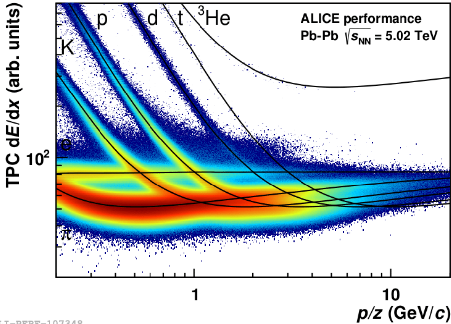
Figure 4.1: \langle dE/dx \rangle performance plot of the ALICE TPC at \sqrt{s_{NN}} = 5.02 TeV [10]. Several particle species are visible together with their parameterized Bethe-Bloch curve.
