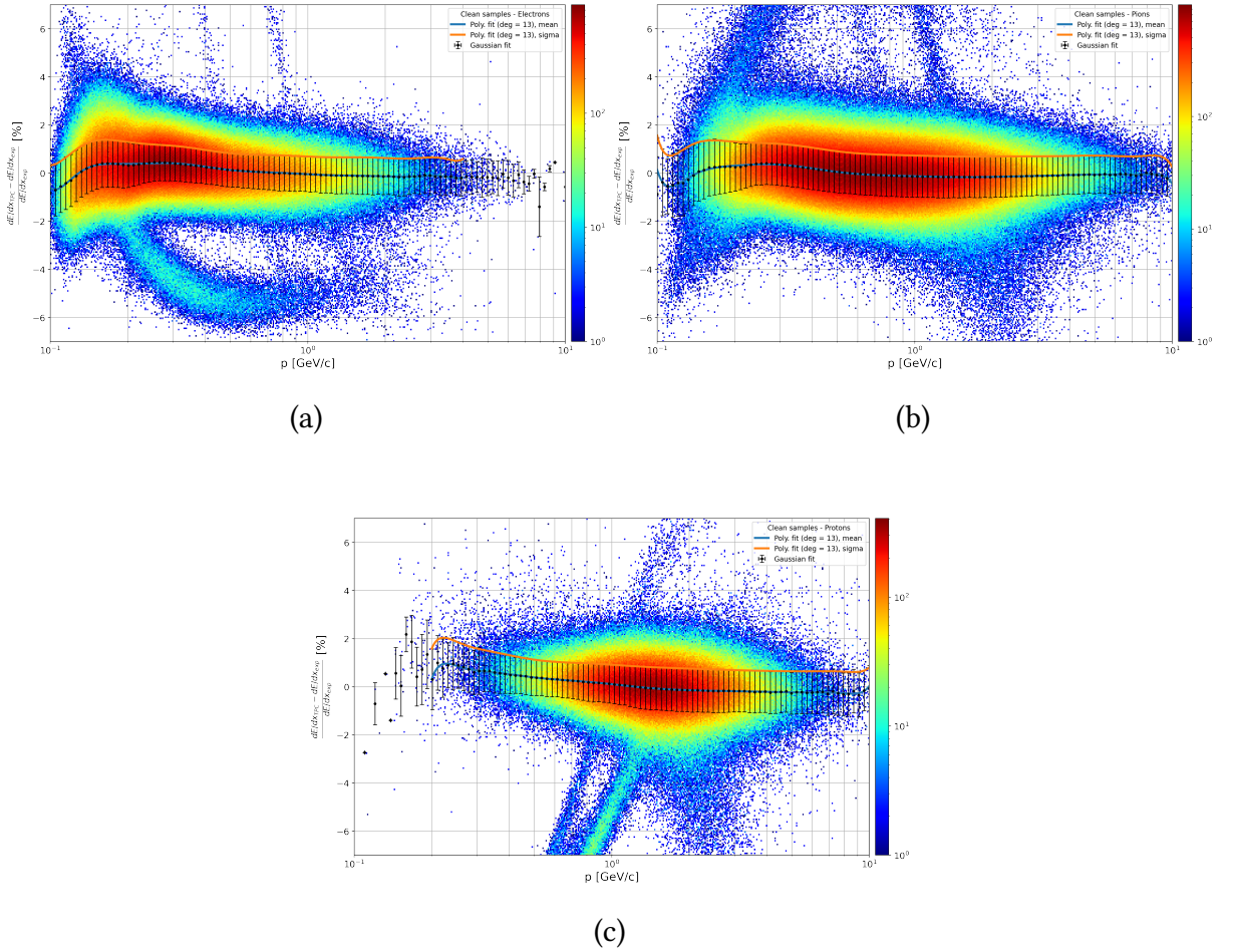
Figure 5.4: Distributions of the TPC dE/dx as a ratio of the Bethe-Bloch function against the measured momentum for electrons (a), pions (b) and protons (c) together with Gaussian fits and polynomials for assessing the purity.
