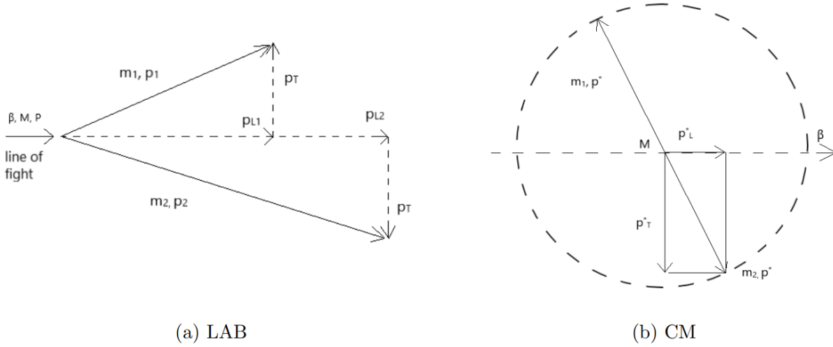
Figure 4.3: Representation of the Armenteros-Podolanski variables \alpha and q_T in the laboratory ((a) LAB) and the center-of-mass ((b) CM) frame [12].
