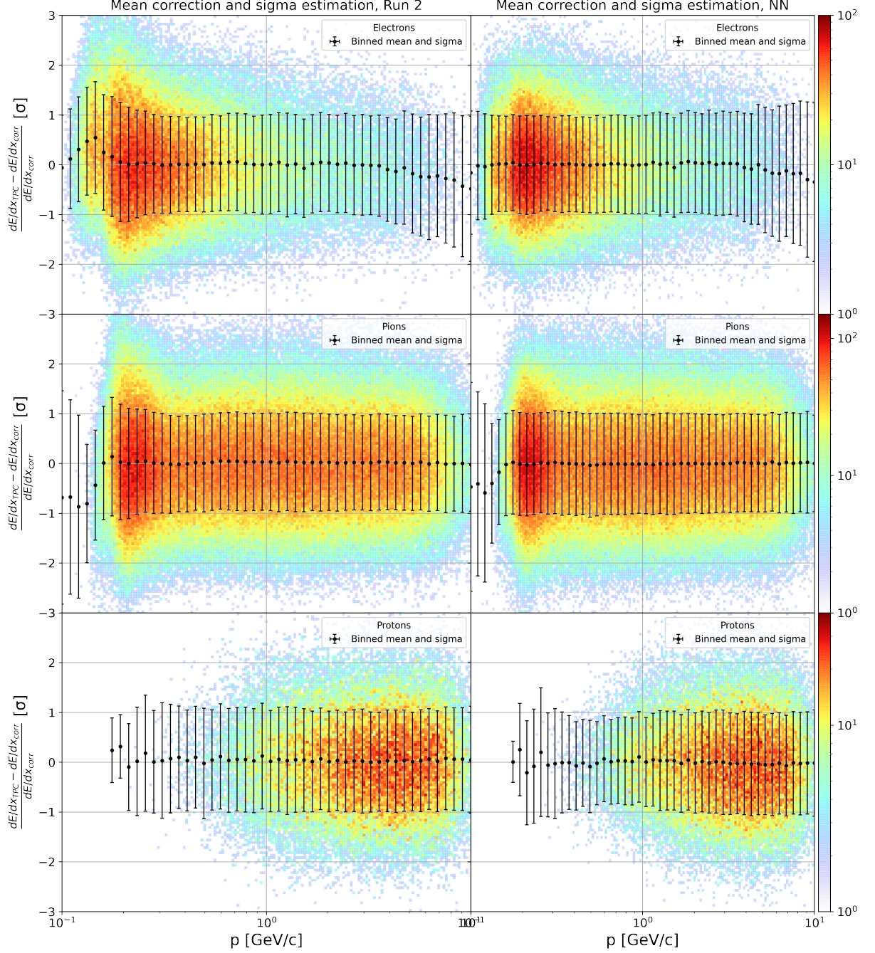
Figure 5.17: N\sigma distributions for identified electrons, pions and protons with the method from Run 2 and the neural network application.
