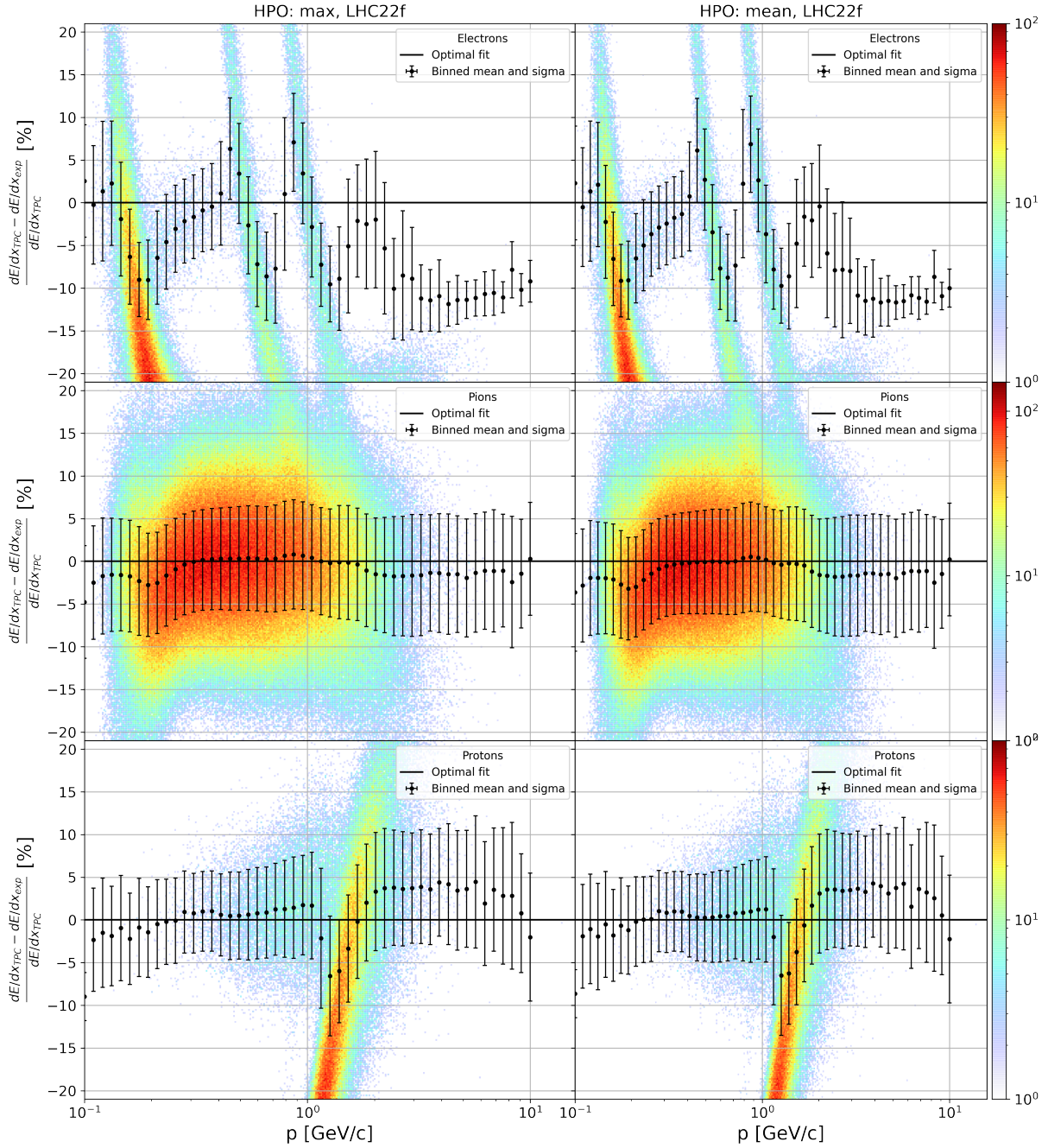
Figure 5.10: Performance of the mean and maximum density estimation on uncleaned data of the LHC22f dataset.
