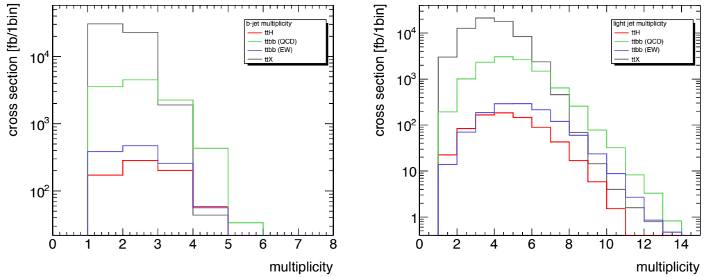
Figure 5.8: Jet multiplicities for b -tagged jets (left) and light jets with p_T > 20 GeV, reconstructed with the Anti- k_T algorithm. Distributions are normalised to 30 \text{ fb}^{-1} .
