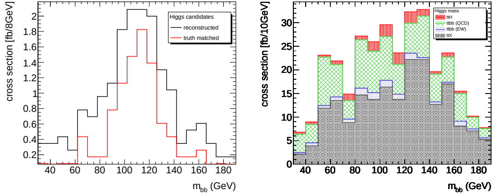
Figure 8.2: Invariant mass distribution of all Higgs candidates for the fat jets analysis. Left: All Higgs candidates and their truth matches found for signal events. Right: Higgs candidates of signal and all backgrounds normalised to 100 \text{ fb}^{-1} .
