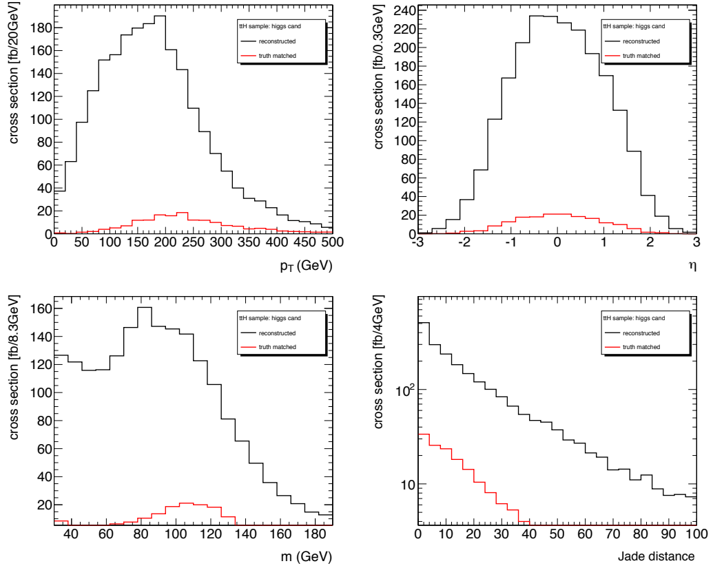
Figure 7.11: Transverse momentum p_T , pseudorapidity \eta , invariant mass m and Jade distance for the up to three in Jade distance leading Higgs candidates for the signal sample. At this point, b -tagging has not been applied. The distributions for all reconstructed and truth matched are normalised to 100 \text{ fb}^{-1} .
