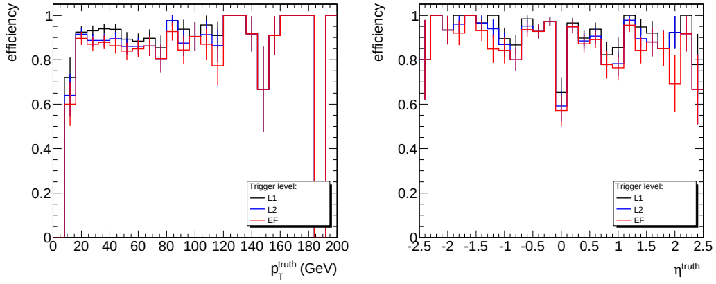
Figure 5.10: Trigger efficiency for each trigger level for the mu10 signature shown for the truth p_T and \eta of the lepton from the top decay.
