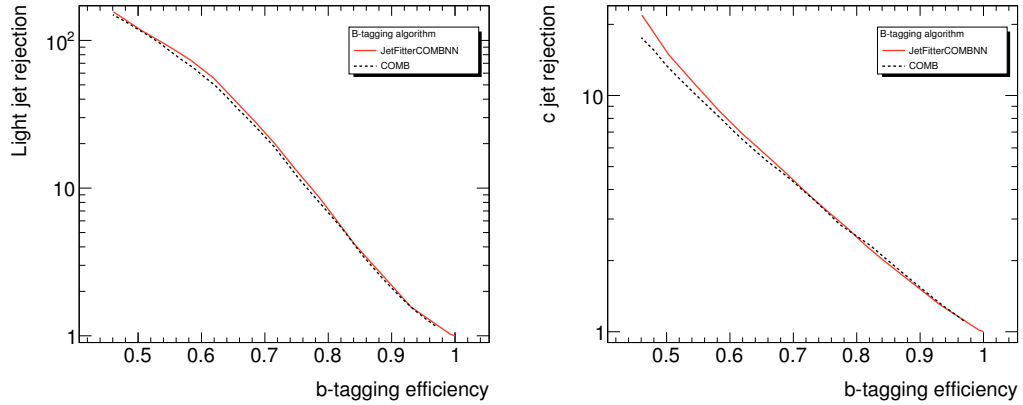
Figure 5.6: Left: Light jet rejection versus b -tagging efficiency of the b -tagging algorithms JetFitterCOMBNN and COMB. Right: c -jet rejection versus b -tagging efficiency of the b -tagging algorithms COMB and JetFitterCOMBNN.
