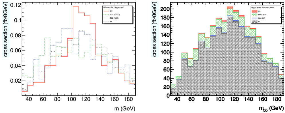
Figure 7.17: Higgs mass distribution of all Higgs candidates found for signal and all background events, normalised to unit area (left) and added up corresponding to their cross-sections, normalised to 100 \text{ fb}^{-1} .
