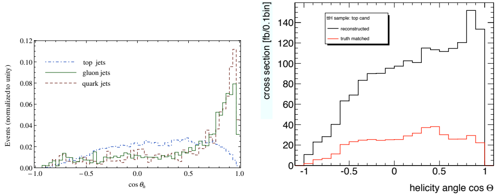
Figure 7.6: Left: Helicity angle distribution for top jets, gluon jets and light-quark jets for p_T > 700 \text{ GeV} , taken from Ref. [54]. The distributions are normalised to unit area. Right: Helicity distribution for the signal sample of all reconstructed top candidates and for all candidates which have been matched to a truth candidate after the top mass window cut has been applied. Distributions are normalised to 100 \text{ fb}^{-1} .
