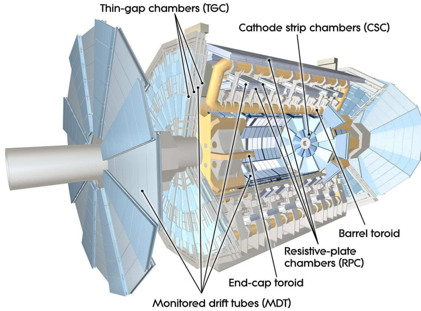
Figure 2.5: Cut-away view of the ATLAS muon system.
