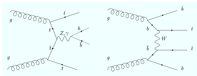
Figure 3.11: Example Feynman diagram of the electroweak t\bar{t}b\bar{b} production.
