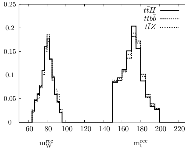
Figure 7.3: Individually normalised m_W^{\text{rec}} and m_t^{\text{rec}} distributions for signal and background (with underlying event). Taken from [3].
