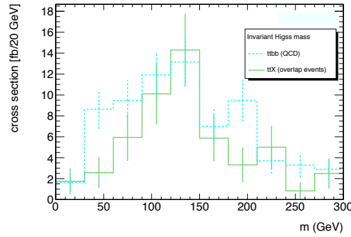
Figure 6.6: Comparison of the invariant Higgs mass distribution of the overlapping events from tt+X sample and the events from the t\bar{t}b\bar{b} sample.
