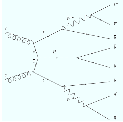
Figure 3.9: Example Feynman diagram of the semileptonic signal process t\bar{t}H^0(H^0 \rightarrow b\bar{b}) .
