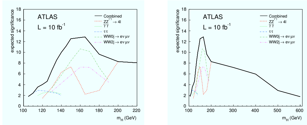
Figure 3.7: ATLAS discovery potential of a SM Higgs boson as a function of the Higgs boson mass, corresponding to an integrated luminosity of 10 \text{ fb}^{-1} , for the low mass range (left) and up to 600 GeV (right). Taken from Ref [5].
