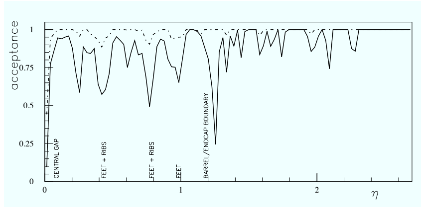
Figure 4.3: Acceptance for the requirements of one superpoint (dash-dotted line) and three superpoints (solid line) in the three stations of the precision chamber system as a function of pseudorapidity and averaged over azimuthal angle. A superpoint is a coincidence of at least six hits in six different sensitive planes in one chamber. Taken from [14].
