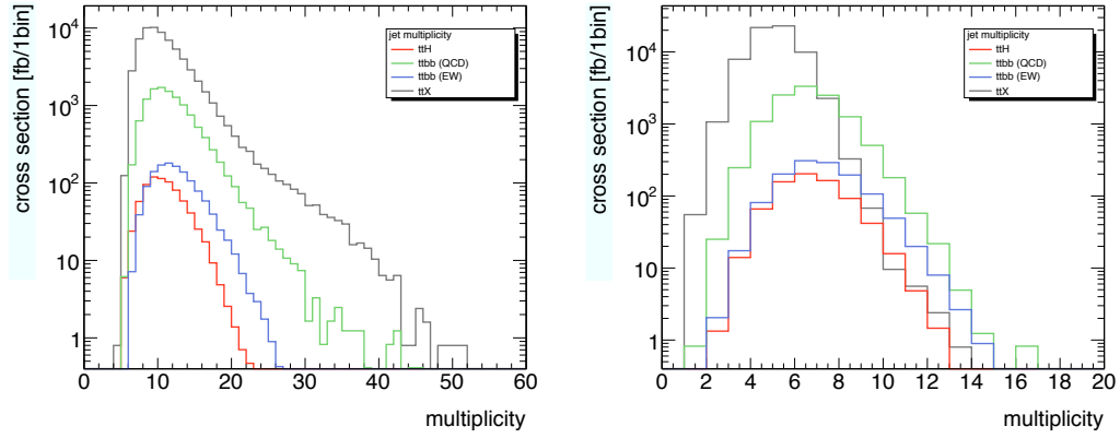
Figure 5.7: Jet multiplicities for all jets (left) and for jets with p_T > 20 GeV, reconstructed with the Anti- k_T algorithm. Both distributions are normalised to 30 fb -1 .
