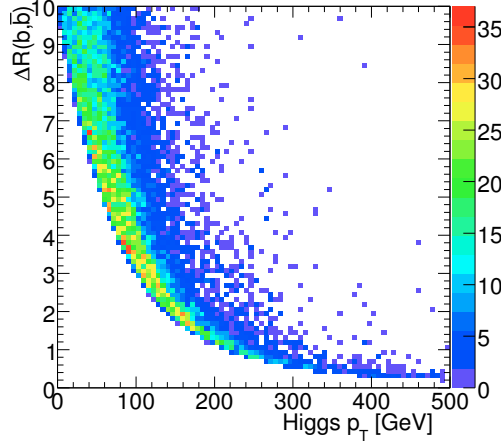
Figure 7.1: Distance in \Delta R = \sqrt{\Delta\phi^2 + \Delta\eta^2} between the two b -quarks from the Higgs boson with a Higgs boson mass of m_H = 120 GeV as a function of the Higgs boson transverse momentum. \Delta\phi represents the distance in azimuthal angle, while \Delta\eta is the distance in pseudo-rapidity. The normalisation is arbitrary. Taken from [82].
