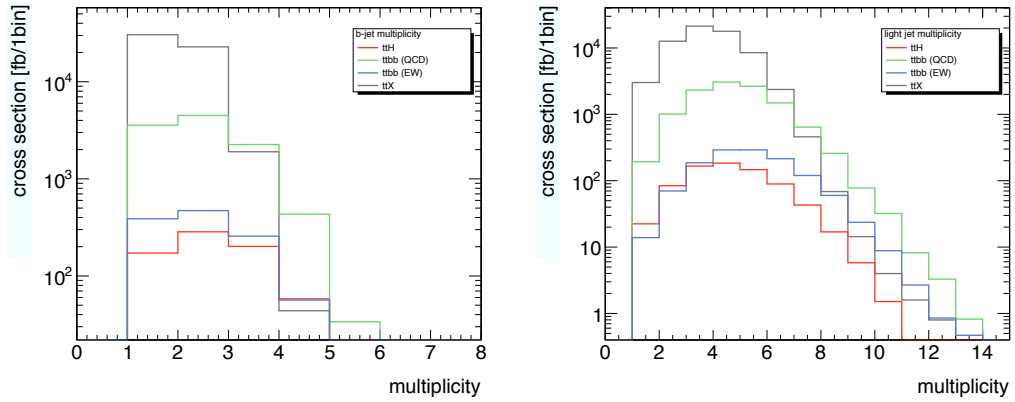
Figure 5.8: Jet multiplicities for b -tagged jets (left) and light jets with p_T > 20 GeV, reconstructed with the Anti- k_T algorithm. Distributions are normalised to 30 fb -1 .
