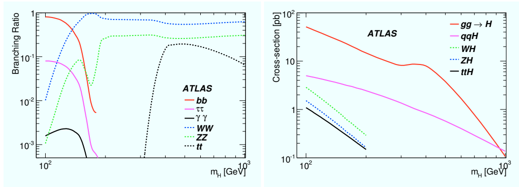
Figure 3.6: Left: Branching ratio of the Higgs boson decaying in the different possible final states as a function of the Higgs boson mass m_H . Right: Cross-sections for the main Higgs boson production modes at the LHC computed at NLO as a function of the Higgs boson mass. Taken from Ref. [5].
