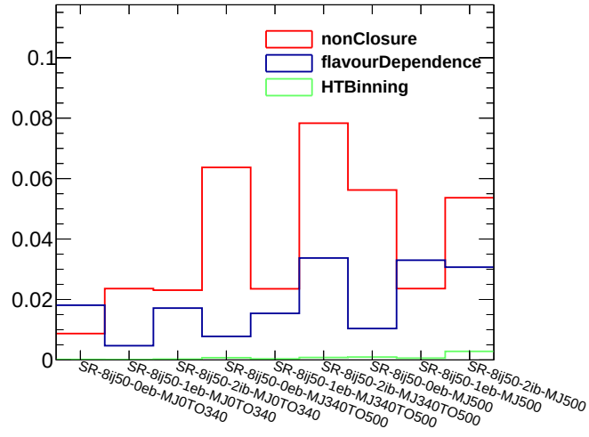
(a) N_{\text{jets}}^{50} \geq 8
