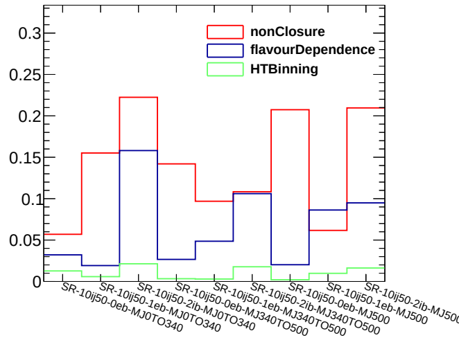
(c) N_{\text{jets}}^{50} \geq 10
