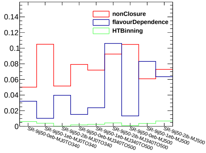
(b) N_{\text{jets}}^{50} \geq 9
