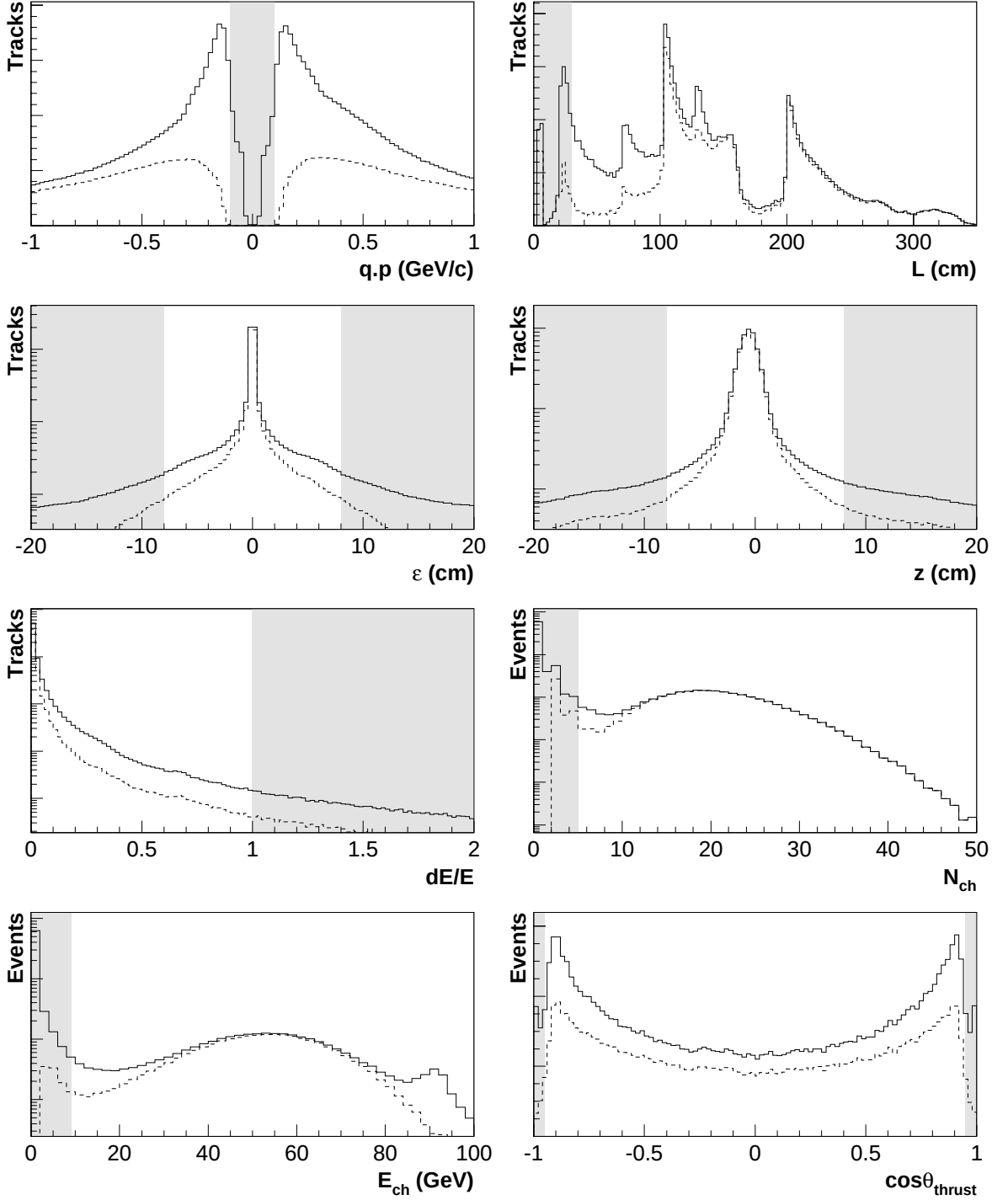
Figure 4.1: Distribution of parameters used in the hadronic event selection. The shaded regions show the cuts detailed in section 4.2.1.
