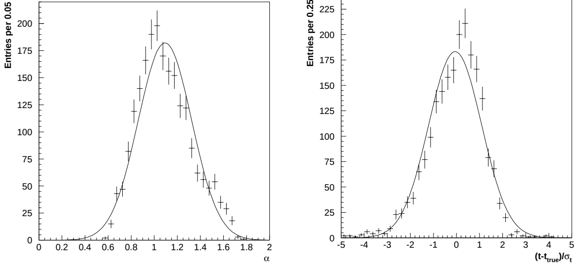
Figure 4.11: Monte Carlo correction for B decay time uncertainty. The first histogram shows \alpha (equation 4.12) plotted for true B \rightarrow J/\psi candidates that pass all cuts (including 2.95 \leq M_{\mu^+\mu^-} < 3.25 \text{ GeV}/c^2 ). It has a central value of \alpha = 1.094 \pm 0.005 and width \sigma_\alpha = 0.232 \pm 0.004 . The second histogram second shows the B decay time pull ((t - t_{\text{true}})/\sigma_t) distribution when these values are used in equation 4.13. It has a central value of -0.058 \pm 0.025 and width 1.150 \pm 0.018 . The curves show the Gaussian fits to the distributions which were used to determine the central values and widths.
