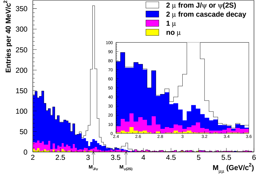
Figure 4.12: Opposite-sign sample composition in simulated data. The components, from top to bottom, are (a) J/\psi \rightarrow \mu^+\mu^- or \psi(2S) \rightarrow \mu^+\mu^- ; (b) two muons from cascade decay: b \rightarrow c\mu^-\bar{\nu}_\mu , c \rightarrow s/d\mu^+\nu_\mu (or charge conjugate); (c) one (or occasionally two) muons, not from any of the above sources: mostly semileptonic B decays with a hadron misidentified as a muon; and (d) neither particle is a muon.
