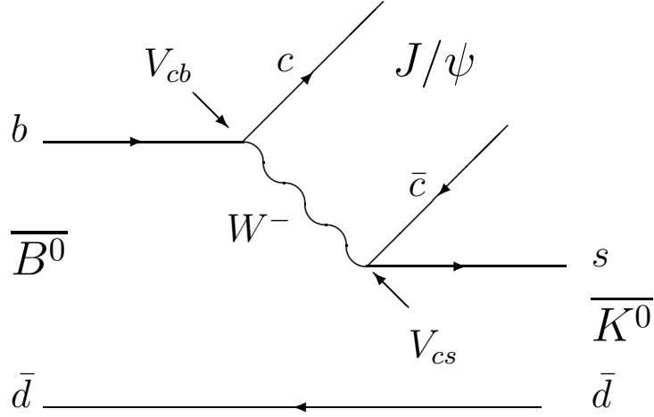
Figure 1.1: Mechanism for the decay B \rightarrow J/\psi K .
