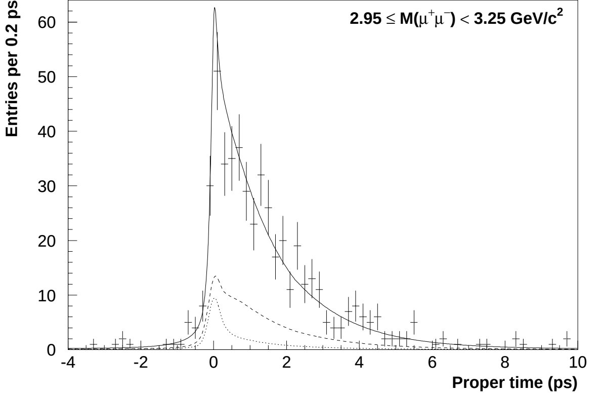
Signal lifetime fit (495 window candidates; \lambda_w = 0.0949 \pm 0.0064 , \lambda_c = 0.172 \pm 0.097 )
