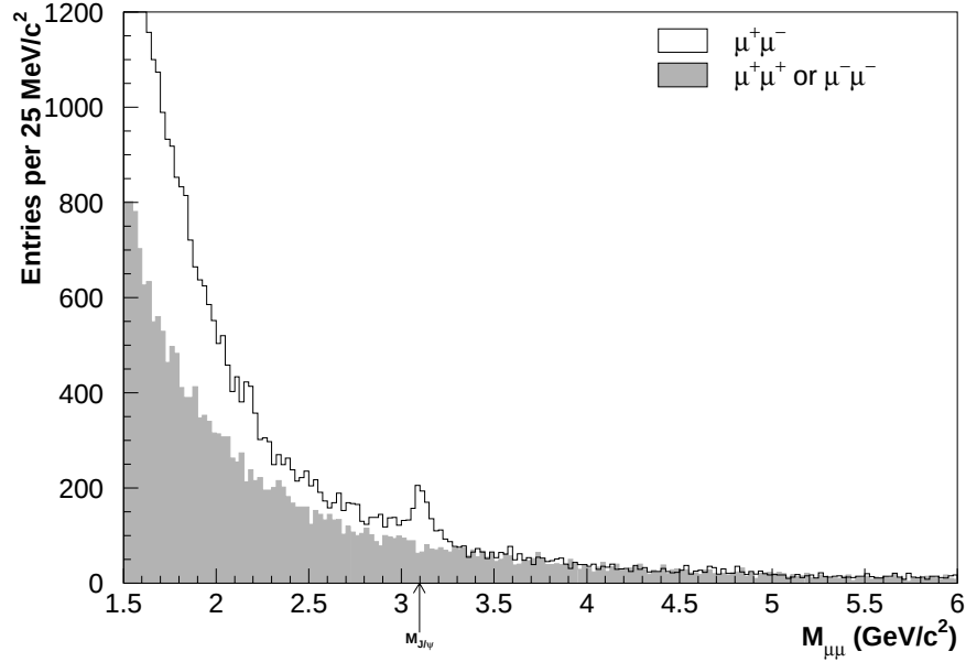
Figure 4.2: Reconstructed masses of all J/\psi candidates passing the initial cuts (1992–5). Candidates with like-signed (shaded histogram) and unlike-signed (unshaded) track charges are shown. The signal at M_{J/\psi} \approx 3.1 \text{ GeV}/c^2 can already be seen (corresponding to 472 \pm 29 \text{ J}/\psi s or (27.7 \pm 1.7)\% of the candidates in 2.95 \leq M_{\mu^+\mu^-} < 3.25 \text{ GeV}/c^2 ).
