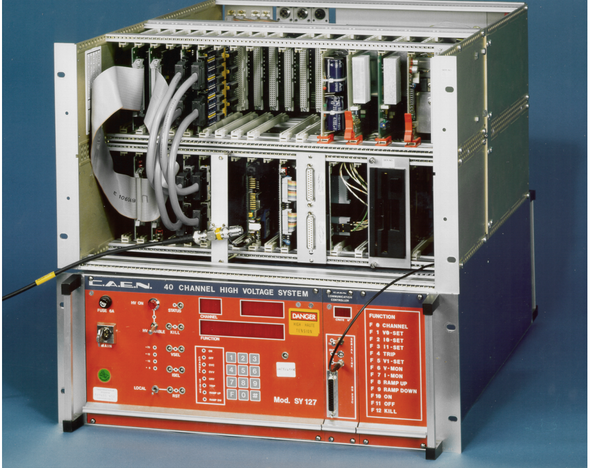
Figure 3.2: The MAC-G64 and CAEN crates. The MAC-G64 crate (on top) consists of a G64 bus below a MAC bus. The G64 bus contains, from left to right, a double-card CAEN interface, two digital input/output cards, a G64-ethernet interface connected to thinwire ethernet, a CPU card with two RS232-C connectors, and a disk controller and drive. The MAC bus contains a double-card CAEN interface, two digital input/output adapters, and the power supplies on the right. Below the MAC-G64 crate is a CAEN high voltage crate, connected to the G64 by CAENnet.
