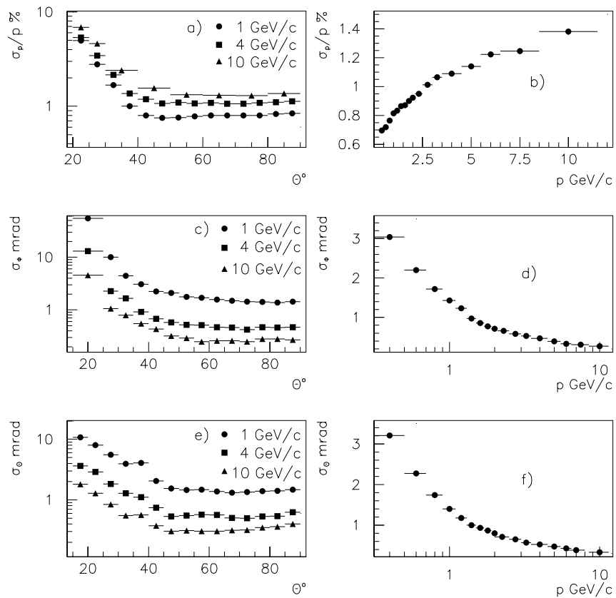
Figure 2.15: Track momentum precisions estimated by comparing simulated and reconstructed parameters. The errors in momentum (a,b), azimuthal angle \phi (c,d), and polar angle \theta (e,f) are shown. The variation of each parameter's precision with respect to \theta is shown on the left; with respect to momentum on the right.
