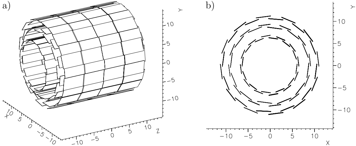
Figure 2.5: Schematic layout of the 1994 Vertex Detector in a) perspective and b) R\phi views. The scale is in cm. The geometry of the 1991–3 detector was similar, except that it did not have the longer innermost layer, and the modules of the outer two layers had a ‘paddle wheel’ arrangement.
