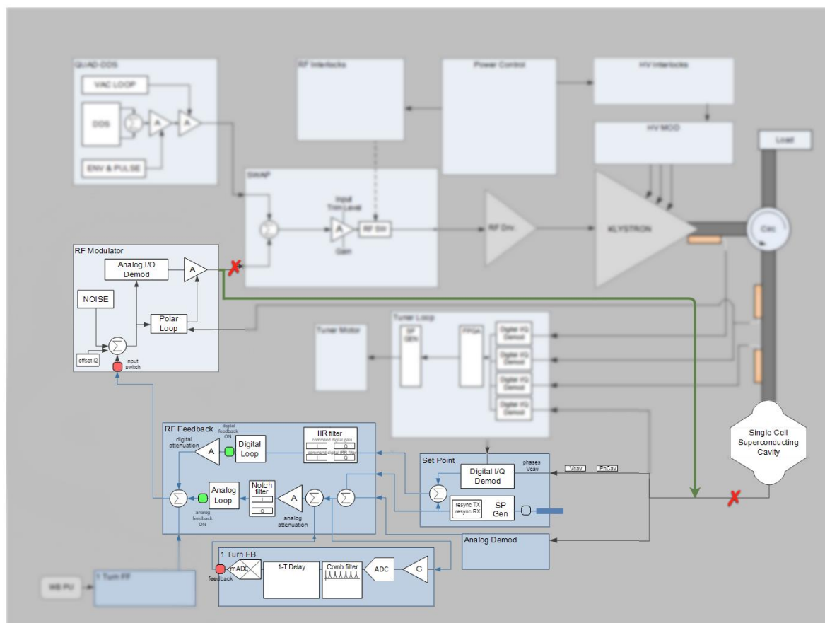
Figure 13: Preparation of the RF Modulator calibration; by-passing the cavity and the klystron by connecting the RF Modulator output to the input of the Analog Demodulator and the Set Point.
