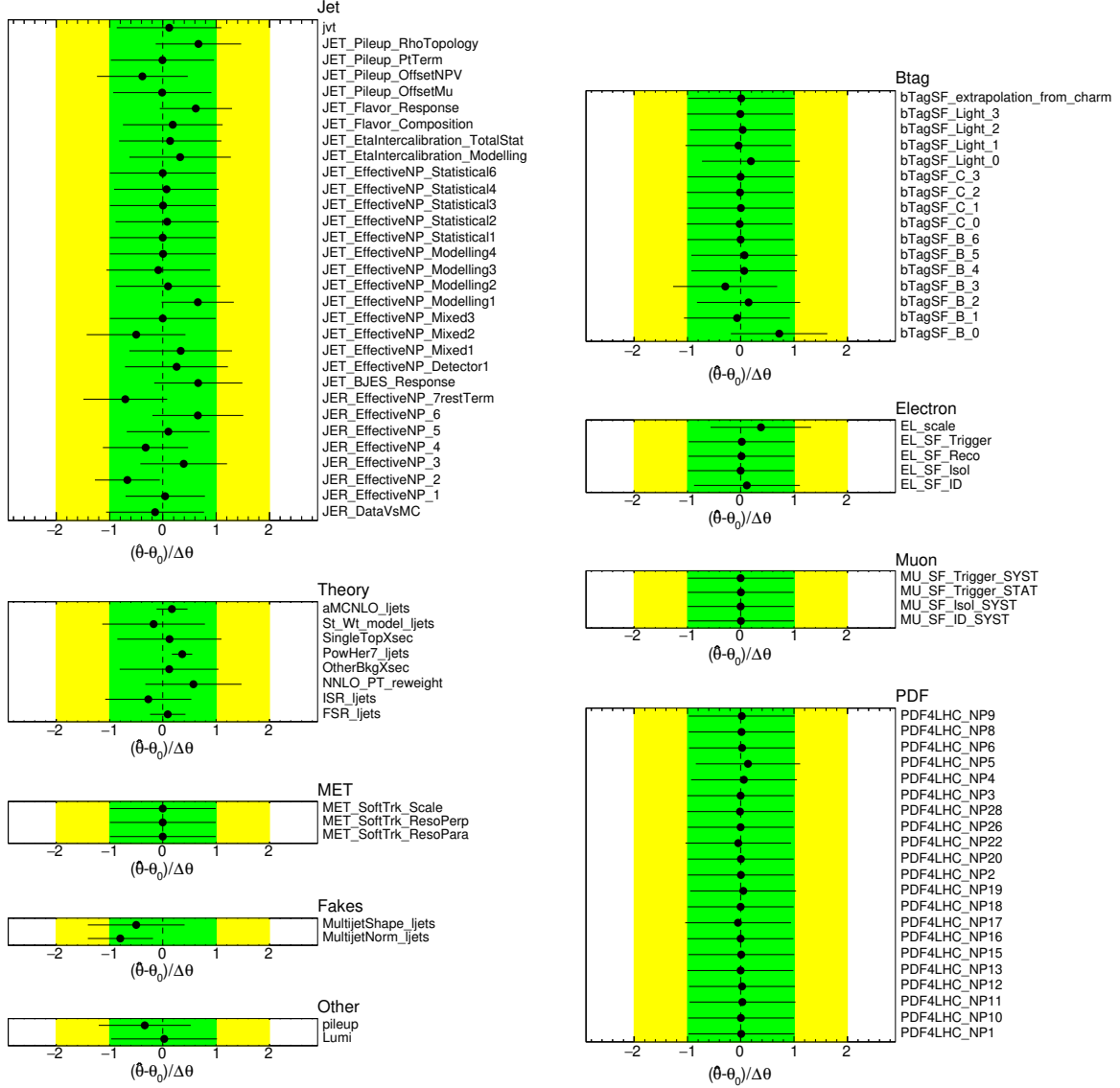
Figure 11.3.: The pull distributions for the NPs used in the fit to the observed data for the lepton+jets channel. The black dots represent the post-fit mean value of the NP, the lines represent the post-fit NP uncertainties. The green and the yellow bands represent the pre-fit one and two standard deviations, respectively.
