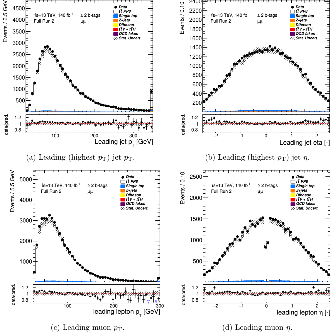
Figure A.10.: Data/MC comparison for basic kinematic properties in the dilepton decay channel with muon-muon events. MC statistical uncertainty together with the normalisation uncertainty is shown by the hashed fields. The first and the last bins correspond to the underflow and the overflow events respectively.
