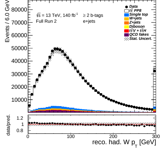
(b) Reconstructed hadronic W boson p_T .
