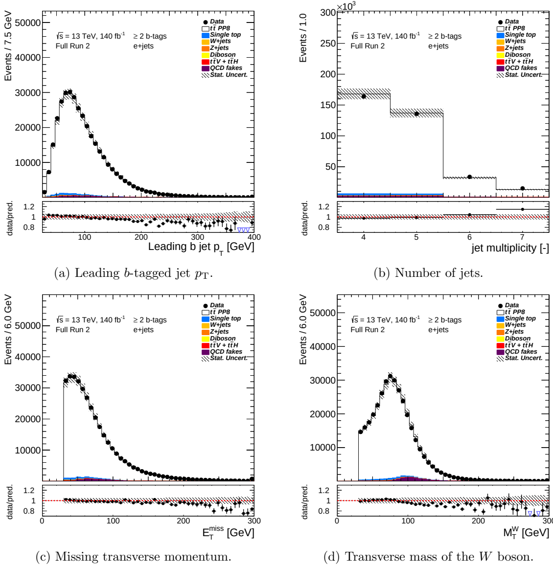
Figure 7.4.: Data/MC comparison for basic kinematic properties in the electron+jets decay channel. Selection on the BDT output score > 0.7 is applied. The hashed bands show the uncertainty originating from finite statistics in the MC samples as well as normalisation uncertainty on each signal/background source. The first and last bin contain underflow and overflow events, respectively.
