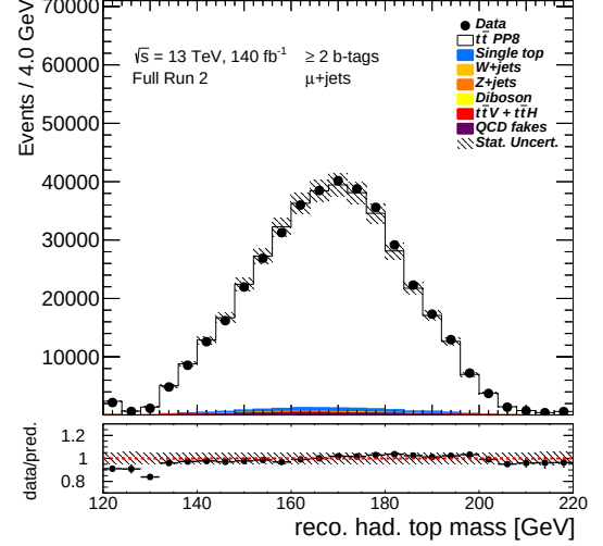
(b) Reconstructed hadronic top-quark mass.
