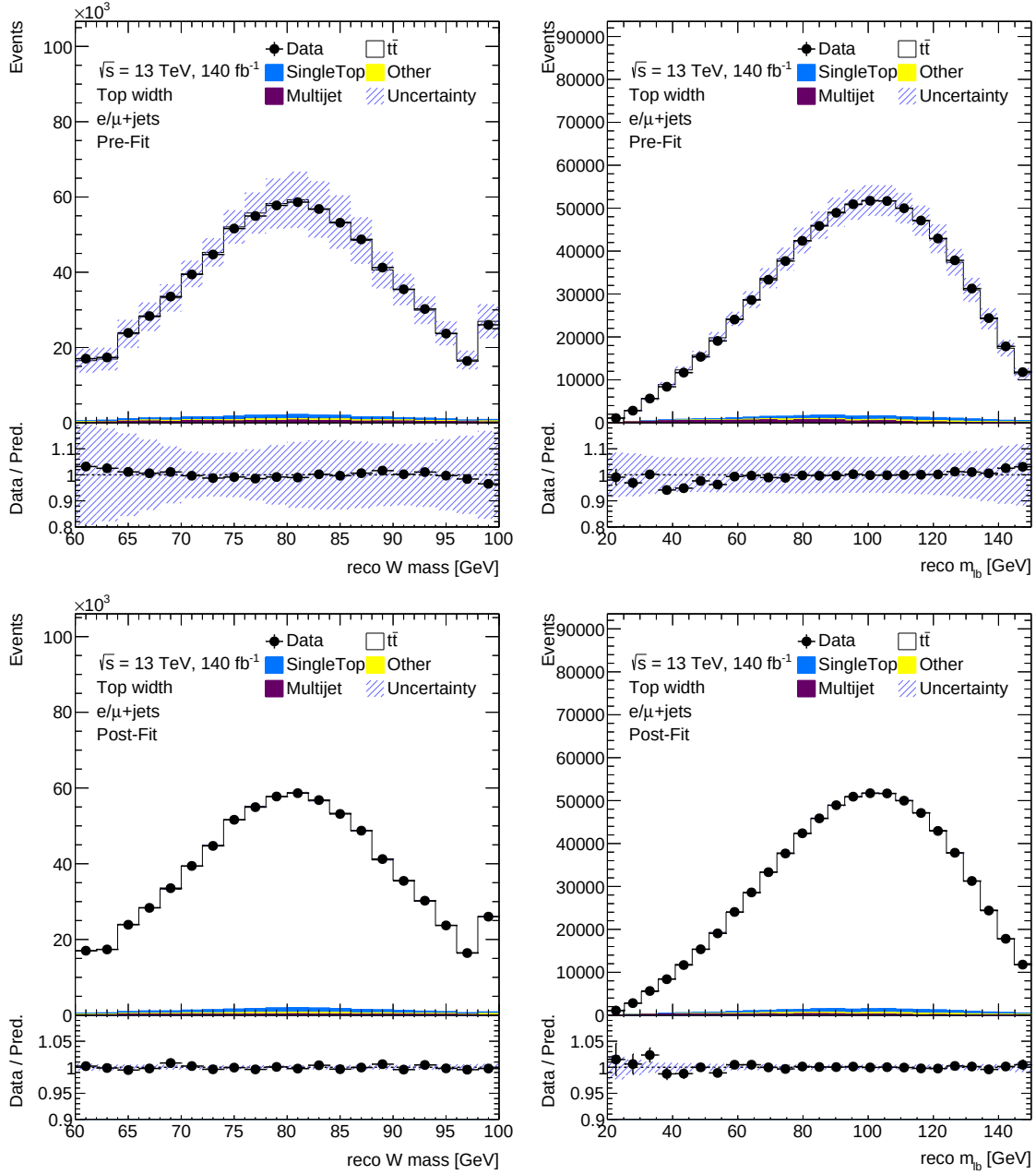
Figure 11.5.: Pre-fit (top) and post-fit (bottom) distributions for the m_W mass distribution (left) and the m_{lb} distribution (right) for the combined electron+jets and muon+jets events. The bottom panel shows the ratio of the data over prediction. The shaded bands represent the total uncertainty. Significant improvement in the agreement between data and prediction is observed as well as decreased total uncertainties after the fit. The SM prediction of \Gamma_t = 1.32 GeV is assumed in the pre-fit plots. The vertical axis in the bottom panel of the post-fit distributions has a reduced range compared to the pre-fit distribution.
