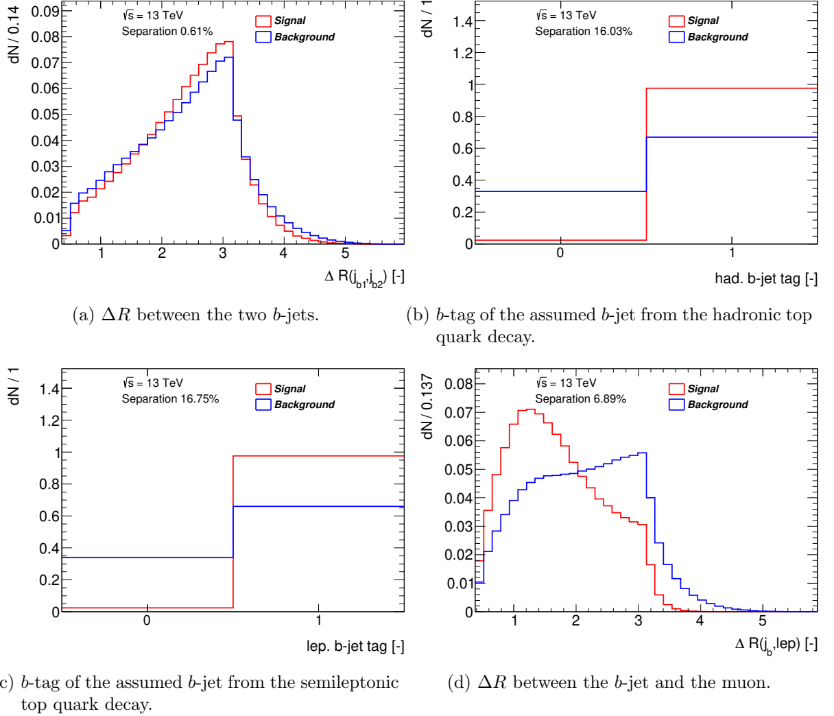
Figure C.5.: Separation power of the input variables for the reconstruction BDT. Signal (red) represents permutations where all four partons from the t\bar{t} decay are correctly assigned to their corresponding jets, while background (blue) denotes permutations where at least one of the partons is not assigned correctly. Signal and background contributions are normalised to unity. Electron+jets and muon+jets events are combined.
