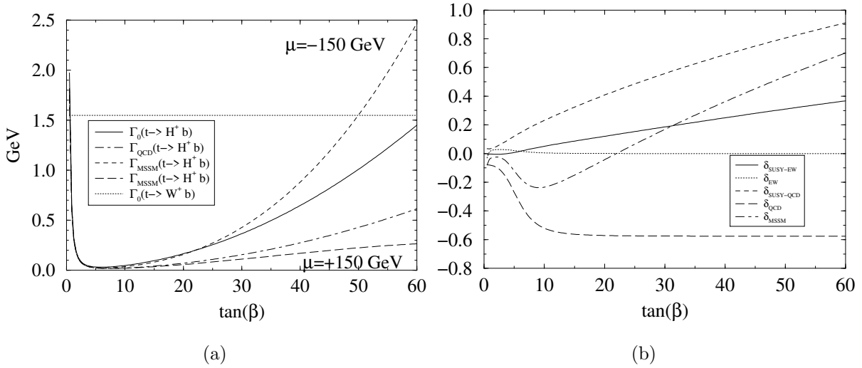
Figure 3.9.: (a) The partial decay width \Gamma(t \rightarrow H^+ b) compared to the SM total decay width as a function of \tan\beta . The results are shown for various SUSY parameter values with the charged Higgs mass m_{H^\pm} = 120 GeV. (b) Relative correction from SUSY and SM to t \rightarrow H^+ b decay. The figures are taken from [134].
