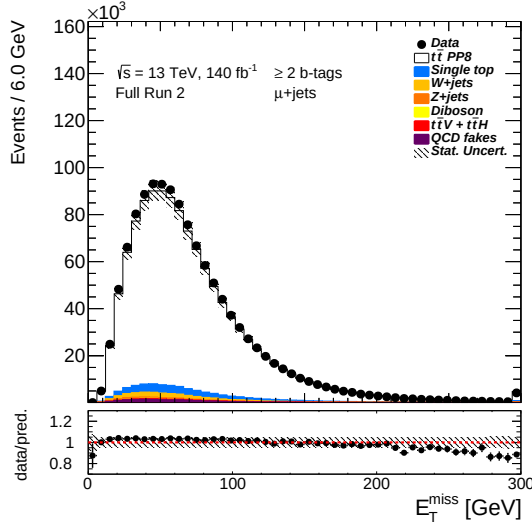
(c) Missing transverse momentum.
