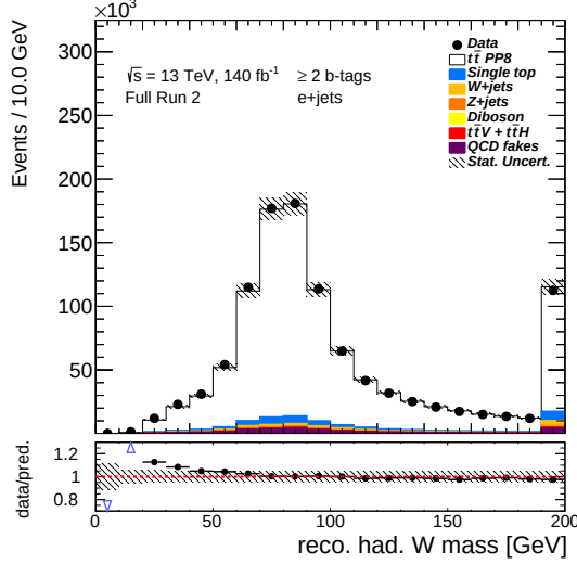
(a) Reconstructed hadronic W boson mass.
