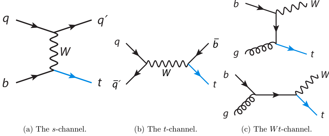
Figure 3.4.: LO Feynman diagrams for single top quark production in s -channel 3.4a, t -channel 3.4b and Wt -channel 3.4c.
