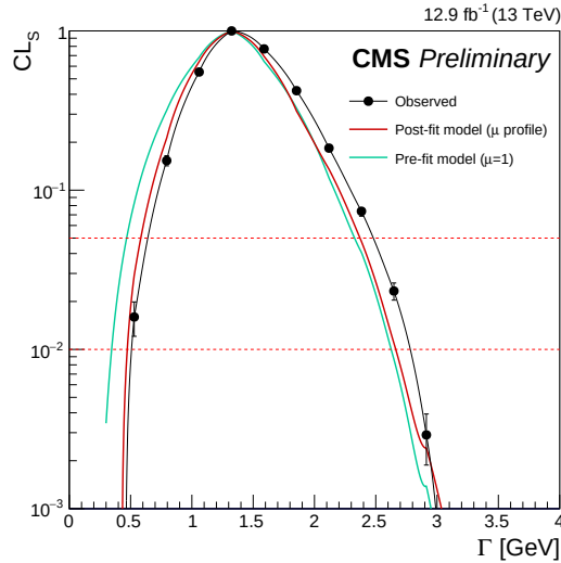
Figure 3.11.: Evolution of the \text{CL}_s as a function of the top-quark decay width. Limits of 95 % and 99 % CL limits are shown as intersections of the curve with the line at \text{CL}_s = 0.05(0.01) . Both pre-fit and post-fit results are shown [155].
