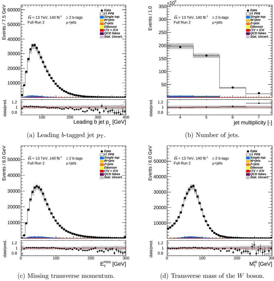
Figure 7.6.: Data/MC comparison for basic kinematic properties in the muon+jets decay channel. Selection on the BDT output score > 0.7 is applied. The hashed bands show the uncertainty originating from finite statistics in the MC samples as well as normalisation uncertainty on each signal/background source. The first and last bin contain underflow and overflow events, respectively.
