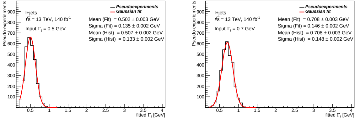
Figure F.1.: Fitted values for 3000 pseudo-experiments in the lepton+jets channel using statistical only fits. Various input widths for the pseudo-data are used: \Gamma_t = 0.5, 0.7, 1.0, 1.5 GeV. Good agreement between the input and the mean fitted value is observed. A deviation from Gaussian shape is observed for input width of 0.5 GeV due to the edge at 0.2 GeV.
