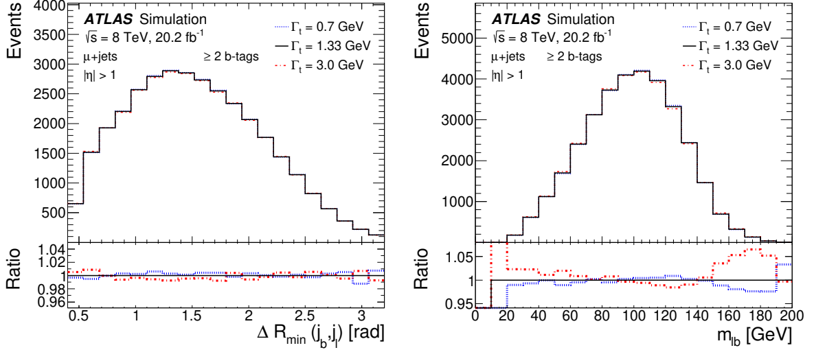
Figure 10.4.: Templates for the \Delta R_{\min}(j_b, j_l) (left) and m_{\ell b} (right) distributions for \Gamma_t = 0.7, 1.33 and 3.0 GeV in the muon+jets channel for events with at least two b -tagged jets in the region with at least one jet with |\eta| > 1 , at \sqrt{s} = 8 TeV [245]. The lower panel shows the ratio of templates with the varied \Gamma_t to the nominal template generated with \Gamma_t = 1.33 GeV. The mass of the top quark is set to m_t = 172.5 GeV.
