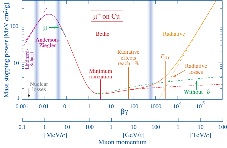
Figure 4.9. A plot of stopping power versus muon momentum. [1]
