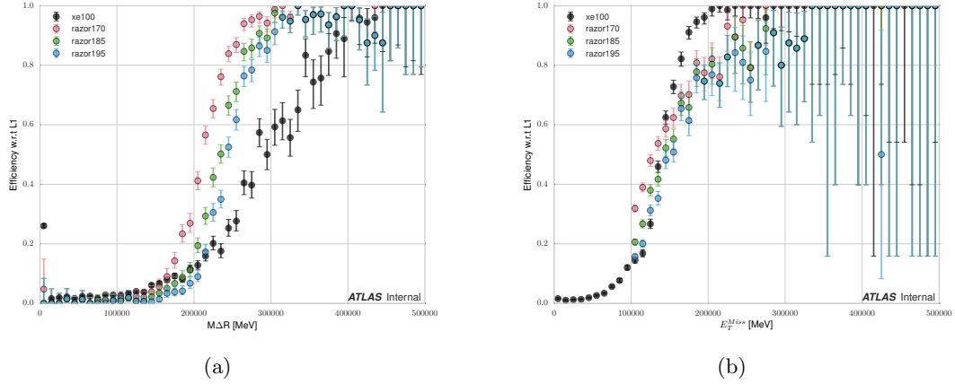
Figure 8.48. The efficiency of Razor and xe100 triggers.
