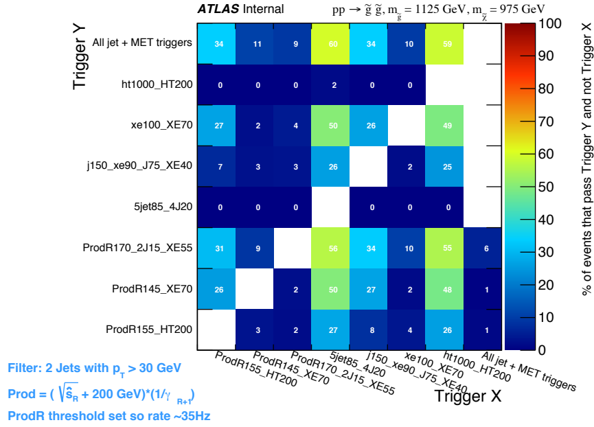
Figure 8.43. The unique rate for triggers in the jet+MET category for a compressed gluino model. Events that pass Trigger Y do not pass Trigger X.
