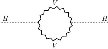
Figure C.9. A Feynman diagram for Higgs self-energy with a one-loop W^\pm or Z^0 correction.
