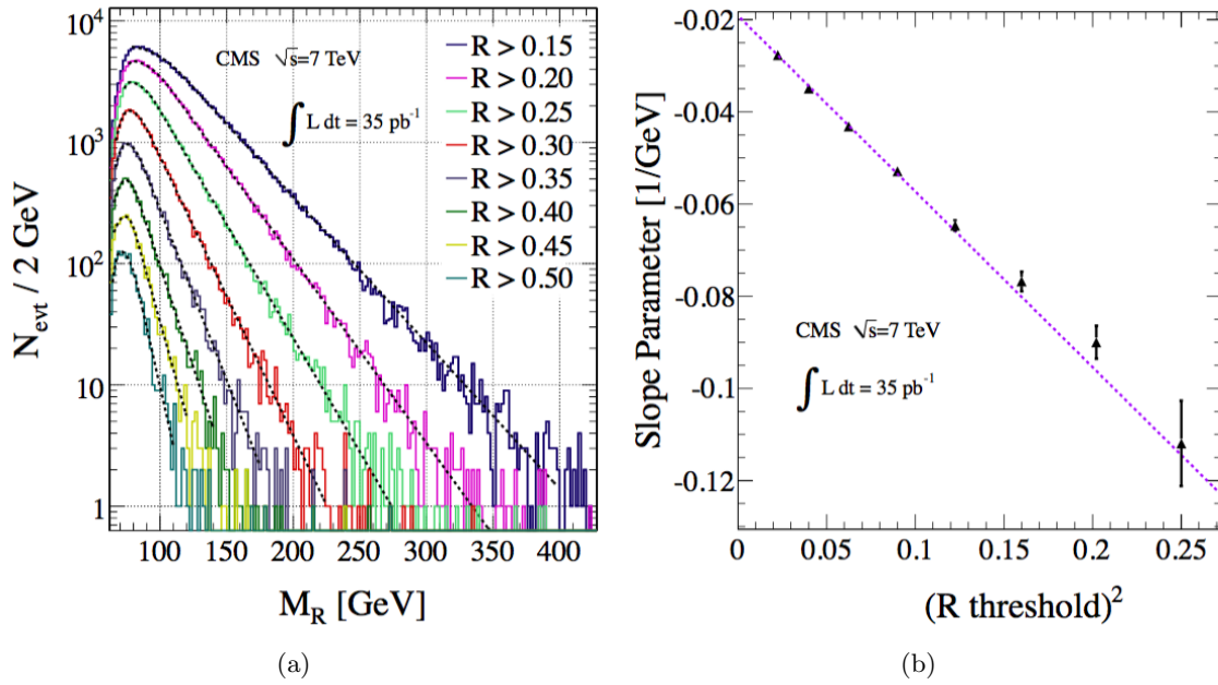
Figure 9.6. The QCD multijet estimate employed by CMS. In (a), the distribution of M_R is shown for increasing R cuts and (b) the slope of the exponential decay is plotted as a function of R^2 .
