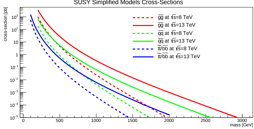
Figure 8.7. The cross-sections for SUSY production at \sqrt{s} = 8 TeV (dashed lines) and \sqrt{s} = 13 TeV (solid lines).
