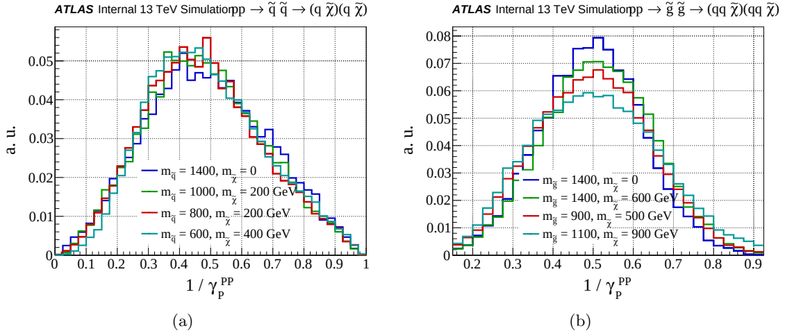
Figure 8.11. A distribution of 1/\gamma_P^{PP} for (a) \tilde{q}\bar{\tilde{q}} \rightarrow q\bar{q}\tilde{\chi}_1^0\tilde{\chi}_1^0 and (b) \tilde{g}\bar{\tilde{g}} \rightarrow q\bar{q}q\bar{q}\tilde{\chi}_1^0\tilde{\chi}_1^0 .
