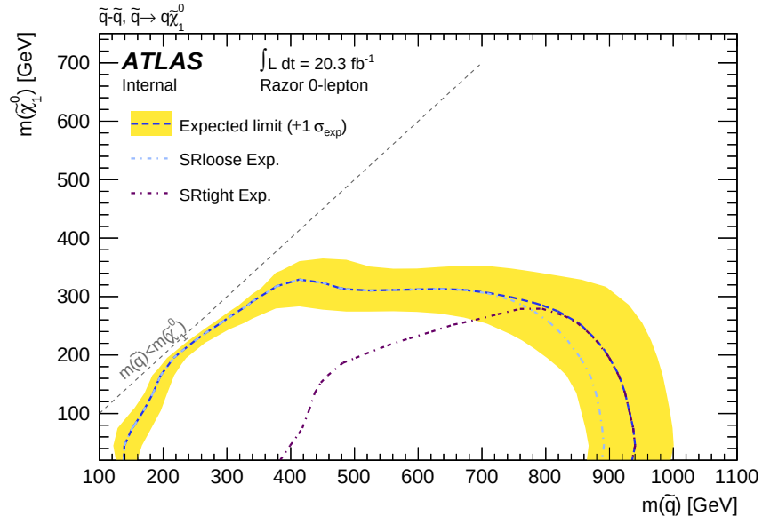
Figure 10.21. The component exclusion results for the m_{\tilde{\chi}_1^0} versus m_{\tilde{q}} in the \tilde{q}\tilde{q} direct decay simplified model.
