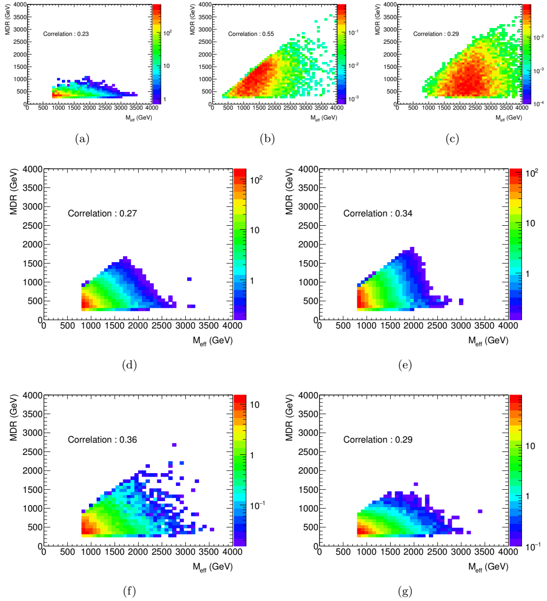
Figure D.12. M_{eff} and M_{\Delta}^R correlation for (a) QCD multijets, (b) \tilde{q}(900), \tilde{\chi}(0) , and (c) \tilde{g}(1400), \tilde{\chi}(0) , (d) W + jets , (e) Z + jets , (f) Diboson, and (g) Top.
