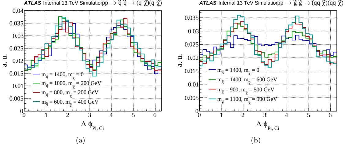
Figure 8.19. A distribution of \Delta\phi_{P_i, C_i} for (a) q\bar{q} \rightarrow q\bar{q}\tilde{\chi}_1^0\tilde{\chi}_1^0 and (b) \tilde{g}\tilde{g} \rightarrow qq\tilde{\chi}_1^0\tilde{\chi}_1^0 .
