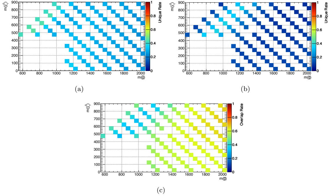
Figure 11.16. SR complementarity between M_{\text{eff}} and RJ for all gluino grid points showing (a) unique rate for M_{\text{eff}} , (b) unique rate for RJ, and (c) overlapping rate.
