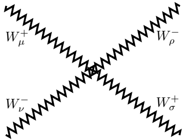
Figure B.20. The Feynman rule for the W^\pm W^\mp W^\pm W^\mp vertex.
