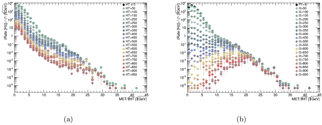
Figure 8.40. A comparison of the rates of E_T^{\text{miss}}/\sqrt{H_T} of various cuts to (a) H_T and (b) \bar{\Pi} .
