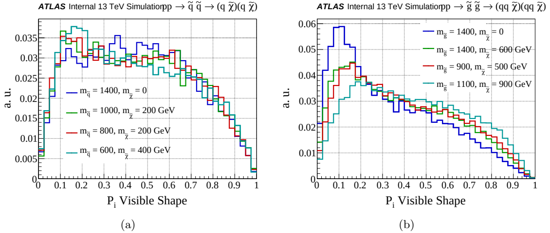
Figure 8.21. A distribution of VS_P for (a) \tilde{q}\tilde{q} \rightarrow qq\tilde{\chi}_1^0\tilde{\chi}_1^0 and (b) \tilde{g}\tilde{g} \rightarrow qq\tilde{\chi}_1^0\tilde{\chi}_1^0 .
