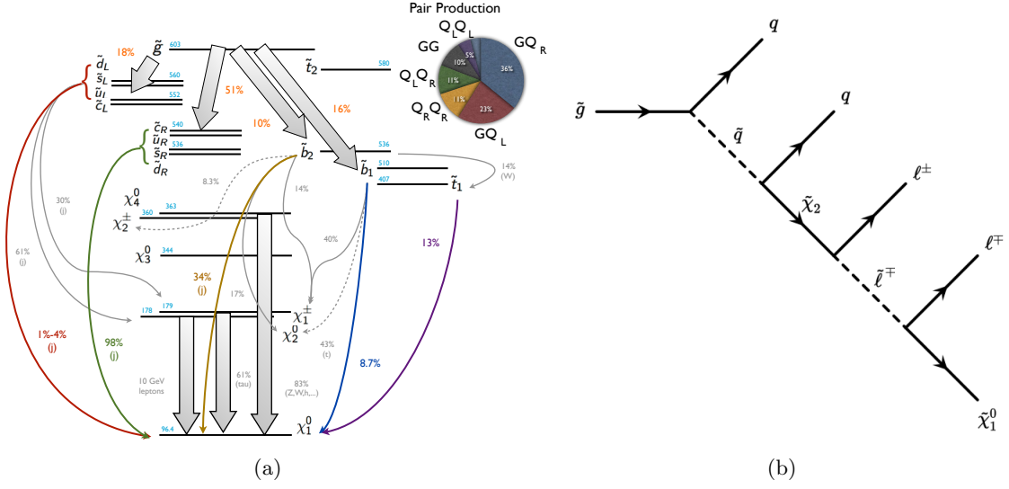
Figure 3.6. A comparison of (a) cMSSM to (b) simplified model gluino decay.
