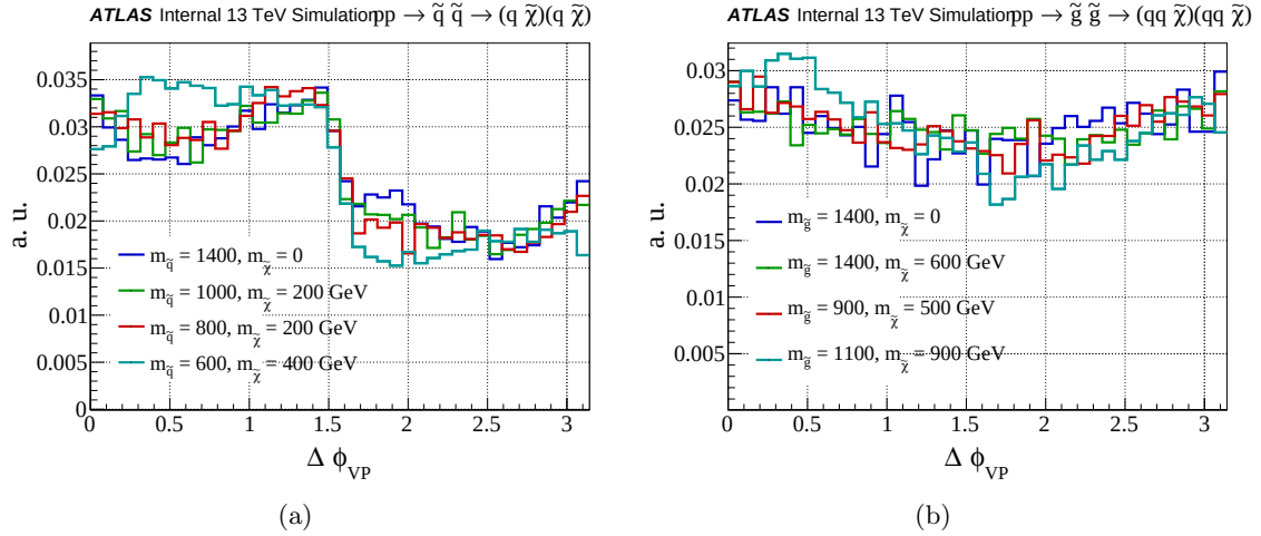
Figure 8.17. A distribution of \Delta\phi_{VP} for (a) \tilde{q}\tilde{q} \rightarrow qq\tilde{\chi}_1^0\tilde{\chi}_1^0 and (b) \tilde{g}\tilde{g} \rightarrow qq\tilde{q}\tilde{q}\tilde{\chi}_1^0\tilde{\chi}_1^0 .
