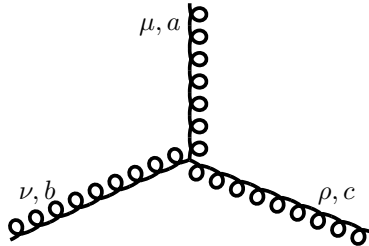
Figure B.16. The Feynman rule for the ggg vertex.
