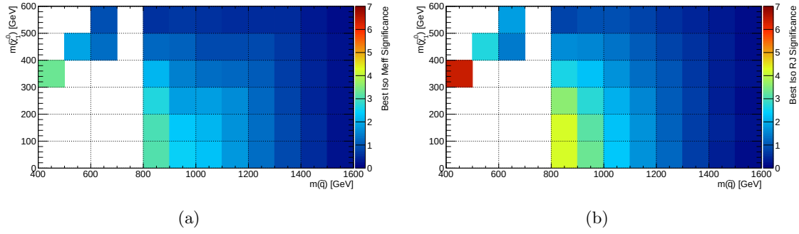
Figure 11.35. Expected exclusion sensitivity to the \tilde{q} direct decay mass plane comparing the most performant (left) M_{\text{eff}} SRs and (right) RJ SRs.
