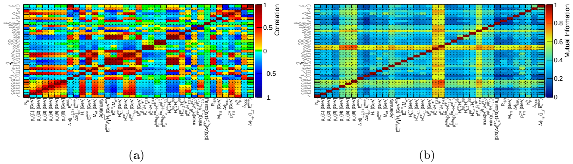
Figure 11.28. Variable (a) correlation and (b) mutual information used for M_{\text{eff}} and RJ analyses for a large mass-splitting gluino simplified model.
