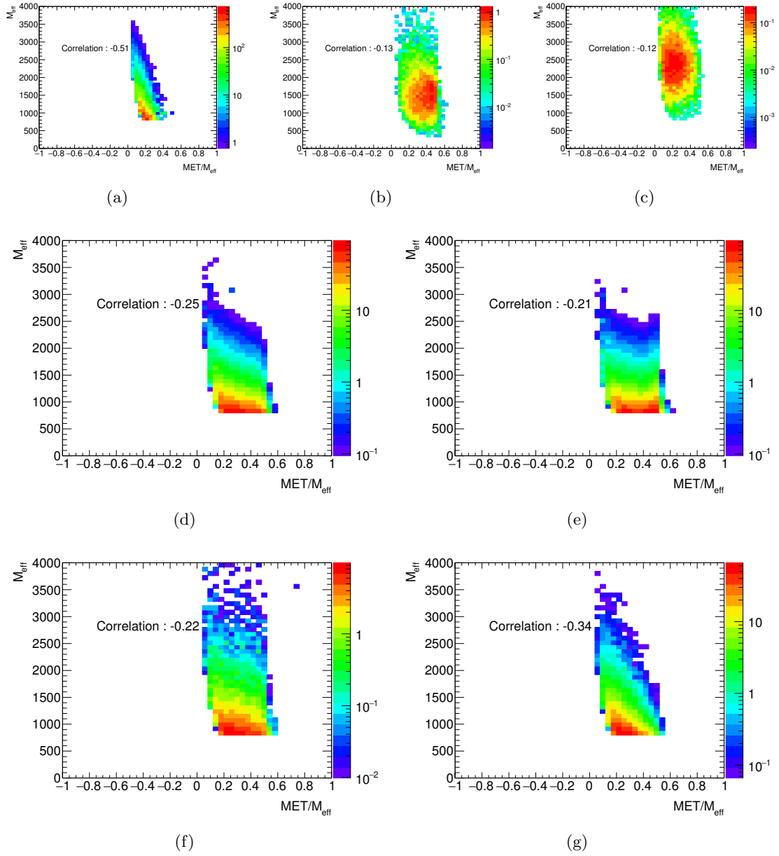
Figure D.11. E_T^{miss}/M_{eff} and M_{eff} correlation for (a) QCD multijets, (b) \tilde{q}(900), \tilde{\chi}(0) , and (c) \tilde{g}(1400), \tilde{\chi}(0) , (d) W + jets , (e) Z + jets , (f) Diboson, and (g) Top.
