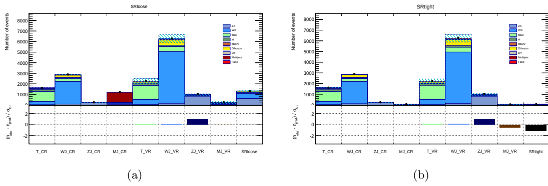
Figure 10.19. The pull on BG weights after the combined fit for (a) SRloose and (b) SRtight.
