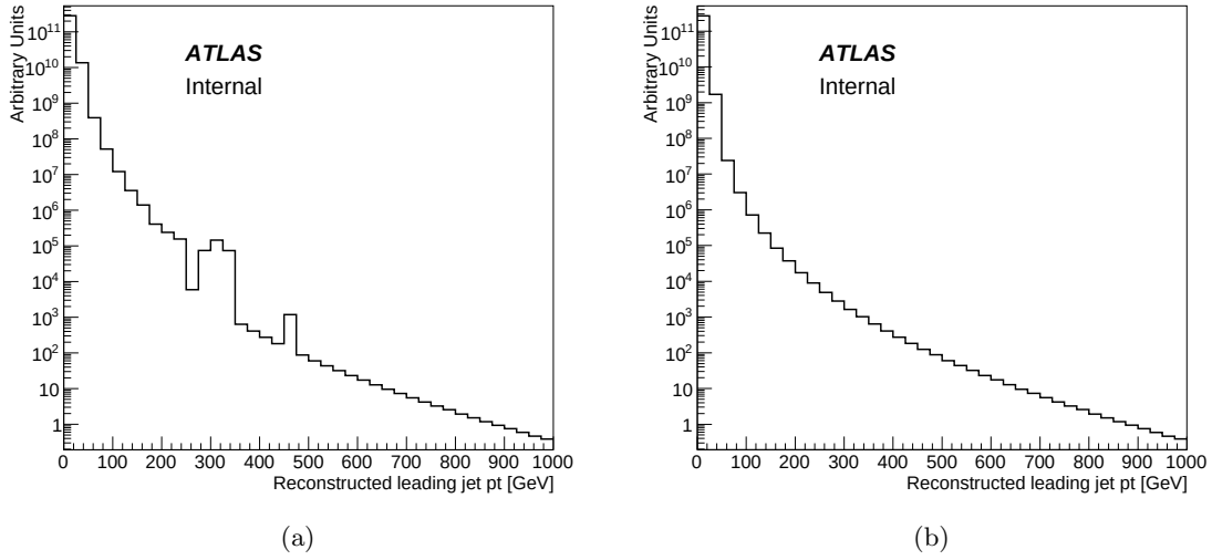
Figure 10.11. A comparison of the leading jet p_T spectrum (a) before and (b) after truth cleaning.
