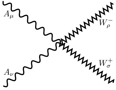
Figure B.17. The Feynman rule for the \gamma^0\gamma^0 W^\pm W^\mp vertex.
