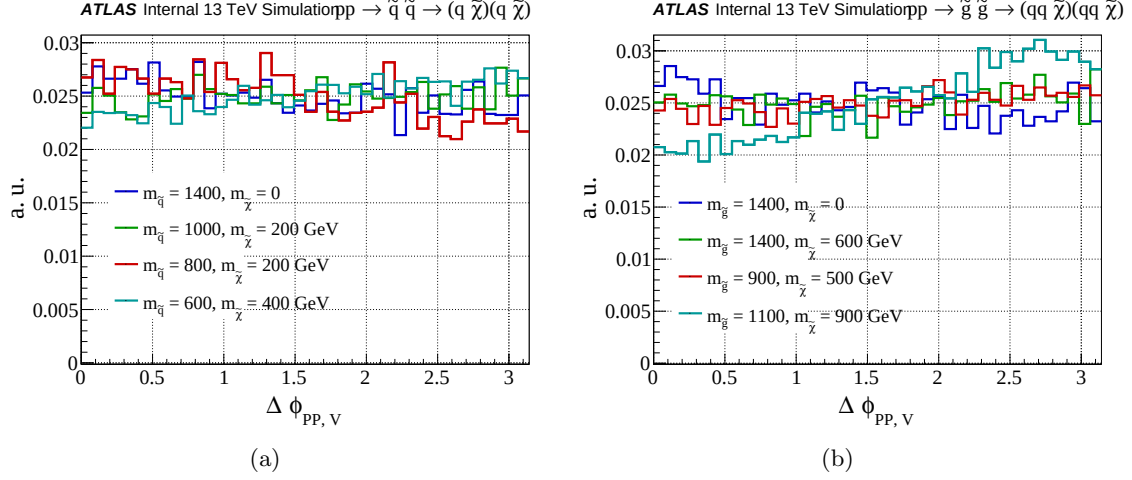
Figure 8.16. A distribution of \Delta\phi_{PP,V} for (a) \tilde{q}\tilde{q} \rightarrow qq\tilde{\chi}_1^0\tilde{\chi}_1^0 and (b) \tilde{g}\tilde{g} \rightarrow qq\tilde{q}\tilde{q}\tilde{\chi}_1^0\tilde{\chi}_1^0 .
