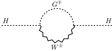
Figure C.5. A Feynman diagram for Higgs self-energy with a one-loop W^\pm and a Goldstone G^\mp correction.
