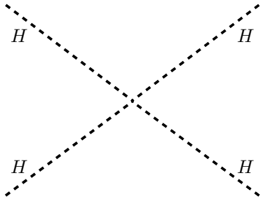
Figure B.27. The Feynman rule for the HHHH vertex.
