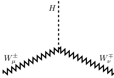
Figure B.22. The Feynman rule for the HW^\pm W^\mp vertex.
