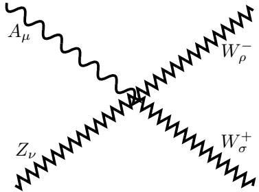
Figure B.19. The Feynman rule for the \gamma^0 W^\pm W^\mp Z^0 vertex.
