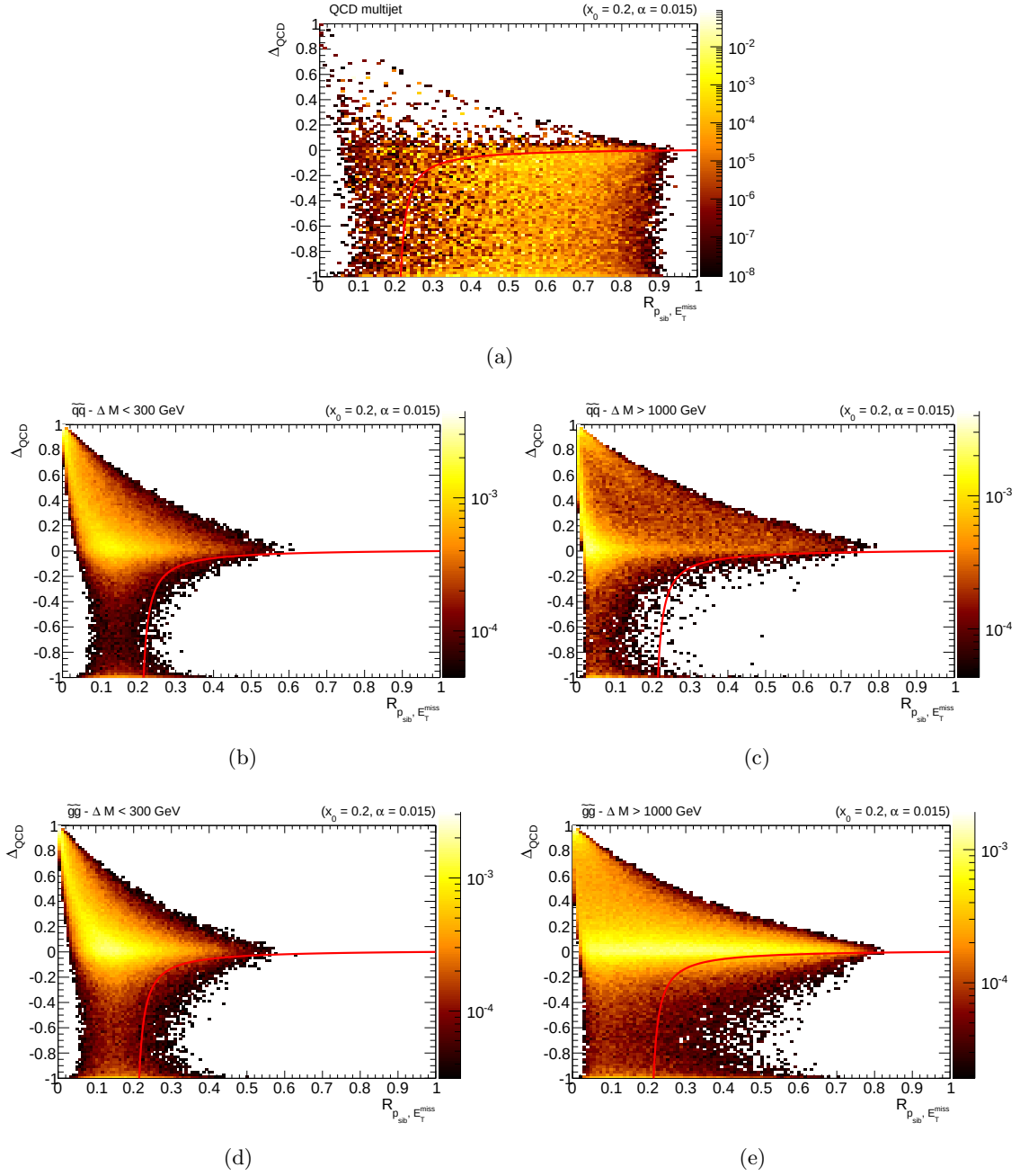
Figure 11.2. The distribution of \Delta_{QCD} versus R_{p_{sib}, E_T^{miss}} for (top) QCD multijets, (middle) \tilde{q} , and (bottom) \tilde{g} decays with (left) M_{Delta} < 300 GeV and (right) M_{\Delta} > 1000 .
