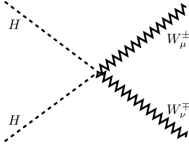
Figure B.23. The Feynman rule for the HHW^\pm W^\mp vertex.
