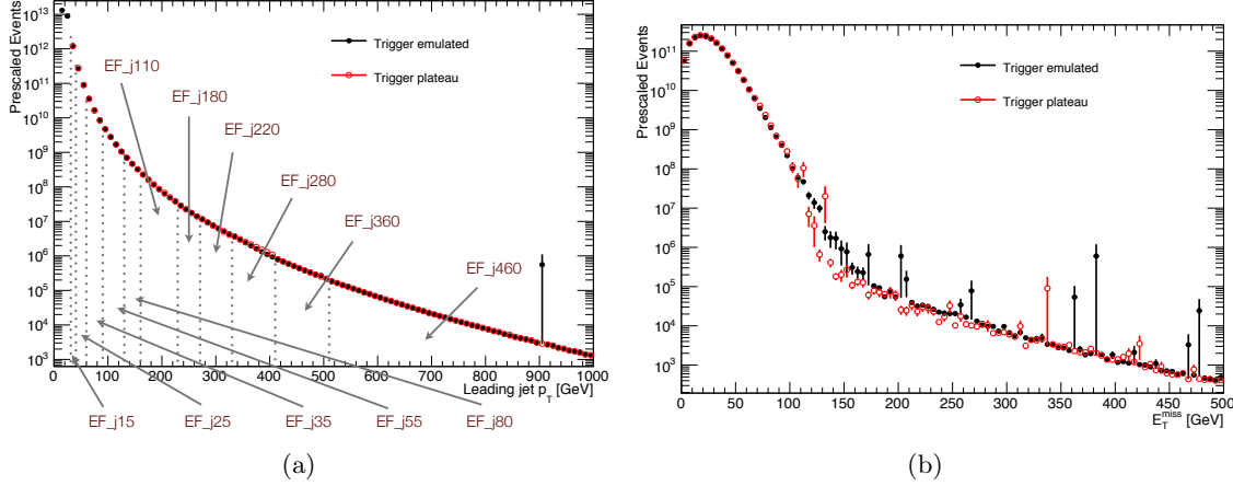
Figure 8.42. A distribution of the reconstructed prescaled data for (a) p_T and (b) E_T^{\text{miss}} for a preliminary validation of the trigger.
