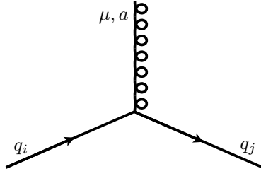
Figure B.13. The Feynman rule for the qqg vertex.
