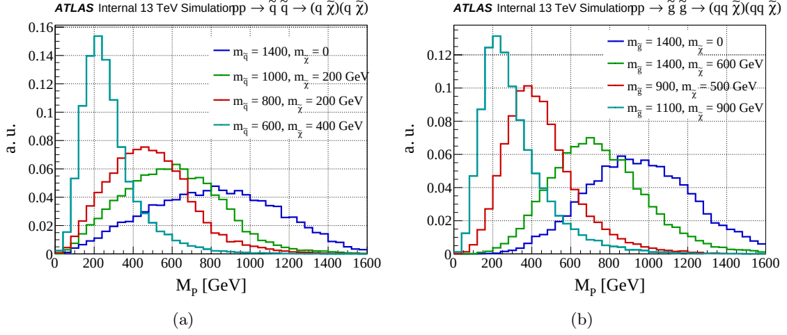
Figure 8.10. A distribution of M_P for (a) \tilde{q}\bar{\tilde{q}} \rightarrow q\bar{q}\tilde{\chi}_1^0\tilde{\chi}_1^0 and (b) \tilde{g}\bar{\tilde{g}} \rightarrow q\bar{q}q\bar{q}\tilde{\chi}_1^0\tilde{\chi}_1^0 .
