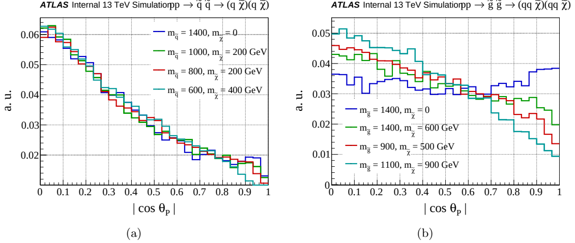
Figure 8.15. A distribution of \cos \theta_P for (a) q\bar{q} \rightarrow qq\tilde{\chi}_1^0\tilde{\chi}_1^0 and (b) g\bar{g} \rightarrow qq\tilde{\chi}_1^0\tilde{\chi}_1^0 .
