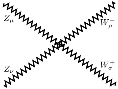
Figure B.18. The Feynman rule for the W^\pm W^\mp Z^0 Z^0 vertex.
