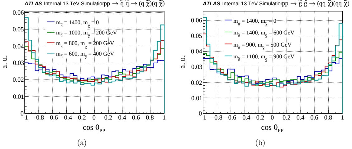
Figure 8.14. A distribution of \cos \theta_{PP} for (a) q\bar{q} \rightarrow qq\tilde{\chi}_1^0\tilde{\chi}_1^0 and (b) g\bar{g} \rightarrow qq\tilde{\chi}_1^0\tilde{\chi}_1^0 .
