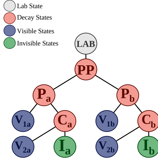
Figure 8.18. The decay tree used for reconstructing pp \rightarrow \widetilde{g}\widetilde{g} \rightarrow qq \widetilde{q}\widetilde{q} \rightarrow qq qq \widetilde{\chi}_1^0 \widetilde{\chi}_1^0 .
