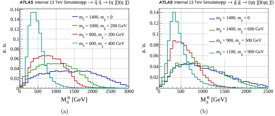
Figure 8.13. A distribution of M_\Delta^R for (a) \tilde{q}\tilde{q} \rightarrow qq \tilde{\chi}_1^0 \tilde{\chi}_1^0 and (b) \tilde{g}\tilde{g} \rightarrow qq q \tilde{\chi}_1^0 \tilde{\chi}_1^0 .
