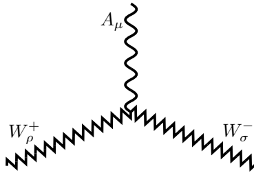
Figure B.14. The Feynman rule for the \gamma^0 W^{\pm} W^{\mp} vertex.
