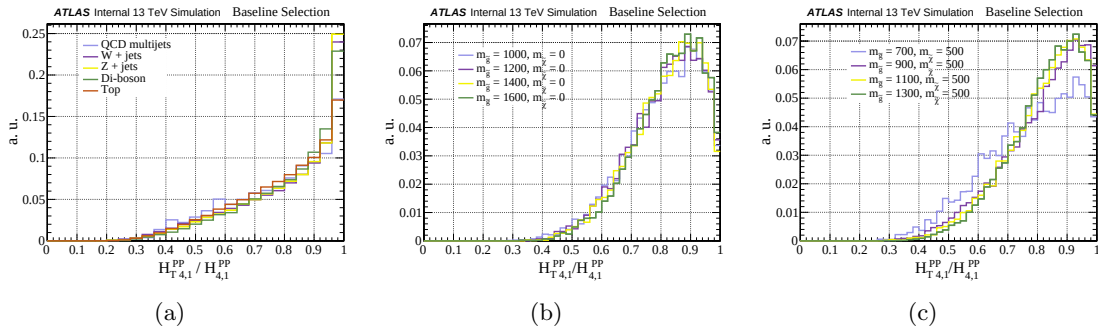
Figure 8.30. A distribution of H_{T,1}^{PP} / H_{4,1}^{PP} for (a) BG, (b) large mass-splitting digluino, and (c) intermediate mass-splitting digluino.
