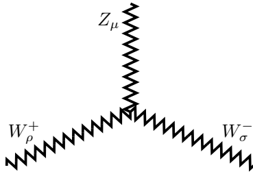
Figure B.15. The Feynman rule for the W^{\pm} W^{\mp} Z^0 vertex.
