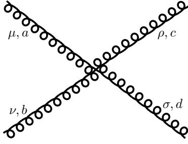
Figure B.21. The Feynman rule for the gggg vertex.
