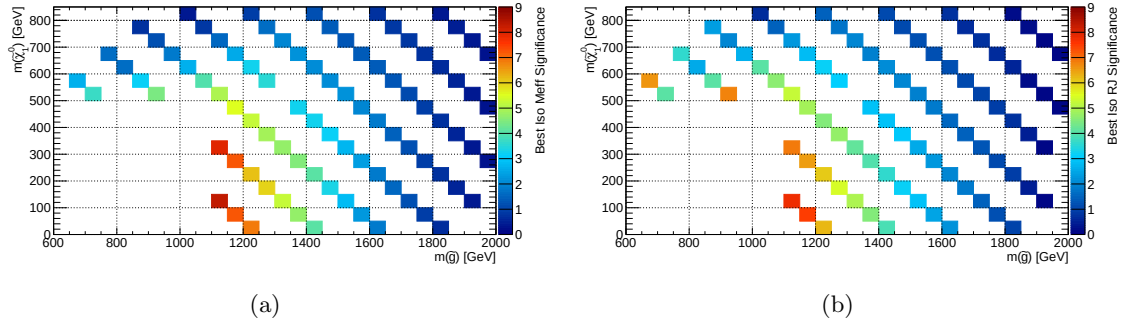
Figure 11.36. Expected exclusion sensitivity to the \tilde{q} direct decay mass plane comparing the most performant (left) M_{\text{eff}} SRs and (right) RJ SRs.
