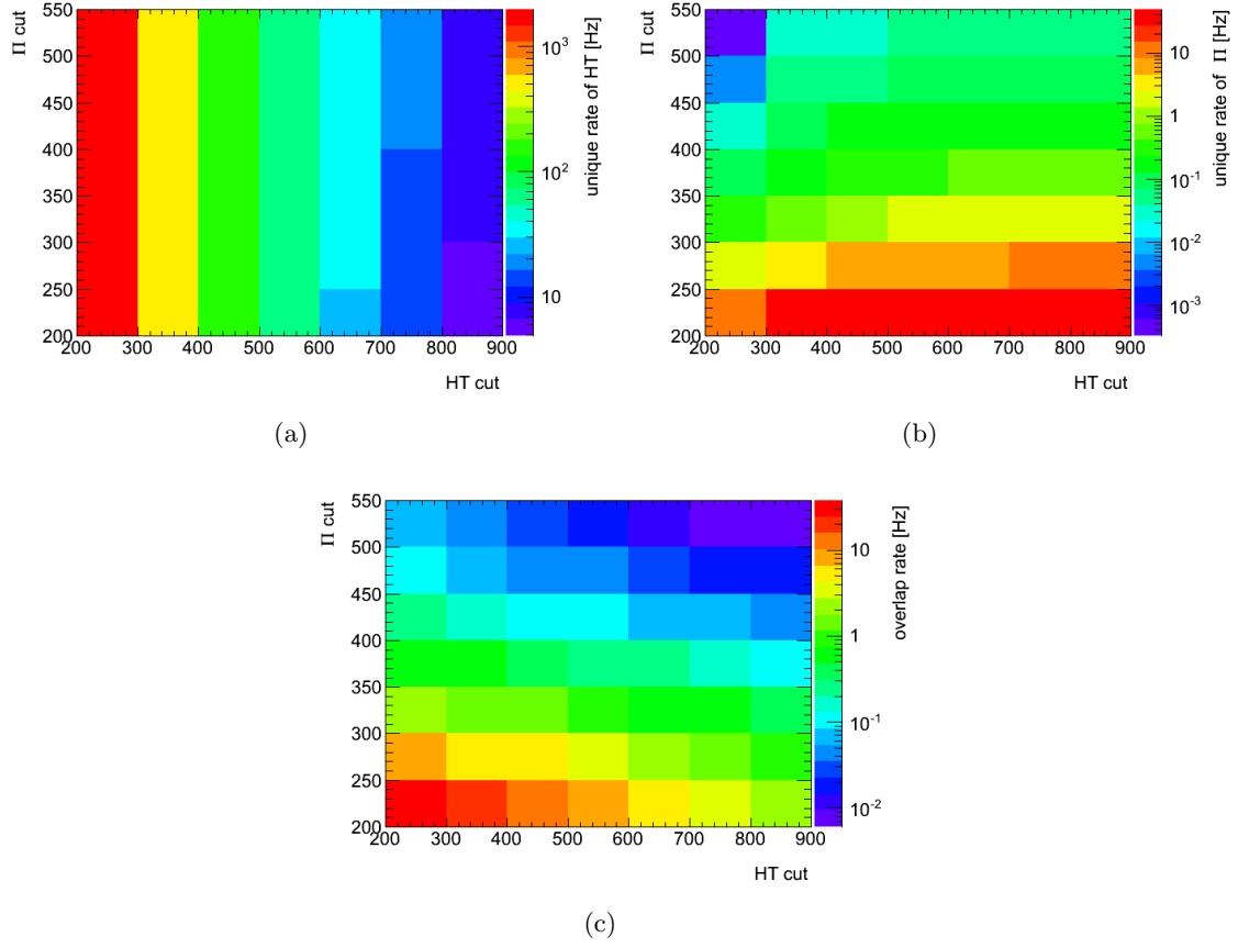
Figure 8.39. A comparison of the rates after various H_T and \bar{\Pi} cuts expected for (a) unique events selected by H_T , (b) unique events selected by \bar{\Pi} , and (c) an overlap of events.
