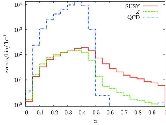
Figure 8.5. A distribution of \alpha_T .
