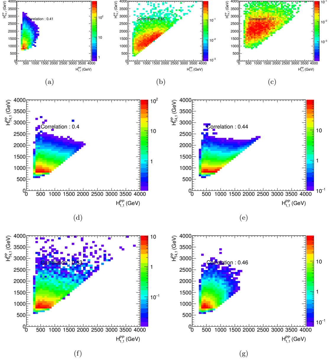
Figure D.18. H_2^{PP} and H_{T_5}^{PP} correlation for (a) QCD multijets, (b) \tilde{q}(900), \tilde{\chi}(0) , and (c) \tilde{g}(1400), \tilde{\chi}(0) , (d) W + jets , (e) Z + jets , (f) Diboson, and (g) Top.
