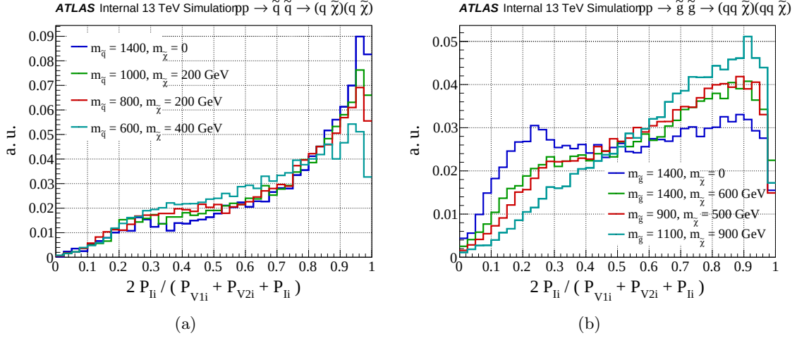
Figure 8.20. A distribution of R_{P_{1i}}^{P_i} for (a) \tilde{q}\tilde{q} \rightarrow qq\tilde{\chi}_1^0\tilde{\chi}_1^0 and (b) \tilde{g}\tilde{g} \rightarrow qq\tilde{\chi}_1^0\tilde{\chi}_1^0 .
