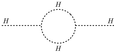
Figure C.6. A Feynman diagram for Higgs self-energy with a one-loop Higgs correction.
