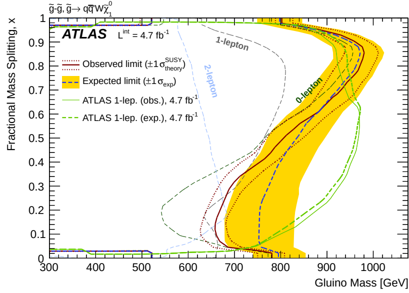
Figure 9.27. An exclusion plot in the m_{\text{frac}} versus m_{\tilde{g}} plane.
