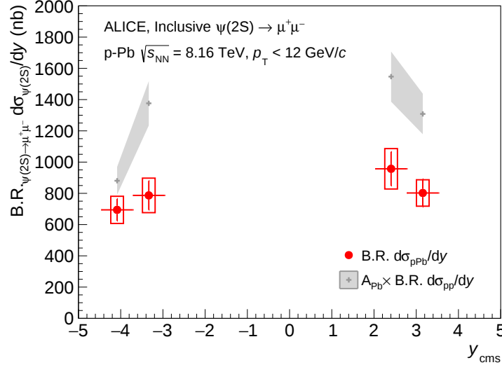
Figure A.12: The differential cross section times branching ratio \text{B.R.}_{\psi(2S) \rightarrow \mu^+ \mu^-} d\sigma^{\psi(2S)} / dy for p_T < 12 GeV/c. The error bars represent the statistical uncertainties, while the boxes correspond to total systematic uncertainties. The grey bands correspond to the reference pp cross section scaled by A_{\text{Pb}} .
