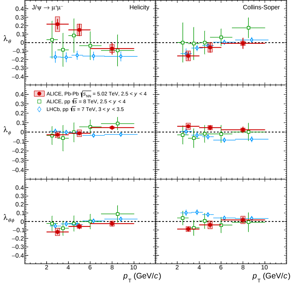
Figure 5.27: Inclusive J/ψ polarization parameters as a function of transverse momentum for Pb–Pb collisions at \sqrt{s_{NN}} = 5.02 TeV [1], compared with results obtained in pp collisions by ALICE at \sqrt{s} = 8 TeV [196] and by LHCb for prompt J/ψ at \sqrt{s} = 7 TeV [159] (the LHCb markers were shifted horizontally by +0.3 GeV/c for better visibility) in the rapidity interval 3 < y < 3.5 . The error bars represent the total uncertainties for the pp results, while for Pb–Pb statistical and systematic uncertainties are plotted separately as a vertical bar and a shaded box, respectively. In the left part of the plot the polarization parameters in the helicity reference frame are reported, in the right those for the Collins-Soper frame.
