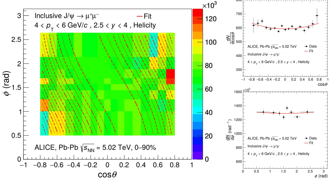
Figure 5.16: Left panel: fit to the J/ \psi corrected distribution as a function of \cos\theta and \phi for 4 < p_T < 6 GeV/ c in the helicity reference frame. Right panel: projection of the two-dimensions distribution and fitting function along \cos\theta and \phi for 4 < p_T < 6 GeV/ c in the helicity reference frame.
