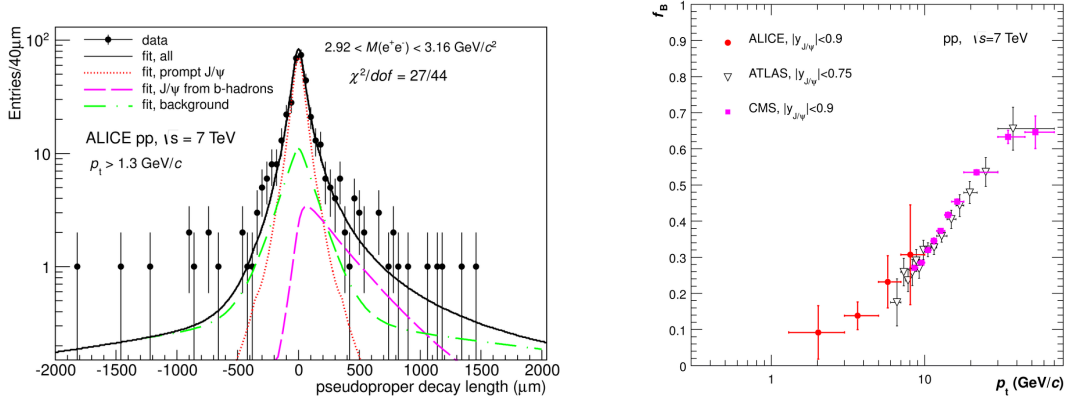
Figure 2.4: Left panel: fit to the J/\psi pseudoproper decay length distribution [78]. Right panel: The fraction of J/\psi from the decay of B -hadrons as a function of p_T compared with results from ATLAS [79] and CMS [80] in pp collisions at \sqrt{s} = 7 TeV.
