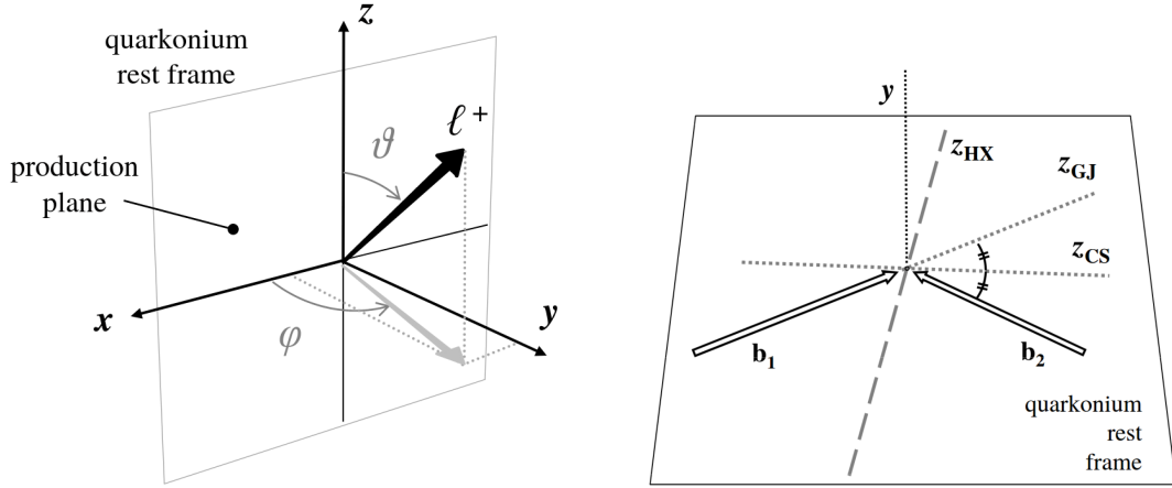
Figure 3.3: Left panel: illustration of the coordinate system used for the measurement of the angular variables for a two body decay. Right panel: representation of the z -axis for different reference frames definitions: helicity (HX), Collins-Soper (CS) and Gottfried-Jackson (GJ). Both the figures are taken from [140].
