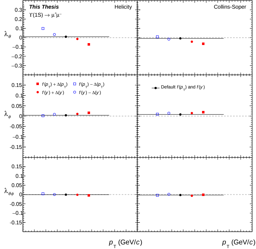
Figure 6.7: Comparison between the three polarization parameters obtained using the alternative and the default p_T and y distributions in the Monte Carlo generation.
