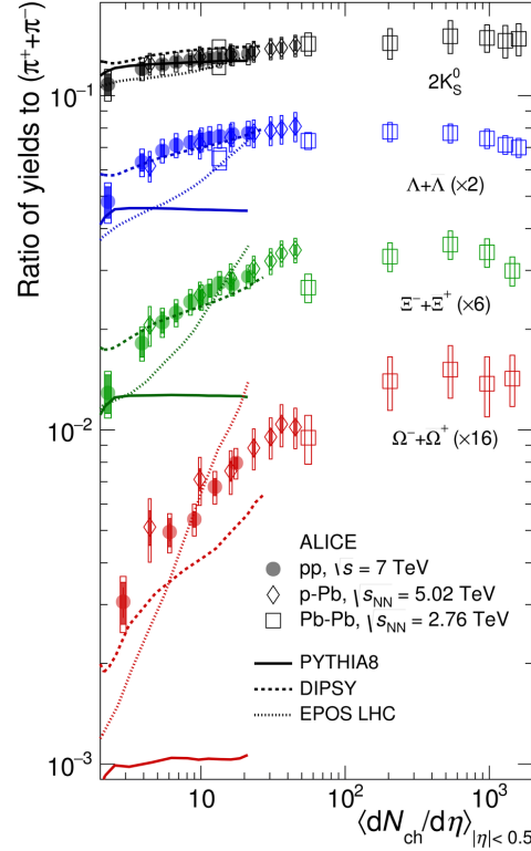
Figure 1.13: p_T -integrated yield ratios to pions ( \pi^+ + \pi^- ) as a function of \langle dN_{\text{ch}}/d\eta \rangle for |y| < 0.5 in pp, p-Pb and Pb-Pb collisions. Results are compared with Monte-Carlo models [42],[43] and [44].
