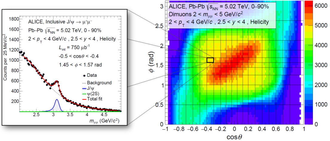
Figure 5.6: Example of signal extraction and corresponding (\cos\theta, \phi) cell on the two-dimensions map populated with dimuons in the mass range 2 < m_{\mu\mu} < 5 GeV/c 2 and for 2 < p_T < 4 GeV/c.
