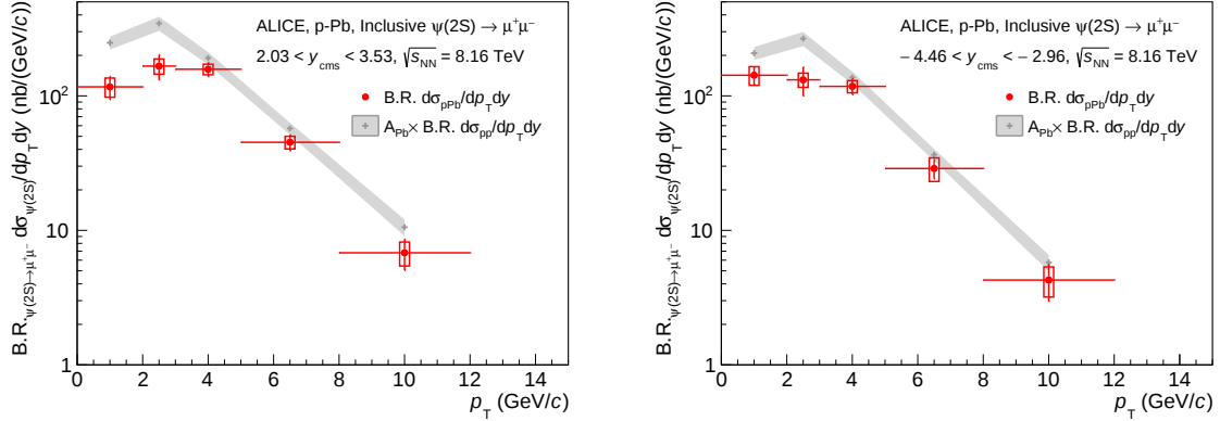
Figure A.13: The differential cross sections B.R._{\psi(2S) \rightarrow \mu^+\mu^-} d^2\sigma^{\psi(2S)}/dp_T dy for p-Pb (left panel) and Pb-p (right panel) collisions at \sqrt{s_{NN}} = 8.16 TeV. The error bars represent the statistical uncertainties, while the boxes correspond to total systematic uncertainties. The grey bands correspond to the reference pp cross section scaled by A_{Pb} .
