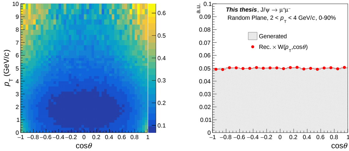
Figure 5.32: Left panel: A \times \varepsilon map as a function of \cos\theta and p_T in the RP reference frame. Right panel: normalized \cos\theta distributions for generated J/ \psi compared with the distribution of reconstructed J/ \psi after the application of the two-dimensions re-weighting.
