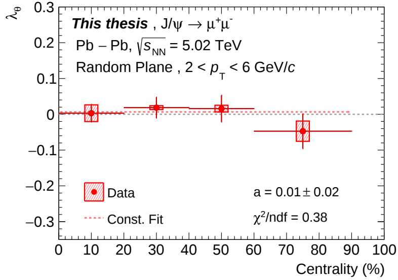
Figure 5.34: \lambda_\theta parameter obtained with dimuon-per-dimuon correction method as a function of centrality in 2 < p_T < 6 GeV/c. The the statistical and systematic uncertainties on signal extraction are shown as a error bar and colored box respectively. The result is then fitted with a constant function.
