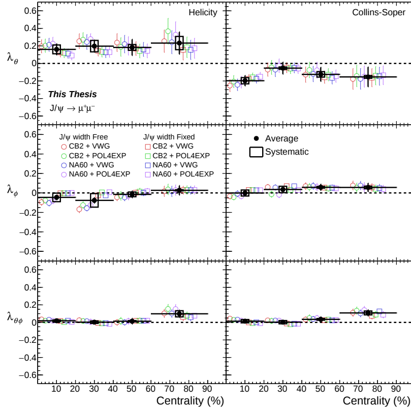
Figure 5.20: Polarization parameters obtained using different signal and background shapes in the raw yield extraction and keeping free/fixed to the Monte Carlo the J/\psi width.
