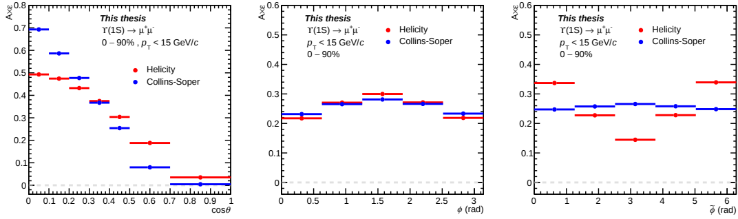
Figure 6.3: A \times \epsilon in the helicity and Collins-Soper reference frame as a function of \cos \theta , \varphi and \tilde{\varphi} for the p_T range 0 < p_T < 15 GeV/ c .
