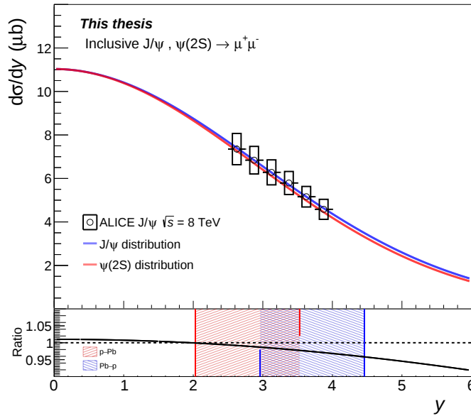
Figure A.11: Top panel: J/\psi and \psi(2S) cross sections as function of the rapidity. Bottom panel: ratio of the J/\psi and \psi(2S) cross sections. The p-Pb and Pb-p rapidity ranges are identified in red and blue respectively.
