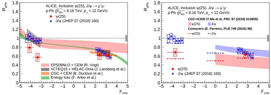
Figure A.20: The y -dependence of R_{pPb} for \psi(2S) and J/\psi [249] in p-Pb collisions at \sqrt{s_{NN}} = 8.16 TeV. The box around R_{pPb} = 1 to correlated systematic uncertainties. The results are compared with models including initial-state effects [121, 117, 118] and coherent energy loss [116, 117] (left panel), and to models which also implement final-state effects [120, 119] (right panel).
