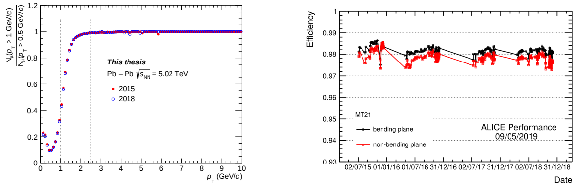
Figure 5.2: Left panel: single muon trigger efficiency as a function of the transverse momentum for 1 GeV/ c threshold. Right panel: efficiency of the RPCs for the muon trigger station MT21 as a function of time in the years 2015 to 2018.
