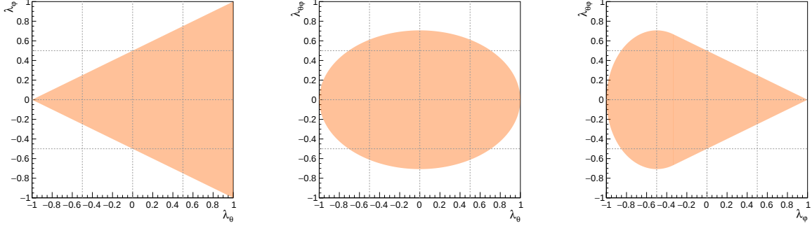
Figure 3.2: Allowed regions for the polarization parameters. Left panel: (\lambda_\theta, \lambda_\varphi) plane. Central panel: (\lambda_\theta, \lambda_{\theta\varphi}) plane. Right panel: (\lambda_\varphi, \lambda_{\theta\varphi}) plane.
