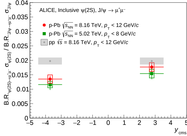
Figure A.14: The ratio B.R._{\psi(2S) \rightarrow \mu^+\mu^-} \sigma^{\psi(2S)} / B.R._{J/\psi \rightarrow \mu^+\mu^-} \sigma^{J/\psi} as a function of y for p-Pb collisions at \sqrt{s_{NN}} = 8.16 and 5.02 TeV [243], compared with the corresponding pp quantity, shown as a grey band and obtained via an interpolation of results at \sqrt{s} = 5, 7, 8 and 13 TeV [92]. The error bars represent the statistical uncertainties, while the boxes correspond to uncorrelated systematic uncertainties.
