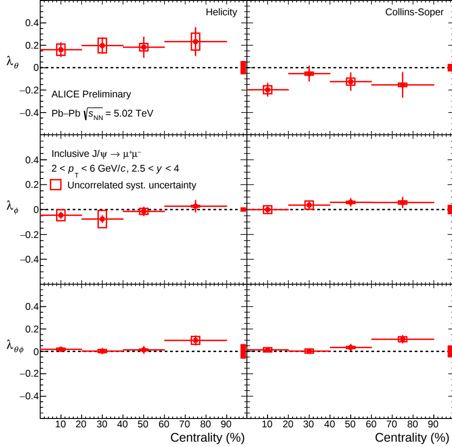
Figure 5.29: Inclusive J/ \psi polarization parameters as a function of centrality for Pb–Pb collisions at \sqrt{s_{\text{NN}}} = 5.02 TeV. The statistical and uncorrelated systematic uncertainties are plotted separately as a vertical bar and a empty box, while the correlated systematic is plotted as red box around zero.
