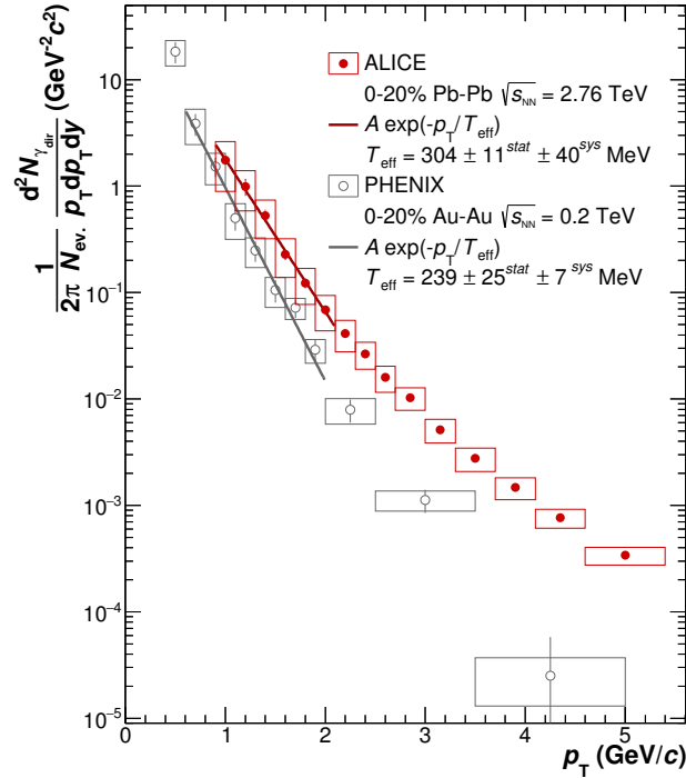
Figure 1.8: Direct photon spectra measured by the ALICE collaboration [27] in Pb–Pb collisions at \sqrt{s_{\text{NN}}} = 2.76 TeV and by the PHENIX collaboration [29] in Au–Au collisions at \sqrt{s_{\text{NN}}} = 200 GeV. Both results are obtained for the 0-20% centrality class and the pQCD contribution is not subtracted.
