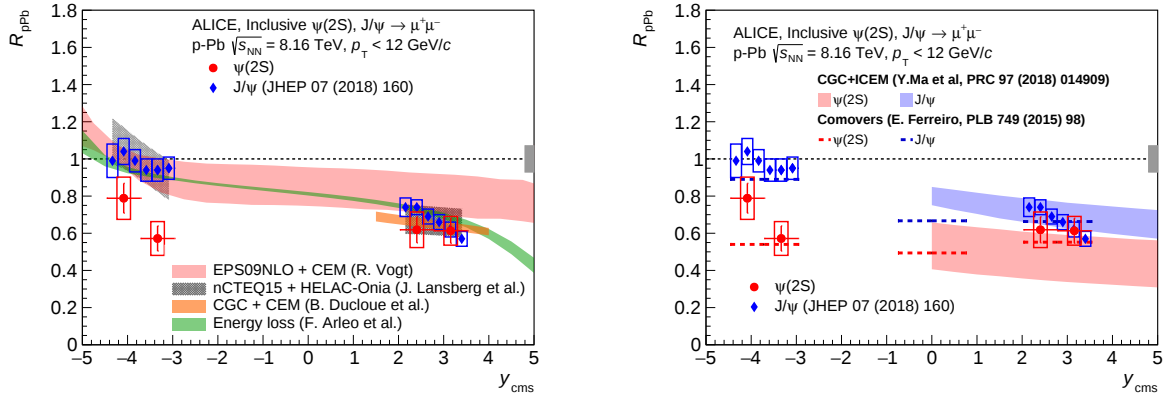
Figure 2.11: Rapidity dependence of the R_{pA} for \psi(2S) and J/\psi in p-Pb collisions at \sqrt{s_{NN}} = 8.16 TeV [2]. Results are compared with models including initial-state effects [121, 117, 118] and coherent energy loss [116, 117] (left panel), and to models which also implement final-state effects [119, 120] (right panel).
