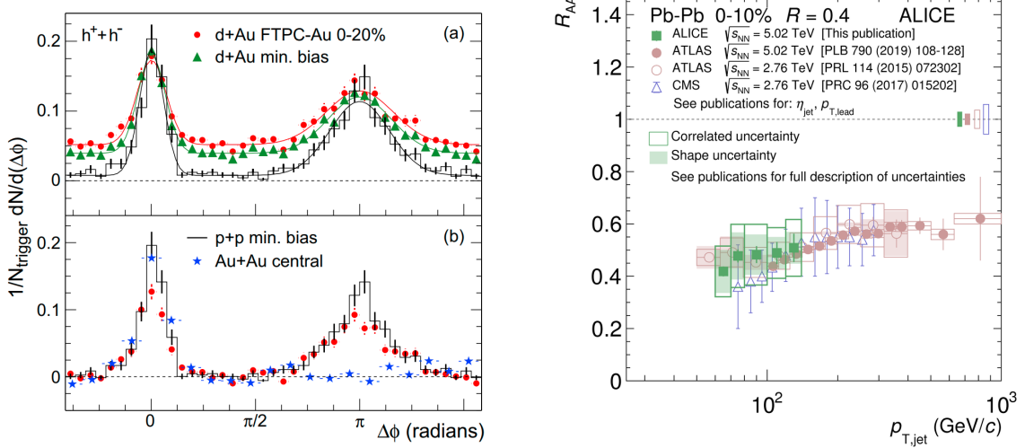
Figure 1.14: Left panel: two-particle azimuthal distributions measured by the STAR collaboration at \sqrt{s_{NN}} = 200 GeV [48] (a) for minimum bias and central d–Au collisions, and for pp collisions; (b) for central d–Au collisions compared with those seen in pp and central Au–Au collisions. Right panel: jet R_{AA} in 0–10% central Pb–Pb collisions for all currently published experimental results [49]. Closed markers denote \sqrt{s_{NN}} = 5.02 TeV and open markers denote \sqrt{s_{NN}} = 2.76 TeV.
