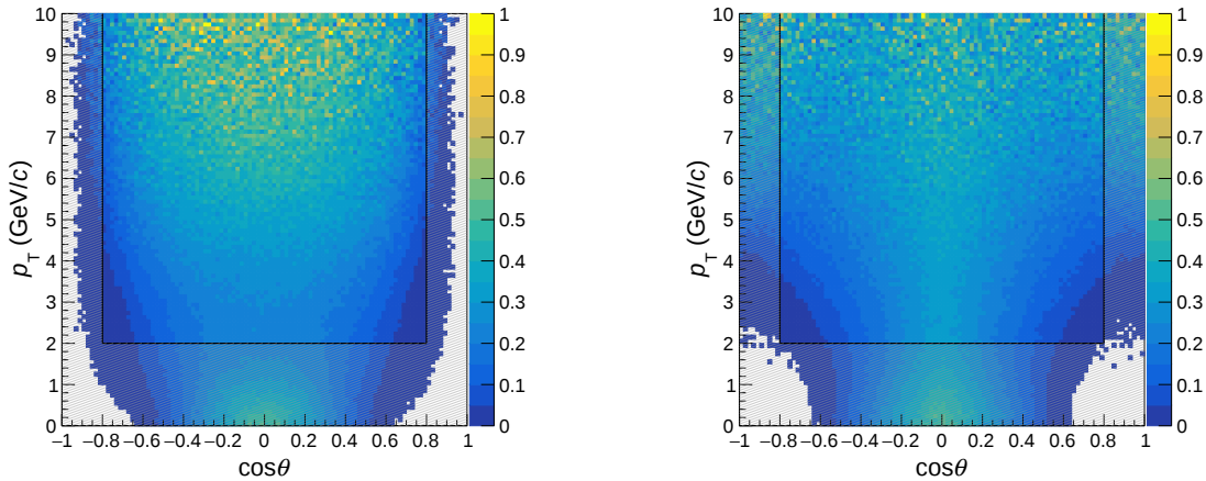
Figure 5.12: A \times \epsilon as a function of \cos\theta and p_T in the helicity (left panel) and Collins-Soper (right panel) reference frames. The fiducial region is indicated with a black rectangle.
