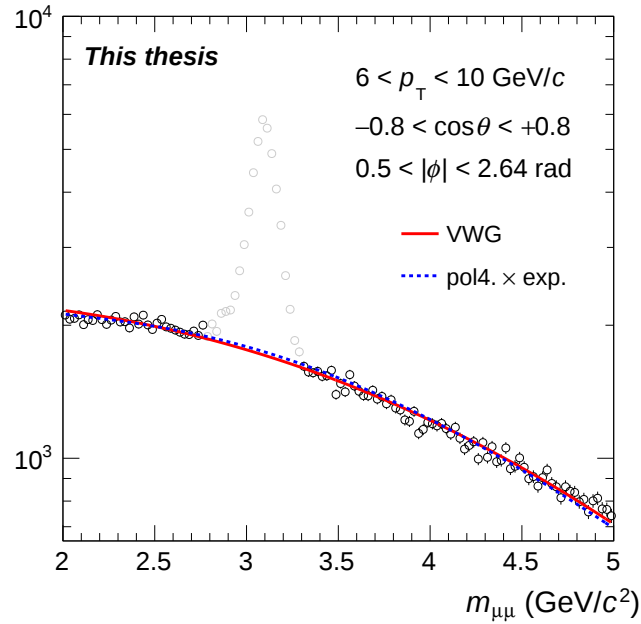
Figure 5.4: Example of fit to the background with a variable width Gaussian (red solid line) and a polynomial times an exponential function (blue dotted line), after having removed the signal peak.
